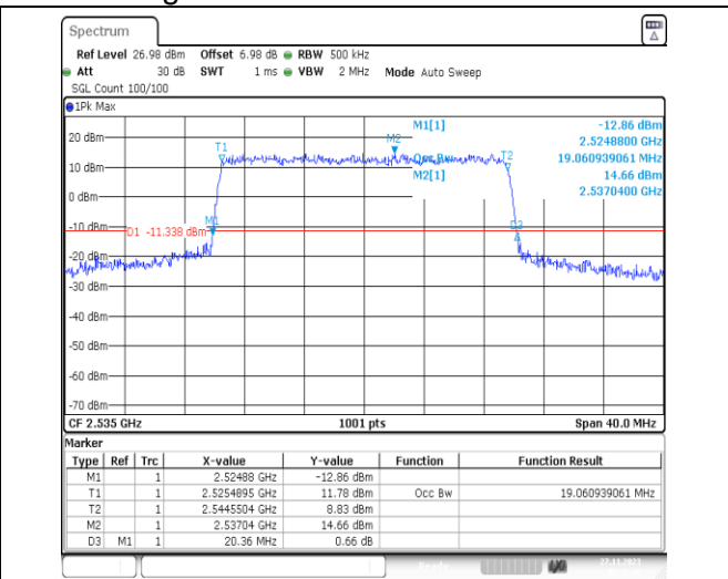
1-N7-PC3-15-20-M-8-CP-64QAM-Outer_Full-106@0 -Ant31-19.061-20.360-≤20-PASS
