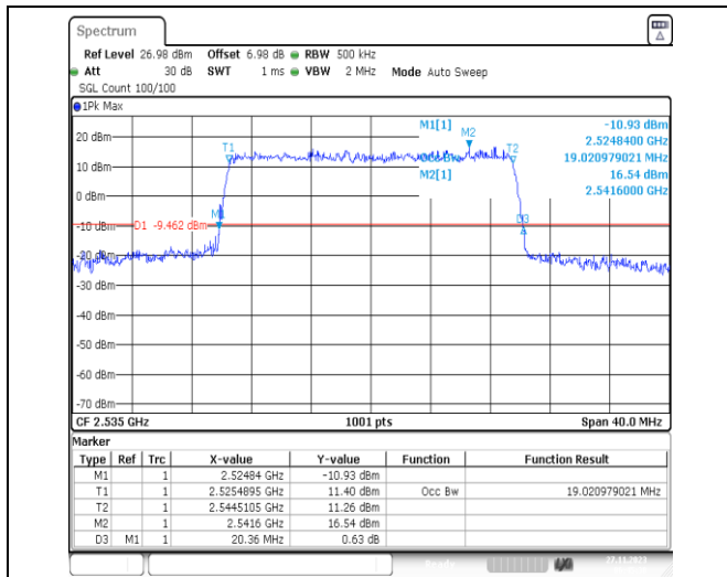
1-N7-PC3-15-20-M-7-CP-16QAM-Outer_Full-106@0 -Ant31-19.021-20.360-≤20-PASS
