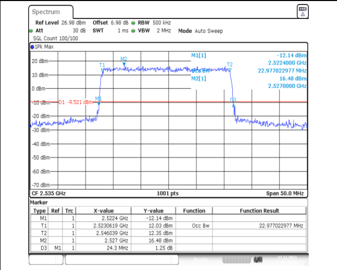
1-N7-PC3-15-25-M-1-DFT-QPSK-Outer_Full-128@0 -Ant31-22.977-24.300-≤25-PASS
