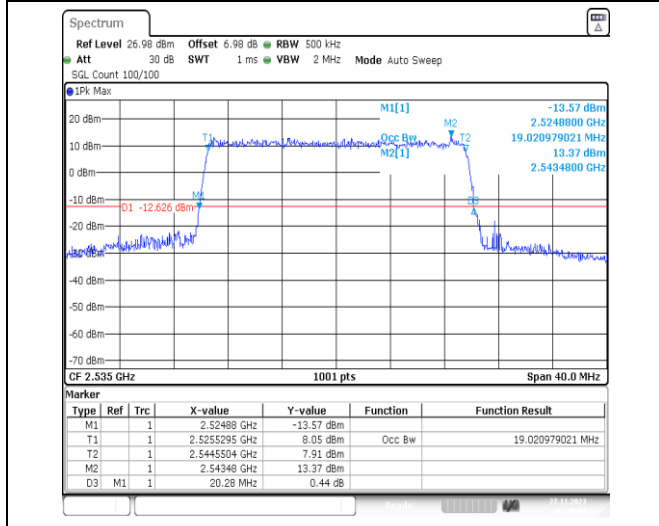
1-N7-PC3-15-20-M-9-CP-256QAM-Outer_Full-106@0 0-Ant31-19.021-20.280-≤20-PASS
