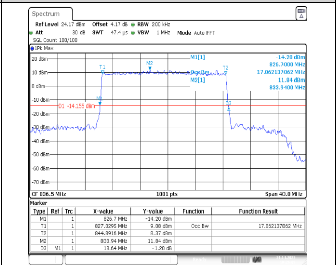
1-N5-PC3-15-20-M-5-DFT-256QAM-Outer_Full-100 @0-Ant41-17.862-18.640-≤20-PASS
