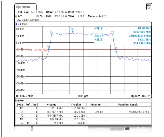
1-N5-PC3-15-10-M-4-DFT-64QAM-Outer_Full-50@0 -Ant41-9.011-9.900-≤10-PASS
