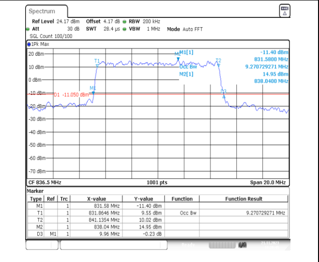
1-N5-PC3-15-10-M-7-CP-16QAM-Outer_Full-52@0- Ant41-9.271-9.960-≤10-PASS
