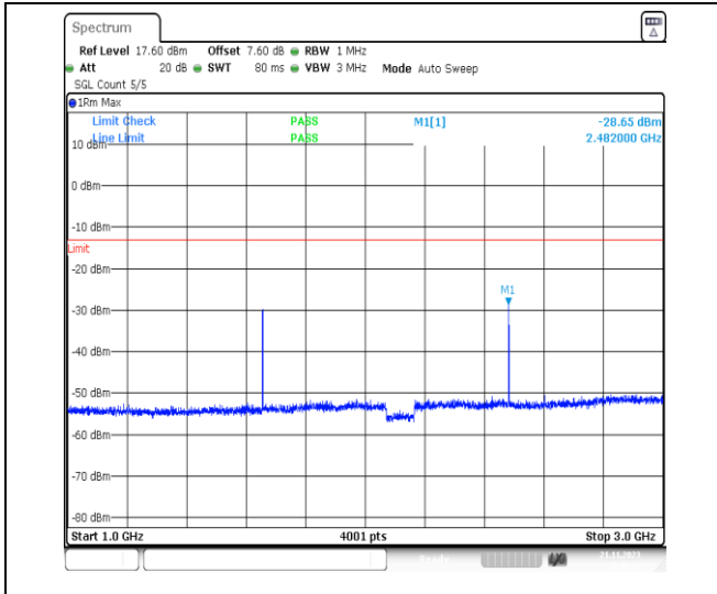
1-N5-PC3-15-20-M-1-DFT-PI2BPSK-Inner_1RB_Lef t-1@1-1000-3000-Ant41-2481.50--28.65--13-PASS
