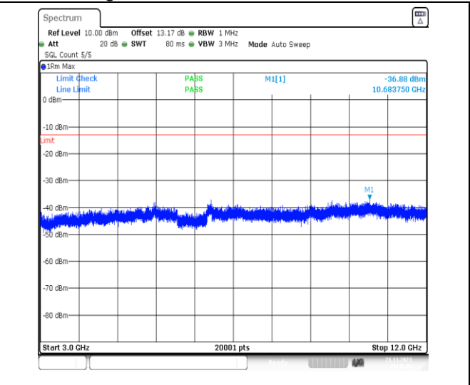
1-N5-PC3-15-20-M-1-DFT-PI2BPSK-Inner_1RB_Left -1@1-3000-12000-Ant41-10694.10--36.88--13-PASS
