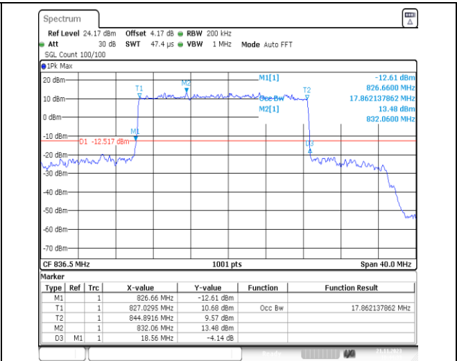
1-N5-PC3-15-20-M-3-DFT-16QAM-Outer_Full-100 @0-Ant41-17.862-18.560-≤20-PASS
