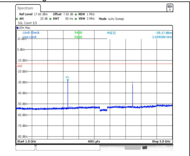
1-N5-PC3-15-20-H-1-DFT-PI2BPSK-Inner_1RB_Left -1 @ 1-1000-3000-Ant41-1659.50--29.17--13-PASS
