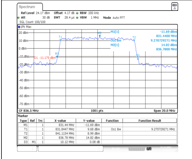
1-N5-PC3-15-10-M-6-CP-QPSK-Outer_Full-52@0-A nt41-9.271-10.120-≤10-PASS
