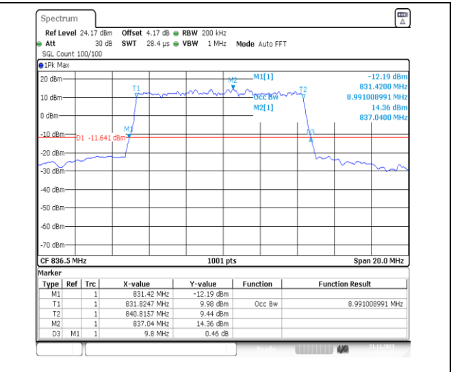
1-N5-PC3-15-10-M-5-DFT-256QAM-Outer_Full-50@0 0-Ant41-8.991-9.800-≤10-PASS
