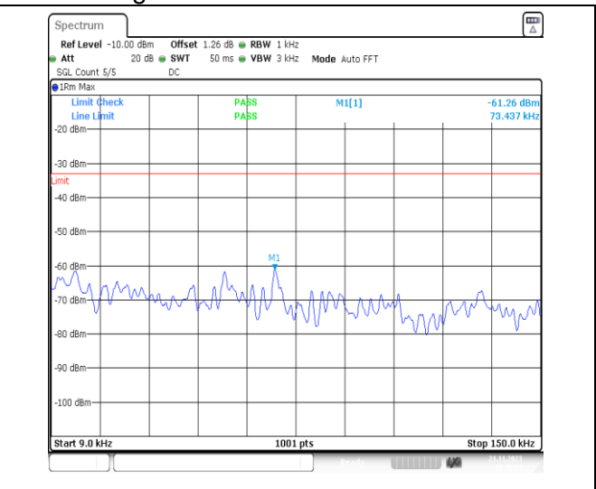
1-N5-PC3-15-20-M-1-DFT-PI2BPSK-Inner_1RB_Left -1 @ 1-0.009-0.15-Ant41-0.02--61.26--33-PASS
