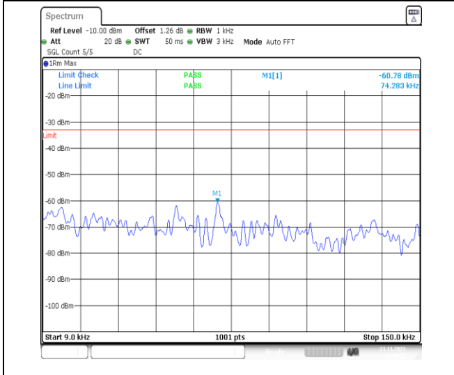
1-N5-PC3-15-20-H-1-DFT-PI2BPSK-Inner_1RB_Left -1@1-0.009-0.15-Ant41-0.01--60.78--33-PASS
