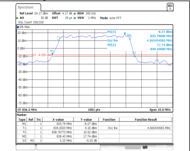
1-N5-PC3-15-5-M-6-CP-QPSK-Outer_Full-25@0-Ant 41-4.565-5.250-≤5-PASS
