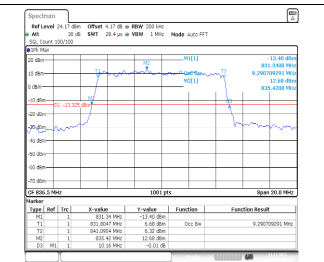
1-N5-PC3-15-10-M-9-CP-256QAM-Outer_Full-52@0 Ant41-9.291-10.160-≤10-PASS
