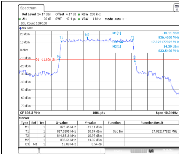
1-N5-PC3-15-20-M-2-DFT-PI2BPSK-Outer_Full-100 @0-Ant41-17.822-18.880-≤20-PASS
