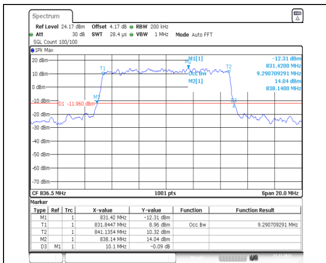
1-N5-PC3-15-10-M-8-CP-64QAM-Outer_Full-52@0 -Ant41-9.291-10.100-≤10-PASS
