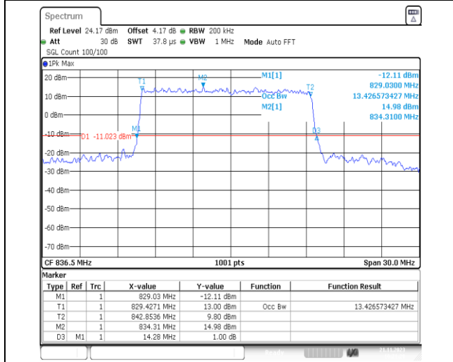
1-N5-PC3-15-15-M-1-DFT-QPSK-Outer_Full-75@0 Ant41-13.427-14.280-≤15-PASS
