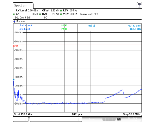
1-N5-PC3-15-20-H-1-DFT-PI2BPSK-Inner_1RB_Left- 1@1-0.15-30-Ant41-0.15--63.30--23-PASS
