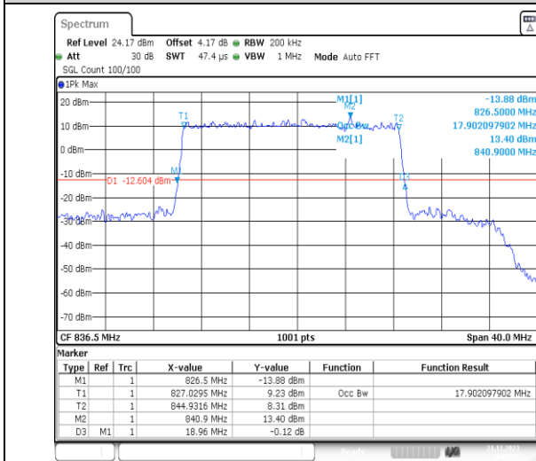
1-N5-PC3-15-20-M-4-DFT-64QAM-Outer_Full-100 @0-Ant41-17.902-18.960-≤20-PASS
