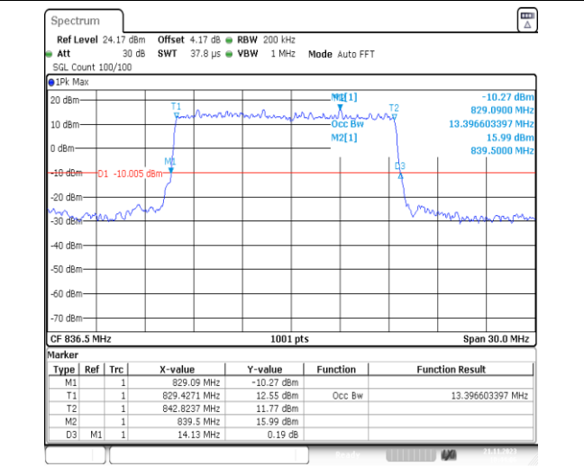
1-N5-PC3-15-15-M-2-DFT-PI2BPSK-Outer_Full-75@0 0-Ant41-13.397-14.130-≤15-PASS
