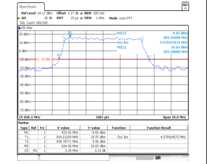
1-N5-PC3-15-5-M-8-CP-64QAM-Outer_Full-25@0-A nt41-4.575-5.290-≤5-PASS
