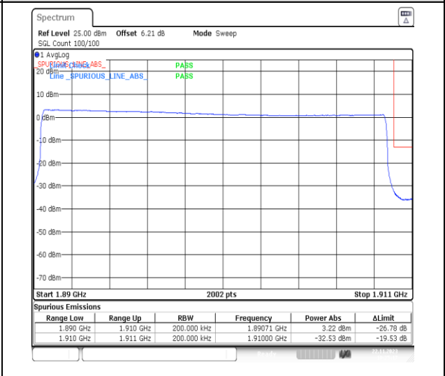
1-N2-PC3-15-20-H-6-CP-QPSK-Outer_Full-106@0-Ant14-1-seegraph-PASS-see graph
