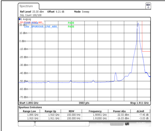
1-N2-PC3-15-15-H-2-DFT-PI2BPSK-Edge_1RB_Right-1@78-Ant14-1-seegraph-PASS-see graph
