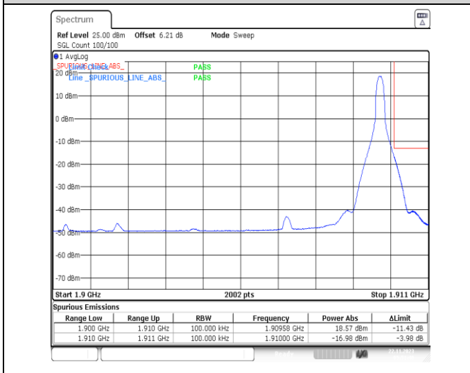
1-N2-PC3-15-10-H-5-CP-QPSK-Edge_1RB_Right-1@51-Ant14-1-seegraph-PASS-see graph
