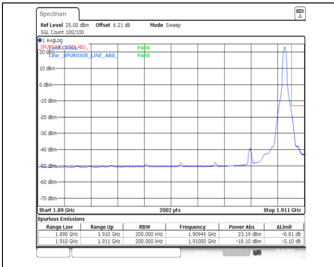
1-N2-PC3-15-20-H-2-DFT-PI2BPSK-Edge_1RB_Right-1@105-Ant14-1-seegraph-PASS-see graph
