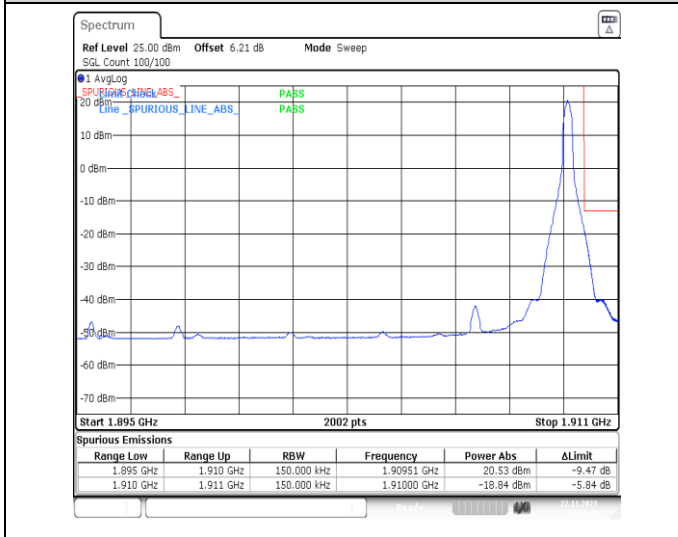
1-N2-PC3-15-15-H-5-CP-QPSK-Edge_1RB_Right-1@78-Ant14-1-seegraph-PASS-see graph
