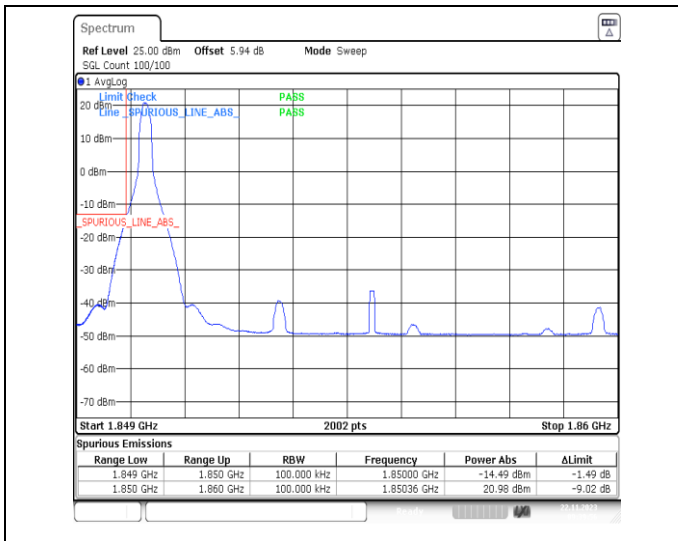
1-N2-PC3-15-10-L-1-DFT-PI2BPSK-Edge_1RB_Left-1 @0-Ant14-1-seegraph-PASS-see graph
