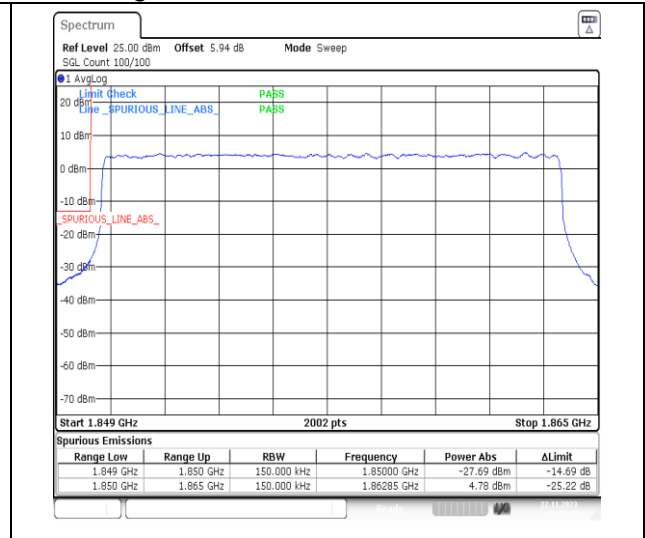
1-N2-PC3-15-15-L-3-DFT-PI2BPSK-Outer_Full-75 @0-Ant14-1-seegraph-PASS-see graph
