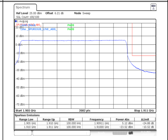
1-N2-PC3-15-5-H-6-CP-QPSK-Outer_Full-25 @0-A nt14-1-seegraph-PASS-see graph
