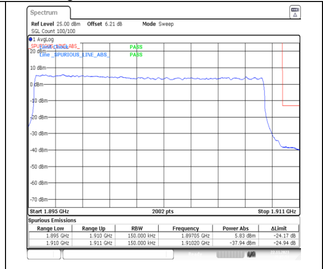
1-N2-PC3-15-15-H-3-DFT-PI2BPSK-Outer_Full-75@0-Ant14-1-seegraph-PASS-see graph
