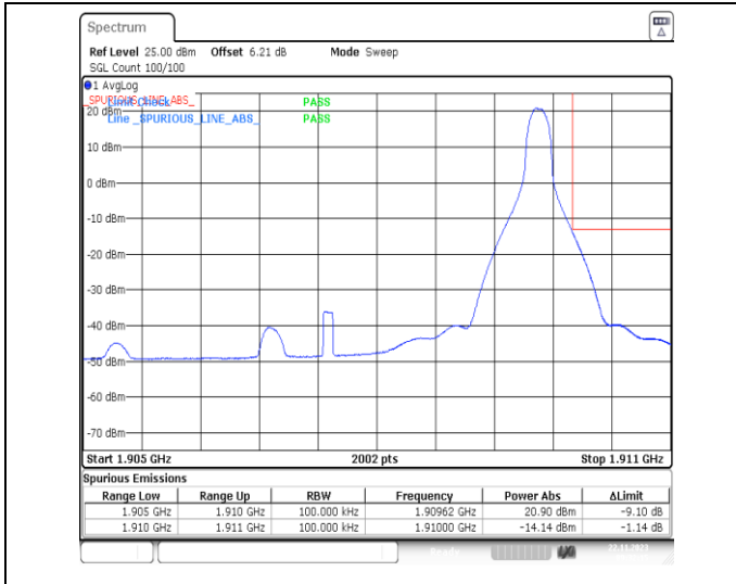
1-N2-PC3-15-5-H-2-DFT-PI2BPSK-Edge_1RB_Right-1 @24-Ant14-1-seegraph-PASS-see graph
