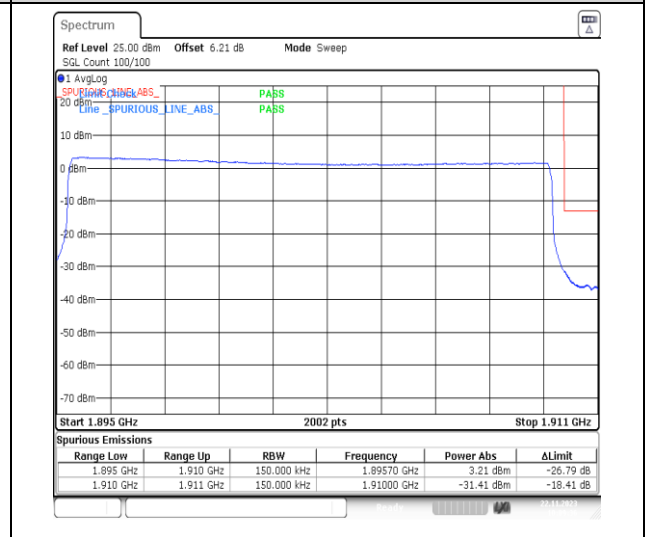
1-N2-PC3-15-15-H-6-CP-QPSK-Outer_Full-79@0-Ant14-1-seegraph-PASS-see graph
