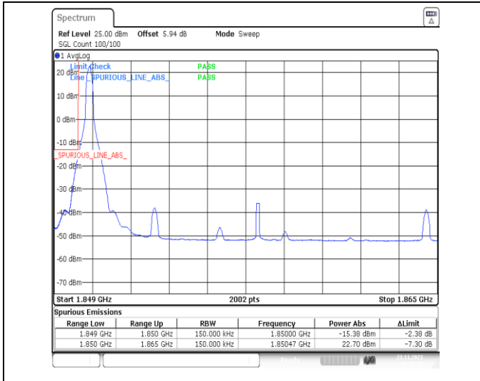
1-N2-PC3-15-15-L-1-DFT-PI2BPSK-Edge_1RB_Left-1 @0-Ant14-1-seegraph-PASS-see graph
