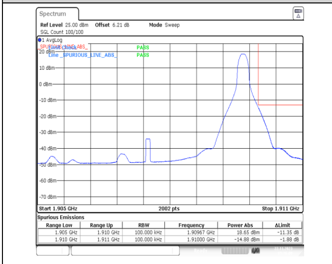
1-N2-PC3-15-5-H-5-CP-QPSK-Edge_1RB_Right-1 @2 4-Ant14-1-seegraph-PASS-see graph
