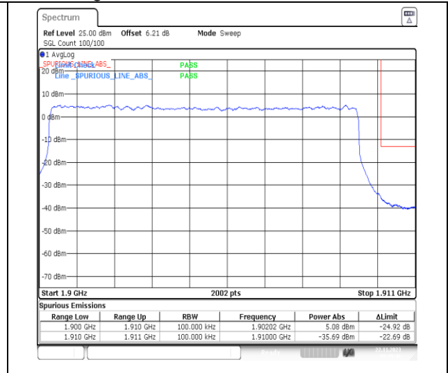
1-N2-PC3-15-10-H-3-DFT-PI2BPSK-Outer_Full-50@0-Ant14-1-seegraph-PASS-see graph
