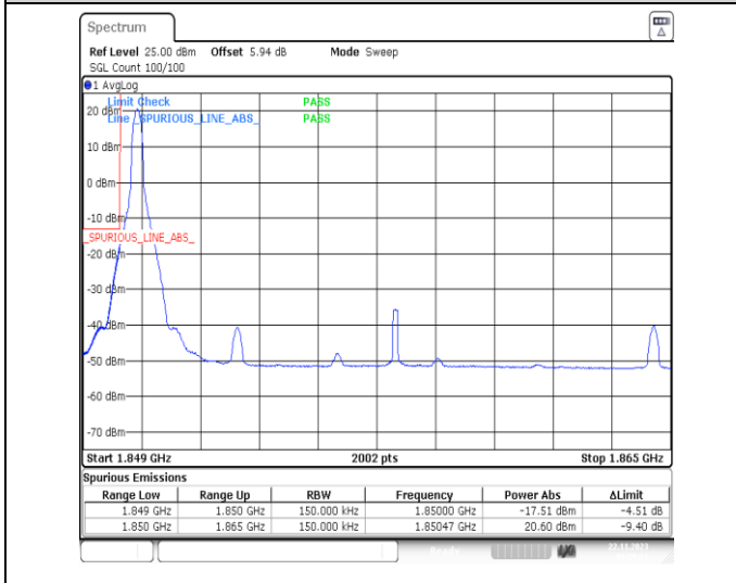
1-N2-PC3-15-15-L-4-CP-QPSK-Edge_1RB_Left-1 @0-Ant14-1-seegraph-PASS-see graph
