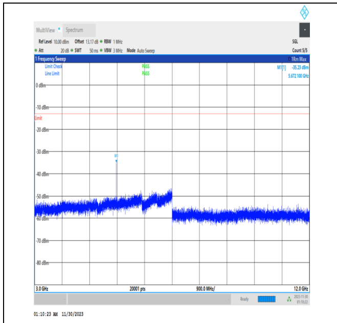
NTNV_N2_PC3_15_20_H_TID1_3000_12000_#1
