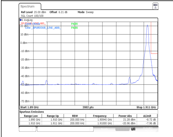
1-N2-PC3-15-20-H-5-CP-QPSK-Edge_1RB_Right-1@105-Ant14-1-seegraph-PASS-see graph
