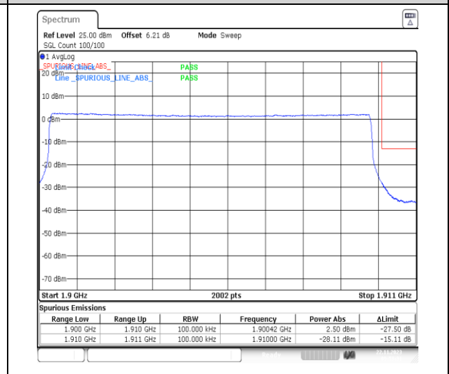
1-N2-PC3-15-10-H-6-CP-QPSK-Outer_Full-52@0-Ant14-1-seegraph-PASS-see graph
