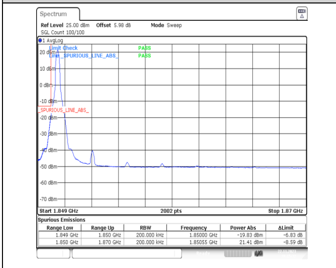
1-N2-PC3-15-20-L-4-CP-QPSK-Edge_1RB_Left-1 @0-Ant14-1-seegraph-PASS-see graph
