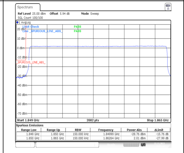
1-N2-PC3-15-15-L-6-CP-QPSK-Outer_Full-79 @0-Ant14-1-seegraph-PASS-see graph
