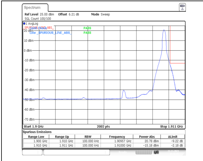
1-N2-PC3-15-10-H-2-DFT-PI2BPSK-Edge_1RB_Right-1@51-Ant14-1-seegraph-PASS-see graph
