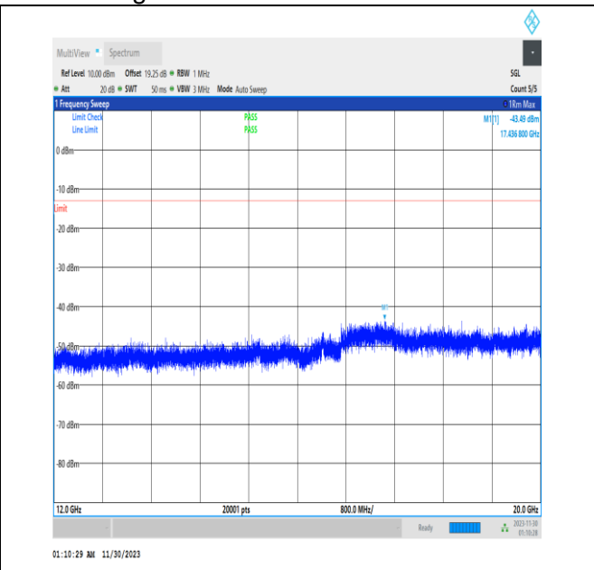
NTNV_N2_PC3_15_20_H_TID1_12000_20000_#1
