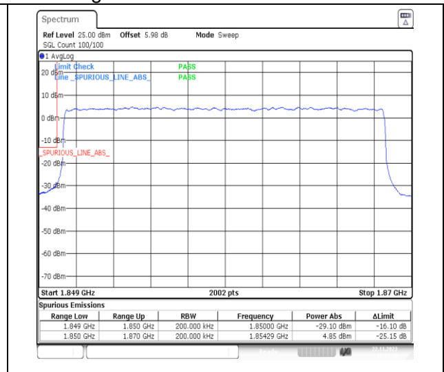
1-N2-PC3-15-20-L-3-DFT-PI2BPSK-Outer_Full-10 @0-Ant14-1-seegraph-PASS-see graph
