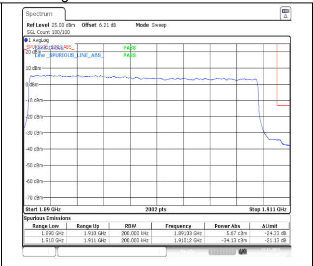
1-N2-PC3-15-20-H-3-DFT-PI2BPSK-Outer_Full-10@0-Ant14-1-seegraph-PASS-see graph
