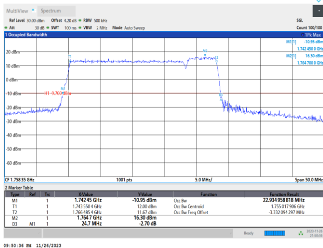
66-66-5MHz-20MHz-QPSK-QPSK-132330-132447-25RB#0-100RB#0
