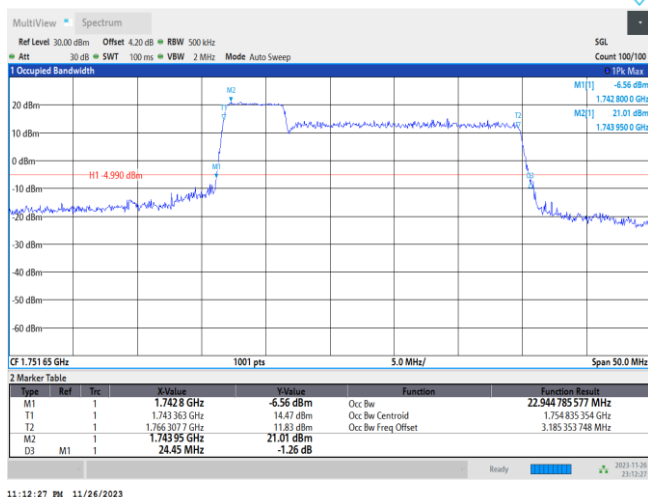
66-66-5MHz-20MHz-16QAM-16QAM-132330-132447-25RB#0-100RB#0
