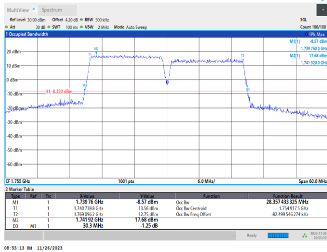
66-66-15MHz-15MHz-256QAM-256QAM-132347-132497-75RB#0-75RB#0
