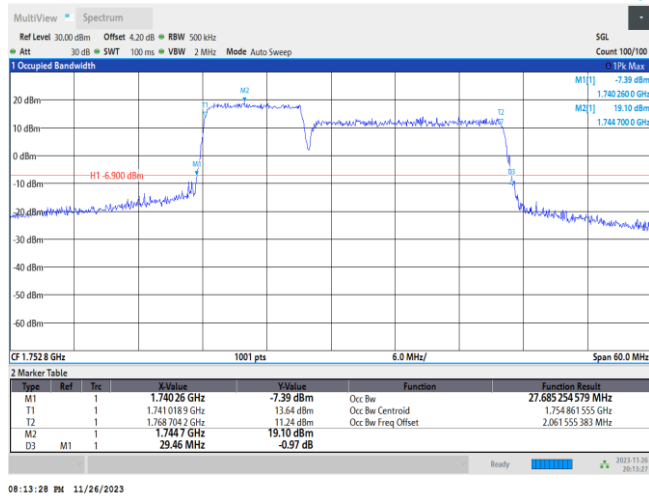
66-66-10MHz-20MHz-64QAM-64QAM-132328-132472-50RB#0-100RB#0
