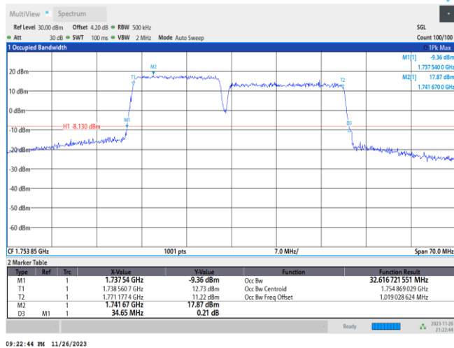
66-66-15MHz-20MHz-16QAM-16QAM-132325-132496-75RB#0-100RB#0
