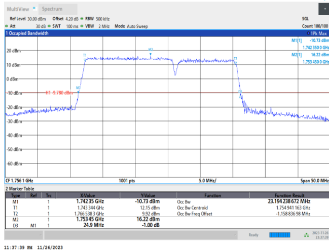
66-66-15MHz-15MHz-QPSK-QPSK-132347-132497-75RB#0-75RB#0
