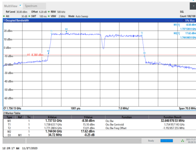
66-66-20MHz-15MHz-16QAM-16QAM-132348-132519-100RB#0-75RB#0
