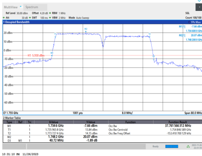
66-66-20MHz-20MHz-16QAM-16QAM-132323-132521-100RB#0-100RB#0
