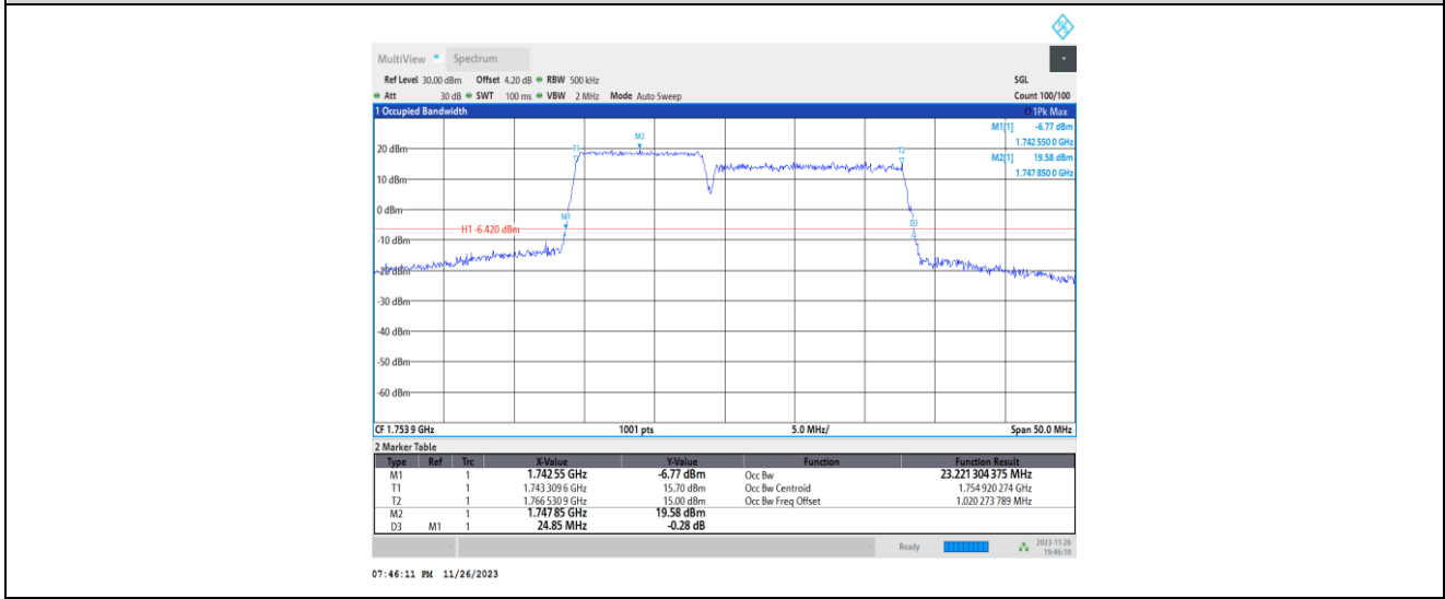
66-66-10MHz-15MHz-16QAM-16QAM-132351-132471-50RB#0-75RB#0
