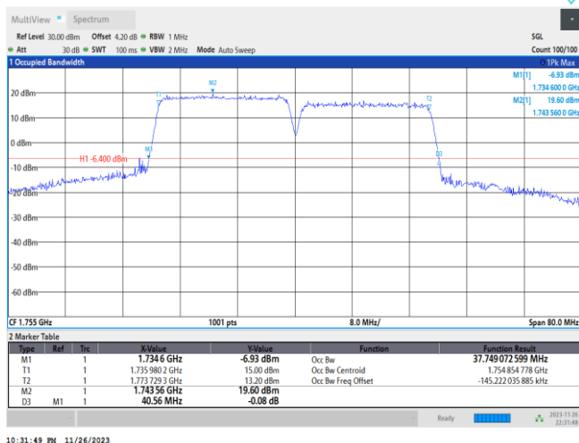
66-66-20MHz-20MHz-64QAM-64QAM-132323-132521-100RB#0-100RB#0
