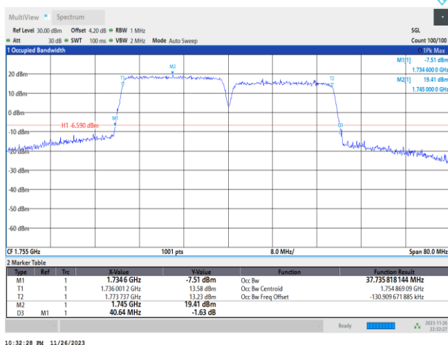
66-66-20MHz-20MHz-256QAM-256QAM-132323-132521-100RB#0-100RB#0
