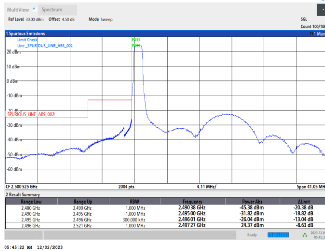
41-41-10MHz-15MHz-QPSK-QPSK-39703-39823-50RB#0-75RB#0
