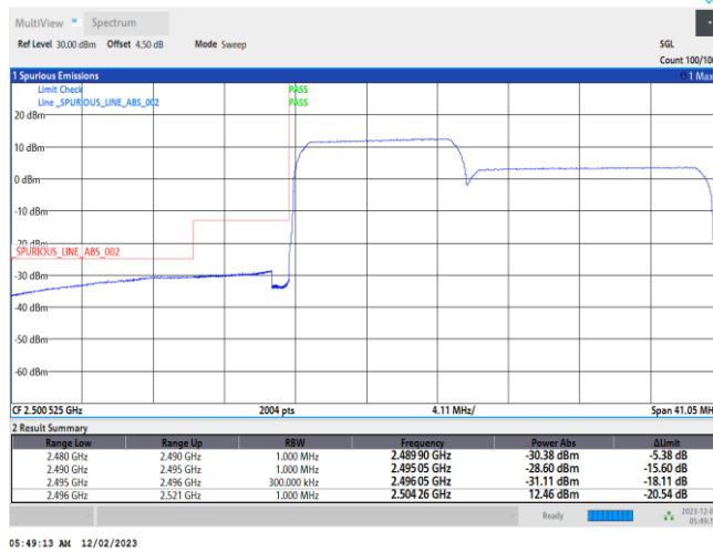
41-41-10MHz-15MHz-QPSK-QPSK-39703-39823-50RB#0-75RB#0
