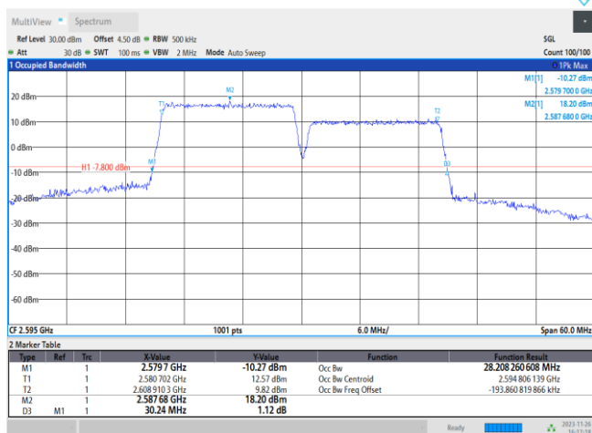
38-38-15MHz-15MHz-16QAM-16QAM-37925-38075-75RB#0-75RB#0
