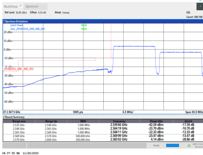
38-38-15MHz-15MHz-QPSK-QPSK-37825-37975-75RB#0-75RB#0
