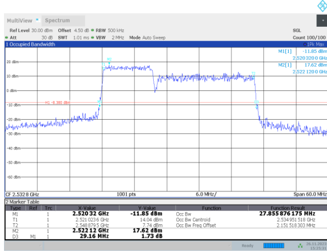
7-7-10MHz-20MHz-QPSK-QPSK-21006-21150-50RB#0-100RB#0
