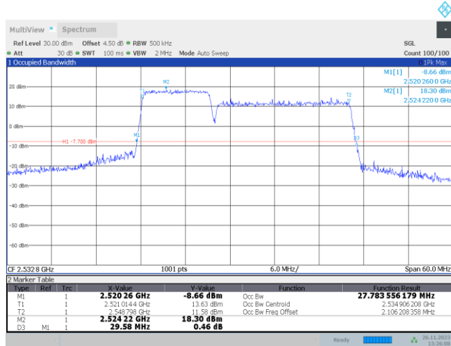
7-7-10MHz-20MHz-16QAM-16QAM-21006-21150-50RB#0-100RB#0
