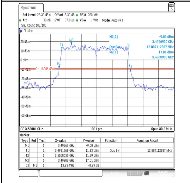
NTNV_N78-3450-3550_PC2_30_15_M_TID2_Ant13#1
