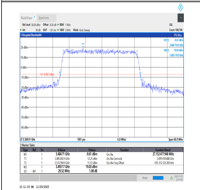
NTNV_N78-3450-3550_PC2_30_30_M_TID4_Ant13#1
