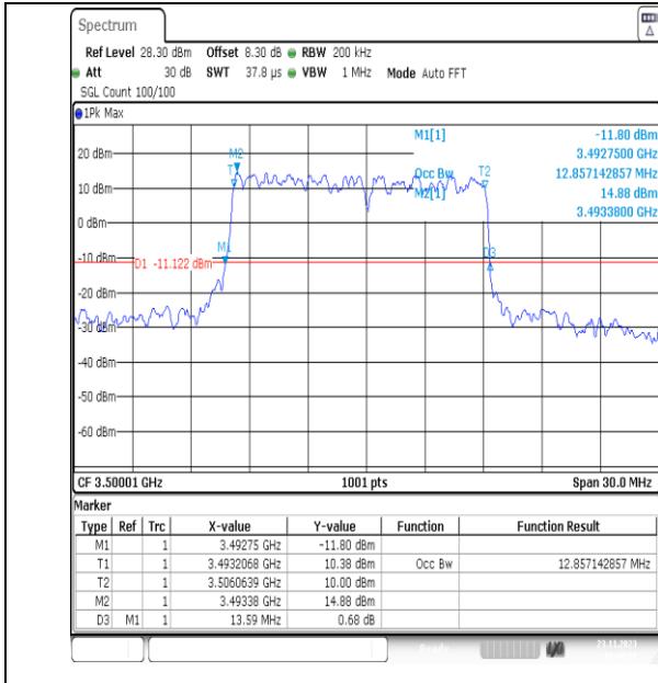
NTNV_N78-3450-3550_PC2_30_15_M_TID4_Ant13#1
