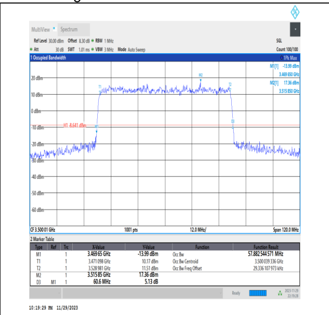
NTNV_N78-3450-3550_PC2_30_60_M_TID4_Ant13#1
