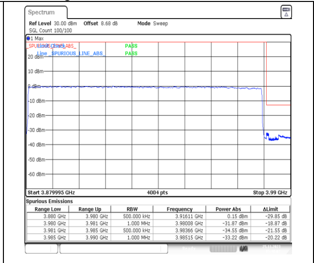
1-N77-3700-3980-PC3-30-100-H-3-DFT-PI2BPSK-Outer_Full-270@0-Ant13-1--PASS-see graph
