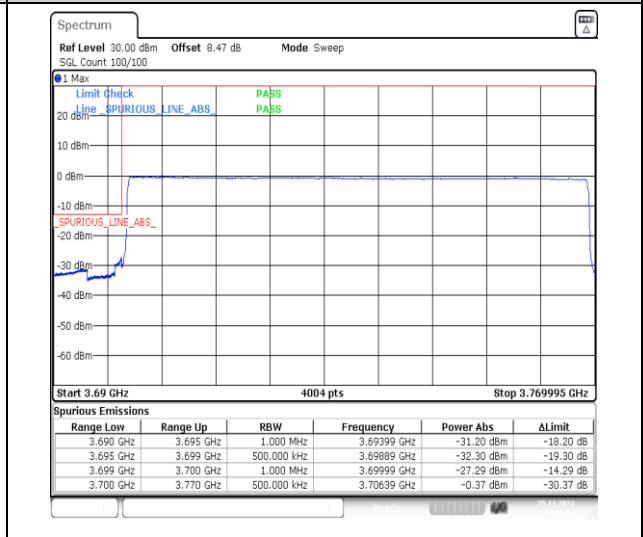
1-N77-3700-3980-PC3-30-70-L-6-CP-QPSK-Outer_Full-189@0-Ant13-1--PASS-see graph
