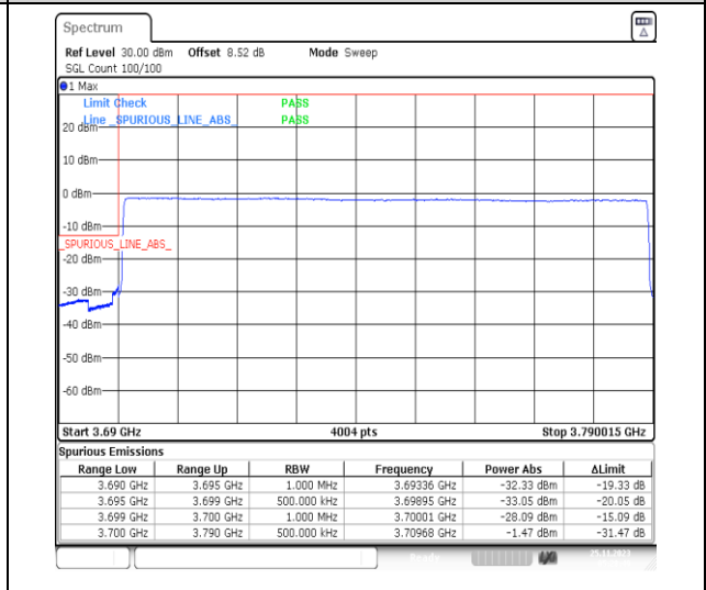
1-N77-3700-3980-PC3-30-90-L-6-CP-QPSK-Outer_Full-245@0-Ant13-1--PASS-see graph
