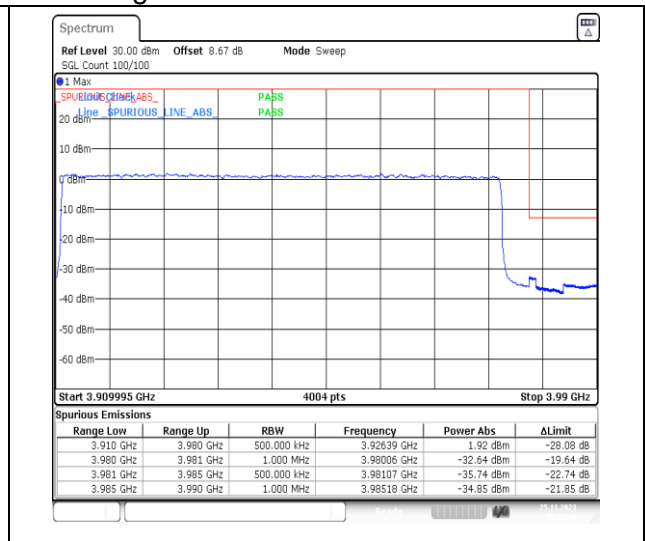
1-N77-3700-3980-PC3-30-70-H-3-DFT-PI2BPSK-Outer_Full-180@0-Ant13-1--PASS-see graph
