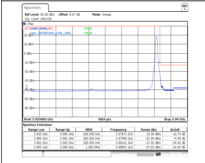
1-N77-3700-3980-PC3-30-50-H-5-CP-QPSK-Edge_1RB_Right-1@132-Ant13-1--PASS-see graph
