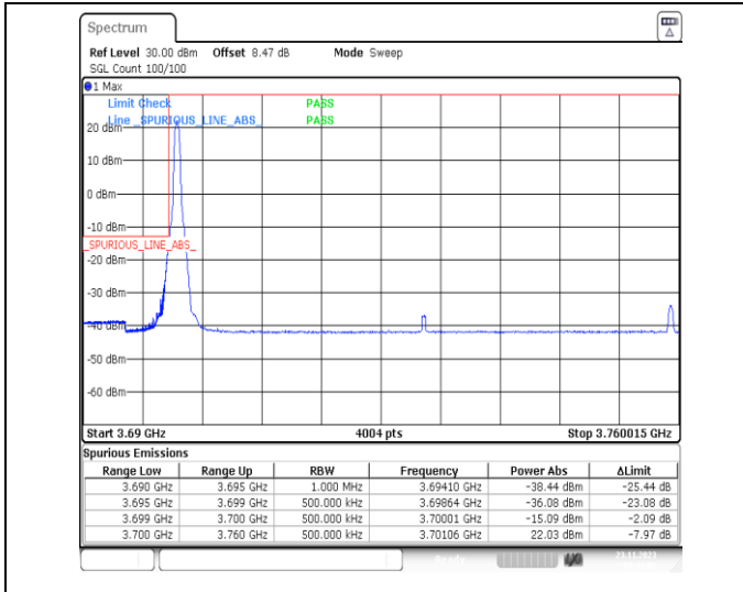
1-N77-3700-3980-PC3-30-60-L-1-DFT-PI2BPSK-Edge_1RB_Left-1@0-Ant13-1--PASS-see graph
