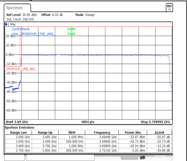
1-N77-3700-3980-PC3-30-100-L-3-DFT-PI2BPSK-Outer_Full-270@0-Ant13-1--PASS-see graph
