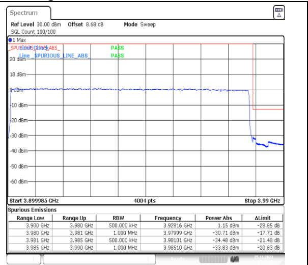
1-N77-3700-3980-PC3-30-80-H-3-DFT-PI2BPSK-Outer_Full-216@0-Ant13-1--PASS-see graph
