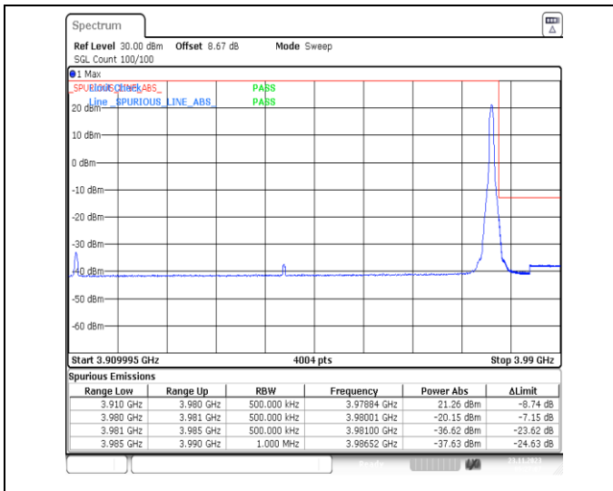
1-N77-3700-3980-PC3-30-70-H-2-DFT-PI2BPSK-Edge_1RB_Right-1@188-Ant13-1--PASS-see graph
