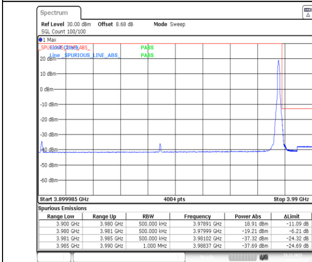
1-N77-3700-3980-PC3-30-80-H-2-DFT-PI2BPSK-Edge_1RB_Right-1@216-Ant13-1--PASS-see graph
