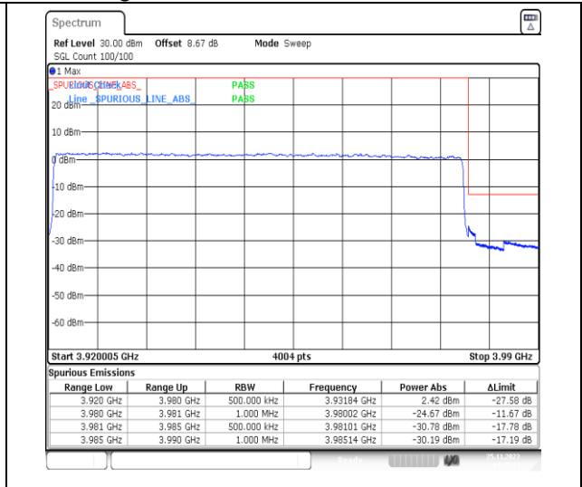
1-N77-3700-3980-PC3-30-60-H-3-DFT-PI2BPSK-Outer_Full-162@0-Ant13-1--PASS-see graph
