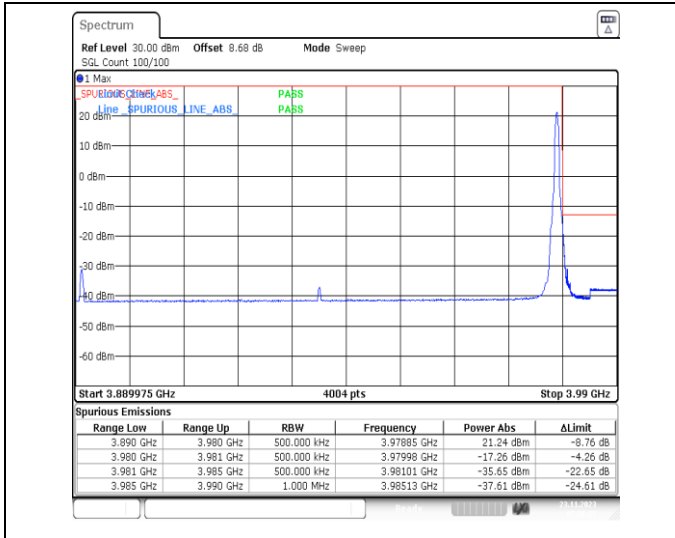
1-N77-3700-3980-PC3-30-90-H-2-DFT-PI2BPSK-Edge_1RB_Right-1@244-Ant13-1--PASS-see graph
