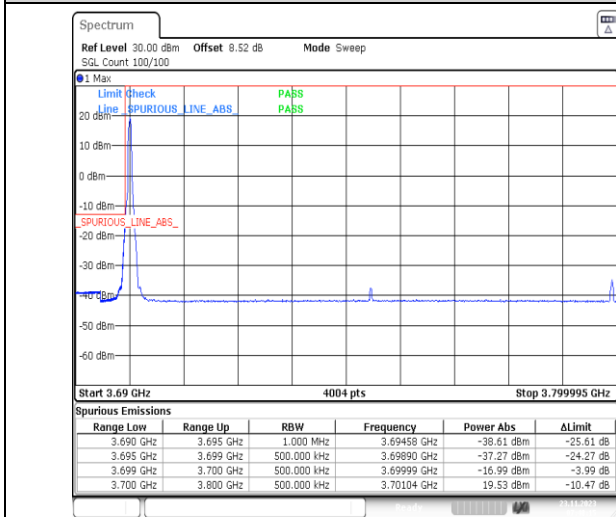
1-N77-3700-3980-PC3-30-100-L-1-DFT-PI2BPSK-Edge_1_RB_Left-1@0-Ant13-1--PASS-see graph
