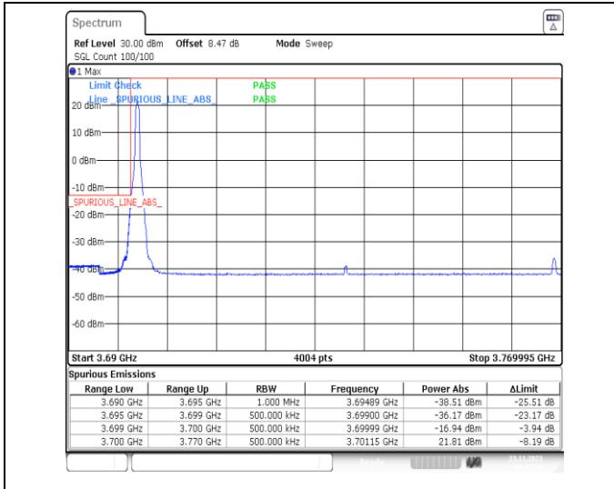
1-N77-3700-3980-PC3-30-70-L-1-DFT-PI2BPSK-Edge_1RB_Left-1@0-Ant13-1--PASS-see graph
