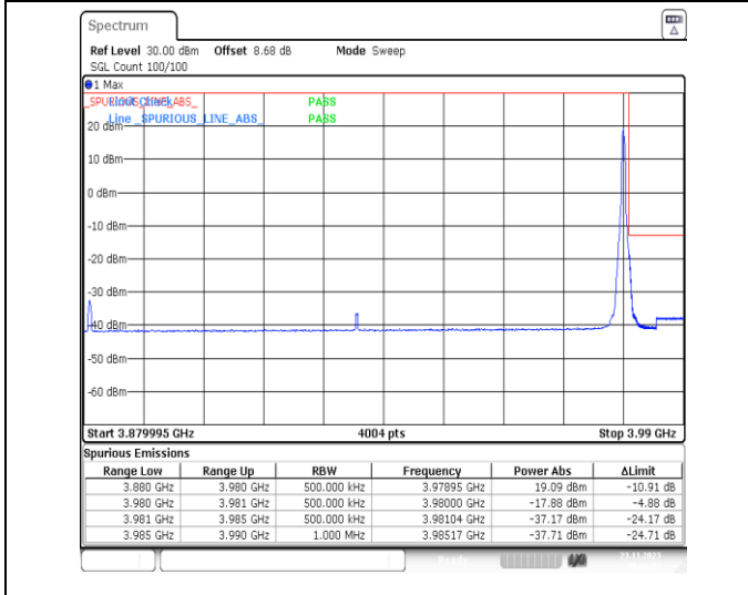
1-N77-3700-3980-PC3-30-100-H-5-CP-QPSK-Edge_1RB_Right-1@272-Ant13-1--PASS-see graph
