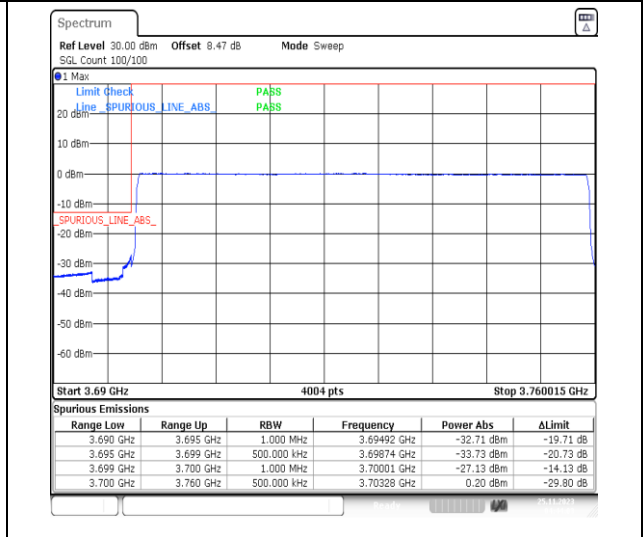
1-N77-3700-3980-PC3-30-60-L-6-CP-QPSK-Outer_Full-162@0-Ant13-1--PASS-see graph
