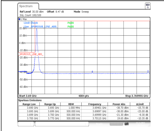
1-N77-3700-3980-PC3-30-70-L-4-CP-QPSK-Edge_1RB_Left-1@0-Ant13-1--PASS-see graph
