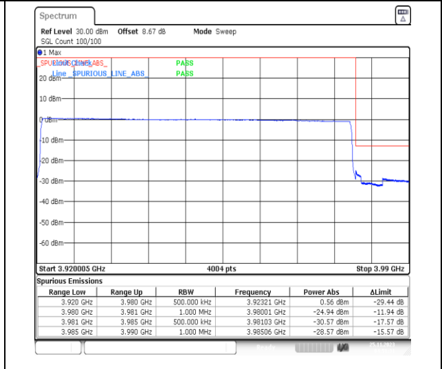
1-N77-3700-3980-PC3-30-60-H-6-CP-QPSK-Outer_Full-162@0-Ant13-1--PASS-see graph
