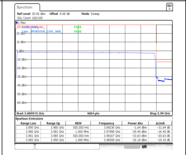
1-N77-3700-3980-PC3-30-90-H-6-CP-QPSK-Outer_Full-245@0-Ant13-1--PASS-see graph
