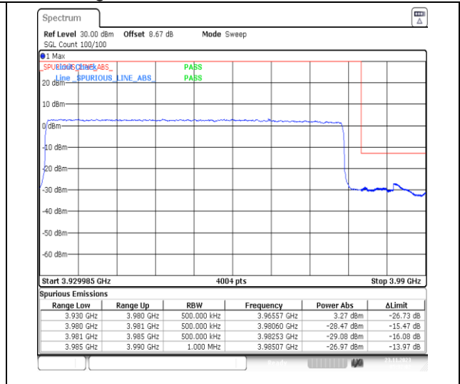
1-N77-3700-3980-PC3-30-50-H-3-DFT-PI2BPSK-Outer_Full-128@0-Ant13-1--PASS-see graph
