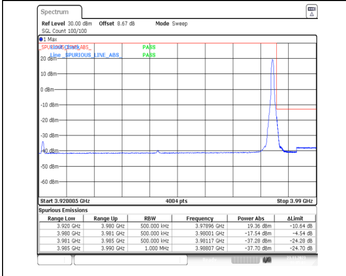
1-N77-3700-3980-PC3-30-60-H-5-CP-QPSK-Edge_1RB_Right-1@161-Ant13-1--PASS-see graph
