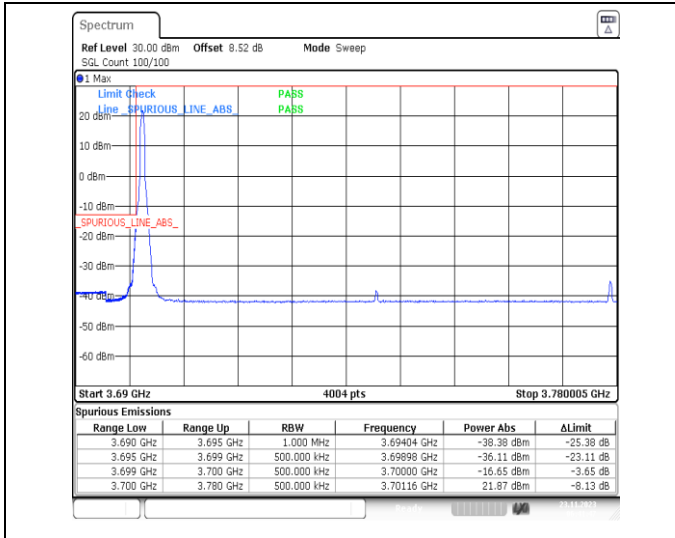
1-N77-3700-3980-PC3-30-80-L-1-DFT-PI2BPSK-Edge_1RB_Left-1@0-Ant13-1--PASS-see graph
