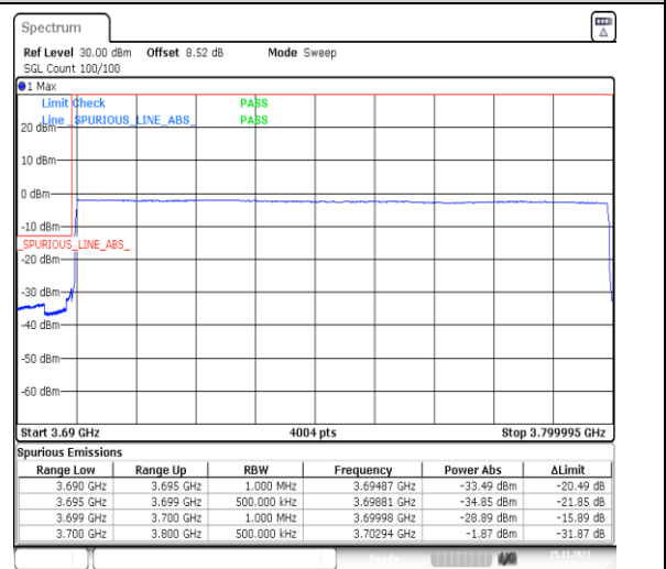
1-N77-3700-3980-PC3-30-100-L-3-DFT-PI2BPSK-Outer_Full-270@0-Ant13-1--PASS-see graph
