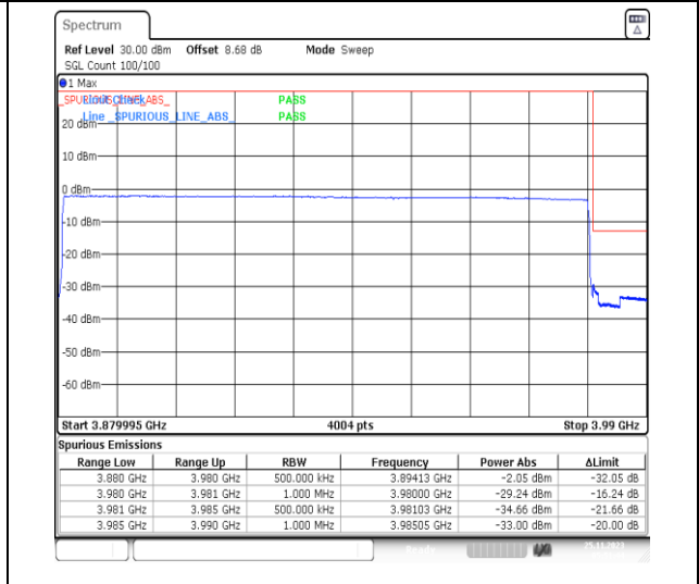
1-N77-3700-3980-PC3-30-100-H-6-CP-QPSK-Outer_Full-273@0-Ant13-1--PASS-see graph
