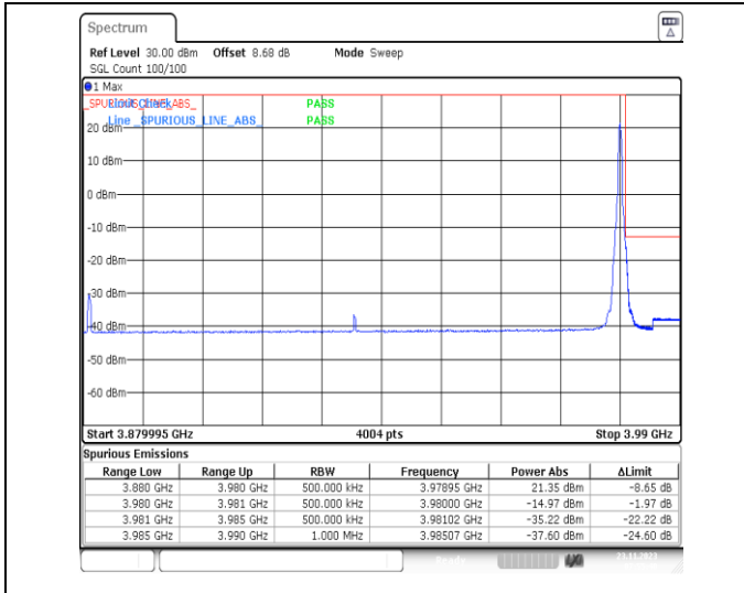
1-N77-3700-3980-PC3-30-100-H-2-DFT-PI2BPSK-Edge_1RB_Right-1@272-Ant13-1--PASS-see graph
