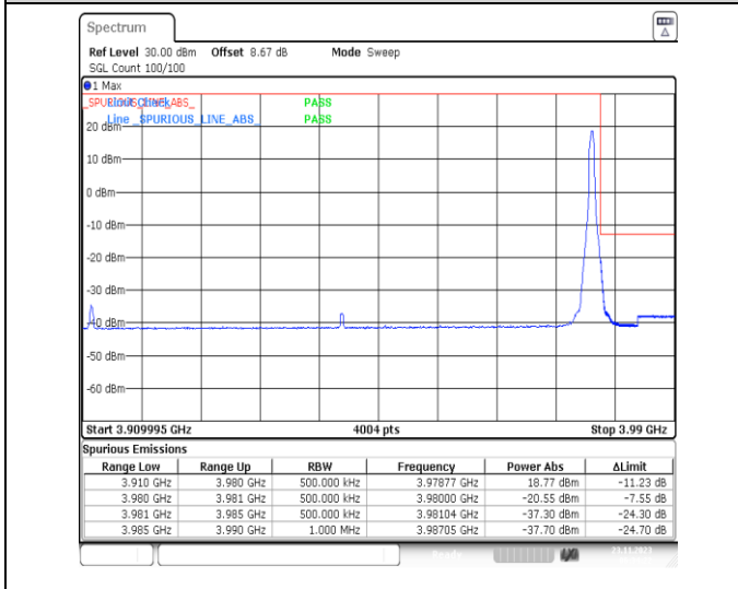
1-N77-3700-3980-PC3-30-70-H-5-CP-QPSK-Edge_1RB_Right-1@188-Ant13-1--PASS-see graph
