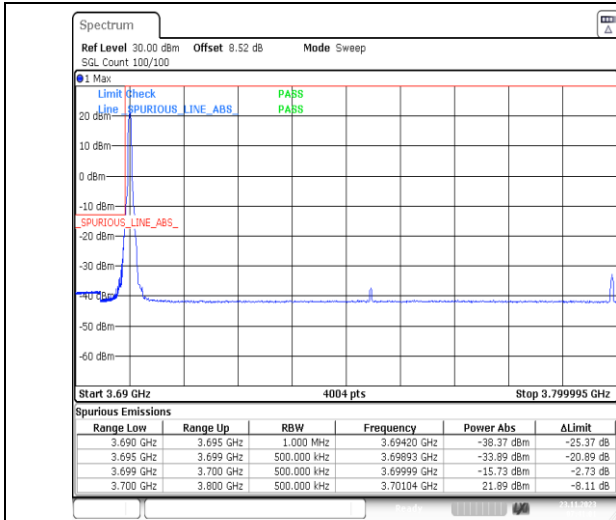
1-N77-3700-3980-PC3-30-100-L-1-DFT-PI2BPSK-Edge_1_RB_Left-1@0-Ant13-1--PASS-see graph
