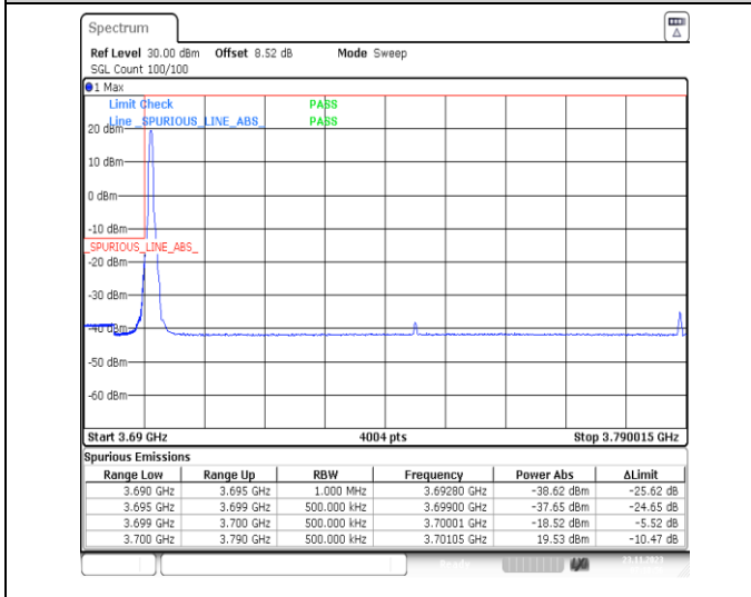
1-N77-3700-3980-PC3-30-90-L-4-CP-QPSK-Edge_1RB_Left-1@0-Ant13-1--PASS-see graph
