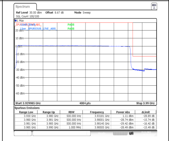
1-N77-3700-3980-PC3-30-50-H-6-CP-QPSK-Outer_Full-133@0-Ant13-1--PASS-see graph
