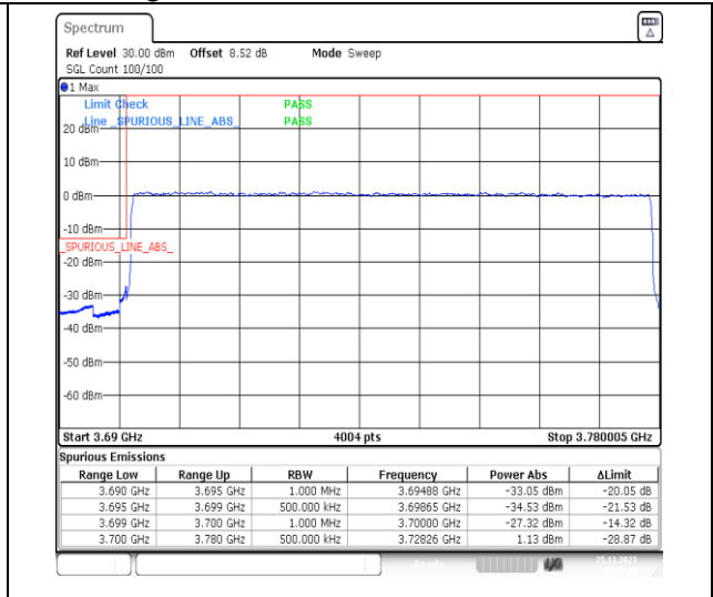
1-N77-3700-3980-PC3-30-80-L-3-DFT-PI2BPSK-Outer_Full-216@0-Ant13-1--PASS-see graph
