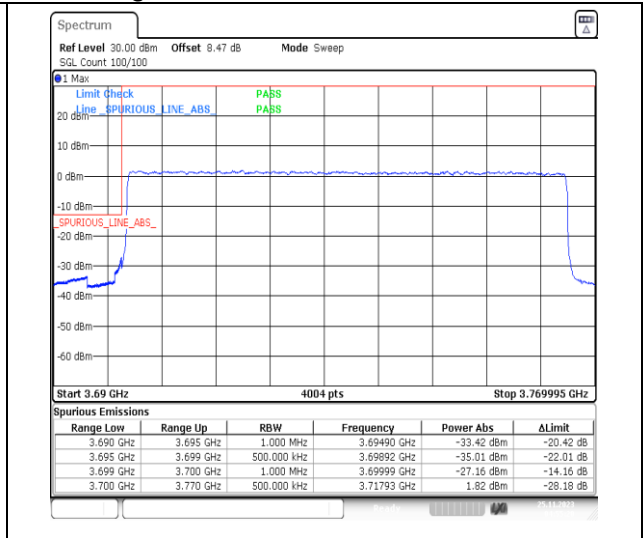
1-N77-3700-3980-PC3-30-70-L-3-DFT-PI2BPSK-Outer_Full-180@0-Ant13-1--PASS-see graph
