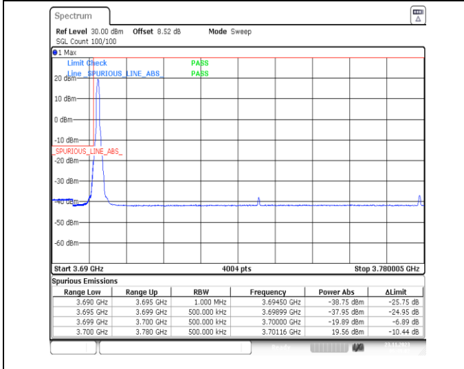
1-N77-3700-3980-PC3-30-80-L-4-CP-QPSK-Edge_1RB_Left-1@0-Ant13-1--PASS-see graph
