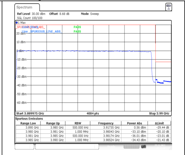
1-N77-3700-3980-PC3-30-90-H-3-DFT-PI2BPSK-Outer_Full-240@0-Ant13-1--PASS-see graph
