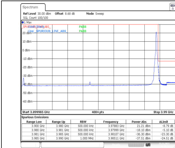
1-N77-3700-3980-PC3-30-80-H-2-DFT-PI2BPSK-Edge_1RB_Right-1@216-Ant13-1--PASS-see graph
