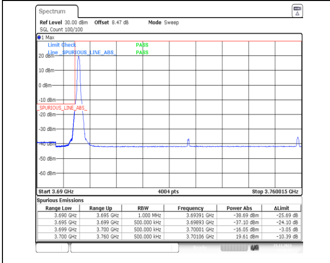
1-N77-3700-3980-PC3-30-60-L-4-CP-QPSK-Edge_1RB_Left-1@0-Ant13-1--PASS-see graph
