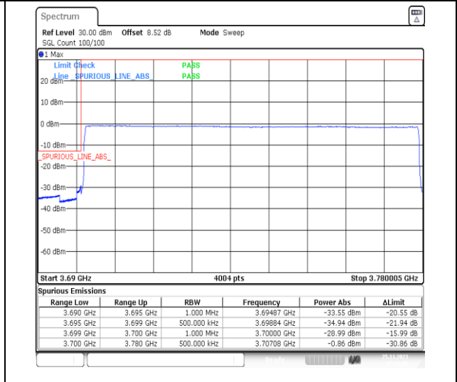
1-N77-3700-3980-PC3-30-80-L-6-CP-QPSK-Outer_Full-217@0-Ant13-1--PASS-see graph
