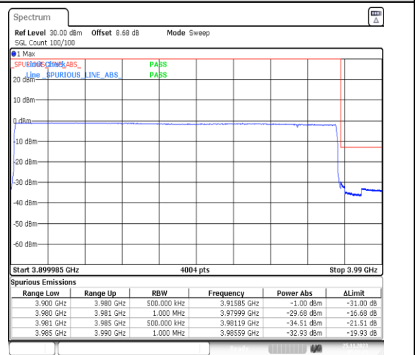
1-N77-3700-3980-PC3-30-80-H-3-DFT-PI2BPSK-Outer_Full-216@0-Ant13-1--PASS-see graph
