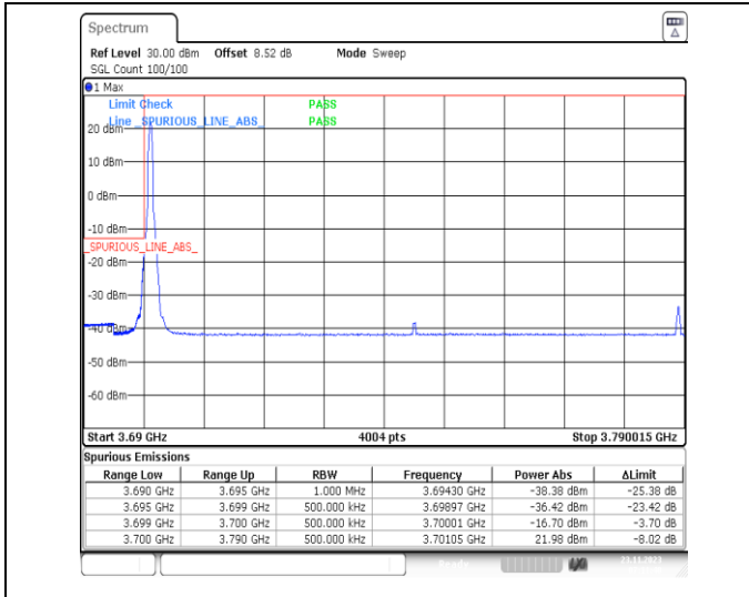
1-N77-3700-3980-PC3-30-90-L-1-DFT-PI2BPSK-Edge_1RB_Left-1@0-Ant13-1--PASS-see graph
