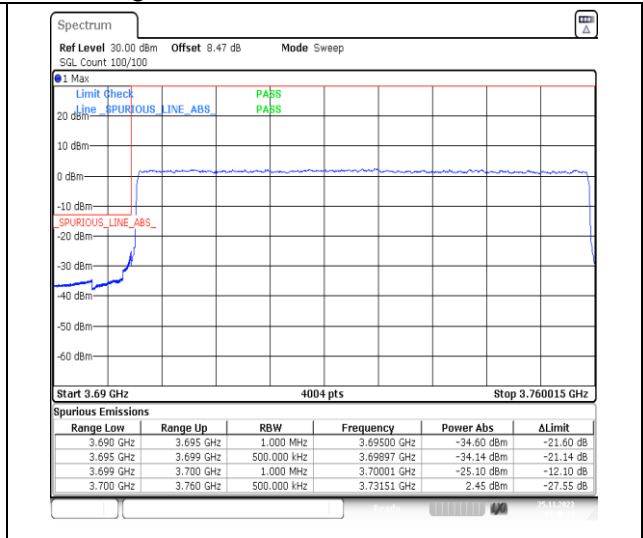
1-N77-3700-3980-PC3-30-60-L-3-DFT-PI2BPSK-Outer_Full-162@0-Ant13-1--PASS-see graph
