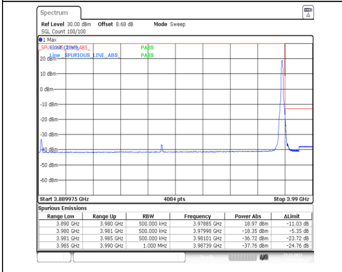
1-N77-3700-3980-PC3-30-90-H-5-CP-QPSK-Edge_1RB_Right-1@244-Ant13-1--PASS-see graph
