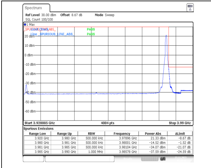
1-N77-3700-3980-PC3-30-60-H-2-DFT-PI2BPSK-Edge_1RB_Right-1@161-Ant13-1--PASS-see graph
