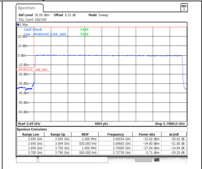
1-N77-3700-3980-PC3-30-90-L-3-DFT-PI2BPSK-Outer_Full-240@0-Ant13-1--PASS-see graph
