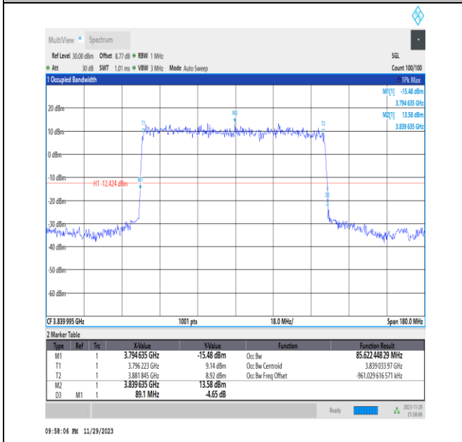
NTNV_N77-3700-3980_PC3_30_90_M_TID2_Ant13#1
