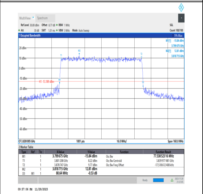
NTNV_N77-3700-3980_PC3_30_80_M_TID8_Ant13#1
