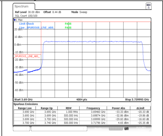
1-N77-3700-3980-PC3-30-40-L-3-DFT-PI2BPSK-Outer_Full-100@0-Ant13-1--PASS-see graph
