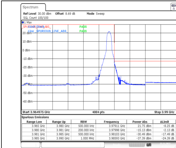
1-N77-3700-3980-PC3-30-15-H-2-DFT-PI2BPSK-Edge_1RB_Right-1@37-Ant13-1--PASS-see graph
