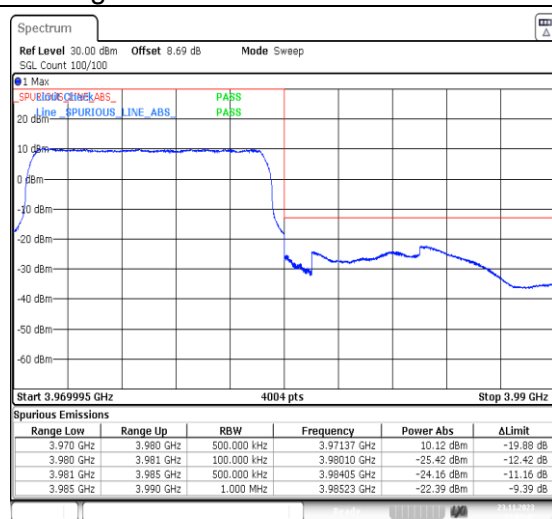
1-N77-3700-3980-PC3-30-10-H-3-DFT-PI2BPSK-Outer_Full-24@0-Ant13-1--PASS-see graph
