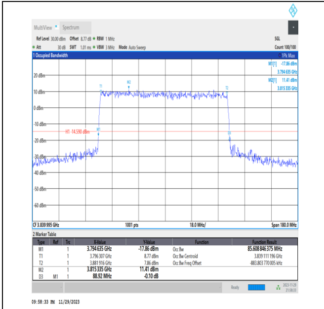
NTNV_N77-3700-3980_PC3_30_90_M_TID4_Ant13#1
