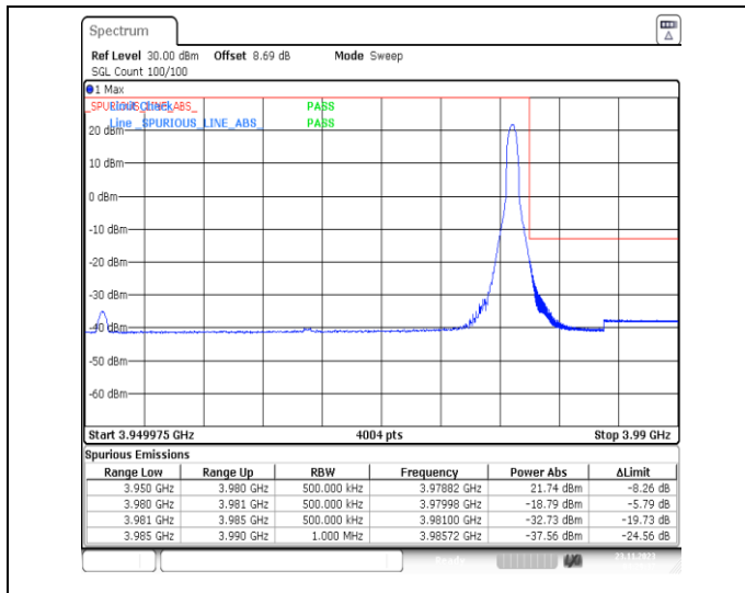
1-N77-3700-3980-PC3-30-30-H-2-DFT-PI2BPSK-Edge_1RB_Right-1@77-Ant13-1--PASS-see graph
