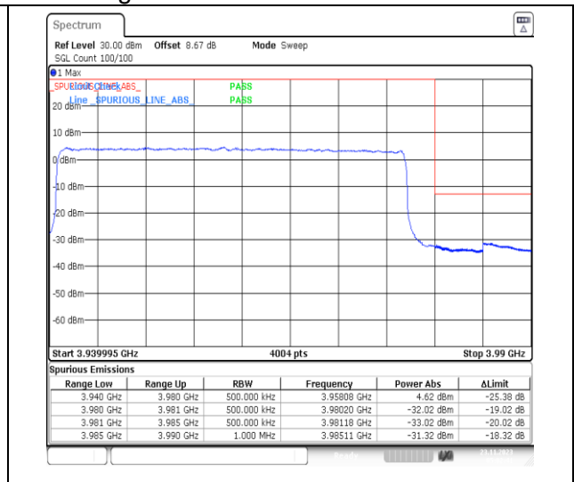
1-N77-3700-3980-PC3-30-40-H-3-DFT-PI2BPSK-Outer_Full-100@0-Ant13-1--PASS-see graph
