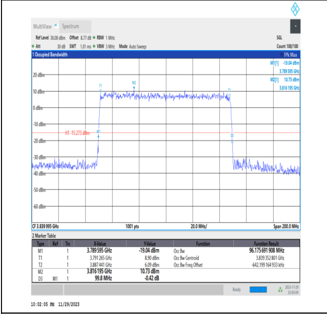
NTVN_N77-3700-3980_PC3_30_100_M_TID5_Ant13#1
