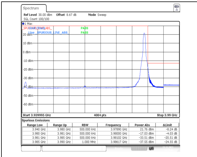
1-N77-3700-3980-PC3-30-40-H-2-DFT-PI2BPSK-Edge_1RB_Right-1@105-Ant13-1--PASS-see graph
