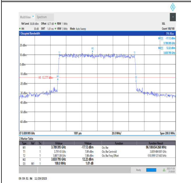
NTNV_N77-3700-3980_PC3_30_100_M_TID1_Ant13#1
