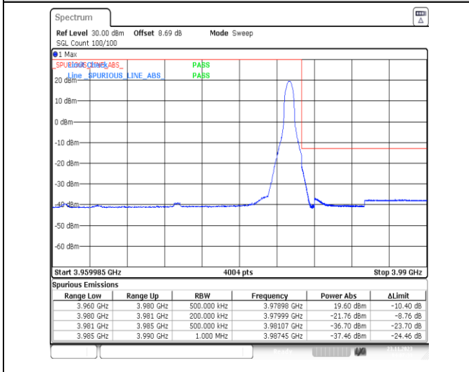
1-N77-3700-3980-PC3-30-20-H-5-CP-QPSK-Edge_1RB_Right-1@50-Ant13-1--PASS-see graph
