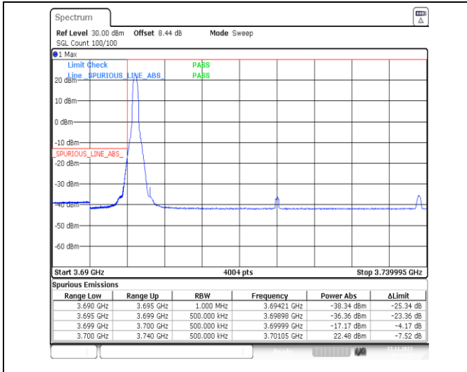
1-N77-3700-3980-PC3-30-40-L-1-DFT-PI2BPSK-Edge_1RB_Left-1@0-Ant13-1--PASS-see graph
