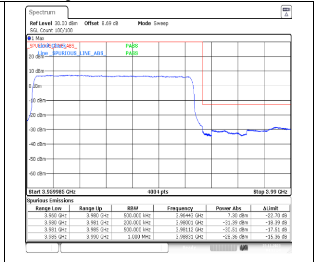
1-N77-3700-3980-PC3-30-20-H-3-DFT-PI2BPSK-Outer_Full-50@0-Ant13-1--PASS-see graph
