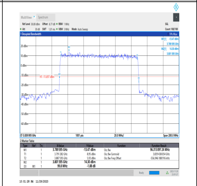
NTNV_N77-3700-3980_PC3_30_100_M_TID2_Ant13#1
