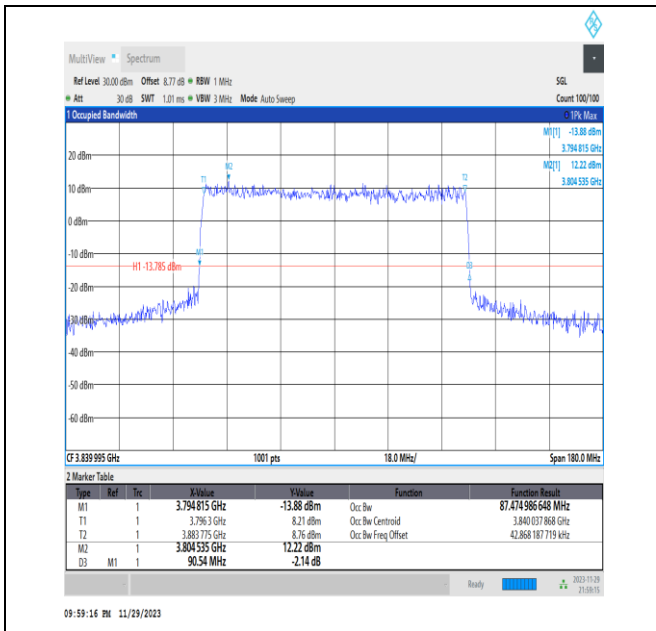
NTNV_N77-3700-3980_PC3_30_90_M_TID8_Ant13#1
