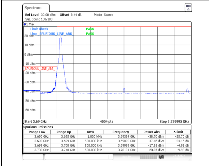
1-N77-3700-3980-PC3-30-40-L-4-CP-QPSK-Edge_1RB_Left-1@0-Ant13-1--PASS-see graph
