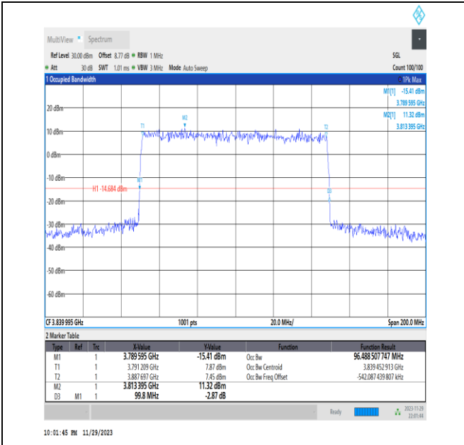
NTVN_N77-3700-3980_PC3_30_100_M_TID3_Ant13#1
