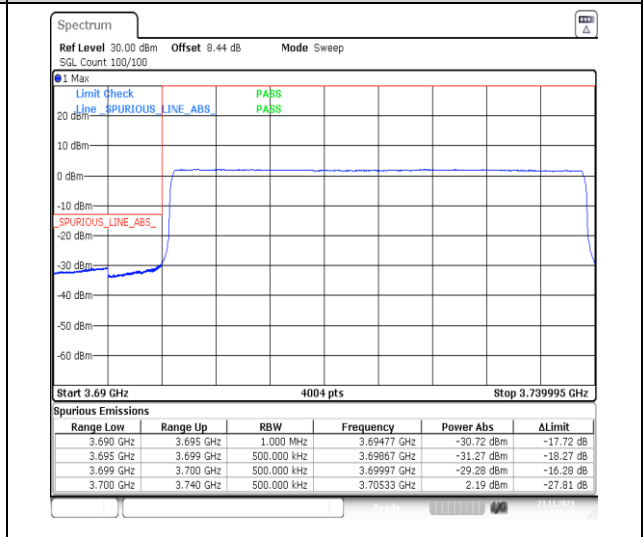
1-N77-3700-3980-PC3-30-40-L-6-CP-QPSK-Outer_Full-106@0-Ant13-1--PASS-see graph
