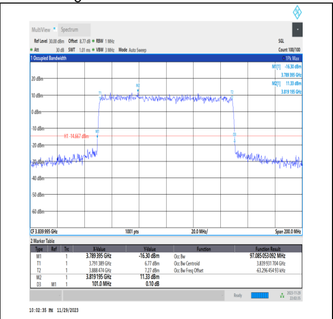
NTVN_N77-3700-3980_PC3_30_100_M_TID8_Ant13#1
