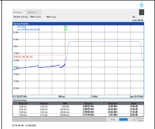
1-N77-3700-3980-PC3-30-15-L-6-CP-QPSK-Outer_Full-38@0-Ant13-1--PASS-see graph
