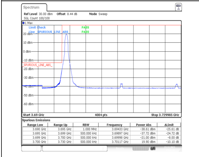
1-N77-3700-3980-PC3-30-30-L-4-CP-QPSK-Edge_1RB_Left-1@0-Ant13-1--PASS-see graph
