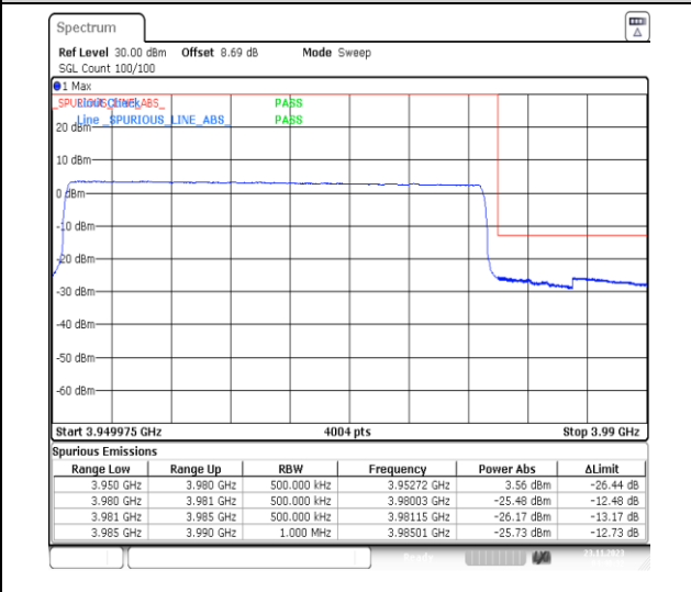
1-N77-3700-3980-PC3-30-30-H-6-CP-QPSK-Outer_Full-78@0-Ant13-1--PASS-see graph
