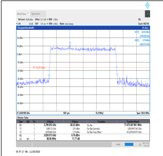
NTNV_N77-3700-3980_PC3_30_80_M_TID9_Ant13#1
