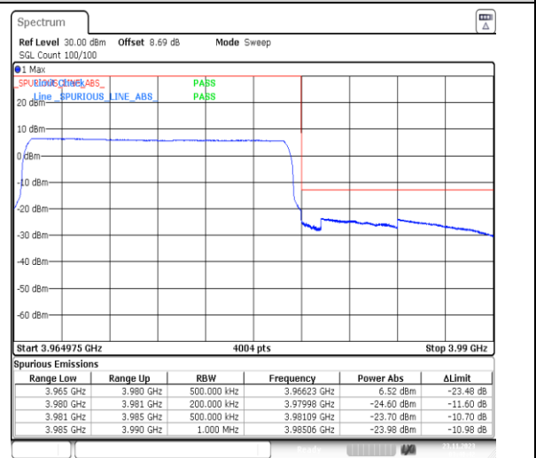
1-N77-3700-3980-PC3-30-15-H-3-DFT-PI2BPSK-Outer_Full-36@0-Ant13-1--PASS-see graph
