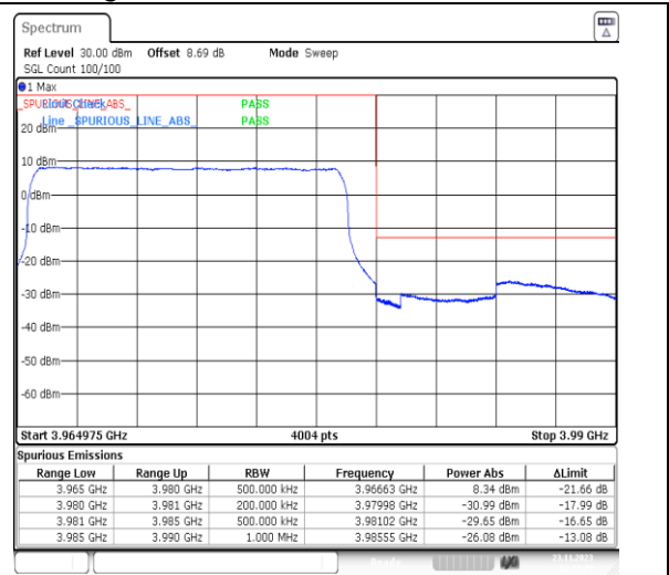
1-N77-3700-3980-PC3-30-15-H-3-DFT-PI2BPSK-Outer_Full-36@0-Ant13-1--PASS-see graph
