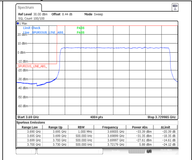
1-N77-3700-3980-PC3-30-30-L-3-DFT-PI2BPSK-Outer_Full-75@0-Ant13-1--PASS-see graph
