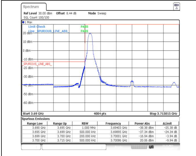
1-N77-3700-3980-PC3-30-15-L-4-CP-QPSK-Edge_1RB_Left-1@0-Ant13-1--PASS-see graph
