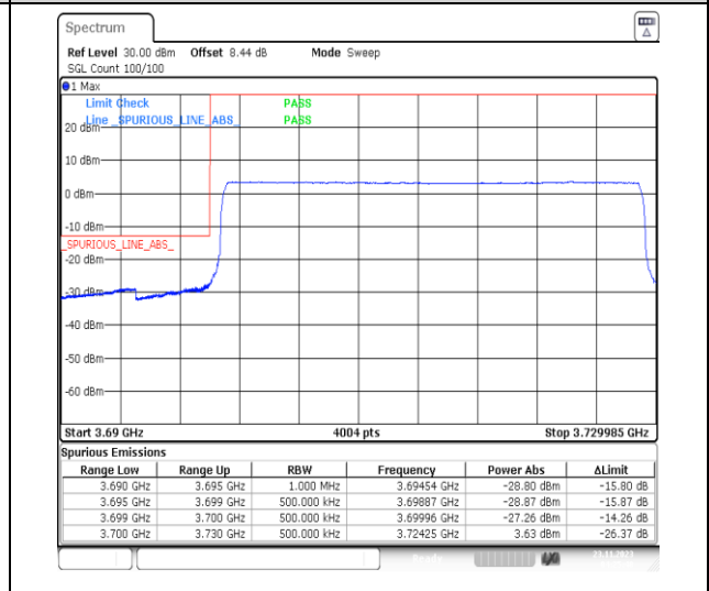
1-N77-3700-3980-PC3-30-30-L-6-CP-QPSK-Outer_Full-78@0-Ant13-1--PASS-see graph
