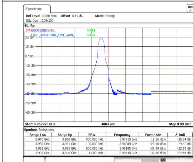
1-N77-3700-3980-PC3-30-10-H-2-DFT-PI2BPSK-Edge_1RB_Right-1@23-Ant13-1--PASS-see graph
