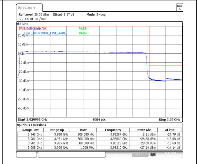
1-N77-3700-3980-PC3-30-40-H-6-CP-QPSK-Outer_Full-106@0-Ant13-1--PASS-see graph
