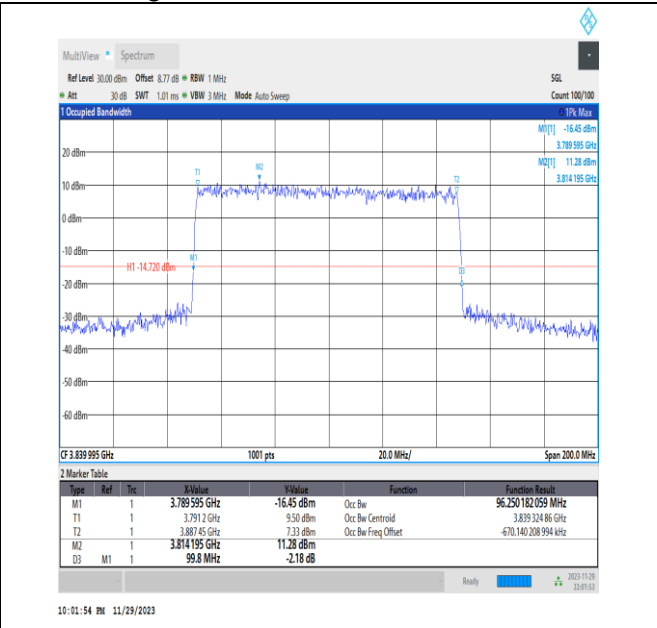
NTVN_N77-3700-3980_PC3_30_100_M_TID4_Ant13#1
