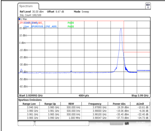
1-N77-3700-3980-PC3-30-40-H-5-CP-QPSK-Edge_1RB_Right-1@105-Ant13-1--PASS-see graph
