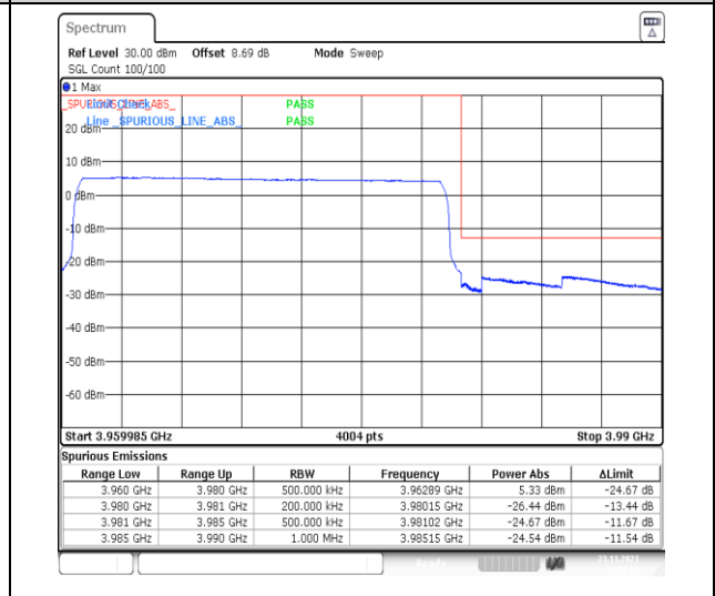
1-N77-3700-3980-PC3-30-20-H-6-CP-QPSK-Outer_Full-51@0-Ant13-1--PASS-see graph
