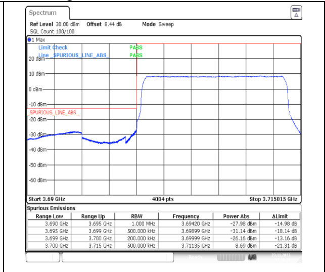
1-N77-3700-3980-PC3-30-15-L-3-DFT-PI2BPSK-Outer_Full-36@0-Ant13-1--PASS-see graph
