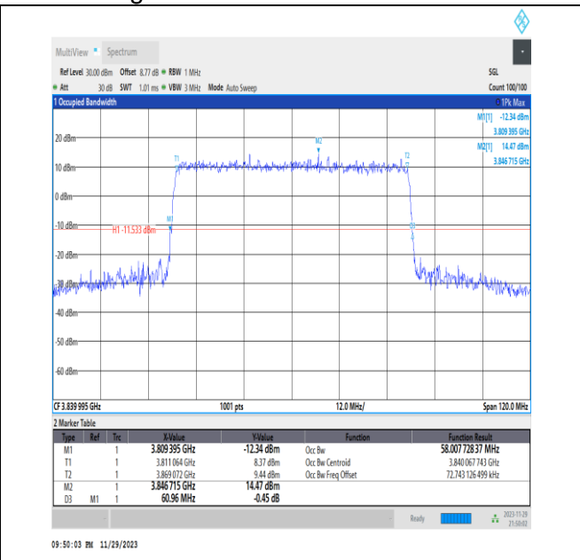
NTNV_N77-3700-3980_PC3_30_60_M_TID4_Ant13#1
