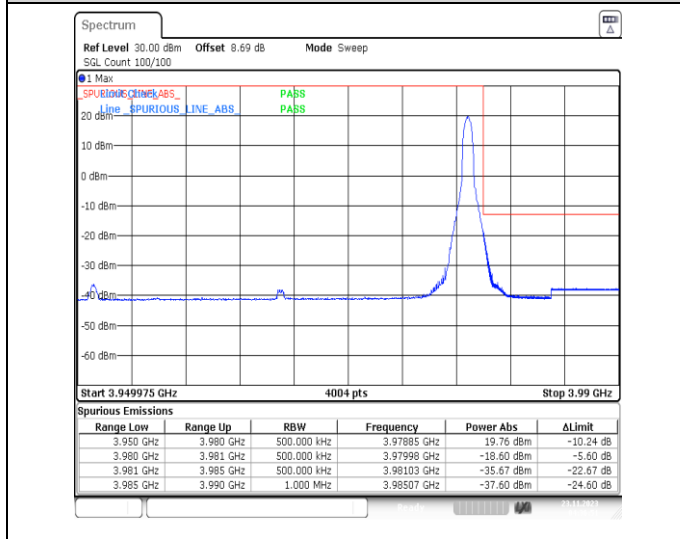
1-N77-3700-3980-PC3-30-30-H-5-CP-QPSK-Edge_1RB_Right-1@77-Ant13-1--PASS-see graph
