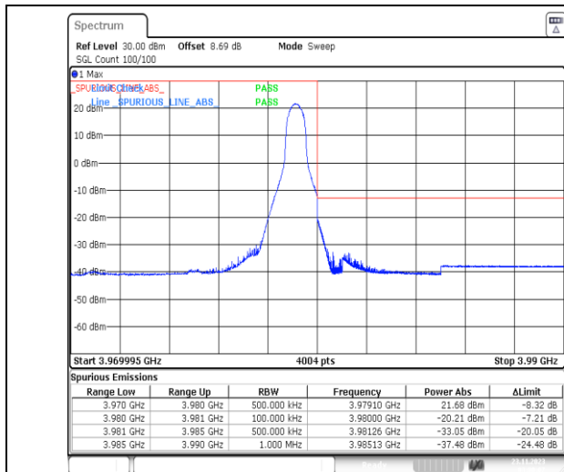
1-N77-3700-3980-PC3-30-10-H-2-DFT-PI2BPSK-Edge_1RB_Right-1@23-Ant13-1--PASS-see graph
