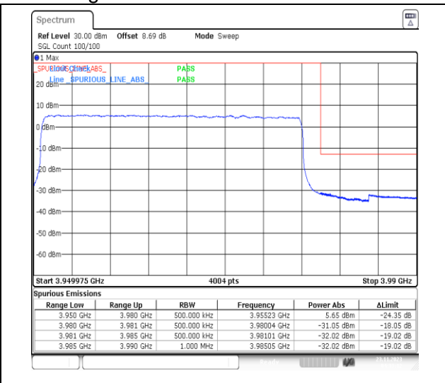
1-N77-3700-3980-PC3-30-30-H-3-DFT-PI2BPSK-Outer_Full-75@0-Ant13-1--PASS-see graph
