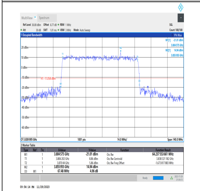
NTNV_N77-3700-3980_PC3_30_70_M_TID4_Ant13#1
