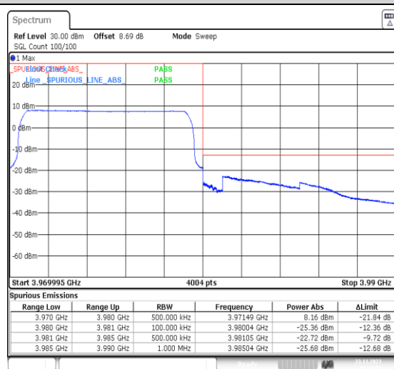
1-N77-3700-3980-PC3-30-10-H-3-DFT-PI2BPSK-Outer_Full-24@0-Ant13-1--PASS-see graph
