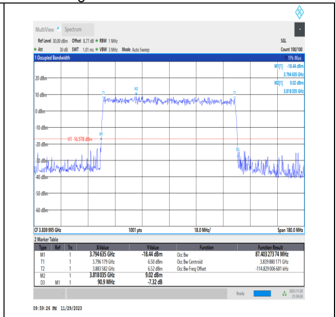
NTNV_N77-3700-3980_PC3_30_90_M_TID9_Ant13#1
