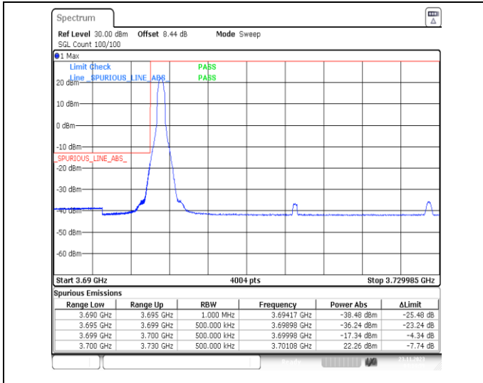
1-N77-3700-3980-PC3-30-30-L-1-DFT-PI2BPSK-Edge_1RB_Left-1@0-Ant13-1--PASS-see graph
