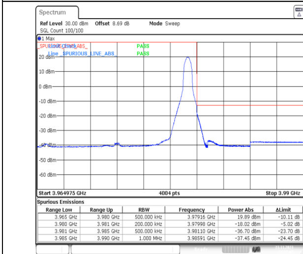
1-N77-3700-3980-PC3-30-15-H-2-DFT-PI2BPSK-Edge_1RB_Right-1@37-Ant13-1--PASS-see graph
