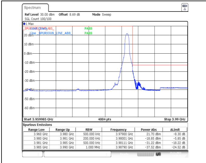
1-N77-3700-3980-PC3-30-20-H-2-DFT-PI2BPSK-Edge_1RB_Right-1@50-Ant13-1--PASS-see graph
