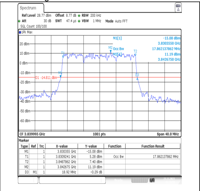
NTNV_N77-3700-3980_PC3_30_20_M_TID4_Ant13#1
