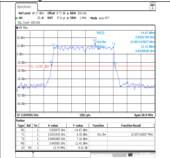
NTNV_N77-3700-3980_PC3_30_15_M_TID5_Ant13#1
