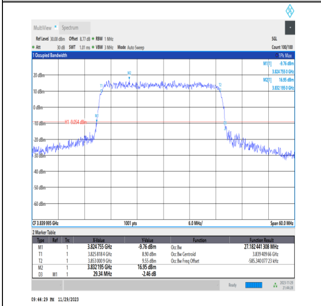
NTNV_N77-3700-3980_PC3_30_30_M_TID8_Ant13#1
