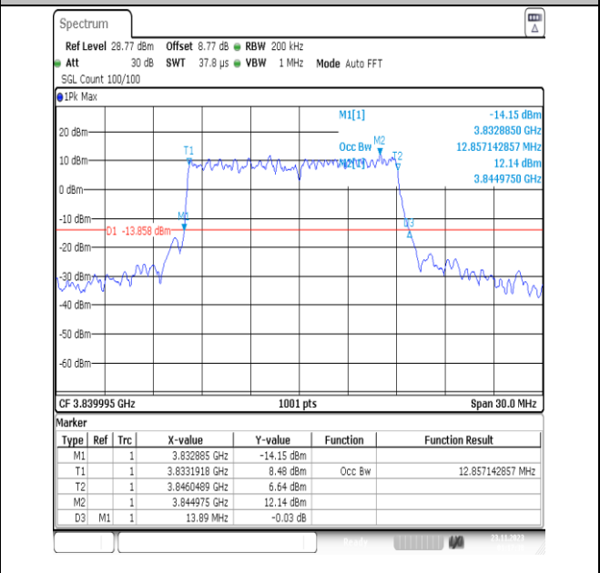
NTNV_N77-3700-3980_PC3_30_15_M_TID3_Ant13#1
