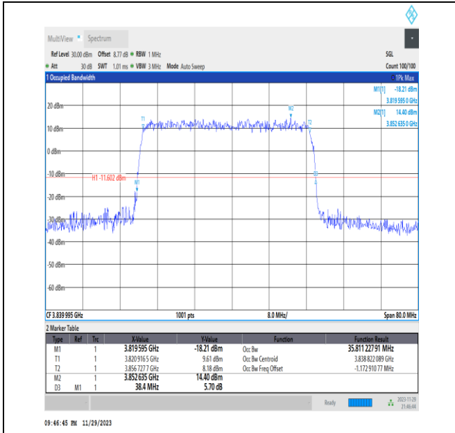
NTNV_N77-3700-3980_PC3_30_40_M_TID9_Ant13#1
