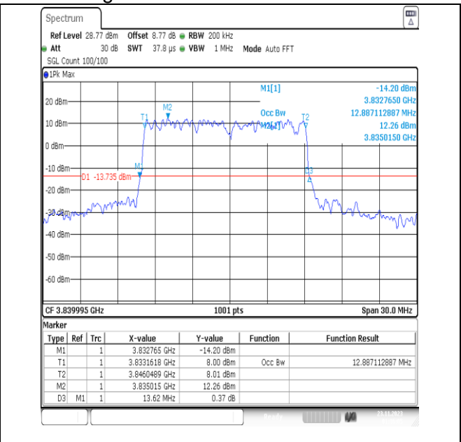
NTNV_N77-3700-3980_PC3_30_15_M_TID1_Ant13#1
