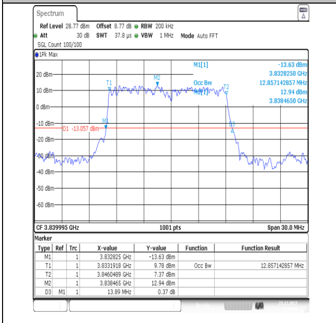
NTNV_N77-3700-3980_PC3_30_15_M_TID2_Ant13#1
