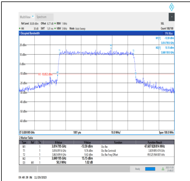
NTNV_N77-3700-3980_PC3_30_50_M_TID8_Ant13#1
