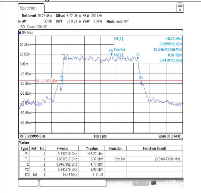
NTNV_N77-3700-3980_PC3_30_15_M_TID9_Ant13#1
