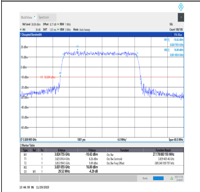
NTNV_N77-3700-3980_PC3_30_30_M_TID4_Ant13#1
