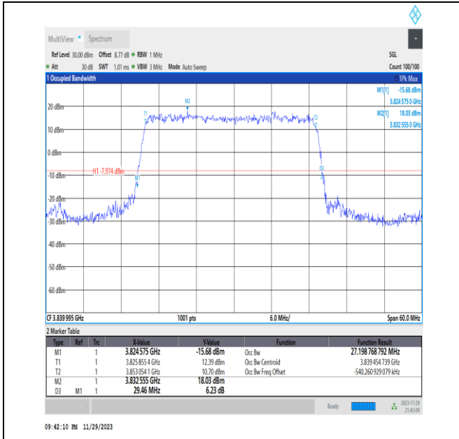
NTNV_N77-3700-3980_PC3_30_30_M_TID2_Ant13#1
