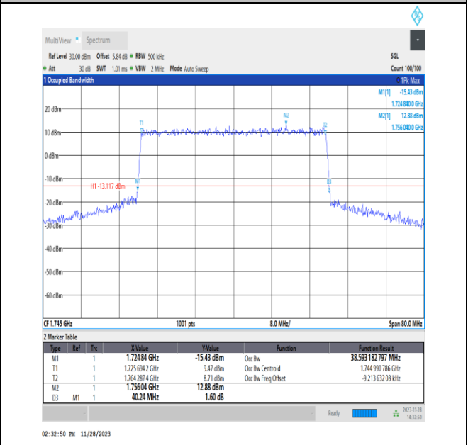
NTNV_N66_PC3_15_40_M_TID8_Ant14#1
