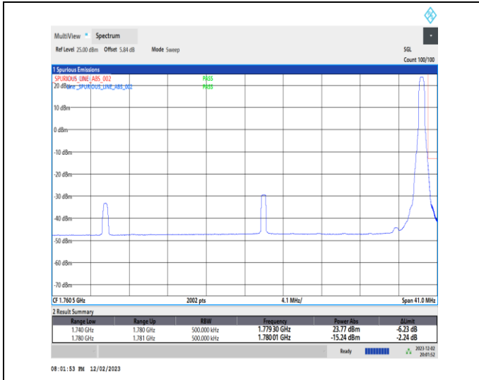
1-N66-PC3-15-35-H-2-DFT-PI2BPSK-Edge_1RB_Right-t-1@187-Ant14-1-seegraph-PASS-see graph
