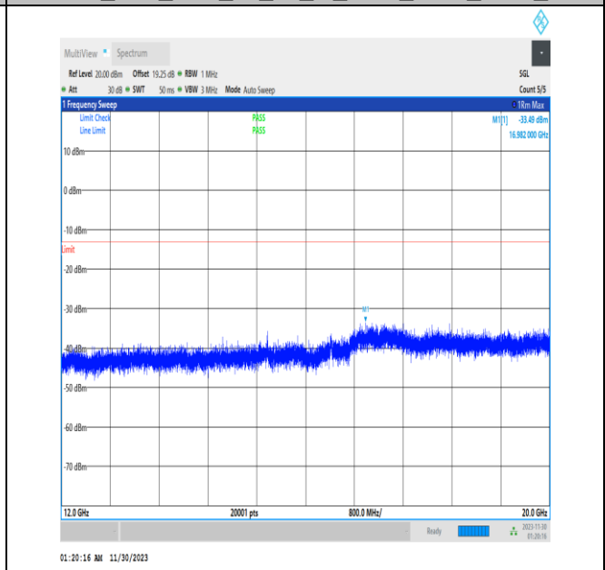
NTVN_N66_PC3_15_40_M_TID1_12000_20000_#1
