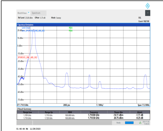
1-N66-PC3-15-10-L-1-DFT-PI2BPSK-Edge_1RB_Left-1@0-Ant14-1-seegraph-PASS-see graph
