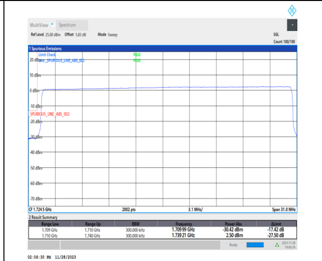
1-N66-PC3-15-30-L-6-CP-QPSK-Outer_Full-160@0-Ant14-1-seegraph-PASS-see graph
