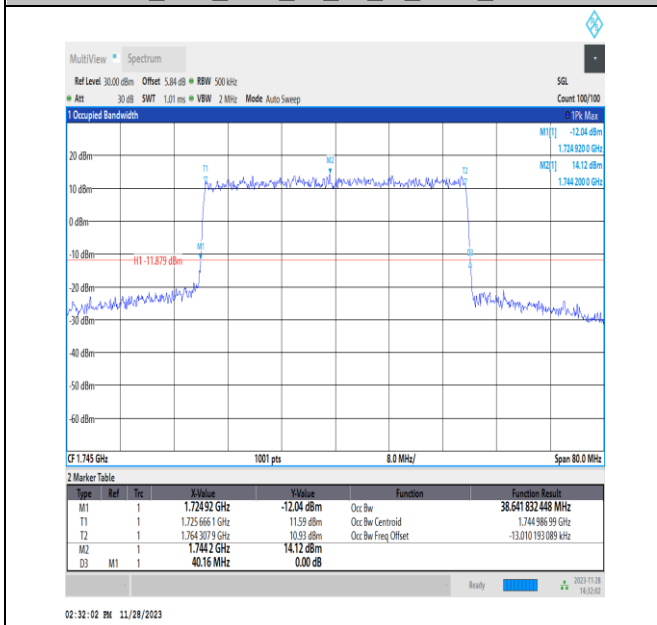
NTNV_N66_PC3_15_40_M_TID3_Ant14#1
