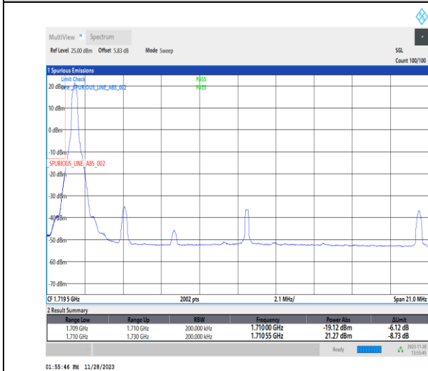
1-N66-PC3-15-20-L-4-CP-QPSK-Edge_1RB_Left-1@0-Ant14-1-seegraph-PASS-see graph
