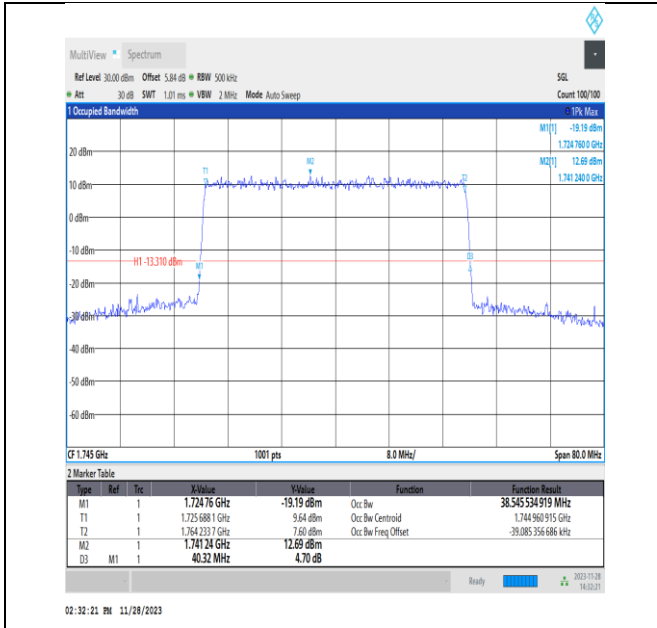
NTNV_N66_PC3_15_40_M_TID5_Ant14#1
