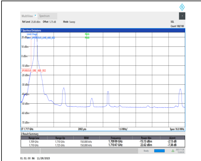
1-N66-PC3-15-15-L-1-DFT-PI2BPSK-Edge_1RB_Left-1@0-Ant14-1-seegraph-PASS-see graph
