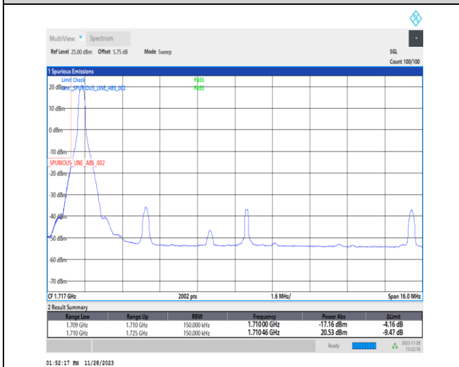
1-N66-PC3-15-15-L-4-CP-QPSK-Edge_1RB_Left-1@0-Ant14-1-seegraph-PASS-see graph
