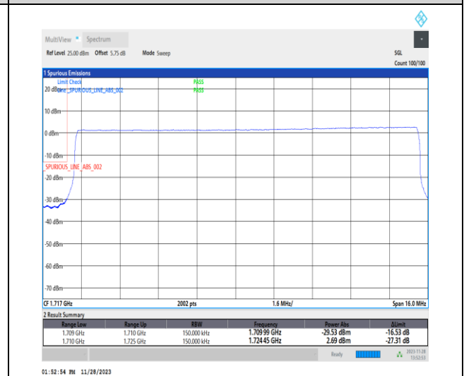
1-N66-PC3-15-15-L-6-CP-QPSK-Outer_Full-79@0-Ant14-1-seegraph-PASS-see graph
