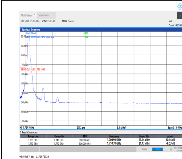
1-N66-PC3-15-30-L-4-CP-QPSK-Edge_1RB_Left-1@0-Ant14-1-seegraph-PASS-see graph
