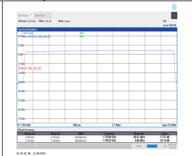
1-N66-PC3-15-30-L-3-DFT-PI2BPSK-Outer_Full-160@0-Ant14-1-seegraph-PASS-see graph
