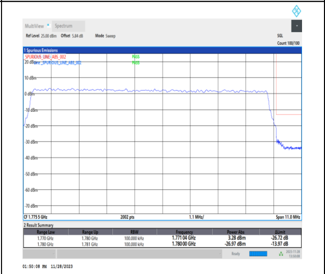
1-N66-PC3-15-10-H-6-CP-QPSK-Outer_Full-52@0-Ant14-1-seegraph-PASS-see graph
