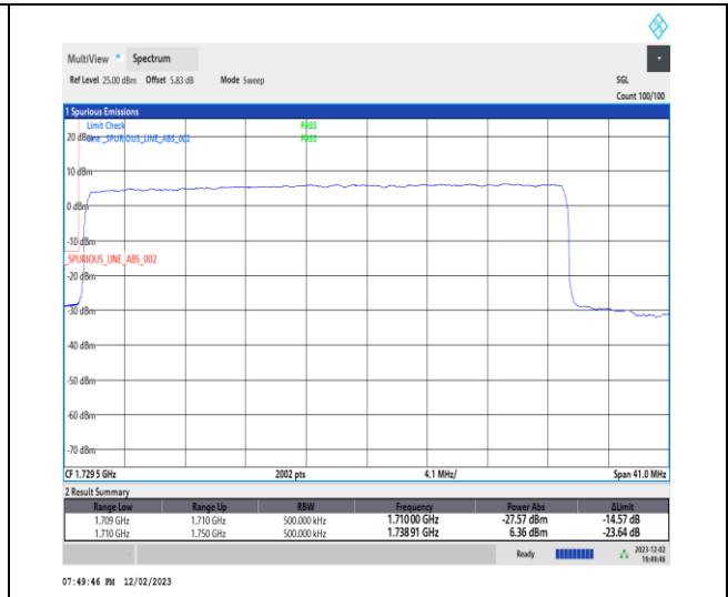
1-N66-PC3-15-35-L-3-DFT-PI2BPSK-Outer_Full-180@0-Ant14-1-seegraph-PASS-see graph
