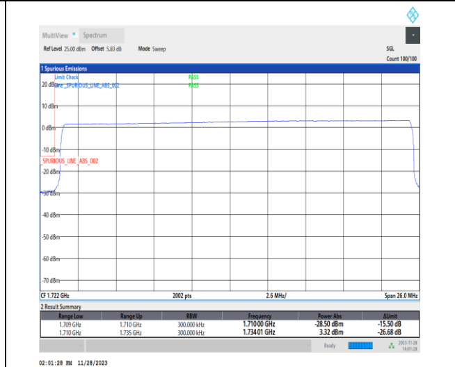
1-N66-PC3-15-25-L-6-CP-QPSK-Outer_Full-133@0-Ant14-1-seegraph-PASS-see graph
