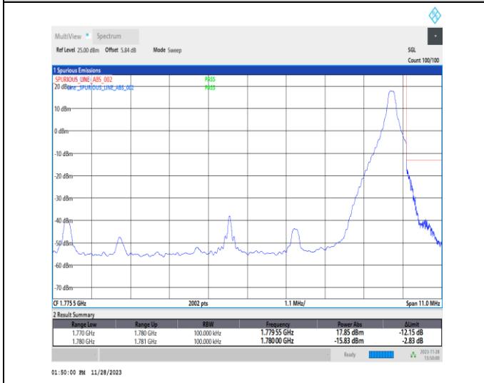
1-N66-PC3-15-10-H-5-CP-QPSK-Edge_1RB_Right-1@51-Ant14-1-seegraph-PASS-see graph
