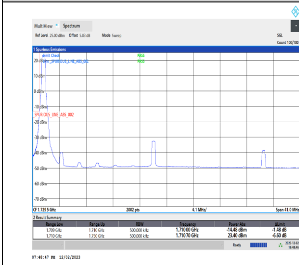
1-N66-PC3-15-35-L-4-CP-QPSK-Edge_1RB_Left-1@0-Ant14-1-seegraph-PASS-see graph
