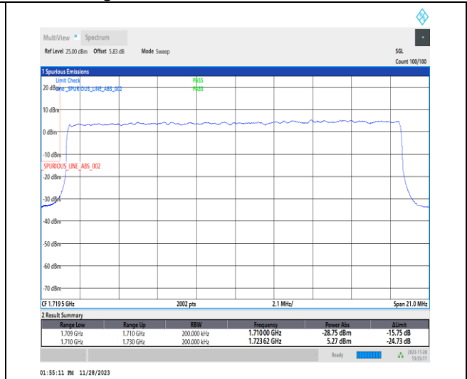
1-N66-PC3-15-20-L-3-DFT-PI2BPSK-Outer_Full-100@0-Ant14-1-seegraph-PASS-see graph
