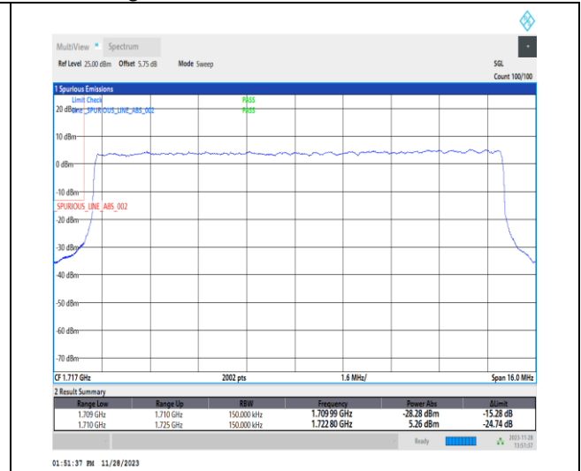
1-N66-PC3-15-15-L-3-DFT-PI2BPSK-Outer_Full-75@0-Ant14-1-seegraph-PASS-see graph
