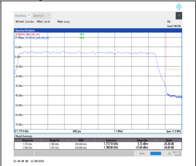
1-N66-PC3-15-10-H-3-DFT-PI2BPSK-Outer_Full-50@0-Ant14-1-seegraph-PASS-see graph
