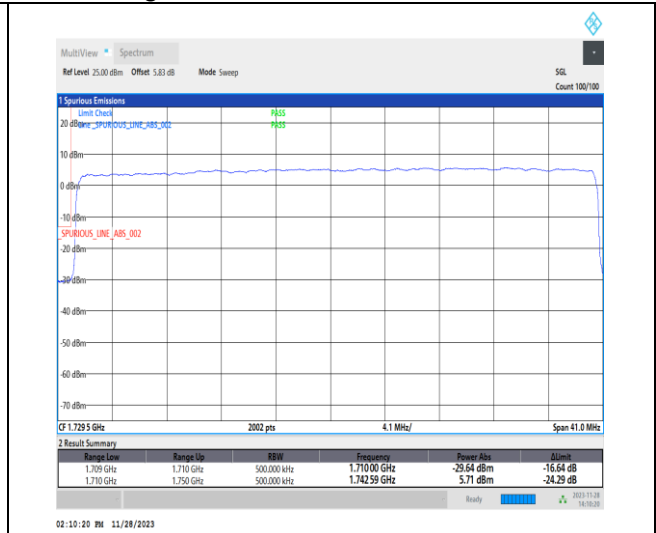
1-N66-PC3-15-40-L-3-DFT-PI2BPSK-Outer_Full-216@0-Ant14-1-seegraph-PASS-see graph
