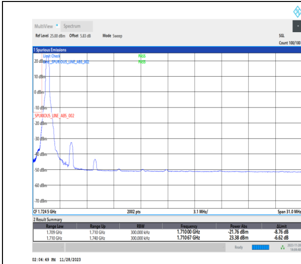
1-N66-PC3-15-30-L-1-DFT-PI2BPSK-Edge_1RB_Left-1@0-Ant14-1-seegraph-PASS-see graph
