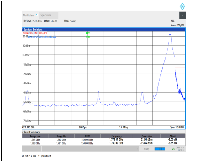
1-N66-PC3-15-15-H-2-DFT-PI2BPSK-Edge_1RB_Right-t-1@78-Ant14-1-seegraph-PASS-see graph
