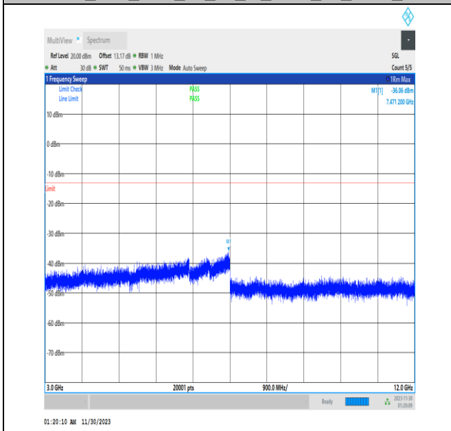
NTVN_N66_PC3_15_40_M_TID1_3000_12000_#1
