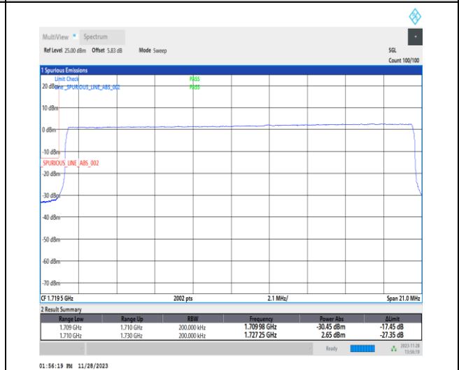
1-N66-PC3-15-20-L-6-CP-QPSK-Outer_Full-106@0-Ant14-1-seegraph-PASS-see graph
