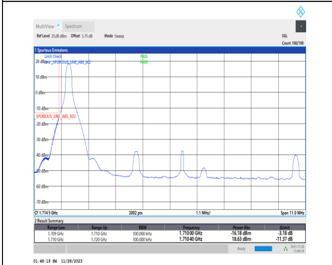
1-N66-PC3-15-10-L-4-CP-QPSK-Edge_1RB_Left-1@0-Ant14-1-seegraph-PASS-see graph
