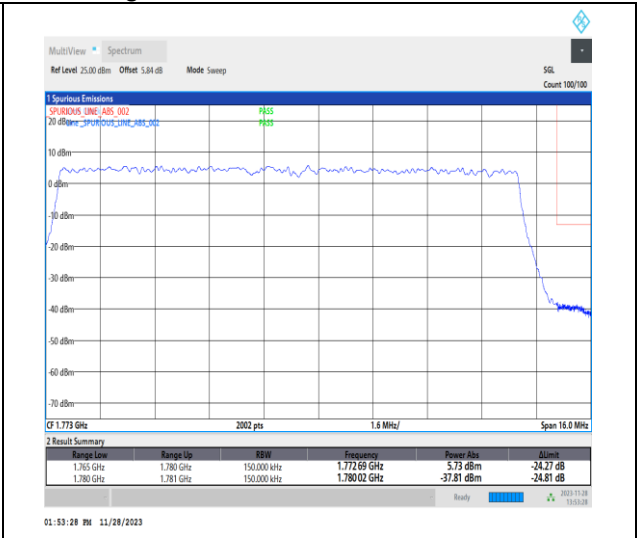
1-N66-PC3-15-15-H-3-DFT-PI2BPSK-Outer_Full-75@0-Ant14-1-seegraph-PASS-see graph
