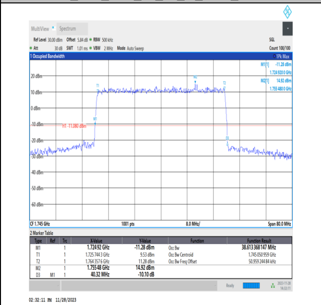
NTNV_N66_PC3_15_40_M_TID4_Ant14#1
