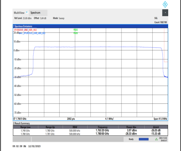
1-N66-PC3-15-35-H-6-CP-QPSK-Outer_Full-188@0-Ant14-1-seegraph-PASS-see graph
