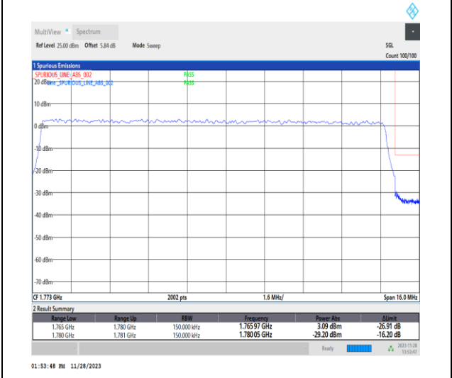
1-N66-PC3-15-15-H-6-CP-QPSK-Outer_Full-79@0-Ant14-1-seegraph-PASS-see graph
