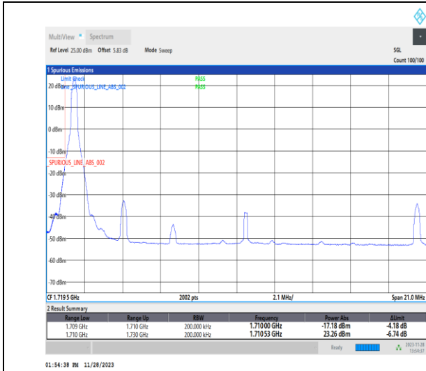
1-N66-PC3-15-20-L-1-DFT-PI2BPSK-Edge_1RB_Left-1@0-Ant14-1-seegraph-PASS-see graph
