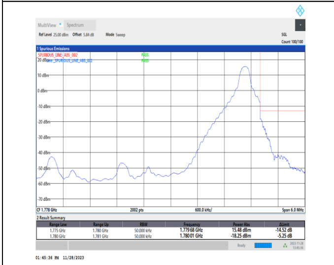
1-N66-PC3-15-5-H-5-CP-QPSK-Edge_1RB_Right-1@24-Ant14-1-seegraph-PASS-see graph
