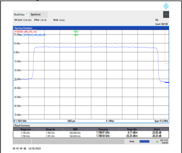
1-N66-PC3-15-35-H-3-DFT-PI2BPSK-Outer_Full-180@0-Ant14-1-seegraph-PASS-see graph
