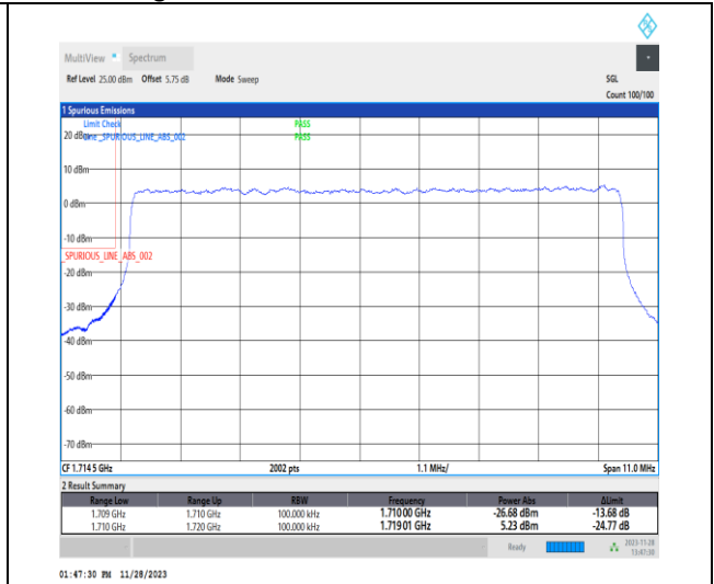
1-N66-PC3-15-10-L-3-DFT-PI2BPSK-Outer_Full-50@0-Ant14-1-seegraph-PASS-see graph
