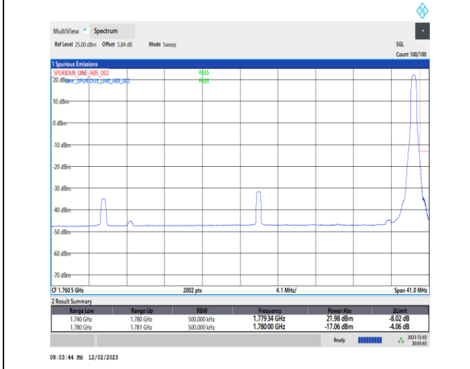
1-N66-PC3-15-35-H-5-CP-QPSK-Edge_1RB_Right-1@187-Ant14-1-seegraph-PASS-see graph
