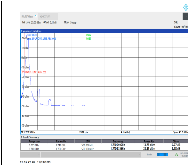
1-N66-PC3-15-40-L-1-DFT-PI2BPSK-Edge_1RB_Left-1@0-Ant14-1-seegraph-PASS-see graph
