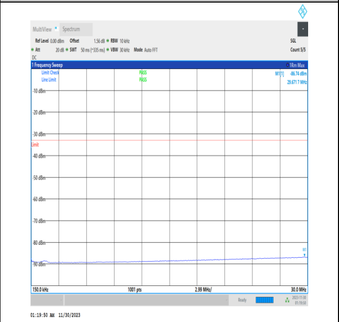
NTNV_N66_PC3_15_40_M_TID1_0.15_30_#1
