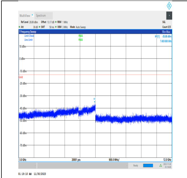
NTNV_N66_PC3_15_40_L_TID1_3000_12000_#1
