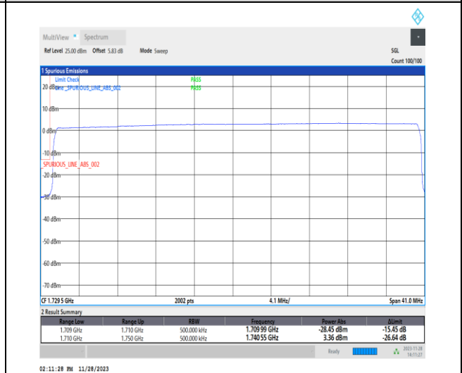
1-N66-PC3-15-40-L-6-CP-QPSK-Outer_Full-216@0-Ant14-1-seegraph-PASS-see graph
