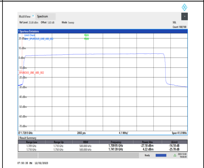
1-N66-PC3-15-35-L-6-CP-QPSK-Outer_Full-188@0-Ant14-1-seegraph-PASS-see graph
