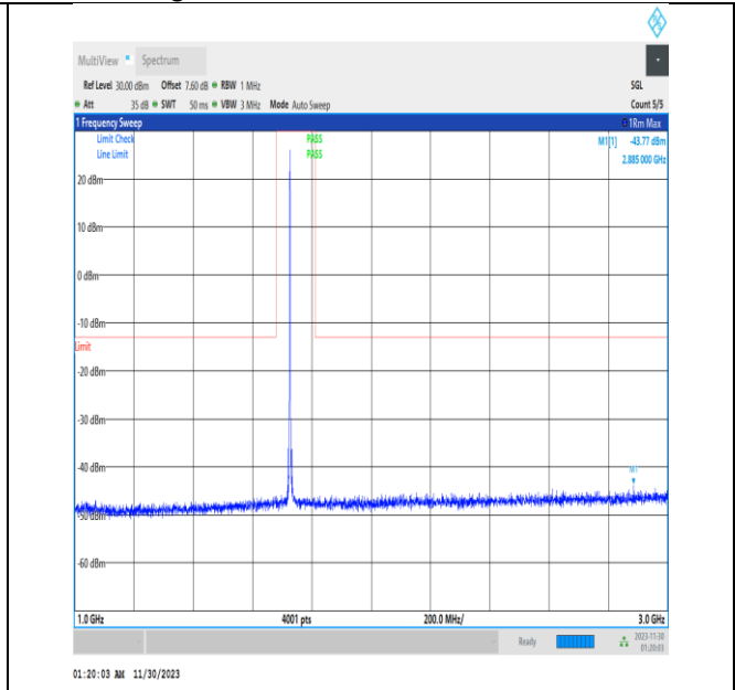
NTVN_N66_PC3_15_40_M_TID1_1000_3000_#1
