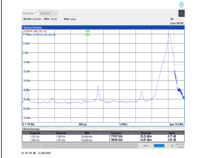
1-N66-PC3-15-15-H-5-CP-QPSK-Edge_1RB_Right-1@78-Ant14-1-seegraph-PASS-see graph
