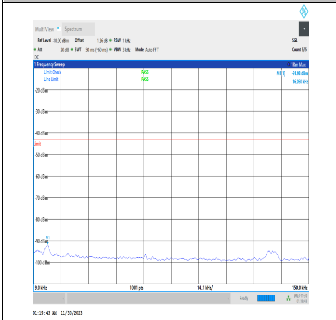
NTNV_N66_PC3_15_40_M_TID1_0.009_0.15_#1
