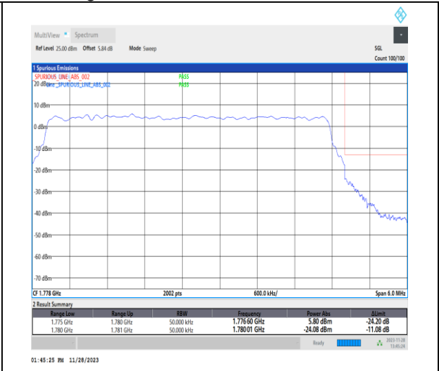
1-N66-PC3-15-5-H-3-DFT-PI2BPSK-Outer_Full-25@0-Ant14-1-seegraph-PASS-see graph
