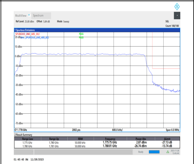
1-N66-PC3-15-5-H-6-CP-QPSK-Outer_Full-25@0-Ant14-1-seegraph-PASS-see graph
