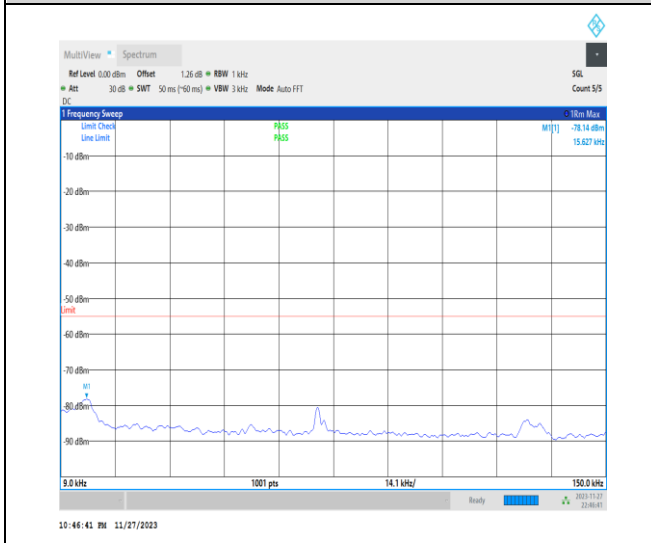
1-N41-PC2-30-100-M-1-DFT-PI2BPSK-Inner_1RB_L Left-1 @ 1-0.009-0.15-Ant31-0.01--78.14--55-PASS
