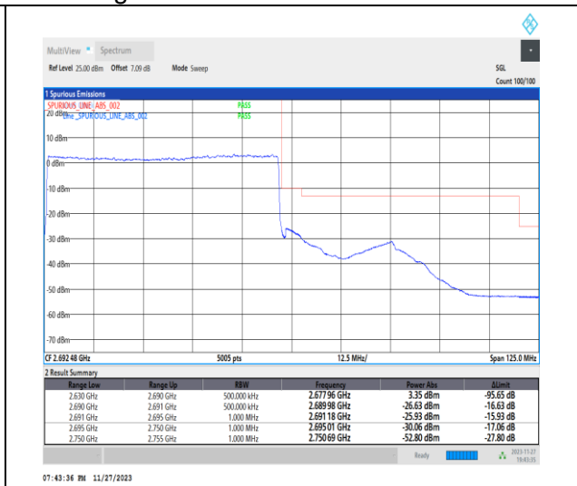
1-N41-PC2-30-60-H-3-DFT-PI2BPSK-Outer_Full-162@0-Ant31-1--PASS-see graph
