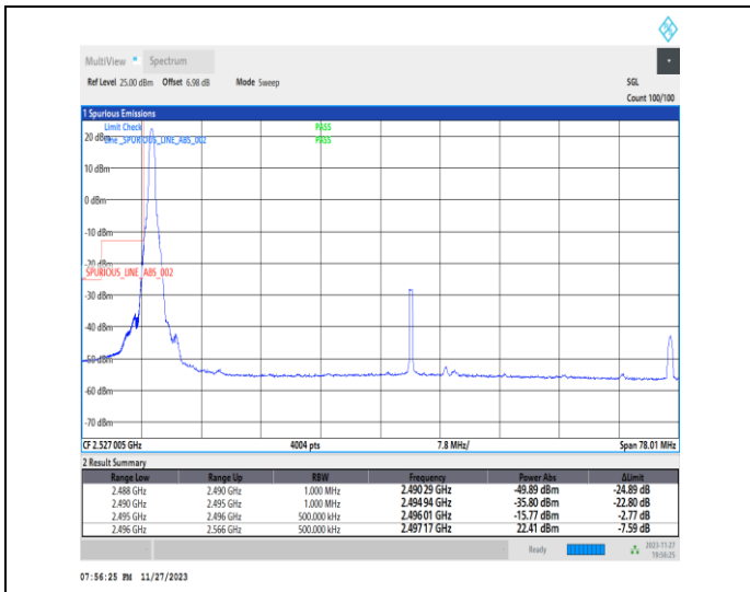
1-N41-PC2-30-70-L-1-DFT-PI2BPSK-Edge_1RB_Left-1@0-Ant31-1--PASS-see graph
