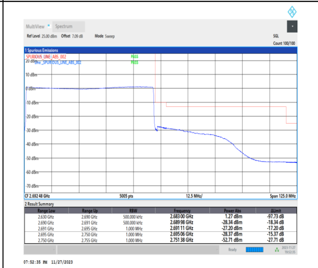
1-N41-PC2-30-60-H-6-CP-QPSK-Outer_Full-162@0-Ant31-1--PASS-see graph
