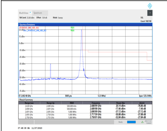
1-N41-PC2-30-60-H-5-CP-QPSK-Edge_1RB_Right-1@161-Ant31-1--PASS-see graph
