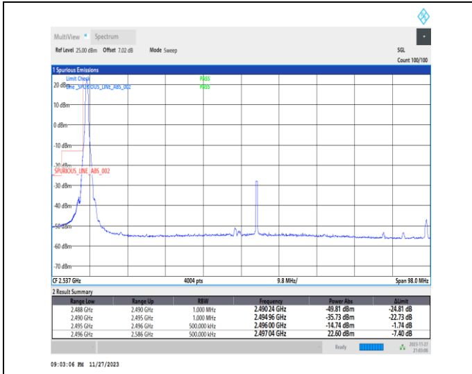
1-N41-PC2-30-90-L-1-DFT-PI2BPSK-Edge_1RB_Left-1@0-Ant31-1--PASS-see graph
