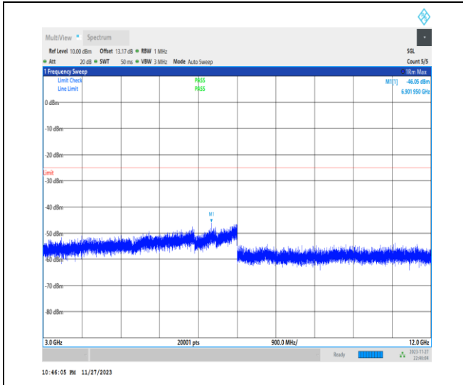
1-N41-PC2-30-100-L-1-DFT-PI2BPSK-Inner_1RB_L eft-1 @ 1-3000-12000-Ant31-10703.10--46.05--25-PA SS
