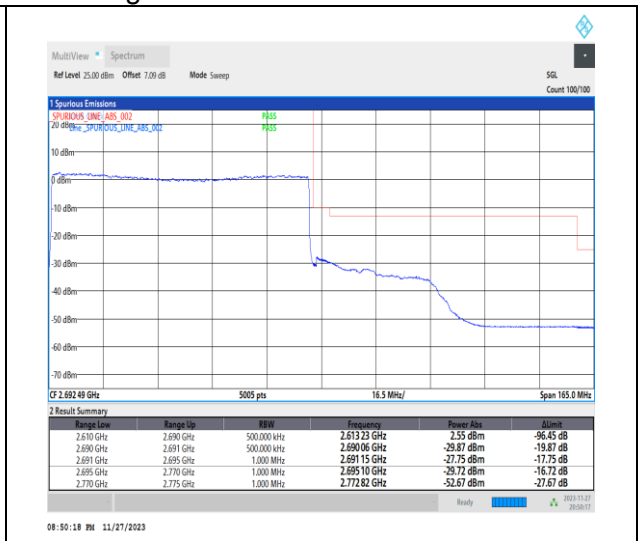
1-N41-PC2-30-80-H-3-DFT-PI2BPSK-Outer_Full-216@0-Ant31-1--PASS-see graph
