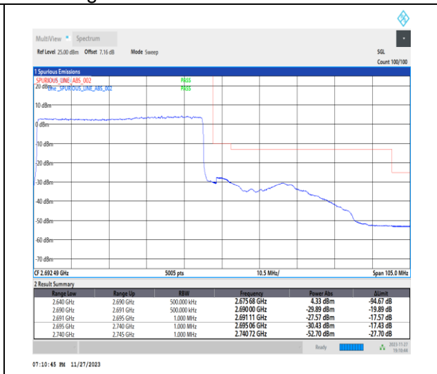
1-N41-PC2-30-50-H-3-DFT-PI2BPSK-Outer_Full-128@0-Ant31-1--PASS-see graph
