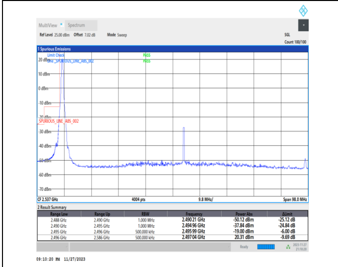
1-N41-PC2-30-90-L-4-CP-QPSK-Edge_1RB_Left-1@0-Ant31-1--PASS-see graph
