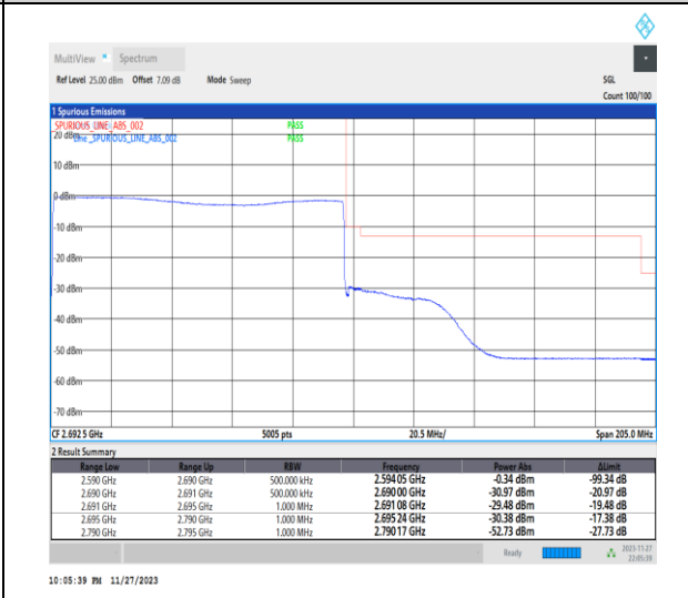
1-N41-PC2-30-100-H-6-CP-QPSK-Outer_Full-273 @0-Ant31-1--PASS-see graph
