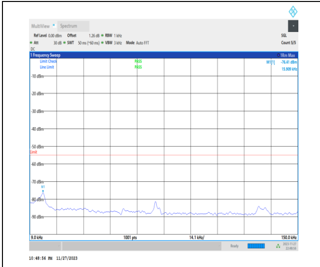
1-N41-PC2-30-100-H-1-DFT-PI2BPSK-Inner_1RB_L eft-1@1-0.009-0.15-Ant31-0.01--76.41--55-PASS
