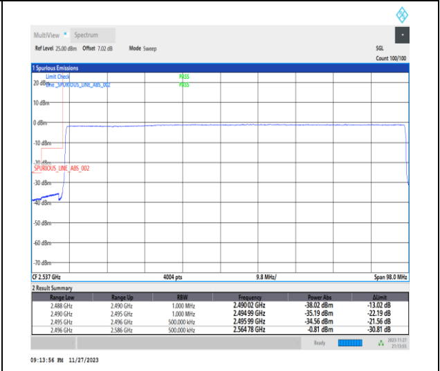
1-N41-PC2-30-90-L-6-CP-QPSK-Outer_Full-245@0-Ant31-1--PASS-see graph
