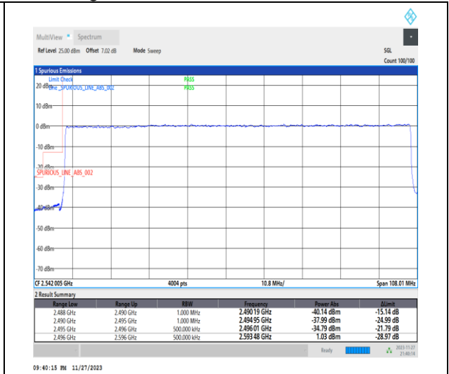
1-N41-PC2-30-100-L-3-DFT-PI2BPSK-Outer_Full-270@0-Ant31-1--PASS-see graph
