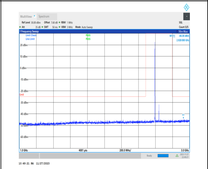
1-N41-PC2-30-100-H-1-DFT-PI2BPSK-Inner_1RB_L eft-1@1-1000-3000-Ant31-2849.50--44.30--25-PASS
