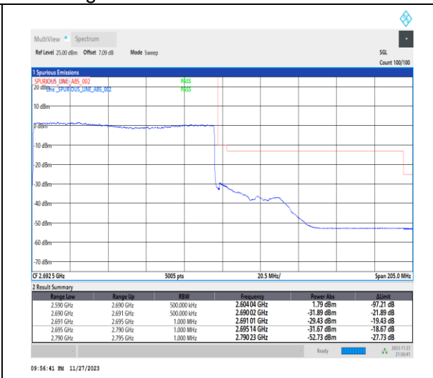
1-N41-PC2-30-100-H-3-DFT-PI2BPSK-Outer_Full-270@0-Ant31-1--PASS-see graph
