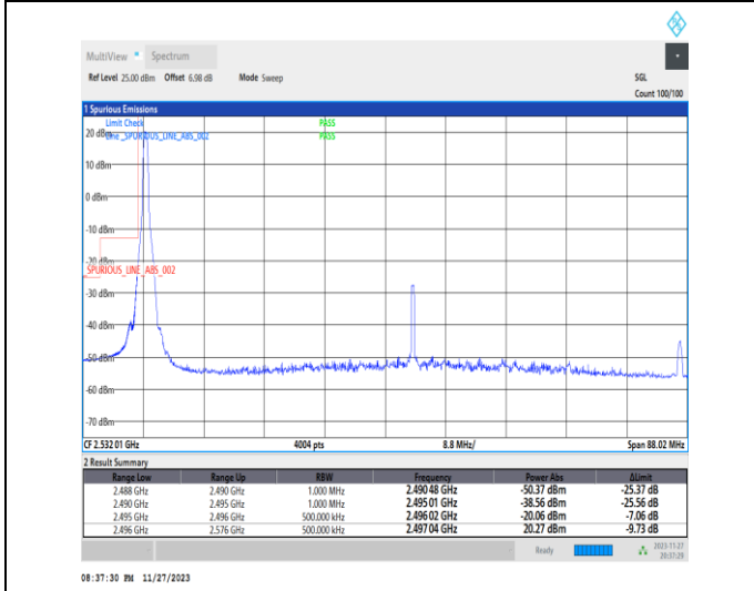
1-N41-PC2-30-80-L-4-CP-QPSK-Edge_1RB_Left-1@0-Ant31-1--PASS-see graph
