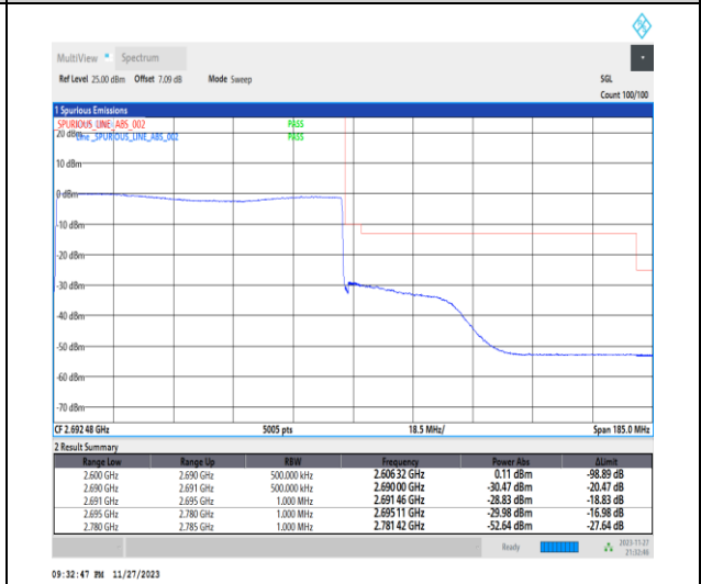
1-N41-PC2-30-90-H-6-CP-QPSK-Outer_Full-245@0-Ant31-1--PASS-see graph
