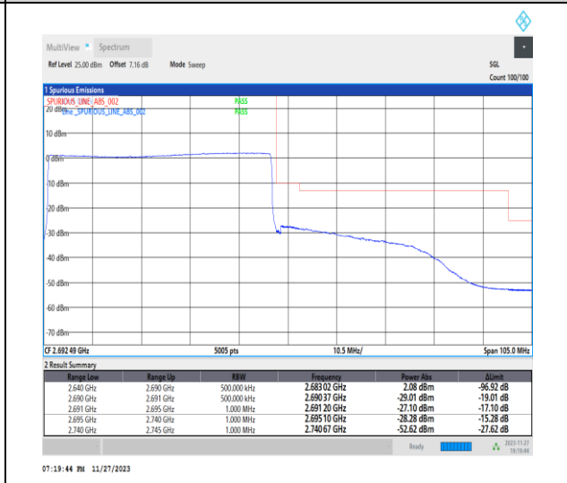
1-N41-PC2-30-50-H-6-CP-QPSK-Outer_Full-133@0-Ant31-1--PASS-see graph
