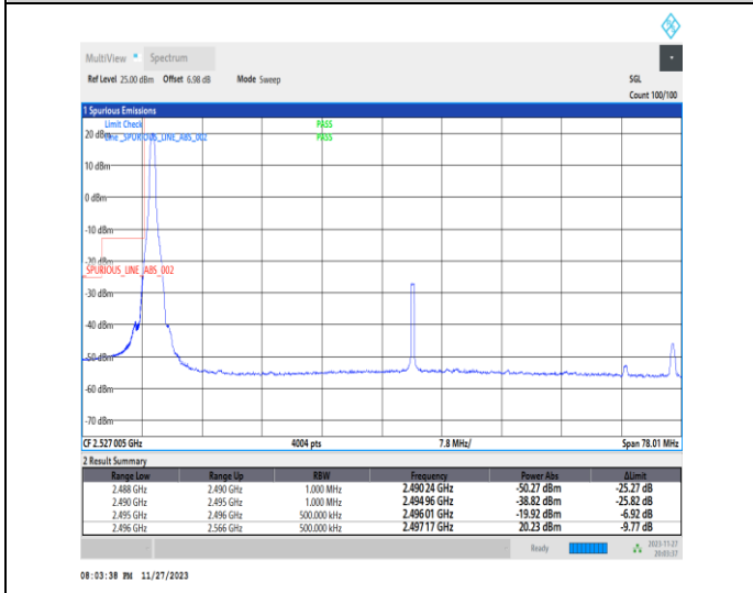
1-N41-PC2-30-70-L-4-CP-QPSK-Edge_1RB_Left-1@0-Ant31-1--PASS-see graph
