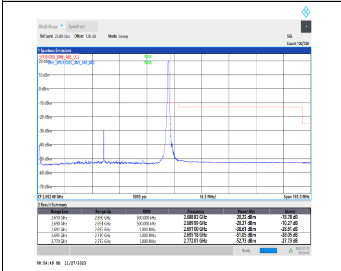
1-N41-PC2-30-80-H-5-CP-QPSK-Edge_1RB_Right-1@216-Ant31-1--PASS-see graph
