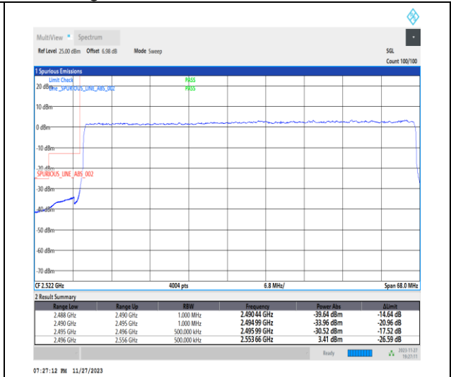
1-N41-PC2-30-60-L-3-DFT-PI2BPSK-Outer_Full-162@0-Ant31-1--PASS-see graph
