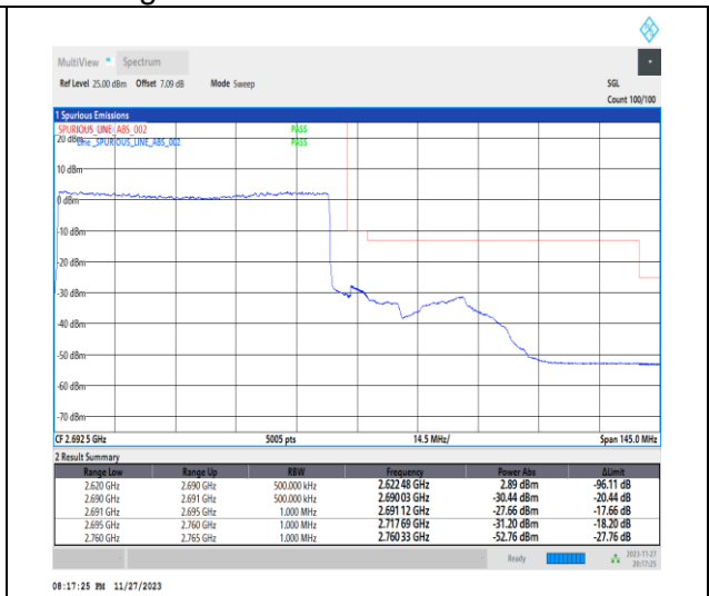
1-N41-PC2-30-70-H-3-DFT-PI2BPSK-Outer_Full-180@0-Ant31-1--PASS-see graph
