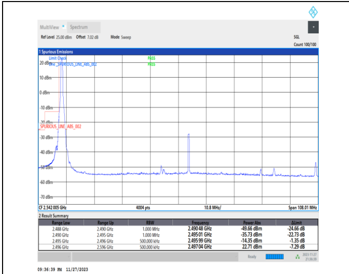
1-N41-PC2-30-100-L-1-DFT-PI2BPSK-Edge_1RB_Left -1@0-Ant31-1--PASS-see graph
