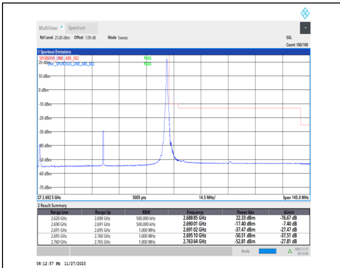
1-N41-PC2-30-70-H-2-DFT-PI2BPSK-Edge_1RB_Right-t-1@188-Ant31-1--PASS-see graph
