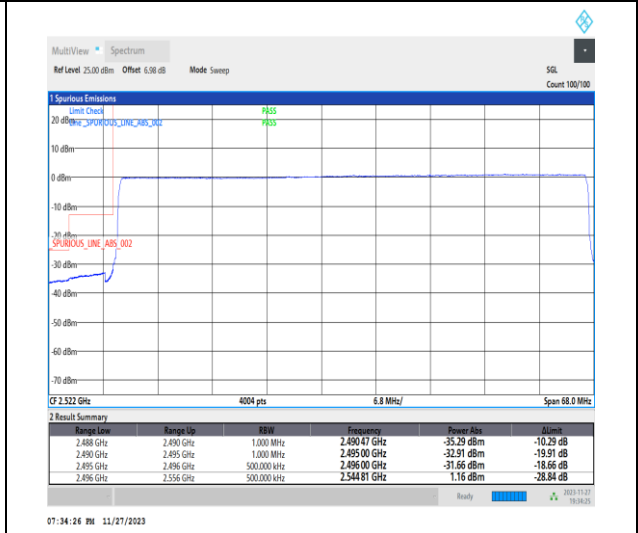
1-N41-PC2-30-60-L-6-CP-QPSK-Outer_Full-162@0-Ant31-1--PASS-see graph
