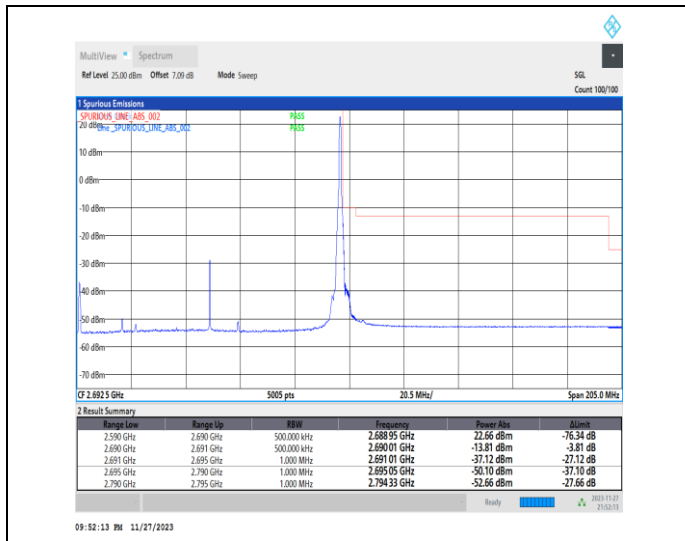
1-N41-PC2-30-100-H-2-DFT-PI2BPSK-Edge_1RB_Rig ht-1@272-Ant31-1--PASS-see graph
