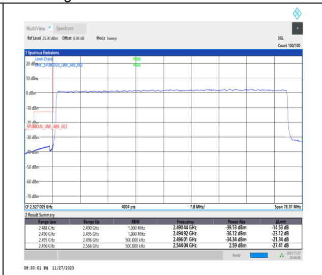
1-N41-PC2-30-70-L-3-DFT-PI2BPSK-Outer_Full-180@0-Ant31-1--PASS-see graph
