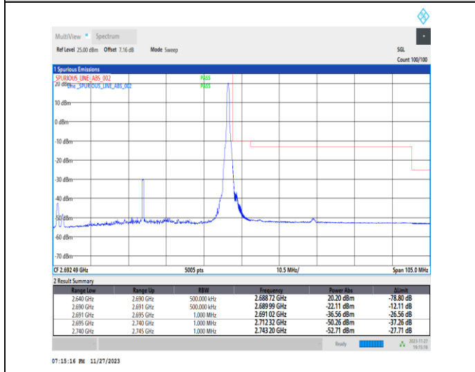
1-N41-PC2-30-50-H-5-CP-QPSK-Edge_1RB_Right-1@132-Ant31-1--PASS-see graph
