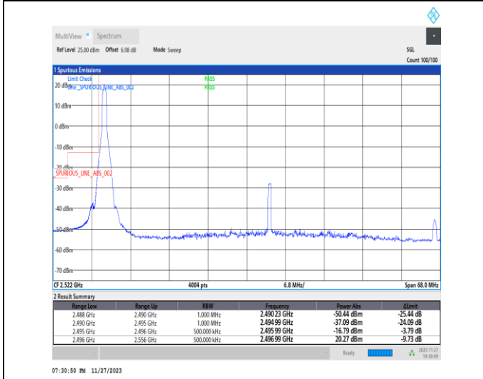
1-N41-PC2-30-60-L-4-CP-QPSK-Edge_1RB_Left-1@0-Ant31-1--PASS-see graph
