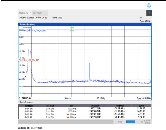
1-N41-PC2-30-100-L-4-CP-QPSK-Edge_1RB_Left1@0-Ant31-1--PASS-see graph
