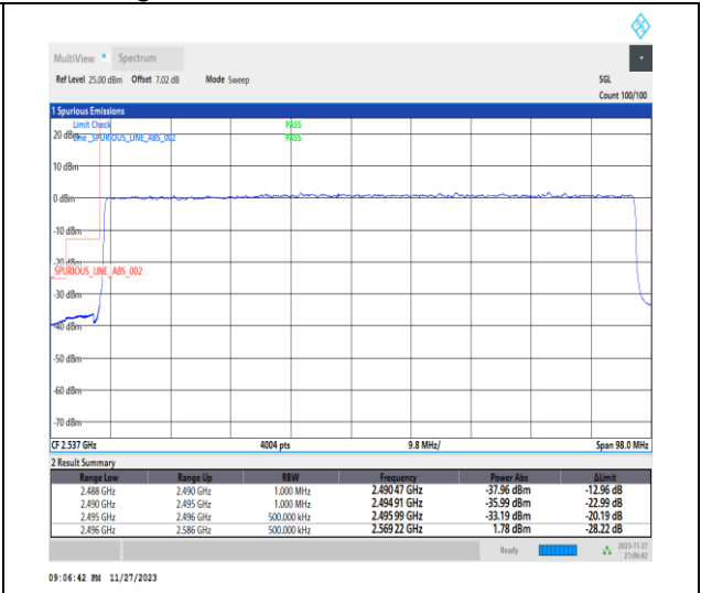
1-N41-PC2-30-90-L-3-DFT-PI2BPSK-Outer_Full-240@0-Ant31-1--PASS-see graph
