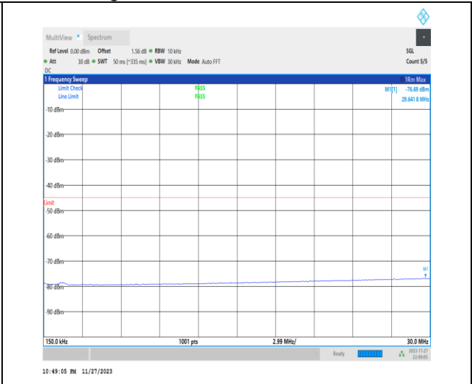
1-N41-PC2-30-100-H-1-DFT-PI2BPSK-Inner_1RB_L eft-1@1-0.15-30-Ant31-28.21--76.69--45-PASS
