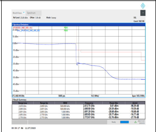
1-N41-PC2-30-80-H-6-CP-QPSK-Outer_Full-217@0-Ant31-1--PASS-see graph
