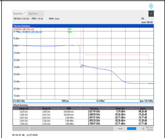
1-N41-PC2-30-70-H-6-CP-QPSK-Outer_Full-189@0-Ant31-1--PASS-see graph
