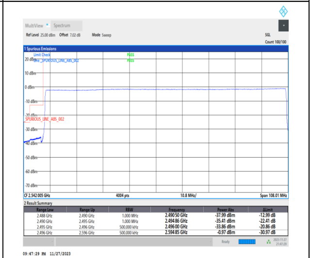
1-N41-PC2-30-100-L-6-CP-QPSK-Outer_Full-273@0-Ant31-1--PASS-see graph
