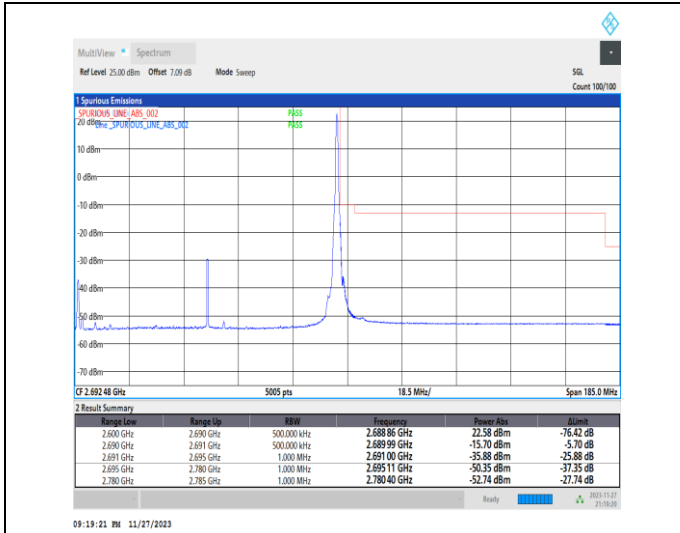
1-N41-PC2-30-90-H-2-DFT-PI2BPSK-Edge_1RB_Right-t-1@244-Ant31-1--PASS-see graph
