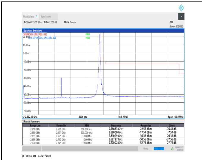
1-N41-PC2-30-80-H-2-DFT-PI2BPSK-Edge_1RB_Right-t-1@216-Ant31-1--PASS-see graph
