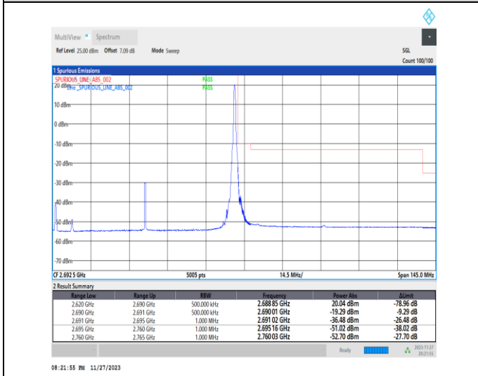
1-N41-PC2-30-70-H-5-CP-QPSK-Edge_1RB_Right-1@188-Ant31-1--PASS-see graph
