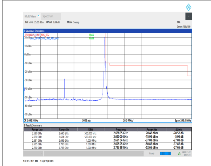
1-N41-PC2-30-100-H-5-CP-QPSK-Edge_1RB_Right-1 @272-Ant31-1--PASS-see graph
