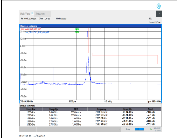
1-N41-PC2-30-90-H-5-CP-QPSK-Edge_1RB_Right-1@244-Ant31-1--PASS-see graph
