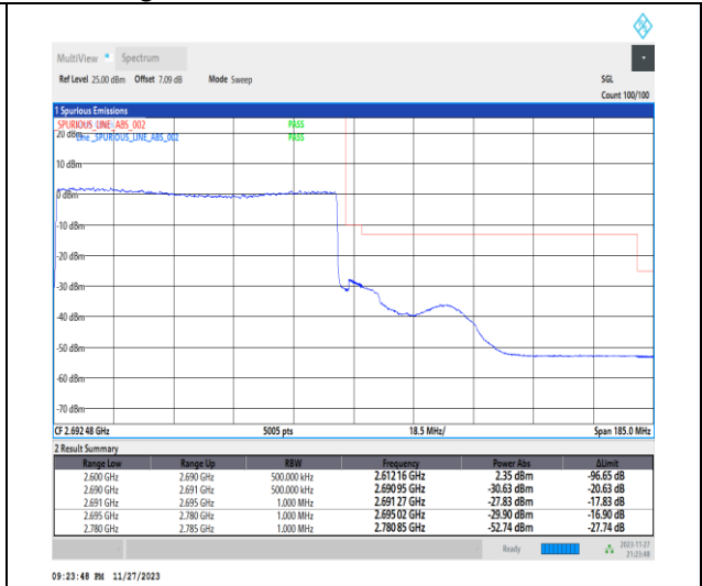
1-N41-PC2-30-90-H-3-DFT-PI2BPSK-Outer_Full-240@0-Ant31-1--PASS-see graph
