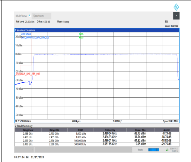
1-N41-PC2-30-70-L-6-CP-QPSK-Outer_Full-189@0-Ant31-1--PASS-see graph
