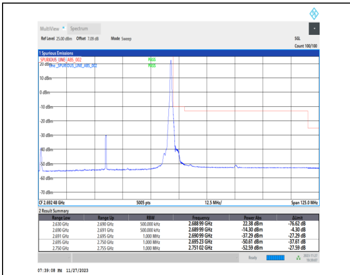
1-N41-PC2-30-60-H-2-DFT-PI2BPSK-Edge_1RB_Right-t-1@161-Ant31-1--PASS-see graph
