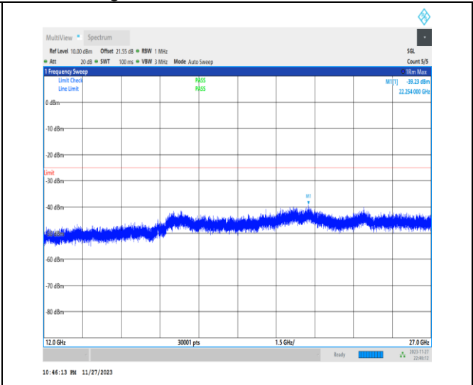
1-N41-PC2-30-100-L-1-DFT-PI2BPSK-Inner_1RB_L eft-1 @ 1-12000-27000-Ant31-24833.50--39.23--25-P ASS
