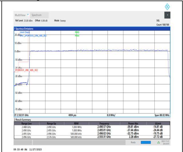
1-N41-PC2-30-80-L-3-DFT-PI2BPSK-Outer_Full-216@0-Ant31-1--PASS-see graph
