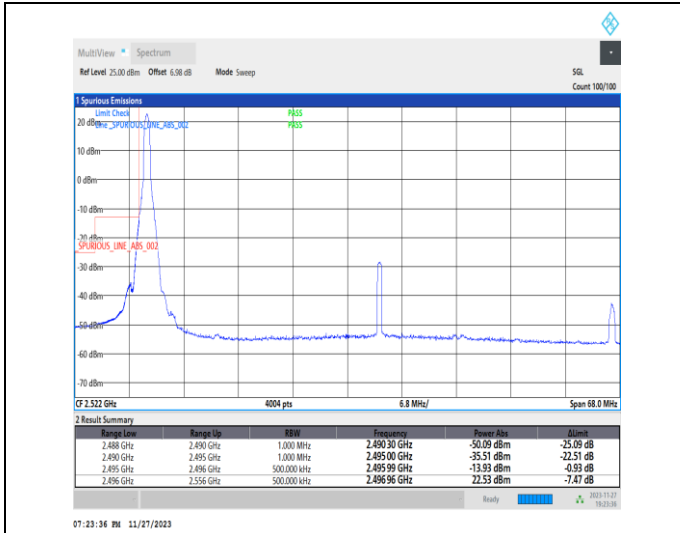
1-N41-PC2-30-60-L-1-DFT-PI2BPSK-Edge_1RB_Left-1@0-Ant31-1--PASS-see graph
