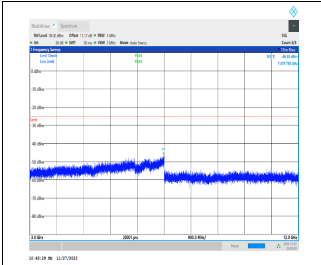
1-N41-PC2-30-100-H-1-DFT-PI2BPSK-Inner_1RB_L eft-1@1-3000-12000-Ant31-5182.95--46.35--25-PAS
