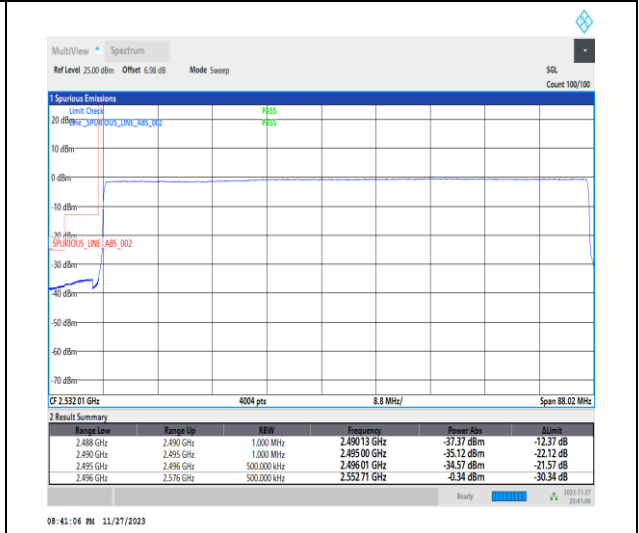
1-N41-PC2-30-80-L-6-CP-QPSK-Outer_Full-217@0-Ant31-1--PASS-see graph
