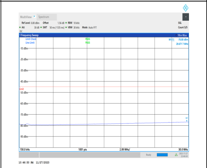
1-N41-PC2-30-100-M-1-DFT-PI2BPSK-Inner_1RB_L eft-1 @ 1-0.15-30-Ant31-22.21--76.80--45-PASS
