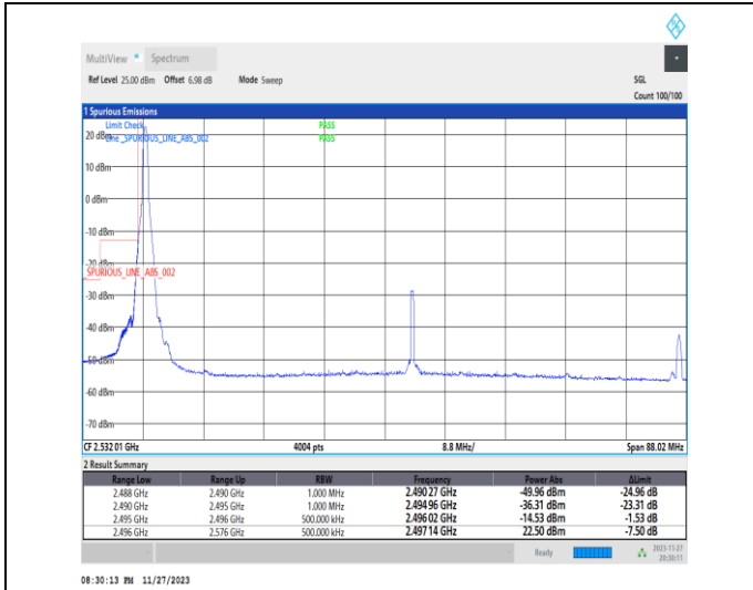
1-N41-PC2-30-80-L-1-DFT-PI2BPSK-Edge_1RB_Left-1@0-Ant31-1--PASS-see graph
