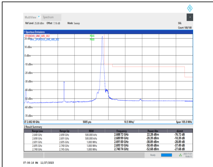
1-N41-PC2-30-50-H-2-DFT-PI2BPSK-Edge_1RB_Right-t-1@132-Ant31-1--PASS-see graph
