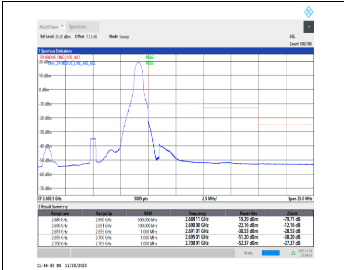
1-N41-PC2-30-10-H-2-DFT-PI2BPSK-Edge_1RB_Righ t-1@23-Ant31-1--PASS-see graph
