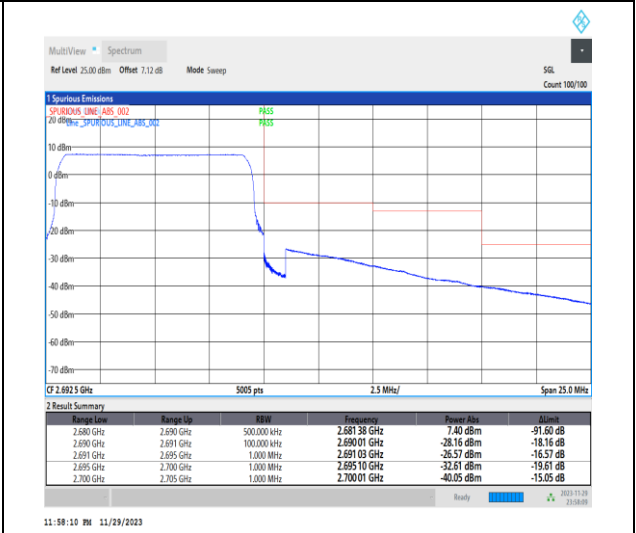
1-N41-PC2-30-10-H-6-CP-QPSK-Outer_Full-24 @0-Ant31-1--PASS-see graph
