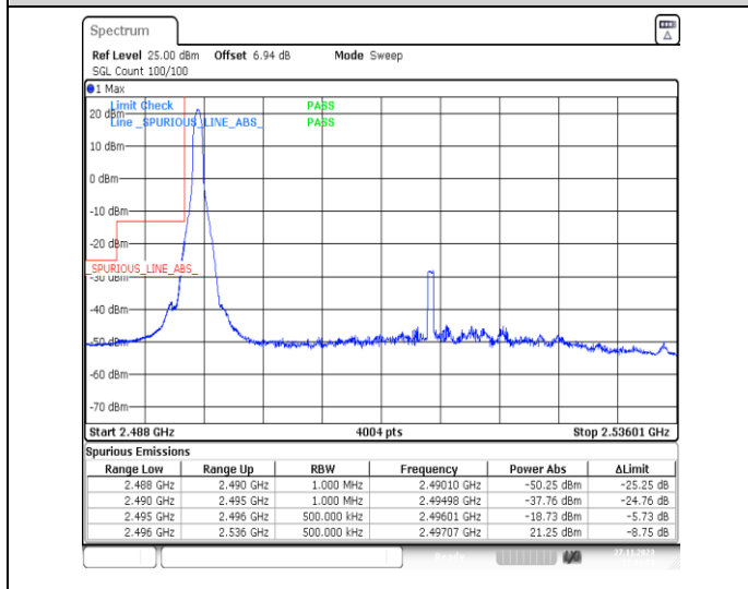
1-N41-PC2-30-40-L-4-CP-QPSK-Edge_1RB_Left-1@0-Ant31-1--PASS-see graph
