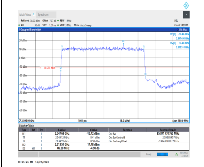
1-N41-PC2-30-90-M-2-DFT-PI2BPSK-Outer_Full-24 @0-Ant31-85.872-89.280-<=90-PASS
