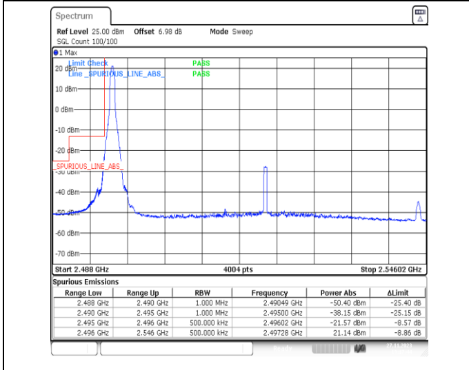
1-N41-PC2-30-50-L-4-CP-QPSK-Edge_1RB_Left-1@0-Ant31-1--PASS-see graph
