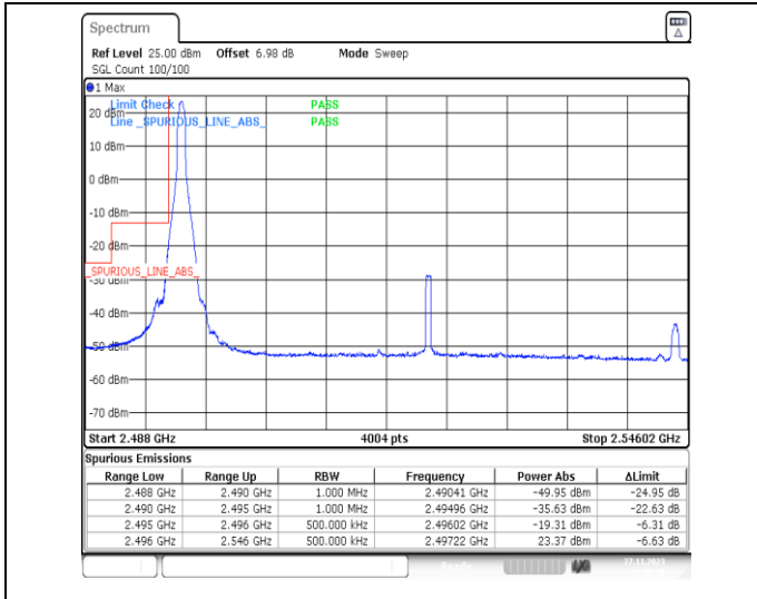
1-N41-PC2-30-50-L-1-DFT-PI2BPSK-Edge_1RB_Left-1@0-Ant31-1--PASS-see graph
