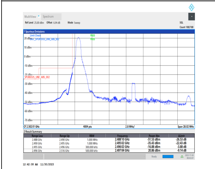
1-N41-PC2-30-20-L-4-CP-QPSK-Edge_1RB_Left-1@0-Ant31-1--PASS-see graph
