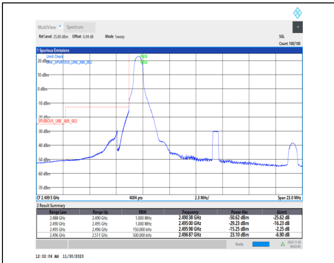
1-N41-PC2-30-15-L-1-DFT-PI2BPSK-Edge_1RB_Left-1@0-Ant31-1--PASS-see graph
