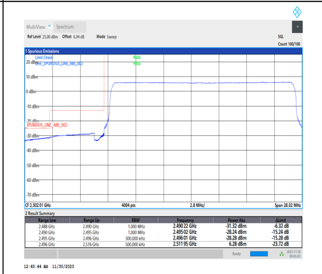
1-N41-PC2-30-20-L-6-CP-QPSK-Outer_Full-51@0-Ant31-1--PASS-see graph
