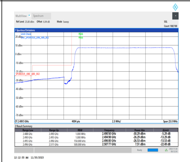
1-N41-PC2-30-15-L-6-CP-QPSK-Outer_Full-38@0-Ant31-1--PASS-see graph
