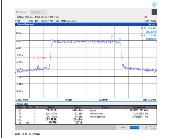
1-N41-PC2-30-60-M-9-CP-256QAM-Outer_Full-162 @0-Ant31-57.787-60.600-≤60-PASS
