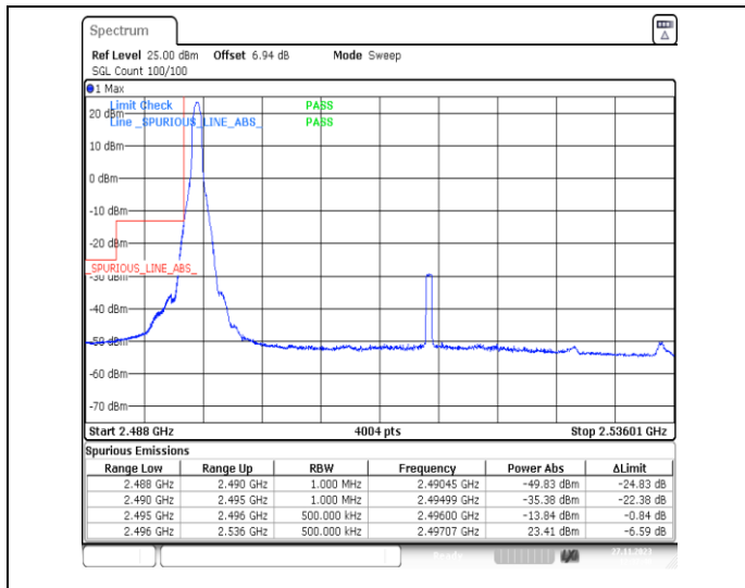
1-N41-PC2-30-40-L-1-DFT-PI2BPSK-Edge_1RB_Left-1@0-Ant31-1--PASS-see graph
