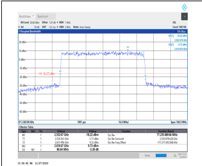
1-N41-PC2-30-80-M-9-CP-256QAM-Outer_Full-217 @0-Ant31-77.235-80.640-<=80-PASS
