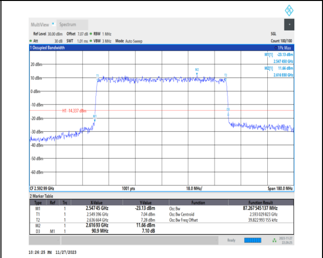
1-N41-PC2-30-90-M-7-CP-16QAM-Outer_Full-245 @0-Ant31-87.268-90.900-<=90-PASS
