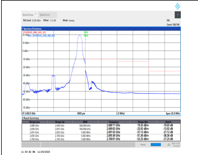
1-N41-PC2-30-10-H-5-CP-QPSK-Edge_1RB_Righ t-1@23-Ant31-1--PASS-see graph
