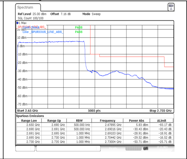
1-N41-PC2-30-40-H-3-DFT-PI2BPSK-Outer_Full-100@0-Ant31-1--PASS-see graph
