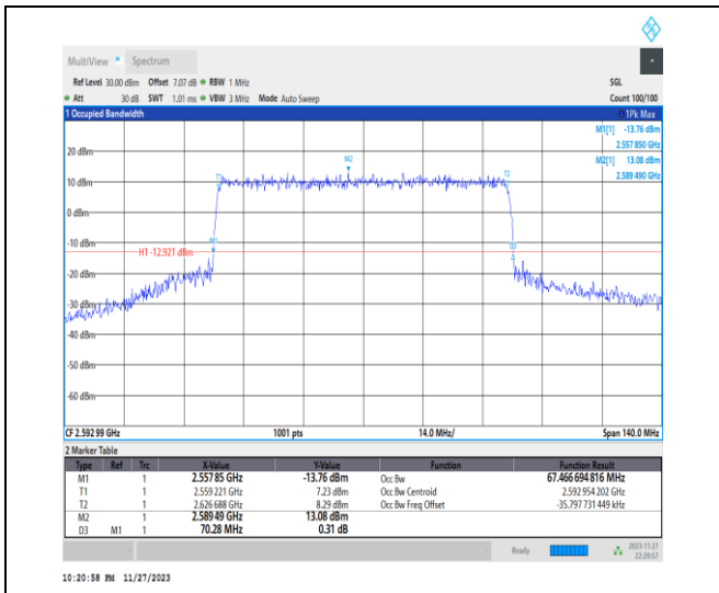
1-N41-PC2-30-70-M-6-CP-QPSK-Outer_Full-189@ 0-Ant31-67.467-70.280-≤70-PASS
