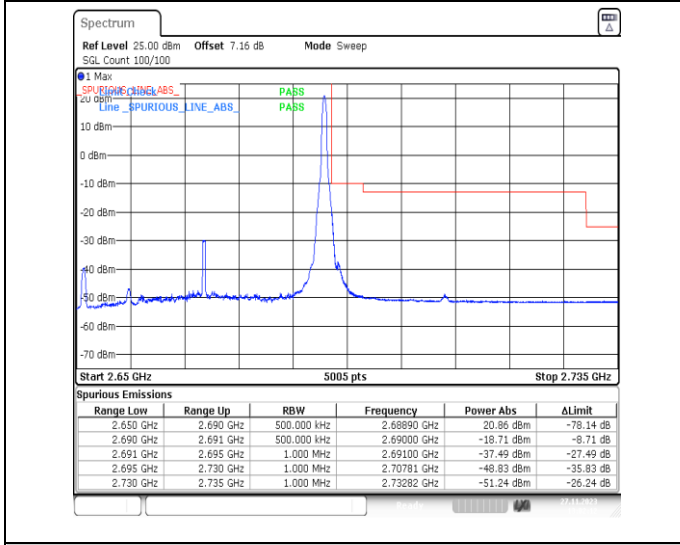
1-N41-PC2-30-40-H-5-CP-QPSK-Edge_1RB_Right-1@105-Ant31-1--PASS-see graph
