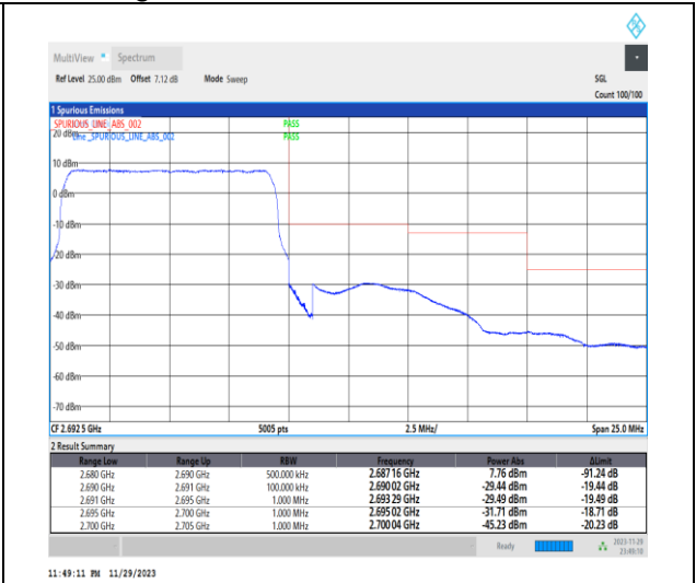
1-N41-PC2-30-10-H-3-DFT-PI2BPSK-Outer_Full-2 4@0-Ant31-1--PASS-see graph
