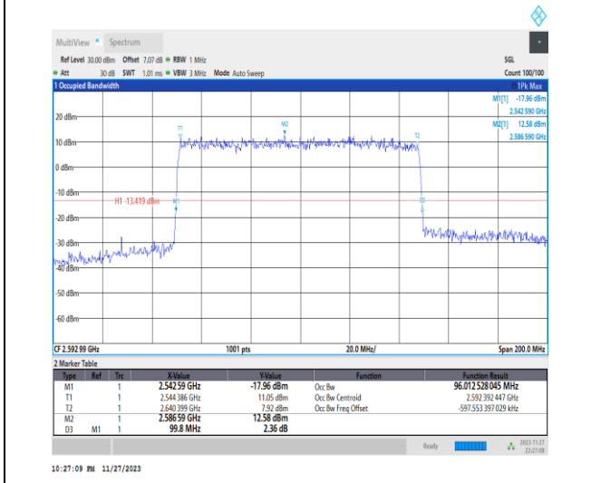
1-N41-PC2-30-100-M-1-DFT-QPSK-Outer_Full-270 @0-Ant31-96.013-99.800-≤100-PASS
