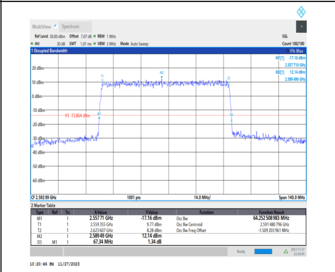
1-N41-PC2-30-70-M-5-DFT-256QAM-Outer_Full-180 @0-Ant31-64.253-67.340-≤70-PASS
