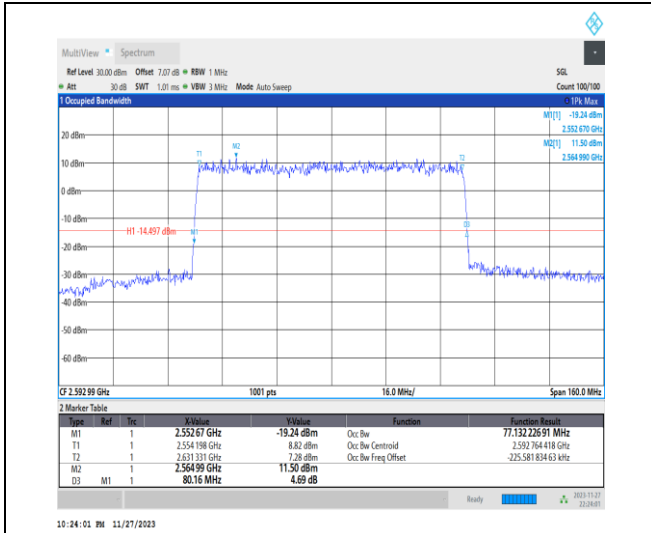
1-N41-PC2-30-80-M-5-DFT-256QAM-Outer_Full-216@0-Ant31-77.132-80.160-≤80-PASS
