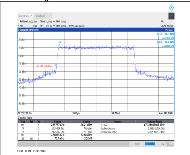
1-N41-PC2-30-70-M-7-CP-16QAM-Outer_Full-189@ 0-Ant31-67.329-70.700-≤70-PASS
