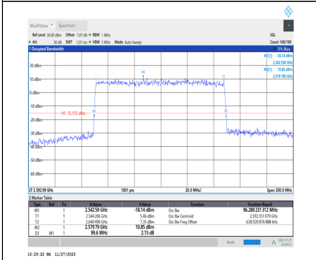
1-N41-PC2-30-100-M-5-DFT-256QAM-Outer_Full-270 70@0-Ant31-96.289-99.600-≤100-PASS
