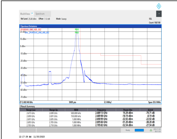
1-N41-PC2-30-15-H-2-DFT-PI2BPSK-Edge_1RB_Righ t-1@37-Ant31-1--PASS-see graph
