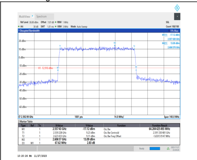
1-N41-PC2-30-70-M-3-DFT-16QAM-Outer_Full-180 @0-Ant31-64.204-67.620-≤70-PASS
