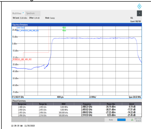
1-N41-PC2-30-20-L-3-DFT-PI2BPSK-Outer_Full-50@0-Ant31-1--PASS-see graph
