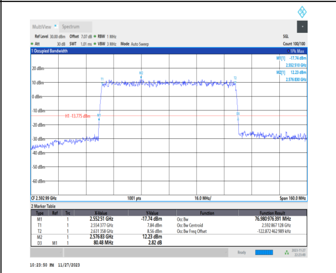
1-N41-PC2-30-80-M-4-DFT-64QAM-Outer_Full-216@0-Ant31-76.981-80.480-≤80-PASS
