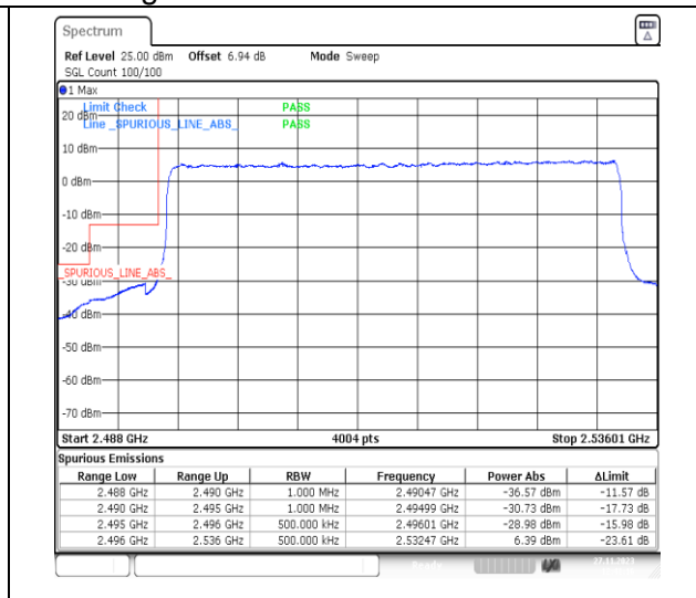
1-N41-PC2-30-40-L-3-DFT-PI2BPSK-Outer_Full-100@0-Ant31-1--PASS-see graph
