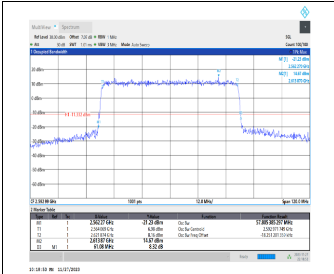
1-N41-PC2-30-60-M-7-CP-16QAM-Outer_Full-162 @0-Ant31-57.805-61.080-≤60-PASS
