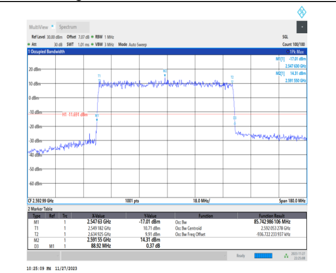
1-N41-PC2-30-90-M-1-DFT-QPSK-Outer_Full-240 @0-Ant31-85.743-88.920-<=90-PASS
