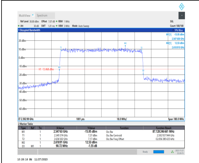
1-N41-PC2-30-90-M-6-CP-QPSK-Outer_Full-245 @0-Ant31-87.128-90.720-<=90-PASS
