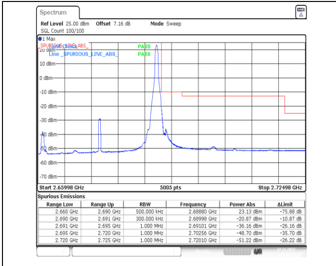
1-N41-PC2-30-30-H-2-DFT-PI2BPSK-Edge_1RB_Righ t-1@77-Ant31-1--PASS-see graph
