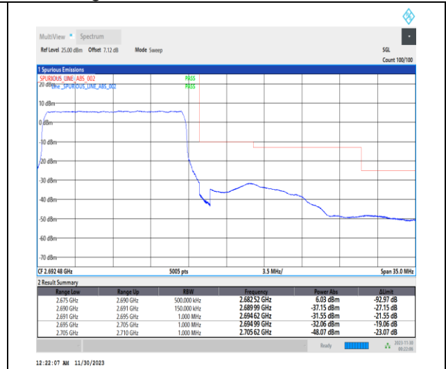
1-N41-PC2-30-15-H-3-DFT-PI2BPSK-Outer_Full-3 6@0-Ant31-1--PASS-see graph
