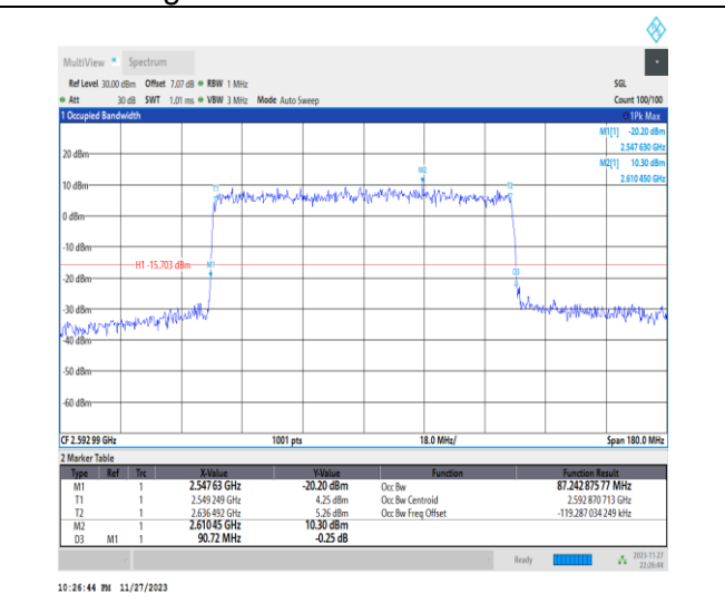
1-N41-PC2-30-90-M-9-CP-256QAM-Outer_Full-245 @0-Ant31-87.243-90.720-≤90-PASS
