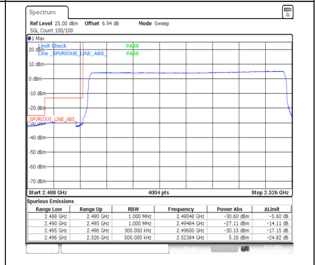
1-N41-PC2-30-30-L-6-CP-QPSK-Outer_Full-78@0-Ant31-1--PASS-see graph
