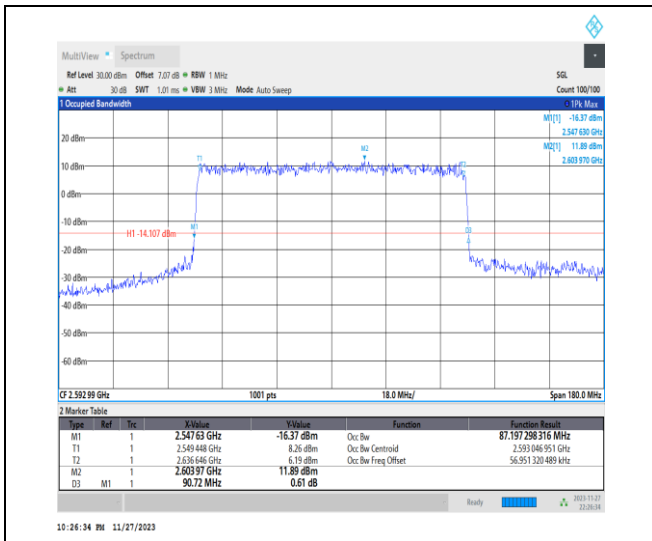
1-N41-PC2-30-90-M-8-CP-64QAM-Outer_Full-245 @0-Ant31-87.197-90.720-≤90-PASS
