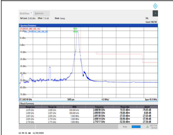
1-N41-PC2-30-20-H-5-CP-QPSK-Edge_1RB_Right-1 @50-Ant31-1--PASS-see graph
