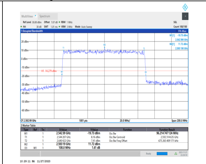
1-N41-PC2-30-100-M-4-DFT-64QAM-Outer_Full-270 @0-Ant31-96.215-100.000-≤100-PASS
