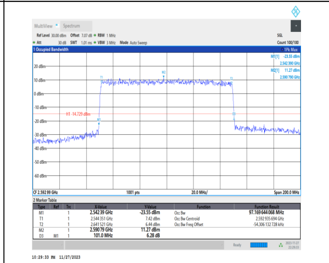
1-N41-PC2-30-100-M-6-CP-QPSK-Outer_Full-273@0 0-Ant31-97.17-101.000-≤100-PASS
