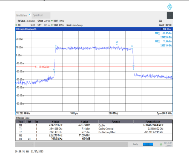
1-N41-PC2-30-100-M-8-CP-64QAM-Outer_Full-273 @0-Ant31-97.185-101.000-≤100-PASS
