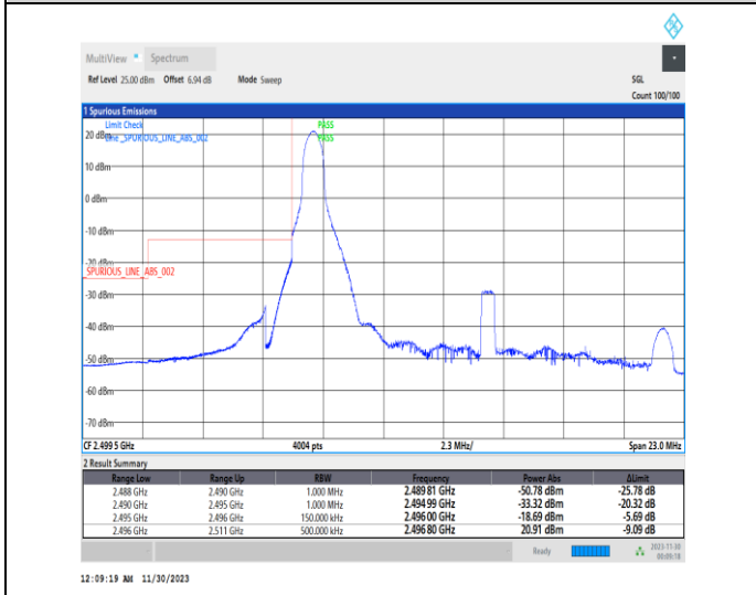
1-N41-PC2-30-15-L-4-CP-QPSK-Edge_1RB_Left-1@0-Ant31-1--PASS-see graph
