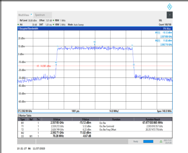
1-N41-PC2-30-70-M-9-CP-256QAM-Outer_Full-189 @0-Ant31-67.477-70.280-≤70-PASS
