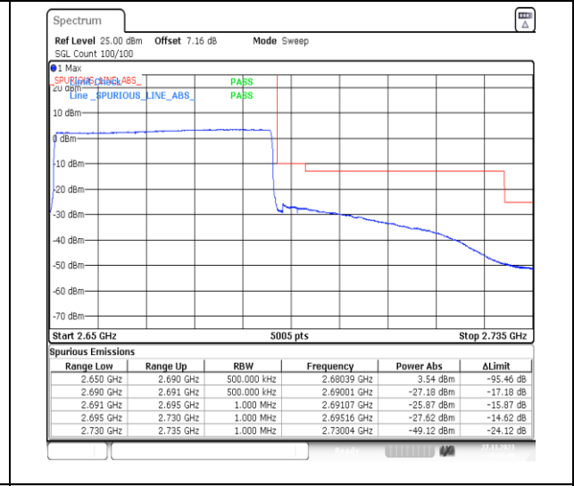
1-N41-PC2-30-40-H-6-CP-QPSK-Outer_Full-106@0-Ant31-1--PASS-see graph
