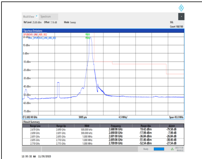
1-N41-PC2-30-20-H-2-DFT-PI2BPSK-Edge_1RB_Righ t-1@50-Ant31-1--PASS-see graph
