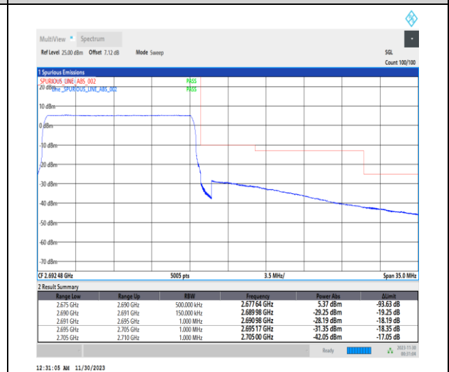
1-N41-PC2-30-15-H-6-CP-QPSK-Outer_Full-38 @0-Ant31-1--PASS-see graph
