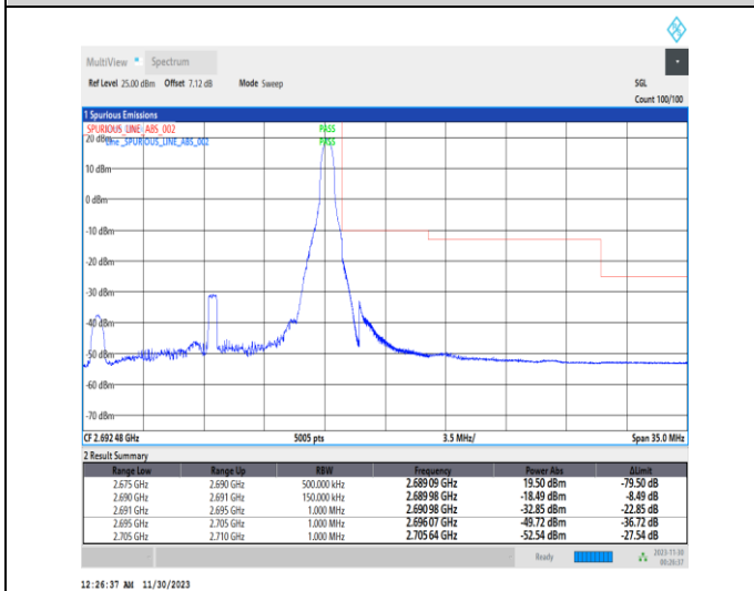
1-N41-PC2-30-15-H-5-CP-QPSK-Edge_1RB_Righ t-1@37-Ant31-1--PASS-see graph
