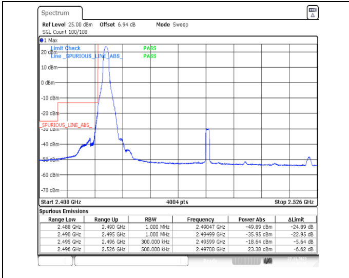
1-N41-PC2-30-30-L-1-DFT-PI2BPSK-Edge_1RB_Left-1@0-Ant31-1--PASS-see graph
