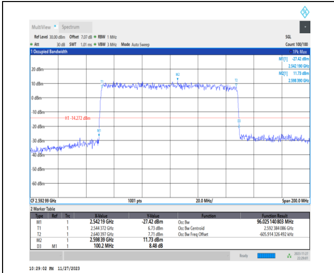
1-N41-PC2-30-100-M-3-DFT-16QAM-Outer_Full-27 0@0-Ant31-96.025-100.200-≤100-PASS
