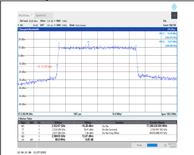
1-N41-PC2-30-80-M-6-CP-QPSK-Outer_Full-217@0-Ant31-77.29-80.800-≤80-PASS
