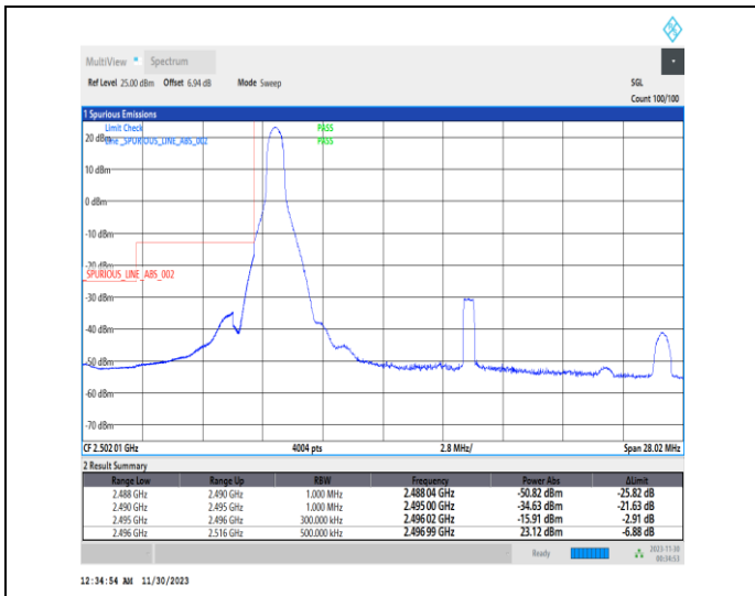
1-N41-PC2-30-20-L-1-DFT-PI2BPSK-Edge_1RB_Left-1@0-Ant31-1--PASS-see graph
