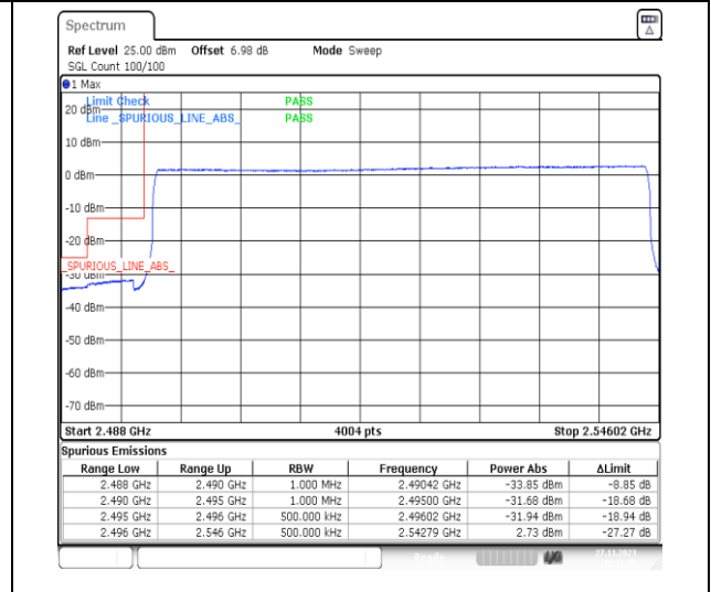
1-N41-PC2-30-50-L-6-CP-QPSK-Outer_Full-133@0-Ant31-1--PASS-see graph
