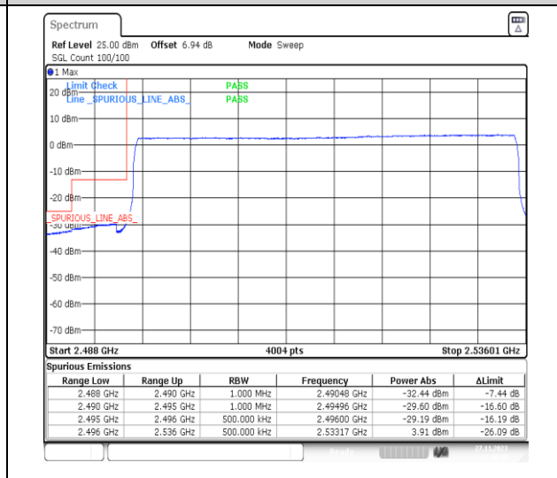
1-N41-PC2-30-40-L-6-CP-QPSK-Outer_Full-106@0-Ant31-1--PASS-see graph
