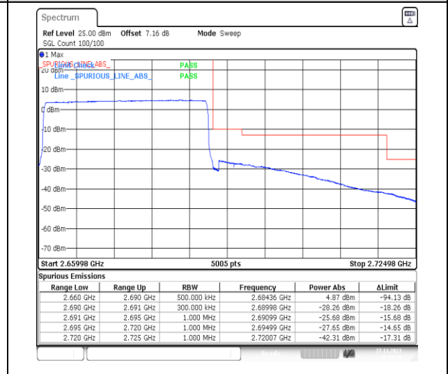
1-N41-PC2-30-30-H-6-CP-QPSK-Outer_Full-78@ 0-Ant31-1--PASS-see graph
