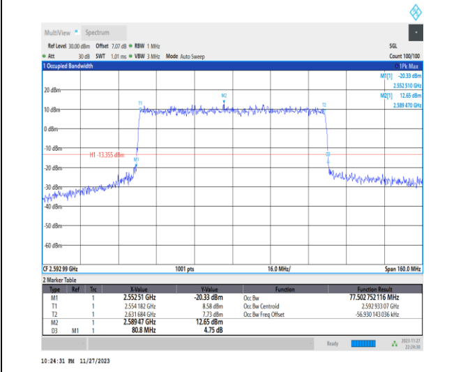
1-N41-PC2-30-80-M-8-CP-64QAM-Outer_Full-217@0-Ant31-77.503-80.800-≤80-PASS
