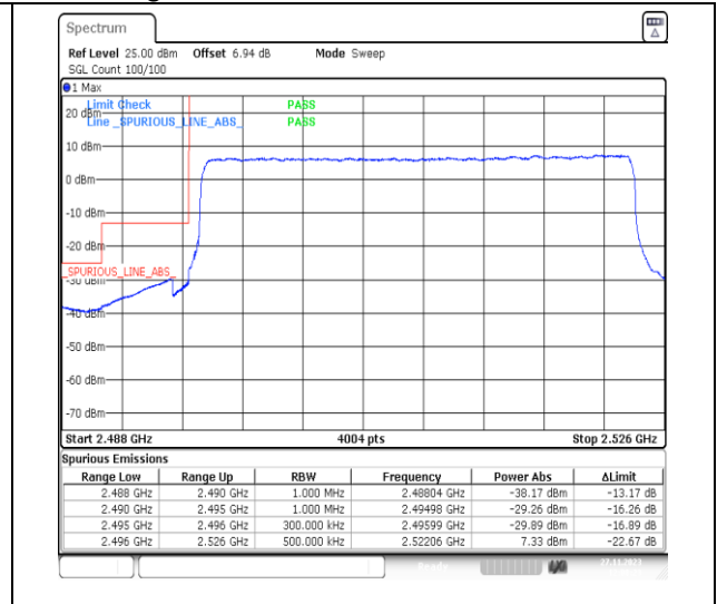
1-N41-PC2-30-30-L-3-DFT-PI2BPSK-Outer_Full-75@0-Ant31-1--PASS-see graph
