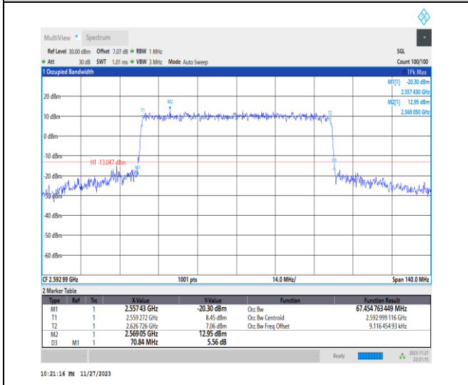
1-N41-PC2-30-70-M-8-CP-64QAM-Outer_Full-189 @0-Ant31-67.455-70.840-≤70-PASS
