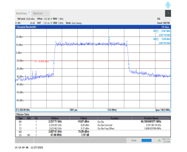
1-N41-PC2-30-70-M-1-DFT-QPSK-Outer_Full-180 @0-Ant31-64.161-67.480-≤70-PASS
