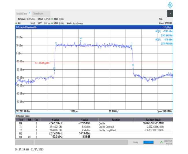
1-N41-PC2-30-100-M-2-DFT-PI2BPSK-Outer_Full-270 @0-Ant31-96.066-100.000-≤100-PASS
