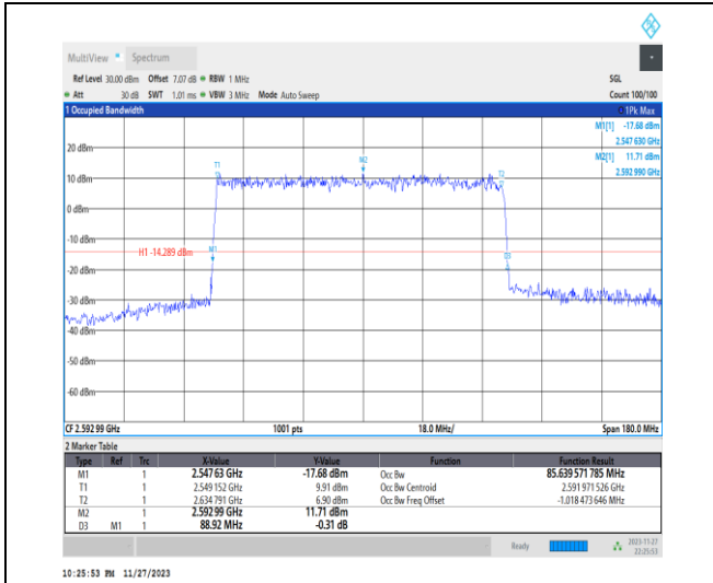
1-N41-PC2-30-90-M-4-DFT-64QAM-Outer_Full-240 @0-Ant31-85.64-88.920-<=90-PASS
