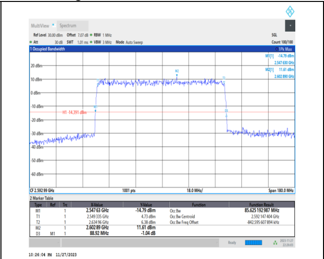
1-N41-PC2-30-90-M-5-DFT-256QAM-Outer_Full-240 @0-Ant31-85.625-88.920-<=90-PASS
