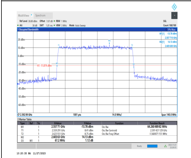
1-N41-PC2-30-70-M-4-DFT-64QAM-Outer_Full-180 @0-Ant31-64.26-67.200-≤70-PASS
