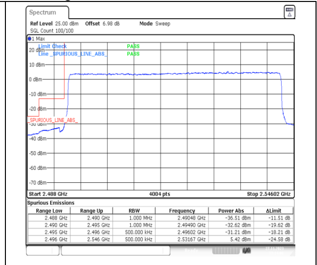
1-N41-PC2-30-50-L-3-DFT-PI2BPSK-Outer_Full-128@0-Ant31-1--PASS-see graph
