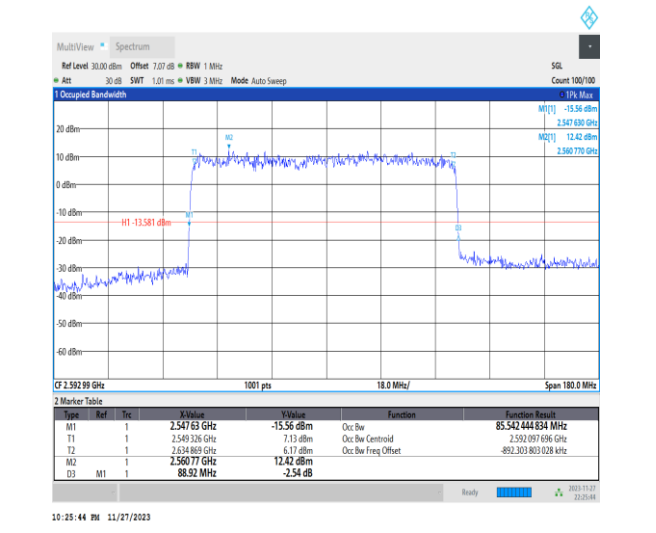
1-N41-PC2-30-90-M-3-DFT-16QAM-Outer_Full-240 @0-Ant31-85.542-88.920-<=90-PASS
