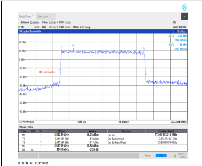
1-N41-PC2-30-100-M-7-CP-16QAM-Outer_Full-273 @0-Ant31-97.299-101.000-≤100-PASS
