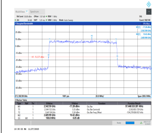
1-N41-PC2-30-100-M-9-CP-256QAM-Outer_Full-27 3@0-Ant31-97.448-100.800-≤100-PASS
