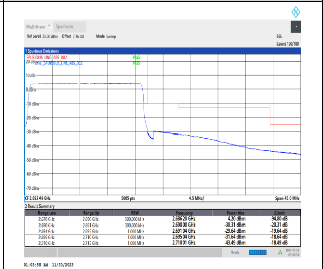
1-N41-PC2-30-20-H-6-CP-QPSK-Outer_Full-51 @ 0-Ant31-1--PASS-see graph
