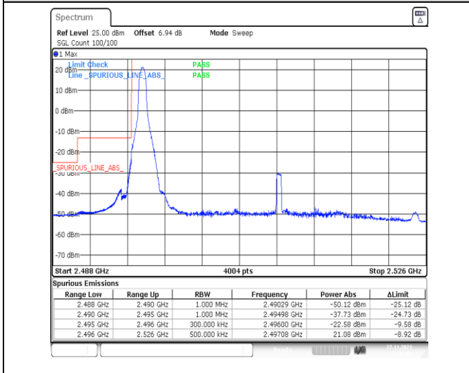
1-N41-PC2-30-30-L-4-CP-QPSK-Edge_1RB_Left-1@0-Ant31-1--PASS-see graph
