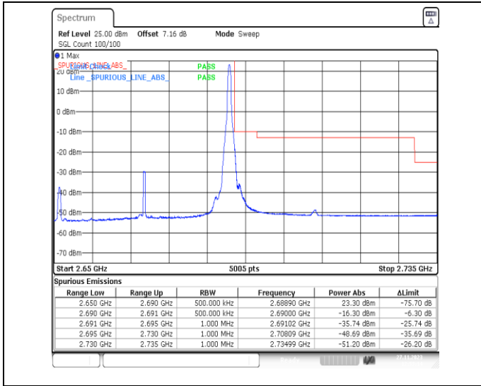
1-N41-PC2-30-40-H-2-DFT-PI2BPSK-Edge_1RB_Right-t-1@105-Ant31-1--PASS-see graph
