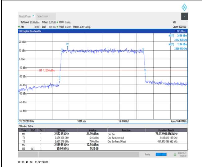
1-N41-PC2-30-80-M-3-DFT-16QAM-Outer_Full-216@0-Ant31-76.913-80.640-≤80-PASS
