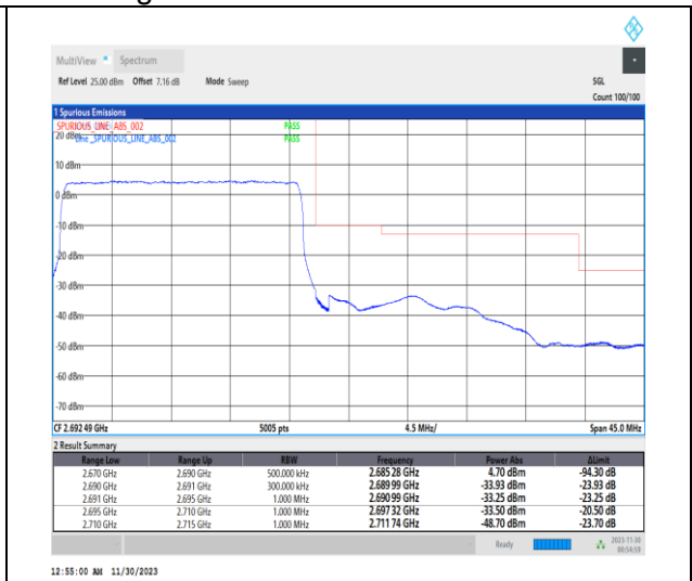
1-N41-PC2-30-20-H-3-DFT-PI2BPSK-Outer_Full-5 0@0-Ant31-1--PASS-see graph
