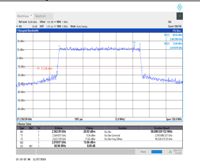
1-N41-PC2-30-60-M-8-CP-64QAM-Outer_Full-162 @0-Ant31-58.098-60.960-≤60-PASS
