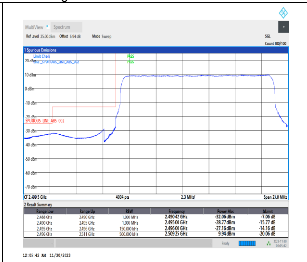
1-N41-PC2-30-15-L-3-DFT-PI2BPSK-Outer_Full-36@0-Ant31-1--PASS-see graph
