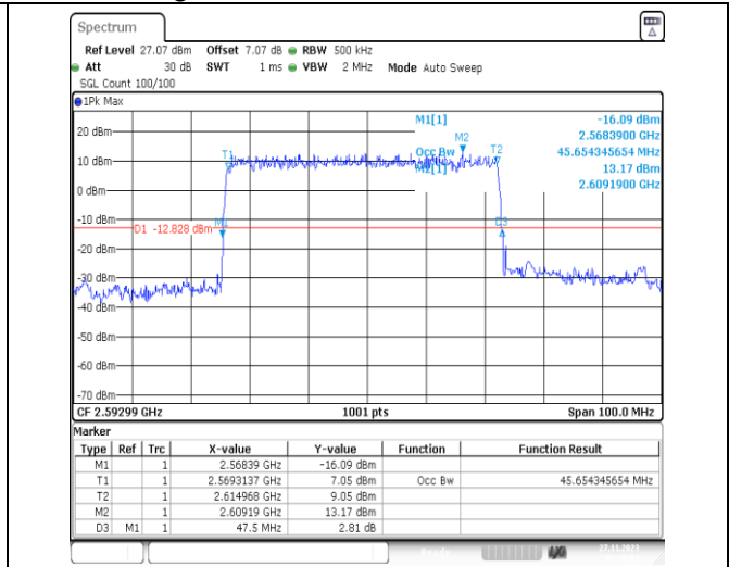
1-N41-PC2-30-50-M-1-DFT-QPSK-Outer_Full-128@ 0-Ant31-45.654-47.500-<=50-PASS
