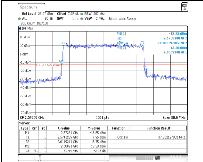
1-N41-PC2-30-40-M-7-CP-16QAM-Outer_Full-106 @0-Ant31-37.802-39.440-≤40-PASS
