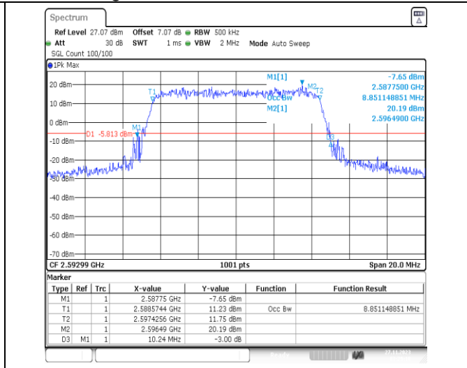
1-N41-PC2-30-10-M-6-CP-QPSK-Outer_Full-24 @0-Ant31-8.851-10.240-≤10-PASS
