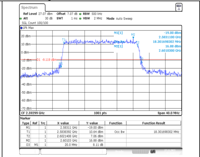
1-N41-PC2-30-20-M-8-CP-64QAM-Outer_Full-51@0- Ant31-18.302-20.000-<=20-PASS
