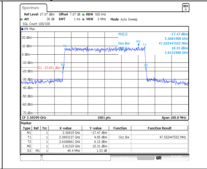
1-N41-PC2-30-50-M-9-CP-256QAM-Outer_Full-133 @0-Ant31-47.552-49.400-≤50-PASS
