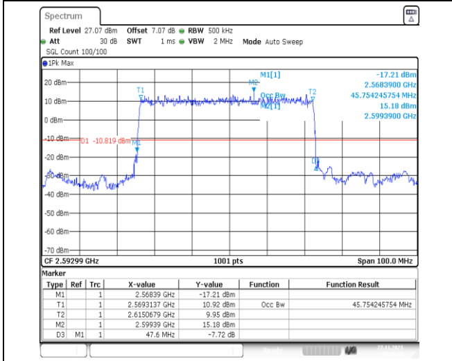
1-N41-PC2-30-50-M-2-DFT-PI2BPSK-Outer_Full-12 8@0-Ant31-45.754-47.600-<=50-PASS
