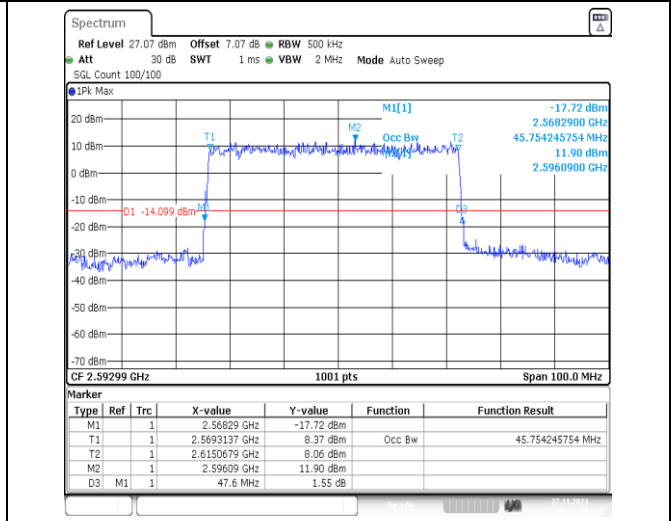
1-N41-PC2-30-50-M-3-DFT-16QAM-Outer_Full-128 @0-Ant31-45.754-47.600-<=50-PASS
