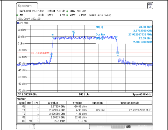
1-N41-PC2-30-30-M-9-CP-256QAM-Outer_Full-78@0-Ant31-27.932-29.400-≤30-PASS
