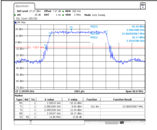
1-N41-PC2-30-15-M-2-DFT-PI2BPSK-Outer_Full-36 @0-Ant31-13.067-14.880-≤15-PASS
