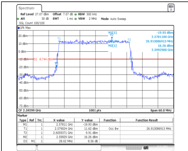
1-N41-PC2-30-30-M-2-DFT-PI2BPSK-Outer_Full-75 @0-Ant31-26.913-28.620-≤30-PASS
