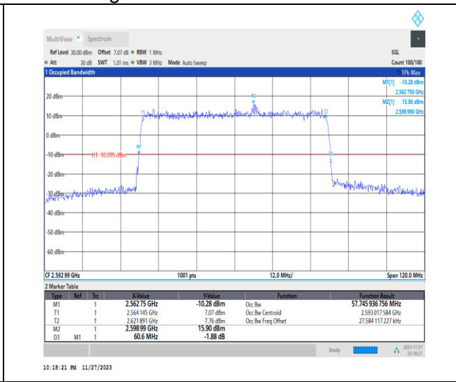
1-N41-PC2-30-60-M-4-DFT-64QAM-Outer_Full-162 @0-Ant31-57.746-60.600-≤60-PASS
