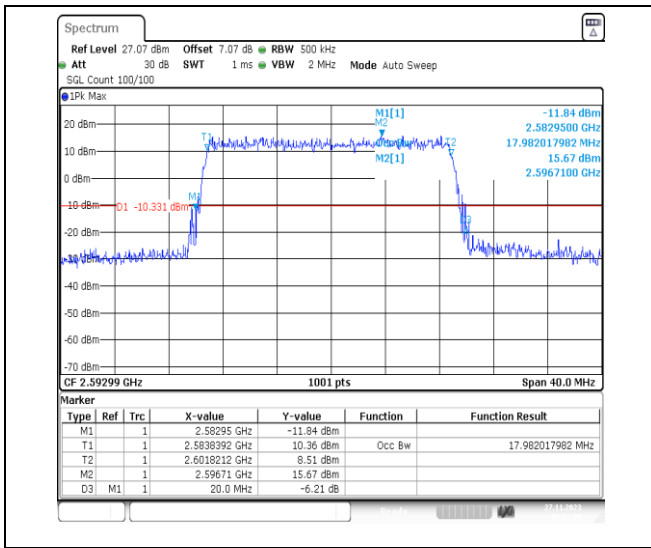
1-N41-PC2-30-20-M-3-DFT-16QAM-Outer_Full-50 @0-Ant31-17.982-20.000-≤20-PASS
