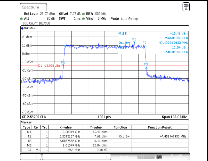
1-N41-PC2-30-50-M-7-CP-16QAM-Outer_Full-133 @0-Ant31-47.453-49.400-≤50-PASS
