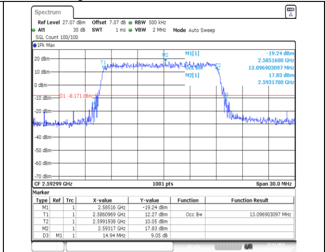
1-N41-PC2-30-15-M-1-DFT-QPSK-Outer_Full-36@0-Ant31-13.097-14.940-≤15-PASS
