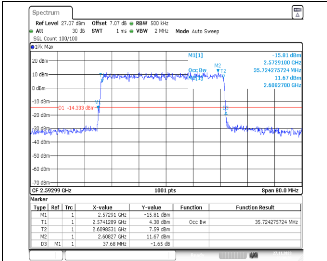
1-N41-PC2-30-40-M-5-DFT-256QAM-Outer_Full-10 @0-Ant31-35.724-37.680-≤40-PASS
