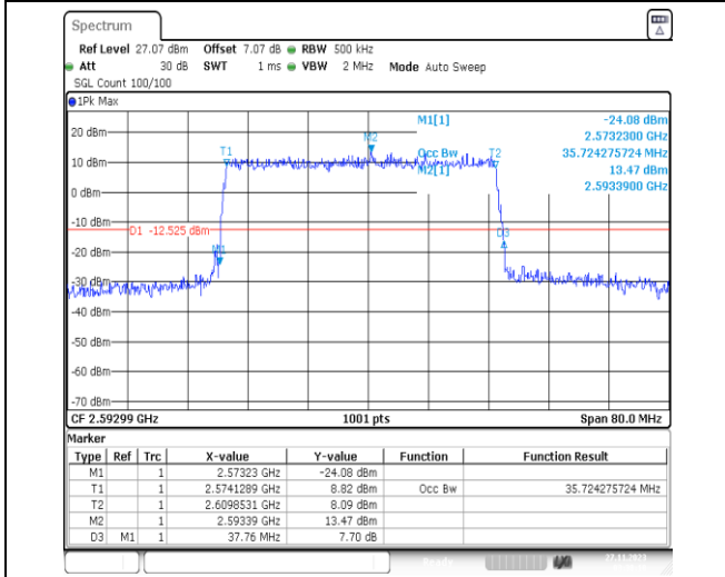
1-N41-PC2-30-40-M-3-DFT-16QAM-Outer_Full-100@0-Ant31-35.724-37.760-≤40-PASS
