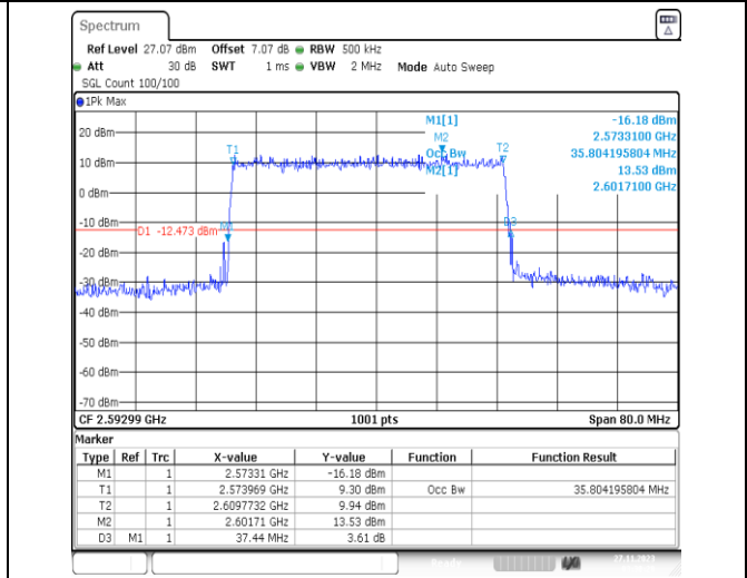
1-N41-PC2-30-40-M-4-DFT-64QAM-Outer_Full-100@0-Ant31-35.804-37.440-≤40-PASS
