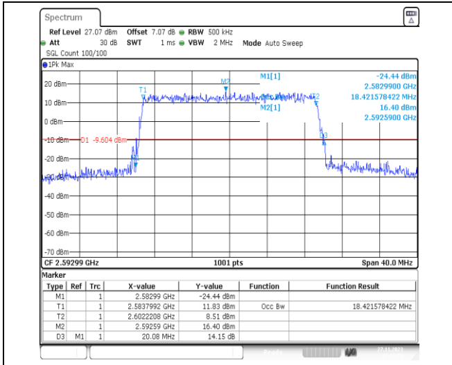
1-N41-PC2-30-20-M-7-CP-16QAM-Outer_Full-51@ 0-Ant31-18.422-20.080-<=20-PASS
