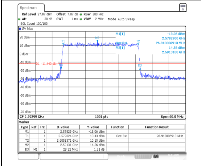
1-N41-PC2-30-30-M-4-DFT-64QAM-Outer_Full-75 @0-Ant31-26.913-28.320-≤30-PASS
