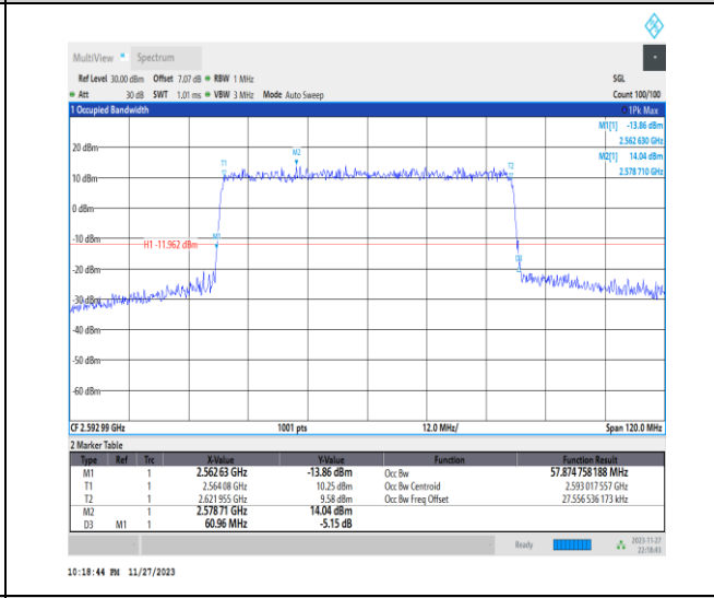
1-N41-PC2-30-60-M-6-CP-QPSK-Outer_Full-162 @0-Ant31-57.875-60.960-≤60-PASS
