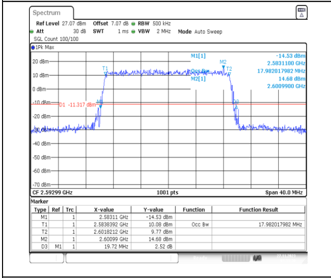
1-N41-PC2-30-20-M-5-DFT-256QAM-Outer_Full-50 @0-Ant31-17.982-19.720-≤20-PASS
