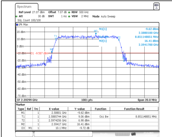
1-N41-PC2-30-10-M-9-CP-256QAM-Outer_Full-24 @0-Ant31-8.851-10.100-≤10-PASS
