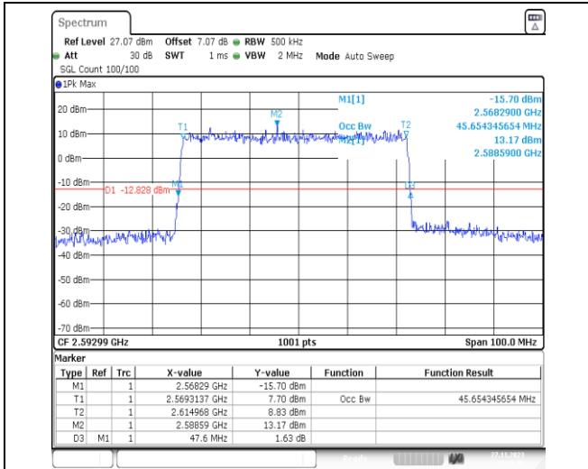
1-N41-PC2-30-50-M-4-DFT-64QAM-Outer_Full-128 @0-Ant31-45.654-47.600-≤50-PASS
