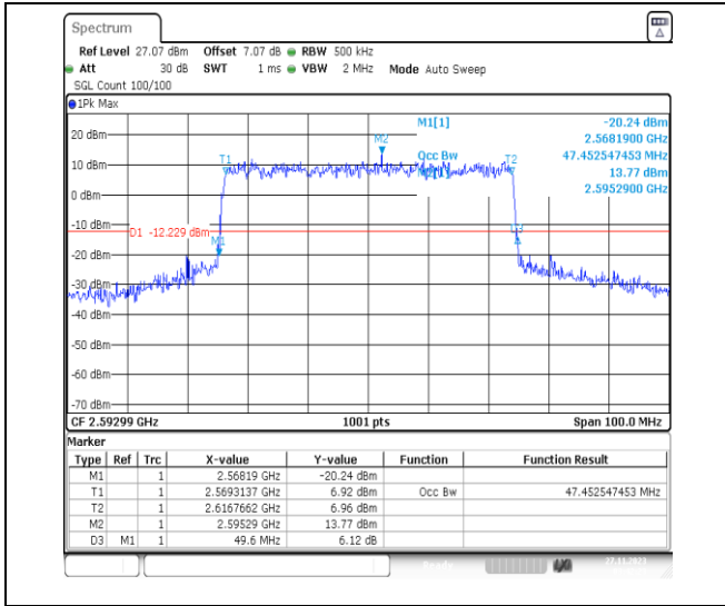
1-N41-PC2-30-50-M-8-CP-64QAM-Outer_Full-133 @0-Ant31-47.453-49.600-≤50-PASS
