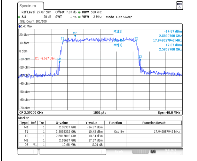
1-N41-PC2-30-20-M-1-DFT-QPSK-Outer_Full-50@0-Ant31-17.942-19.680-≤20-PASS
