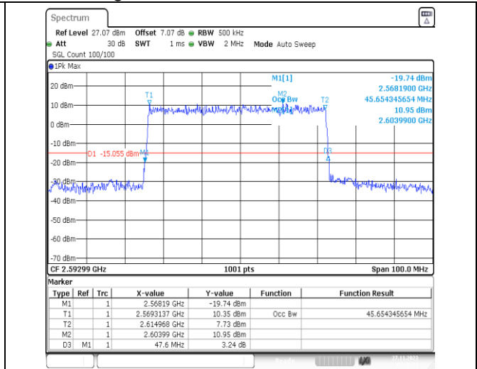
1-N41-PC2-30-50-M-5-DFT-256QAM-Outer_Full-128 @0-Ant31-45.654-47.600-≤50-PASS
