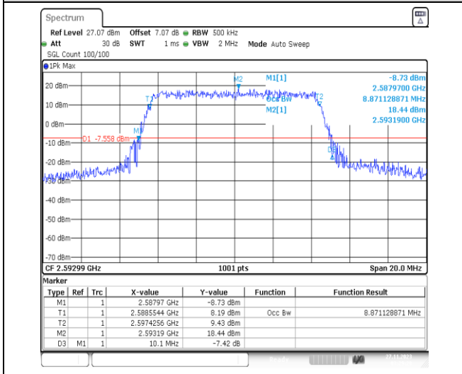
1-N41-PC2-30-10-M-7-CP-16QAM-Outer_Full-24 @0-Ant31-8.871-10.100-≤10-PASS
