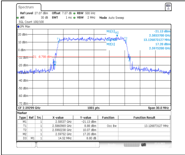
1-N41-PC2-30-15-M-4-DFT-64QAM-Outer_Full-36 @0-Ant31-13.127-14.520-≤15-PASS
