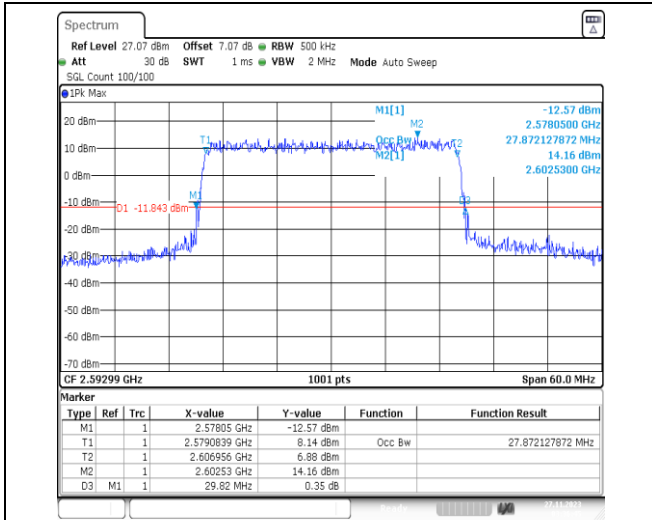
1-N41-PC2-30-30-M-6-CP-QPSK-Outer_Full-78@0-Ant31-27.872-29.820-≤30-PASS
