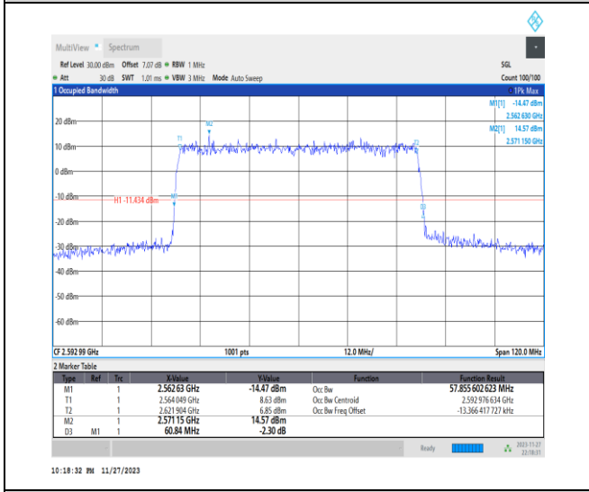
1-N41-PC2-30-60-M-5-DFT-256QAM-Outer_Full-16 @0-Ant31-57.856-60.840-≤60-PASS
