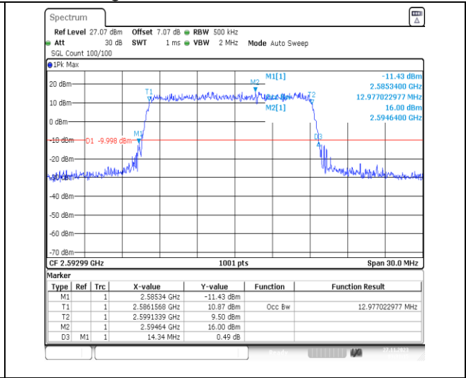
1-N41-PC2-30-15-M-5-DFT-256QAM-Outer_Full-36 @0-Ant31-12.977-14.340-≤15-PASS
