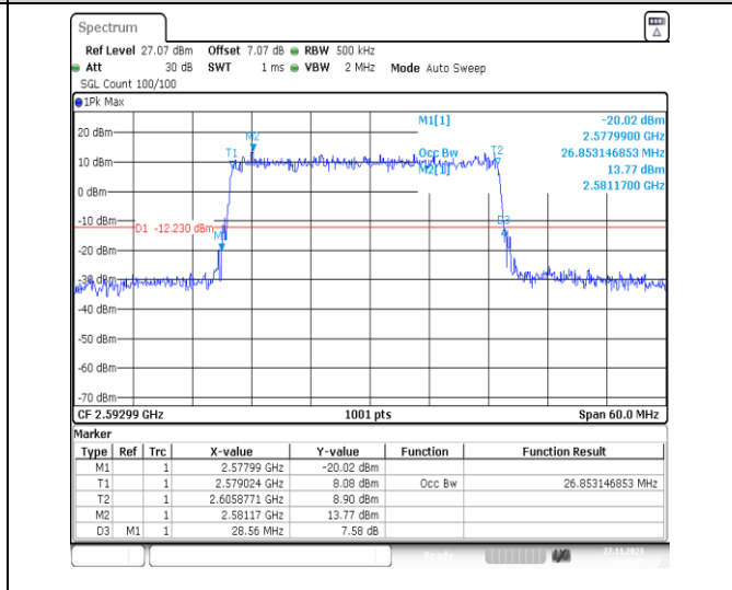
1-N41-PC2-30-30-M-5-DFT-256QAM-Outer_Full-75 @0-Ant31-26.853-28.560-≤30-PASS
