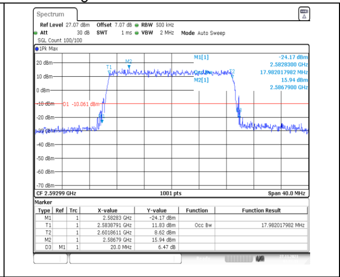
1-N41-PC2-30-20-M-4-DFT-64QAM-Outer_Full-50 @0-Ant31-17.982-20.000-≤20-PASS
