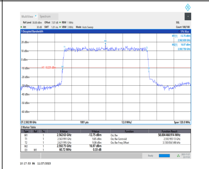
1-N41-PC2-30-60-M-2-DFT-PI2BPSK-Outer_Full-162 @0-Ant31-58.004-60.720-≤60-PASS
