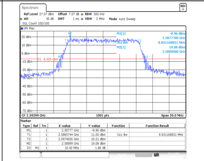
1-N41-PC2-30-10-M-8-CP-64QAM-Outer_Full-24 @0-Ant31-8.831-10.420-≤10-PASS
