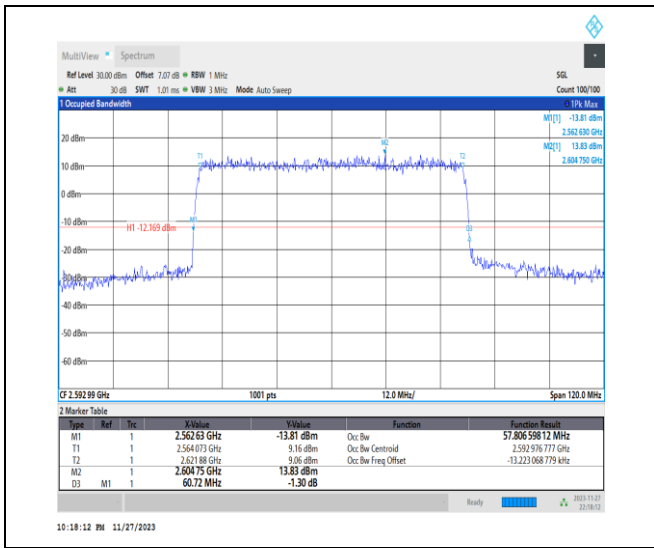
1-N41-PC2-30-60-M-3-DFT-16QAM-Outer_Full-162 @0-Ant31-57.807-60.720-≤60-PASS
