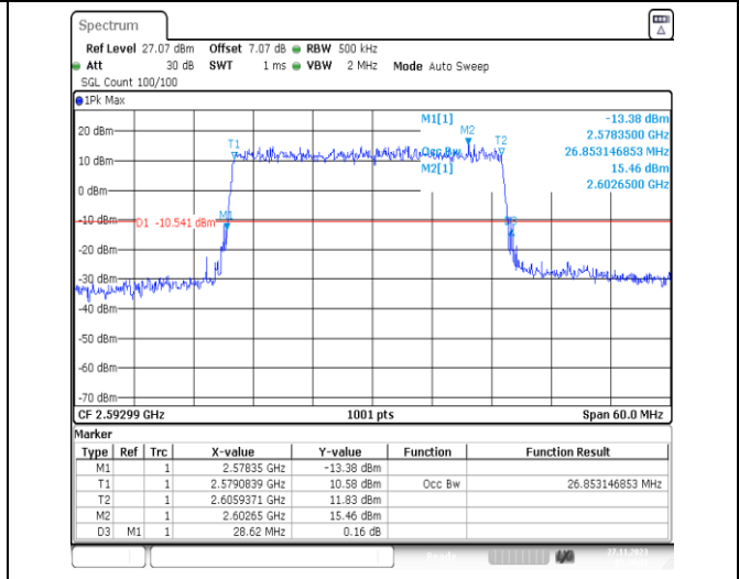
1-N41-PC2-30-30-M-1-DFT-QPSK-Outer_Full-75@0- Ant31-26.853-28.620-<=30-PASS
