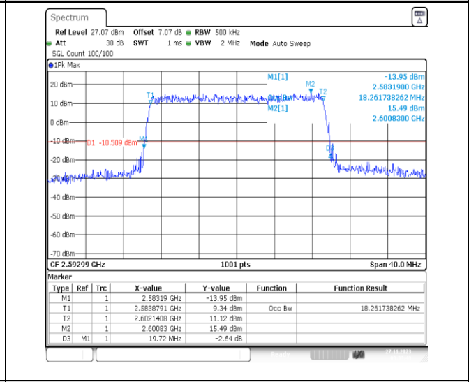
1-N41-PC2-30-20-M-6-CP-QPSK-Outer_Full-51 @0-Ant31-18.262-19.720-≤20-PASS
