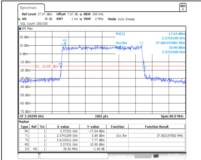
1-N41-PC2-30-40-M-9-CP-256QAM-Outer_Full-106 @0-Ant31-37.802-39.920-<=40-PASS
