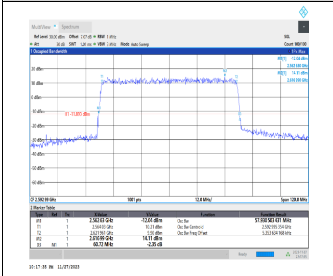
1-N41-PC2-30-60-M-1-DFT-QPSK-Outer_Full-162 @0-Ant31-57.931-60.720-≤60-PASS
