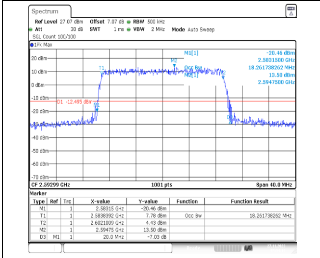
1-N41-PC2-30-20-M-9-CP-256QAM-Outer_Full-51 @0-Ant31-18.262-20.000-<=20-PASS
