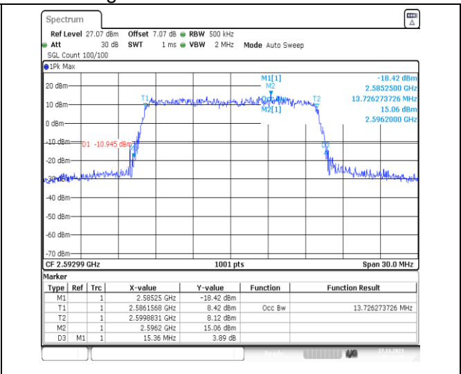
1-N41-PC2-30-15-M-9-CP-256QAM-Outer_Full-38@0-Ant31-13.726-15.360-≤15-PASS
