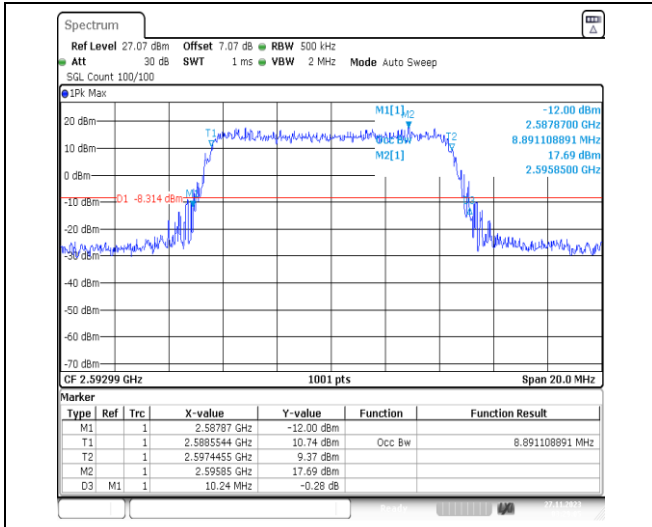
1-N41-PC2-30-10-M-5-DFT-256QAM-Outer_Full-24 @0-Ant31-8.891-10.240-≤10-PASS
