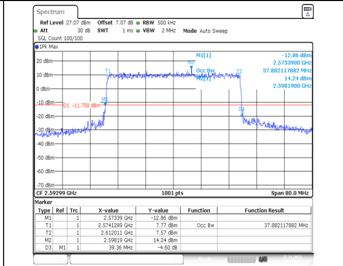
1-N41-PC2-30-40-M-8-CP-64QAM-Outer_Full-106 @0-Ant31-37.882-39.360-≤40-PASS
