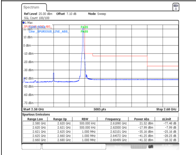
1-N38-PC3-30-40-H-5-CP-QPSK-Edge_1RB_Right-1@105-Ant31-1--PASS-see graph
