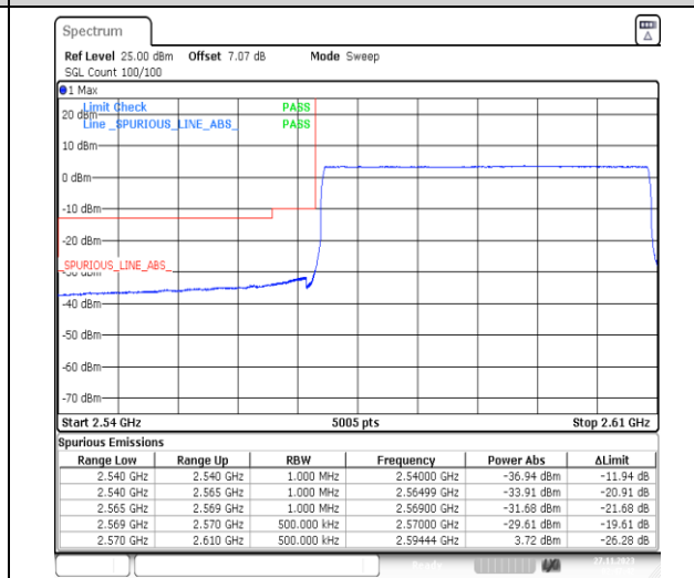
1-N38-PC3-30-40-L-6-CP-QPSK-Outer_Full-106@0-Ant31-1--PASS-see graph
