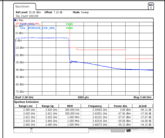
1-N38-PC3-30-40-H-6-CP-QPSK-Outer_Full-106@0-Ant31-1--PASS-see graph
