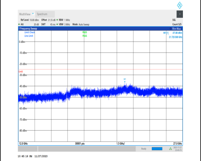
1-N38-PC3-30-40-M-1-DFT-PI2BPSK-Inner_1RB_Lef t-1 @ 1-12000-27000-Ant31-15106.00--37.08--25-PAS S
