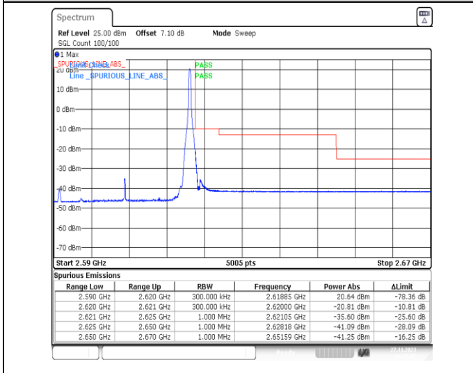
1-N38-PC3-30-30-H-5-CP-QPSK-Edge_1RB_Right-1 @77-Ant31-1--PASS-see graph
