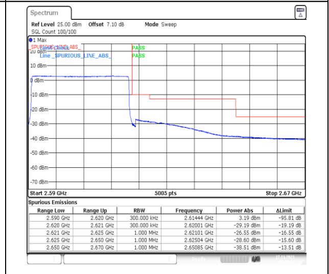
1-N38-PC3-30-30-H-6-CP-QPSK-Outer_Full-78@ 0-Ant31-1--PASS-see graph
