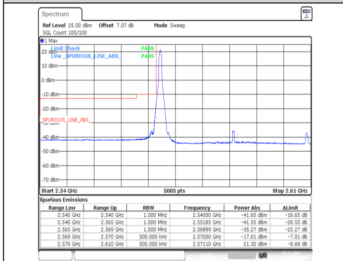
1-N38-PC3-30-40-L-4-CP-QPSK-Edge_1RB_Left-1@0-Ant31-1--PASS-see graph
