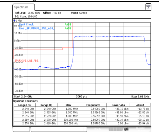
1-N38-PC3-30-40-L-3-DFT-PI2BPSK-Outer_Full-100@0-Ant31-1--PASS-see graph
