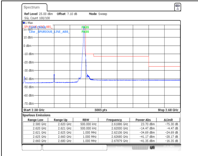
1-N38-PC3-30-40-H-2-DFT-PI2BPSK-Edge_1RB_Right-t-1@105-Ant31-1--PASS-see graph
