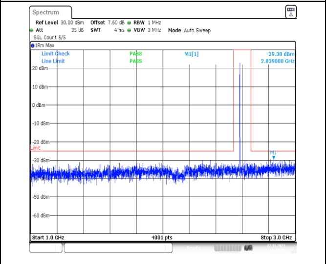
1-N38-PC3-30-40-H-1-DFT-PI2BPSK-Inner_1RB_Lef t-1@1-1000-3000-Ant31-2839.00--29.38--25-PASS
