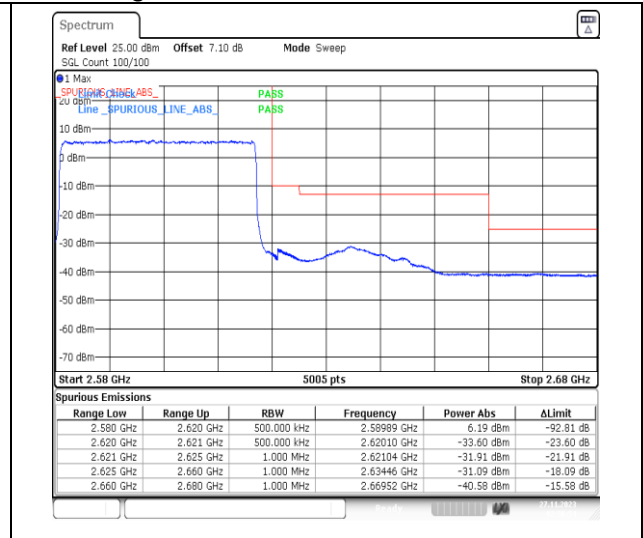
1-N38-PC3-30-40-H-3-DFT-PI2BPSK-Outer_Full-100@0-Ant31-1--PASS-see graph
