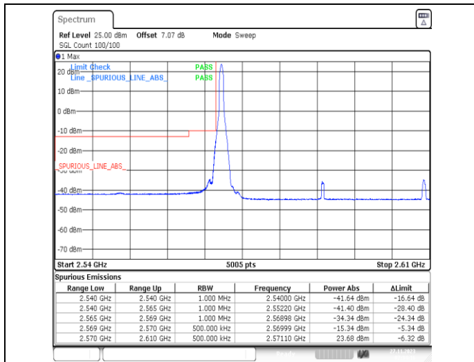
1-N38-PC3-30-40-L-1-DFT-PI2BPSK-Edge_1RB_Left-1@0-Ant31-1--PASS-see graph
