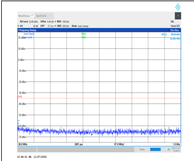
1-N38-PC3-30-40-M-1-DFT-PI2BPSK-Inner_1RB_L eft-1 @ 1-30-1000-Ant31-866.14--58.64--35-PASS
