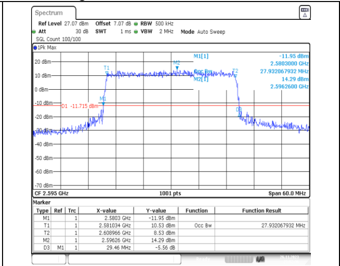
1-N38-PC3-30-30-M-7-CP-16QAM-Outer_Full-78@0-Ant31-27.932-29.460-≤30-PASS
