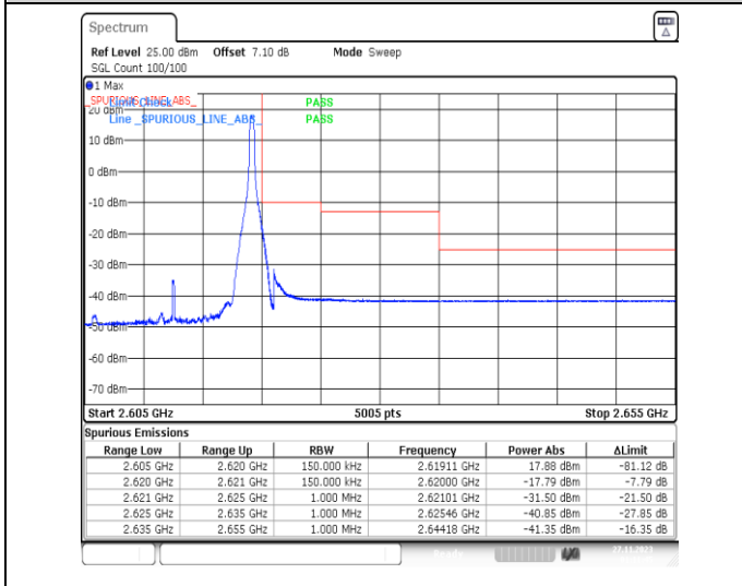
1-N38-PC3-30-15-H-5-CP-QPSK-Edge_1RB_Right-1@37-Ant31-1--PASS-see graph
