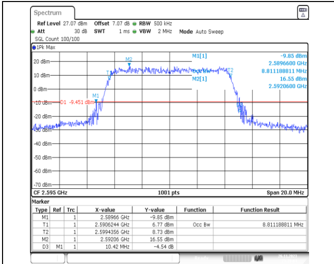
1-N38-PC3-30-10-M-9-CP-256QAM-Outer_Full-24@ 0-Ant31-8.811-10.420-≤10-PASS
