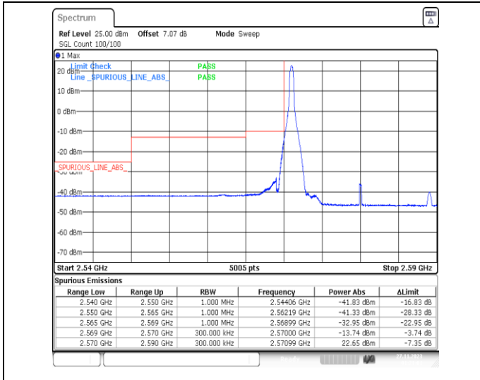
1-N38-PC3-30-20-L-1-DFT-PI2BPSK-Edge_1RB_Left-1@0-Ant31-1--PASS-see graph
