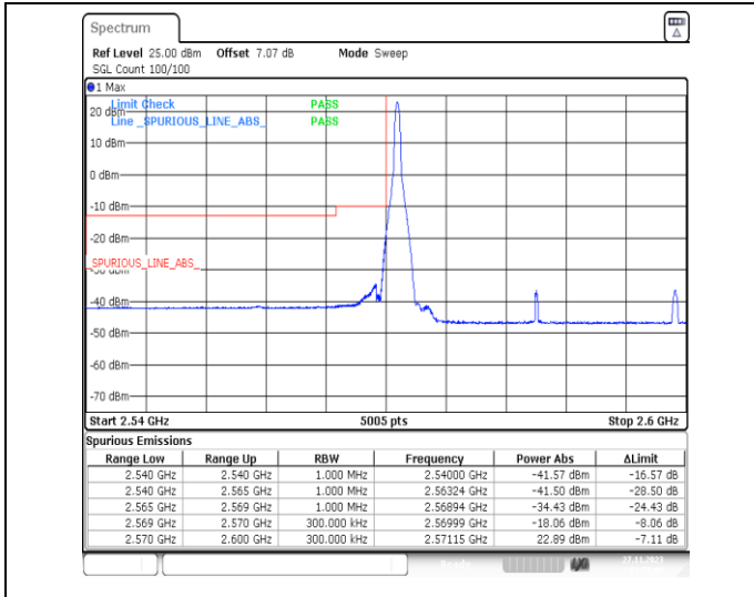
1-N38-PC3-30-30-L-1-DFT-PI2BPSK-Edge_1RB_Left-1@0-Ant31-1--PASS-see graph
