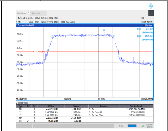
1-N38-PC3-30-15-M-1-DFT-QPSK-Outer_Full-36@ 0-Ant31-13.505-15.510-≤15-PASS
