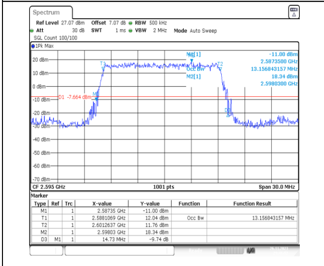
1-N38-PC3-30-15-M-2-DFT-PI2BPSK-Outer_Full-36 @0-Ant31-13.157-14.730-≤15-PASS
