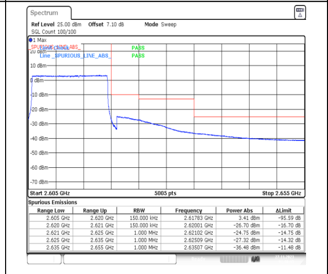
1-N38-PC3-30-15-H-6-CP-QPSK-Outer_Full-38@0-Ant31-1--PASS-see graph
