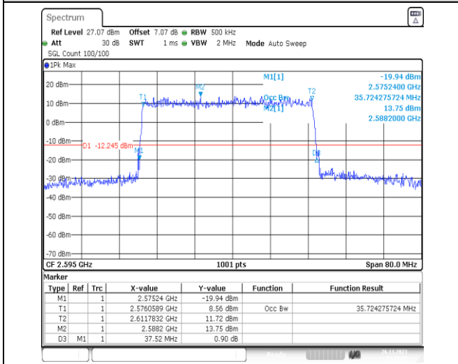
1-N38-PC3-30-40-M-3-DFT-16QAM-Outer_Full-100@0-Ant31-35.724-37.520-≤40-PASS
