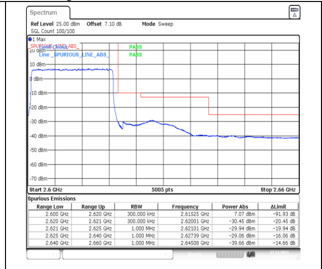
1-N38-PC3-30-20-H-3-DFT-PI2BPSK-Outer_Full-50@0-Ant31-1--PASS-see graph
