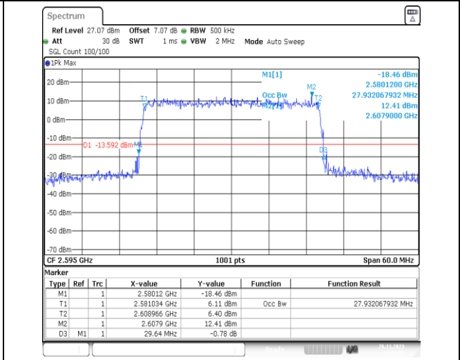
1-N38-PC3-30-30-M-9-CP-256QAM-Outer_Full-78@0-Ant31-27.932-29.640-≤30-PASS
