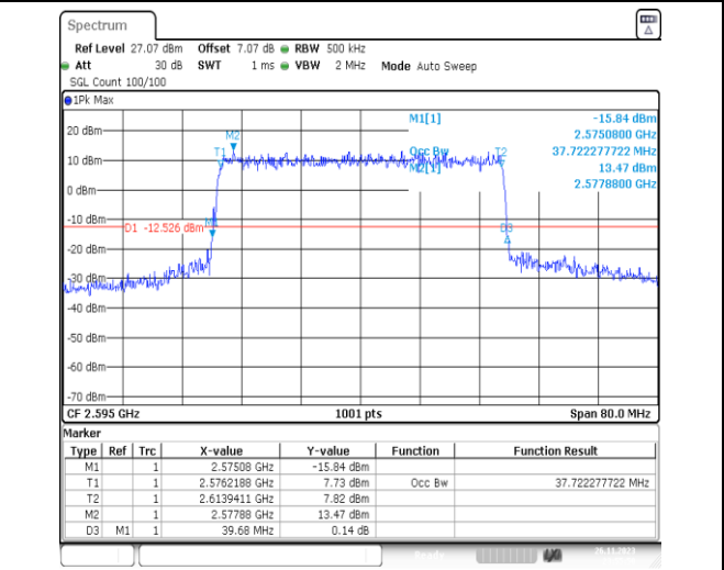
1-N38-PC3-30-40-M-8-CP-64QAM-Outer_Full-106 @0-Ant31-37.722-39.680-≤40-PASS
