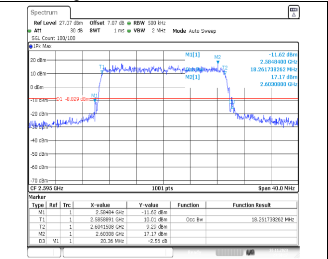
1-N38-PC3-30-20-M-8-CP-64QAM-Outer_Full-51@0 -Ant31-18.262-20.360-≤20-PASS
