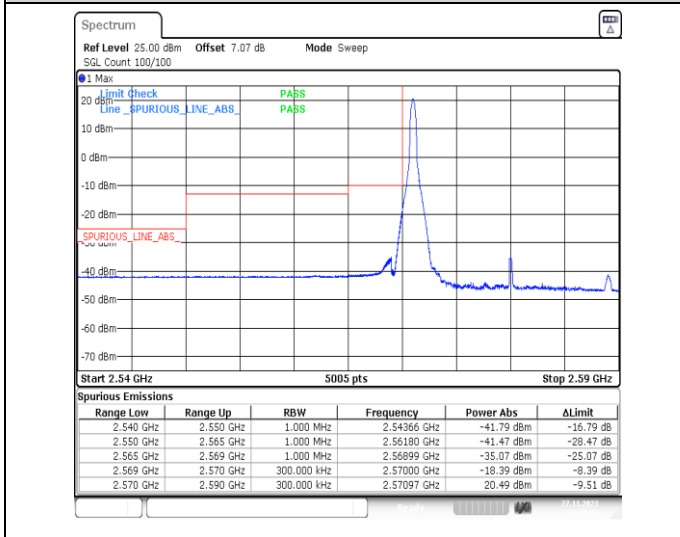
1-N38-PC3-30-20-L-4-CP-QPSK-Edge_1RB_Left-1@0-Ant31-1--PASS-see graph
