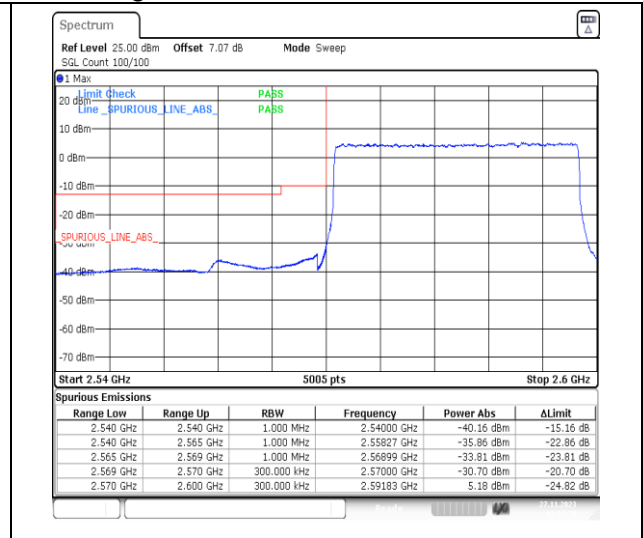
1-N38-PC3-30-30-L-3-DFT-PI2BPSK-Outer_Full-75@0-Ant31-1--PASS-see graph
