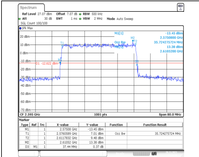
1-N38-PC3-30-40-M-5-DFT-256QAM-Outer_Full-100 @0-Ant31-35.724-37.440-≤40-PASS
