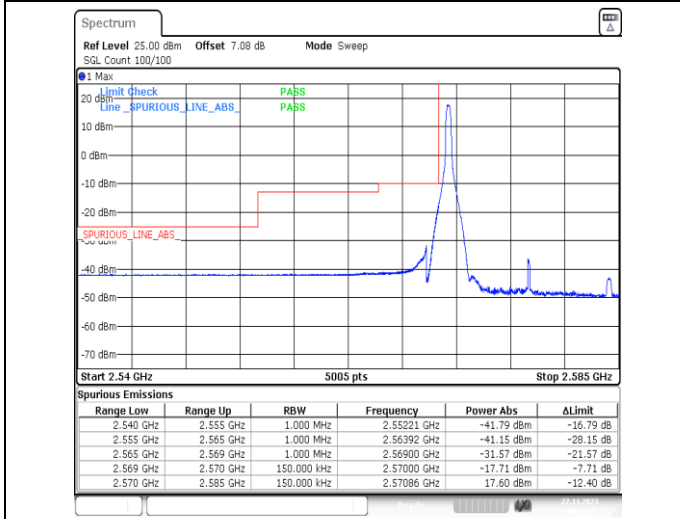
1-N38-PC3-30-15-L-4-CP-QPSK-Edge_1RB_Left-1@0-Ant31-1--PASS-see graph
