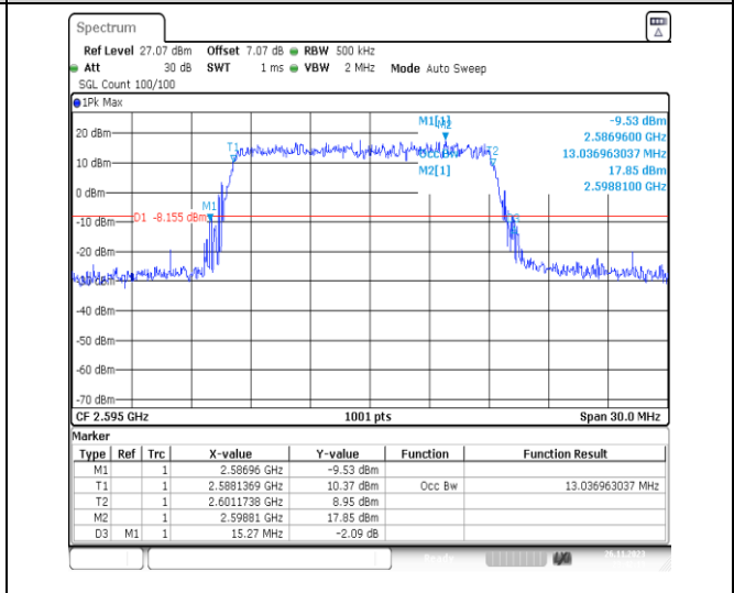
1-N38-PC3-30-15-M-3-DFT-16QAM-Outer_Full-36@ 0-Ant31-13.037-15.270-≤15-PASS
