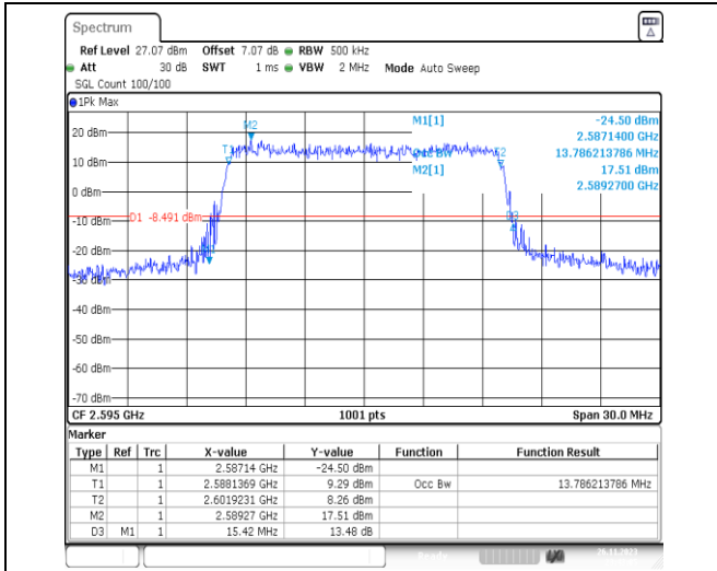
1-N38-PC3-30-15-M-8-CP-64QAM-Outer_Full-38@0 -Ant31-13.786-15.420-≤15-PASS
