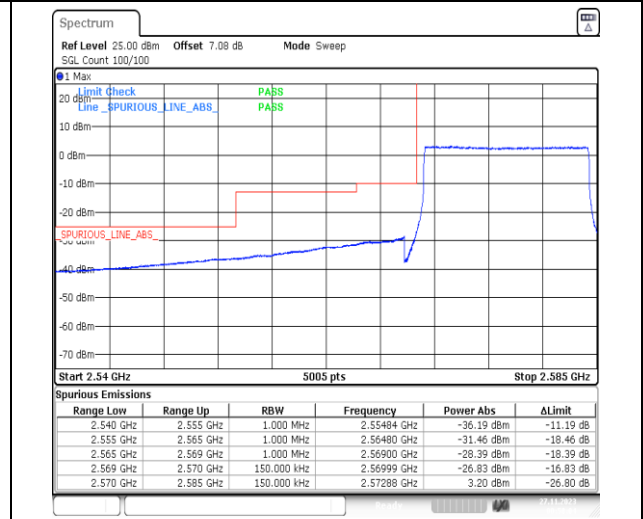
1-N38-PC3-30-15-L-6-CP-QPSK-Outer_Full-38@0-Ant31-1--PASS-see graph
