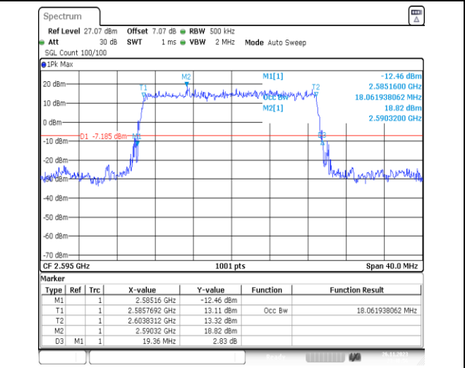
1-N38-PC3-30-20-M-2-DFT-PI2BPSK-Outer_Full-50@0-Ant31-18.062-19.360-≤20-PASS
