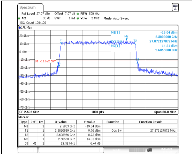
1-N38-PC3-30-30-M-6-CP-QPSK-Outer_Full-78@0-Ant31-27.872-29.520-≤30-PASS
