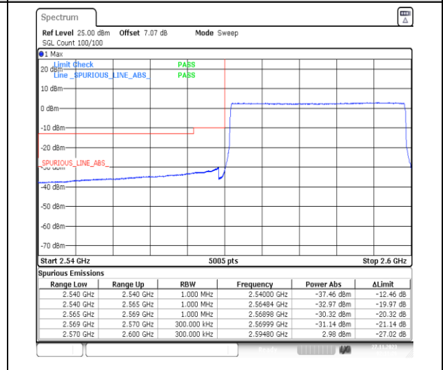
1-N38-PC3-30-30-L-6-CP-QPSK-Outer_Full-78@0-Ant31-1--PASS-see graph
