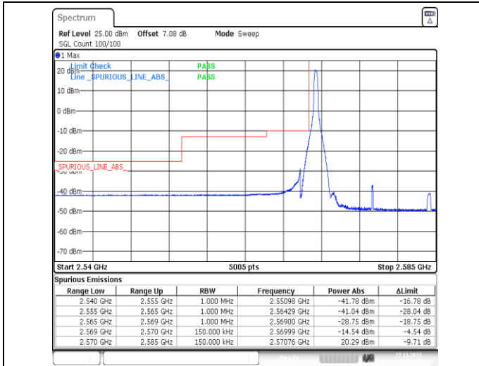
1-N38-PC3-30-15-L-1-DFT-PI2BPSK-Edge_1RB_Left-1@0-Ant31-1--PASS-see graph
