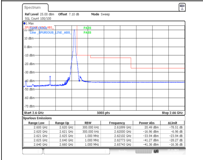
1-N38-PC3-30-20-H-5-CP-QPSK-Edge_1RB_Right-1@50-Ant31-1--PASS-see graph
