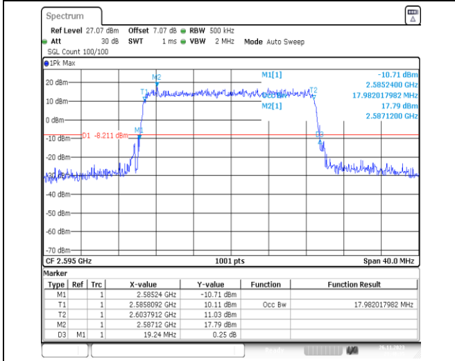
1-N38-PC3-30-20-M-1-DFT-QPSK-Outer_Full-50@0 -Ant31-17.982-19.240-≤20-PASS
