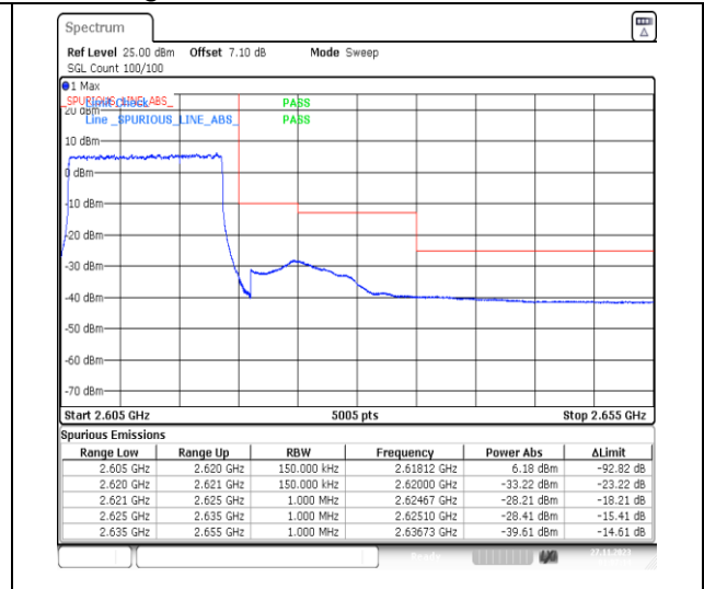
1-N38-PC3-30-15-H-3-DFT-PI2BPSK-Outer_Full-36@0-Ant31-1--PASS-see graph
