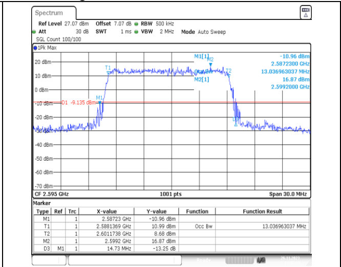
1-N38-PC3-30-15-M-5-DFT-256QAM-Outer_Full-36 @0-Ant31-13.037-14.730-≤15-PASS
