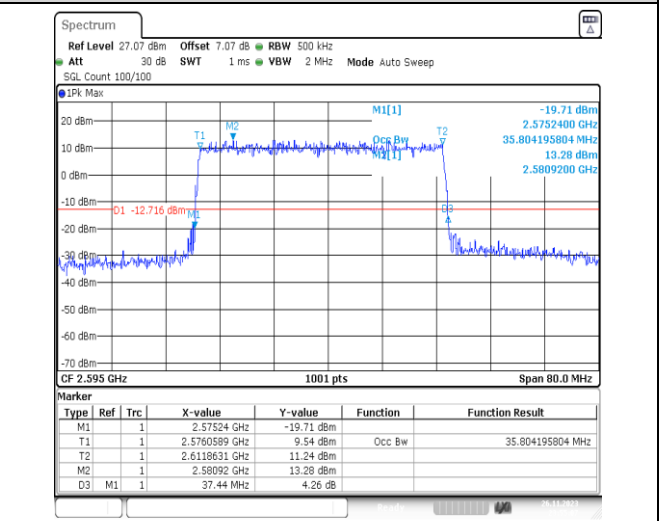
1-N38-PC3-30-40-M-4-DFT-64QAM-Outer_Full-100@0-Ant31-35.804-37.440-≤40-PASS
