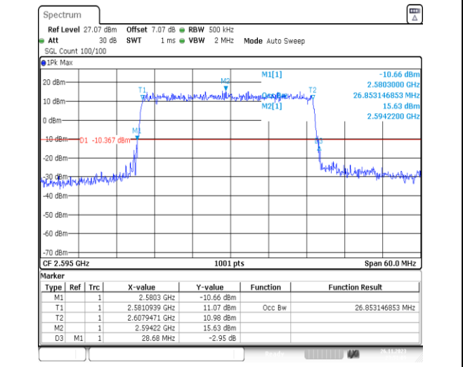
1-N38-PC3-30-30-M-1-DFT-QPSK-Outer_Full-75@0 -Ant31-26.853-28.680-≤30-PASS
