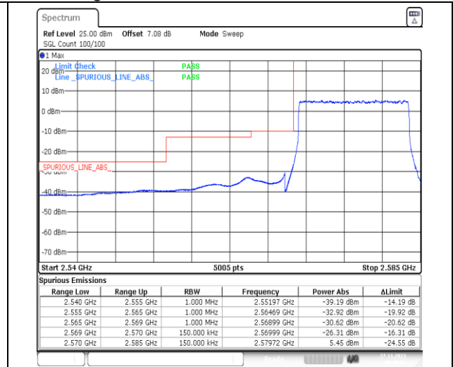
1-N38-PC3-30-15-L-3-DFT-PI2BPSK-Outer_Full-36@0-Ant31-1--PASS-see graph
