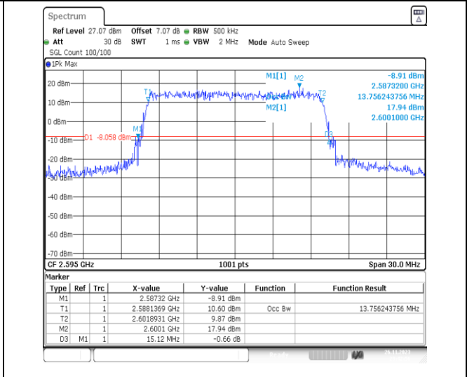
1-N38-PC3-30-15-M-7-CP-16QAM-Outer_Full-38@0- -Ant31-13.756-15.120-≤15-PASS
