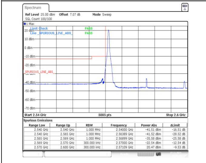
1-N38-PC3-30-30-L-4-CP-QPSK-Edge_1RB_Left-1@0-Ant31-1--PASS-see graph
