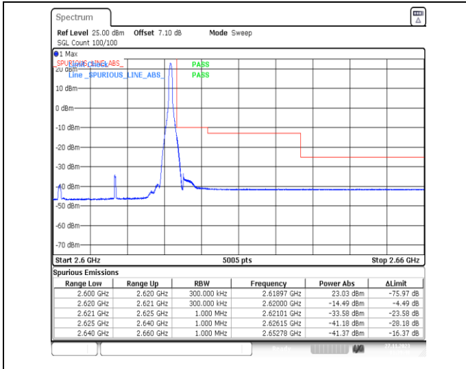
1-N38-PC3-30-20-H-2-DFT-PI2BPSK-Edge_1RB_Right-t-1@50-Ant31-1--PASS-see graph
