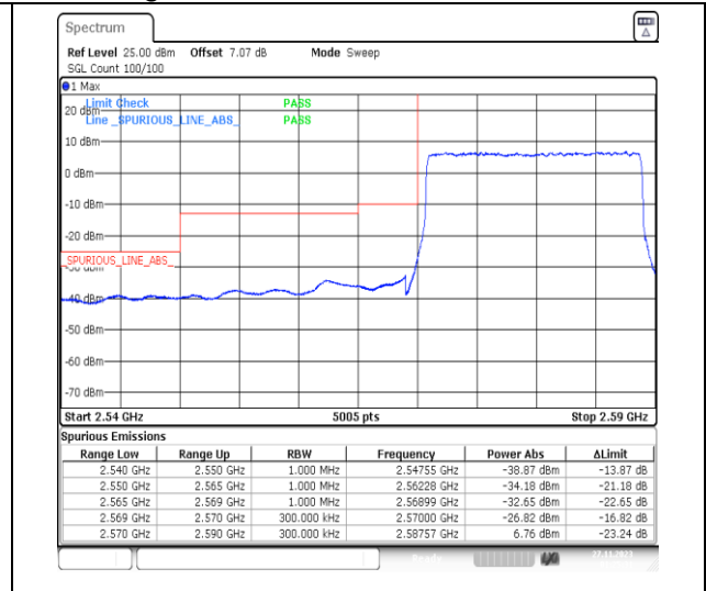
1-N38-PC3-30-20-L-3-DFT-PI2BPSK-Outer_Full-50@0-Ant31-1--PASS-see graph
