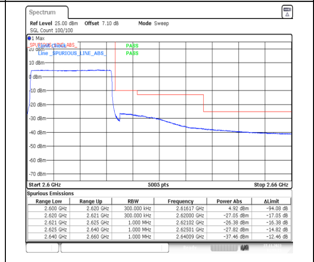
1-N38-PC3-30-20-H-6-CP-QPSK-Outer_Full-51@0-Ant31-1--PASS-see graph
