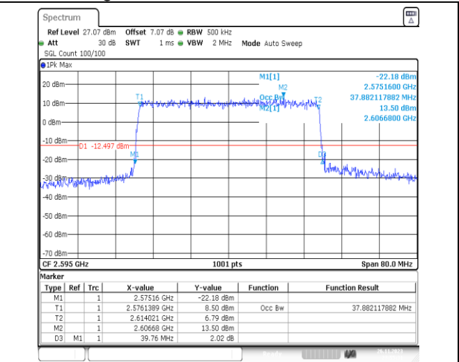
1-N38-PC3-30-40-M-6-CP-QPSK-Outer_Full-106 @0-Ant31-37.882-39.760-≤40-PASS
