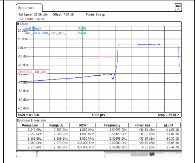
1-N38-PC3-30-20-L-6-CP-QPSK-Outer_Full-51@0-Ant31-1--PASS-see graph
