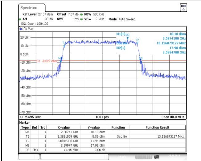
1-N38-PC3-30-15-M-4-DFT-64QAM-Outer_Full-36@ 0-Ant31-13.127-14.460-≤15-PASS
