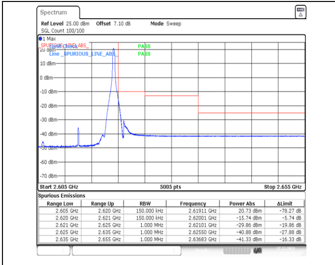
1-N38-PC3-30-15-H-2-DFT-PI2BPSK-Edge_1RB_Right-t-1@37-Ant31-1--PASS-see graph
