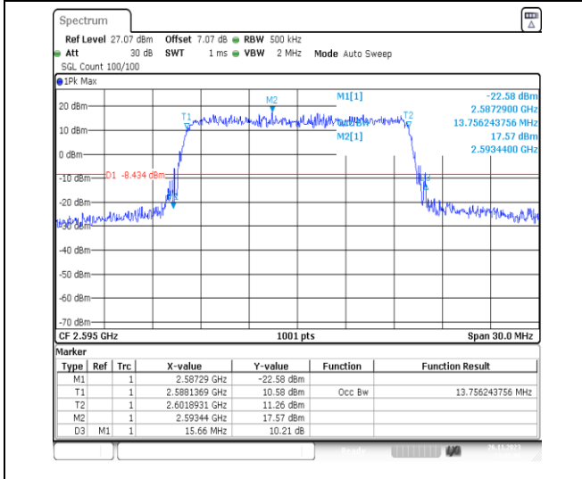
1-N38-PC3-30-15-M-6-CP-QPSK-Outer_Full-38@0- Ant31-13.756-15.660-≤15-PASS
