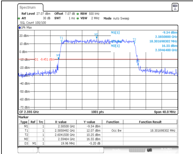
1-N38-PC3-30-20-M-7-CP-16QAM-Outer_Full-51@0 -Ant31-18.302-19.960-≤20-PASS
