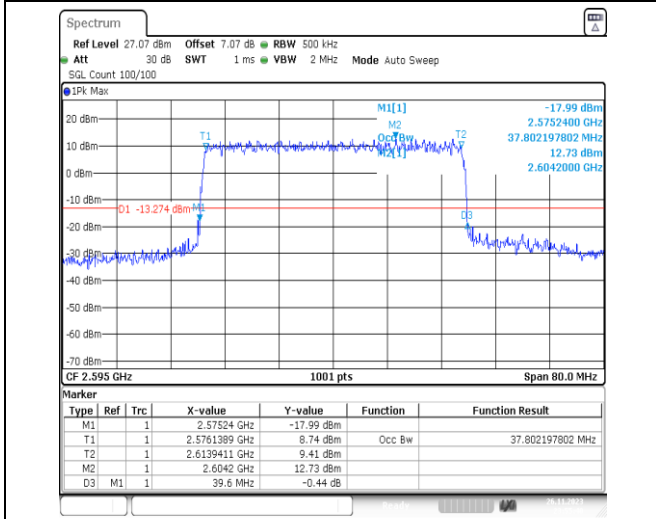
1-N38-PC3-30-40-M-7-CP-16QAM-Outer_Full-106 @0-Ant31-37.802-39.600-≤40-PASS
