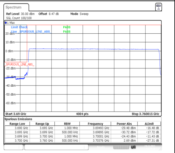
1-N78-3700-3800-PC2-30-60-L-6-CP-QPSK-Outer_Full-162@0-Ant13-1--PASS-see graph
