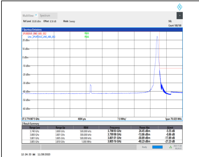
1-N78-3700-3800-PC2-30-60-H-2-DFT-PI2BPSK-Edge_1RB_Right-1@161-Ant13-1--PASS-see graph
