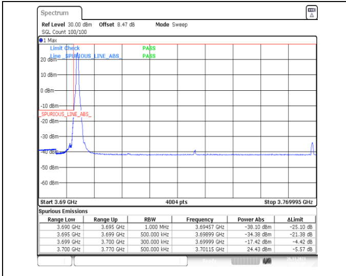
1-N78-3700-3800-PC2-30-70-L-1-DFT-PI2BPSK-Edge_1RB_Left-1@0-Ant13-1--PASS-see graph
