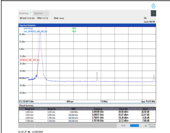
1-N78-3700-3800-PC2-30-60-L-4-CP-QPSK-Edge_1RB_Left-1@0-Ant13-1--PASS-see graph
