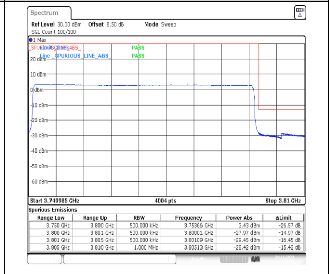
1-N78-3700-3800-PC2-30-50-H-6-CP-QPSK-Outer_Full-133@0-Ant13-1--PASS-see graph
