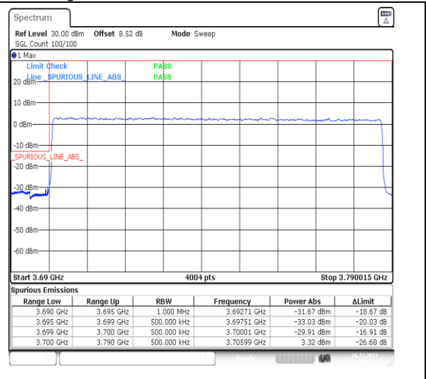
1-N78-3700-3800-PC2-30-90-L-3-DFT-PI2BPSK-Outer_Full-240@0-Ant13-1--PASS-see graph
