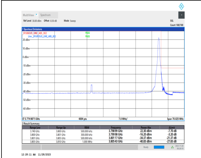
1-N78-3700-3800-PC2-30-60-H-5-CP-QPSK-Edge_1RB_Right-1@161-Ant13-1--PASS-see graph
