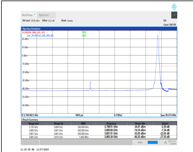
1-N78-3700-3800-PC2-30-80-H-2-DFT-PI2BPSK-Edge_1RB_Right-1@216-Ant13-1--PASS-see graph
