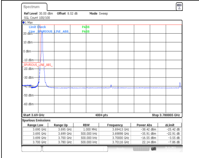
1-N78-3700-3800-PC2-30-80-L-4-CP-QPSK-Edge_1RB_Left-1@0-Ant13-1--PASS-see graph
