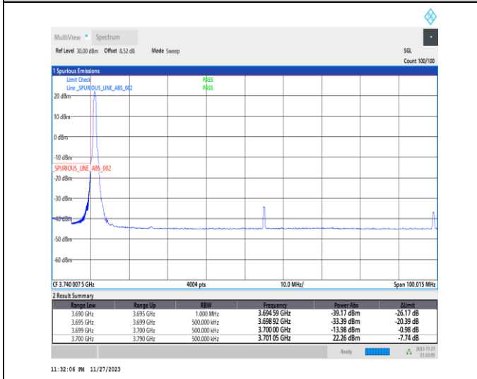
1-N78-3700-3800-PC2-30-90-L-4-CP-QPSK-Edge_1RB_Left-1@0-Ant13-1--PASS-see graph
