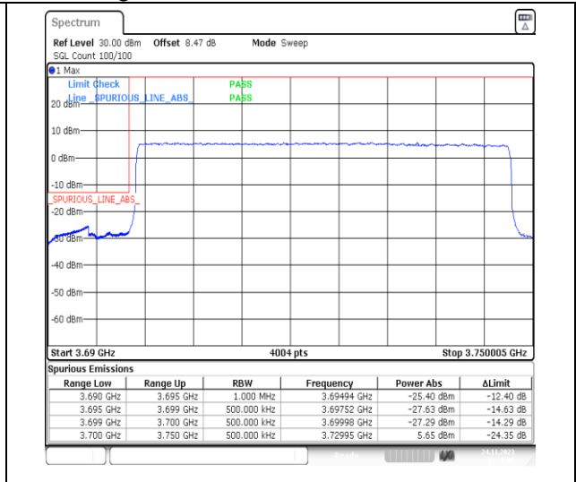
1-N78-3700-3800-PC2-30-50-L-3-DFT-PI2BPSK-Outer_Full-128@0-Ant13-1--PASS-see graph
