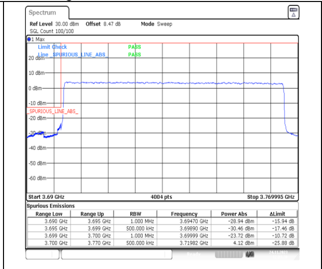
1-N78-3700-3800-PC2-30-70-L-3-DFT-PI2BPSK-Outer_Full-180@0-Ant13-1--PASS-see graph
