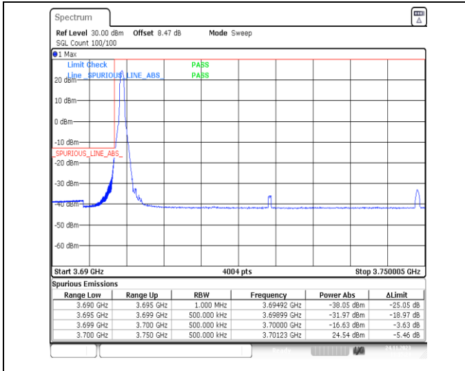
1-N78-3700-3800-PC2-30-50-L-1-DFT-PI2BPSK-Edge_1RB_Left-1@0-Ant13-1--PASS-see graph
