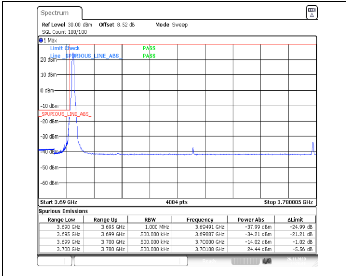
1-N78-3700-3800-PC2-30-80-L-1-DFT-PI2BPSK-Edge_1RB_Left-1@0-Ant13-1--PASS-see graph
