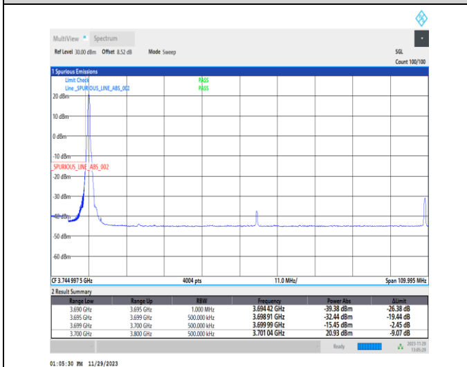
1-N78-3700-3800-PC2-30-100-L-4-CP-QPSK-Edge_1RB_Left-1@0-Ant13-1--PASS-see graph
