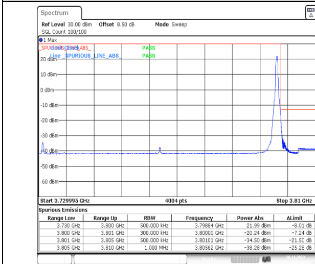
1-N78-3700-3800-PC2-30-70-H-2-DFT-PI2BPSK-Edge_1RB_Right-1@188-Ant13-1--PASS-see graph
