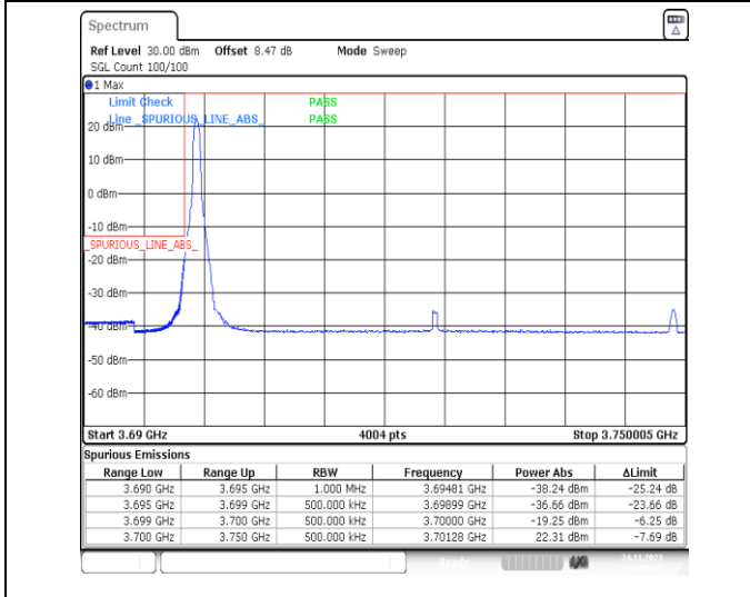
1-N78-3700-3800-PC2-30-50-L-4-CP-QPSK-Edge_1RB_Left-1@0-Ant13-1--PASS-see graph
