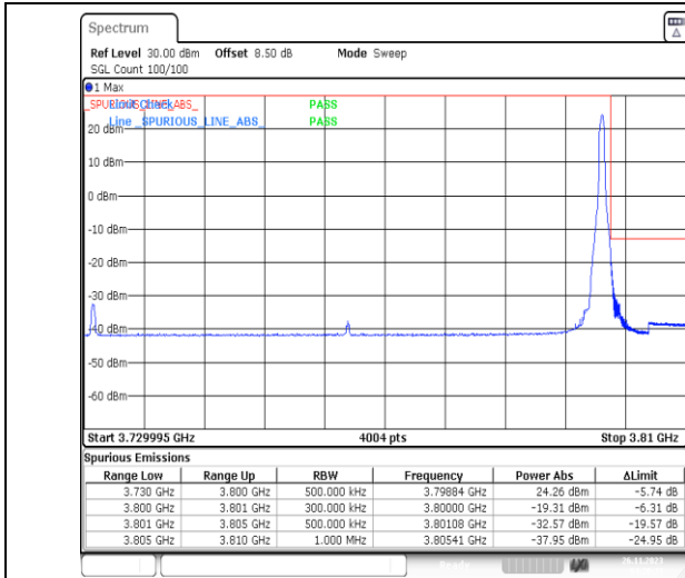
1-N78-3700-3800-PC2-30-70-H-2-DFT-PI2BPSK-Edge_1RB_Right-1@188-Ant13-1--PASS-see graph
