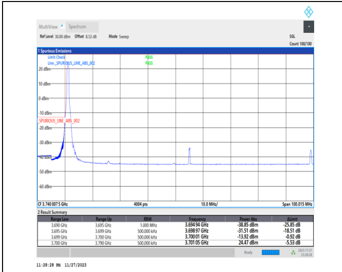
1-N78-3700-3800-PC2-30-90-L-1-DFT-PI2BPSK-Edge_1RB_Left-1@0-Ant13-1--PASS-see graph
