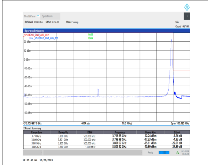
1-N78-3700-3800-PC2-30-90-H-5-CP-QPSK-Edge_1RB_Right-1@244-Ant13-1--PASS-see graph
