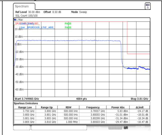
1-N78-3700-3800-PC2-30-50-H-3-DFT-PI2BPSK-Outer_Full-128@0-Ant13-1--PASS-see graph
