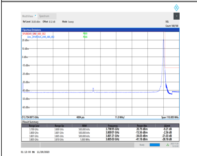
1-N78-3700-3800-PC2-30-100-H-5-CP-QPSK-Edge_1RB_Right-1@272-Ant13-1--PASS-see graph
