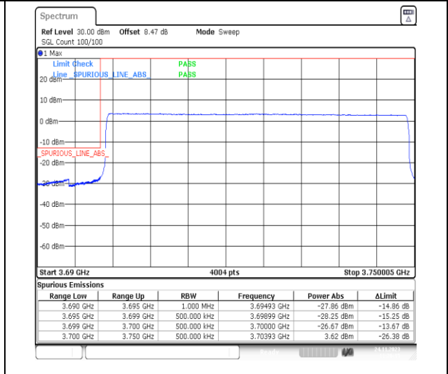
1-N78-3700-3800-PC2-30-50-L-6-CP-QPSK-Outer_Full-133@0-Ant13-1--PASS-see graph
