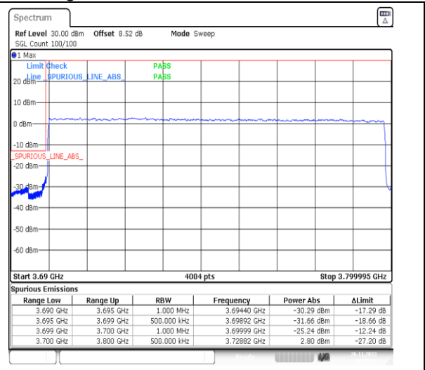
1-N78-3700-3800-PC2-30-100-L-3-DFT-PI2BPSK-Outer_Full-270@0-Ant13-1--PASS-see graph
