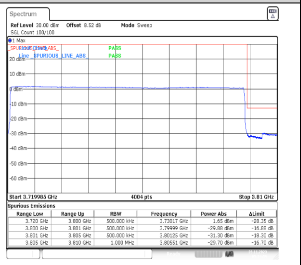
1-N78-3700-3800-PC2-30-80-H-6-CP-QPSK-Outer_Full-217@0-Ant13-1--PASS-see graph
