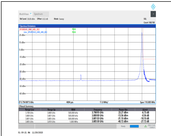
1-N78-3700-3800-PC2-30-100-H-2-DFT-PI2BPSK-Edge_e_1RB_Right-1@272-Ant13-1--PASS-see graph
