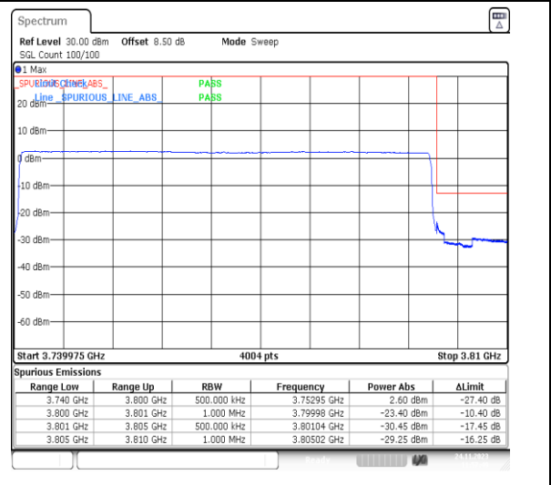
1-N78-3700-3800-PC2-30-60-H-6-CP-QPSK-Outer_Full-162@0-Ant13-1--PASS-see graph
