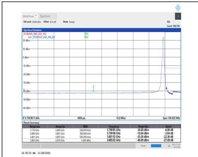
1-N78-3700-3800-PC2-30-90-H-2-DFT-PI2BPSK-Edge_1RB_Right-1@244-Ant13-1--PASS-see graph
