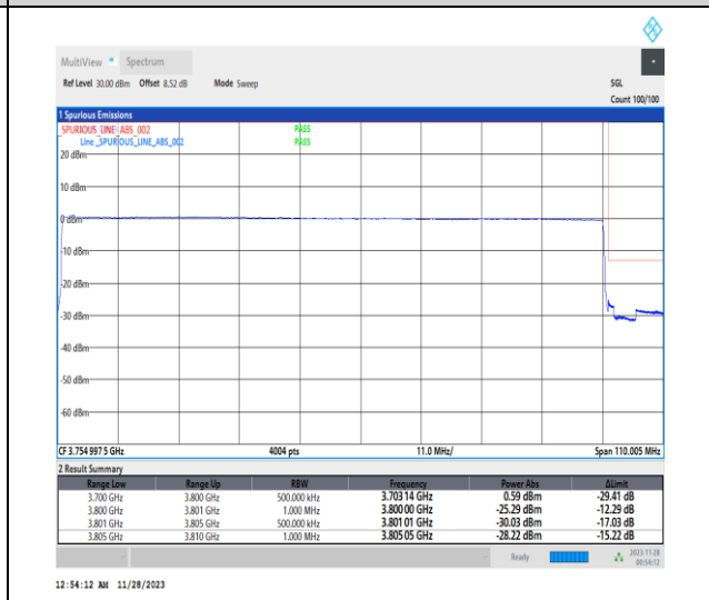
1-N78-3700-3800-PC2-30-100-H-6-CP-QPSK-Outer_Full-273@0-Ant13-1--PASS-see graph
