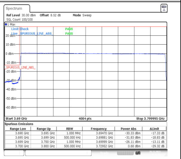
1-N78-3700-3800-PC2-30-100-L-6-CP-QPSK-Outer_Full-273@0-Ant13-1--PASS-see graph
