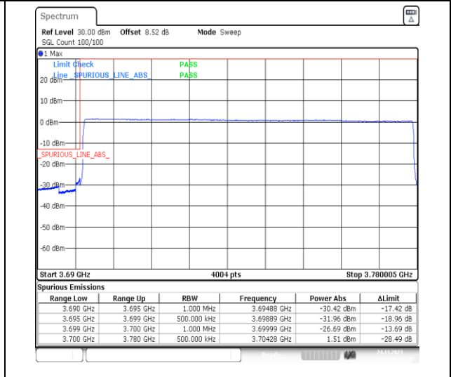
1-N78-3700-3800-PC2-30-80-L-6-CP-QPSK-Outer_Full-217@0-Ant13-1--PASS-see graph
