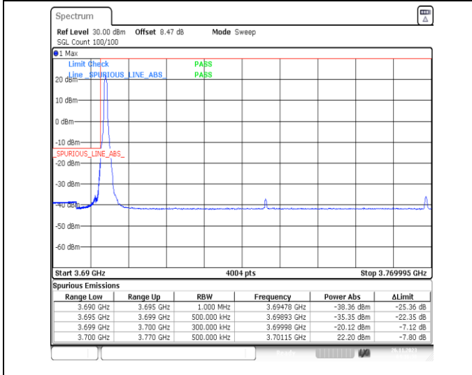
1-N78-3700-3800-PC2-30-70-L-4-CP-QPSK-Edge_1RB_Left-1@0-Ant13-1--PASS-see graph
