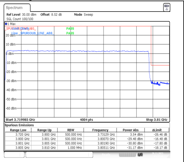
1-N78-3700-3800-PC2-30-80-H-3-DFT-PI2BPSK-Outer_Full-216@0-Ant13-1--PASS-see graph
