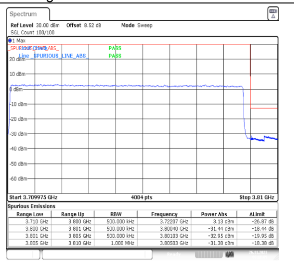
1-N78-3700-3800-PC2-30-90-H-3-DFT-PI2BPSK-Outer_Full-240@0-Ant13-1--PASS-see graph
