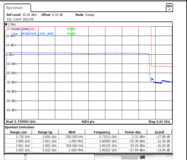
1-N78-3700-3800-PC2-30-70-H-3-DFT-PI2BPSK-Outer_Full-180@0-Ant13-1--PASS-see graph
