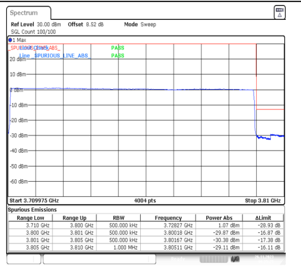
1-N78-3700-3800-PC2-30-90-H-6-CP-QPSK-Outer_Full-245@0-Ant13-1--PASS-see graph
