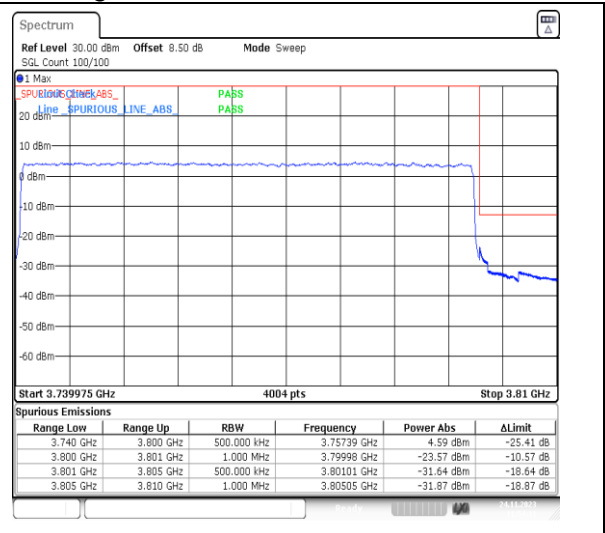
1-N78-3700-3800-PC2-30-60-H-3-DFT-PI2BPSK-Outer_Full-162@0-Ant13-1--PASS-see graph
