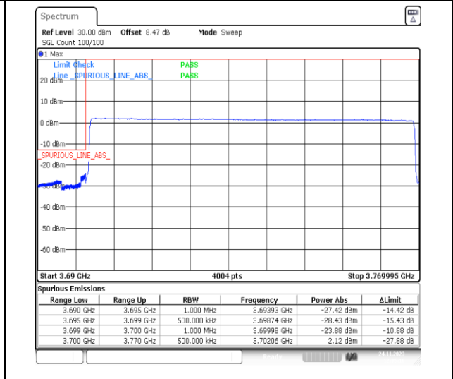
1-N78-3700-3800-PC2-30-70-L-6-CP-QPSK-Outer_Full-189@0-Ant13-1--PASS-see graph
