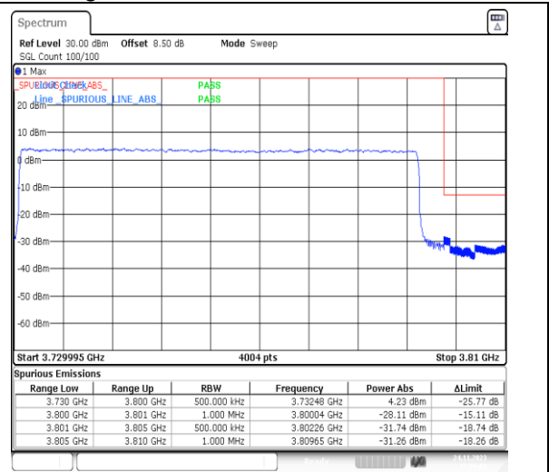
1-N78-3700-3800-PC2-30-70-H-3-DFT-PI2BPSK-Outer_Full-180@0-Ant13-1--PASS-see graph
