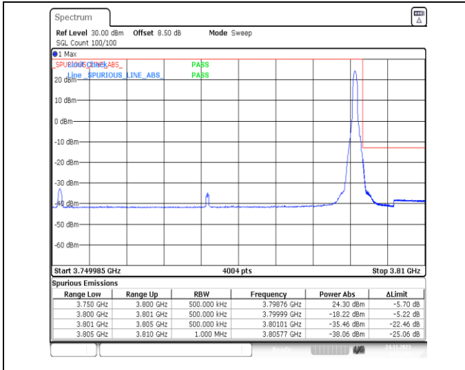
1-N78-3700-3800-PC2-30-50-H-2-DFT-PI2BPSK-Edge_1RB_Right-1@132-Ant13-1--PASS-see graph
