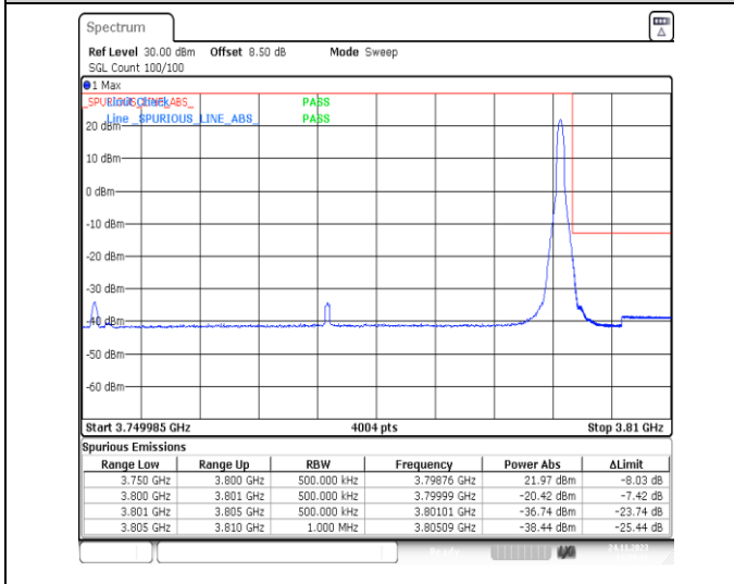
1-N78-3700-3800-PC2-30-50-H-5-CP-QPSK-Edge_1RB_Right-1@132-Ant13-1--PASS-see graph
