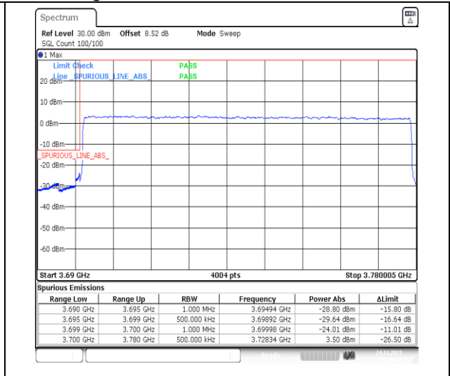
1-N78-3700-3800-PC2-30-80-L-3-DFT-PI2BPSK-Outer_Full-216@0-Ant13-1--PASS-see graph
