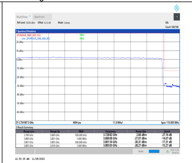
1-N78-3700-3800-PC2-30-100-H-3-DFT-PI2BPSK-Outer_Full-270@0-Ant13-1--PASS-see graph
