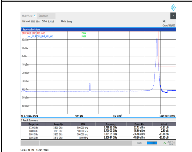
1-N78-3700-3800-PC2-30-80-H-5-CP-QPSK-Edge_1RB_Right-1@216-Ant13-1--PASS-see graph
