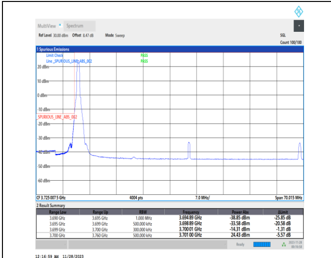
1-N78-3700-3800-PC2-30-60-L-1-DFT-PI2BPSK-Edge_1RB_Left-1@0-Ant13-1--PASS-see graph
