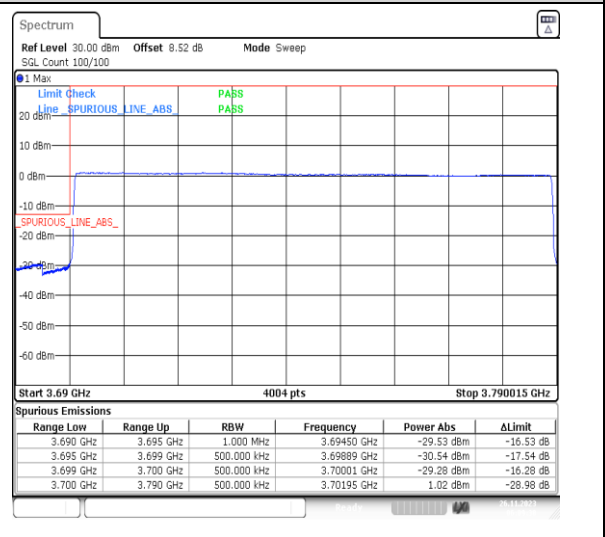
1-N78-3700-3800-PC2-30-90-L-6-CP-QPSK-Outer_Full-245@0-Ant13-1--PASS-see graph
