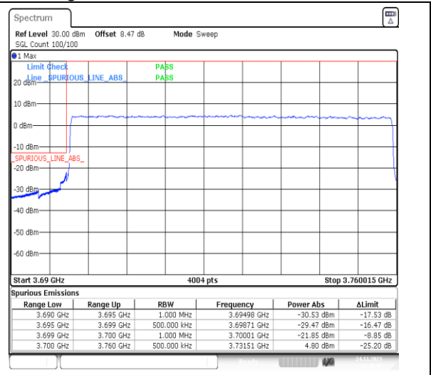
1-N78-3700-3800-PC2-30-60-L-3-DFT-PI2BPSK-Outer_Full-162@0-Ant13-1--PASS-see graph
