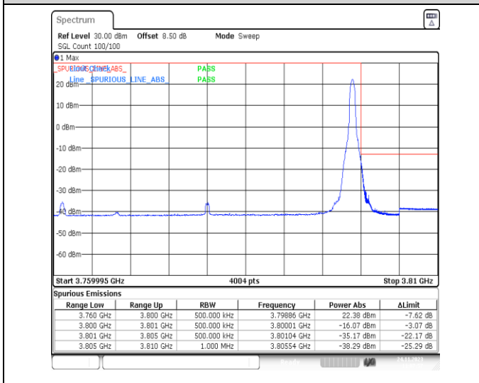
1-N78-3700-3800-PC2-30-40-H-5-CP-QPSK-Edge_1RB_Right-1@105-Ant13-1--PASS-see graph
