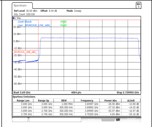
1-N78-3700-3800-PC2-30-40-L-6-CP-QPSK-Outer_Full-106@0-Ant13-1--PASS-see graph
