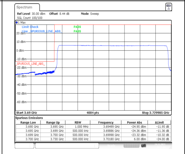
1-N78-3700-3800-PC2-30-30-L-6-CP-QPSK-Outer_Full-78@0-Ant13-1--PASS-see graph
