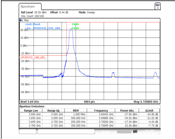
1-N78-3700-3800-PC2-30-20-L-4-CP-QPSK-Edge_1RB_Left-1@0-Ant13-1--PASS-see graph
