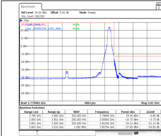
1-N78-3700-3800-PC2-30-20-H-2-DFT-PI2BPSK-Edge_1RB_Right-1@50-Ant13-1--PASS-see graph
