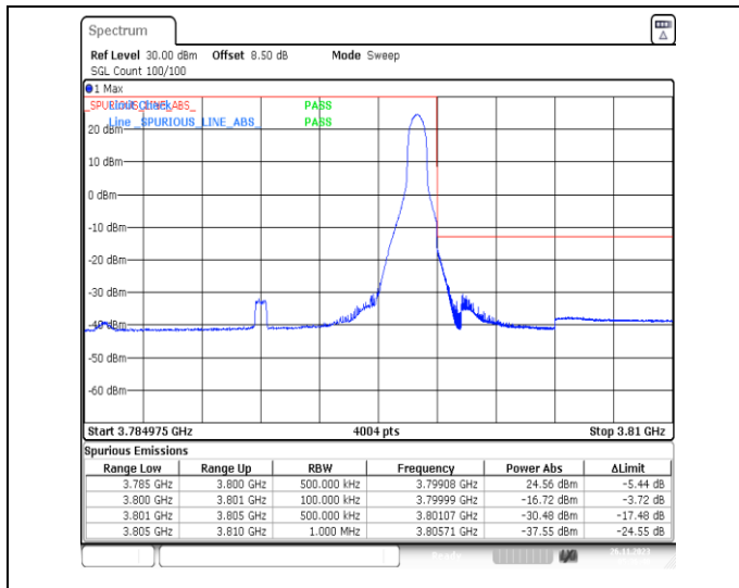
1-N78-3700-3800-PC2-30-15-H-2-DFT-PI2BPSK-Edge_1RB_Right-1@37-Ant13-1--PASS-see graph
