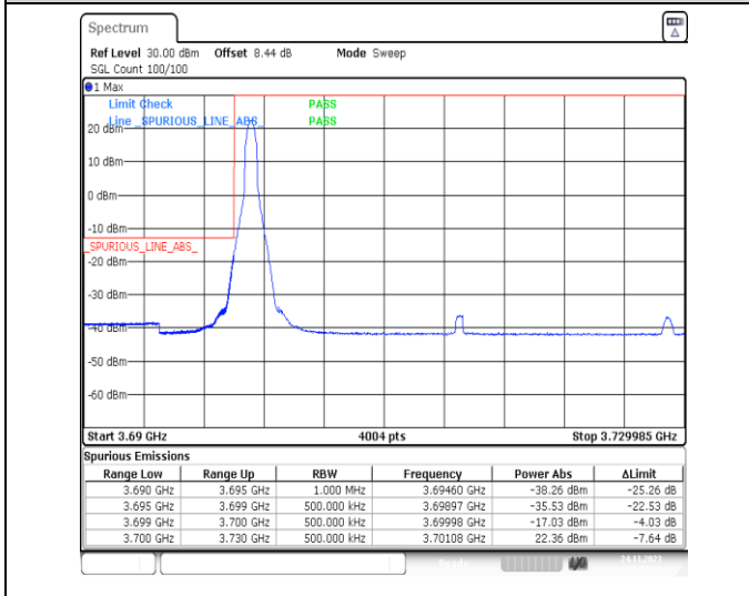
1-N78-3700-3800-PC2-30-30-L-4-CP-QPSK-Edge_1RB_Left-1@0-Ant13-1--PASS-see graph
