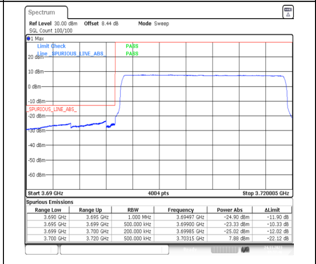
1-N78-3700-3800-PC2-30-20-L-6-CP-QPSK-Outer_Full-51@0-Ant13-1--PASS-see graph
