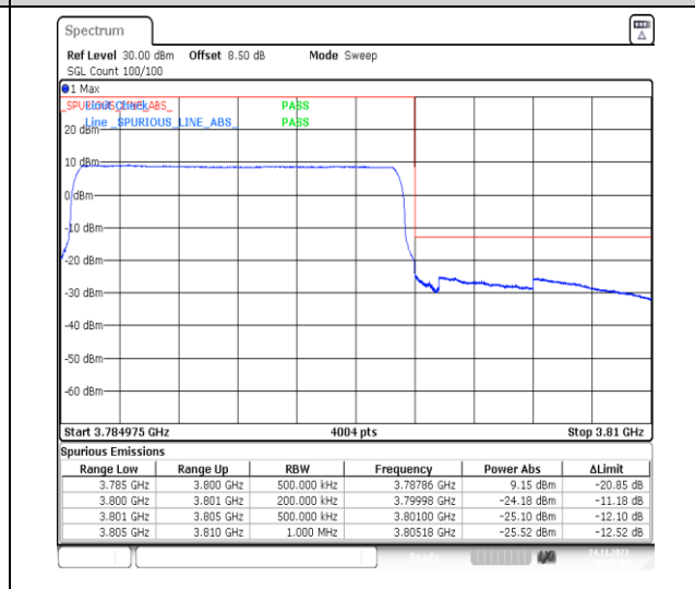
1-N78-3700-3800-PC2-30-15-H-6-CP-QPSK-Outer_Full-38@0-Ant13-1--PASS-see graph
