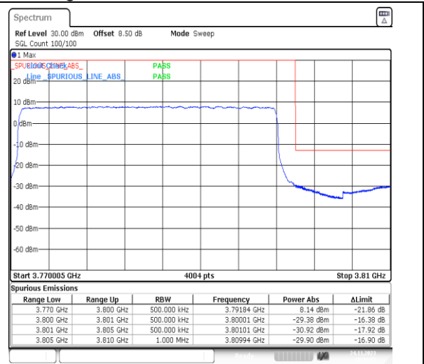
1-N78-3700-3800-PC2-30-30-H-3-DFT-PI2BPSK-Outer_Full-75@0-Ant13-1--PASS-see graph
