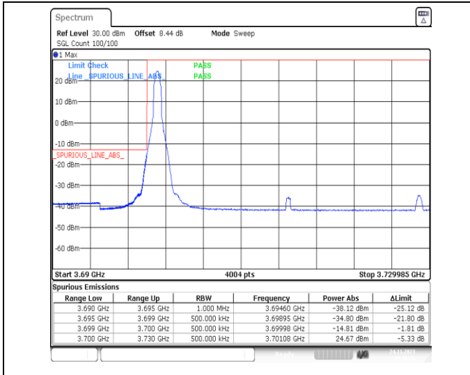
1-N78-3700-3800-PC2-30-30-L-1-DFT-PI2BPSK-Edge_1RB_Left-1@0-Ant13-1--PASS-see graph
