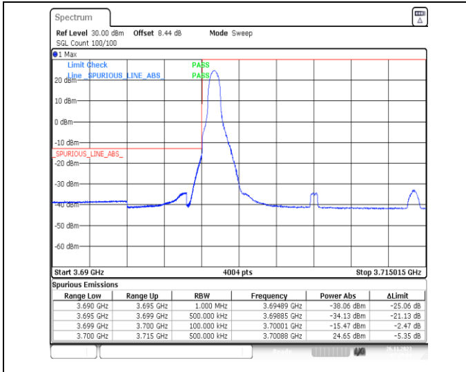
1-N78-3700-3800-PC2-30-15-L-1-DFT-PI2BPSK-Edge_1RB_Left-1@0-Ant13-1--PASS-see graph
