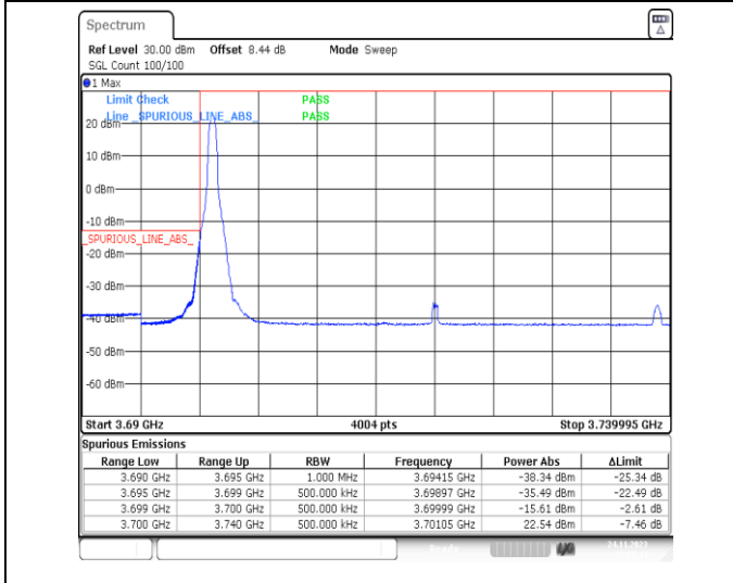
1-N78-3700-3800-PC2-30-40-L-4-CP-QPSK-Edge_1RB_Left-1@0-Ant13-1--PASS-see graph
