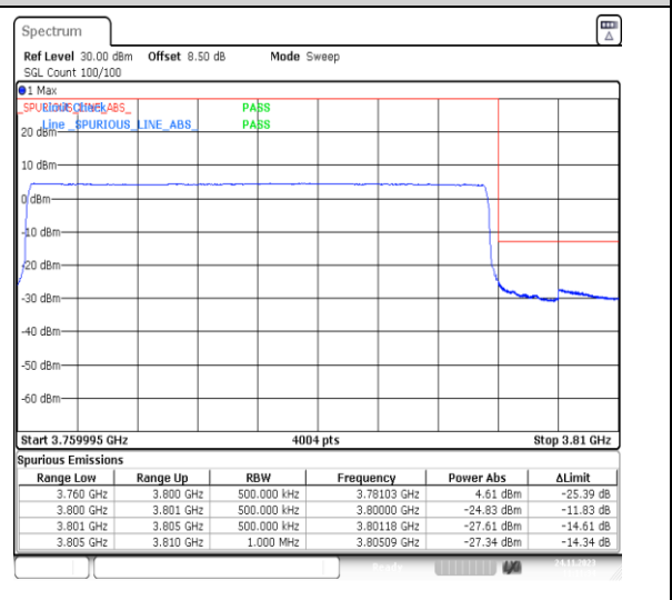
1-N78-3700-3800-PC2-30-40-H-6-CP-QPSK-Outer_Full-106@0-Ant13-1--PASS-see graph
