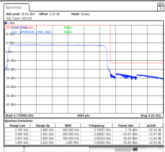
1-N78-3700-3800-PC2-30-20-H-3-DFT-PI2BPSK-Outer_Full-50@0-Ant13-1--PASS-see graph
