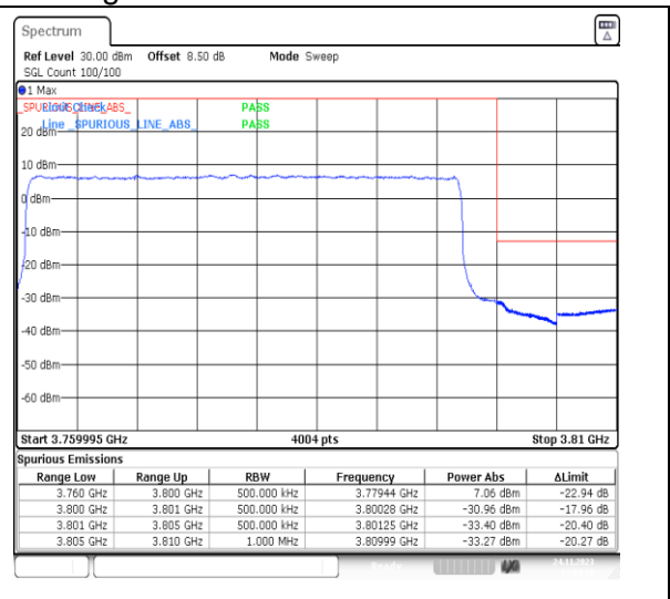
1-N78-3700-3800-PC2-30-40-H-3-DFT-PI2BPSK-Outer_Full-100@0-Ant13-1--PASS-see graph
