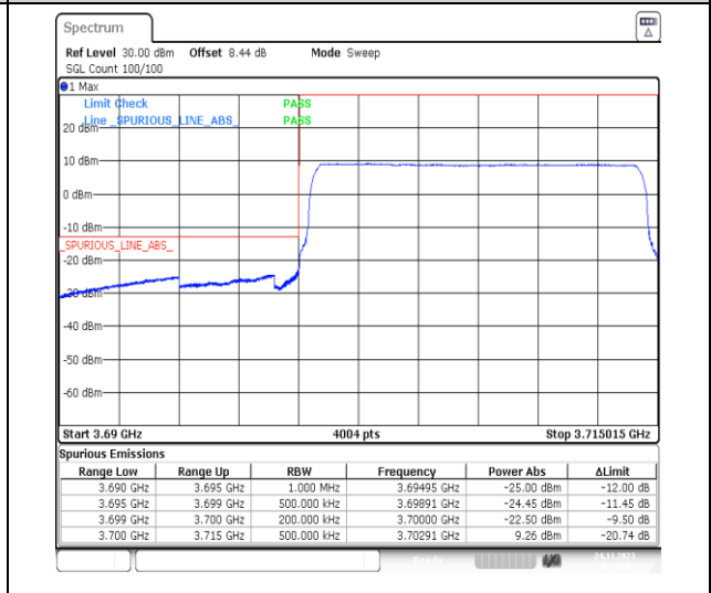
1-N78-3700-3800-PC2-30-15-L-6-CP-QPSK-Outer_Full-38@0-Ant13-1--PASS-see graph
