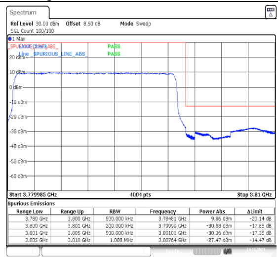
1-N78-3700-3800-PC2-30-20-H-3-DFT-PI2BPSK-Outer_Full-50@0-Ant13-1--PASS-see graph
