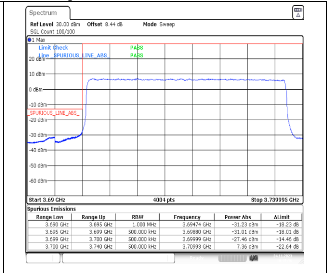
1-N78-3700-3800-PC2-30-40-L-3-DFT-PI2BPSK-Outer_Full-100@0-Ant13-1--PASS-see graph
