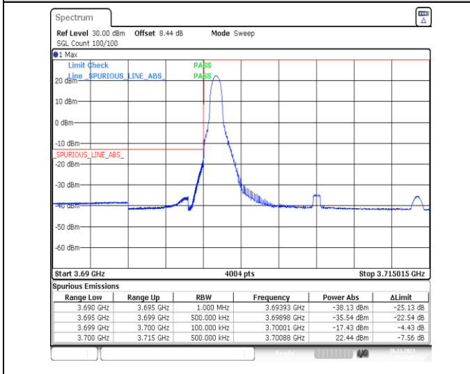
1-N78-3700-3800-PC2-30-15-L-4-CP-QPSK-Edge_1RB_Left-1@0-Ant13-1--PASS-see graph
