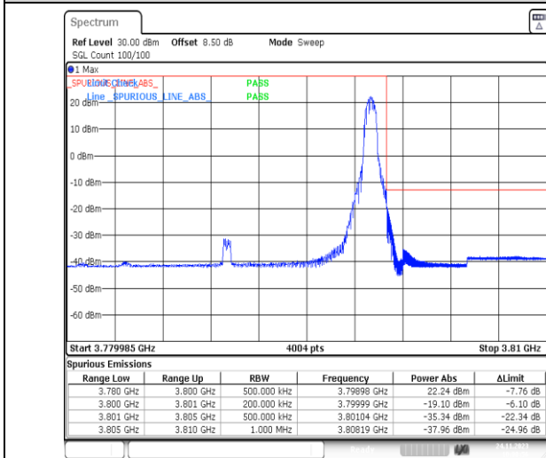
1-N78-3700-3800-PC2-30-20-H-2-DFT-PI2BPSK-Edge_1RB_Right-1@50-Ant13-1--PASS-see graph
