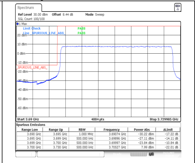
1-N78-3700-3800-PC2-30-30-L-3-DFT-PI2BPSK-Outer_Full-75@0-Ant13-1--PASS-see graph
