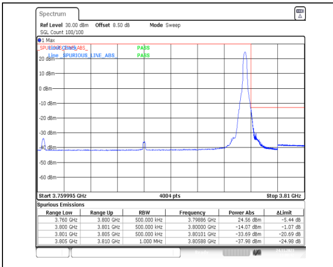
1-N78-3700-3800-PC2-30-40-H-2-DFT-PI2BPSK-Edge_1RB_Right-1@105-Ant13-1--PASS-see graph
