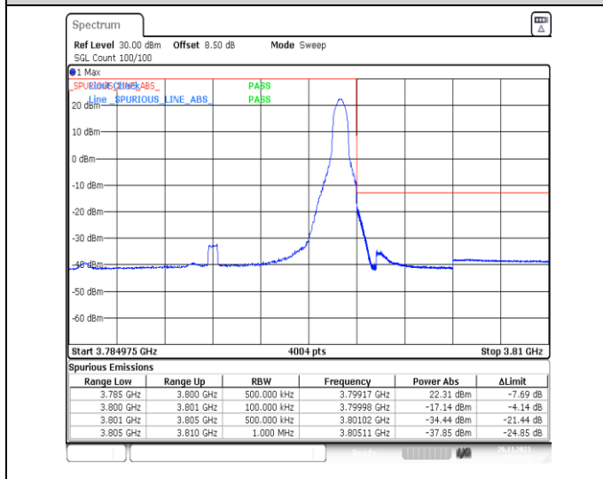
1-N78-3700-3800-PC2-30-15-H-5-CP-QPSK-Edge_1RB_Right-1@37-Ant13-1--PASS-see graph
