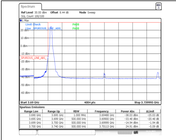
1-N78-3700-3800-PC2-30-40-L-1-DFT-PI2BPSK-Edge_1RB_Left-1@0-Ant13-1--PASS-see graph
