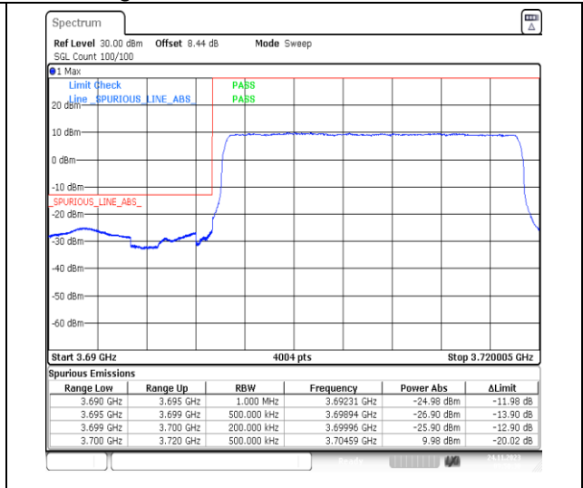
1-N78-3700-3800-PC2-30-20-L-3-DFT-PI2BPSK-Outer_Full-50@0-Ant13-1--PASS-see graph
