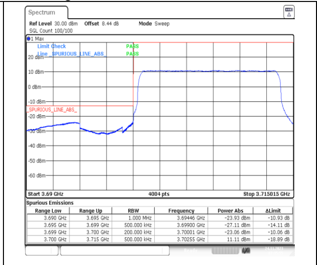
1-N78-3700-3800-PC2-30-15-L-3-DFT-PI2BPSK-Outer_Full-36@0-Ant13-1--PASS-see graph
