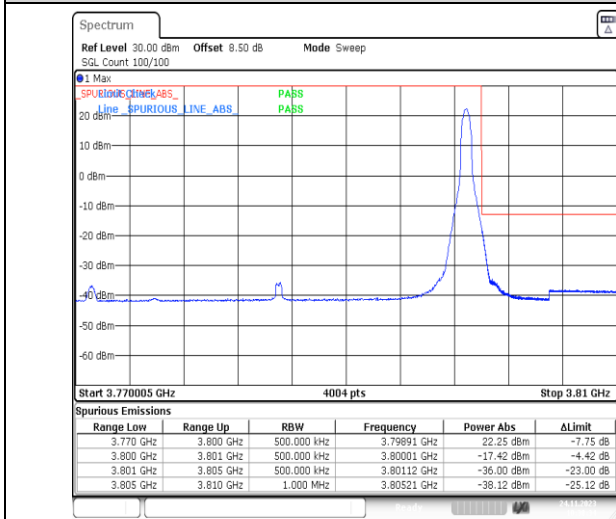
1-N78-3700-3800-PC2-30-30-H-2-DFT-PI2BPSK-Edge_1RB_Right-1@77-Ant13-1--PASS-see graph
