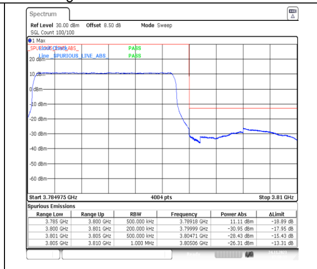
1-N78-3700-3800-PC2-30-15-H-3-DFT-PI2BPSK-Outer_Full-36@0-Ant13-1--PASS-see graph
