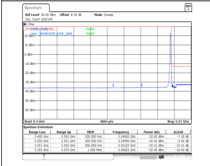
1-N78-3450-3550-PC2-30-60-H-5-CP-QPSK-Edge_1RB_Right-1@161-Ant13-1--PASS-see graph
