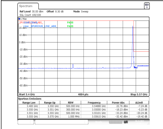
1-N78-3450-3550-PC2-30-80-H-5-CP-QPSK-Edge_1RB_Right-1@216-Ant13-1--PASS-see graph
