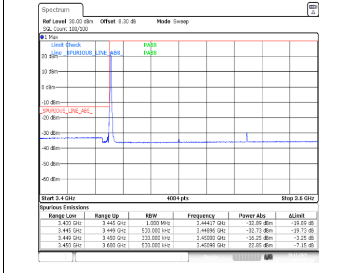
1-N78-3450-3550-PC2-30-100-L-4-CP-QPSK-Edge_1RB_Left-1@0-Ant13-1--PASS-see graph
