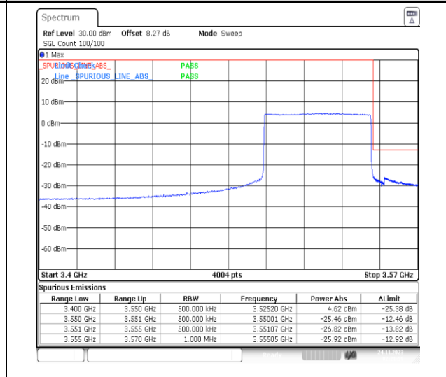
1-N78-3450-3550-PC2-30-50-H-6-CP-QPSK-Outer_Full-133@0-Ant13-1--PASS-see graph
