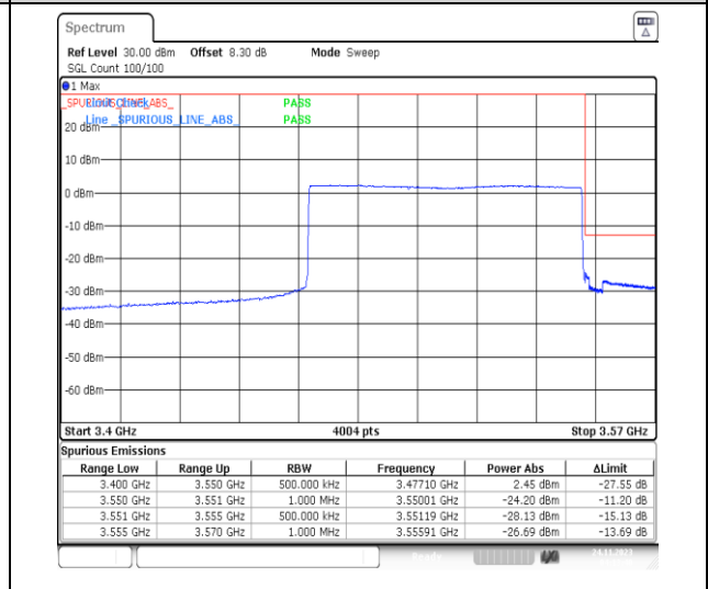
1-N78-3450-3550-PC2-30-80-H-6-CP-QPSK-Outer_Full-217@0-Ant13-1--PASS-see graph
