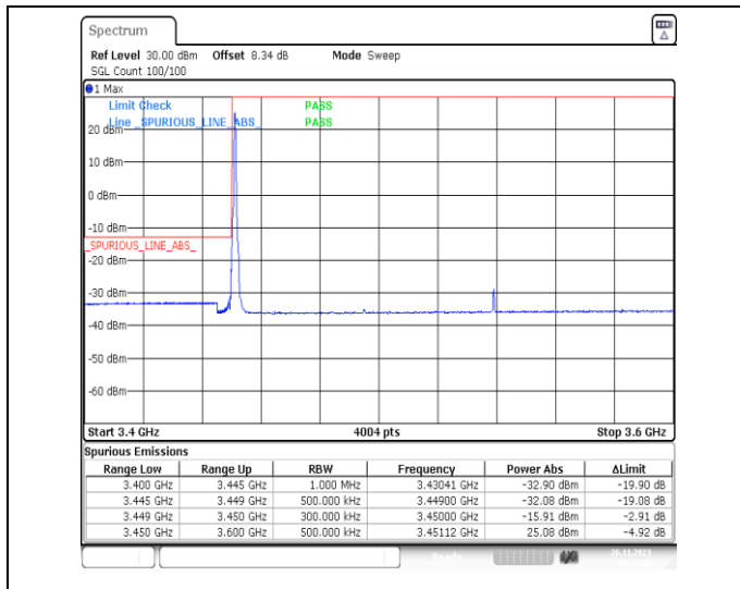
1-N78-3450-3550-PC2-30-90-L-1-DFT-PI2BPSK-Edge_1RB_Left-1@0-Ant13-1--PASS-see graph
