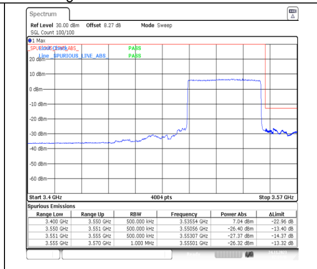
1-N78-3450-3550-PC2-30-50-H-3-DFT-PI2BPSK-Outer_Full-128@0-Ant13-1--PASS-see graph
