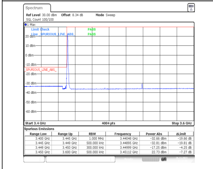
1-N78-3450-3550-PC2-30-90-L-4-CP-QPSK-Edge_1RB_Left-1@0-Ant13-1--PASS-see graph
