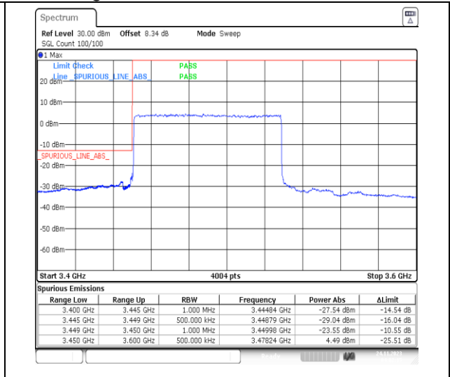
1-N78-3450-3550-PC2-30-80-L-3-DFT-PI2BPSK-Outer_Full-216@0-Ant13-1--PASS-see graph
