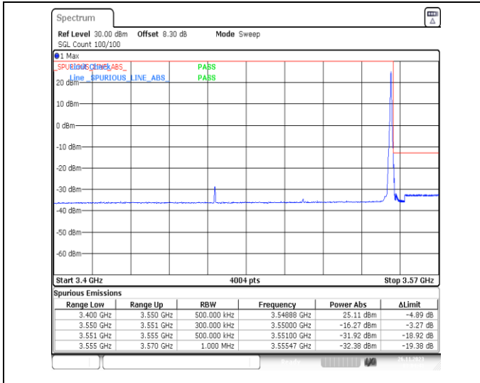
1-N78-3450-3550-PC2-30-80-H-2-DFT-PI2BPSK-Edge_1RB_Right-1@216-Ant13-1--PASS-see graph
