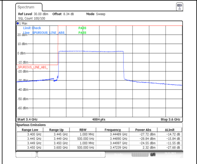
1-N78-3450-3550-PC2-30-80-L-6-CP-QPSK-Outer_Full-217@0-Ant13-1--PASS-see graph
