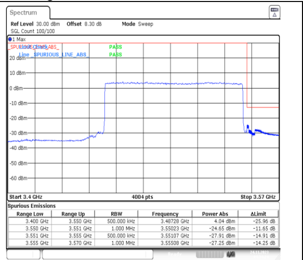
1-N78-3450-3550-PC2-30-90-H-3-DFT-PI2BPSK-Outer_Full-240@0-Ant13-1--PASS-see graph
