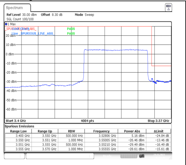
1-N78-3450-3550-PC2-30-70-H-3-DFT-PI2BPSK-Outer_Full-180@0-Ant13-1--PASS-see graph
