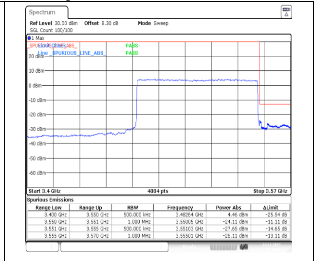
1-N78-3450-3550-PC2-30-80-H-3-DFT-PI2BPSK-Outer_Full-216@0-Ant13-1--PASS-see graph
