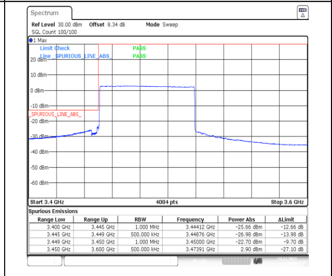
1-N78-3450-3550-PC2-30-70-L-6-CP-QPSK-Outer_Full-189@0-Ant13-1--PASS-see graph
