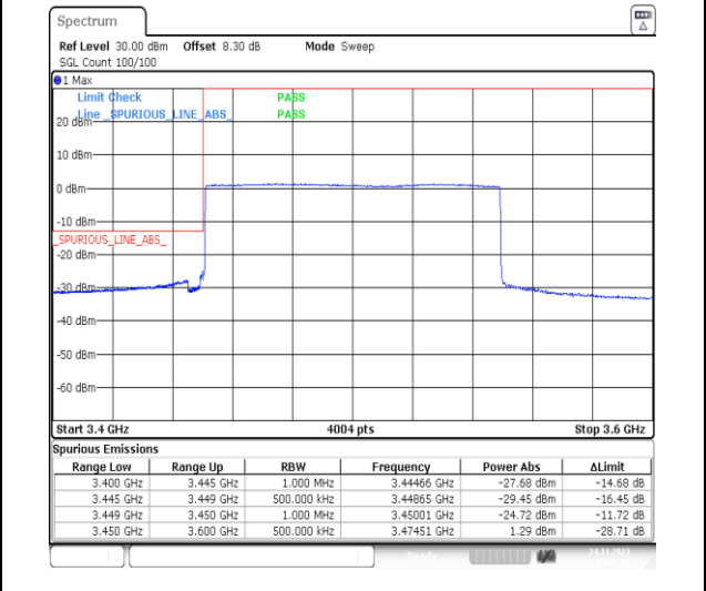
1-N78-3450-3550-PC2-30-100-L-6-CP-QPSK-Outer_Full-273@0-Ant13-1--PASS-see graph
