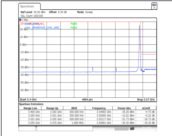
1-N78-3450-3550-PC2-30-60-H-2-DFT-PI2BPSK-Edge_1RB_Right-1@161-Ant13-1--PASS-see graph
