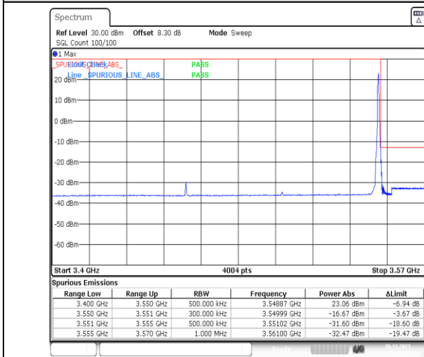
1-N78-3450-3550-PC2-30-90-H-2-DFT-PI2BPSK-Edge_1RB_Right-1@244-Ant13-1--PASS-see graph
