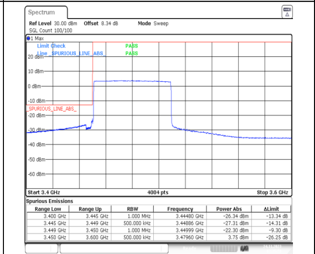
1-N78-3450-3550-PC2-30-60-L-6-CP-QPSK-Outer_Full-162@0-Ant13-1--PASS-see graph
