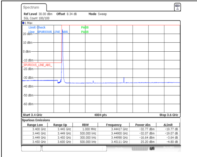
1-N78-3450-3550-PC2-30-80-L-1-DFT-PI2BPSK-Edge_1RB_Left-1@0-Ant13-1--PASS-see graph
