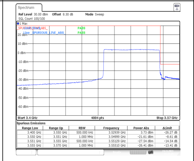
1-N78-3450-3550-PC2-30-60-H-6-CP-QPSK-Outer_Full-162@0-Ant13-1--PASS-see graph
