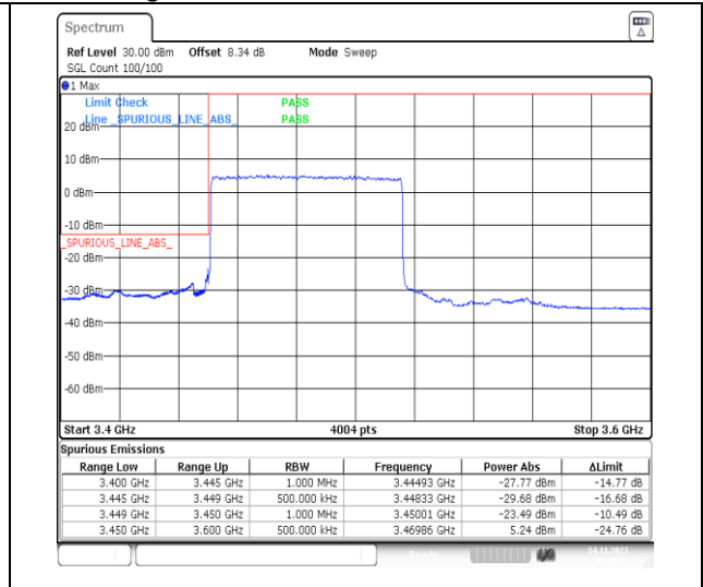
1-N78-3450-3550-PC2-30-70-L-3-DFT-PI2BPSK-Outer_Full-180@0-Ant13-1--PASS-see graph
