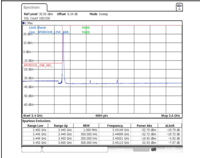
1-N78-3450-3550-PC2-30-70-L-4-CP-QPSK-Edge_1RB_Left-1@0-Ant13-1--PASS-see graph
