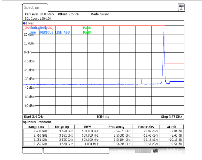
1-N78-3450-3550-PC2-30-50-H-5-CP-QPSK-Edge_1RB_Right-1@132-Ant13-1--PASS-see graph
