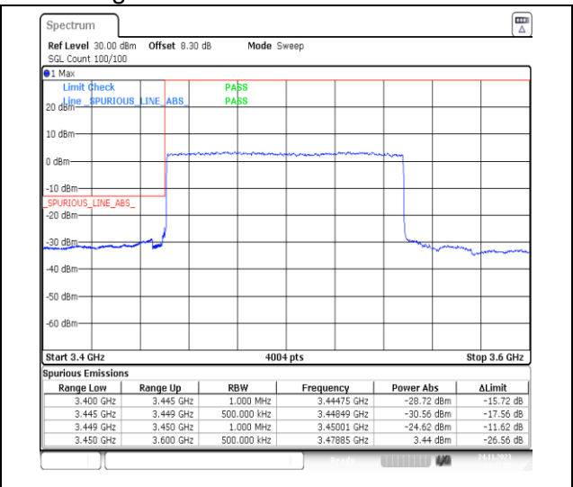
1-N78-3450-3550-PC2-30-100-L-3-DFT-PI2BPSK-Outer_Full-270@0-Ant13-1--PASS-see graph
