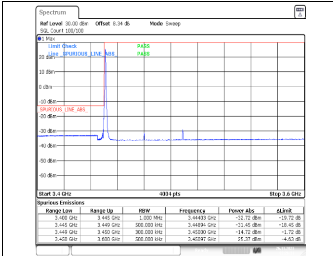
1-N78-3450-3550-PC2-30-60-L-1-DFT-PI2BPSK-Edge_1RB_Left-1@0-Ant13-1--PASS-see graph
