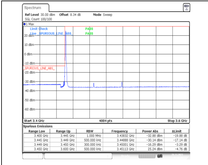
1-N78-3450-3550-PC2-30-70-L-1-DFT-PI2BPSK-Edge_1RB_Left-1@0-Ant13-1--PASS-see graph
