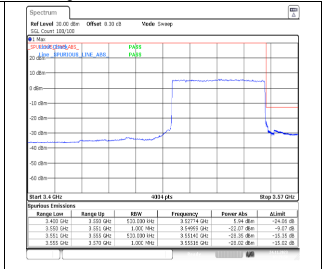
1-N78-3450-3550-PC2-30-60-H-3-DFT-PI2BPSK-Outer_Full-162@0-Ant13-1--PASS-see graph
