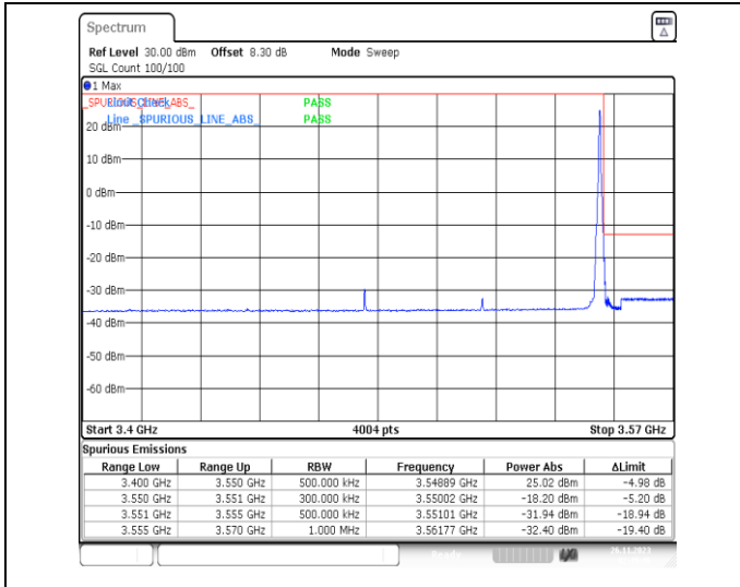
1-N78-3450-3550-PC2-30-70-H-2-DFT-PI2BPSK-Edge_1RB_Right-1@188-Ant13-1--PASS-see graph
