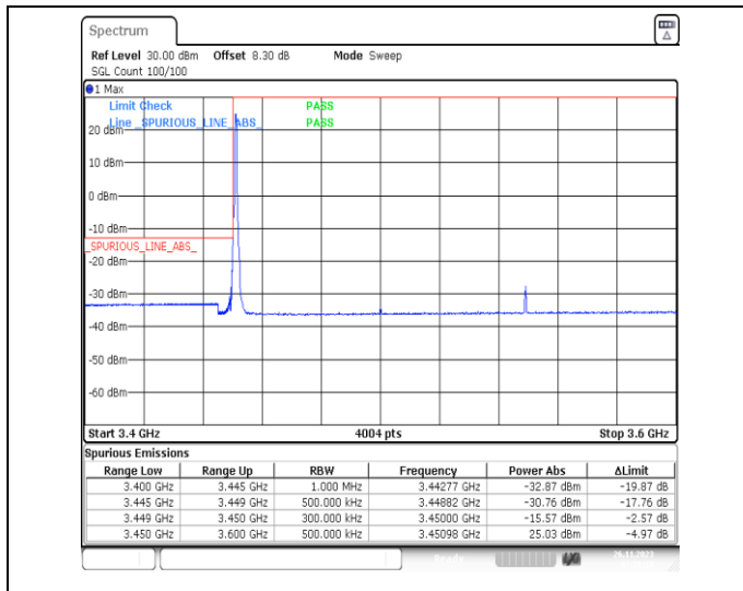
1-N78-3450-3550-PC2-30-100-L-1-DFT-PI2BPSK-Edge_e_1RB_Left-1@0-Ant13-1--PASS-see graph
