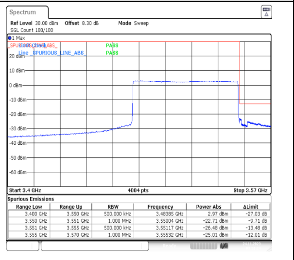
1-N78-3450-3550-PC2-30-70-H-6-CP-QPSK-Outer_Full-189@0-Ant13-1--PASS-see graph
