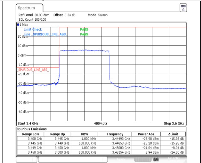
1-N78-3450-3550-PC2-30-60-L-3-DFT-PI2BPSK-Outer_Full-162@0-Ant13-1--PASS-see graph
