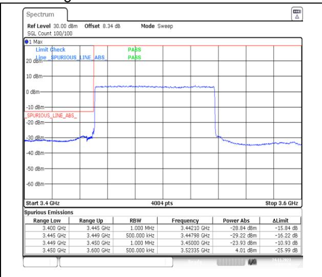
1-N78-3450-3550-PC2-30-90-L-3-DFT-PI2BPSK-Outer_Full-240@0-Ant13-1--PASS-see graph
