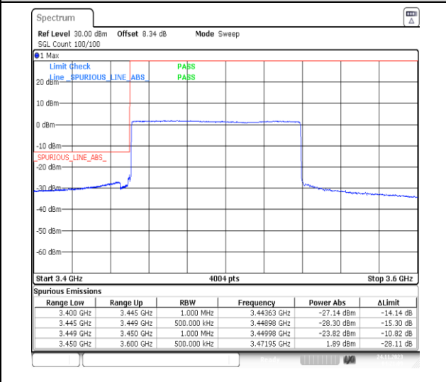
1-N78-3450-3550-PC2-30-90-L-6-CP-QPSK-Outer_Full-245@0-Ant13-1--PASS-see graph
