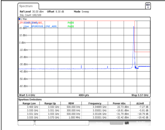
1-N78-3450-3550-PC2-30-70-H-5-CP-QPSK-Edge_1RB_Right-1@188-Ant13-1--PASS-see graph
