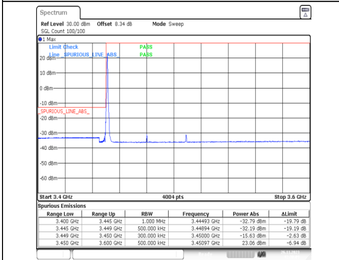
1-N78-3450-3550-PC2-30-60-L-4-CP-QPSK-Edge_1RB_Left-1@0-Ant13-1--PASS-see graph
