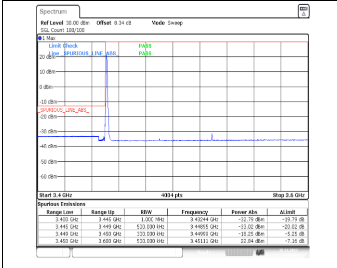
1-N78-3450-3550-PC2-30-80-L-4-CP-QPSK-Edge_1RB_Left-1@0-Ant13-1--PASS-see graph
