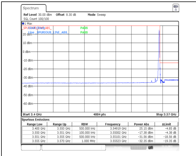
1-N78-3450-3550-PC2-30-10-H-2-DFT-PI2BPSK-Edge_1RB_Right-1@23-Ant13-1--PASS-see graph
