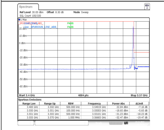
1-N78-3450-3550-PC2-30-10-H-5-CP-QPSK-Edge_1RB_Right-1@23-Ant13-1--PASS-see graph
