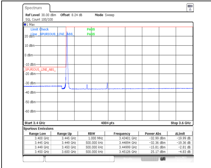
1-N78-3450-3550-PC2-30-50-L-1-DFT-PI2BPSK-Edge_1RB_Left-1@0-Ant13-1--PASS-see graph
