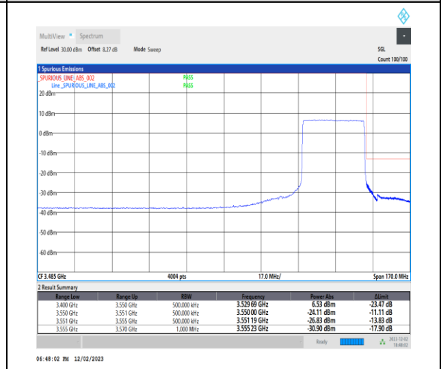
1-N78-3450-3550-PC2-30-30-H-6-CP-QPSK-Outer_Full-78@0-Ant13-1--PASS-see graph
