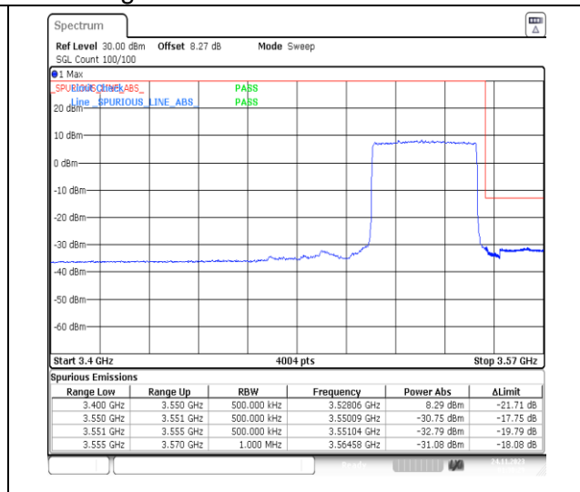
1-N78-3450-3550-PC2-30-40-H-3-DFT-PI2BPSK-Outer_Full-100@0-Ant13-1--PASS-see graph
