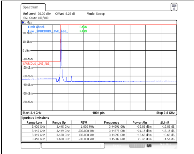
1-N78-3450-3550-PC2-30-15-L-1-DFT-PI2BPSK-Edge_1RB_Left-1@0-Ant13-1--PASS-see graph
