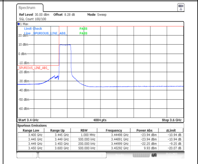
1-N78-3450-3550-PC2-30-15-L-6-CP-QPSK-Outer_Full-38@0-Ant13-1--PASS-see graph
