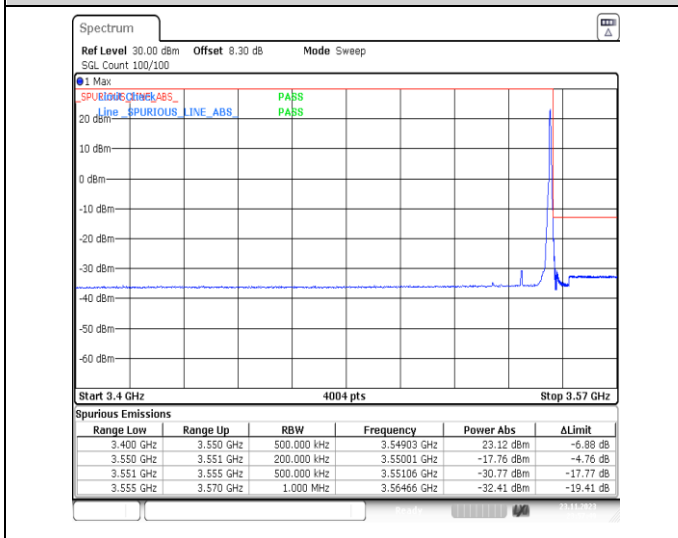
1-N78-3450-3550-PC2-30-20-H-5-CP-QPSK-Edge_1RB_Right-1@50-Ant13-1--PASS-see graph
