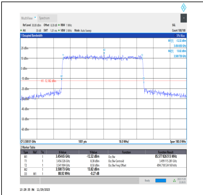
NTNV_N78-3450-3550_PC2_30_90_M_TID4_Ant13#1
