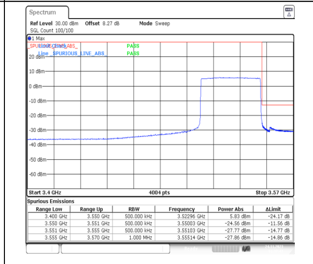
1-N78-3450-3550-PC2-30-40-H-6-CP-QPSK-Outer_Full-106@0-Ant13-1--PASS-see graph
