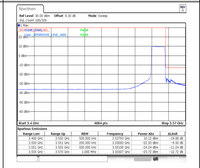
1-N78-3450-3550-PC2-30-15-H-6-CP-QPSK-Outer_Full-38@0-Ant13-1--PASS-see graph
