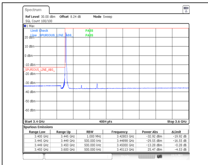
1-N78-3450-3550-PC2-30-40-L-1-DFT-PI2BPSK-Edge_1RB_Left-1@0-Ant13-1--PASS-see graph
