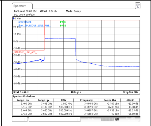
1-N78-3450-3550-PC2-30-50-L-6-CP-QPSK-Outer_Full-133@0-Ant13-1--PASS-see graph
