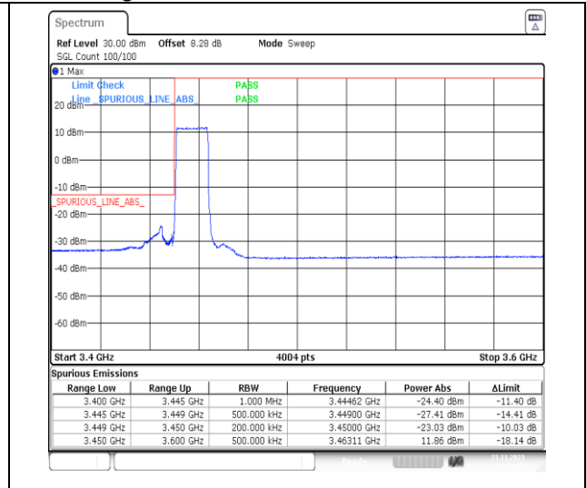
1-N78-3450-3550-PC2-30-15-L-3-DFT-PI2BPSK-Outer_Full-36@0-Ant13-1--PASS-see graph
