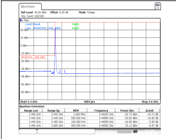
1-N78-3450-3550-PC2-30-15-L-4-CP-QPSK-Edge_1RB_Left-1@0-Ant13-1--PASS-see graph
