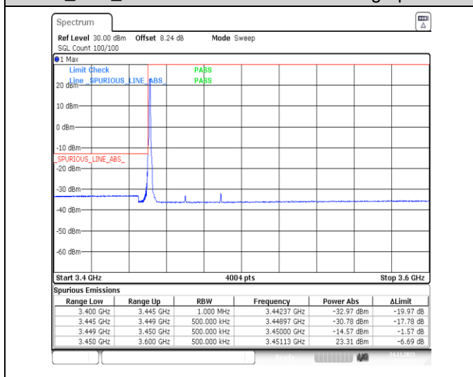
1-N78-3450-3550-PC2-30-40-L-4-CP-QPSK-Edge_1RB_Left-1@0-Ant13-1--PASS-see graph
