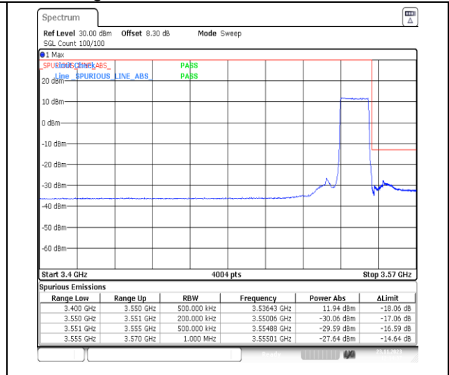
1-N78-3450-3550-PC2-30-15-H-3-DFT-PI2BPSK-Outer_Full-36@0-Ant13-1--PASS-see graph
