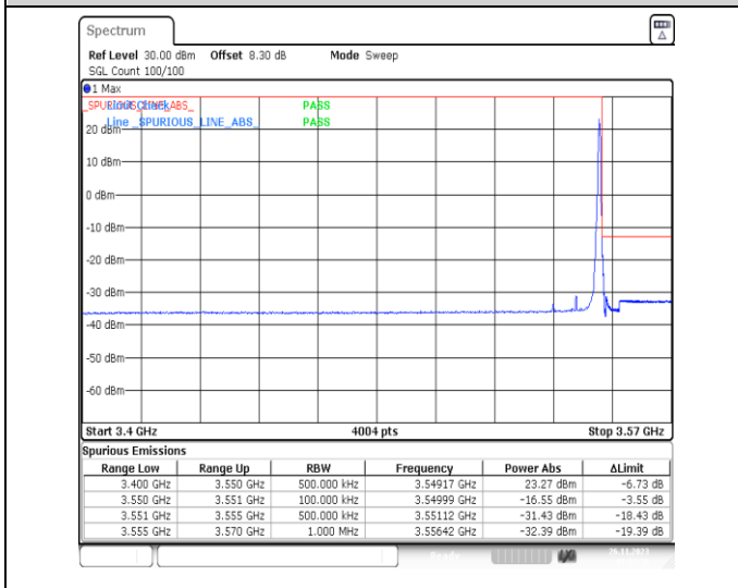
1-N78-3450-3550-PC2-30-15-H-5-CP-QPSK-Edge_1RB_Right-1@37-Ant13-1--PASS-see graph
