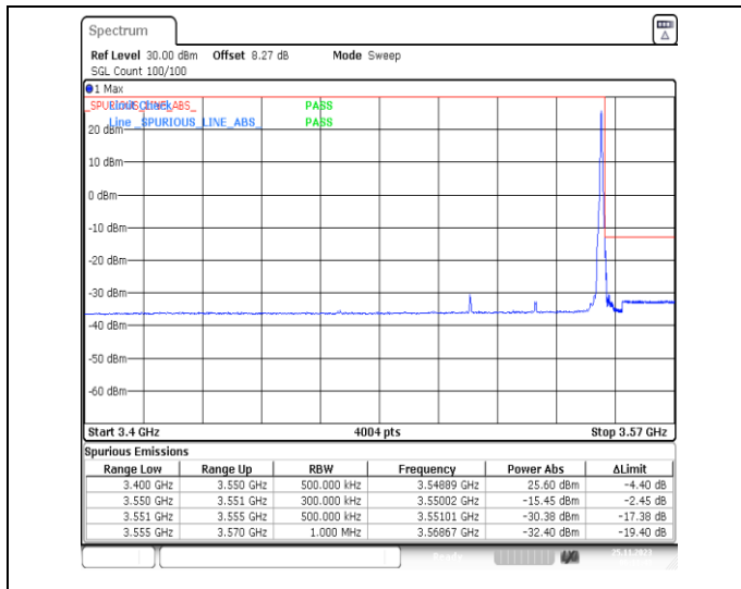
1-N78-3450-3550-PC2-30-40-H-2-DFT-PI2BPSK-Edge_1RB_Right-1@105-Ant13-1--PASS-see graph
