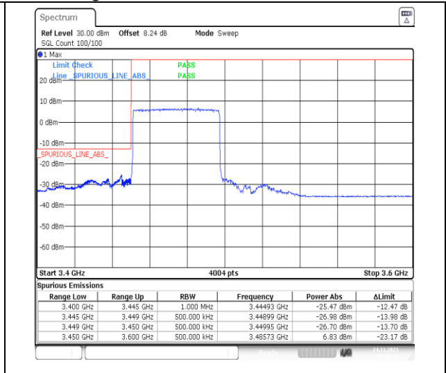
1-N78-3450-3550-PC2-30-50-L-3-DFT-PI2BPSK-Outer_Full-128@0-Ant13-1--PASS-see graph
