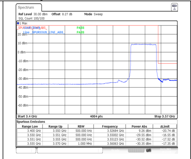
1-N78-3450-3550-PC2-30-30-H-3-DFT-PI2BPSK-Outer_Full-75@0-Ant13-1--PASS-see graph
