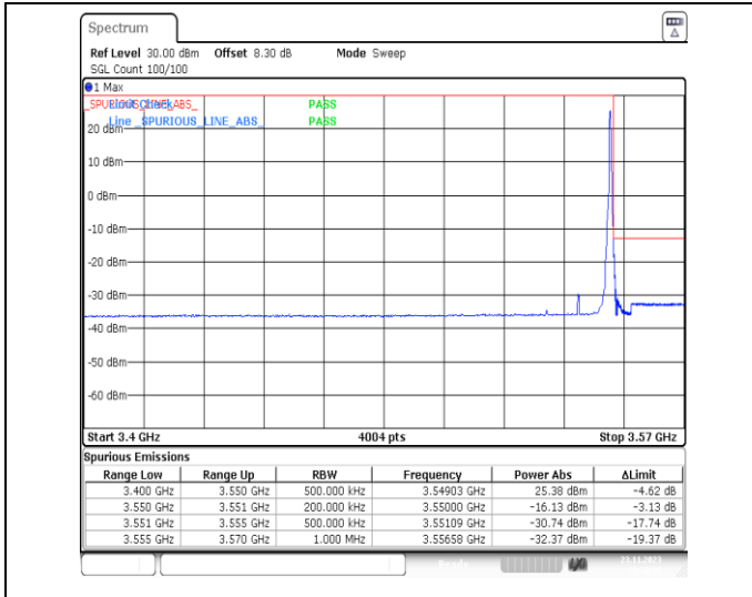
1-N78-3450-3550-PC2-30-20-H-2-DFT-PI2BPSK-Edge_1RB_Right-1@50-Ant13-1--PASS-see graph
