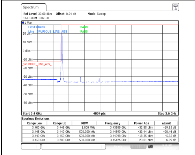
1-N78-3450-3550-PC2-30-50-L-4-CP-QPSK-Edge_1RB_Left-1@0-Ant13-1--PASS-see graph
