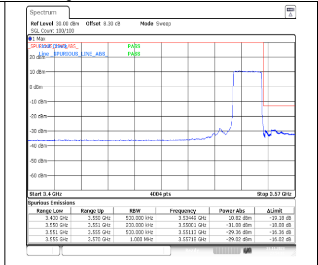
1-N78-3450-3550-PC2-30-20-H-3-DFT-PI2BPSK-Outer_Full-50@0-Ant13-1--PASS-see graph
