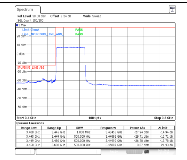
1-N78-3450-3550-PC2-30-40-L-3-DFT-PI2BPSK-Outer_Full-100@0-Ant13-1--PASS-see graph
