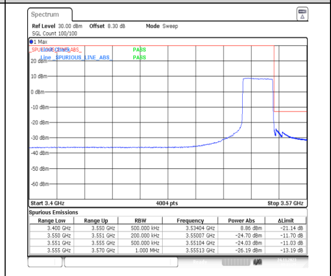
1-N78-3450-3550-PC2-30-20-H-6-CP-QPSK-Outer_Full-51@0-Ant13-1--PASS-see graph
