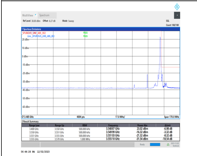
1-N78-3450-3550-PC2-30-30-H-5-CP-QPSK-Edge_1RB_Right-1@77-Ant13-1--PASS-see graph
