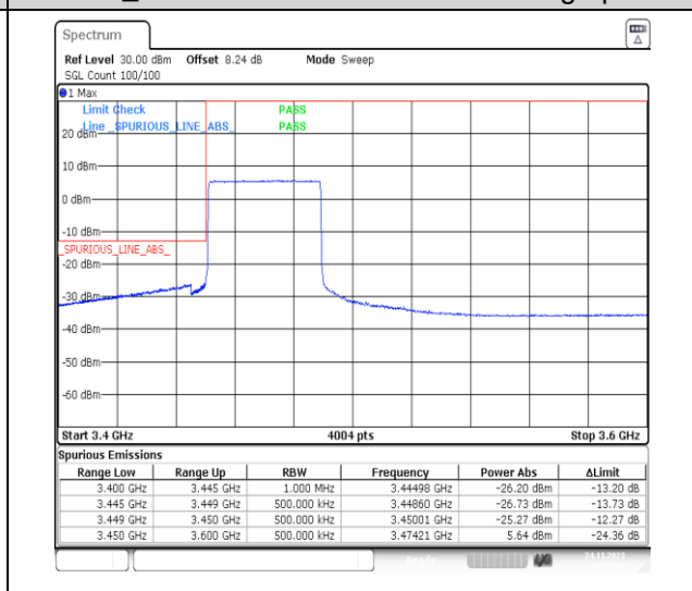
1-N78-3450-3550-PC2-30-40-L-6-CP-QPSK-Outer_Full-106@0-Ant13-1--PASS-see graph
