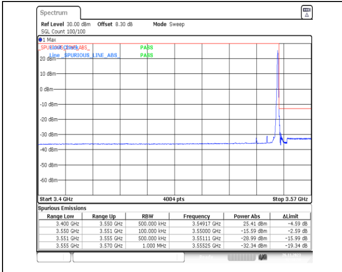
1-N78-3450-3550-PC2-30-15-H-2-DFT-PI2BPSK-Edge_1RB_Right-1@37-Ant13-1--PASS-see graph
