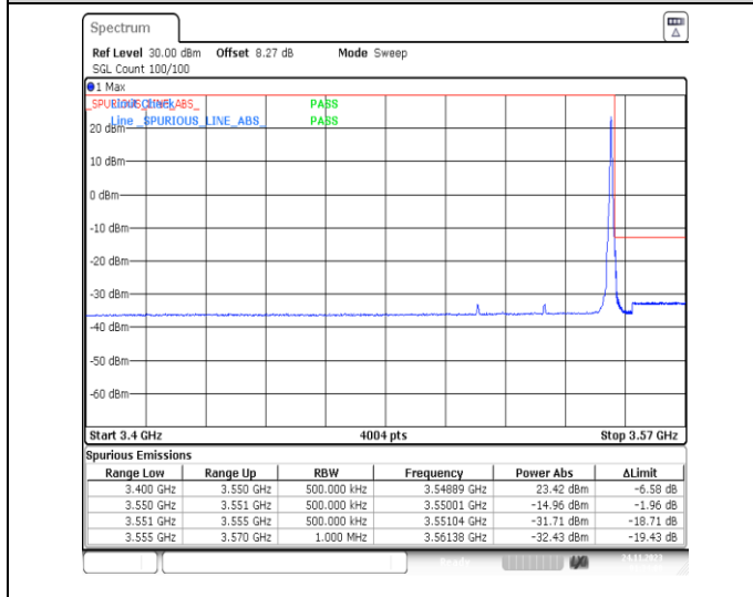
1-N78-3450-3550-PC2-30-40-H-5-CP-QPSK-Edge_1RB_Right-1@105-Ant13-1--PASS-see graph
