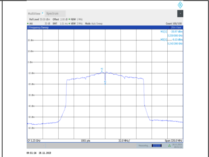
11ax160MIMO-Ant25-5250_UNII-1-PASS
