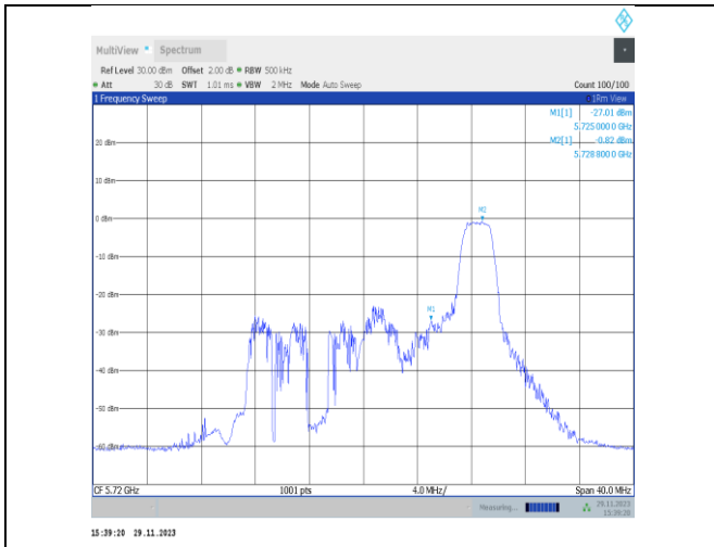
11ax20MIMO-Ant22-5720 UNII-3-26Tone-RU8-PASS
