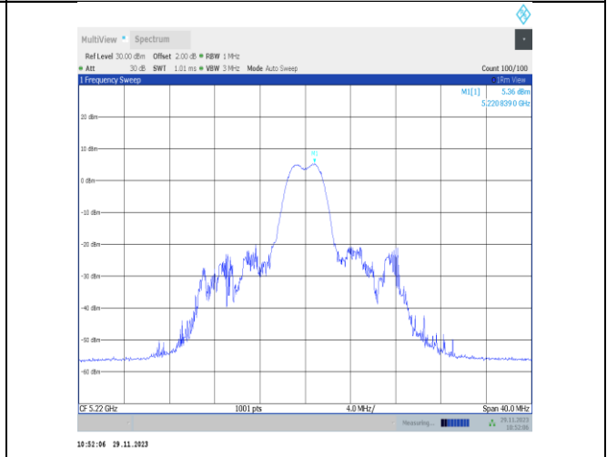
11ax20MIMO-Ant25-5220-26Tone-RU4-PASS
