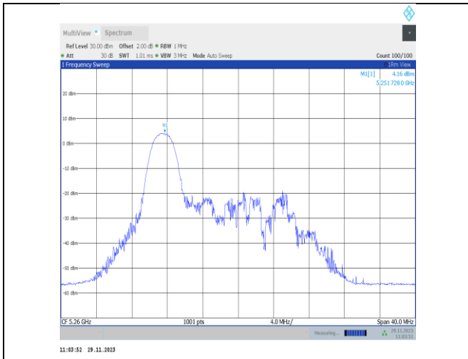
11ax20MIMO-Ant22-5260-26Tone-RU0-PASS
