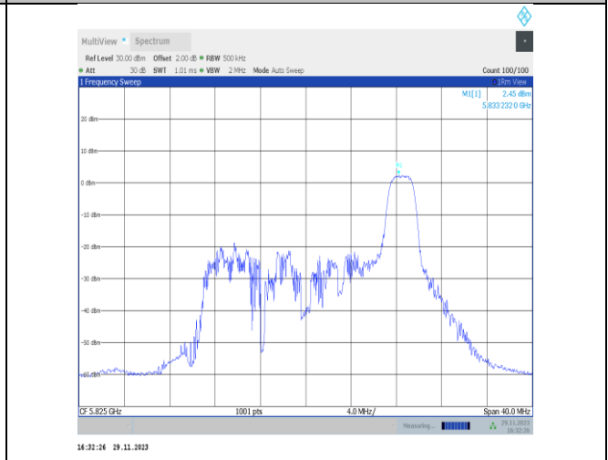
11ax20MIMO-Ant25-5825-26Tone-RU8-PASS
