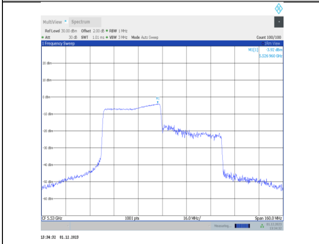
11ax80MIMO-Ant22-5530-484Tone-RU65-PASS
