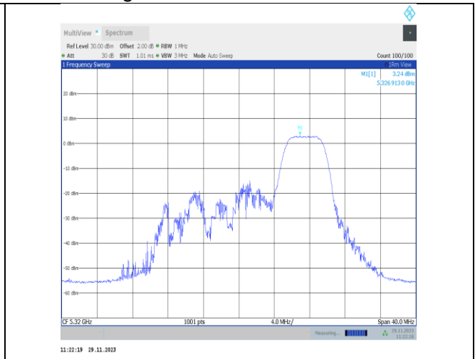
11ax20MIMO-Ant22-5320-52Tone-RU40-PASS
