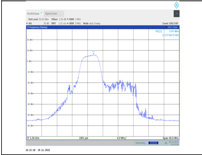
11ax20MIMO-Ant25-5580-52Tone-RU38-PASS
