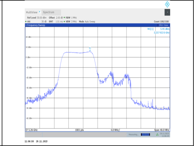
11ax20MIMO-Ant25-5260-106Tone-RU53-PASS
