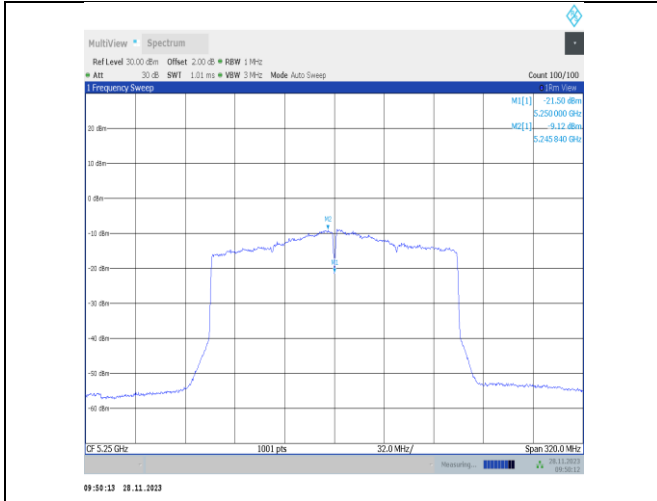
11ax160MIMO-Ant22-5250_UNII-1-PASS
