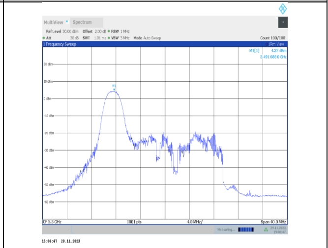
11ax20MIMO-Ant25-5500-26Tone-RU0-PASS
