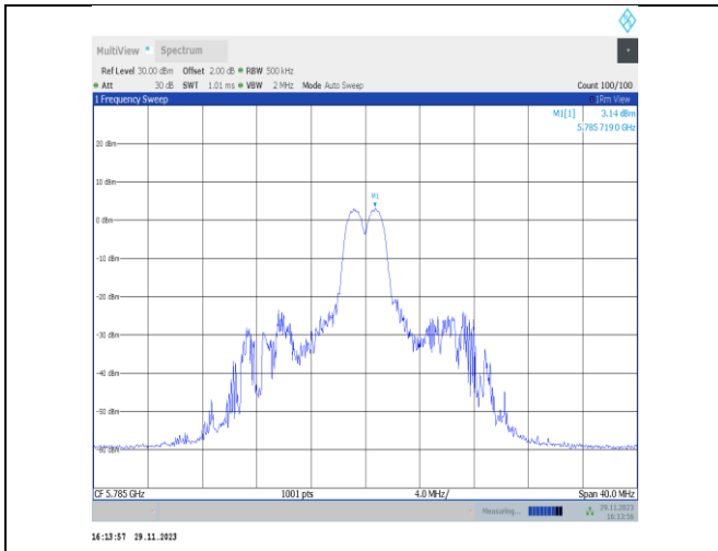
11ax20MIMO-Ant22-5785-26Tone-RU4-PASS
