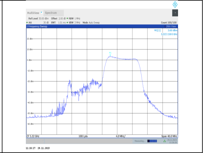
11ax20MIMO-Ant25-5320-106Tone-RU54-PASS
