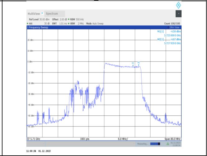
11ax40MIMO-Ant25-5710_UNII-3-242Tone-RU62-PASS
