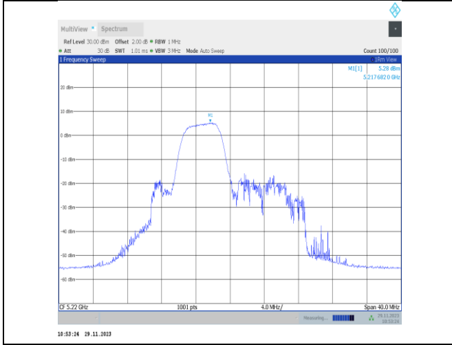
11ax20MIMO-Ant25-5220-52Tone-RU38-PASS
