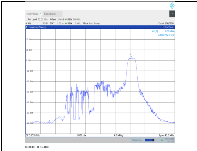
11ax20MIMO-Ant22-5825-26Tone-RU8-PASS
