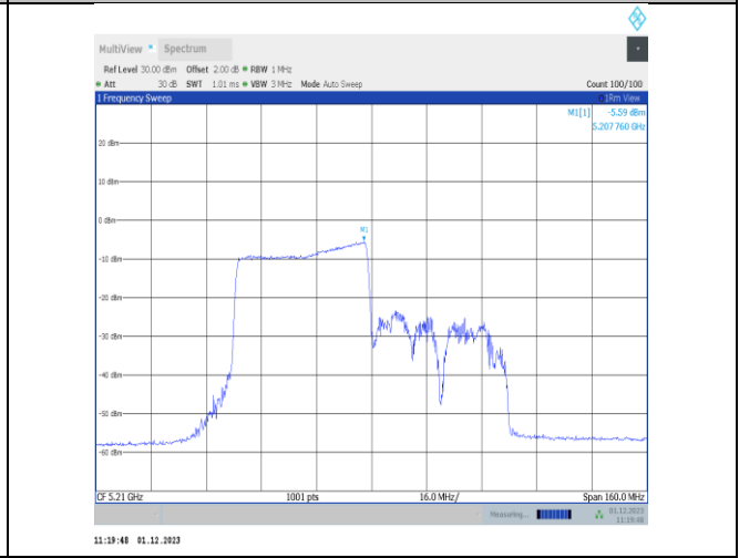
11ax80MIMO-Ant25-5210-484Tone-RU65-PASS
