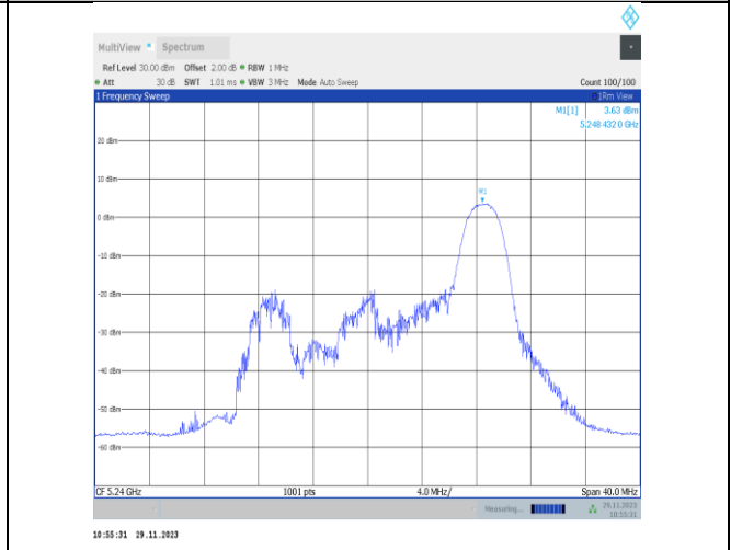
11ax20MIMO-Ant25-5240-26Tone-RU8-PASS
