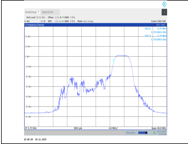
11ax20MIMO-Ant25-5720 UNII-2C-52Tone-RU40-PASS
