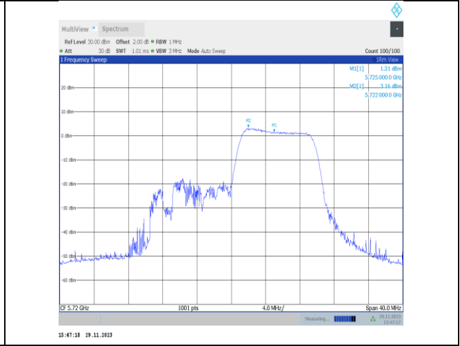
11ax20MIMO-Ant25-5720 UNII-2C-106Tone-RU54-PASS
