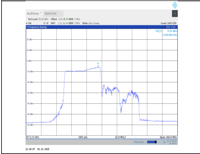
11ax80MIMO-Ant22-5210-484Tone-RU65-PASS
