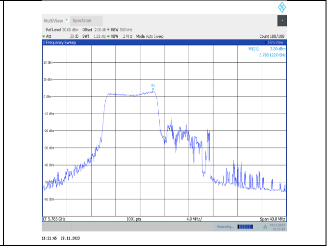
11ax20MIMO-Ant25-5785-106Tone-RU53-PASS
