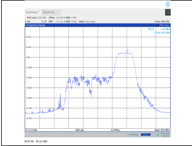
11ax20MIMO-Ant25-5240-52Tone-RU40-PASS
