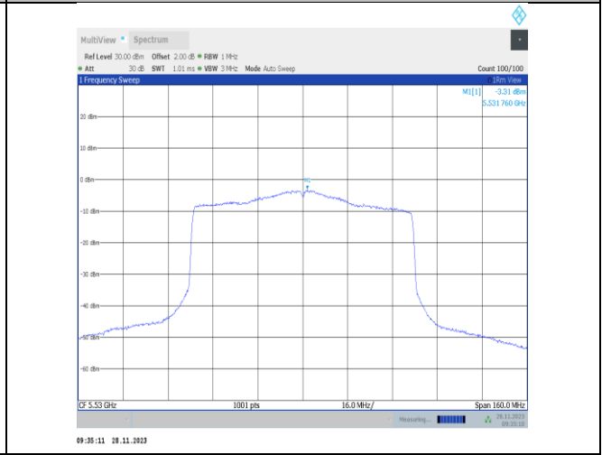
11ax80MIMO-Ant25-5530-PASS
