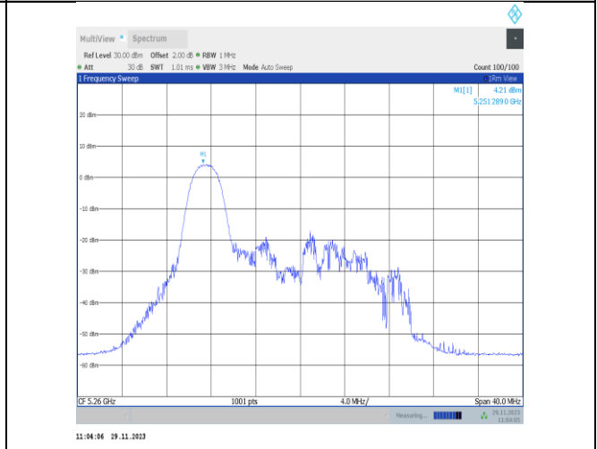
11ax20MIMO-Ant25-5260-26Tone-RU0-PASS
