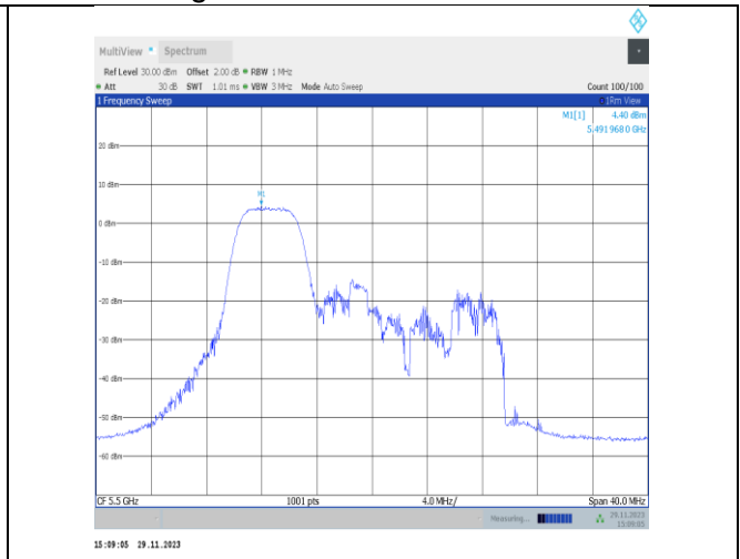
11ax20MIMO-Ant22-5500-52Tone-RU37-PASS
