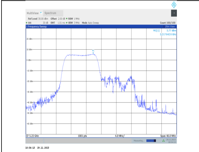
11ax20MIMO-Ant22-5220-106Tone-RU53-PASS
