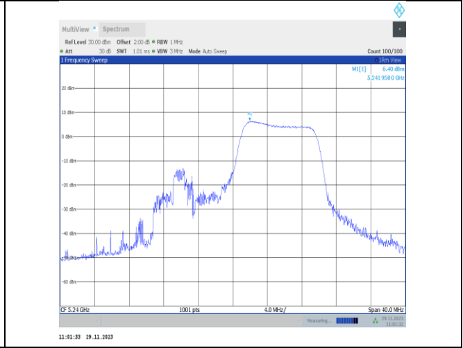
11ax20MIMO-Ant25-5240-106Tone-RU54-PASS
