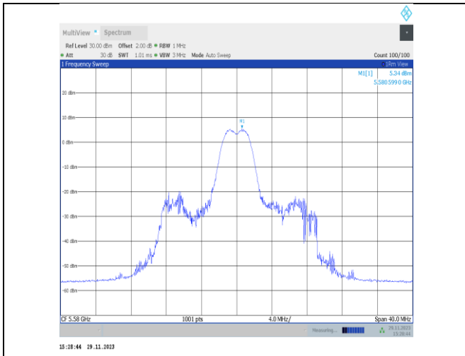
11ax20MIMO-Ant22-5580-26Tone-RU4-PASS
