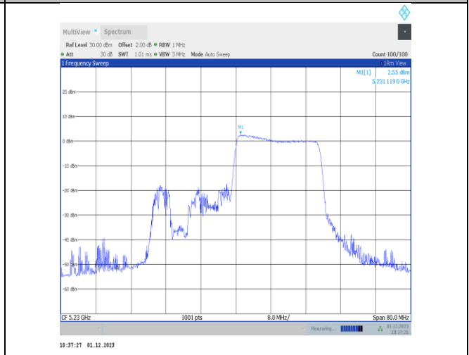
11ax40MIMO-Ant25-5230-242Tone-RU62-PASS
