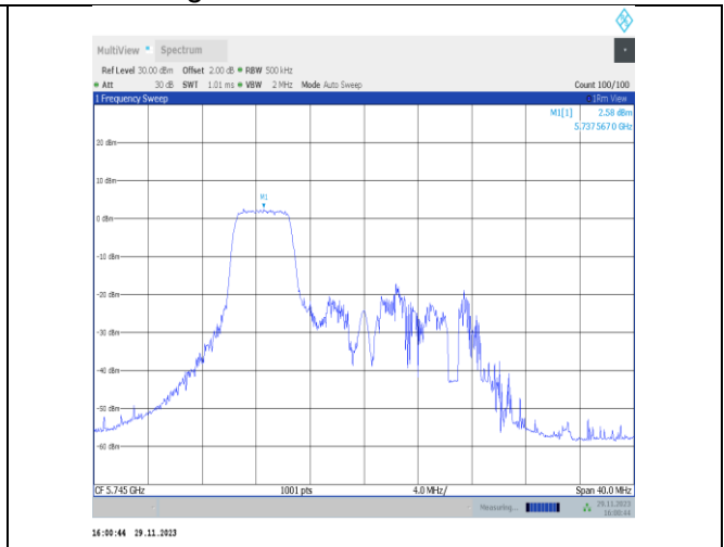
11ax20MIMO-Ant22-5745-52Tone-RU37-PASS
