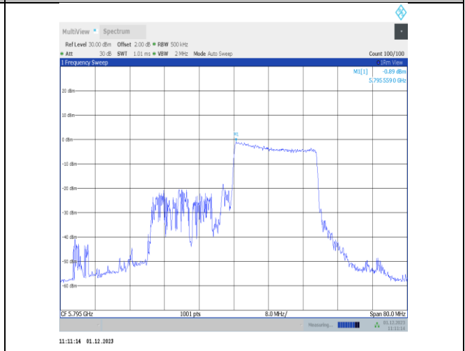
11ax40MIMO-Ant25-5795-242Tone-RU62-PASS
