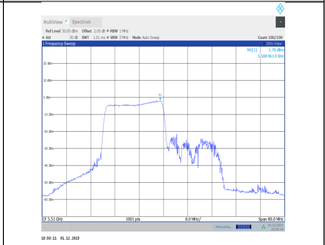
11ax40MIMO-Ant25-5510-242Tone-RU61-PASS
