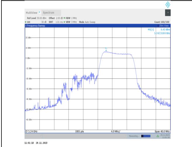
11ax20MIMO-Ant22-5240-106Tone-RU54-PASS
