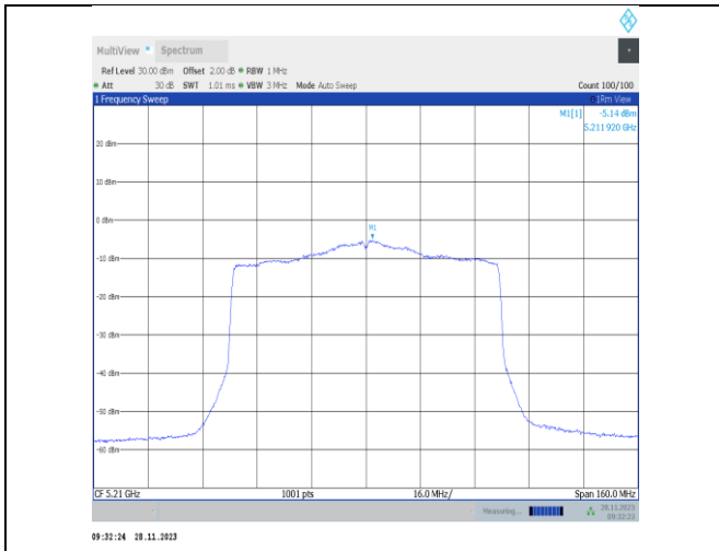
11ax80MIMO-Ant22-5210-PASS
