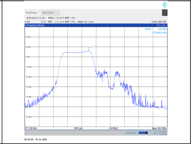
11ax20MIMO-Ant25-5580-106Tone-RU53-PASS
