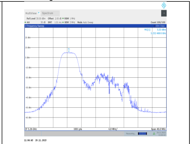
11ax20MIMO-Ant22-5260-52Tone-RU37-PASS
