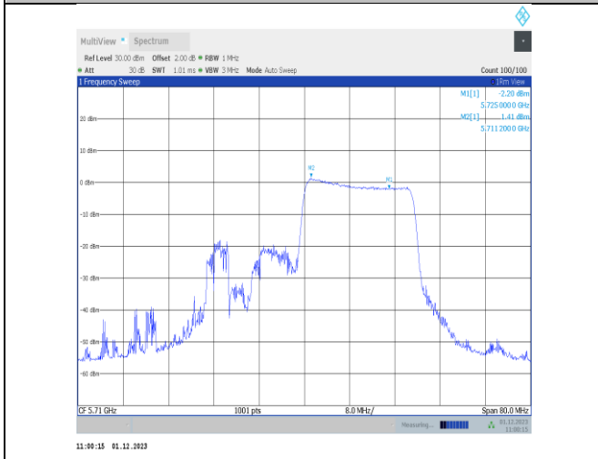
11ax40MIMO-Ant22-5710_UNII-2C-242Tone-RU62-PASS
