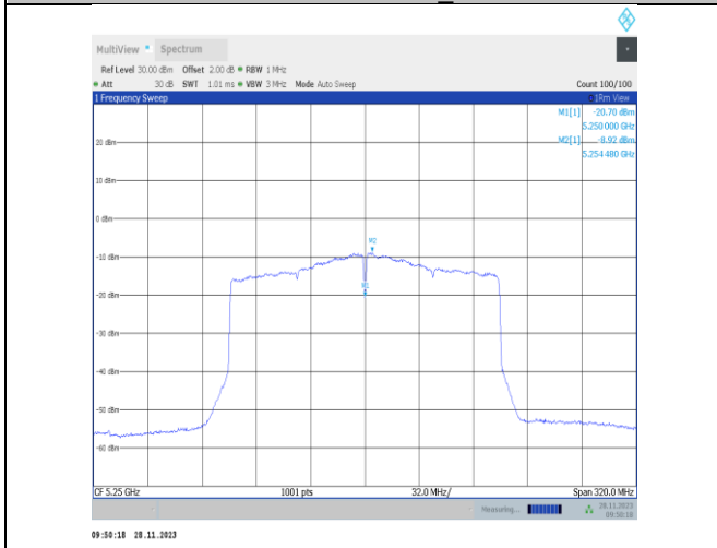
11ax160MIMO-Ant22-5250_UNII-2A-PASS
