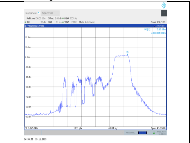
11ax20MIMO-Ant22-5825-52Tone-RU40-PASS
