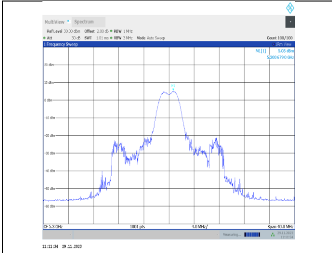
11ax20MIMO-Ant22-5300-26Tone-RU4-PASS
