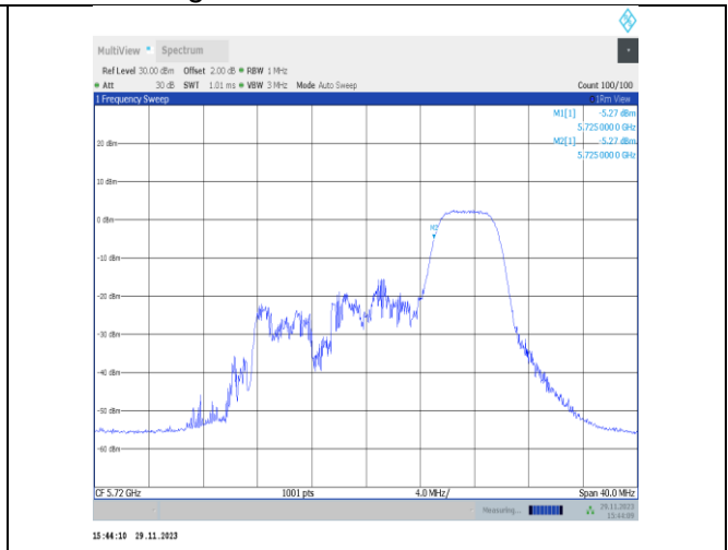
11ax20MIMO-Ant22-5720 UNII-2C-52Tone-RU40-PASS
