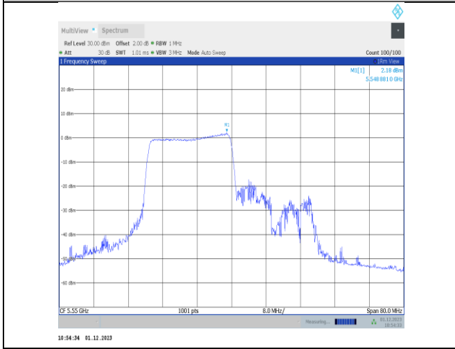
11ax40MIMO-Ant22-5550-242Tone-RU61-PASS
