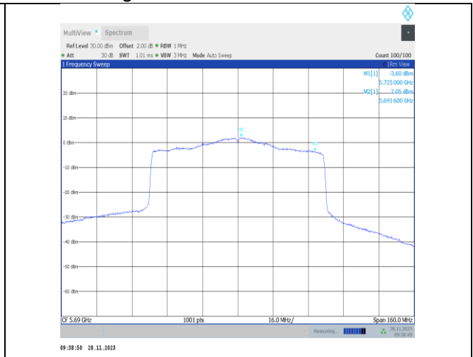
11ax80MIMO-Ant25-5690_UNII-2C-PASS
