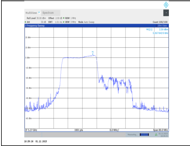
11ax40MIMO-Ant22-5270-242Tone-RU61-PASS
