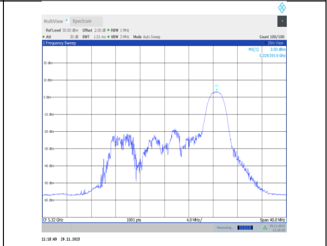
11ax20MIMO-Ant25-5320-26Tone-RU8-PASS
