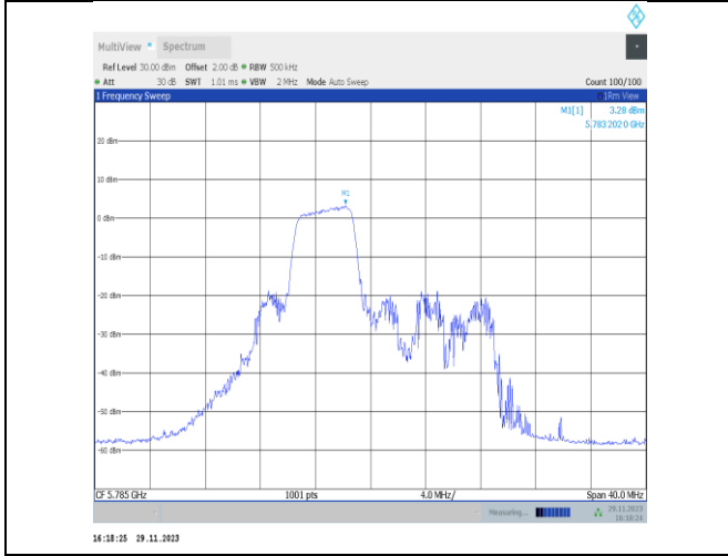
11ax20MIMO-Ant25-5785-52Tone-RU38-PASS
