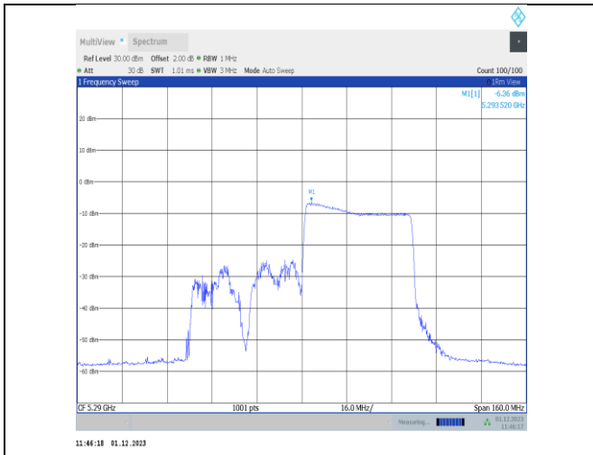
11ax80MIMO-Ant22-5290-484Tone-RU66-PASS
