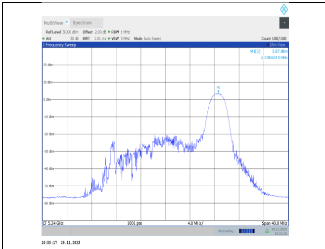
11ax20MIMO-Ant22-5240-26Tone-RU8-PASS
