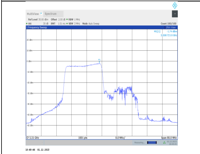
11ax40MIMO-Ant22-5510-242Tone-RU61-PASS
