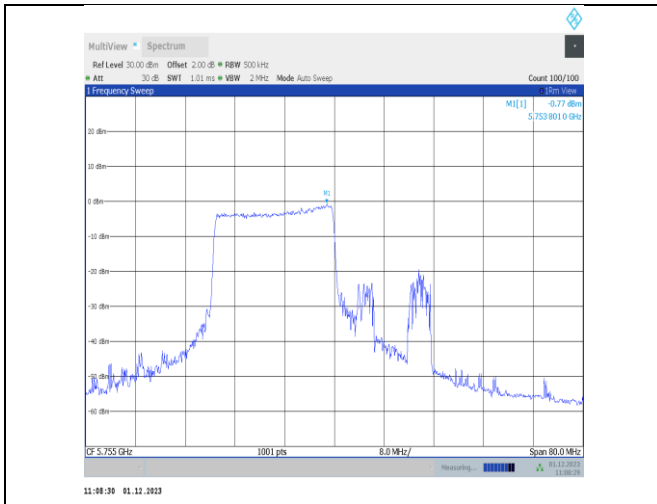
11ax40MIMO-Ant22-5755-242Tone-RU61-PASS
