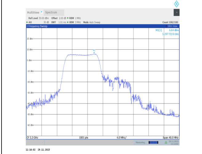
11ax20MIMO-Ant22-5300-106Tone-RU53-PASS
