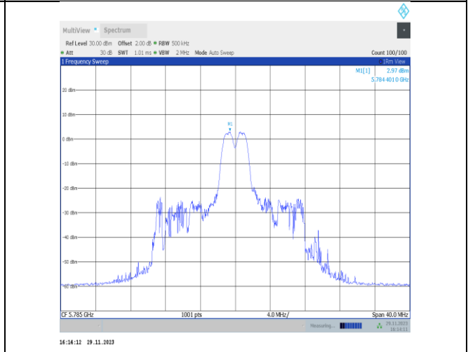
11ax20MIMO-Ant25-5785-26Tone-RU4-PASS
