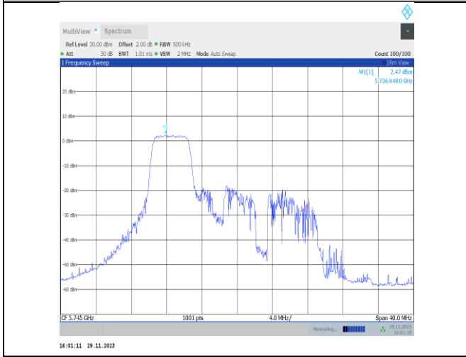
11ax20MIMO-Ant25-5745-52Tone-RU37-PASS
