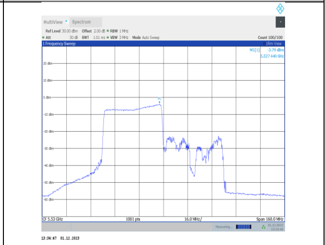
11ax80MIMO-Ant25-5530-484Tone-RU65-PASS
