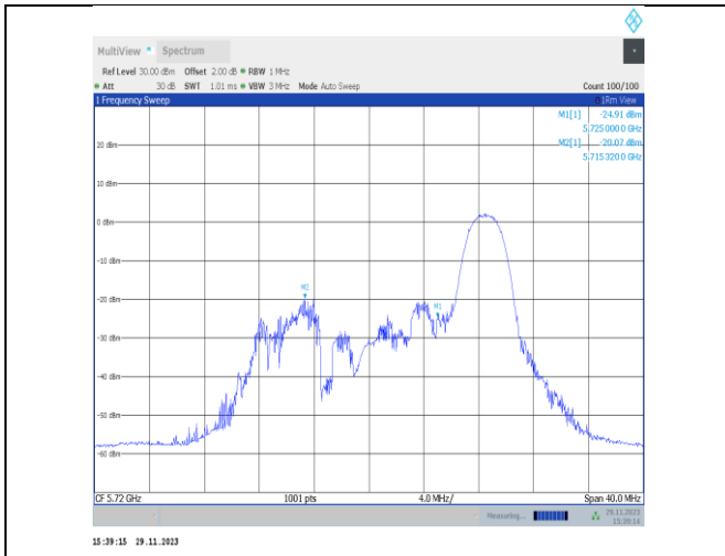
11ax20MIMO-Ant22-5720 UNII-2C-26Tone-RU8-PASS
