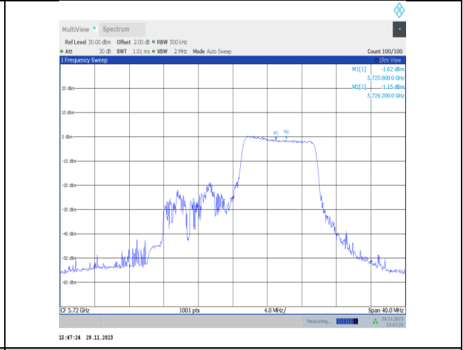
11ax20MIMO-Ant25-5720 UNII-3-106Tone-RU54-PASS
