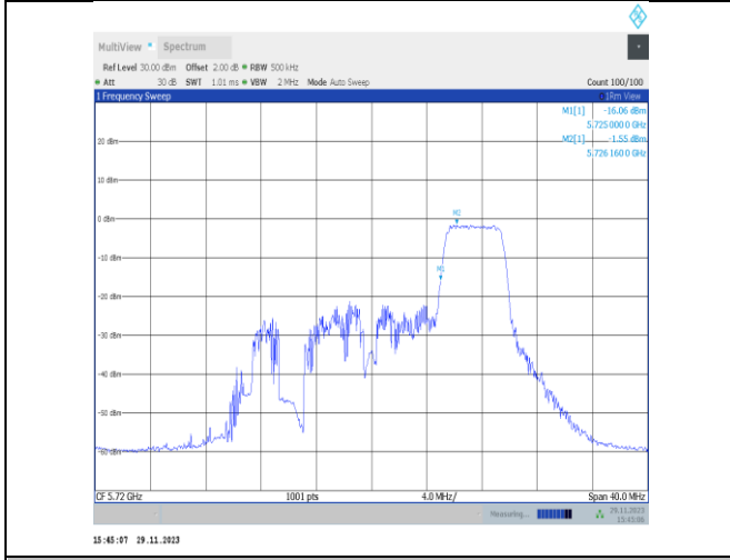
11ax20MIMO-Ant25-5720 UNII-3-52Tone-RU40-PASS
