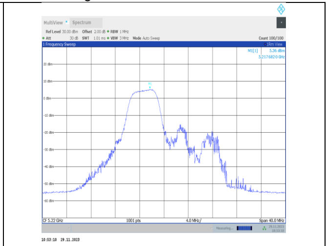
11ax20MIMO-Ant22-5220-52Tone-RU38-PASS
