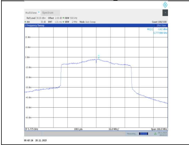
11ax80MIMO-Ant22-5775-PASS
