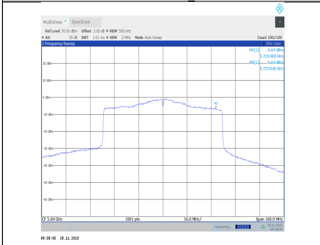
11ax80MIMO-Ant22-5690_UNII-3-PASS
