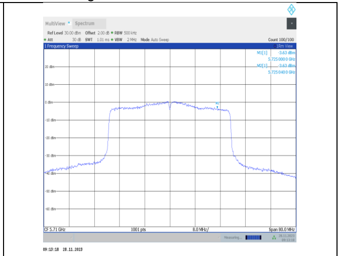
11ax40MIMO-Ant25-5710 UNII-3-PASS
