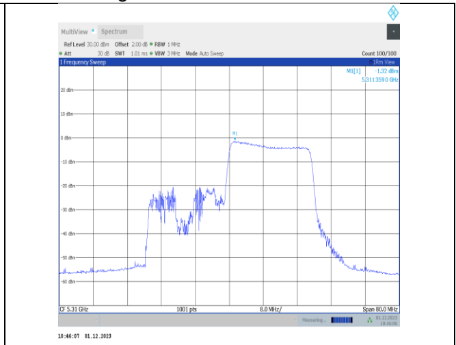
11ax40MIMO-Ant25-5310-242Tone-RU62-PASS
