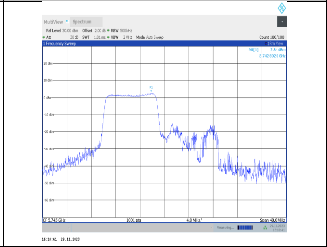
11ax20MIMO-Ant25-5745-106Tone-RU53-PASS
