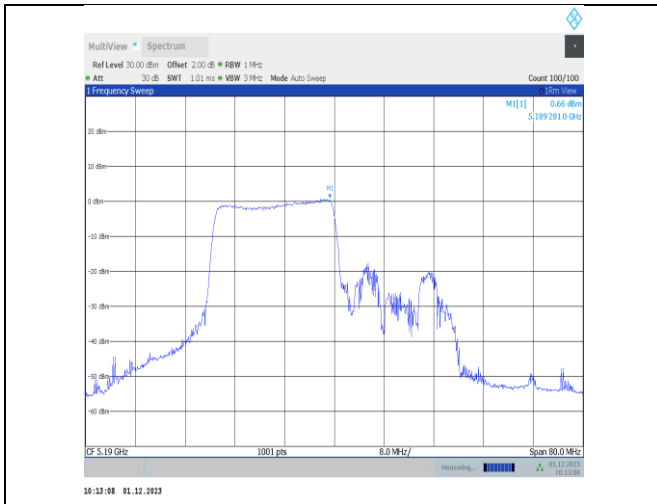
11ax40MIMO-Ant22-5190-242Tone-RU61-PASS
