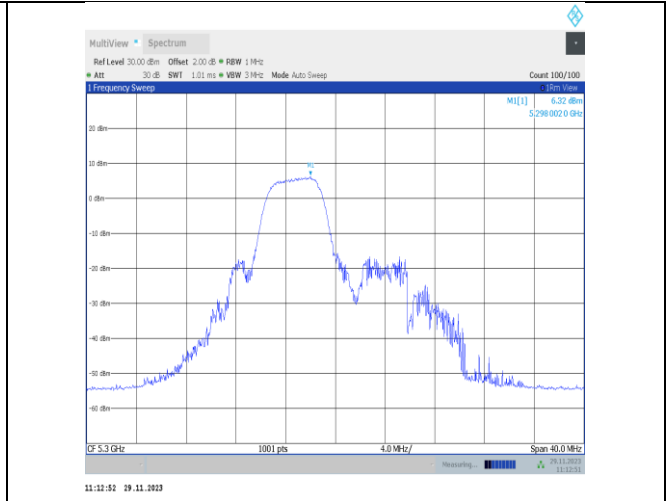
11ax20MIMO-Ant22-5300-52Tone-RU38-PASS
