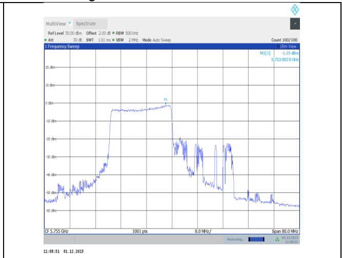
11ax40MIMO-Ant25-5755-242Tone-RU61-PASS
