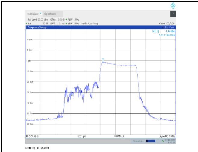
11ax40MIMO-Ant22-5310-242Tone-RU62-PASS
