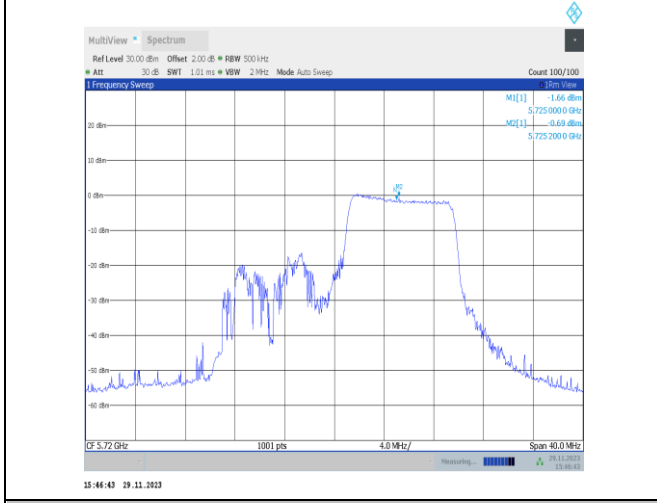
11ax20MIMO-Ant22-5720 UNII-3-106Tone-RU54-PASS
