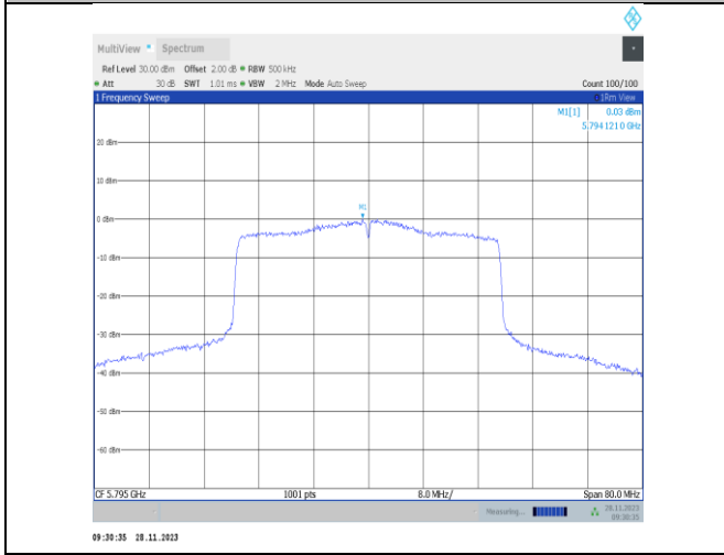
11ax40MIMO-Ant22-5795-PASS
