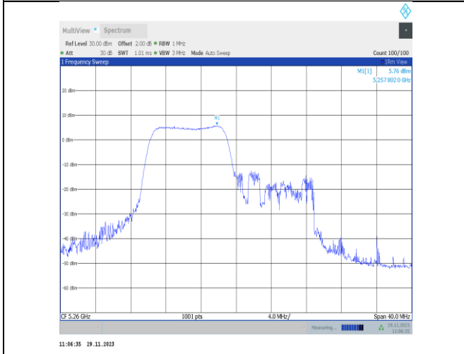
11ax20MIMO-Ant22-5260-106Tone-RU53-PASS
