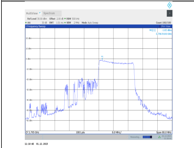
11ax40MIMO-Ant22-5795-242Tone-RU62-PASS
