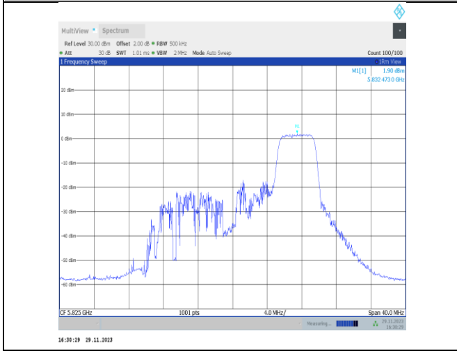
11ax20MIMO-Ant25-5825-52Tone-RU40-PASS
