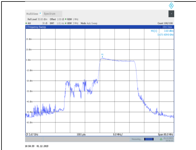
11ax40MIMO-Ant22-5670-242Tone-RU62-PASS
