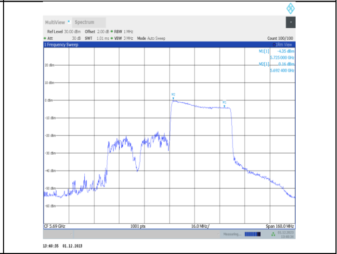
11ax80MIMO-Ant25-5690 UNII-2C-484Tone-RU66-PASS
