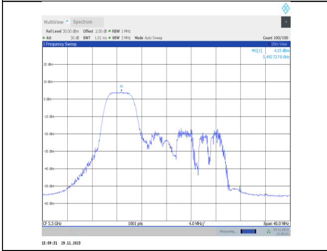
11ax20MIMO-Ant25-5500-52Tone-RU37-PASS
