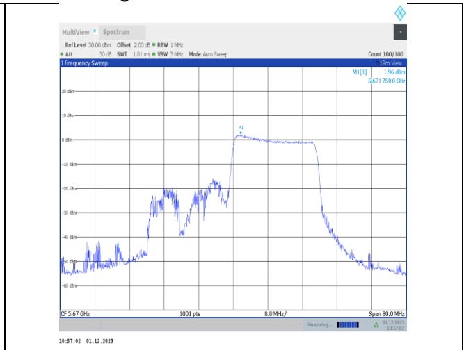
11ax40MIMO-Ant25-5670-242Tone-RU62-PASS
