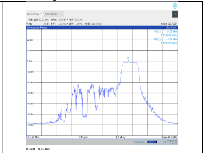
11ax20MIMO-Ant22-5720 UNII-3-52Tone-RU40-PASS
