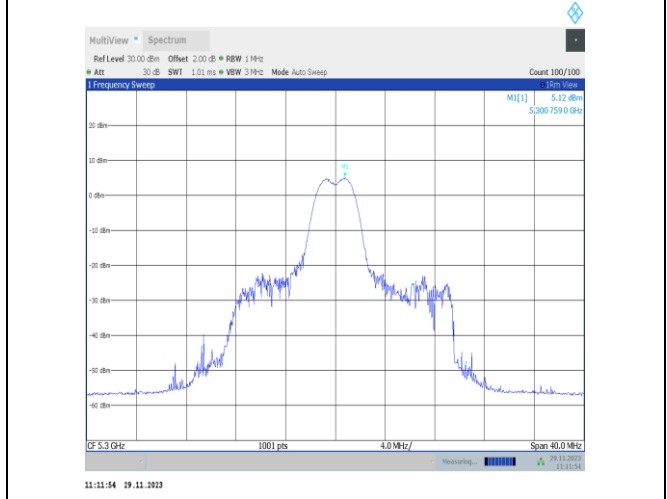
11ax20MIMO-Ant25-5300-26Tone-RU4-PASS
