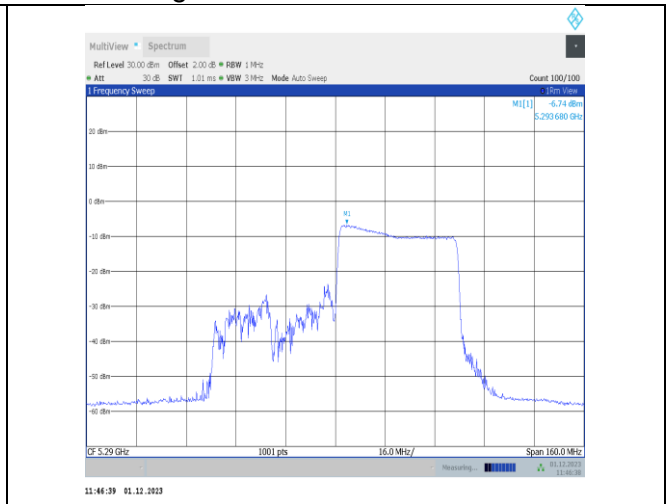
11ax80MIMO-Ant25-5290-484Tone-RU66-PASS
