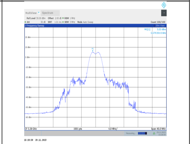
11ax20MIMO-Ant25-5580-26Tone-RU4-PASS
