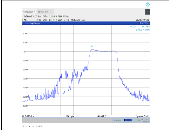
11ax20MIMO-Ant22-5825-106Tone-RU54-PASS
