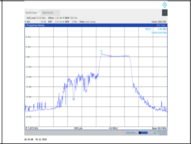
11ax20MIMO-Ant25-5825-106Tone-RU54-PASS
