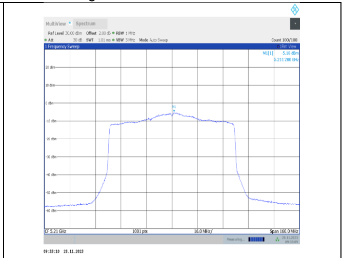
11ax80MIMO-Ant25-5210-PASS
