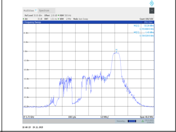
11ax20MIMO-Ant25-5720 UNII-3-26Tone-RU8-PASS
