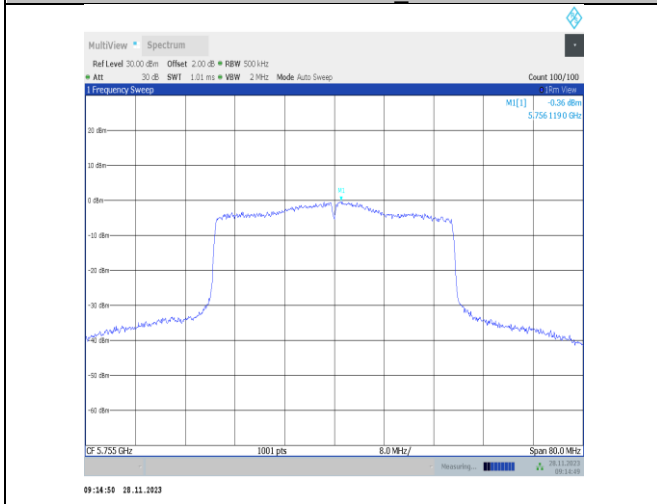
11ax40MIMO-Ant22-5755-PASS
