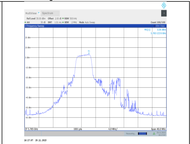
11ax20MIMO-Ant22-5785-52Tone-RU38-PASS
