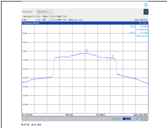
11ax80MIMO-Ant22-5690_UNII-2C-PASS
