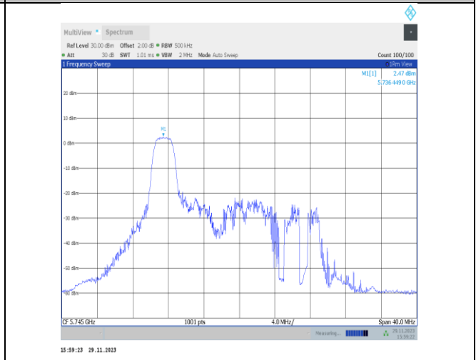
11ax20MIMO-Ant25-5745-26Tone-RU0-PASS
