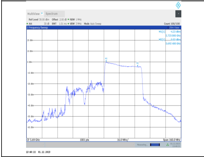
11ax80MIMO-Ant22-5690 UNII-2C-484Tone-RU66-PASS
