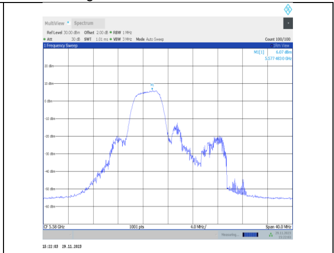
11ax20MIMO-Ant22-5580-52Tone-RU38-PASS
