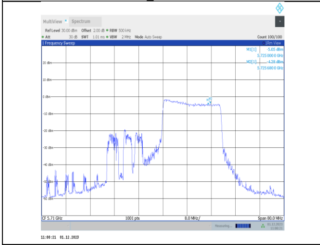
11ax40MIMO-Ant22-5710_UNII-3-242Tone-RU62-PASS
