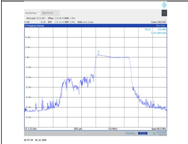
11ax40MIMO-Ant22-5230-242Tone-RU62-PASS
