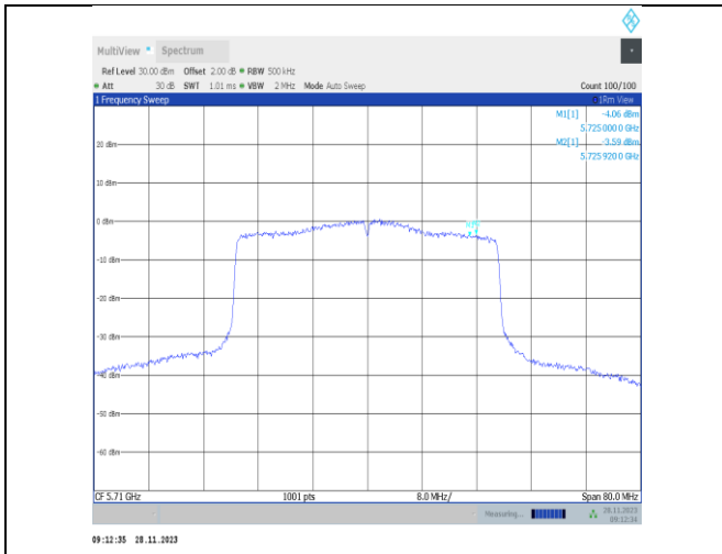
11ax40MIMO-Ant22-5710 UNII-3-PASS
