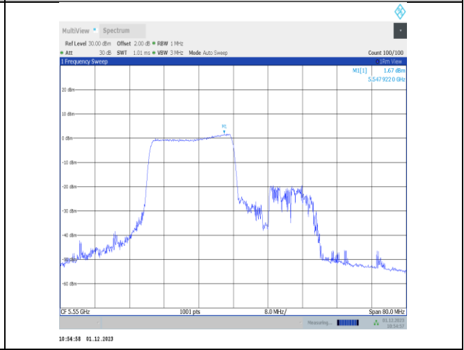
11ax40MIMO-Ant25-5550-242Tone-RU61-PASS
