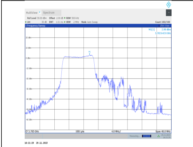
11ax20MIMO-Ant22-5785-106Tone-RU53-PASS
