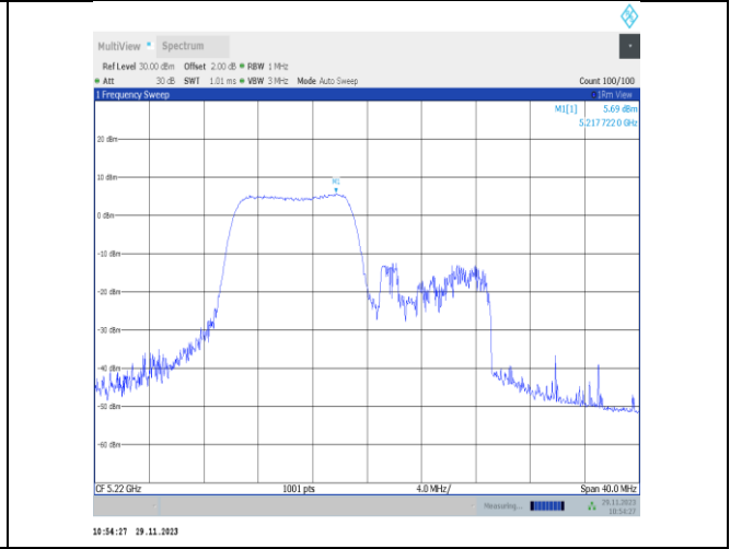
11ax20MIMO-Ant25-5220-106Tone-RU53-PASS
