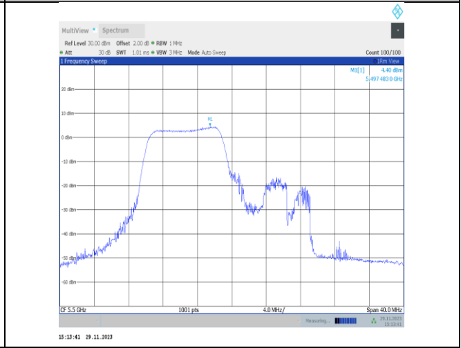
11ax20MIMO-Ant25-5500-106Tone-RU53-PASS
