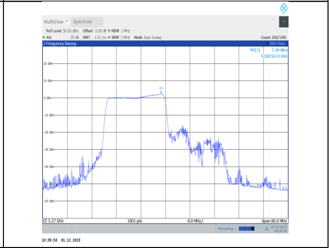
11ax40MIMO-Ant25-5270-242Tone-RU61-PASS
