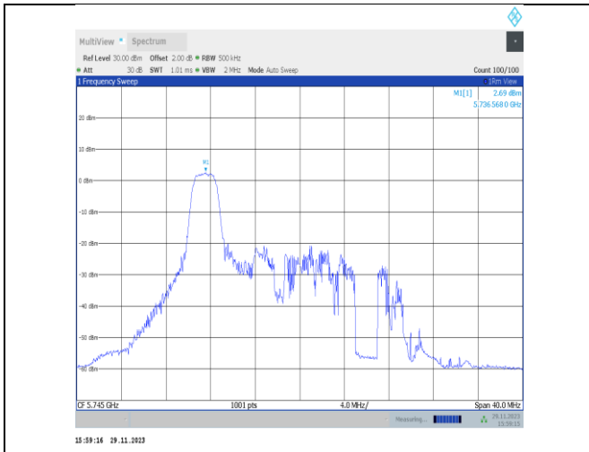
11ax20MIMO-Ant22-5745-26Tone-RU0-PASS
