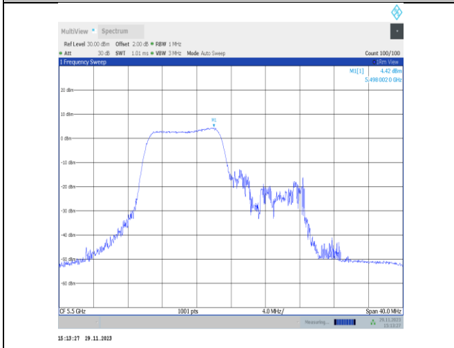
11ax20MIMO-Ant22-5500-106Tone-RU53-PASS
