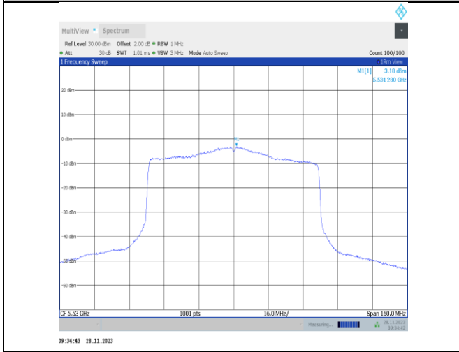
11ax80MIMO-Ant22-5530-PASS
