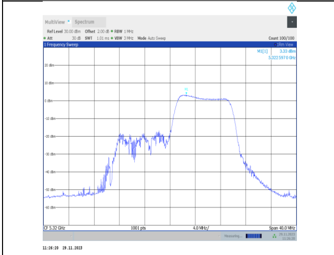
11ax20MIMO-Ant22-5320-106Tone-RU54-PASS
