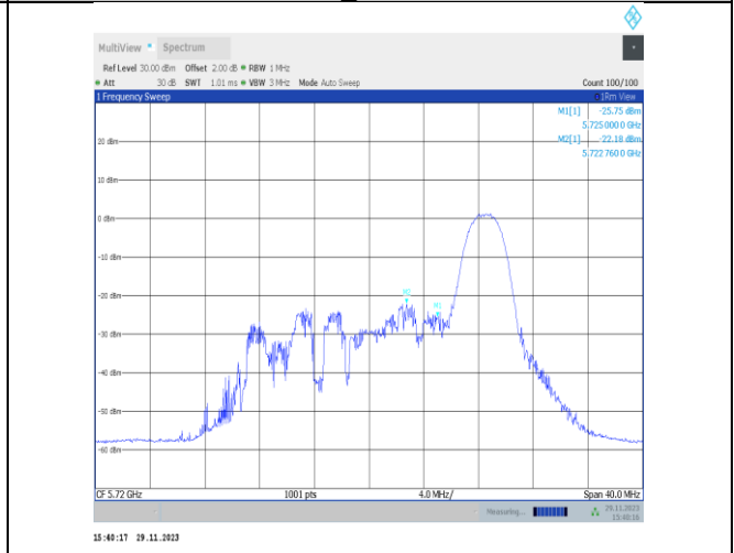
11ax20MIMO-Ant25-5720 UNII-2C-26Tone-RU8-PASS
