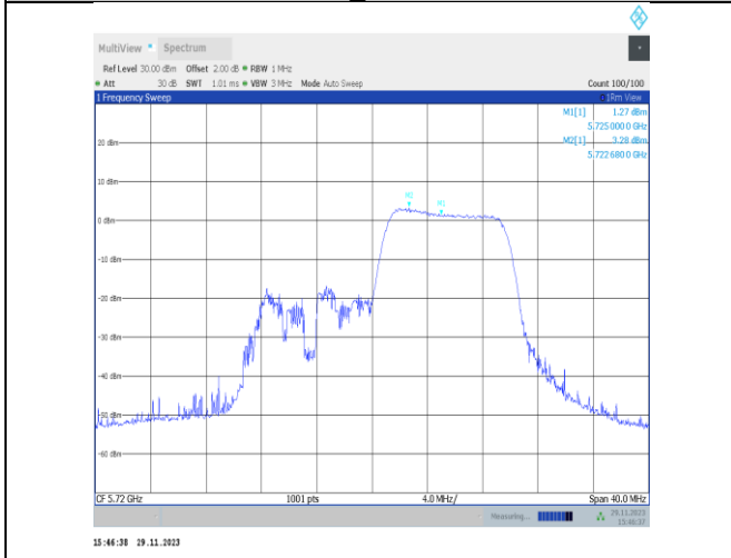
11ax20MIMO-Ant22-5720 UNII-2C-106Tone-RU54-PASS
