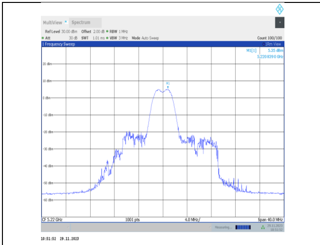
11ax20MIMO-Ant22-5220-26Tone-RU4-PASS
