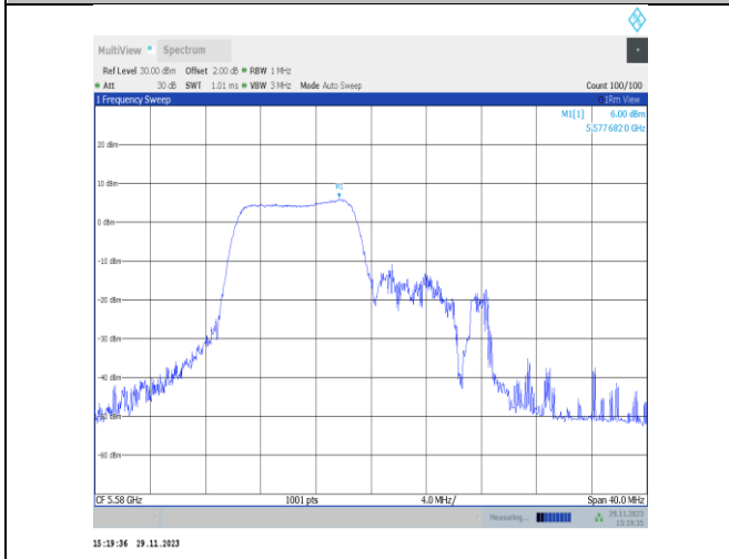
11ax20MIMO-Ant22-5580-106Tone-RU53-PASS
