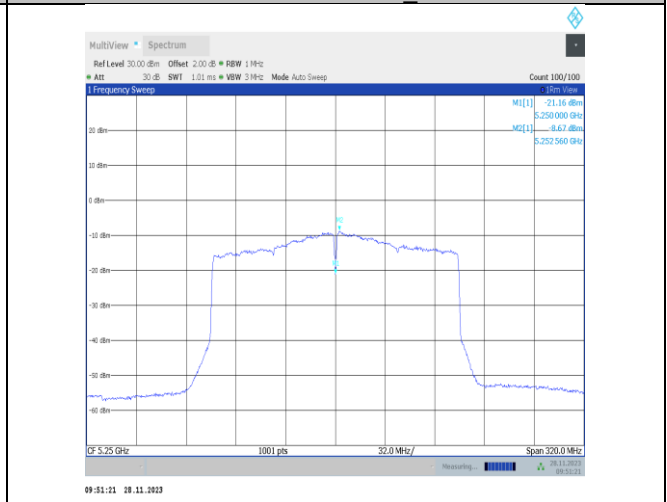
11ax160MIMO-Ant25-5250_UNII-2A-PASS
