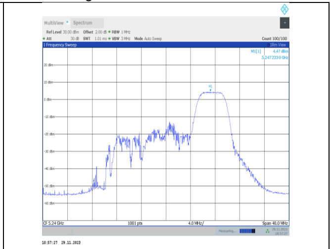
11ax20MIMO-Ant22-5240-52Tone-RU40-PASS
