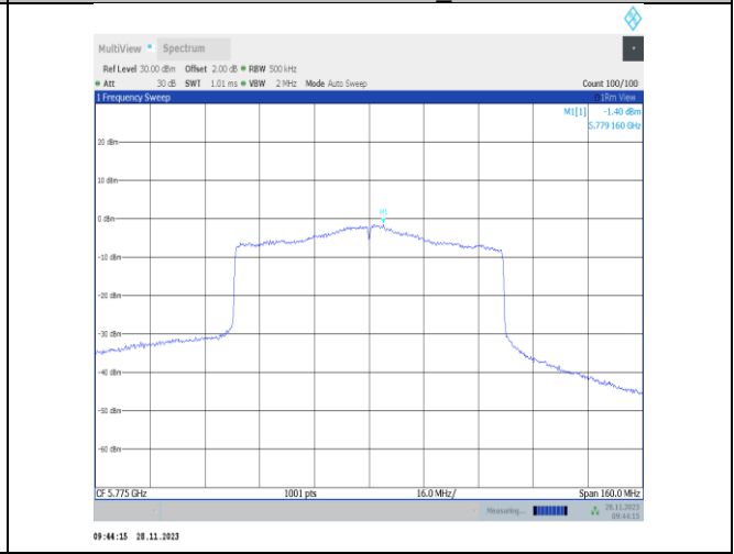
11ax80MIMO-Ant25-5775-PASS
