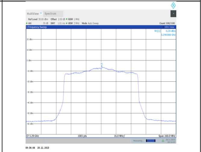
11ax80MIMO-Ant25-5290-PASS
