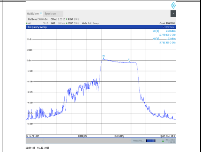
11ax40MIMO-Ant25-5710_UNII-2C-242Tone-RU62-PASS
