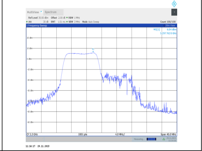
11ax20MIMO-Ant25-5300-106Tone-RU53-PASS
