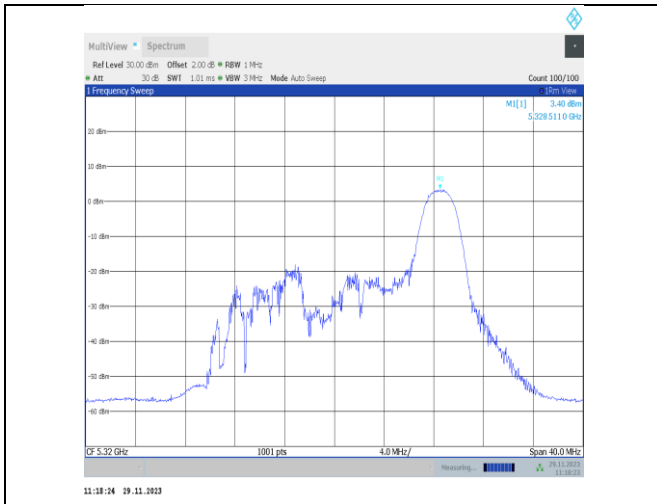
11ax20MIMO-Ant22-5320-26Tone-RU8-PASS
