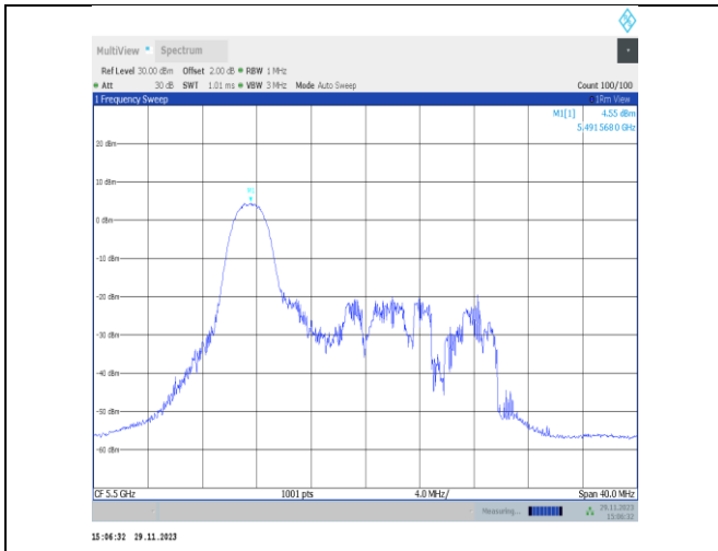
11ax20MIMO-Ant22-5500-26Tone-RU0-PASS
