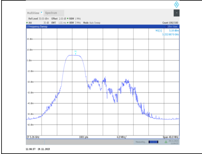
11ax20MIMO-Ant25-5260-52Tone-RU37-PASS
