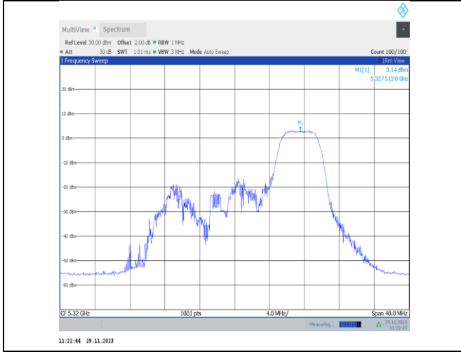
11ax20MIMO-Ant25-5320-52Tone-RU40-PASS
