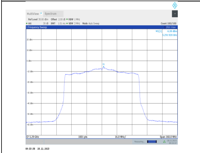
11ax80MIMO-Ant22-5290-PASS
