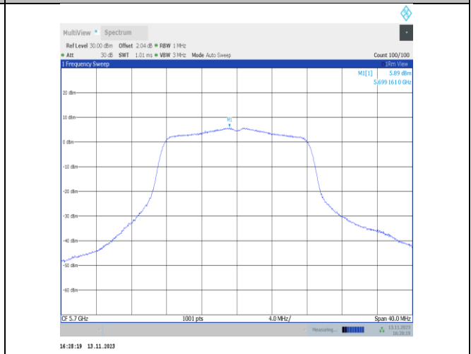
11a-CDD-Ant25-5700-PASS
