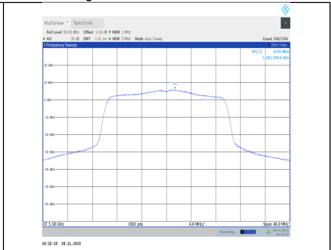
11ax20MIMO-Ant25-5580-PASS
