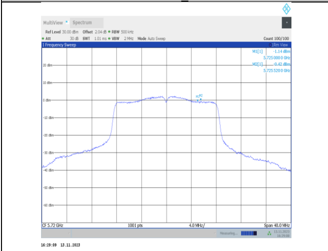
11a-CDD-Ant22-5720 UNII-3-PASS
