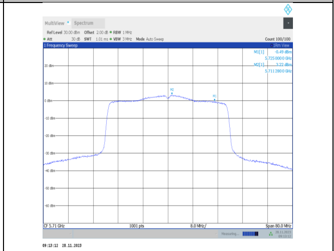
11ax40MIMO-Ant25-5710 UNII-2C-PASS
