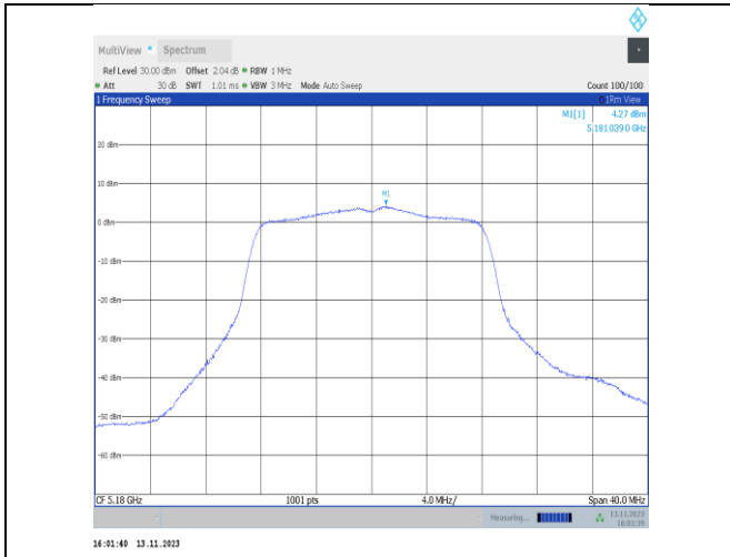
11a-CDD-Ant22-5180-PASS
