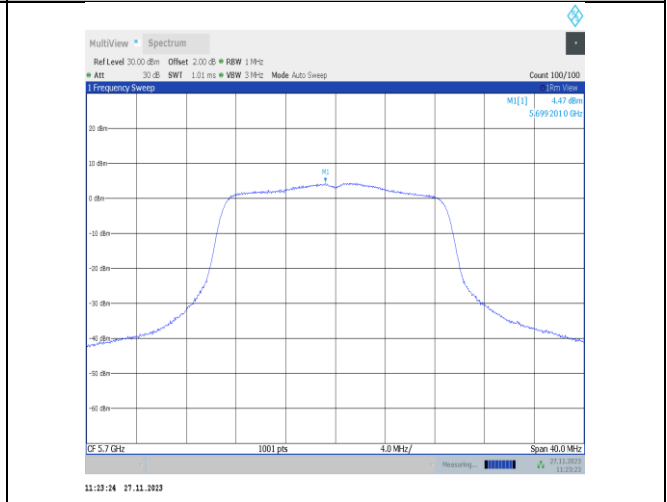
11n20MIMO-Ant25-5700-PASS
