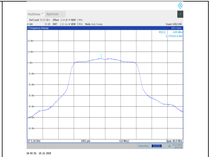
11a-CDD-Ant25-5180-PASS
