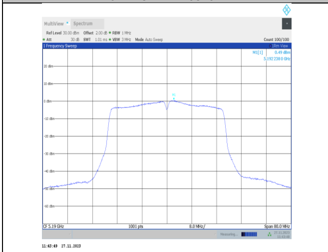
11n40MIMO-Ant22-5190-PASS
