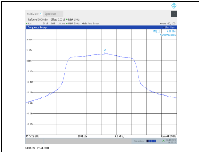
11n20MIMO-Ant22-5220-PASS
