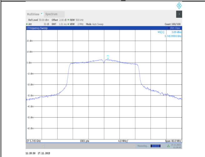
11n20MIMO-Ant22-5745-PASS
