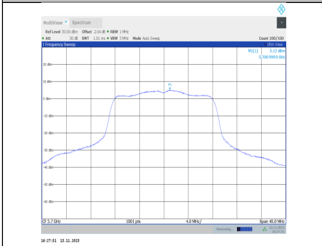
11a-CDD-Ant22-5700-PASS
