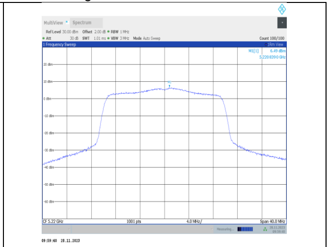
11ax20MIMO-Ant25-5220-PASS
