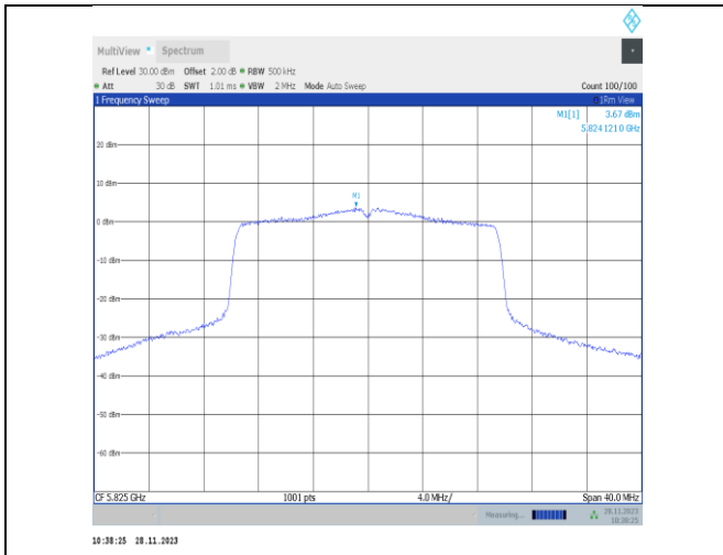
11ax20MIMO-Ant22-5825-PASS
