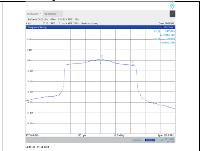
11ac80MIMO-Ant25-5690_UNII-2C-PASS
