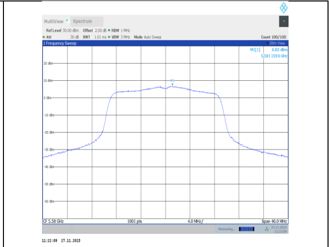
11n20MIMO-Ant25-5580-PASS
