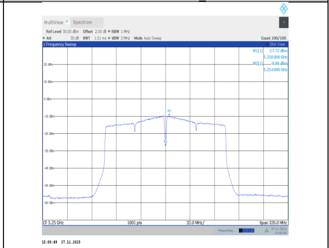
11ac160MIMO-Ant25-5250_UNII-2A-PASS
