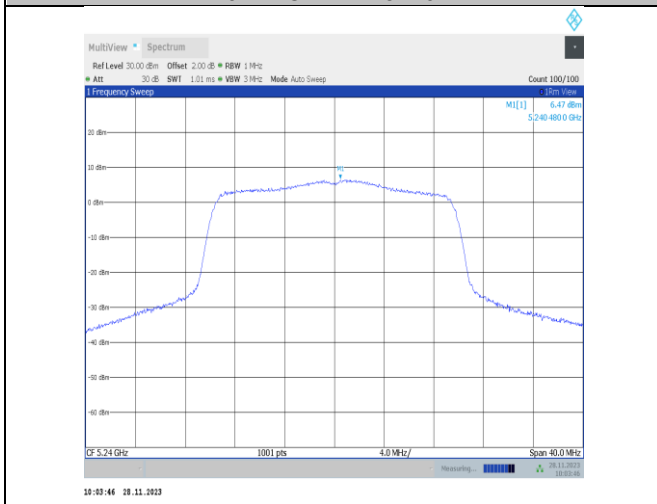
11ax20MIMO-Ant22-5240-PASS
