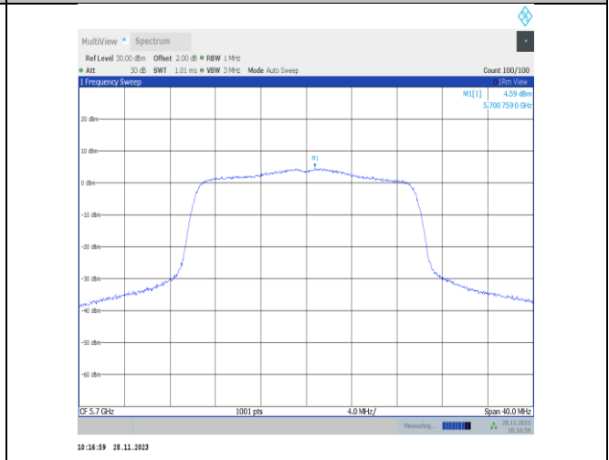
11ax20MIMO-Ant25-5700-PASS
