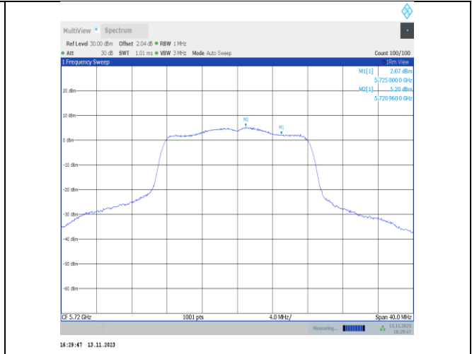
11a-CDD-Ant25-5720 UNII-2C-PASS
