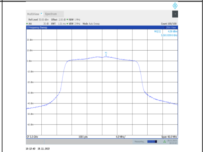
11ax20MIMO-Ant25-5500-PASS
