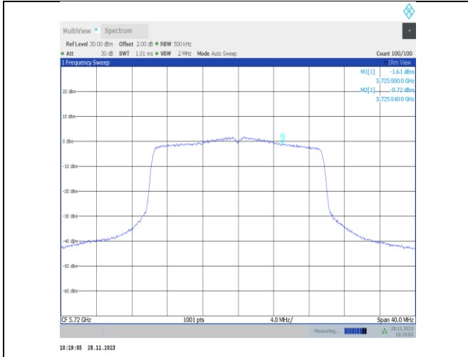
11ax20MIMO-Ant22-5720 UNII-3-PASS
