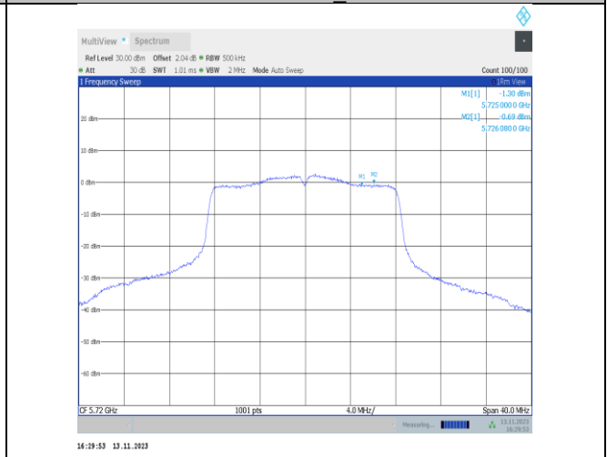
11a-CDD-Ant25-5720 UNII-3-PASS
