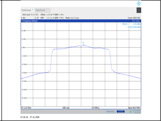
11ax40MIMO-Ant25-5230-PASS
