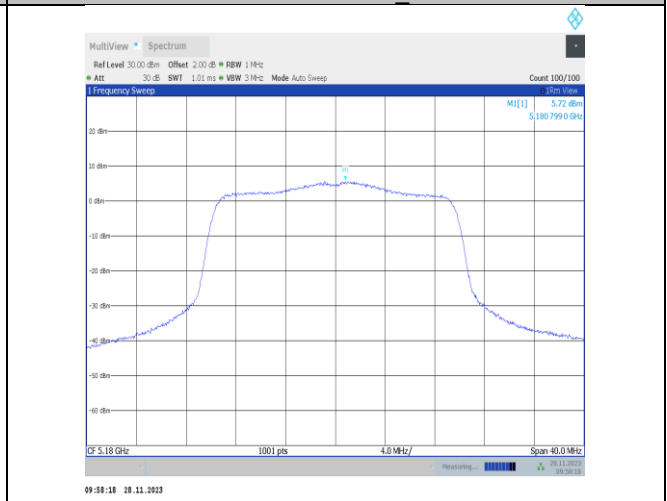
11ax20MIMO-Ant25-5180-PASS
