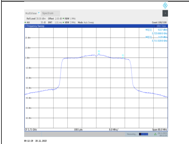
11ax40MIMO-Ant22-5710 UNII-2C-PASS
