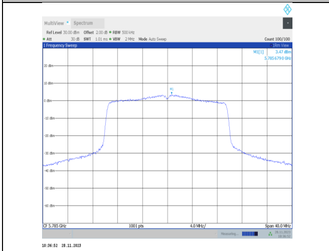
11ax20MIMO-Ant22-5785-PASS
