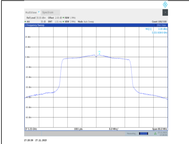
11ax40MIMO-Ant22-5550-PASS
