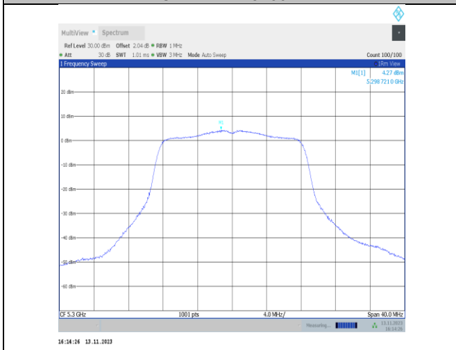
11a-CDD-Ant22-5300-PASS
