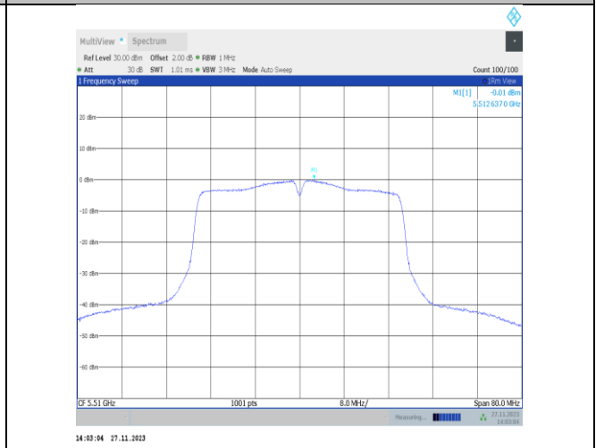
11n40MIMO-Ant25-5510-PASS
