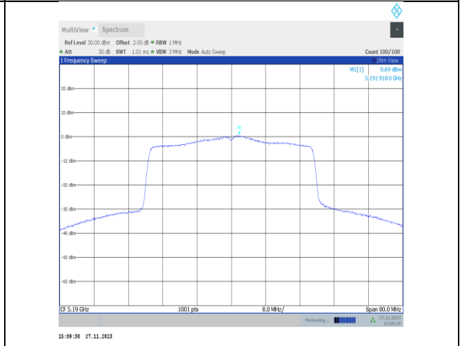
11ax40MIMO-Ant25-5190-PASS
