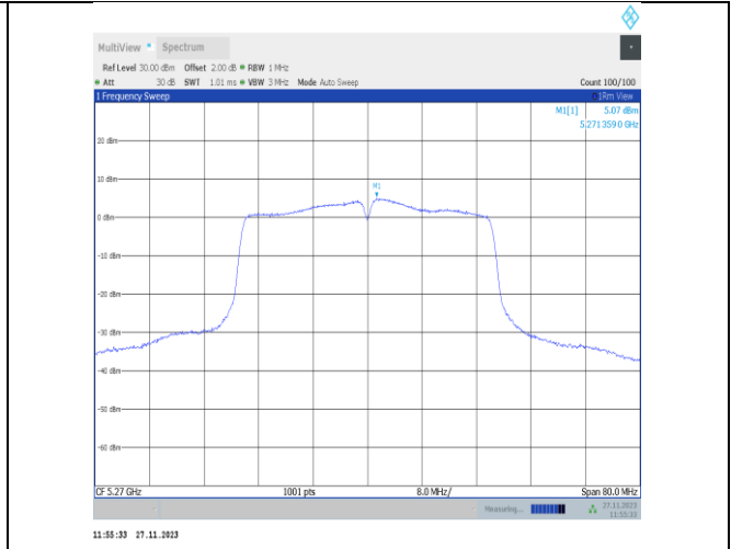
11n40MIMO-Ant25-5270-PASS
