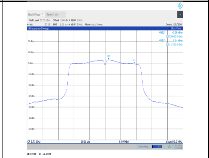
11n40MIMO-Ant25-5710 UNII-2C-PASS
