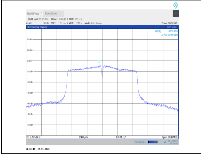
11n40MIMO-Ant22-5795-PASS
