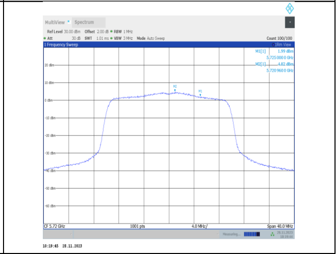
11ax20MIMO-Ant25-5720 UNII-2C-PASS
