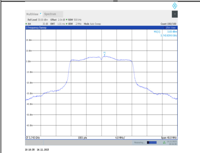
11a-CDD-Ant22-5745-PASS
