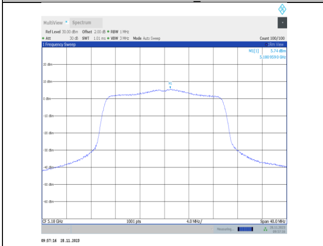
11ax20MIMO-Ant22-5180-PASS
