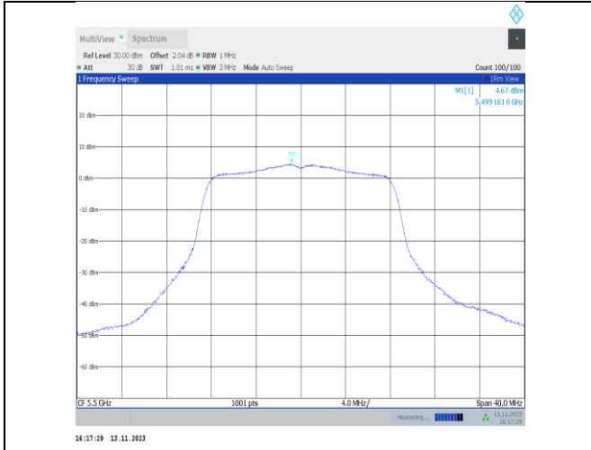
11a-CDD-Ant22-5500-PASS
