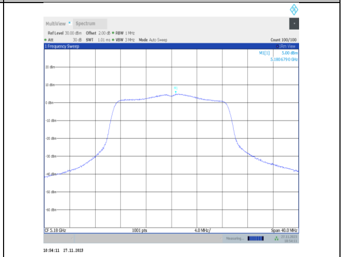
11n20MIMO-Ant25-5180-PASS
