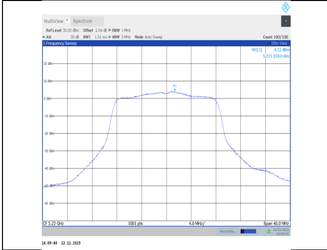
11a-CDD-Ant22-5220-PASS
