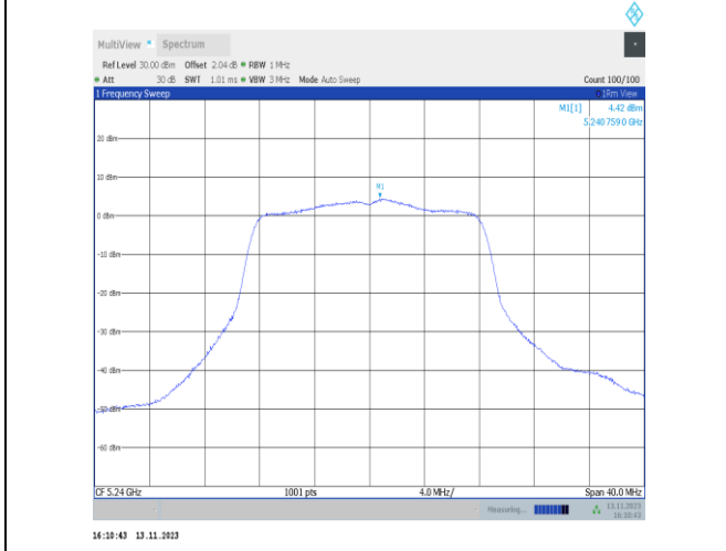
11a-CDD-Ant22-5240-PASS
