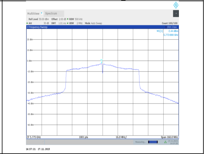
11ac80MIMO-Ant25-5775-PASS
