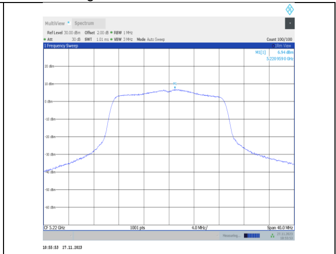
11n20MIMO-Ant25-5220-PASS
