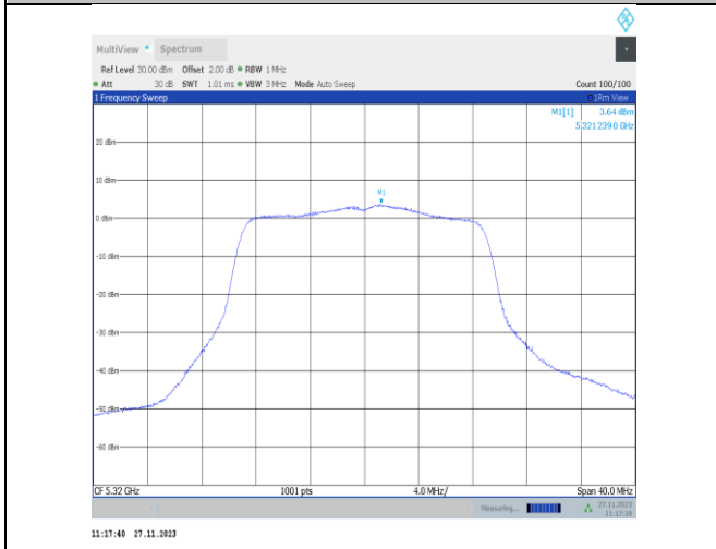
11n20MIMO-Ant22-5320-PASS
