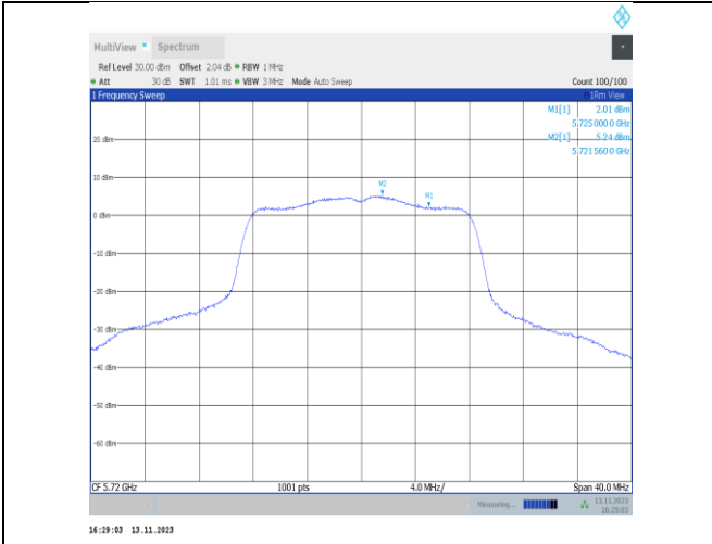
11a-CDD-Ant22-5720 UNII-2C-PASS
