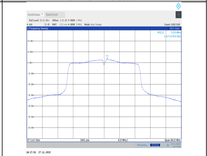
11n40MIMO-Ant25-5670-PASS
