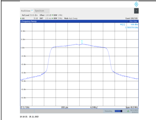
11ax20MIMO-Ant22-5700-PASS
