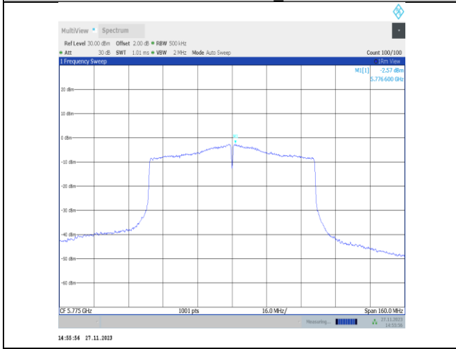
11ac80MIMO-Ant22-5775-PASS
