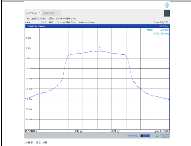
11a-CDD-Ant22-5580-PASS
