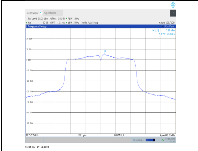
11n40MIMO-Ant22-5270-PASS
