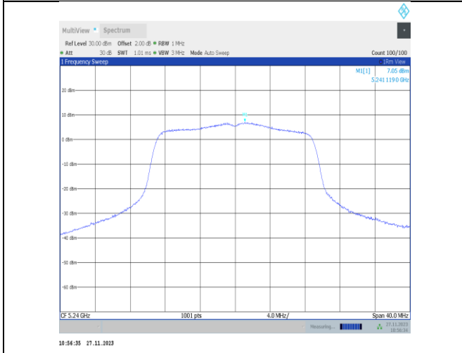
11n20MIMO-Ant22-5240-PASS
