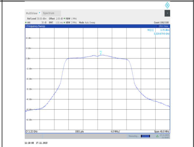
11n20MIMO-Ant25-5320-PASS
