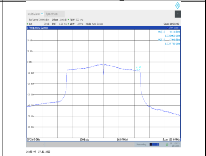
11ac80MIMO-Ant25-5690_UNII-3-PASS
