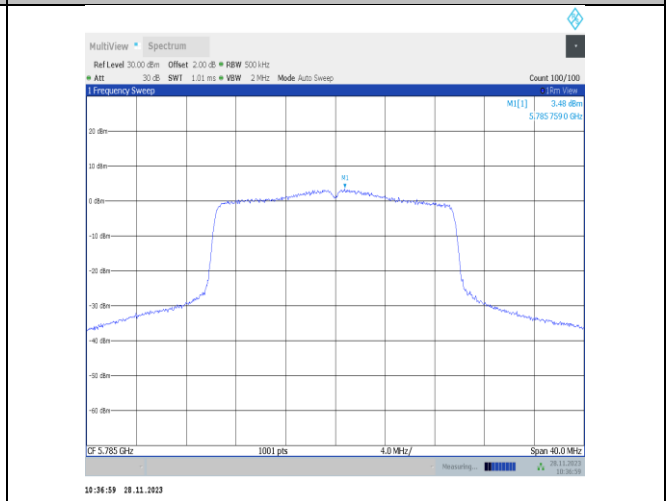
11ax20MIMO-Ant25-5785-PASS
