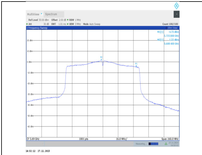
11ac80MIMO-Ant22-5690_UNII-2C-PASS
