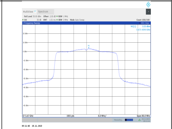
11ax40MIMO-Ant25-5670-PASS
