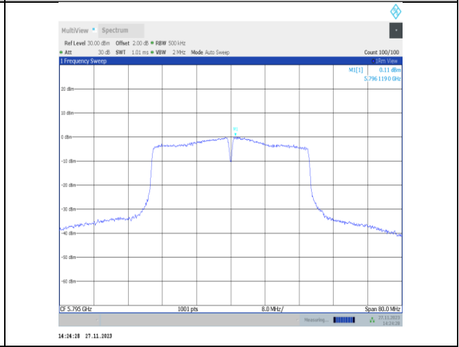
11n40MIMO-Ant25-5795-PASS
