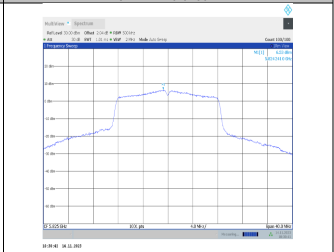
11a-CDD-Ant25-5825-PASS
