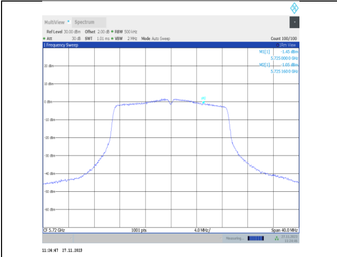
11n20MIMO-Ant22-5720 UNII-3-PASS
