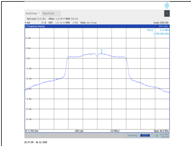
11a-CDD-Ant22-5785-PASS
