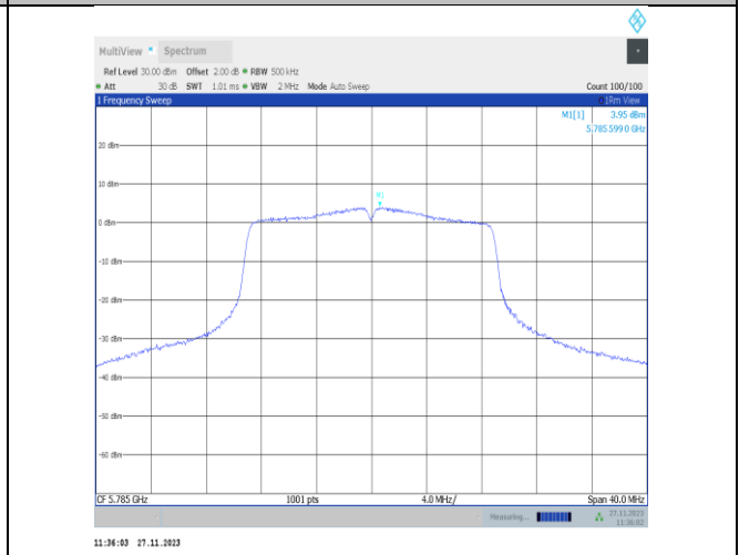
11n20MIMO-Ant25-5785-PASS
