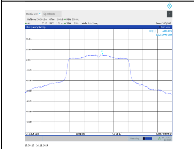
11a-CDD-Ant22-5825-PASS
