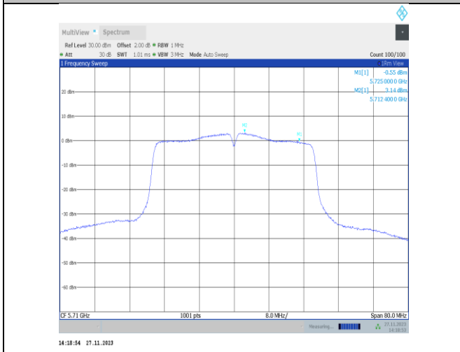
11n40MIMO-Ant22-5710 UNII-2C-PASS
