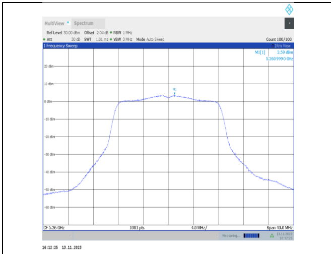
11a-CDD-Ant22-5260-PASS
