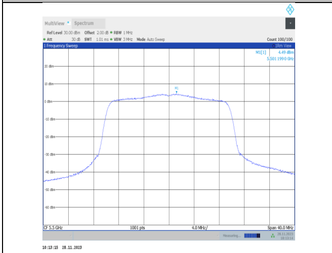
11ax20MIMO-Ant22-5500-PASS
