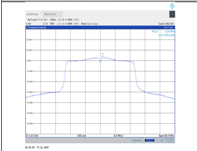
11n40MIMO-Ant22-5670-PASS
