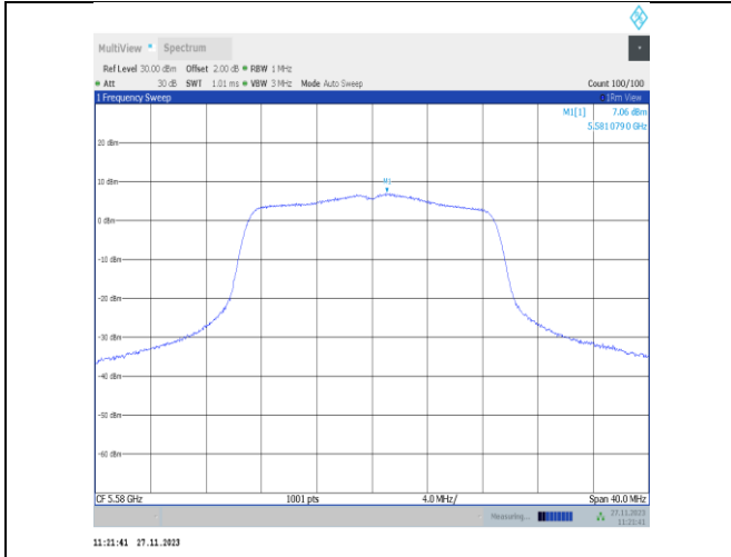
11n20MIMO-Ant22-5580-PASS
