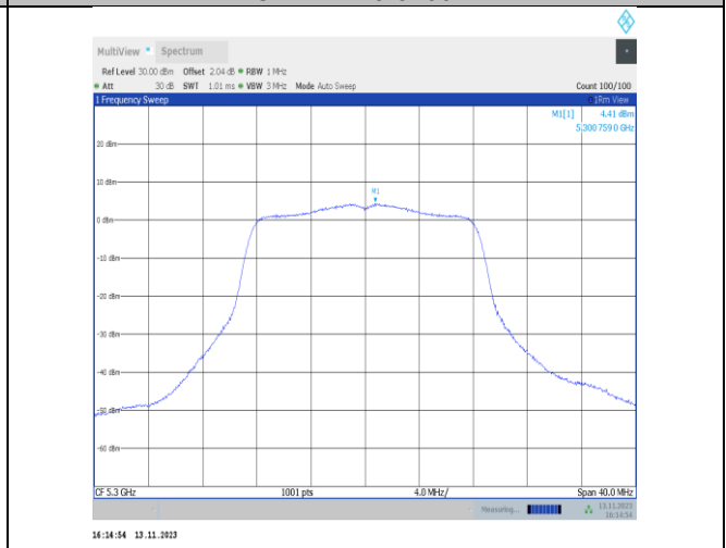
11a-CDD-Ant25-5300-PASS
