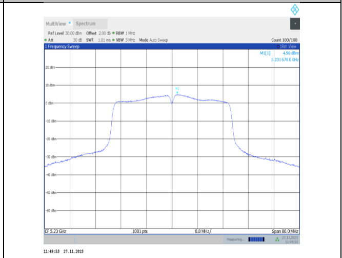
11n40MIMO-Ant25-5230-PASS
