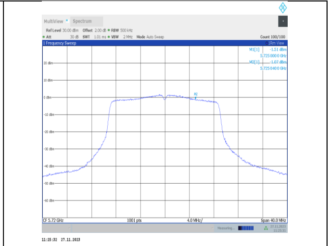
11n20MIMO-Ant25-5720 UNII-3-PASS
