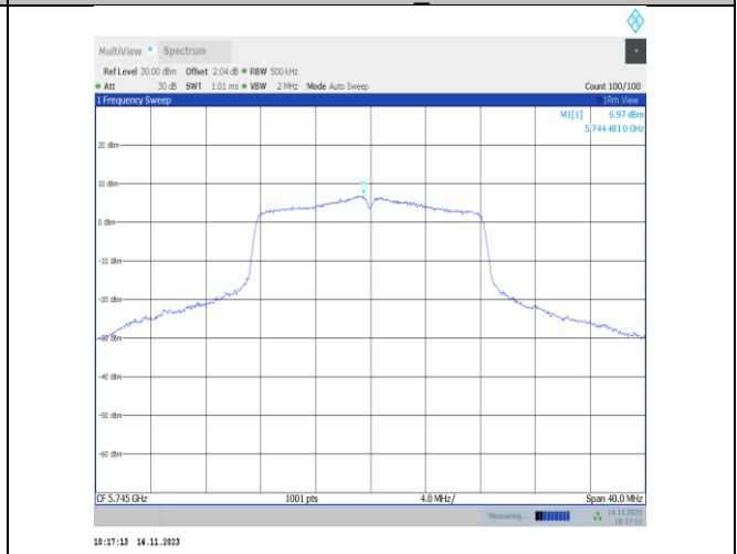
11a-CDD-Ant25-5745-PASS
