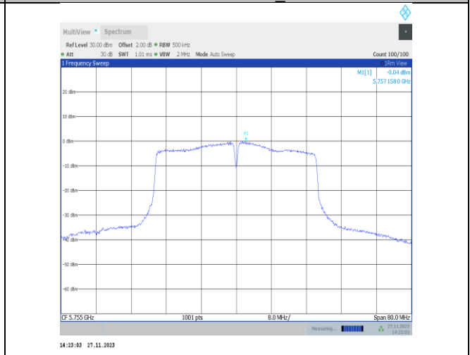
11n40MIMO-Ant25-5755-PASS
