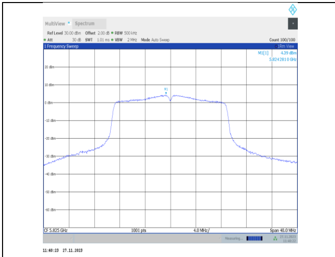
11n20MIMO-Ant22-5825-PASS
