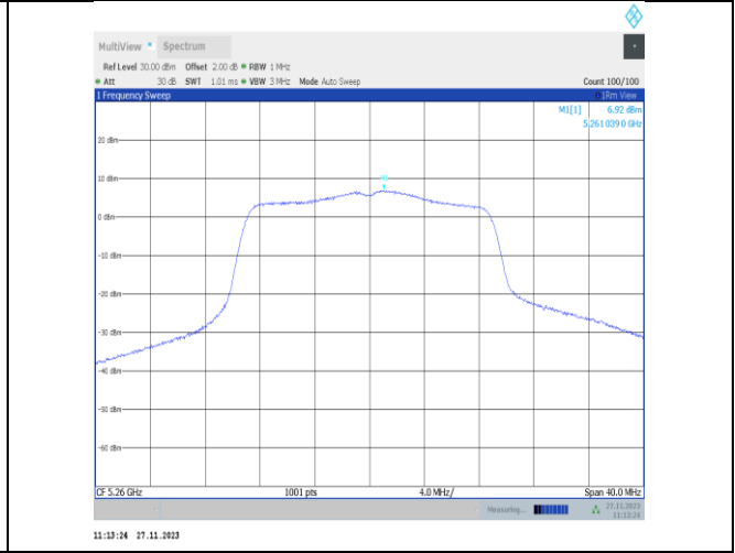
11n20MIMO-Ant25-5260-PASS
