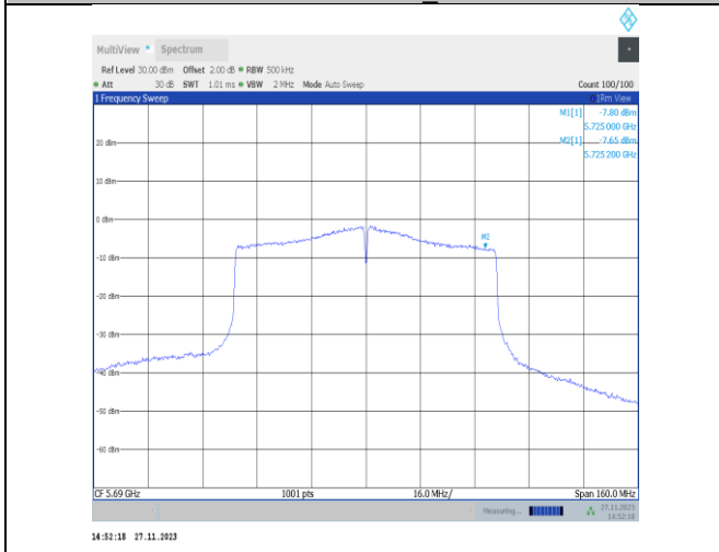
11ac80MIMO-Ant22-5690_UNII-3-PASS
