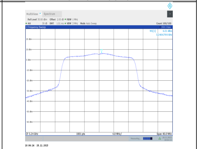
11ax20MIMO-Ant25-5240-PASS
