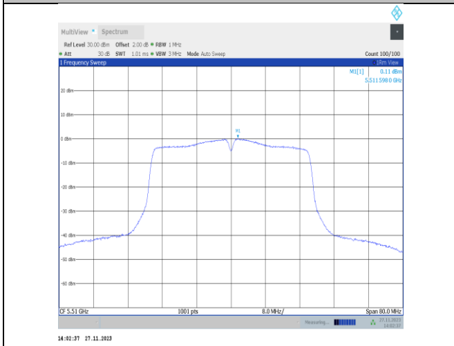
11n40MIMO-Ant22-5510-PASS
