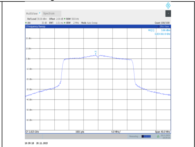
11ax20MIMO-Ant25-5825-PASS
