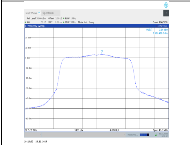
11ax20MIMO-Ant22-5320-PASS
