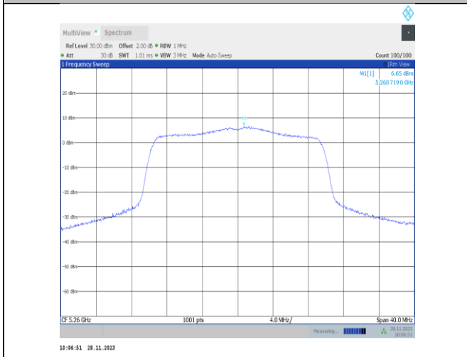
11ax20MIMO-Ant22-5260-PASS
