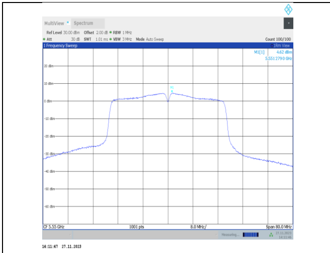
11n40MIMO-Ant22-5550-PASS
