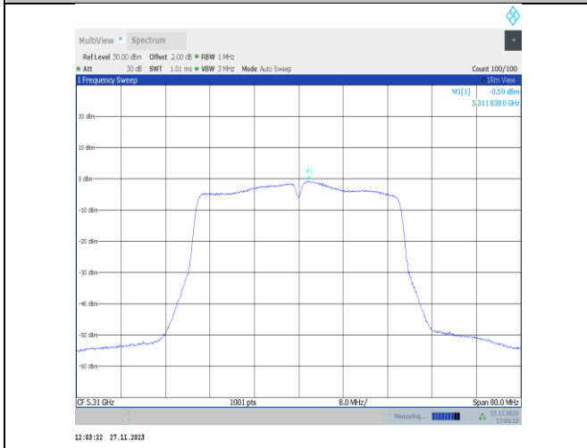
11n40MIMO-Ant22-5310-PASS
