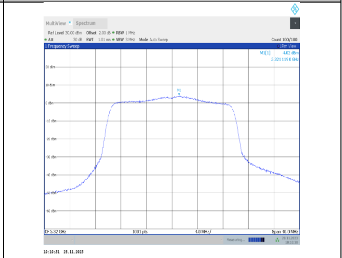
11ax20MIMO-Ant25-5320-PASS
