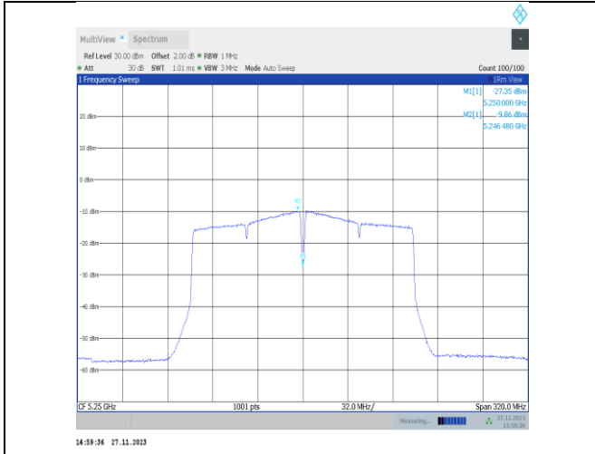
11ac160MIMO-Ant22-5250_UNII-1-PASS
