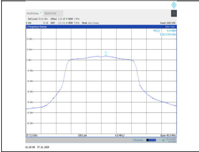
11n20MIMO-Ant22-5500-PASS
