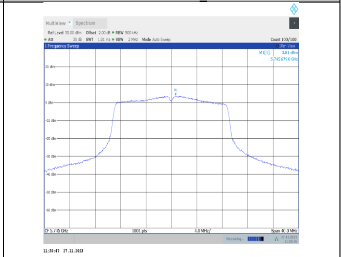
11n20MIMO-Ant25-5745-PASS
