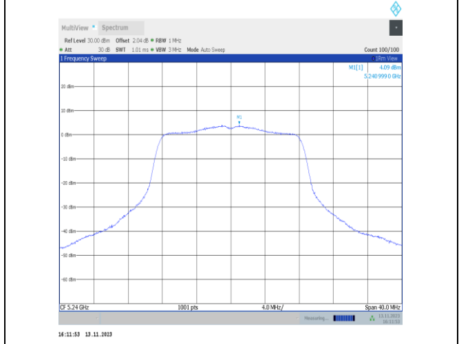
11a-CDD-Ant25-5240-PASS
