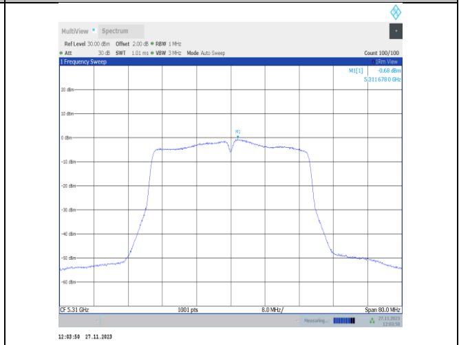
11n40MIMO-Ant25-5310-PASS
