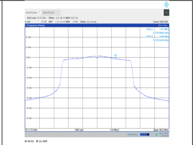
11ax20MIMO-Ant25-5720 UNII-3-PASS
