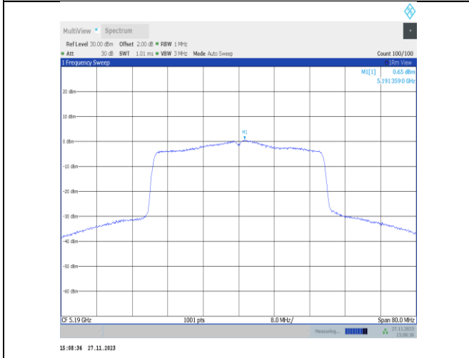
11ax40MIMO-Ant22-5190-PASS
