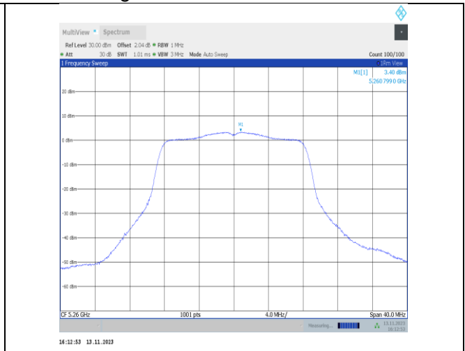
11a-CDD-Ant25-5260-PASS
