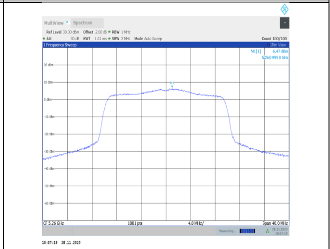
11ax20MIMO-Ant25-5260-PASS
