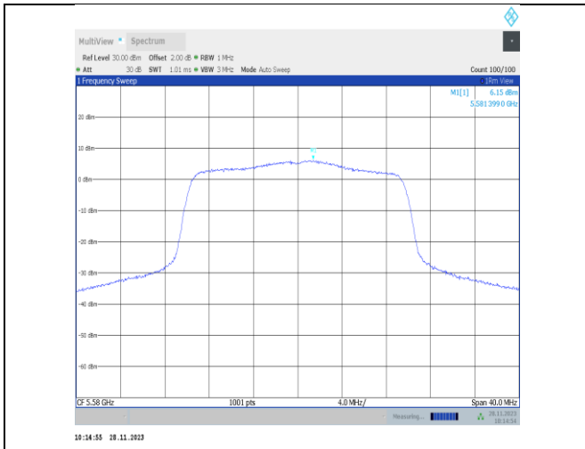
11ax20MIMO-Ant22-5580-PASS
