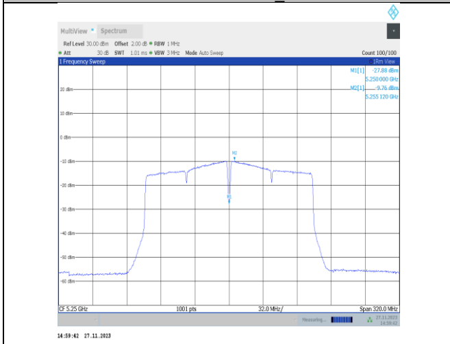
11ac160MIMO-Ant22-5250_UNII-2A-PASS
