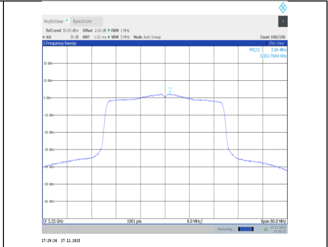
11ax40MIMO-Ant25-5550-PASS
