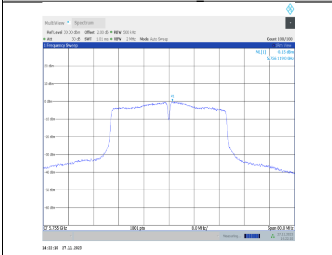
11n40MIMO-Ant22-5755-PASS
