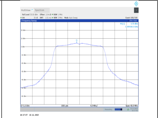
11a-CDD-Ant25-5500-PASS
