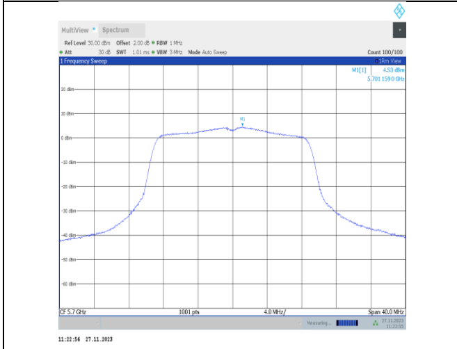
11n20MIMO-Ant22-5700-PASS
