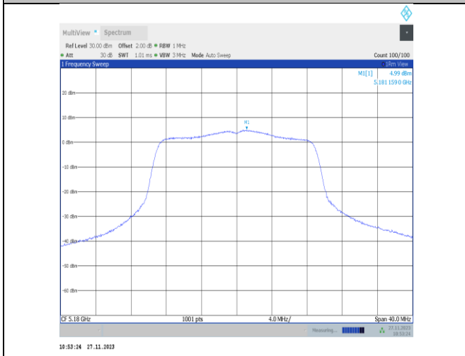
11n20MIMO-Ant22-5180-PASS
