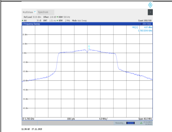
11n20MIMO-Ant22-5785-PASS
