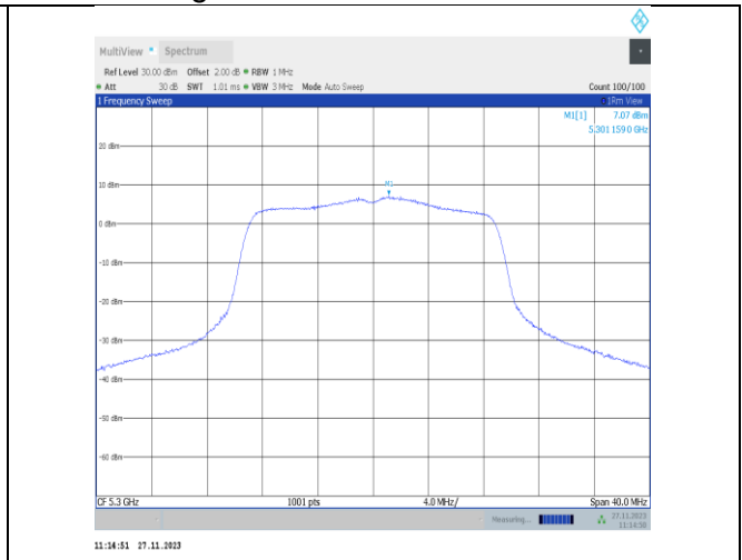
11n20MIMO-Ant25-5300-PASS
