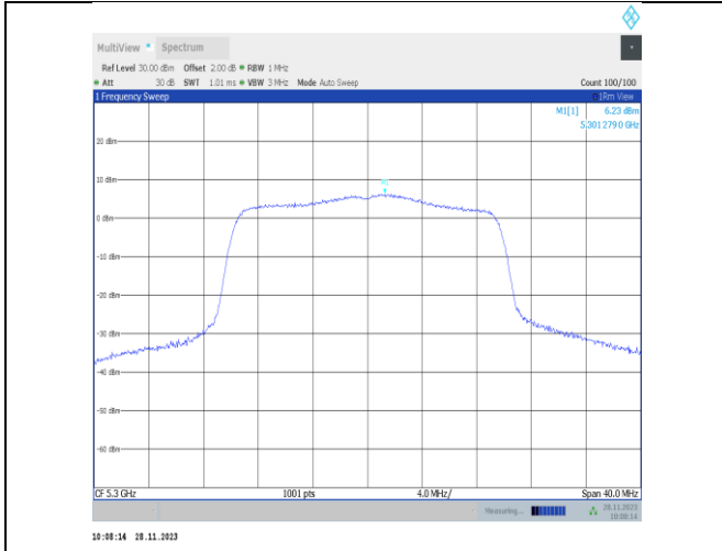
11ax20MIMO-Ant22-5300-PASS
