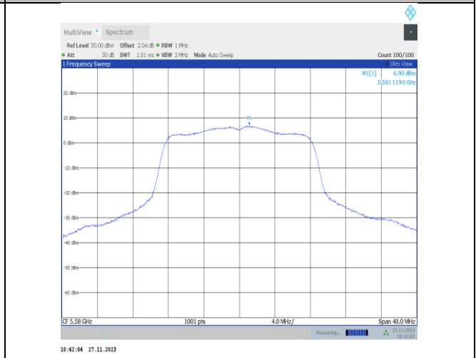
11a-CDD-Ant25-5580-PASS
