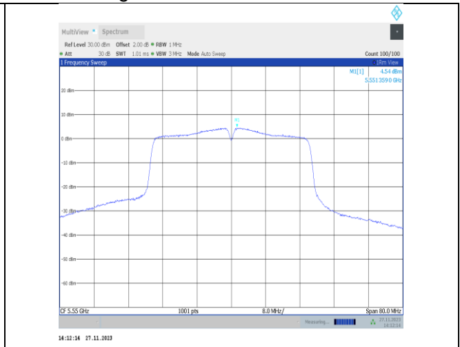
11n40MIMO-Ant25-5550-PASS
