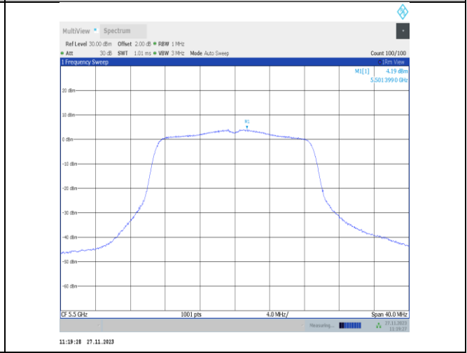
11n20MIMO-Ant25-5500-PASS
