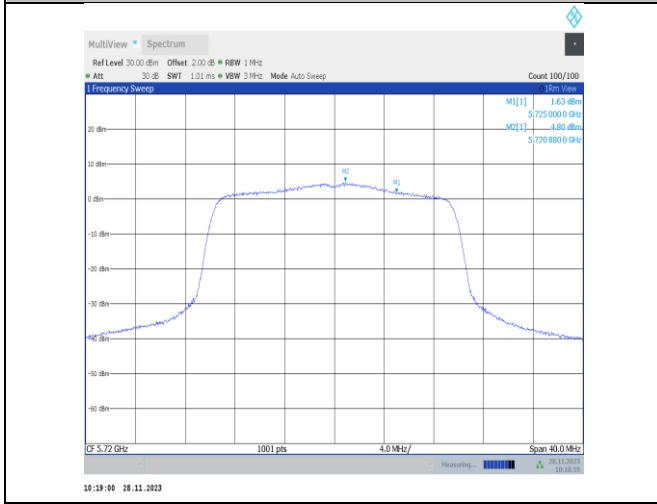
11ax20MIMO-Ant22-5720 UNII-2C-PASS
