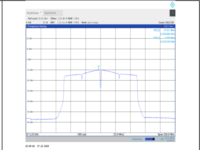
11ac160MIMO-Ant25-5250_UNII-1-PASS
