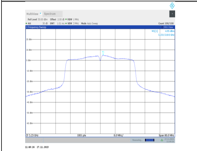
11n40MIMO-Ant22-5230-PASS
