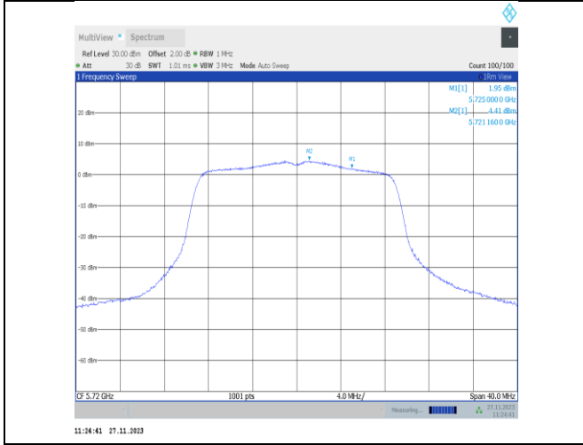
11n20MIMO-Ant22-5720 UNII-2C-PASS
