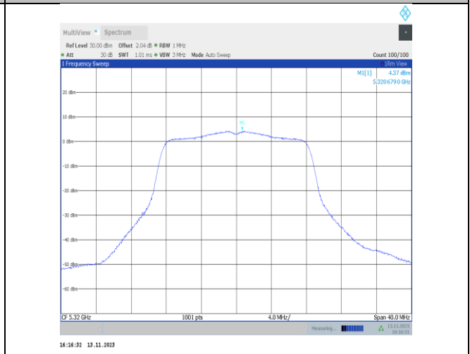
11a-CDD-Ant25-5320-PASS
