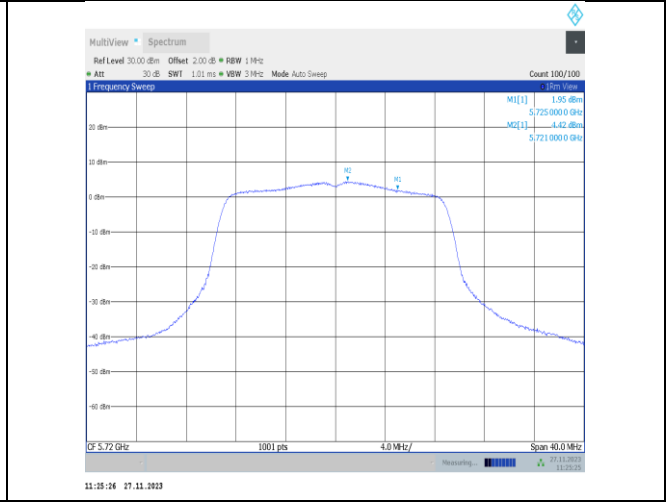
11n20MIMO-Ant25-5720 UNII-2C-PASS
