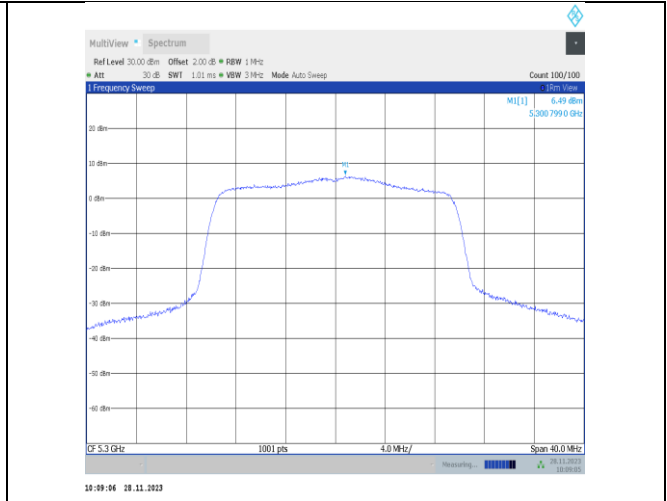
11ax20MIMO-Ant25-5300-PASS
