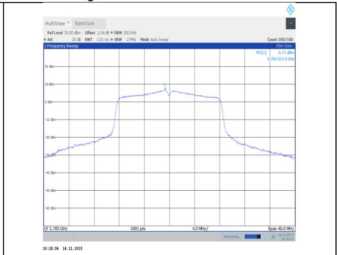
11a-CDD-Ant25-5785-PASS
