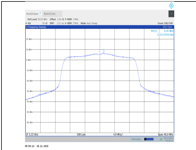
11ax20MIMO-Ant22-5220-PASS
