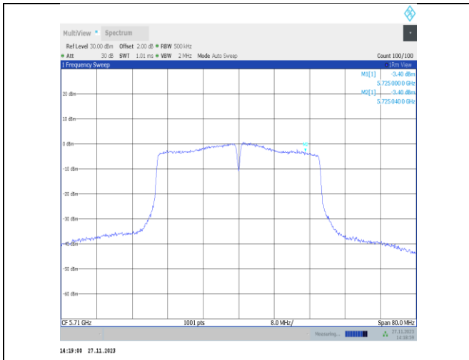
11n40MIMO-Ant22-5710 UNII-3-PASS
