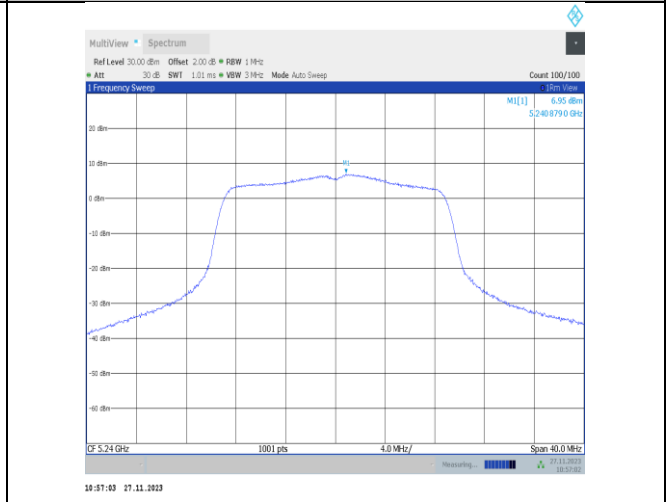
11n20MIMO-Ant25-5240-PASS
