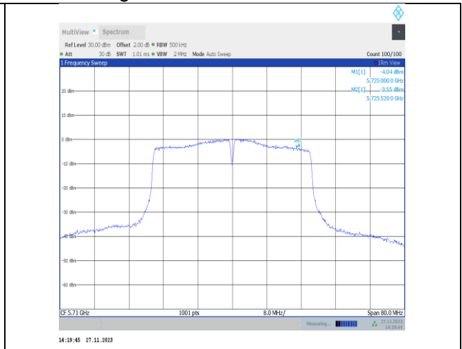
11n40MIMO-Ant25-5710 UNII-3-PASS
