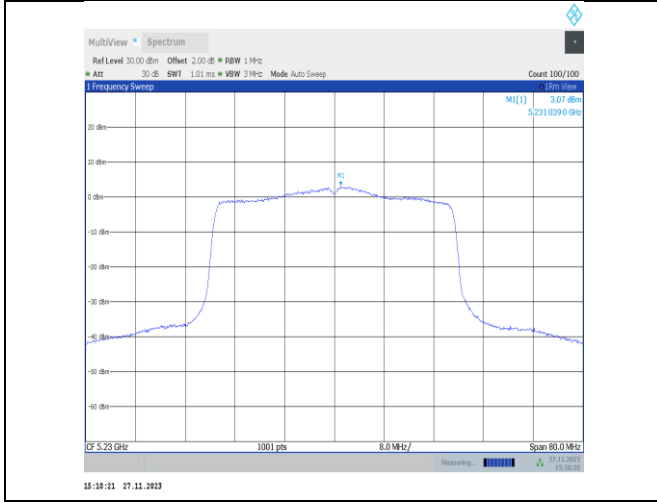
11ax40MIMO-Ant22-5230-PASS
