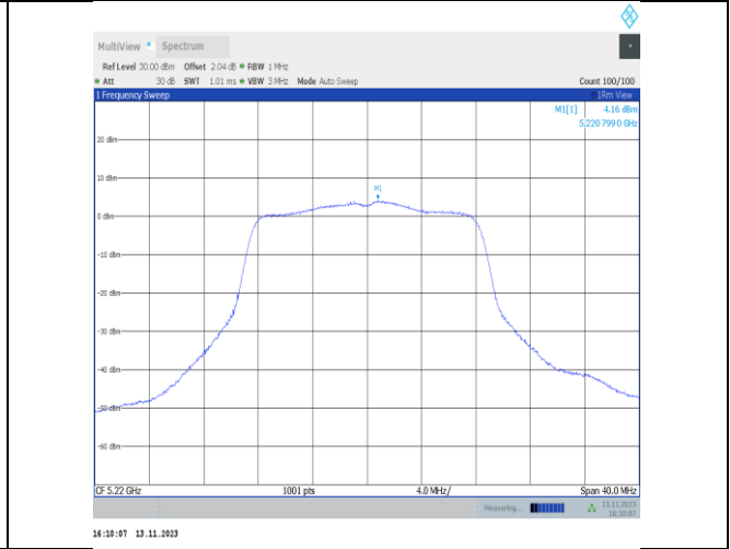
11a-CDD-Ant25-5220-PASS
