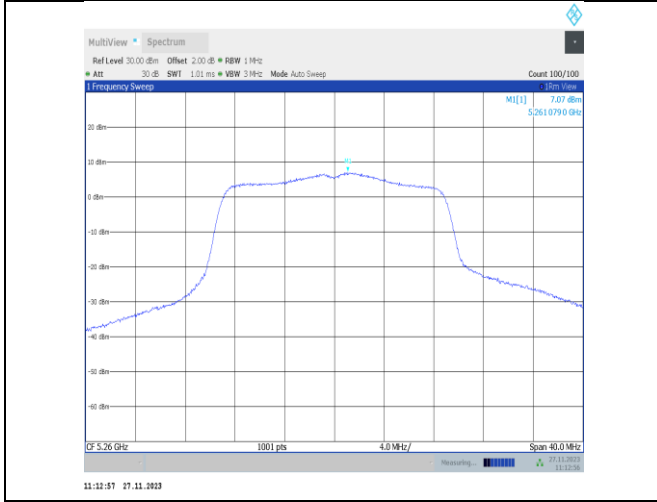
11n20MIMO-Ant22-5260-PASS
