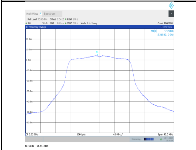
11a-CDD-Ant22-5320-PASS
