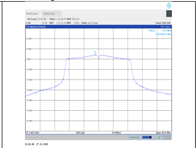
11n20MIMO-Ant25-5825-PASS
