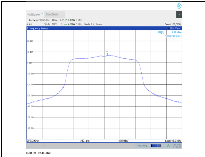
11n20MIMO-Ant22-5300-PASS
