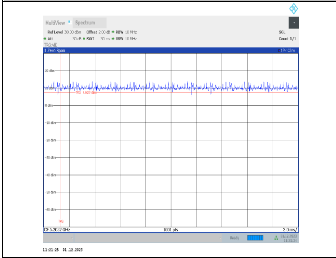
NTVN-11ax80MIMO-Ant22-5210-484Tone-RU65
