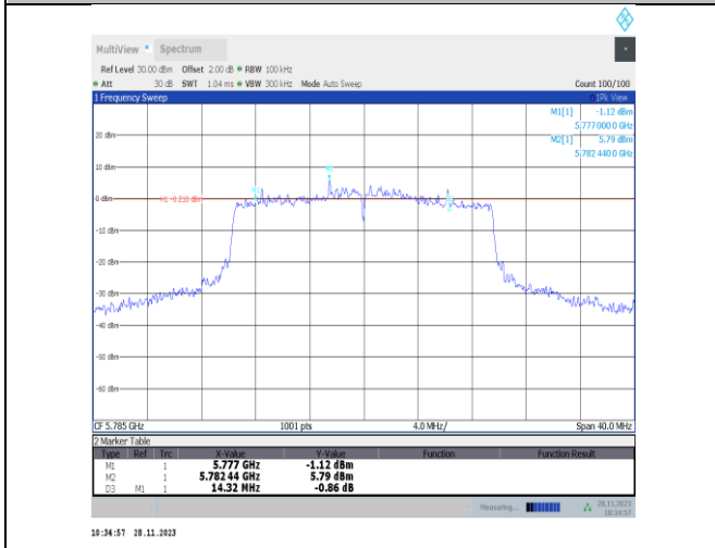
11ax20MIMO-Ant22-5785-PASS
