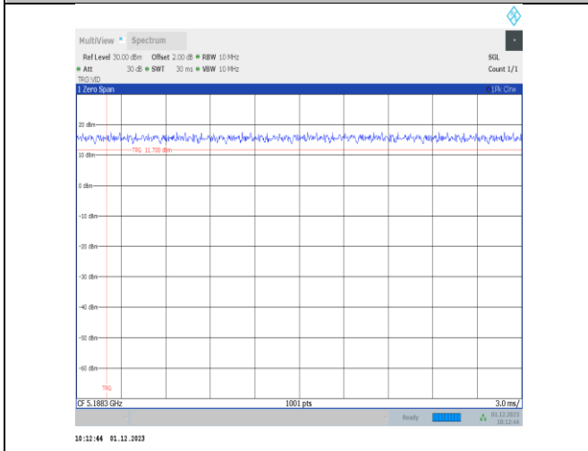
NTVN-11ax40MIMO-Ant22-5190-242Tone-RU61
