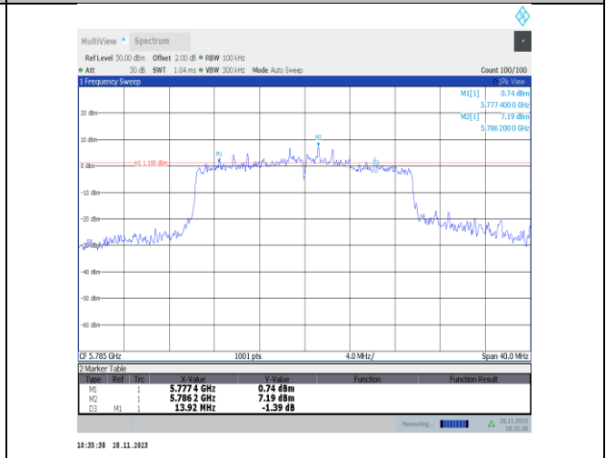
11ax20MIMO-Ant25-5785-PASS
