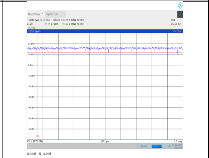
NTVN-11ax40MIMO-Ant25-5190-242Tone-RU61
