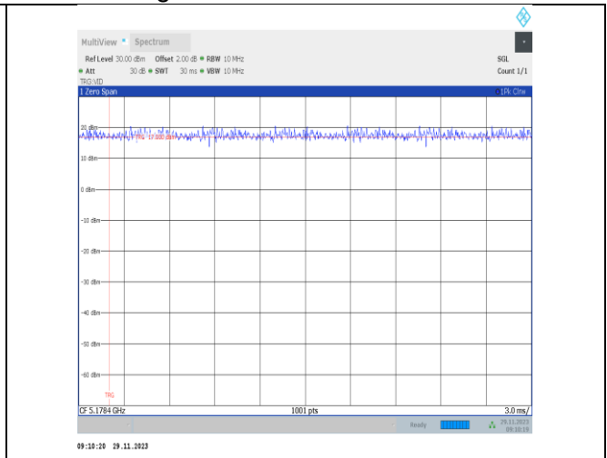
NTVN-11ax20MIMO-Ant25-5180-106Tone-RU53
