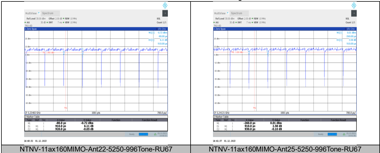
NTNV-11ax160MIMO-Ant22-5250-996Tone-RU67
