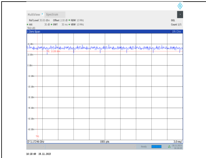
NTVN-11ax20MIMO-Ant25-5180-52Tone-RU37
