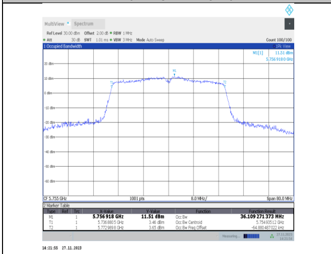
11n40MIMO-Ant22-5755
