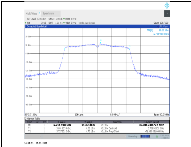
11n40MIMO-Ant22-5710
