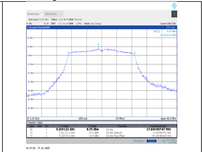
11n20MIMO-Ant25-5320
