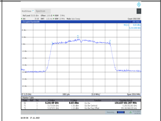
11ac160MIMO-Ant25-5250
