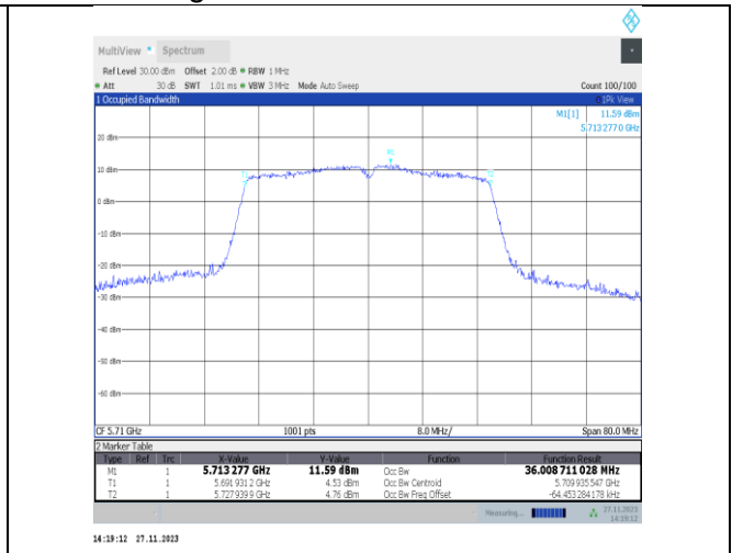
11n40MIMO-Ant25-5710
