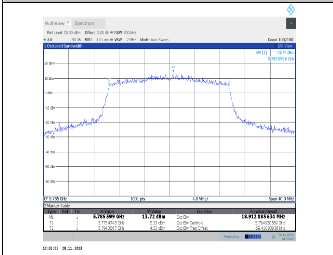
11ax20MIMO-Ant22-5785
