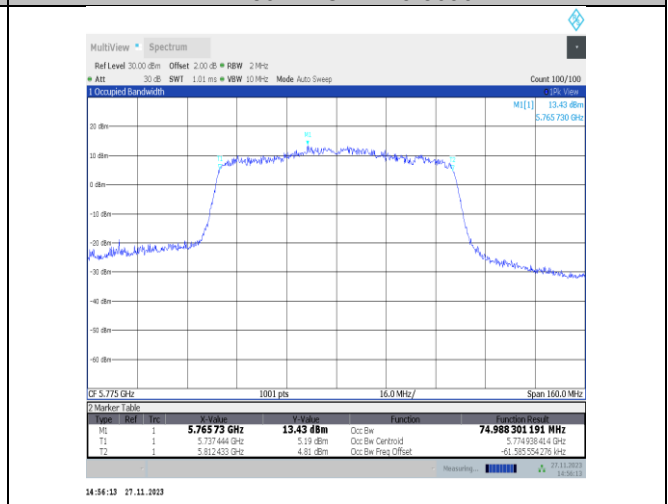
11ac80MIMO-Ant25-5775
