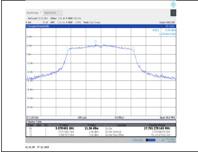
11n20MIMO-Ant22-5580
