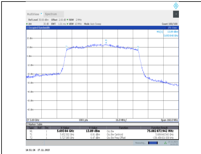
11ac80MIMO-Ant22-5690
