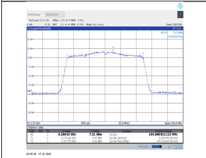
11ac160MIMO-Ant22-5250
