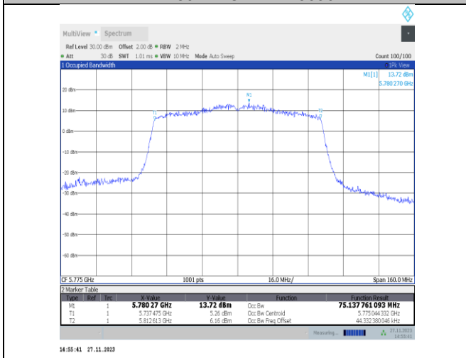
11ac80MIMO-Ant22-5775
