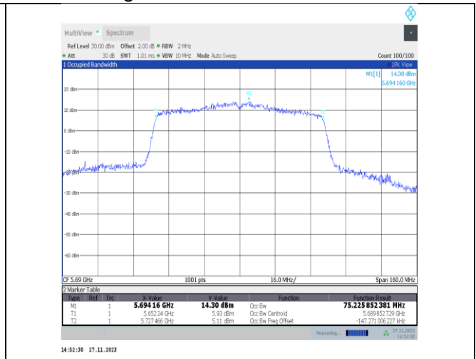
11ac80MIMO-Ant25-5690
