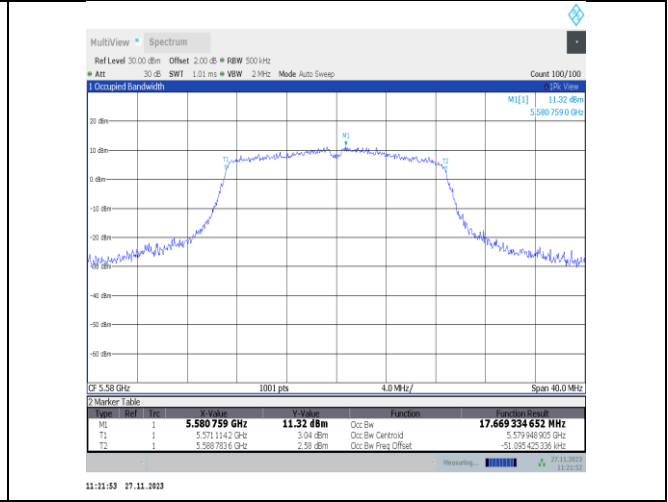
11n20MIMO-Ant25-5580
