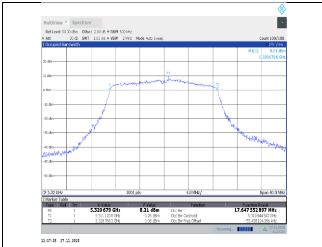
11n20MIMO-Ant22-5320
