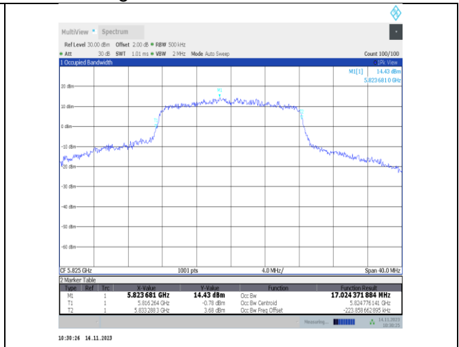
11a-CDD-Ant25-5825
