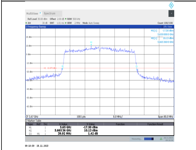
11ax40MIMO-Ant22-5670
