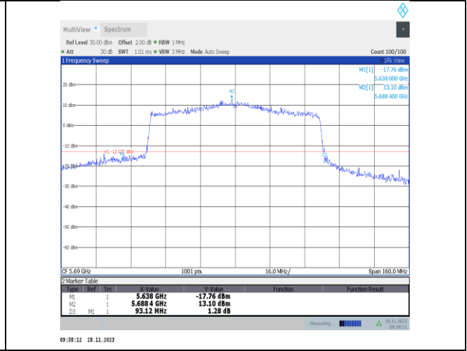
11ax80MIMO-Ant25-5690
