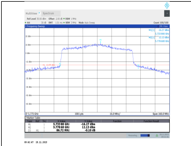
11ax80MIMO-Ant22-5775
