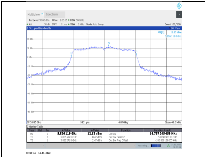
11a-CDD-Ant22-5825
