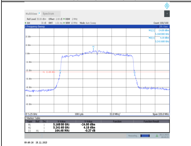
11ax160MIMO-Ant22-5250
