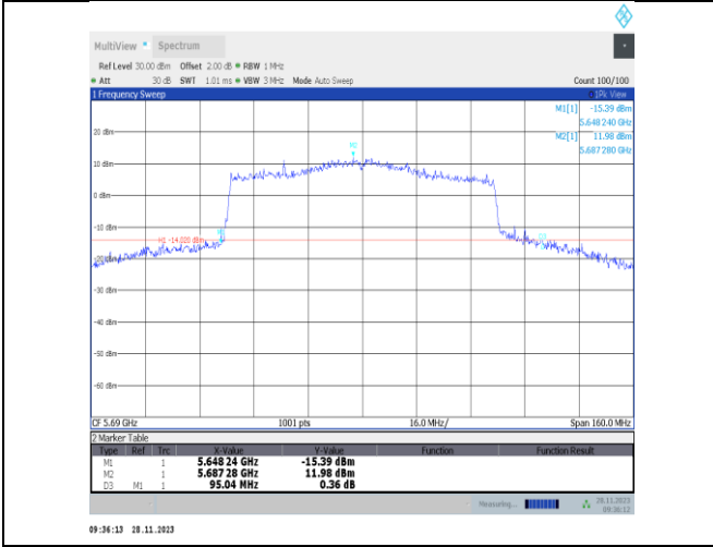
11ax80MIMO-Ant22-5690
