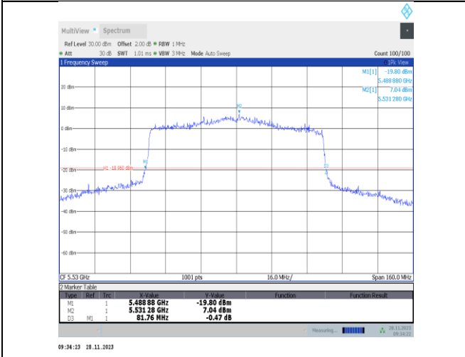
11ax80MIMO-Ant22-5530
