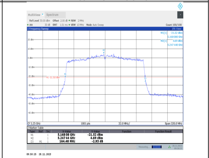
11ax160MIMO-Ant25-5250
