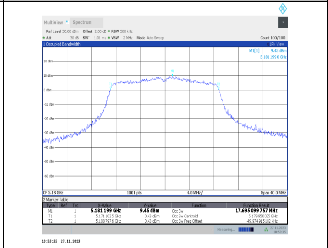
11n20MIMO-Ant25-5180
