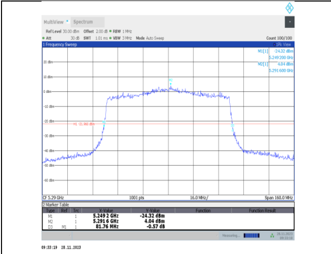
11ax80MIMO-Ant22-5290
