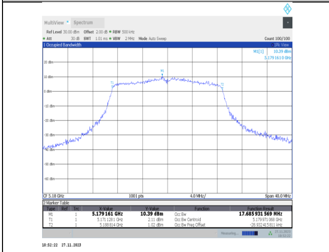
11n20MIMO-Ant22-5180
