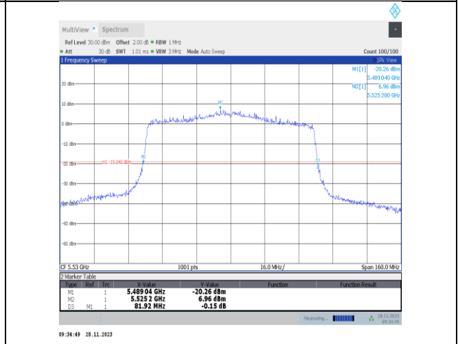
11ax80MIMO-Ant25-5530
