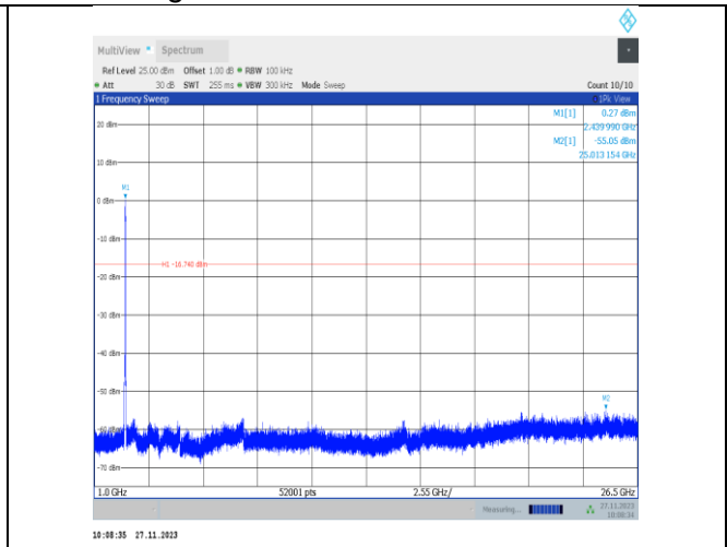
11ax40MIMO-Ant25-2437-1000~26500-PASS
