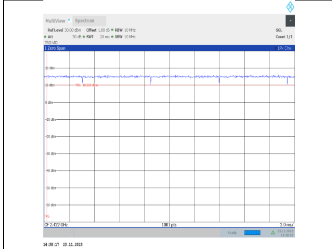
NTNV-11n40MIMO-Ant22-2422
