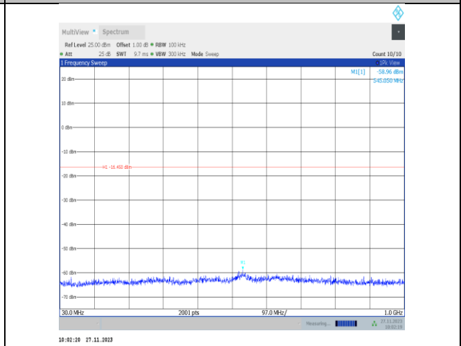
11ax40MIMO-Ant22-2427-30~1000-PASS
