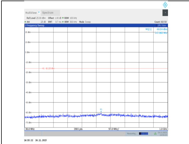
11VHT40MIMO-Ant25-2437-30~1000-PASS
