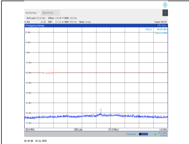
11VHT40MIMO-Ant25-2422-30~1000-PASS
