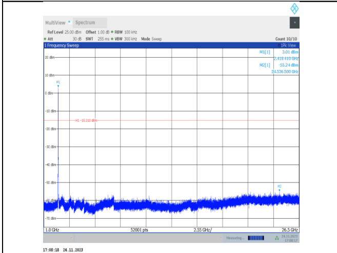
11ax20MIMO-Ant22-2417-1000~26500-PASS
