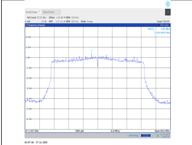
11ax40MIMO-Ant22-2437-0~Reference-PASS
