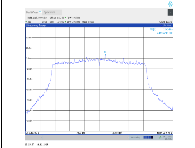
11ax20MIMO-Ant22-2412-0~Reference-PASS
