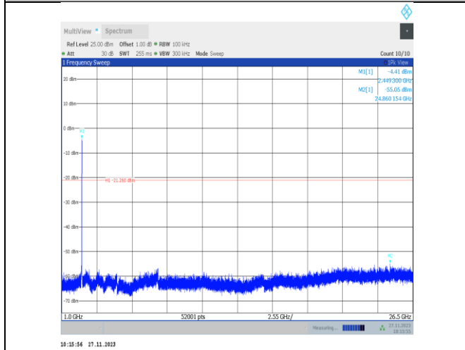
11ax40MIMO-Ant22-2452-1000~26500-PASS
