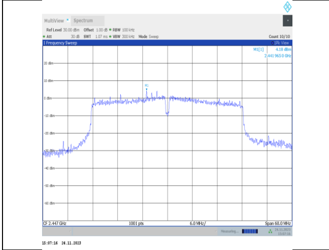
11VHT40MIMO-Ant22-2447-0~Reference-PASS
