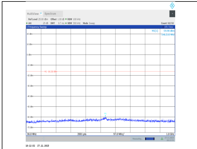
11ax40MIMO-Ant25-2447-30~1000-PASS
