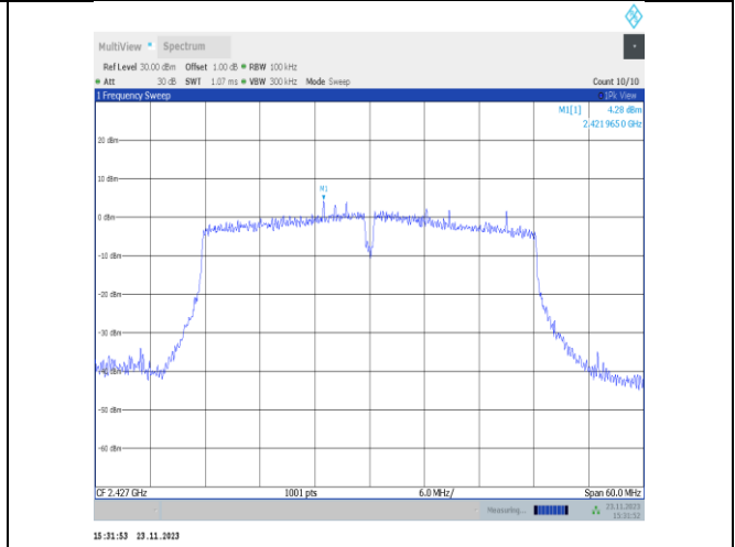
11VHT40MIMO-Ant25-2427-0~Reference-PASS
