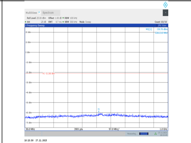
11ax40MIMO-Ant22-2452-30~1000-PASS
