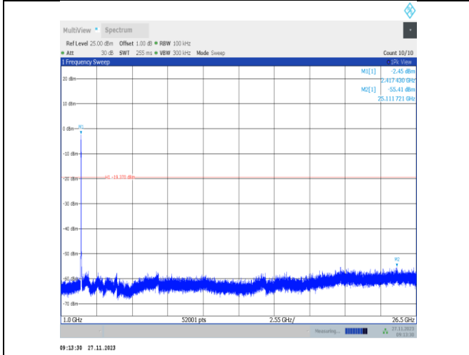
11ax40MIMO-Ant22-2422-1000~26500-PASS
