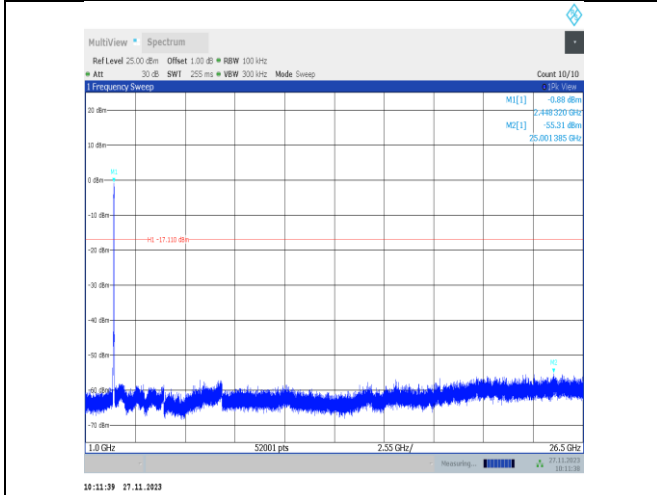
11ax40MIMO-Ant22-2447-1000~26500-PASS
