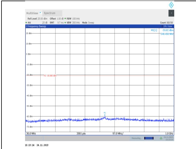
11VHT40MIMO-Ant25-2452-30~1000-PASS
