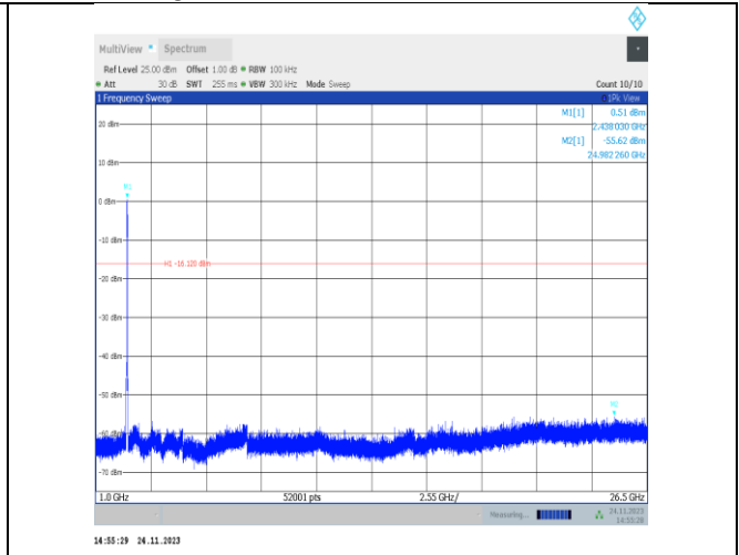
11VHT40MIMO-Ant25-2437-1000~26500-PASS
