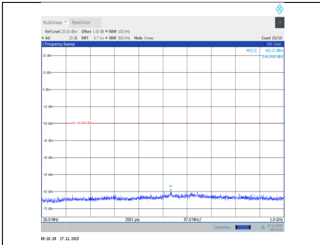
11ax40MIMO-Ant25-2422-30~1000-PASS
