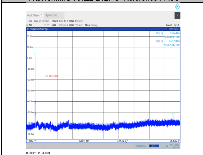
11ax40MIMO-Ant22-2427-1000~26500-PASS
