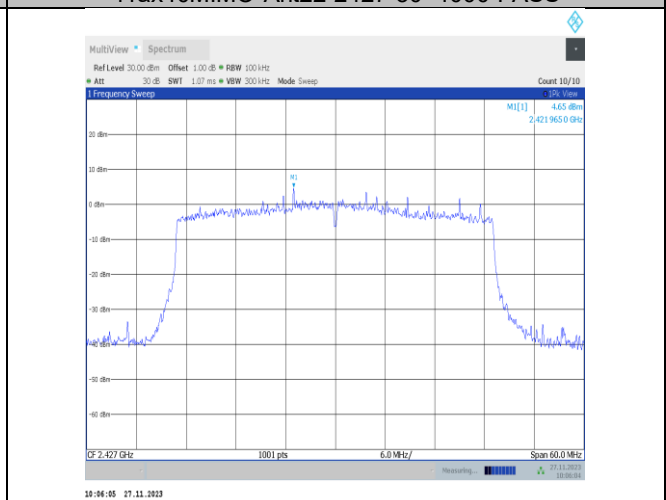
11ax40MIMO-Ant25-2427-0~Reference-PASS
