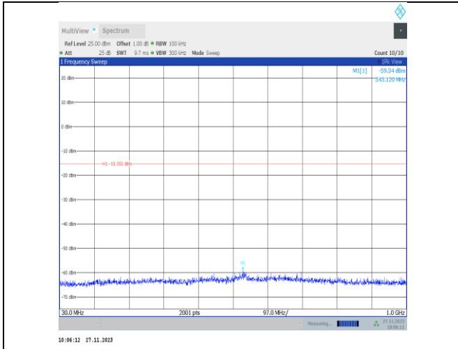
11ax40MIMO-Ant25-2427-30~1000-PASS
