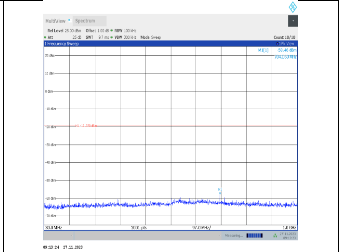
11ax40MIMO-Ant22-2422-30~1000-PASS
