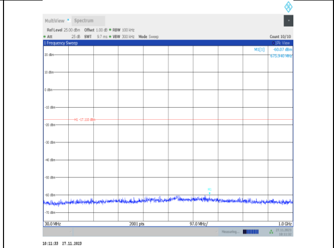
11ax40MIMO-Ant22-2447-30~1000-PASS
