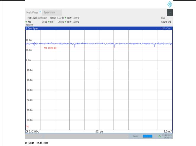
NTVN-11ax40MIMO-Ant25-2422
