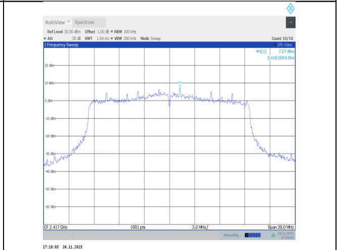
11ax20MIMO-Ant25-2417-0~Reference-PASS
