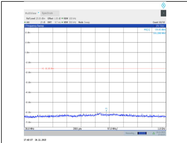
11ax20MIMO-Ant25-2462-30~1000-PASS
