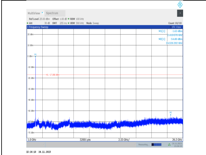
11ax20MIMO-Ant22-2412-1000~26500-PASS
