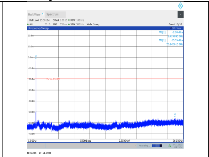
11ax40MIMO-Ant25-2422-1000~26500-PASS
