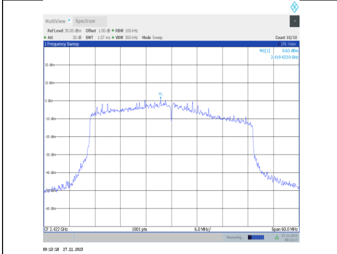
11ax40MIMO-Ant22-2422-0~Reference-PASS
