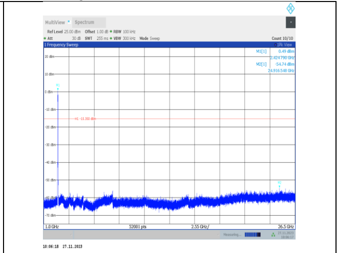
11ax40MIMO-Ant25-2427-1000~26500-PASS
