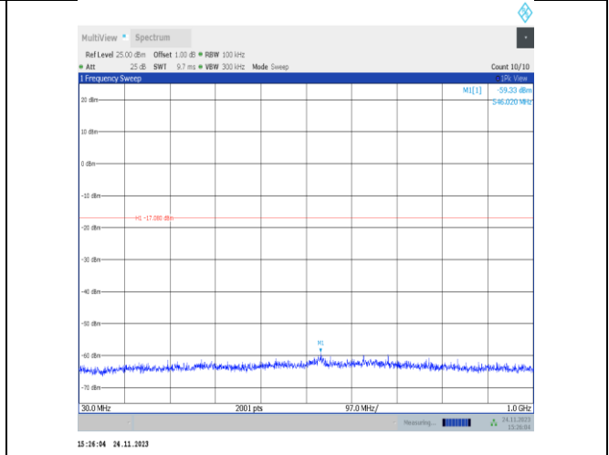
11ax20MIMO-Ant22-2412-30~1000-PASS
