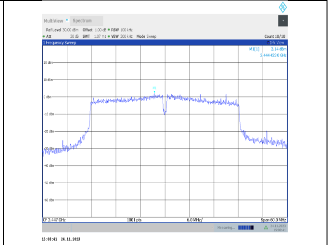
11VHT40MIMO-Ant25-2447-0~Reference-PASS
