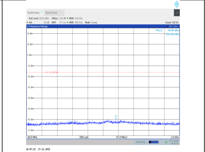
11ax40MIMO-Ant22-2437-30~1000-PASS
