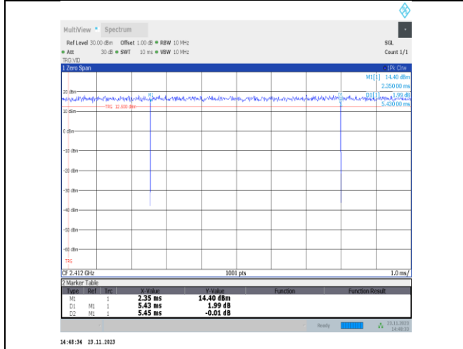
NTNV-11VHT20MIMO-Ant22-2412
