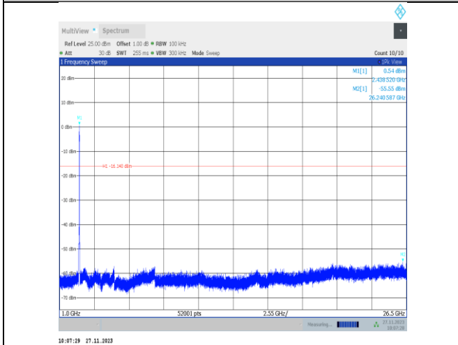
11ax40MIMO-Ant22-2437-1000~26500-PASS
