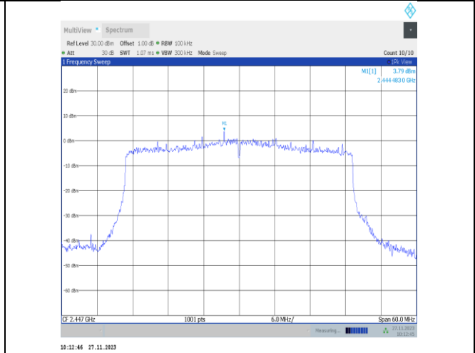
11ax40MIMO-Ant25-2447-0~Reference-PASS
