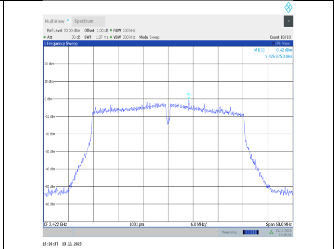
11VHT40MIMO-Ant25-2422-0~Reference-PASS
