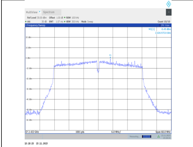
11VHT40MIMO-Ant22-2422-0~Reference-PASS
