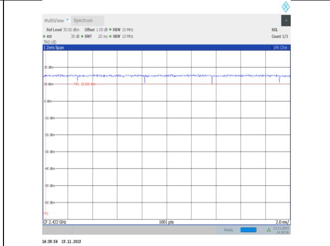
NTNV-11n40MIMO-Ant25-2422
