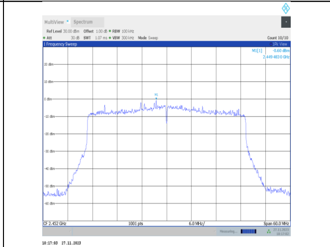
11ax40MIMO-Ant25-2452-0~Reference-PASS
