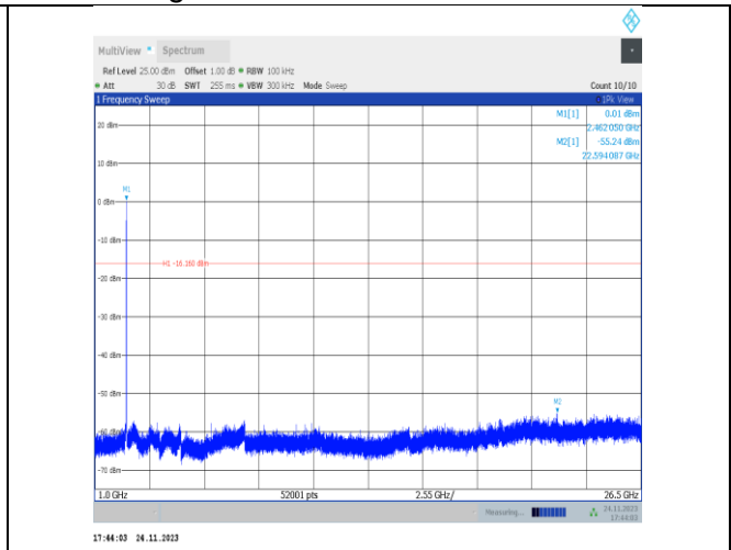
11ax20MIMO-Ant25-2462-1000~26500-PASS
