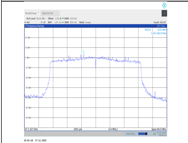
11ax40MIMO-Ant22-2427-0~Reference-PASS
