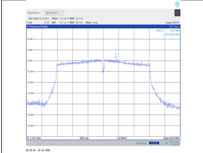
11VHT40MIMO-Ant22-2427-0~Reference-PASS
