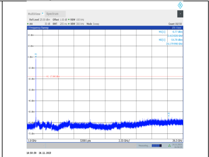
11ax20MIMO-Ant25-2412-1000~26500-PASS
