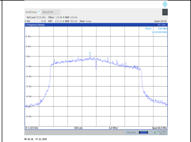
11ax40MIMO-Ant25-2422-0~Reference-PASS
