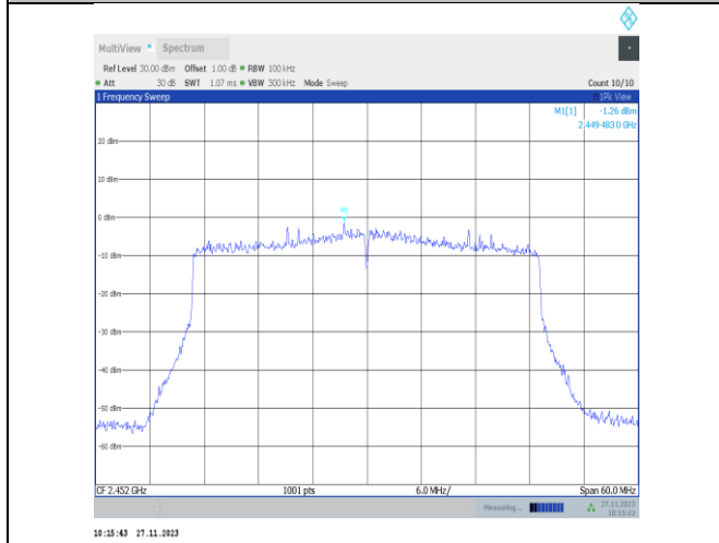
11ax40MIMO-Ant22-2452-0~Reference-PASS
