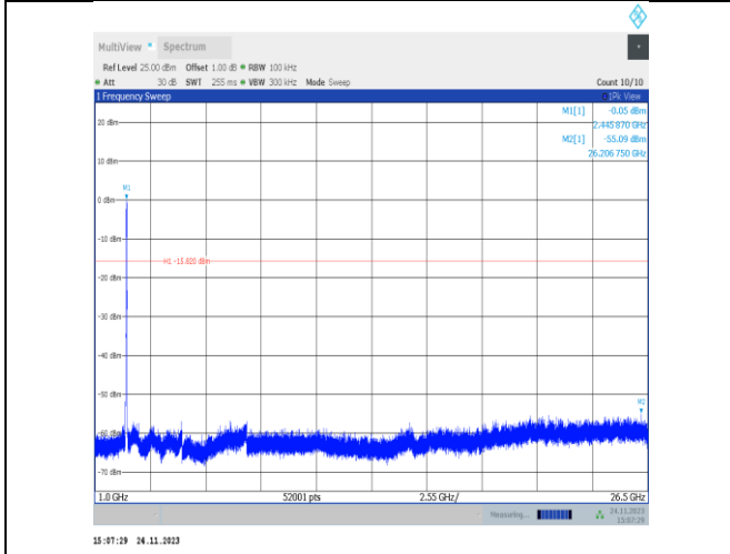
11VHT40MIMO-Ant22-2447-1000~26500-PASS
