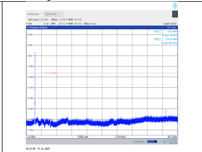
11ax40MIMO-Ant25-2447-1000~26500-PASS
