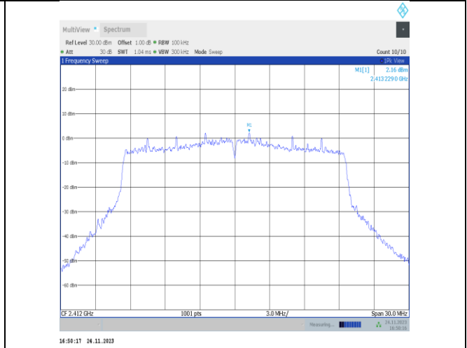
11ax20MIMO-Ant25-2412-0~Reference-PASS
