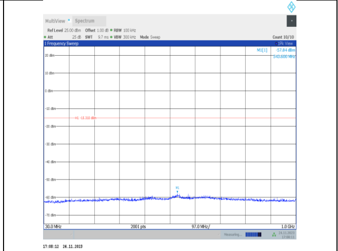
11ax20MIMO-Ant22-2417-30~1000-PASS
