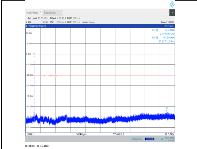
11VHT40MIMO-Ant22-2422-1000~26500-PASS
