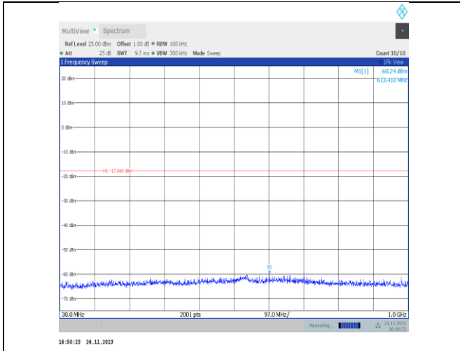
11ax20MIMO-Ant25-2412-30~1000-PASS
