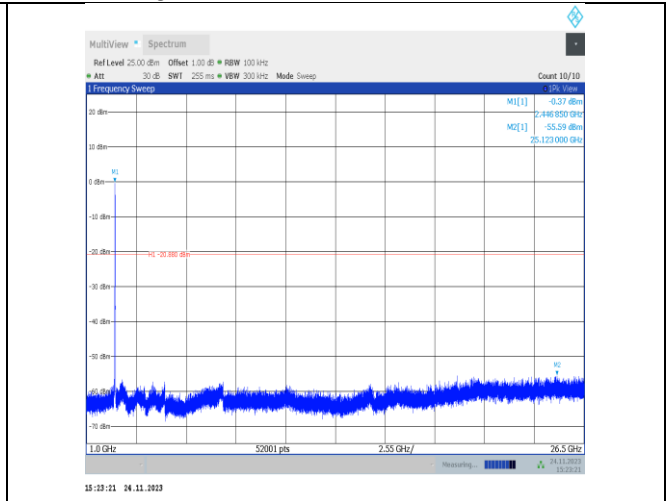
11VHT40MIMO-Ant25-2452-1000~26500-PASS
