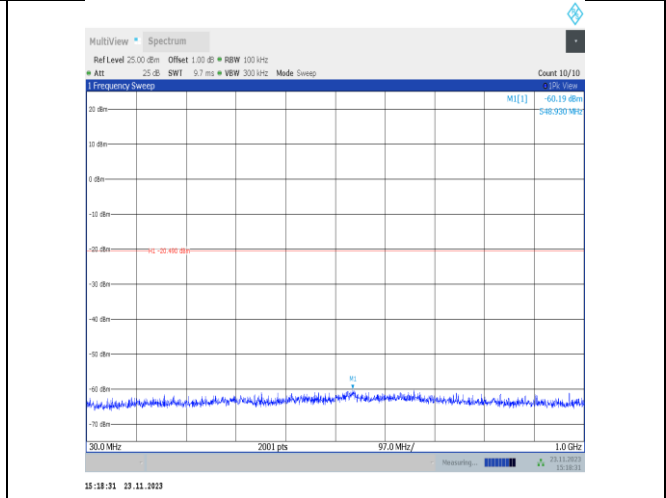
11VHT40MIMO-Ant22-2422-30~1000-PASS
