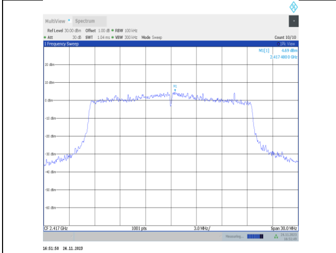
11ax20MIMO-Ant22-2417-0~Reference-PASS
