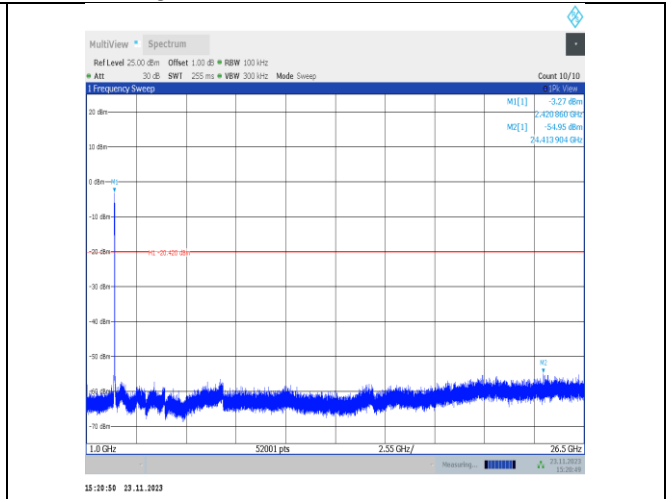
11VHT40MIMO-Ant25-2422-1000~26500-PASS
