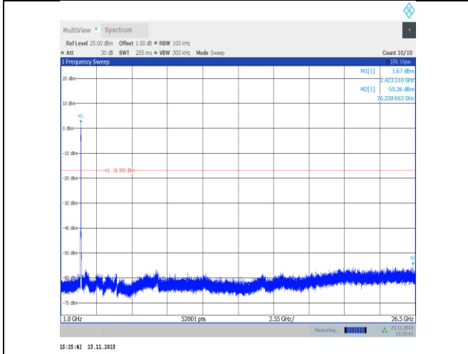
11VHT40MIMO-Ant22-2427-1000~26500-PASS
