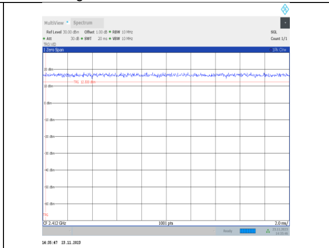
NTNV-11n20MIMO-Ant25-2412
