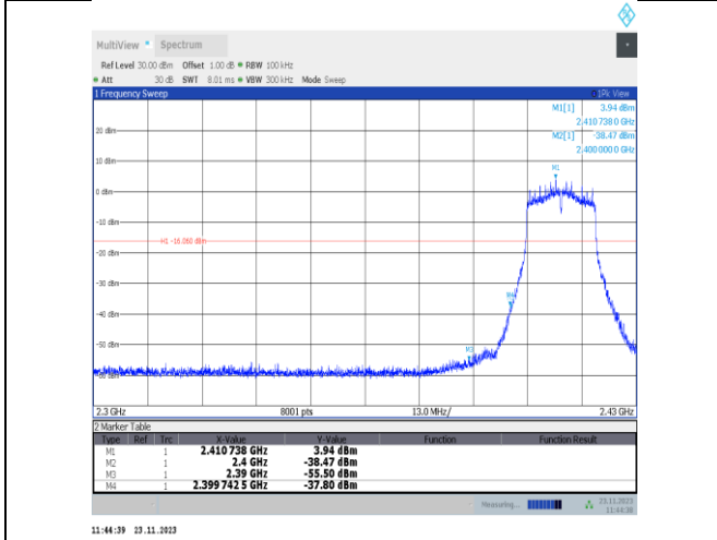
11g-CDD-Ant22-2412-PASS
