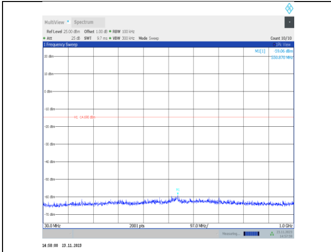
11VHT20MIMO-Ant25-2417-30~1000-PASS
