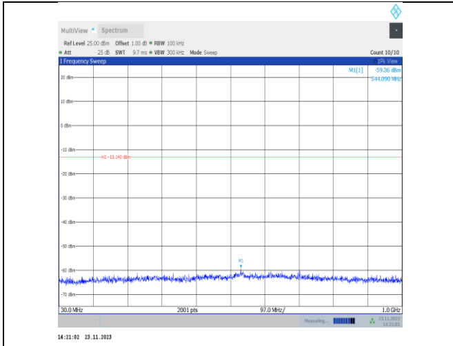
11g-CDD-Ant25-2457-30~1000-PASS
