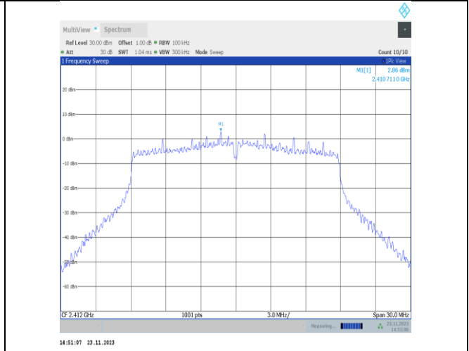
11VHT20MIMO-Ant25-2412-0~Reference-PASS
