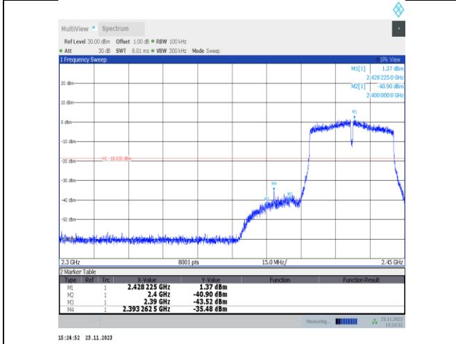
11VHT40MIMO-Ant22-2427-PASS
