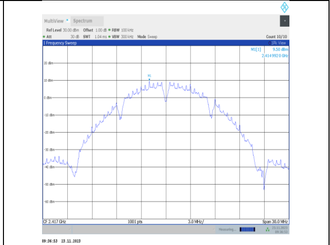
11b-CDD-Ant25-2417-0~Reference-PASS
