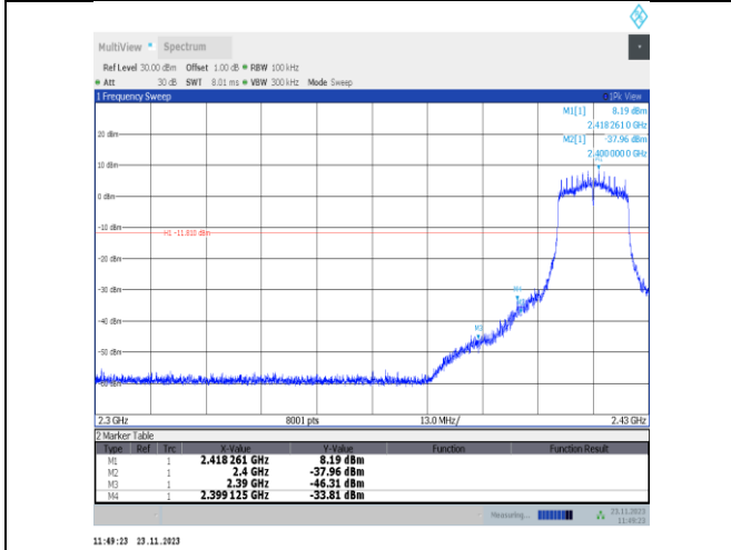
11g-CDD-Ant22-2417-PASS
