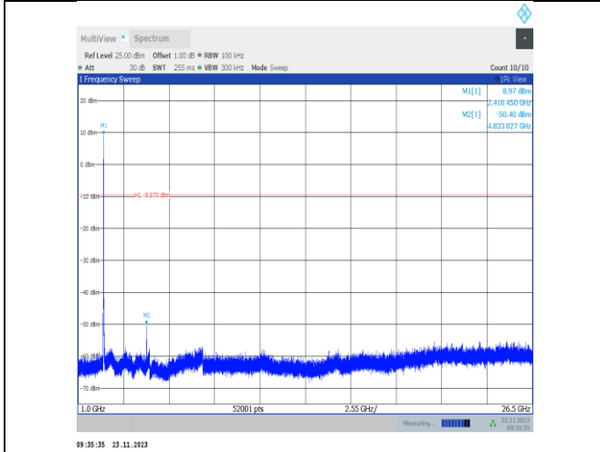
11b-CDD-Ant22-2417-1000~26500-PASS
