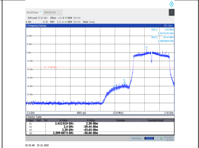
11VHT40MIMO-Ant25-2427-PASS
