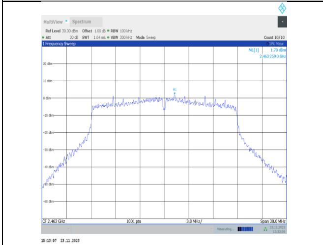
11VHT20MIMO-Ant22-2462-0~Reference-PASS
