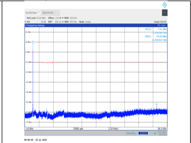
11b-CDD-Ant25-2437-1000~26500-PASS
