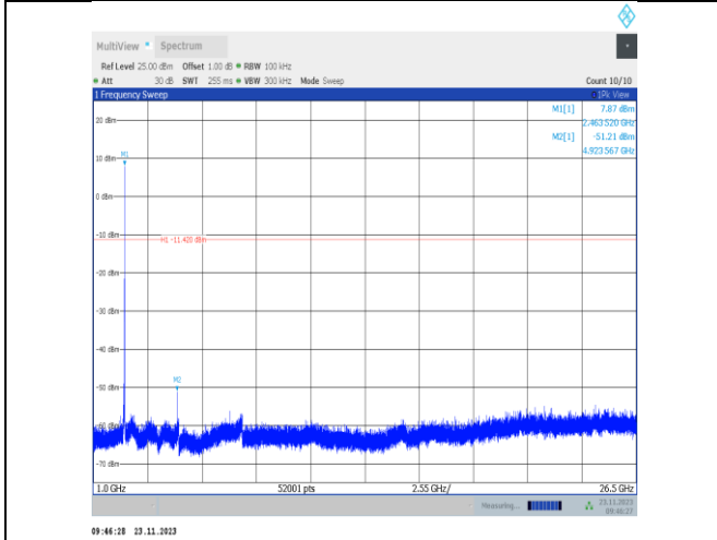
11b-CDD-Ant22-2462-1000~26500-PASS
