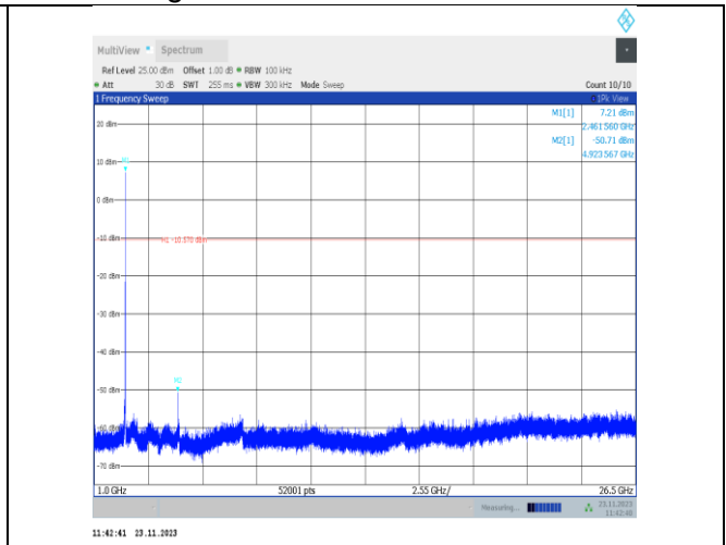
11b-CDD-Ant25-2462-1000~26500-PASS
