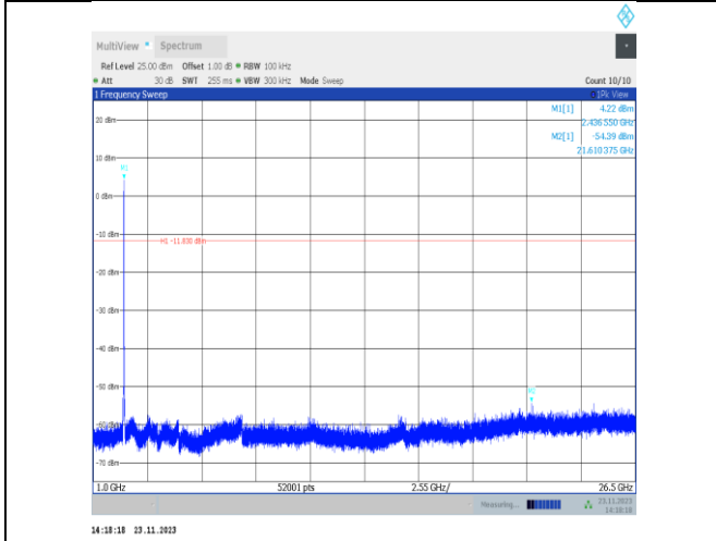
11g-CDD-Ant22-2437-1000~26500-PASS
