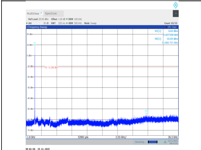
11b-CDD-Ant22-2437-1000~26500-PASS
