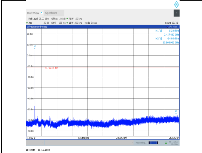
11g-CDD-Ant22-2417-1000~26500-PASS
