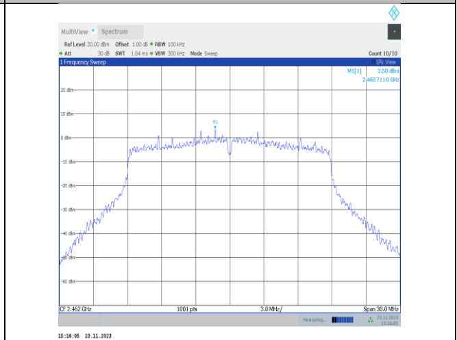
11VHT20MIMO-Ant25-2462-0~Reference-PASS
