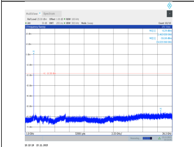
11VHT20MIMO-Ant22-2462-1000~26500-PASS
