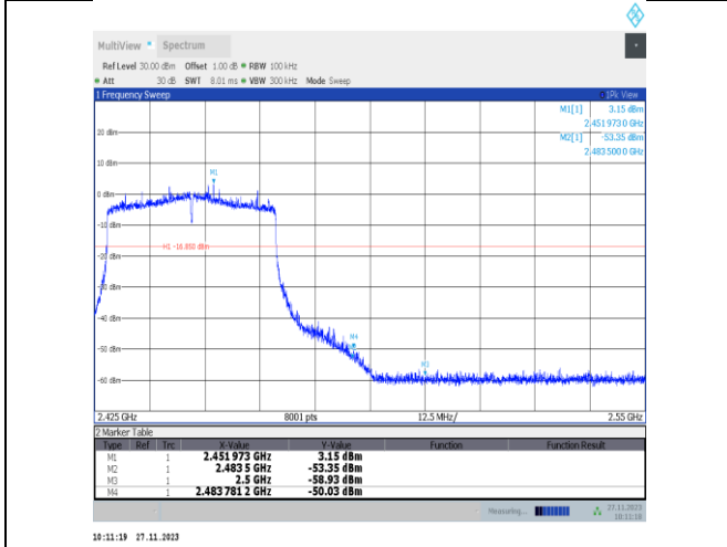
11ax40MIMO-Ant22-2447-PASS
