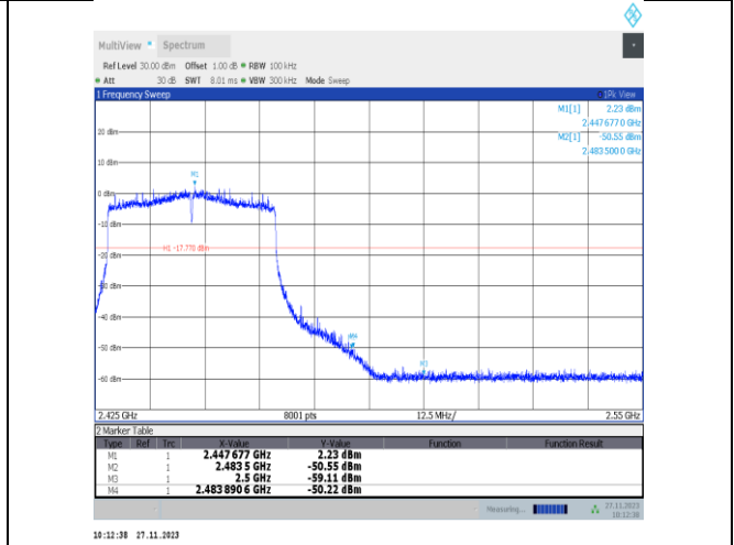
11ax40MIMO-Ant25-2447-PASS
