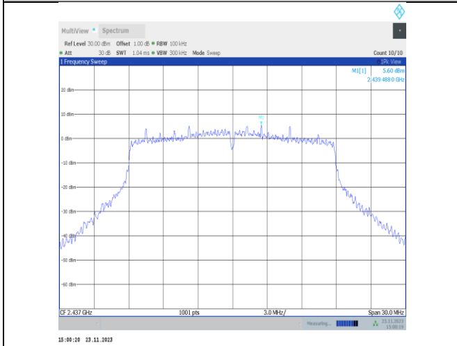
11VHT20MIMO-Ant22-2437-0~Reference-PASS
