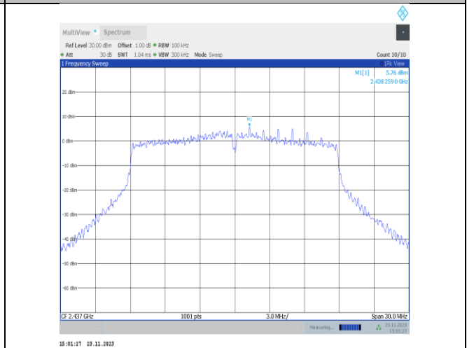
11VHT20MIMO-Ant25-2437-0~Reference-PASS
