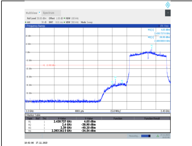
11ax40MIMO-Ant22-2427-PASS
