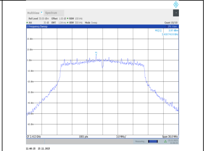
11g-CDD-Ant25-2412-0~Reference-PASS
