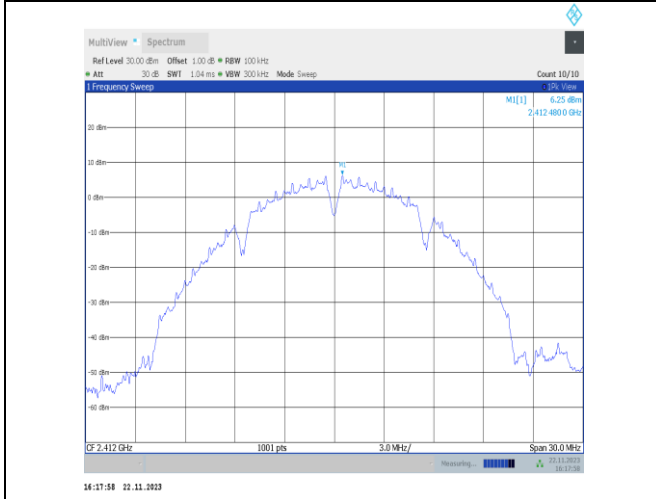
11b-CDD-Ant22-2412-0~Reference-PASS
