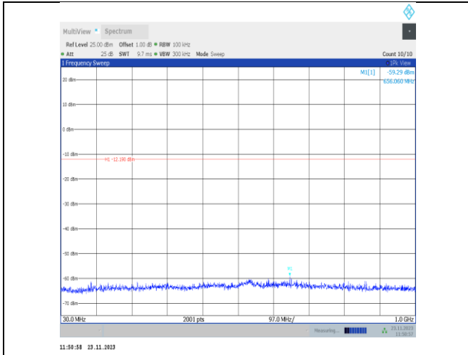
11g-CDD-Ant25-2417-30~1000-PASS
