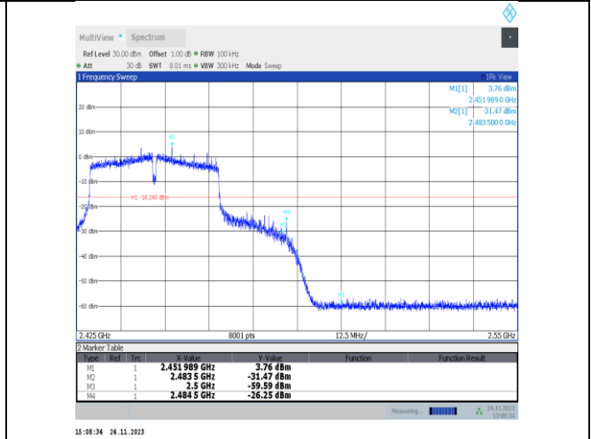
11VHT40MIMO-Ant25-2447-PASS
