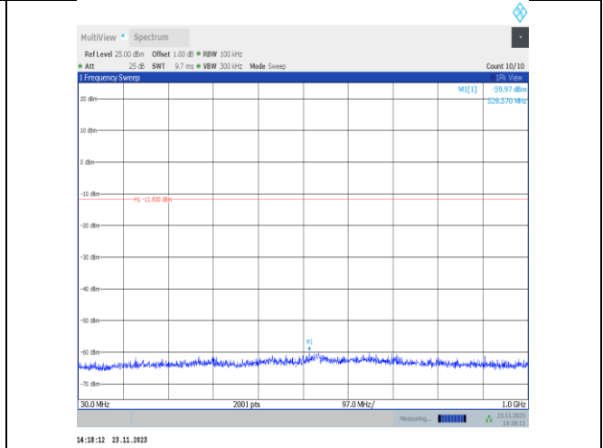
11g-CDD-Ant22-2437-30~1000-PASS
