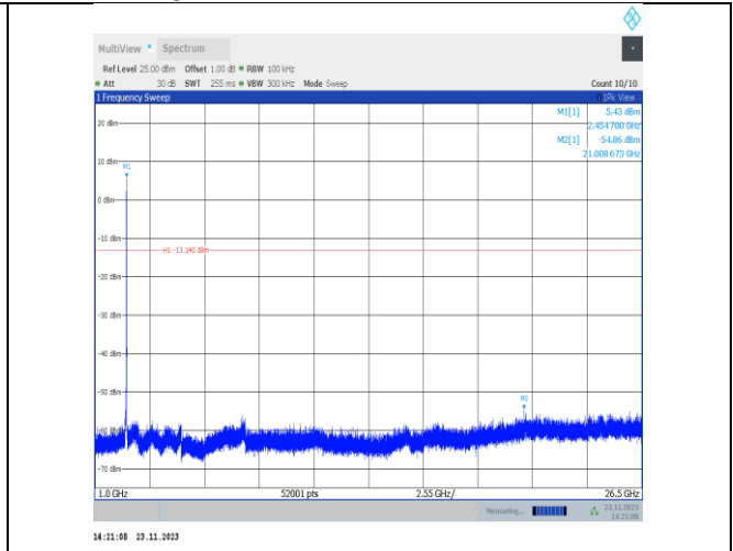
11g-CDD-Ant25-2457-1000~26500-PASS
