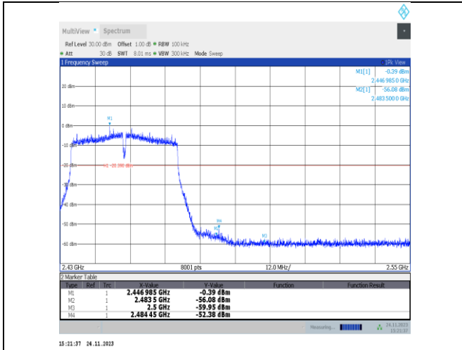
11VHT40MIMO-Ant22-2452-PASS
