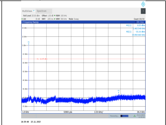
11g-CDD-Ant25-2462-1000~26500-PASS
