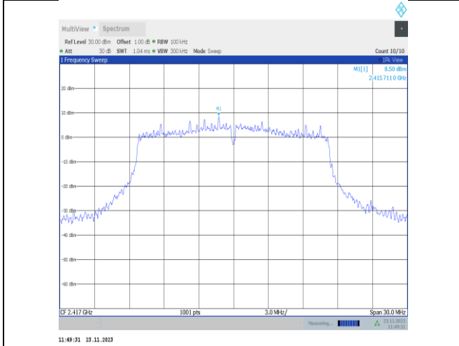
11g-CDD-Ant22-2417-0~Reference-PASS
