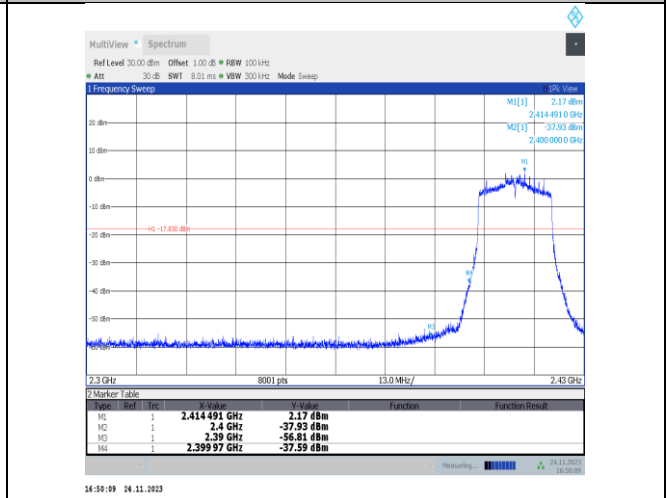
11ax20MIMO-Ant25-2412-PASS
