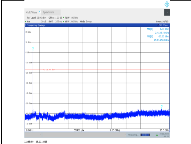
11g-CDD-Ant22-2412-1000~26500-PASS
