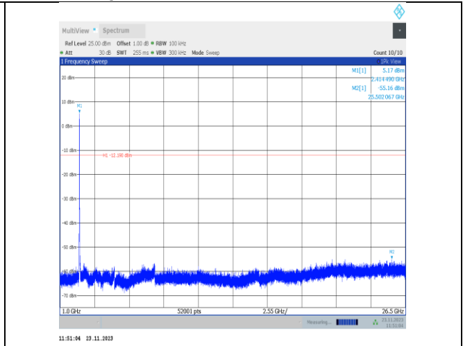
11g-CDD-Ant25-2417-1000~26500-PASS
