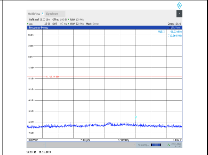
11VHT20MIMO-Ant22-2462-30~1000-PASS
