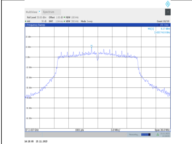
11g-CDD-Ant22-2437-0~Reference-PASS
