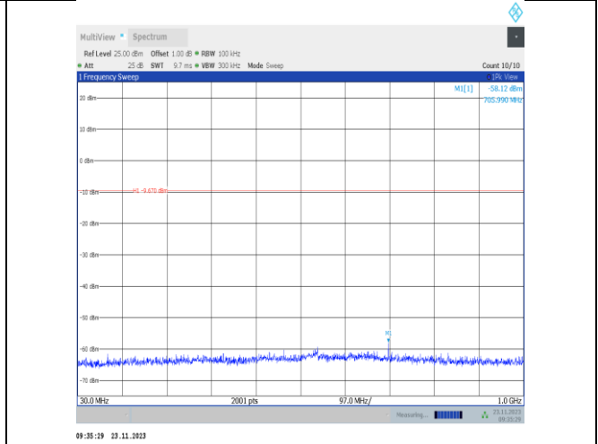
11b-CDD-Ant22-2417-30~1000-PASS
