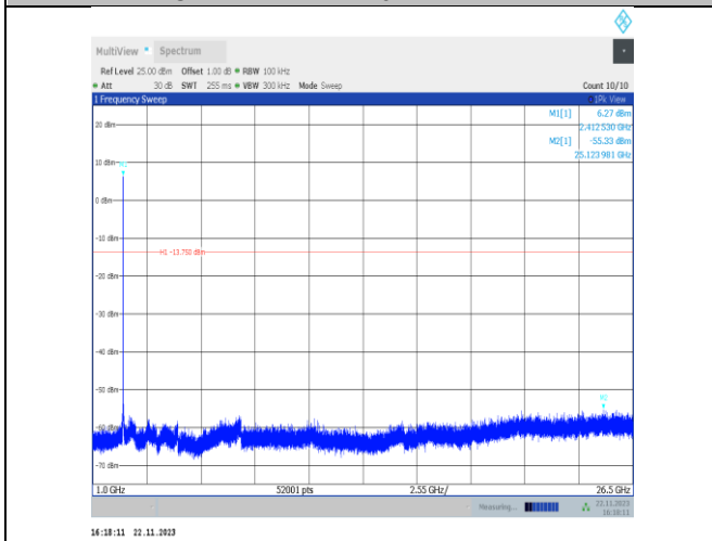
11b-CDD-Ant22-2412-1000~26500-PASS
