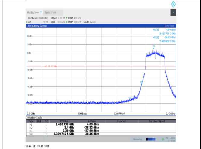
11g-CDD-Ant25-2412-PASS
