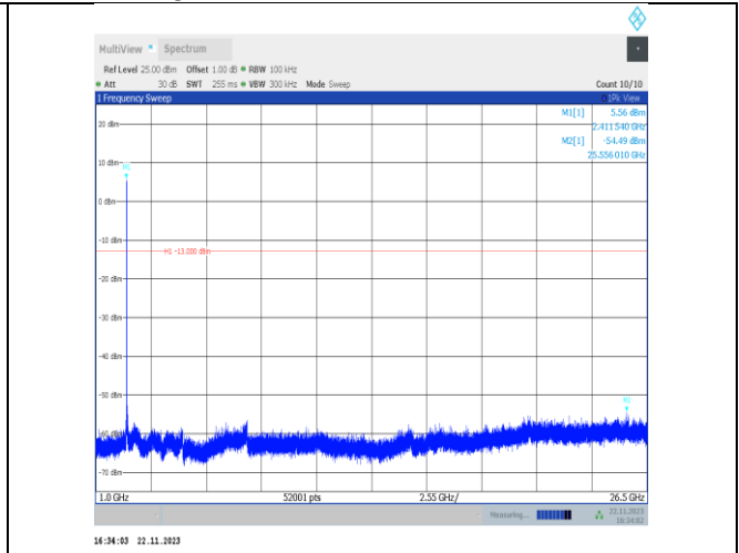
11b-CDD-Ant25-2412-1000~26500-PASS
