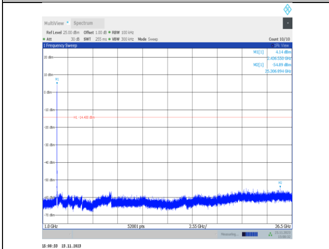
11VHT20MIMO-Ant22-2437-1000~26500-PASS
