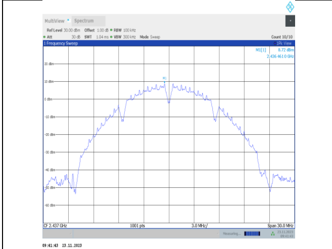
11b-CDD-Ant22-2437-0~Reference-PASS
