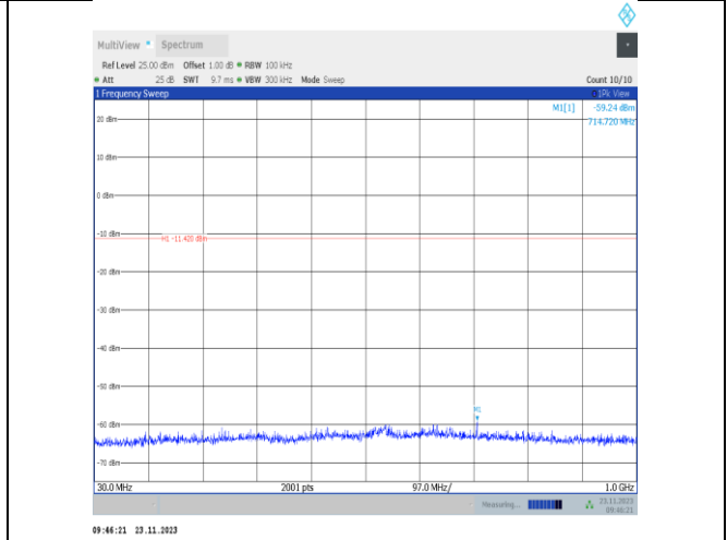
11b-CDD-Ant22-2462-30~1000-PASS
