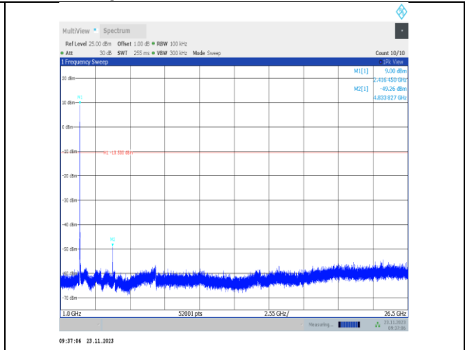
11b-CDD-Ant25-2417-1000~26500-PASS
