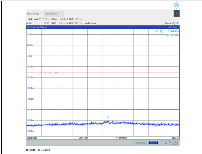
11g-CDD-Ant25-2462-30~1000-PASS
