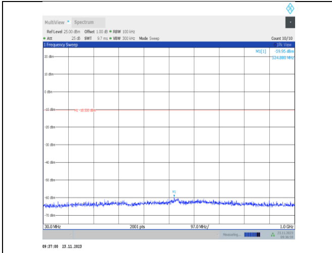
11b-CDD-Ant25-2417-30~1000-PASS
