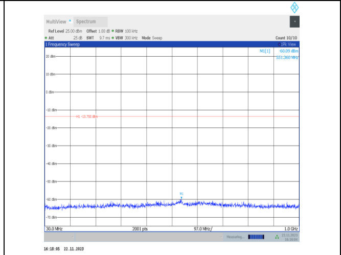
11b-CDD-Ant22-2412-30~1000-PASS
