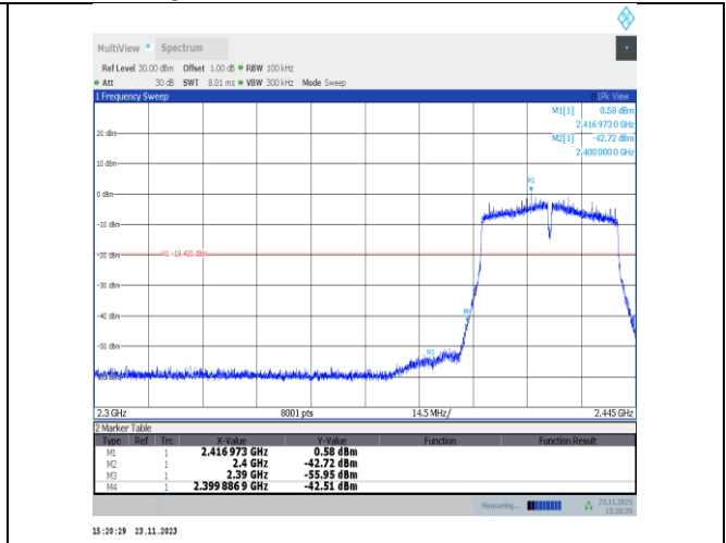
11VHT40MIMO-Ant25-2422-PASS
