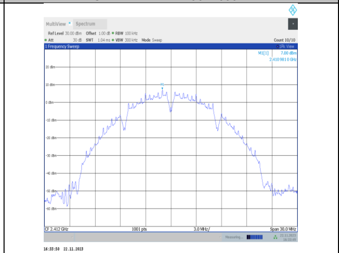
11b-CDD-Ant25-2412-0~Reference-PASS
