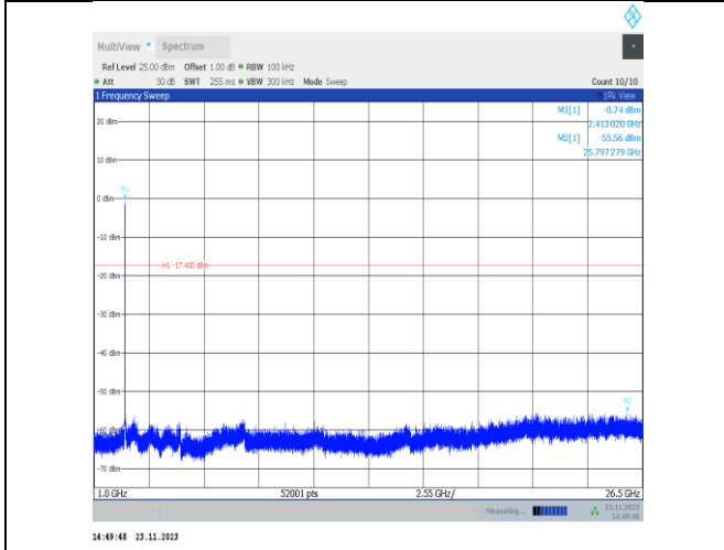
11VHT20MIMO-Ant22-2412-1000~26500-PASS
