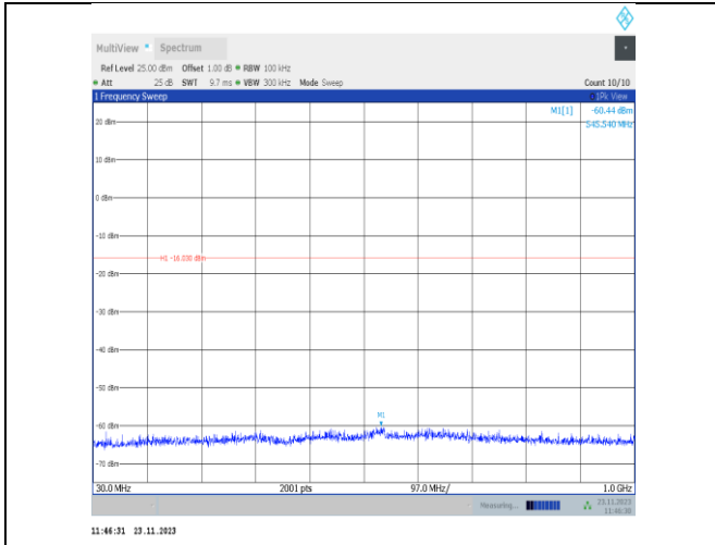
11g-CDD-Ant25-2412-30~1000-PASS
