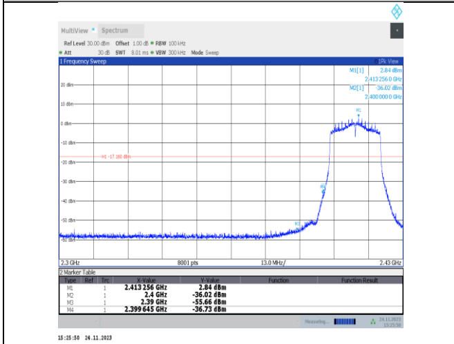
11ax20MIMO-Ant22-2412-PASS
