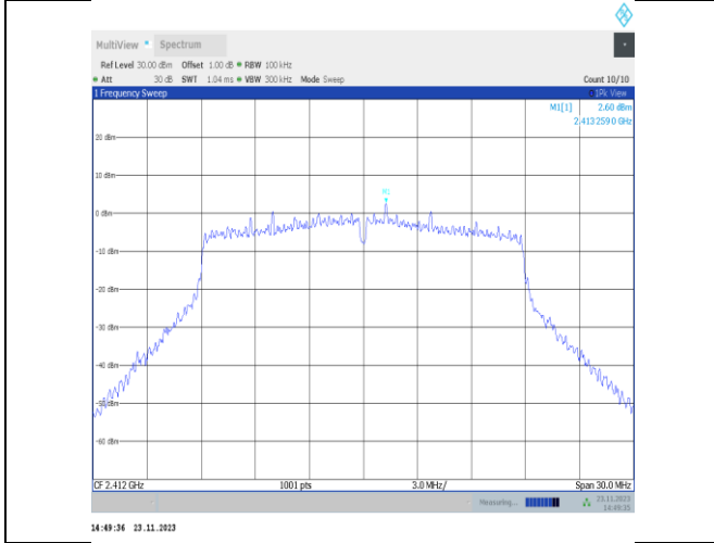
11VHT20MIMO-Ant22-2412-0~Reference-PASS
