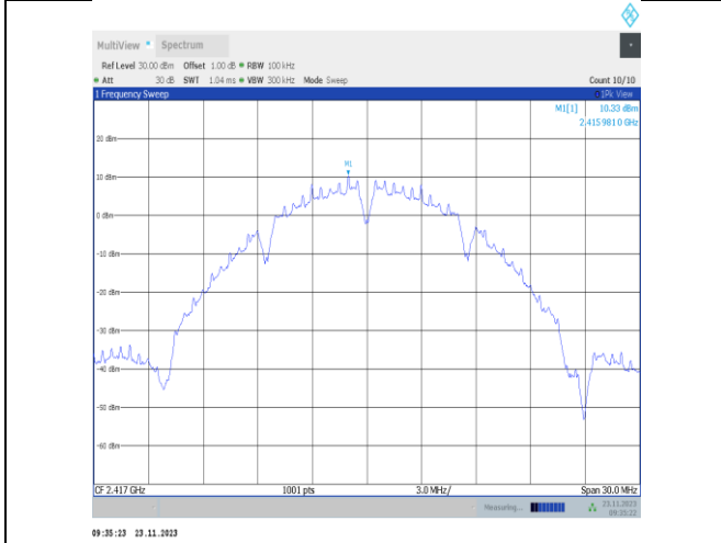
11b-CDD-Ant22-2417-0~Reference-PASS
