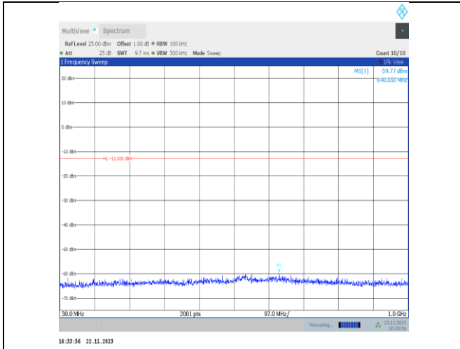
11b-CDD-Ant25-2412-30~1000-PASS
