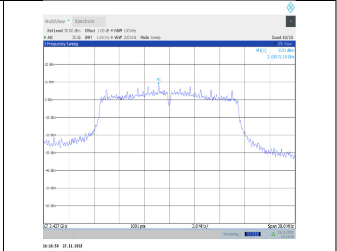
11g-CDD-Ant25-2437-0~Reference-PASS
