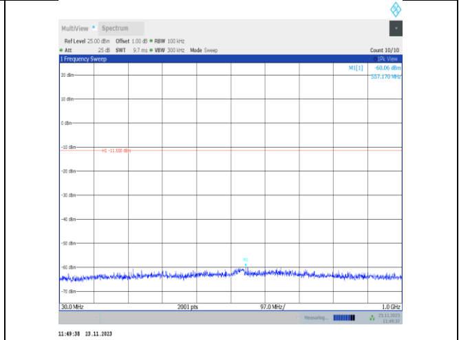
11g-CDD-Ant22-2417-30~1000-PASS
