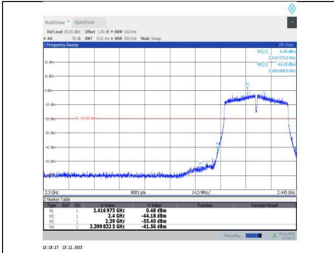
11VHT40MIMO-Ant22-2422-PASS
