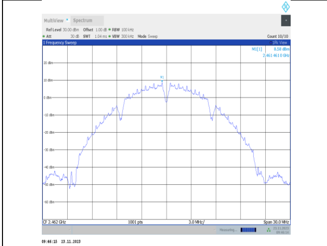
11b-CDD-Ant22-2462-0~Reference-PASS
