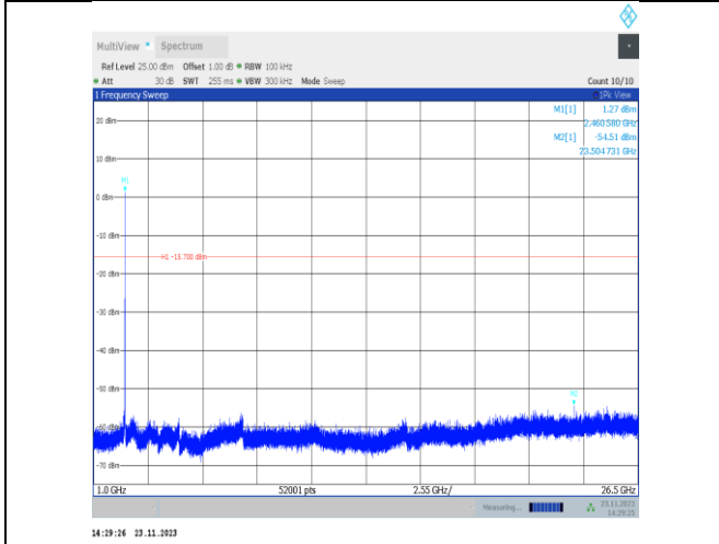
11g-CDD-Ant22-2462-1000~26500-PASS
