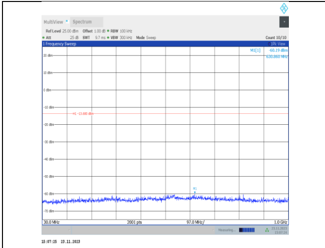
11VHT20MIMO-Ant25-2457-30~1000-PASS
