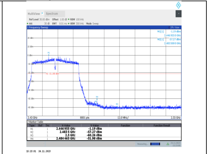
11VHT40MIMO-Ant25-2452-PASS
