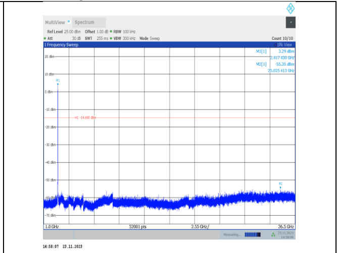
11VHT20MIMO-Ant25-2417-1000~26500-PASS
