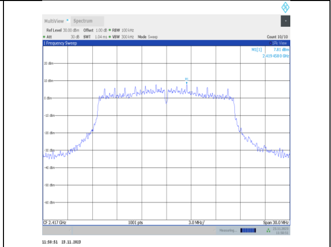
11g-CDD-Ant25-2417-0~Reference-PASS
