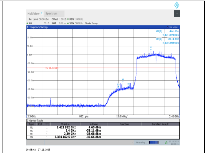
11ax40MIMO-Ant25-2427-PASS
