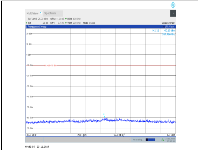
11b-CDD-Ant25-2437-30~1000-PASS
