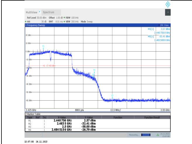
11VHT40MIMO-Ant22-2447-PASS
