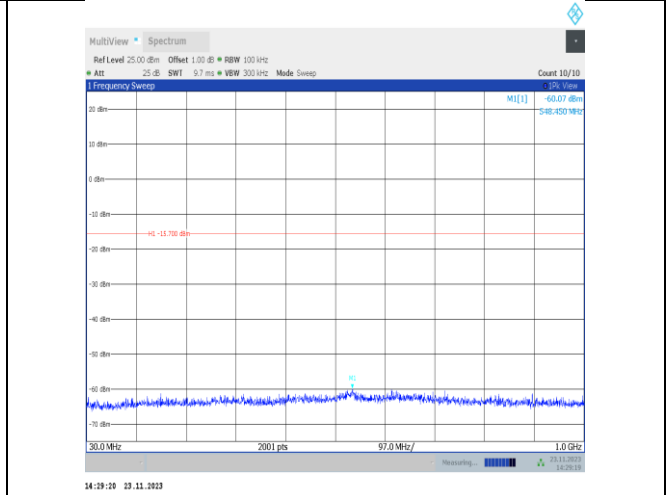
11g-CDD-Ant22-2462-30~1000-PASS
