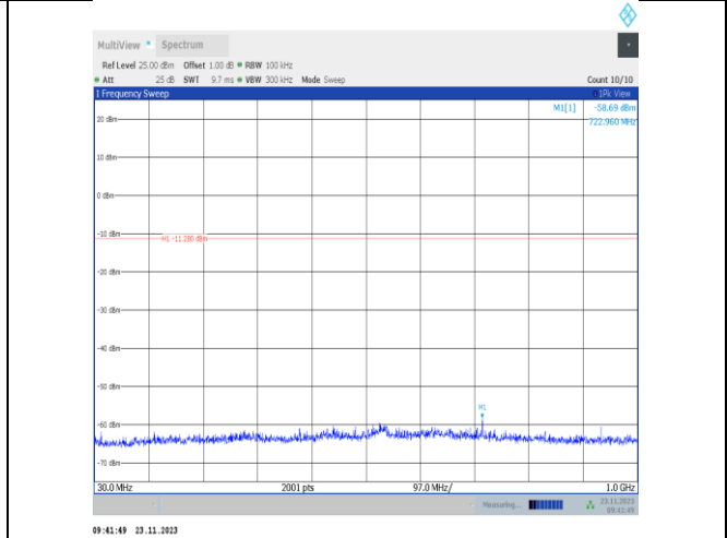
11b-CDD-Ant22-2437-30~1000-PASS
