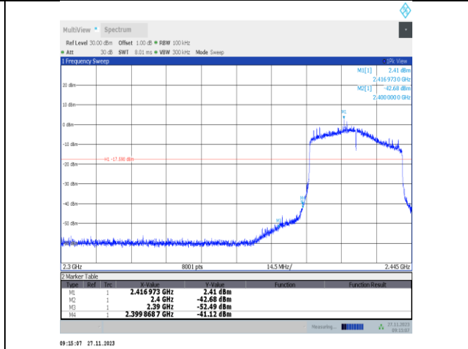
11ax40MIMO-Ant25-2422-PASS
