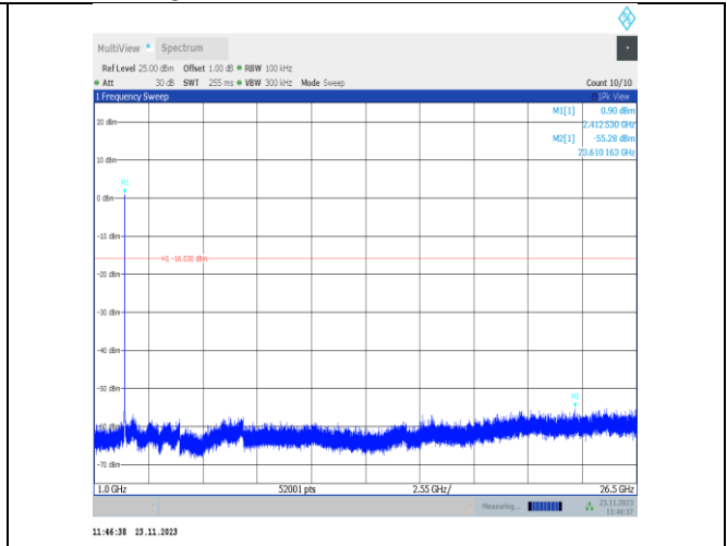
11g-CDD-Ant25-2412-1000~26500-PASS
