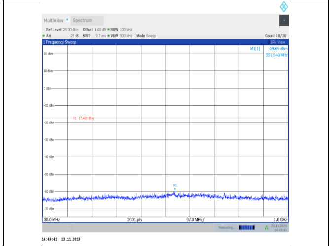
11VHT20MIMO-Ant22-2412-30~1000-PASS
