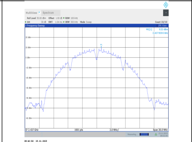
11b-CDD-Ant25-2437-0~Reference-PASS
