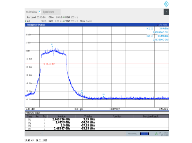
11ax20MIMO-Ant25-2462-PASS
