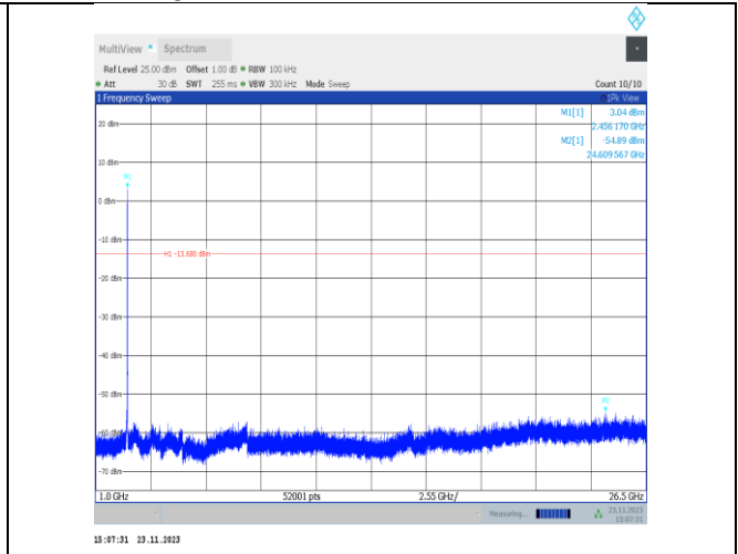
11VHT20MIMO-Ant25-2457-1000~26500-PASS
