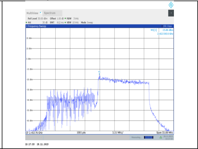
11ax40MIMO-Ant25-2452-242Tone-RU62-PASS
