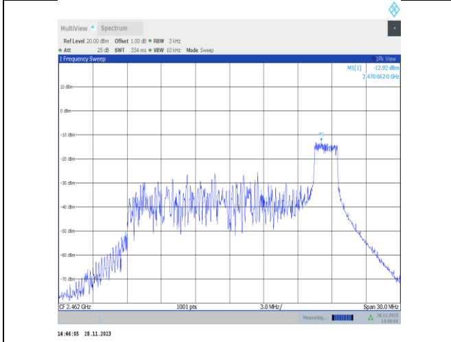
11ax20MIMO-Ant22-2462-26Tone-RU8-PASS
