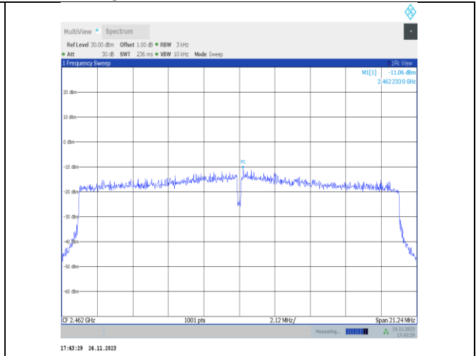
11ax20MIMO-Ant25-2462-PASS
