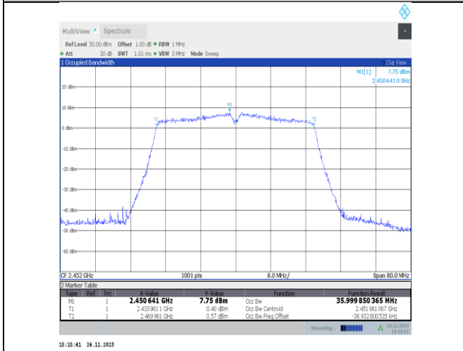
11VHT40MIMO-Ant22-2452
