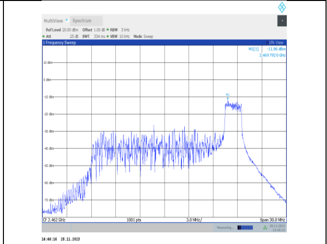
11ax20MIMO-Ant25-2462-26Tone-RU8-PASS
