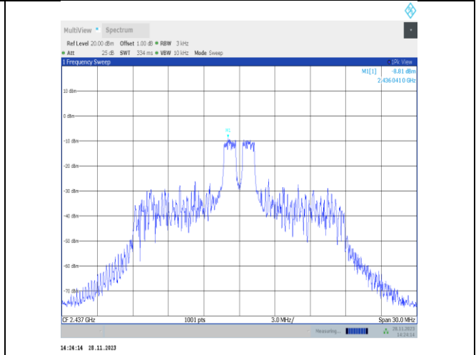
11ax20MIMO-Ant25-2437-26Tone-RU4-PASS
