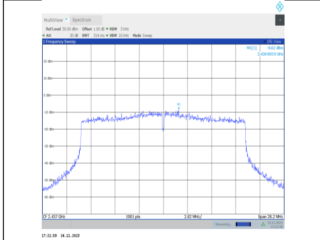
11ax20MIMO-Ant22-2437-PASS
