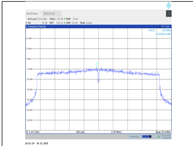
11ax20MIMO-Ant22-2417-PASS
