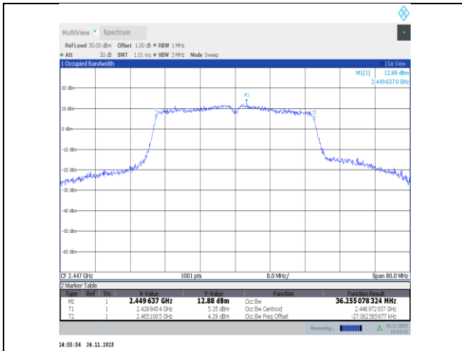
11VHT40MIMO-Ant22-2447
