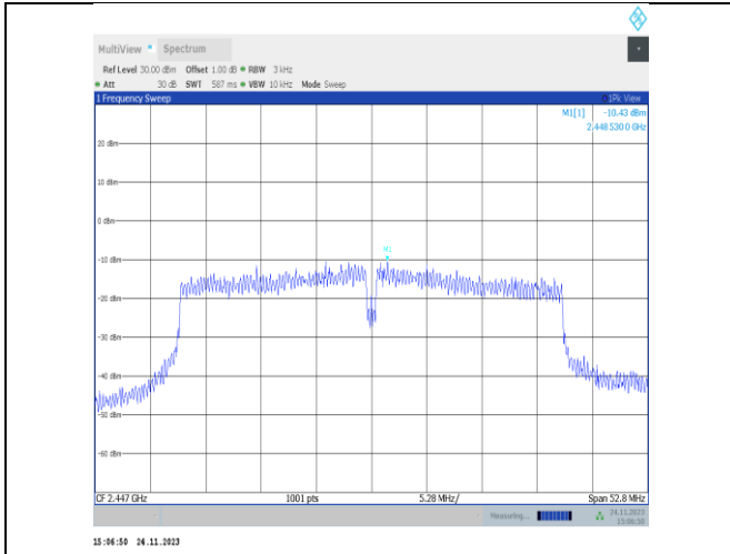
11VHT40MIMO-Ant22-2447-PASS
