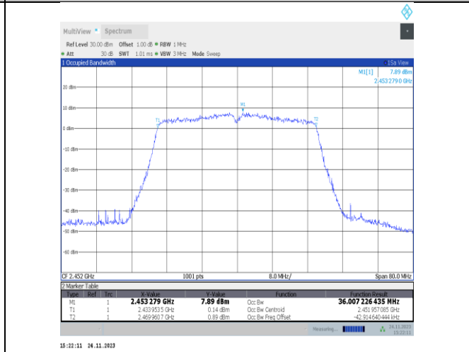
11VHT40MIMO-Ant25-2452
