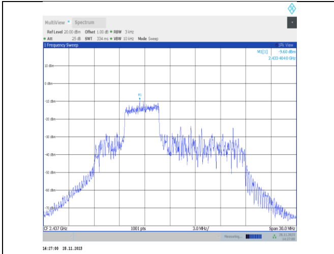
11ax20MIMO-Ant25-2437-52Tone-RU38-PASS
