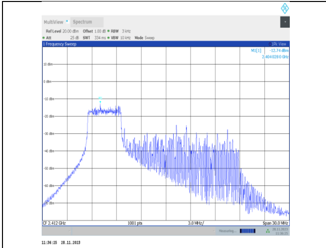
11ax20MIMO-Ant25-2412-52Tone-RU37-PASS
