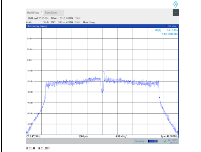
11VHT40MIMO-Ant22-2452-PASS
