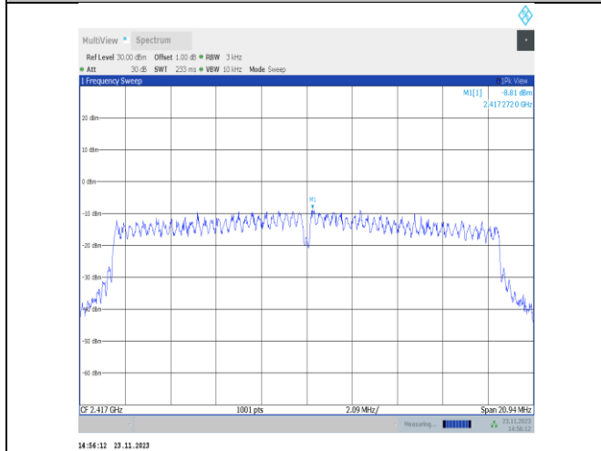
11VHT20MIMO-Ant22-2417-PASS
