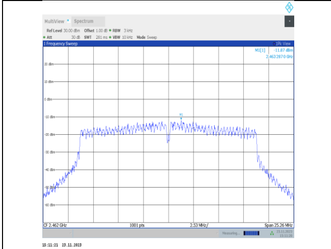
11VHT20MIMO-Ant22-2462-PASS
