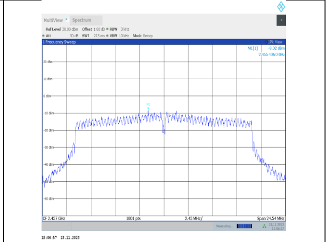
11VHT20MIMO-Ant25-2457-PASS
