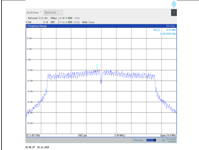
11VHT20MIMO-Ant22-2457-PASS
