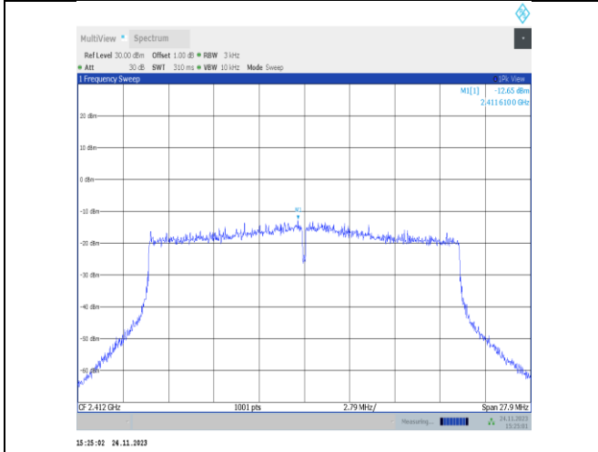
11ax20MIMO-Ant22-2412-PASS
