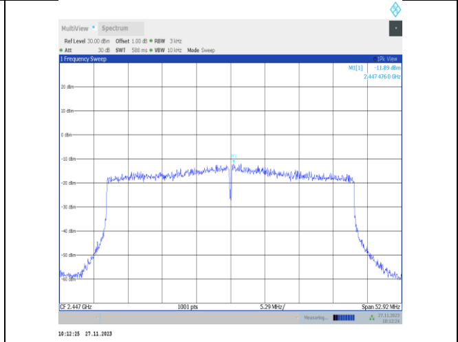
11ax40MIMO-Ant25-2447-PASS
