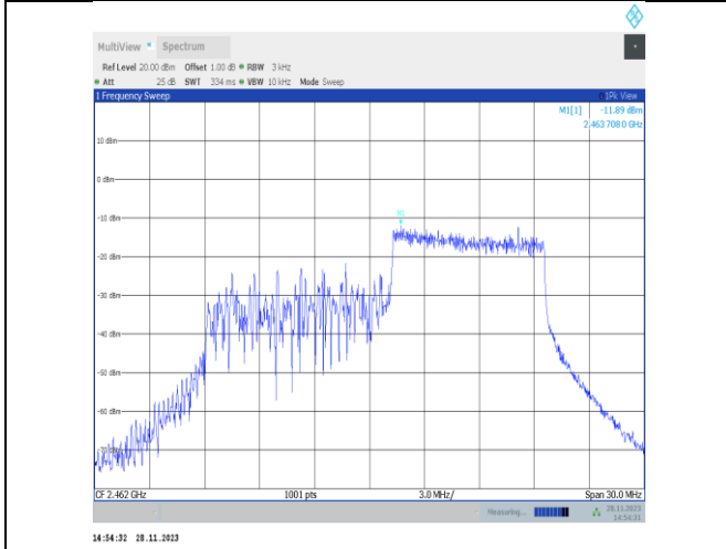
11ax20MIMO-Ant22-2462-106Tone-RU54-PASS
