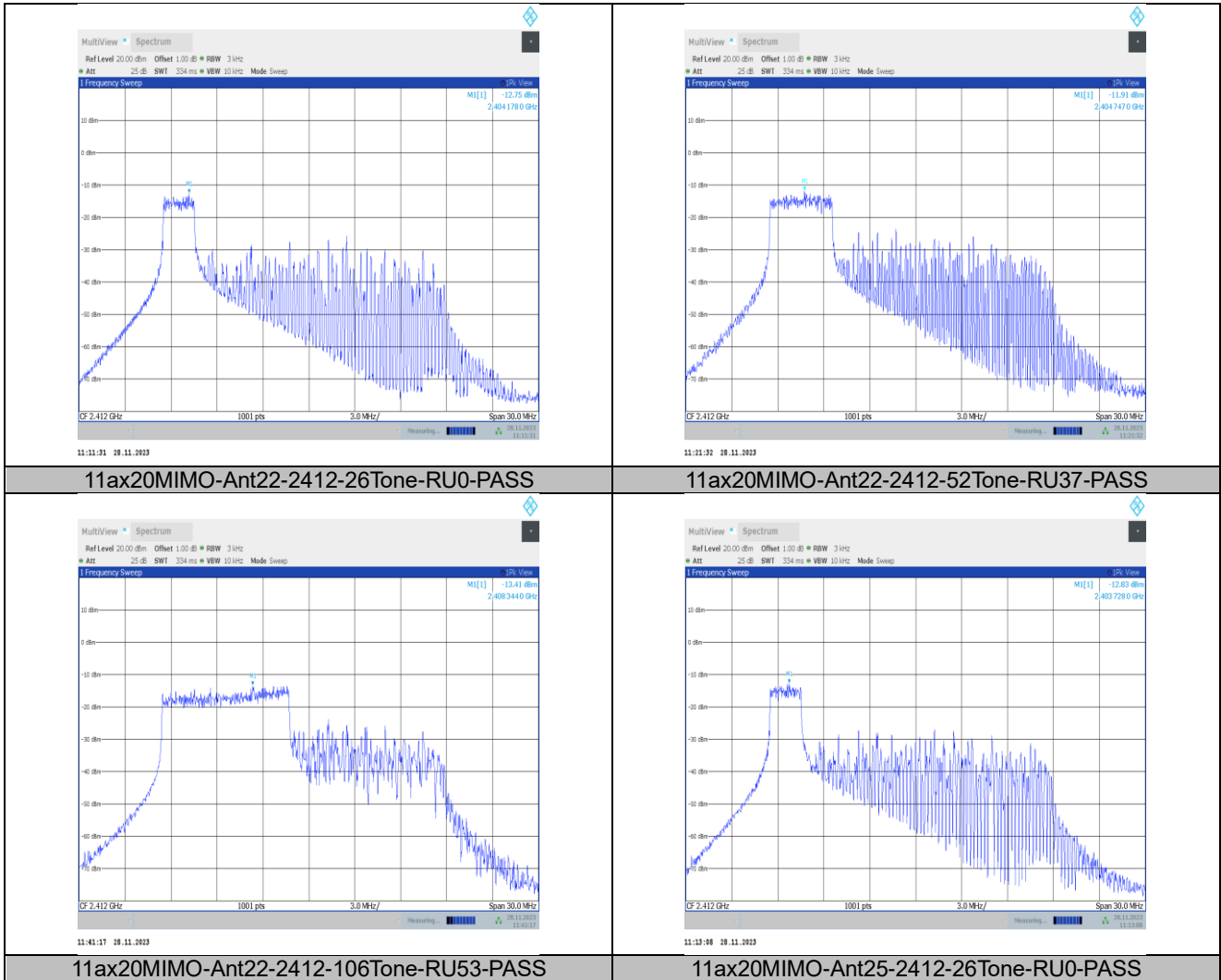
11ax20MIMO-Ant22-2412-106Tone-RU53-PASS
