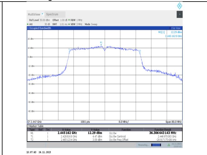
11VHT40MIMO-Ant25-2447
