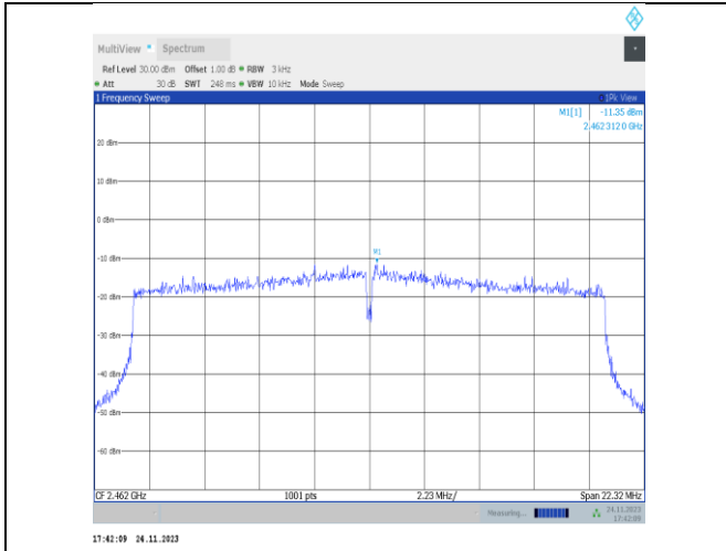
11ax20MIMO-Ant22-2462-PASS
