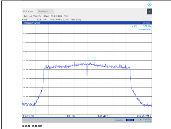
11ax40MIMO-Ant22-2437-PASS
