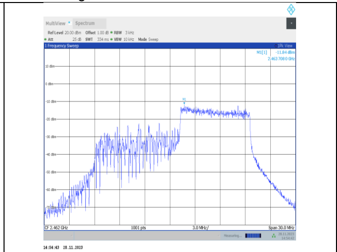
11ax20MIMO-Ant25-2462-106Tone-RU54-PASS
