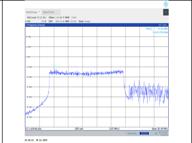
11ax40MIMO-Ant25-2437-242Tone-RU61-PASS
