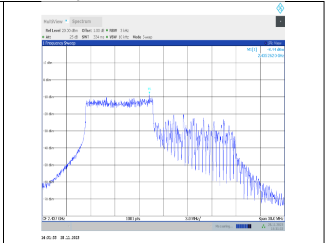
11ax20MIMO-Ant25-2437-106Tone-RU53-PASS
