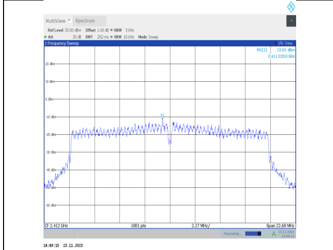
11VHT20MIMO-Ant22-2412-PASS
