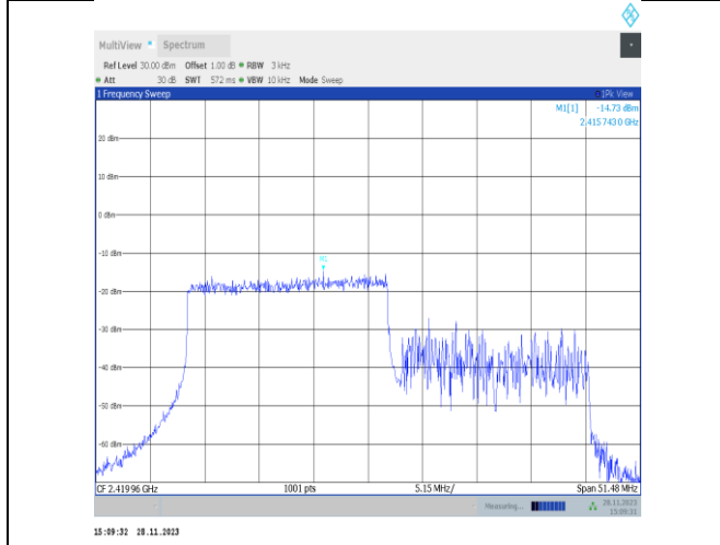
11ax40MIMO-Ant22-2422-242Tone-RU61-PASS
