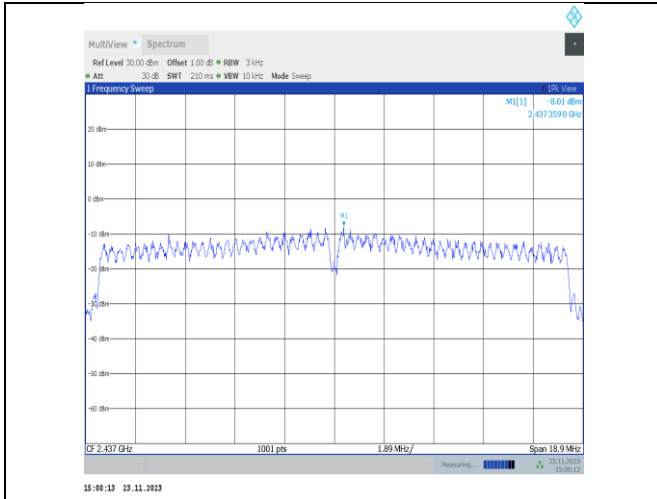
11VHT20MIMO-Ant22-2437-PASS
