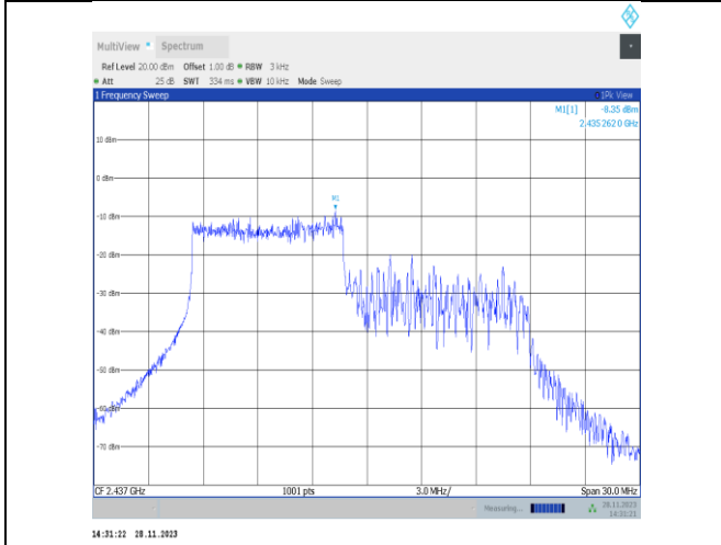
11ax20MIMO-Ant22-2437-106Tone-RU53-PASS
