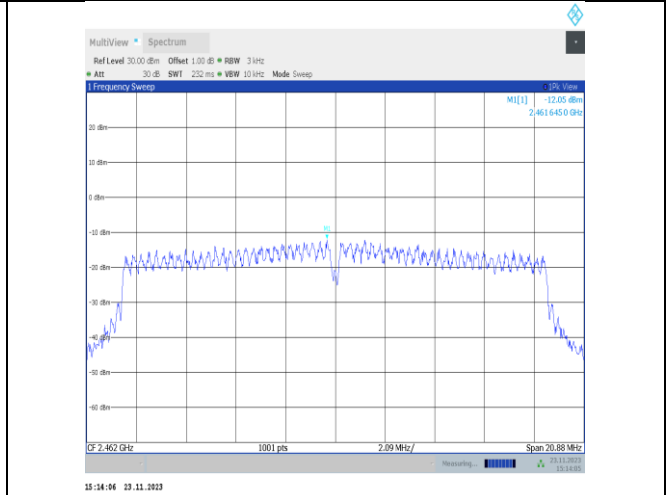
11VHT20MIMO-Ant25-2462-PASS
