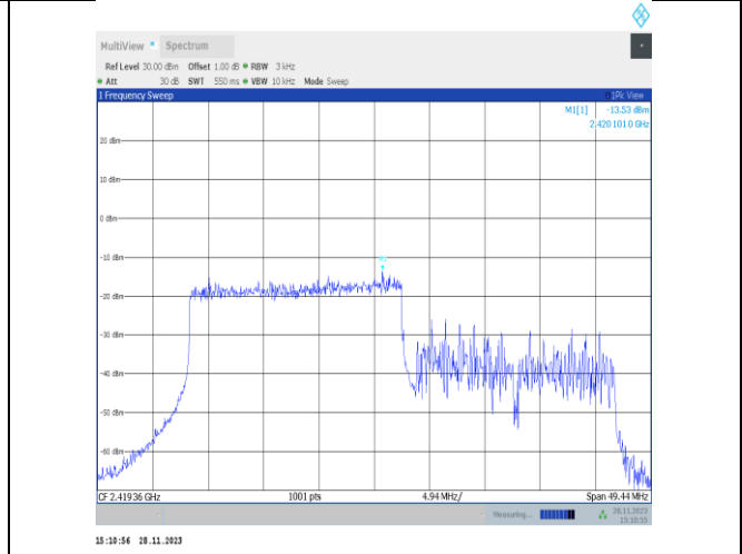
11ax40MIMO-Ant25-2422-242Tone-RU61-PASS
