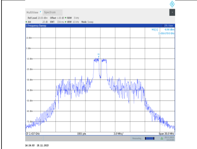
11ax20MIMO-Ant22-2437-26Tone-RU4-PASS
