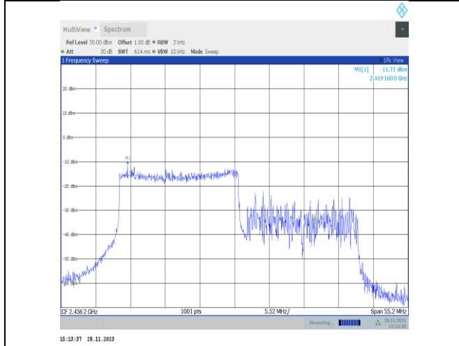
11ax40MIMO-Ant22-2437-242Tone-RU61-PASS
