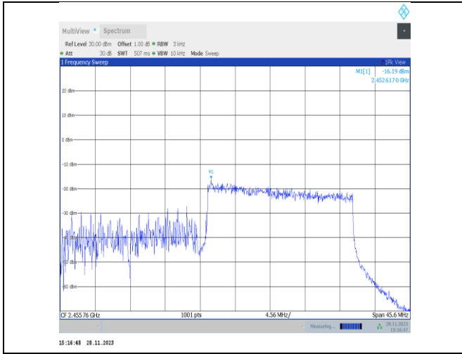
11ax40MIMO-Ant22-2452-242Tone-RU62-PASS
