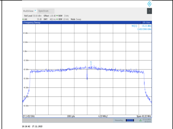
11ax40MIMO-Ant25-2452-PASS
