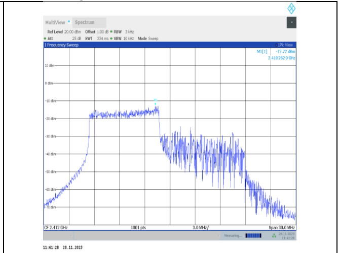
11ax20MIMO-Ant25-2412-106Tone-RU53-PASS
