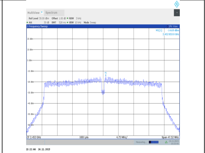
11VHT40MIMO-Ant25-2452-PASS
