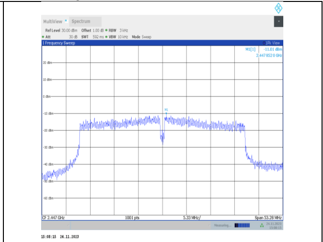
11VHT40MIMO-Ant25-2447-PASS
