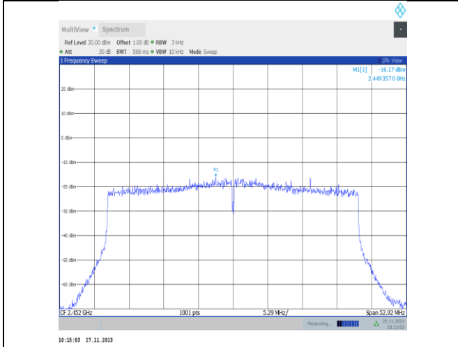
11ax40MIMO-Ant22-2452-PASS
