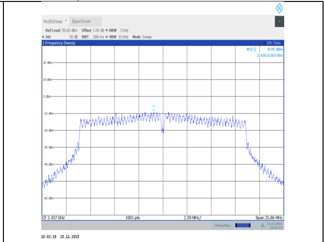
11VHT20MIMO-Ant25-2437-PASS
