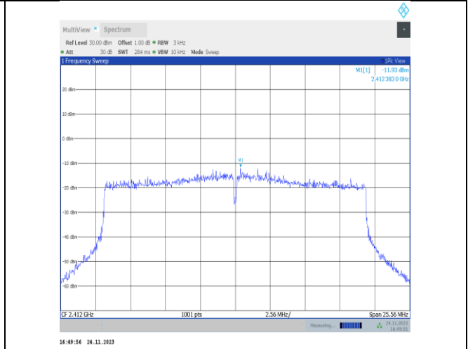
11ax20MIMO-Ant25-2412-PASS
