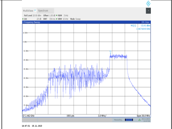
11ax20MIMO-Ant22-2462-52Tone-RU40-PASS
