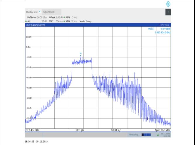
11ax20MIMO-Ant22-2437-52Tone-RU38-PASS
