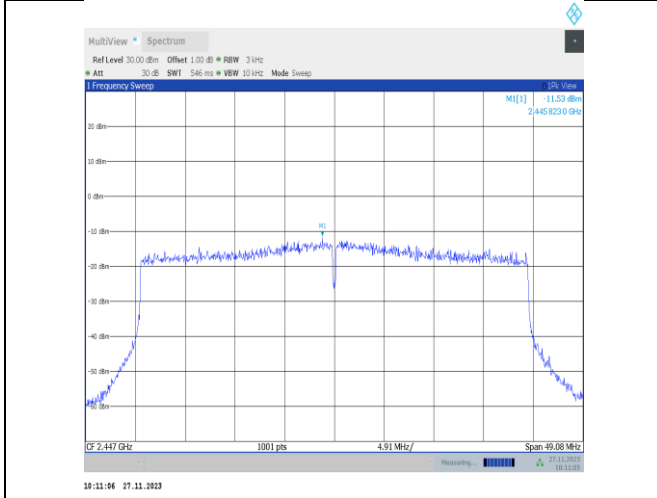
11ax40MIMO-Ant22-2447-PASS
