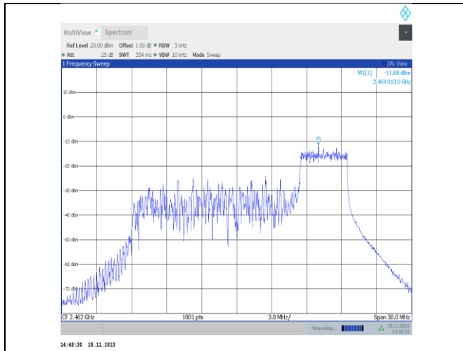
11ax20MIMO-Ant25-2462-52Tone-RU40-PASS
