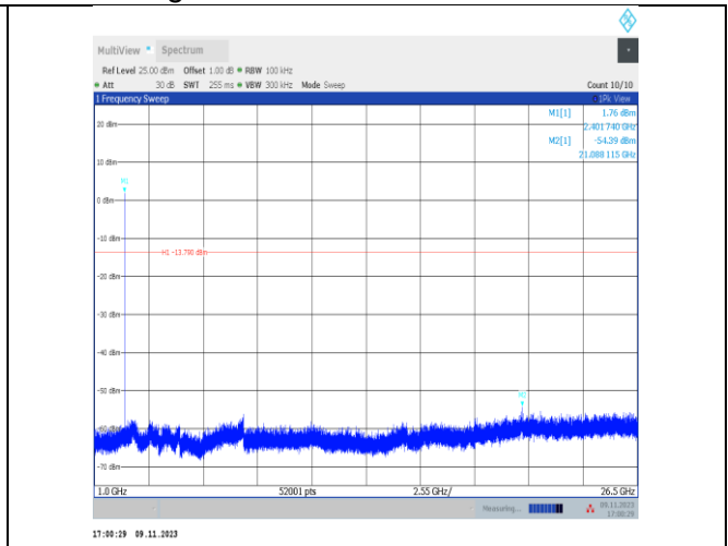
BLE_2M-Ant25-2402-1000~26500-PASS
