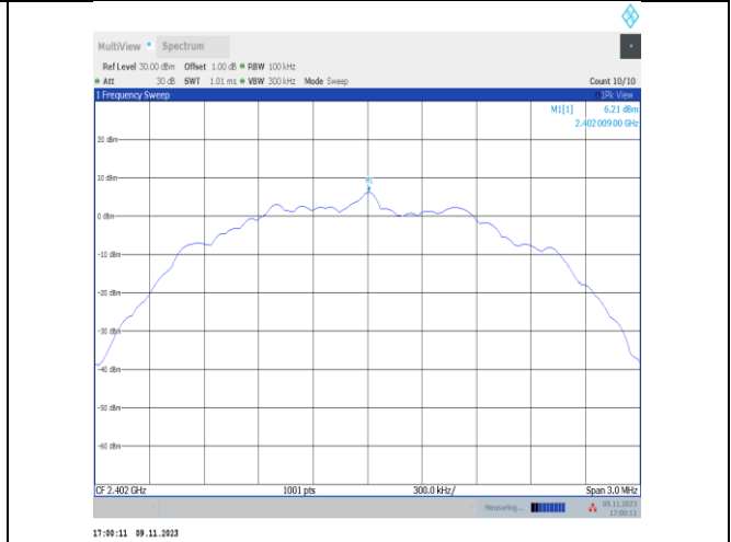
BLE_2M-Ant25-2402-0~Reference-PASS
