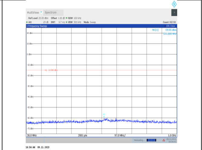
BLE_1M-Ant25-2480-30~1000-PASS
