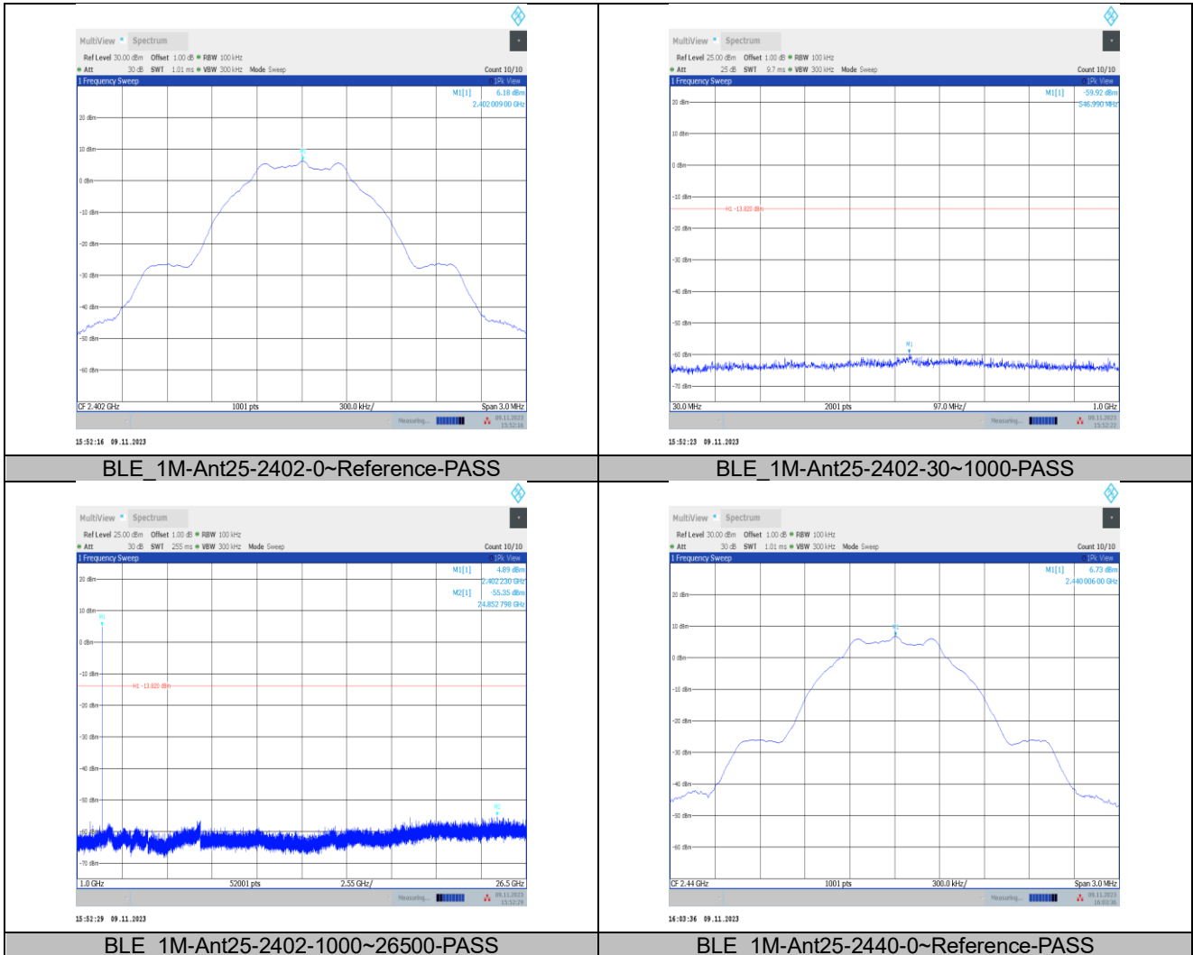
BLE_1M-Ant25-2402-1000~26500-PASS
