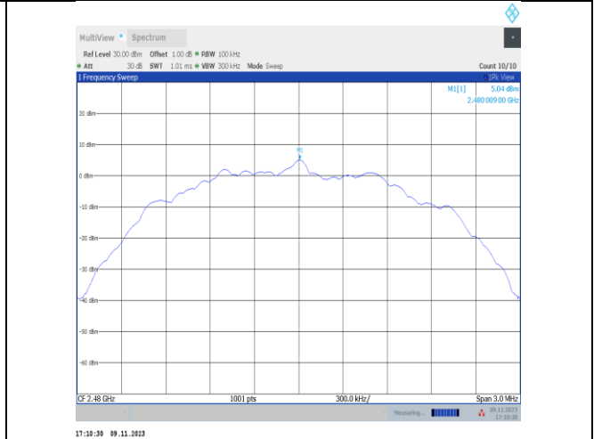
BLE_2M-Ant25-2480-0~Reference-PASS
