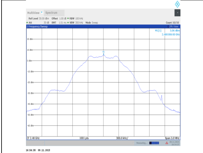
BLE_1M-Ant25-2480-0~Reference-PASS
