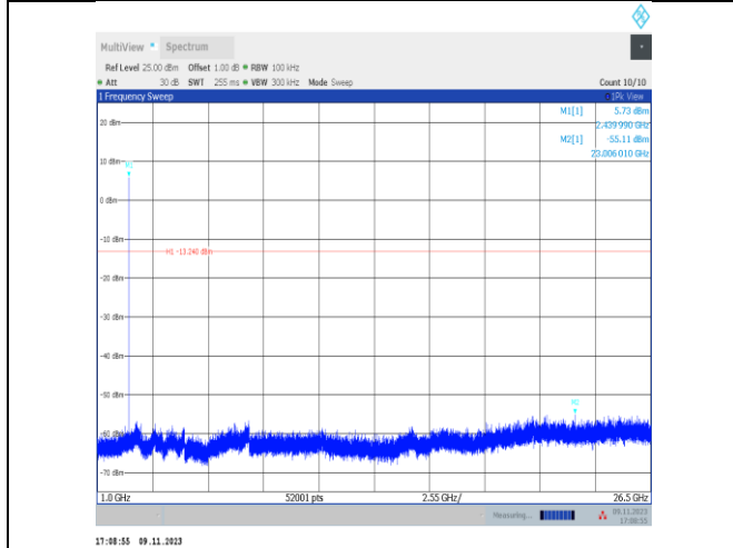
BLE_2M-Ant25-2440-1000~26500-PASS
