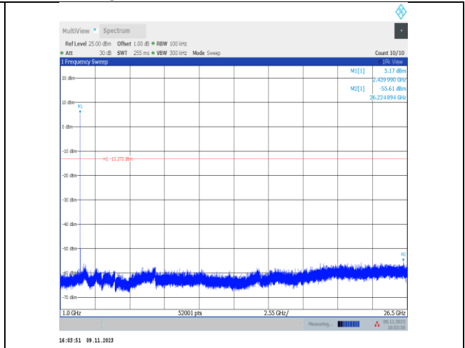
BLE_1M-Ant25-2440-1000~26500-PASS
