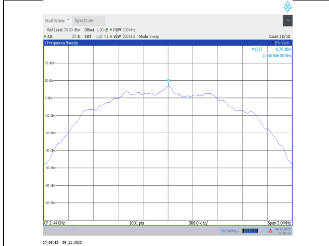
BLE_2M-Ant25-2440-0~Reference-PASS
