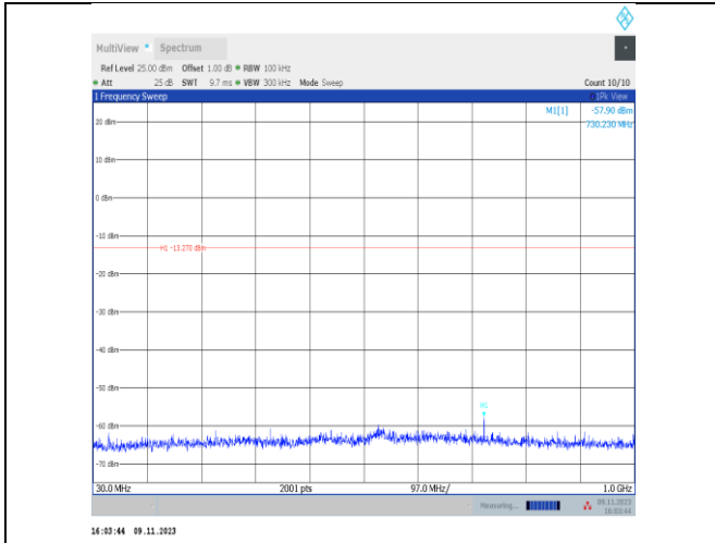
BLE_1M-Ant25-2440-30~1000-PASS
