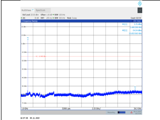
BLE_1M-Ant25-2480-1000~26500-PASS
