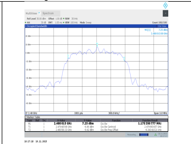
2DH5-Ant25-2480
