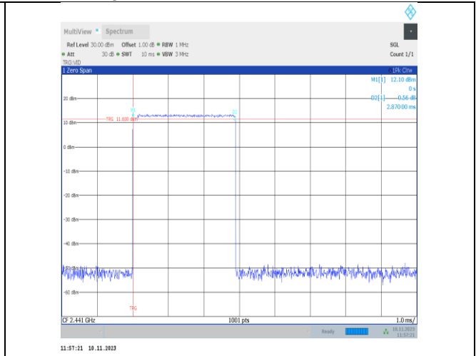
2DH5-Ant25-Hop-PASS
