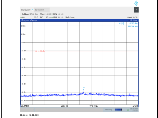
DH5-Ant25-2480-30~1000-PASS
