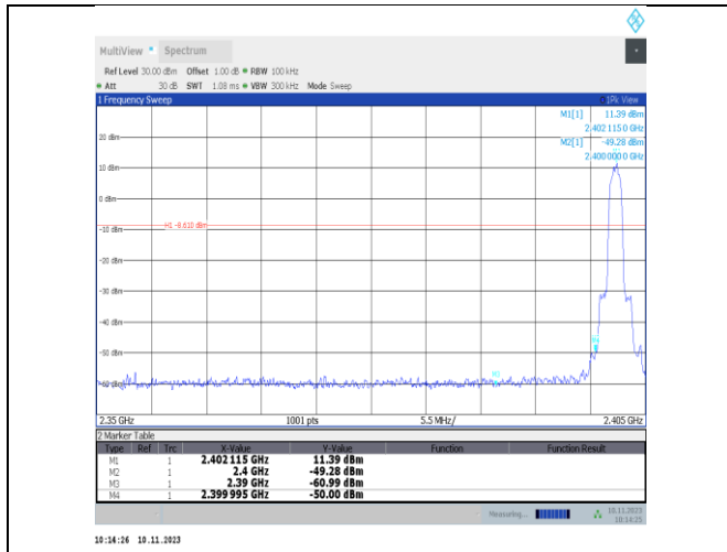
2DH5-Ant25-2402-PASS
