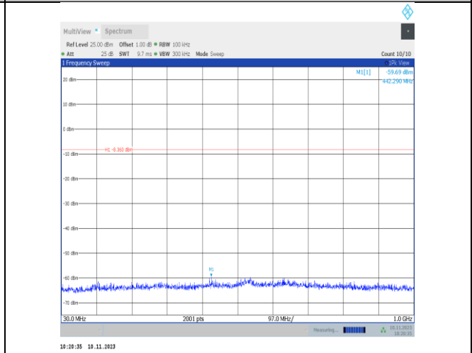
3DH5-Ant25-2402-30~1000-PASS
