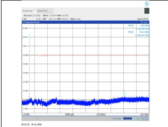
DH5-Ant25-2480-1000~26500-PASS
