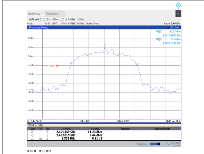
3DH5-Ant25-2402
