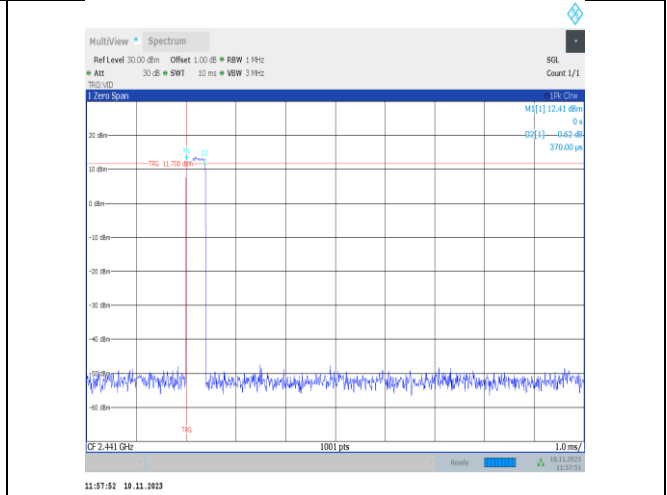
2DH1-Ant25-Hop-PASS
