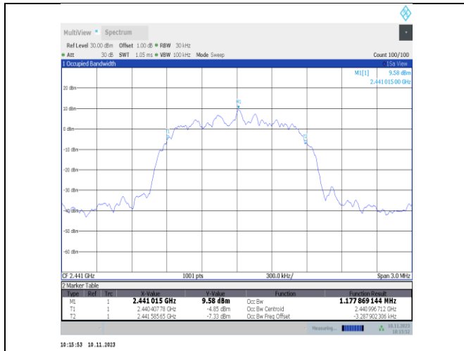
2DH5-Ant25-2441
