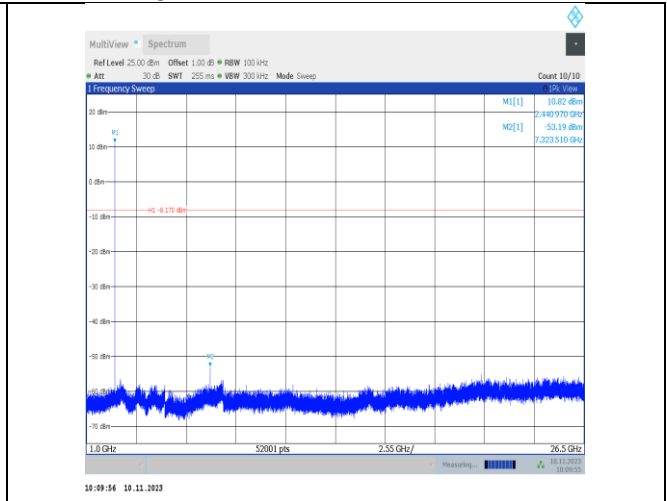
DH5-Ant25-2441-1000~26500-PASS
