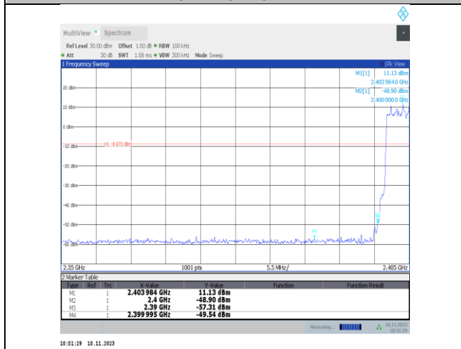
2DH5-Ant25-Hop_2402-PASS
