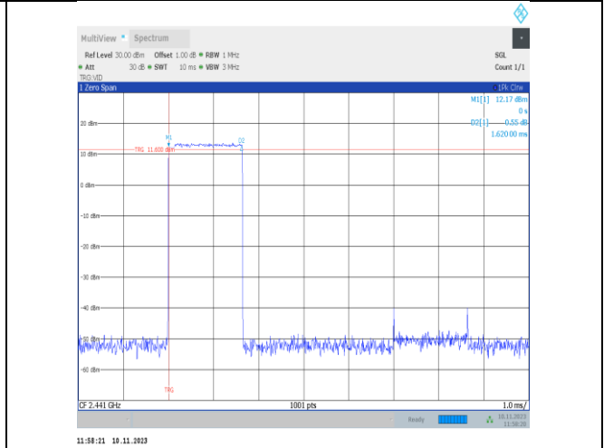
2DH3-Ant25-Hop-PASS
