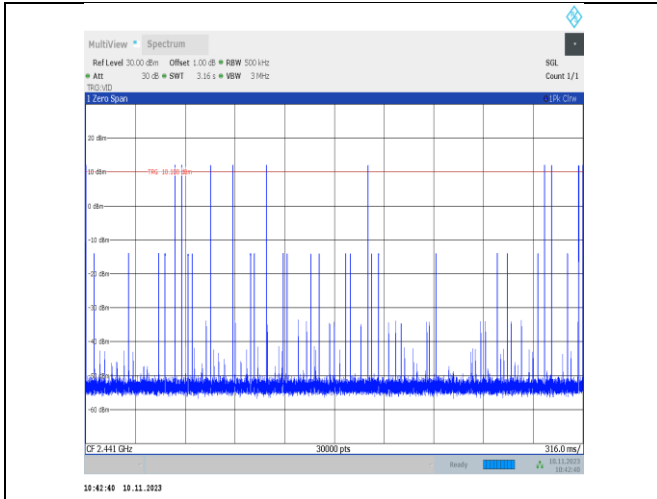
DH5-Ant25-Hop-PASS
