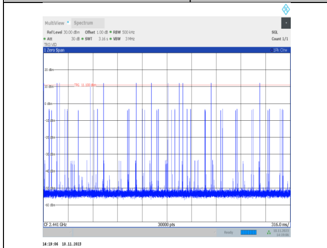
3DH3-Ant25-Hop-PASS
