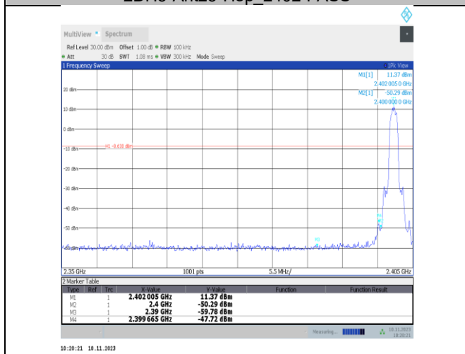
3DH5-Ant25-2402-PASS
