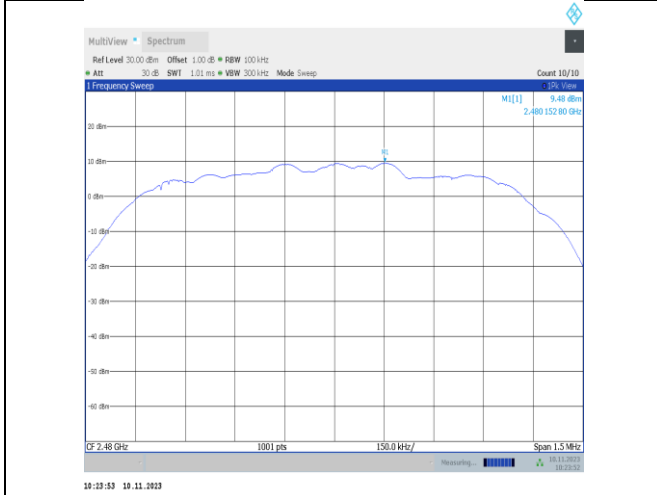
3DH5-Ant25-2480-0~Reference-PASS
