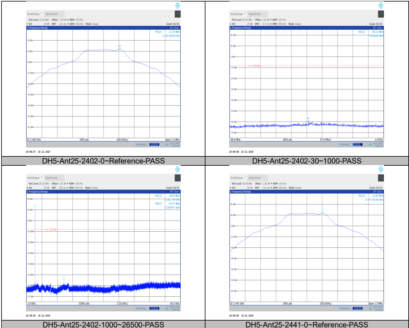
DH5-Ant25-2402-1000~26500-PASS
