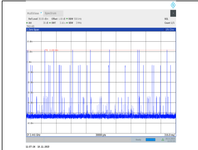
2DH5-Ant25-Hop-PASS
