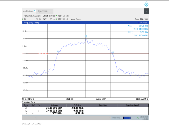
3DH5-Ant25-2441
