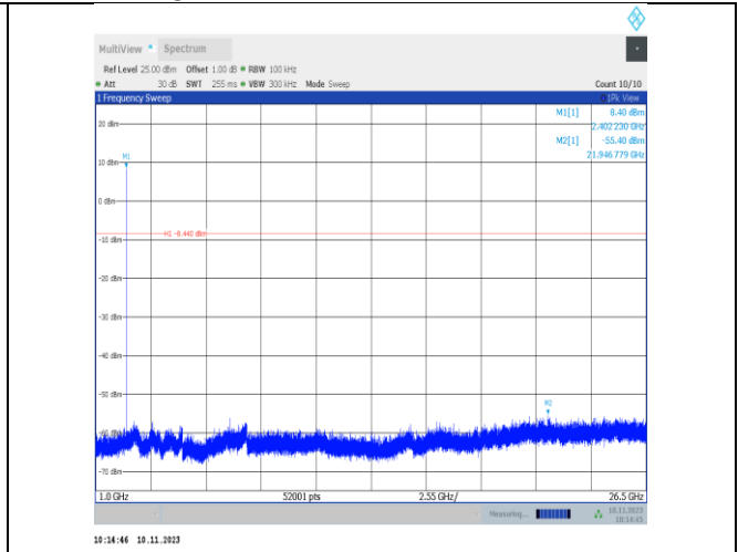
2DH5-Ant25-2402-1000~26500-PASS
