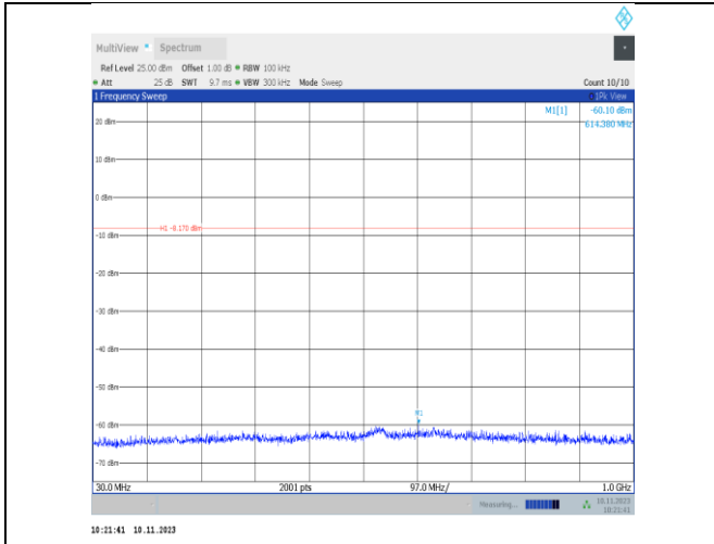
3DH5-Ant25-2441-30~1000-PASS
