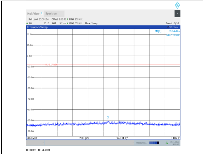
DH5-Ant25-2441-30~1000-PASS
