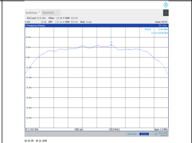
3DH5-Ant25-2441-0~Reference-PASS
