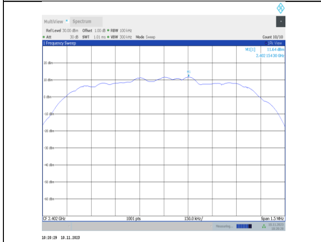
3DH5-Ant25-2402-0~Reference-PASS
