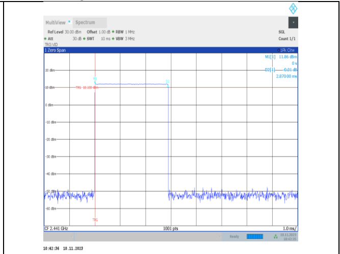
DH5-Ant25-Hop-PASS
