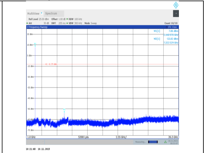
3DH5-Ant25-2441-1000~26500-PASS
