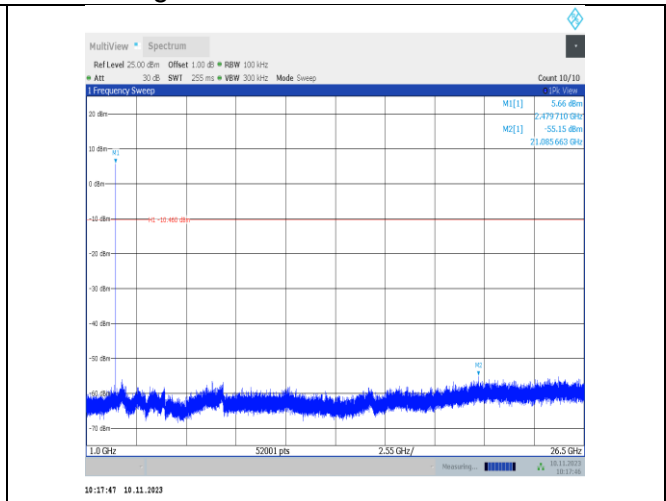
2DH5-Ant25-2480-1000~26500-PASS
