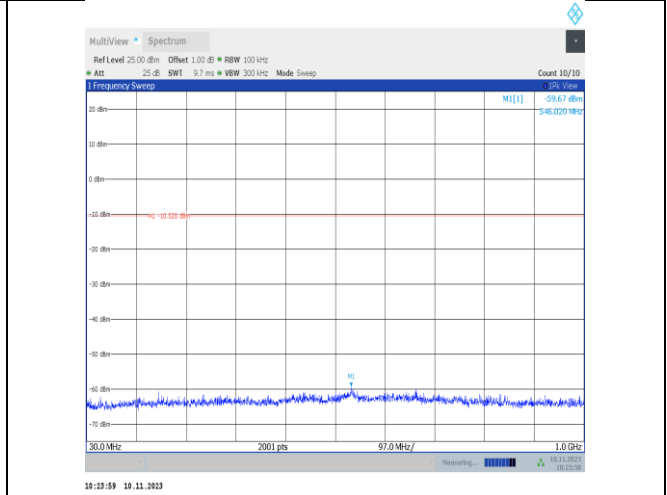
3DH5-Ant25-2480-30~1000-PASS
