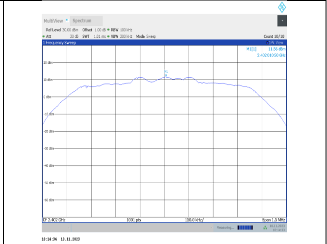
2DH5-Ant25-2402-0~Reference-PASS
