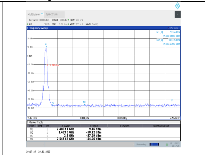
2DH5-Ant25-2480-PASS
