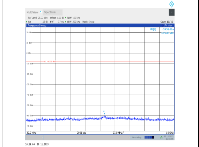
2DH5-Ant25-2441-30~1000-PASS
