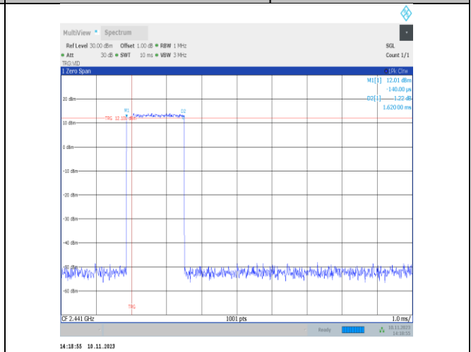
3DH3-Ant25-Hop-PASS
