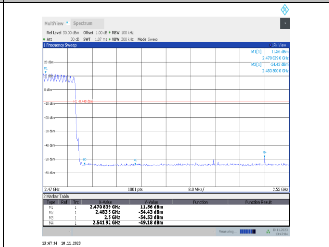
2DH5-Ant25-Hop_2480-PASS
