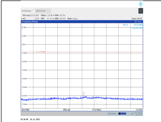
2DH5-Ant25-2402-30~1000-PASS
