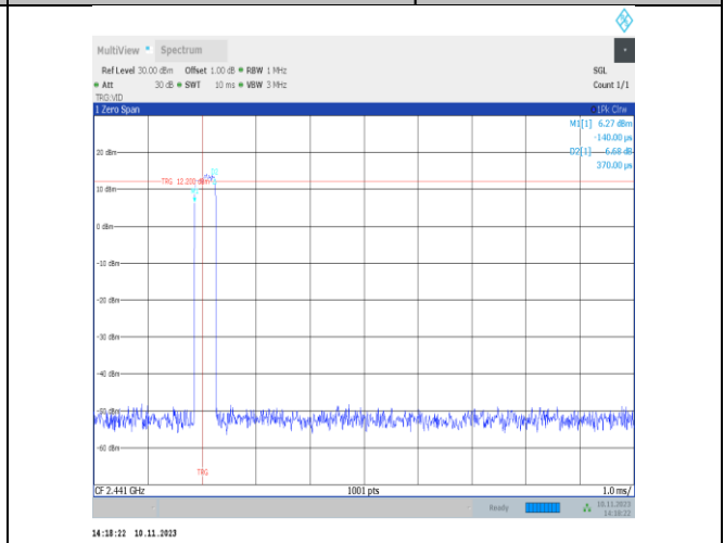
3DH1-Ant25-Hop-PASS
