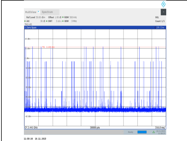
2DH3-Ant25-Hop-PASS
