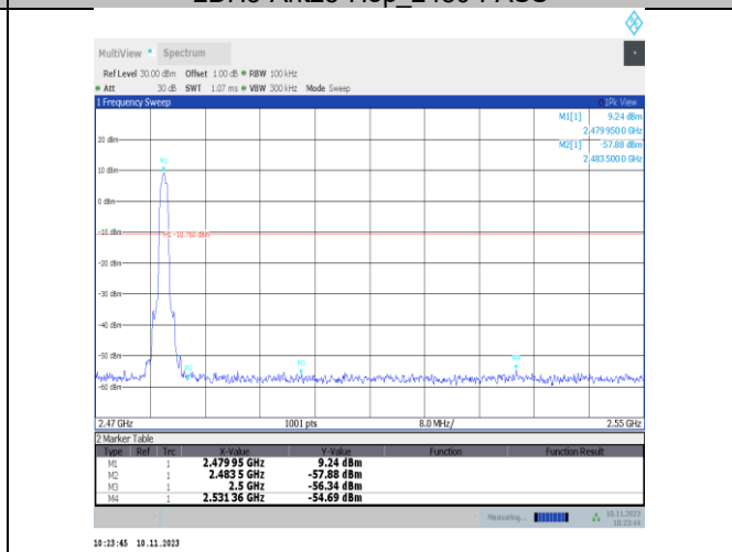
3DH5-Ant25-2480-PASS
