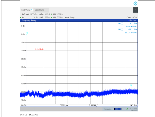
2DH5-Ant25-2441-1000~26500-PASS
