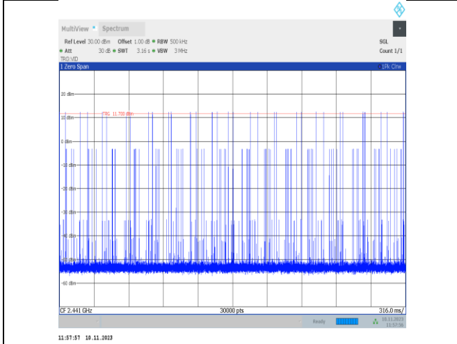
2DH1-Ant25-Hop-PASS
