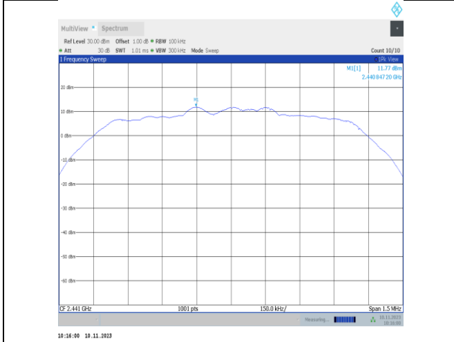
2DH5-Ant25-2441-0~Reference-PASS
