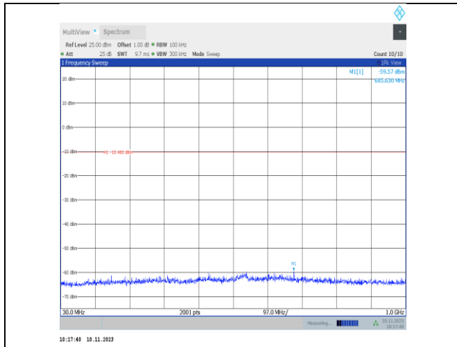
2DH5-Ant25-2480-30~1000-PASS
