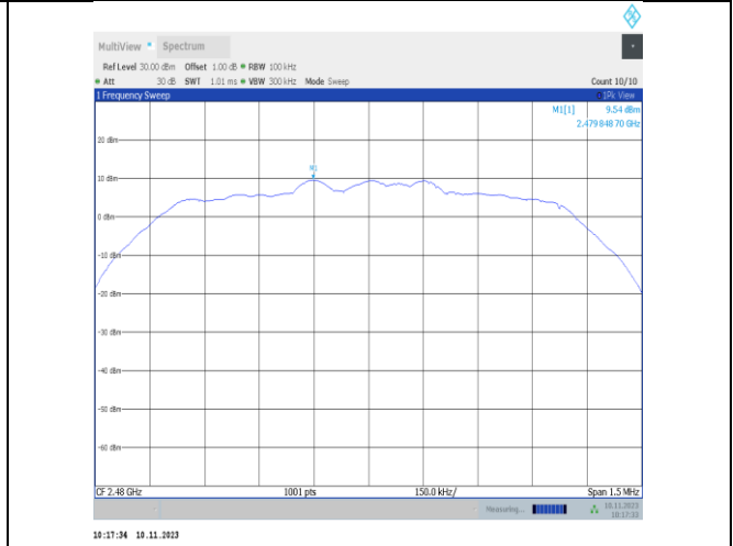
2DH5-Ant25-2480-0~Reference-PASS
