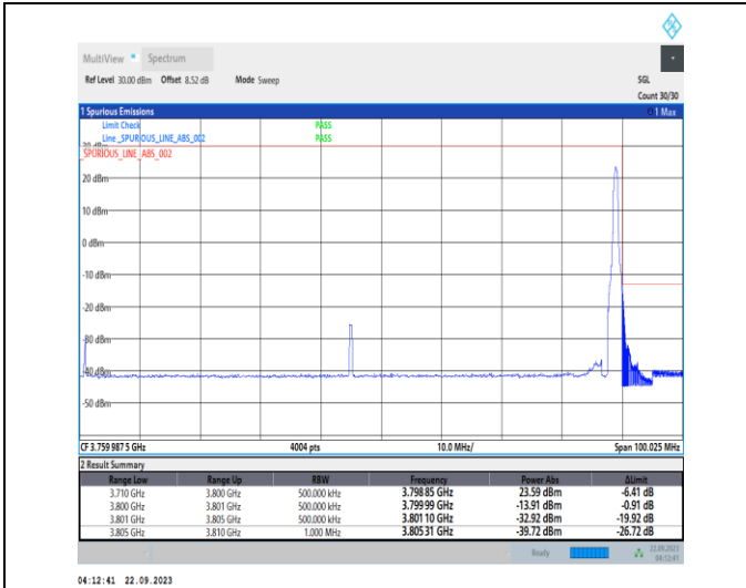
1-N78-3700-3800-PC2-30-90-H-2-DFT-PI2BPSK-Edge_1RB_Right-1@244-Ant12-1--PASS-see graph
