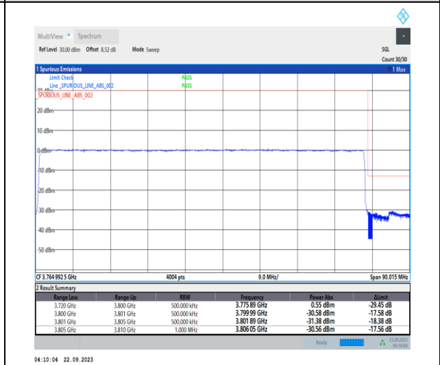
1-N78-3700-3800-PC2-30-80-H-6-CP-QPSK-Outer_Full-217@0-Ant12-1--PASS-see graph
