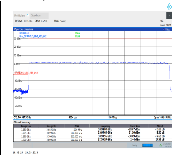
1-N78-3700-3800-PC2-30-100-L-3-DFT-PI2BPSK-Outer_Full-270@0-Ant12-1--PASS-see graph
