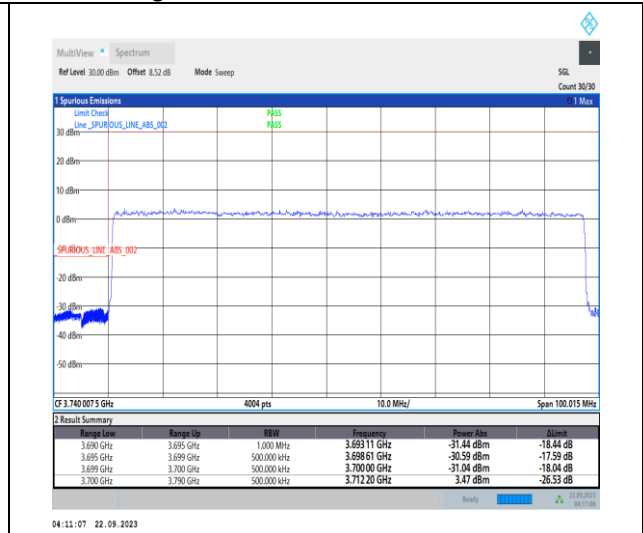
1-N78-3700-3800-PC2-30-90-L-3-DFT-PI2BPSK-Outer_Full-240@0-Ant12-1--PASS-see graph
