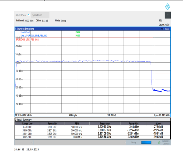
1-N78-3700-3800-PC2-30-80-H-3-DFT-PI2BPSK-Outer_Full-216@0-Ant12-1--PASS-see graph
