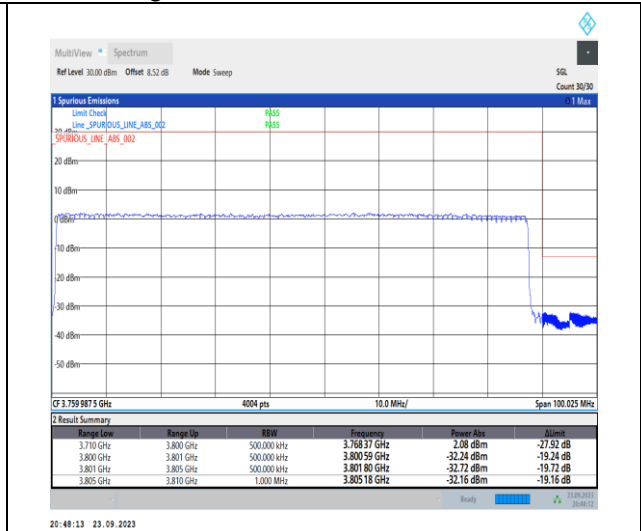
1-N78-3700-3800-PC2-30-90-H-3-DFT-PI2BPSK-Outer_Full-240@0-Ant12-1--PASS-see graph
