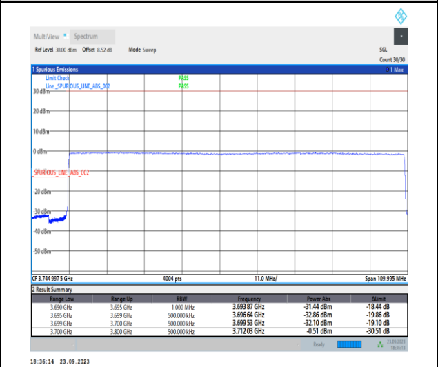
1-N78-3700-3800-PC2-30-100-L-6-CP-QPSK-Outer_Full-273@0-Ant12-1--PASS-see graph
