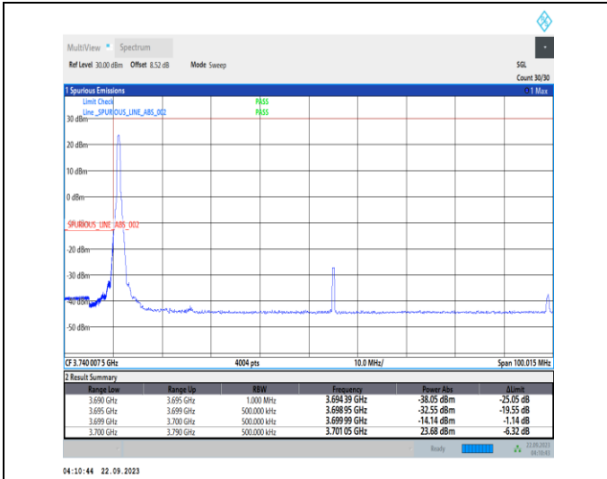
1-N78-3700-3800-PC2-30-90-L-1-DFT-PI2BPSK-Edge_1RB_Left-1@0-Ant12-1--PASS-see graph
