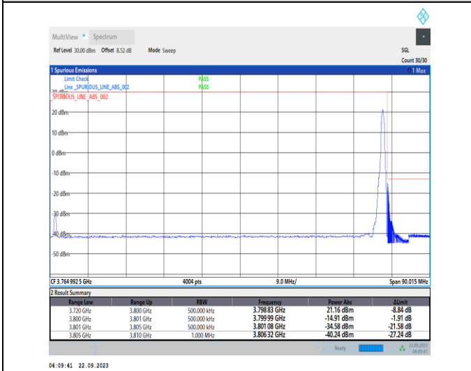
1-N78-3700-3800-PC2-30-80-H-5-CP-QPSK-Edge_1RB_Right-1@216-Ant12-1--PASS-see graph
