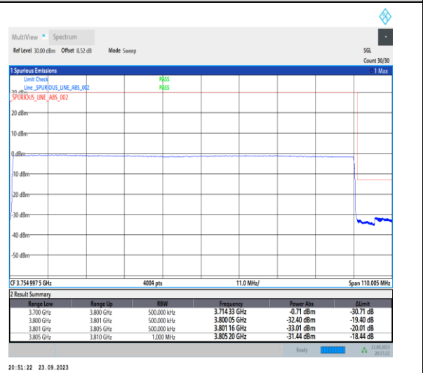
1-N78-3700-3800-PC2-30-100-H-6-CP-QPSK-Outer_Full-273@0-Ant12-1--PASS-see graph
