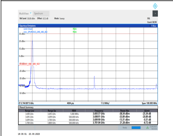
1-N78-3700-3800-PC2-30-100-L-4-CP-QPSK-Edge_1RB_Left-1@0-Ant12-1--PASS-see graph
