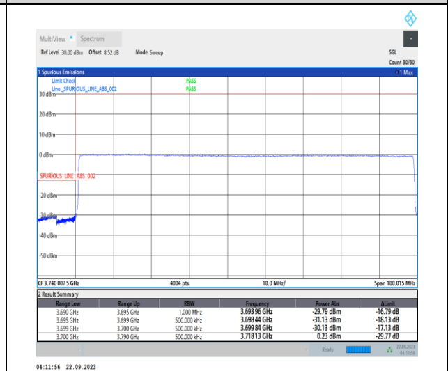
1-N78-3700-3800-PC2-30-90-L-6-CP-QPSK-Outer_Full-245@0-Ant12-1--PASS-see graph
