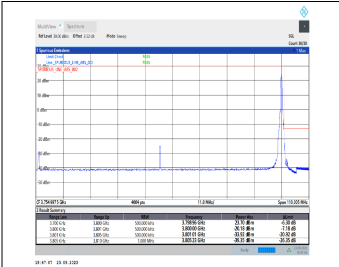
1-N78-3700-3800-PC2-30-100-H-2-DFT-PI2BPSK-Edge_1_RB_Right-1@272-Ant12-1--PASS-see graph
