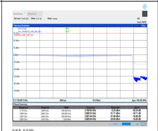
1-N78-3700-3800-PC2-30-90-H-6-CP-QPSK-Outer_Full-245@0-Ant12-1--PASS-see graph
