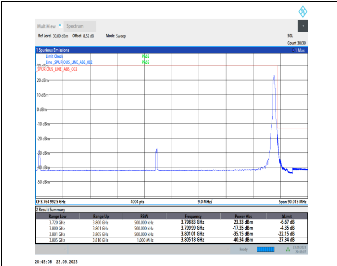
1-N78-3700-3800-PC2-30-80-H-2-DFT-PI2BPSK-Edge_1RB_Right-1@216-Ant12-1--PASS-see graph
