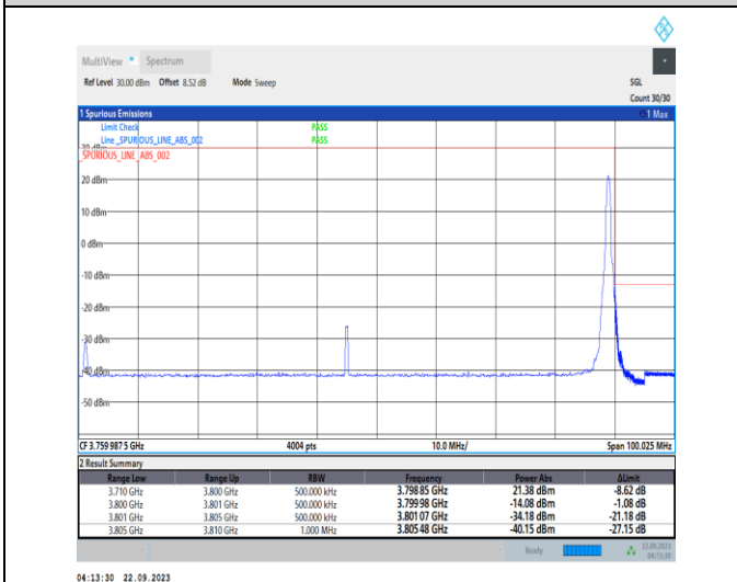
1-N78-3700-3800-PC2-30-90-H-5-CP-QPSK-Edge_1RB_Right-1@244-Ant12-1--PASS-see graph
