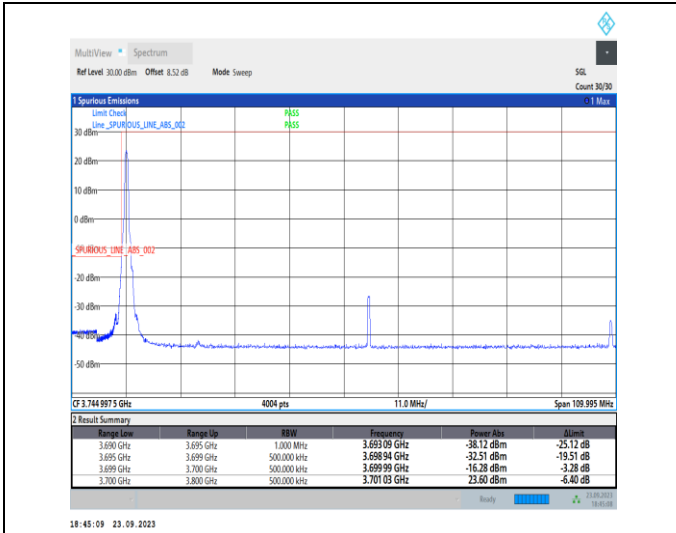
1-N78-3700-3800-PC2-30-100-L-1-DFT-PI2BPSK-Edge_e_1RB_Left-1@0-Ant12-1--PASS-see graph
