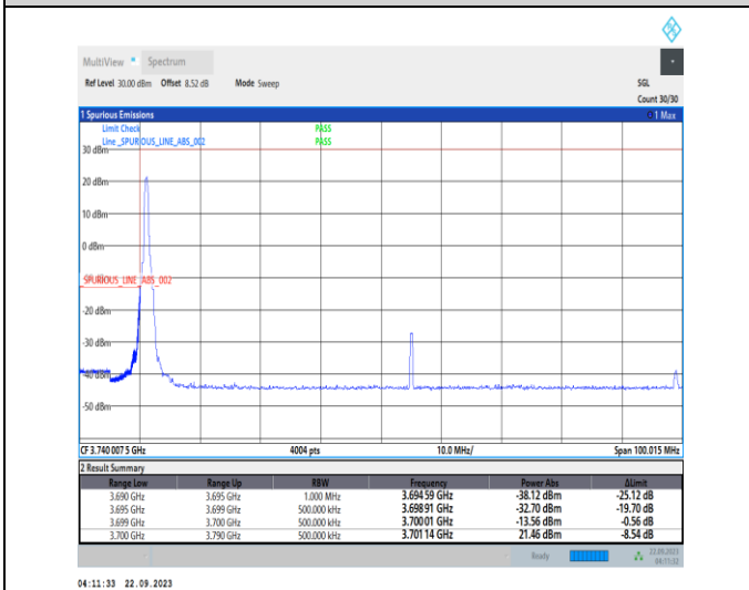
1-N78-3700-3800-PC2-30-90-L-4-CP-QPSK-Edge_1RB_Left-1@0-Ant12-1--PASS-see graph
