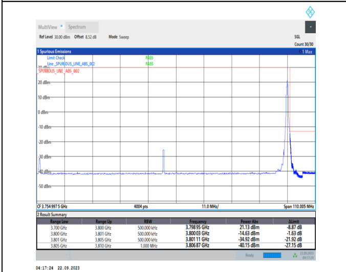
1-N78-3700-3800-PC2-30-100-H-5-CP-QPSK-Edge_1_RB_Right-1@272-Ant12-1--PASS-see graph
