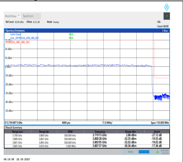
1-N78-3700-3800-PC2-30-100-H-3-DFT-PI2BPSK-Outer_Full-270@0-Ant12-1--PASS-see graph
