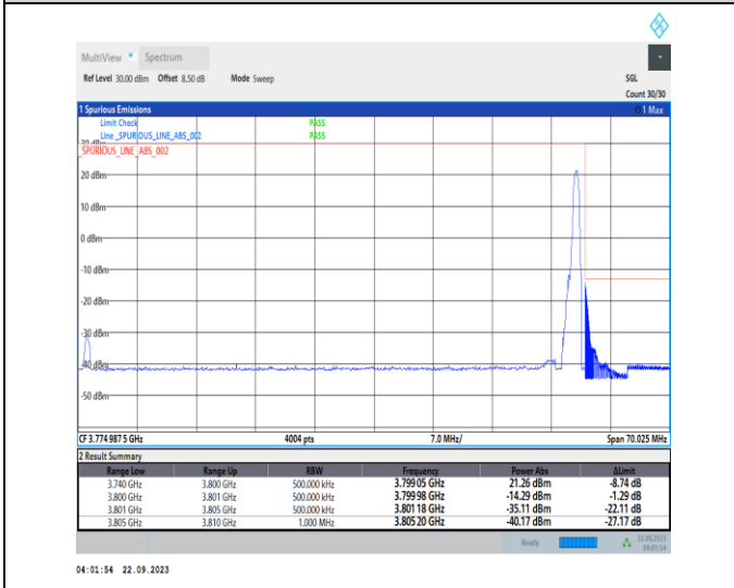
1-N78-3700-3800-PC2-30-60-H-5-CP-QPSK-Edge_1RB_Right-1@161-Ant12-1--PASS-see graph
