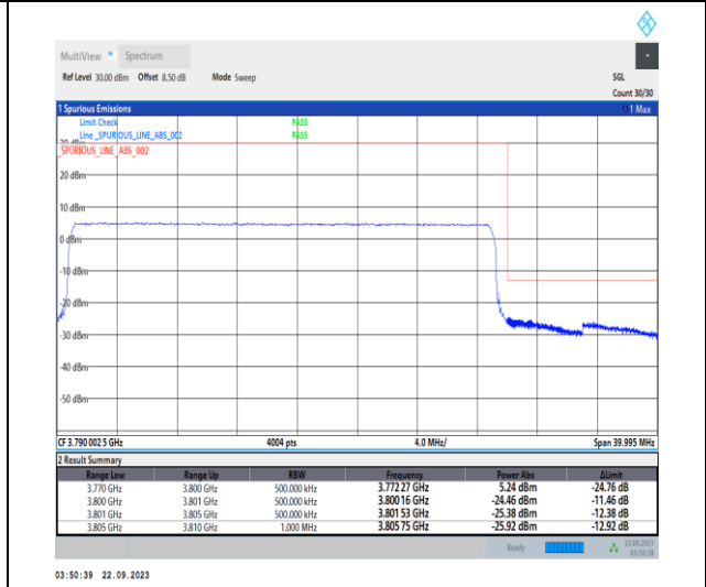
1-N78-3700-3800-PC2-30-30-H-6-CP-QPSK-Outer_Full-78@0-Ant12-1--PASS-see graph
