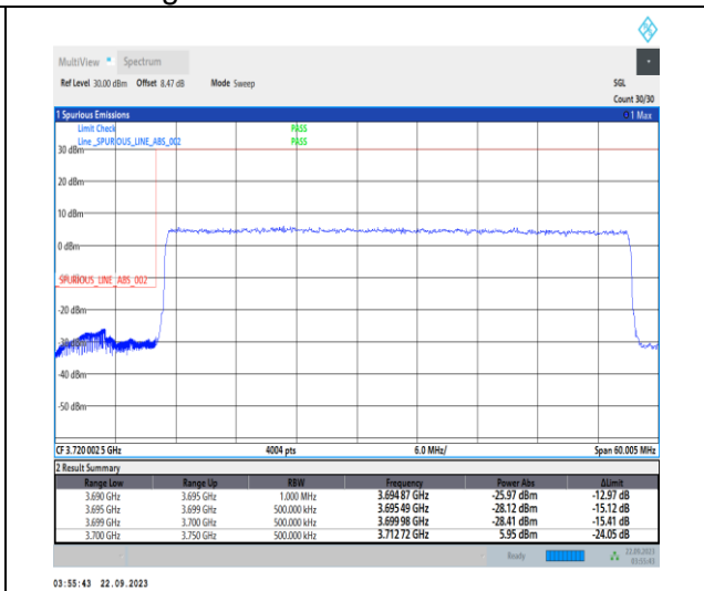
1-N78-3700-3800-PC2-30-50-L-3-DFT-PI2BPSK-Outer_Full-128@0-Ant12-1--PASS-see graph
