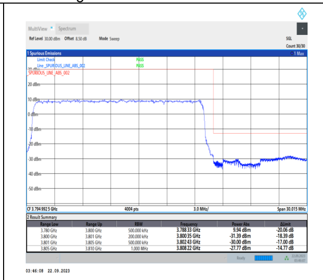
1-N78-3700-3800-PC2-30-20-H-3-DFT-PI2BPSK-Outer_Full-50@0-Ant12-1--PASS-see graph
