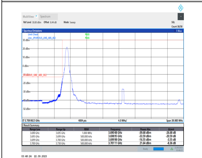
1-N78-3700-3800-PC2-30-30-L-4-CP-QPSK-Edge_1RB_Left-1@0-Ant12-1--PASS-see graph
