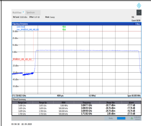
1-N78-3700-3800-PC2-30-50-L-6-CP-QPSK-Outer_Full-133@0-Ant12-1--PASS-see graph
