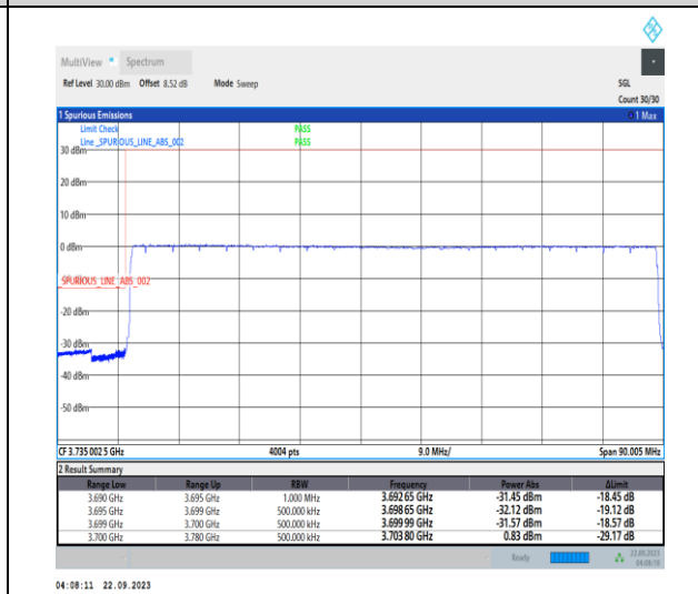
1-N78-3700-3800-PC2-30-80-L-6-CP-QPSK-Outer_Full-217@0-Ant12-1--PASS-see graph
