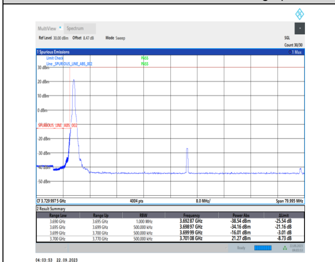
1-N78-3700-3800-PC2-30-70-L-4-CP-QPSK-Edge_1RB_Left-1@0-Ant12-1--PASS-see graph
