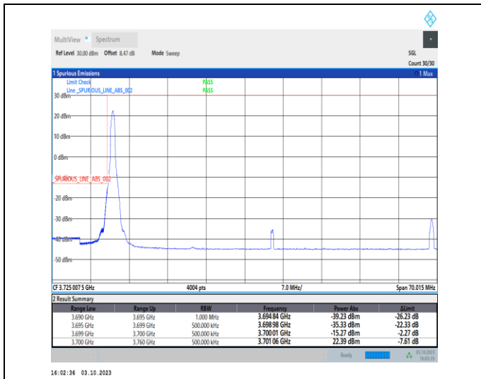
1-N78-3700-3800-PC2-30-60-L-1-DFT-PI2BPSK-Edge_1RB_Left-1@0-Ant12-1--PASS-see graph
