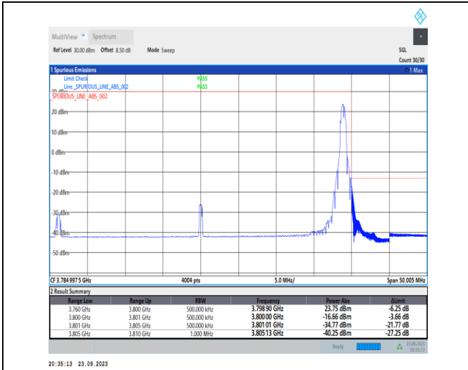
1-N78-3700-3800-PC2-30-40-H-2-DFT-PI2BPSK-Edge_1RB_Right-1@105-Ant12-1--PASS-see graph
