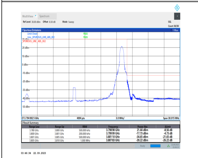
1-N78-3700-3800-PC2-30-20-H-5-CP-QPSK-Edge_1RB_Right-1@50-Ant12-1--PASS-see graph
