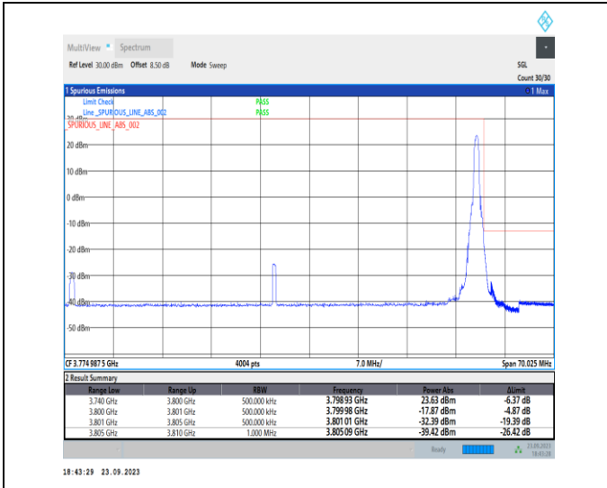
1-N78-3700-3800-PC2-30-60-H-2-DFT-PI2BPSK-Edge_1RB_Right-1@161-Ant12-1--PASS-see graph
