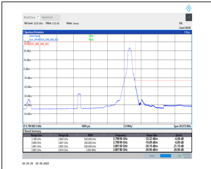
1-N78-3700-3800-PC2-30-20-H-2-DFT-PI2BPSK-Edge_1RB_Right-1@50-Ant12-1--PASS-see graph
