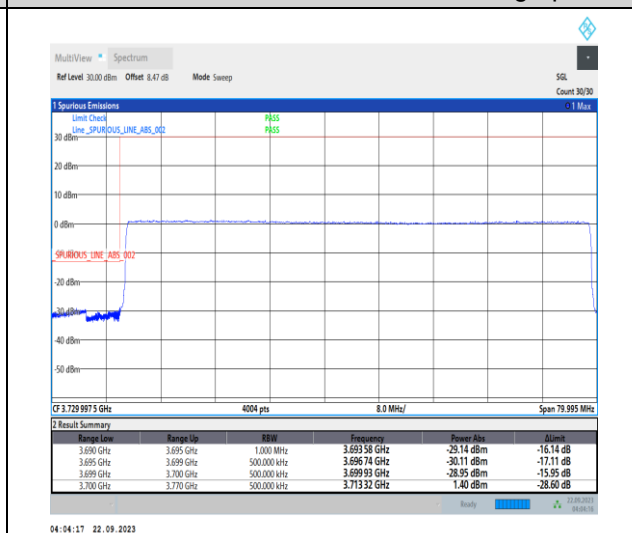
1-N78-3700-3800-PC2-30-70-L-6-CP-QPSK-Outer_Full-189@0-Ant12-1--PASS-see graph
