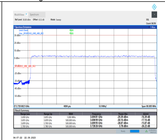
1-N78-3700-3800-PC2-30-80-L-3-DFT-PI2BPSK-Outer_Full-216@0-Ant12-1--PASS-see graph
