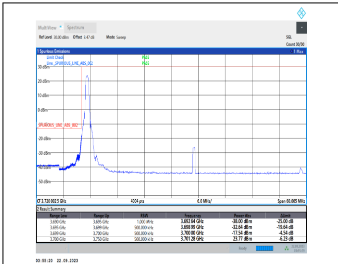
1-N78-3700-3800-PC2-30-50-L-1-DFT-PI2BPSK-Edge_1RB_Left-1@0-Ant12-1--PASS-see graph
