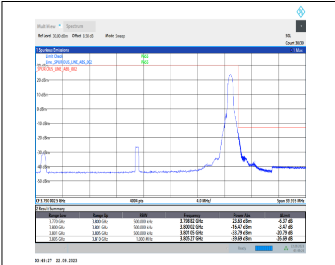
1-N78-3700-3800-PC2-30-30-H-2-DFT-PI2BPSK-Edge_1RB_Right-1@77-Ant12-1--PASS-see graph
