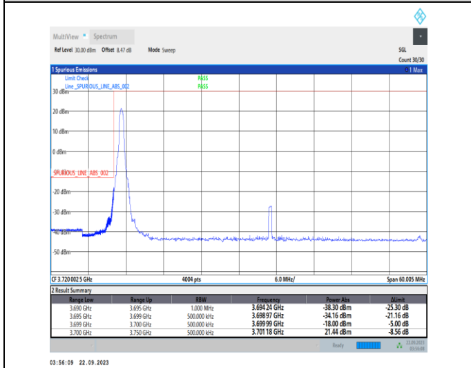
1-N78-3700-3800-PC2-30-50-L-4-CP-QPSK-Edge_1RB_Left-1@0-Ant12-1--PASS-see graph
