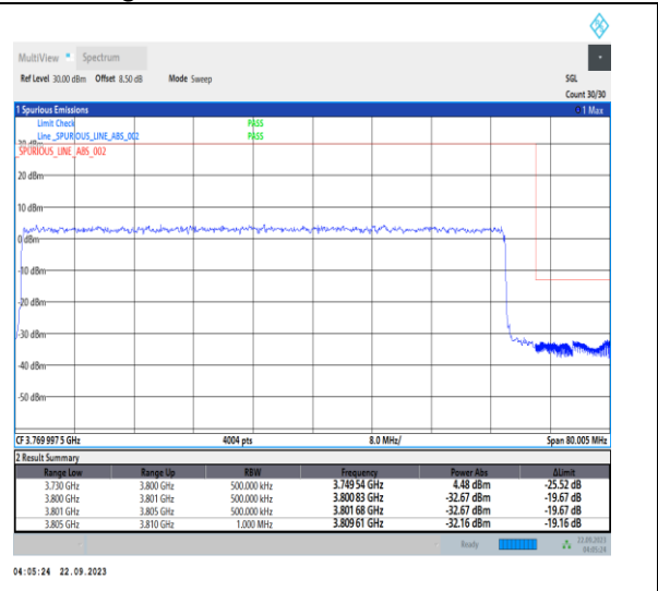
1-N78-3700-3800-PC2-30-70-H-3-DFT-PI2BPSK-Outer_Full-180@0-Ant12-1--PASS-see graph
