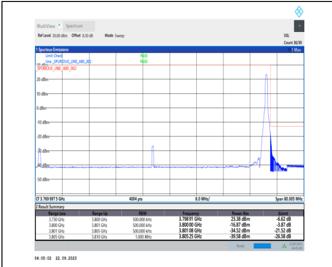
1-N78-3700-3800-PC2-30-70-H-2-DFT-PI2BPSK-Edge_1RB_Right-1@188-Ant12-1--PASS-see graph
