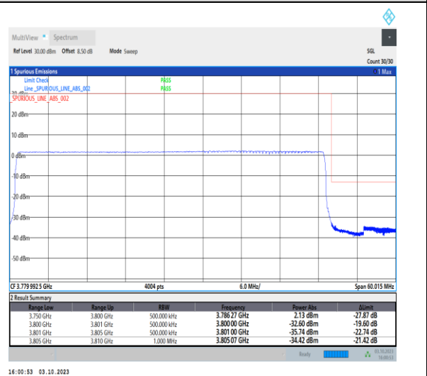
1-N78-3700-3800-PC2-30-50-H-6-CP-QPSK-Outer_Full-133@0-Ant12-1--PASS-see graph
