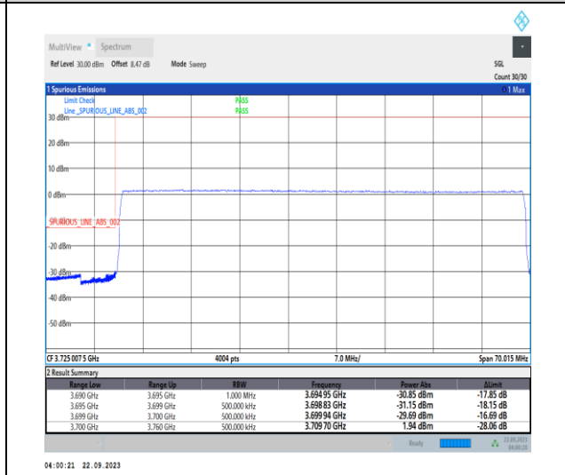
1-N78-3700-3800-PC2-30-60-L-6-CP-QPSK-Outer_Full-162@0-Ant12-1--PASS-see graph
