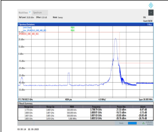
1-N78-3700-3800-PC2-30-30-H-5-CP-QPSK-Edge_1RB_Right-1@77-Ant12-1--PASS-see graph
