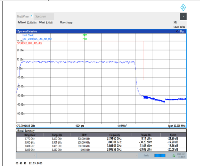
1-N78-3700-3800-PC2-30-30-H-3-DFT-PI2BPSK-Outer_Full-75@0-Ant12-1--PASS-see graph
