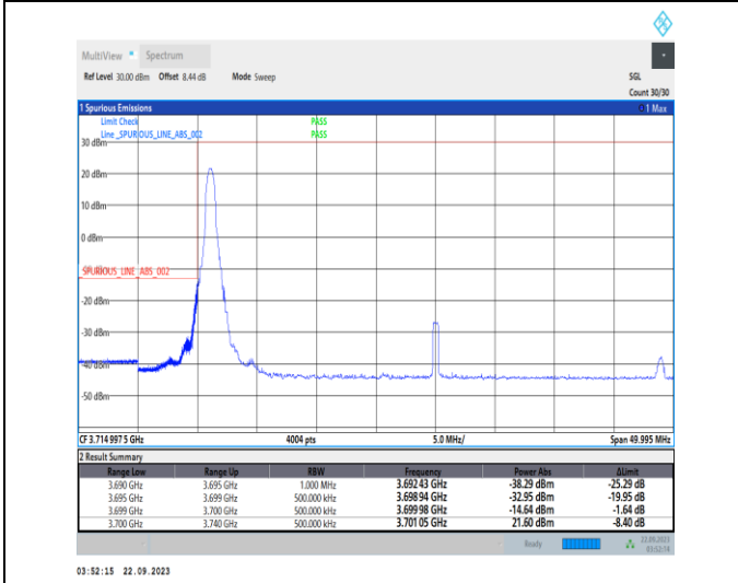
1-N78-3700-3800-PC2-30-40-L-4-CP-QPSK-Edge_1RB_Left-1@0-Ant12-1--PASS-see graph
