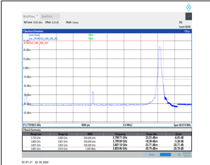
1-N78-3700-3800-PC2-30-50-H-2-DFT-PI2BPSK-Edge_1RB_Right-1@132-Ant12-1--PASS-see graph
