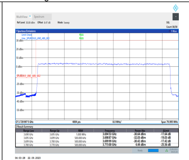
1-N78-3700-3800-PC2-30-70-L-3-DFT-PI2BPSK-Outer_Full-180@0-Ant12-1--PASS-see graph
