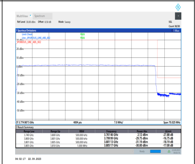
1-N78-3700-3800-PC2-30-60-H-6-CP-QPSK-Outer_Full-162@0-Ant12-1--PASS-see graph
