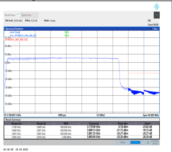
1-N78-3700-3800-PC2-30-40-H-3-DFT-PI2BPSK-Outer_Full-100@0-Ant12-1--PASS-see graph
