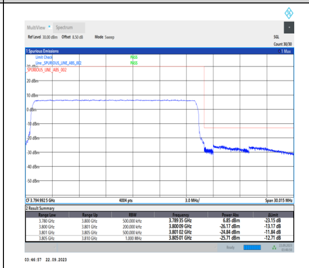
1-N78-3700-3800-PC2-30-20-H-6-CP-QPSK-Outer_Full-51@0-Ant12-1--PASS-see graph
