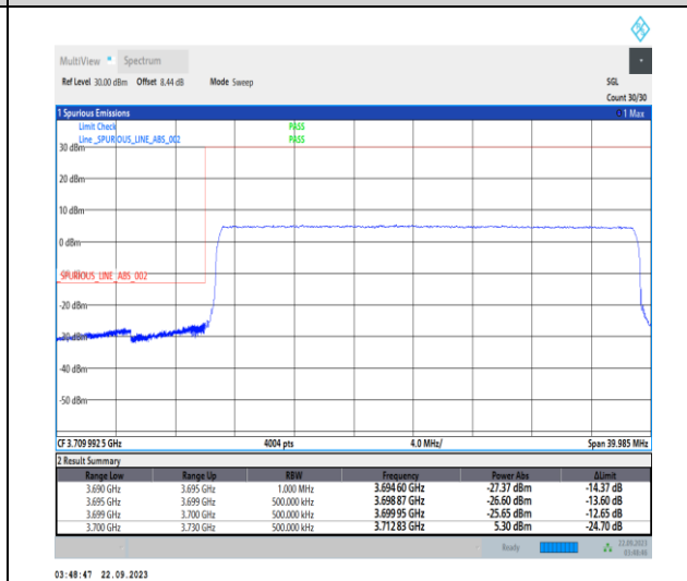
1-N78-3700-3800-PC2-30-30-L-6-CP-QPSK-Outer_Full-78@0-Ant12-1--PASS-see graph
