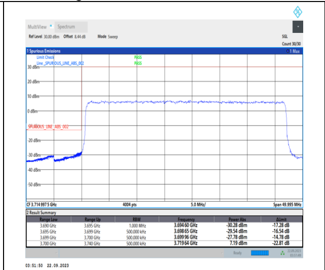
1-N78-3700-3800-PC2-30-40-L-3-DFT-PI2BPSK-Outer_Full-100@0-Ant12-1--PASS-see graph
