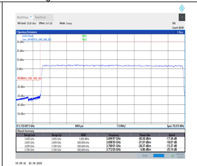
1-N78-3700-3800-PC2-30-60-L-3-DFT-PI2BPSK-Outer_Full-162@0-Ant12-1--PASS-see graph
