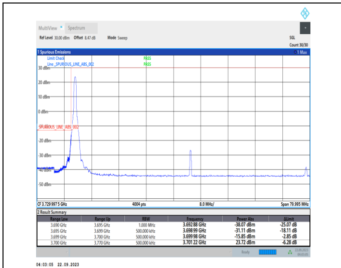
1-N78-3700-3800-PC2-30-70-L-1-DFT-PI2BPSK-Edge_1RB_Left-1@0-Ant12-1--PASS-see graph
