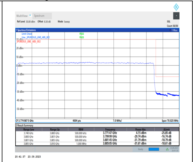
1-N78-3700-3800-PC2-30-60-H-3-DFT-PI2BPSK-Outer_Full-162@0-Ant12-1--PASS-see graph
