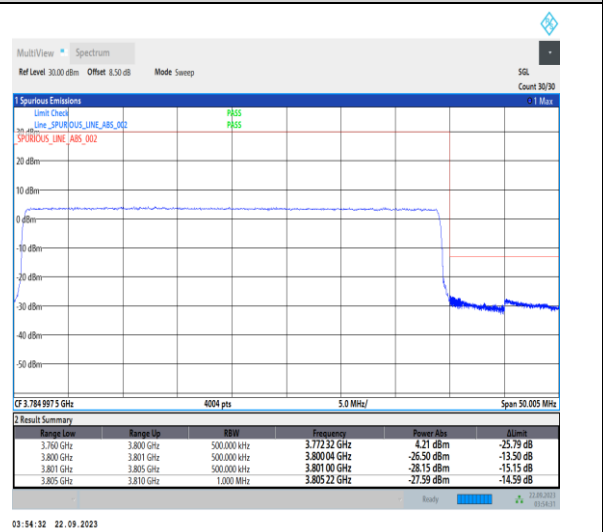
1-N78-3700-3800-PC2-30-40-H-6-CP-QPSK-Outer_Full-106@0-Ant12-1--PASS-see graph
