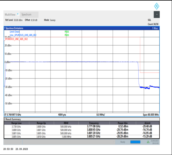
1-N78-3700-3800-PC2-30-70-H-6-CP-QPSK-Outer_Full-189@0-Ant12-1--PASS-see graph
