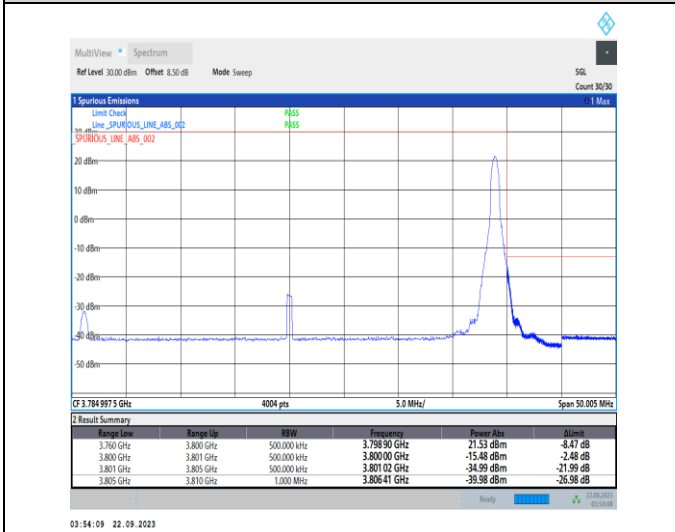
1-N78-3700-3800-PC2-30-40-H-5-CP-QPSK-Edge_1RB_Right-1@105-Ant12-1--PASS-see graph
