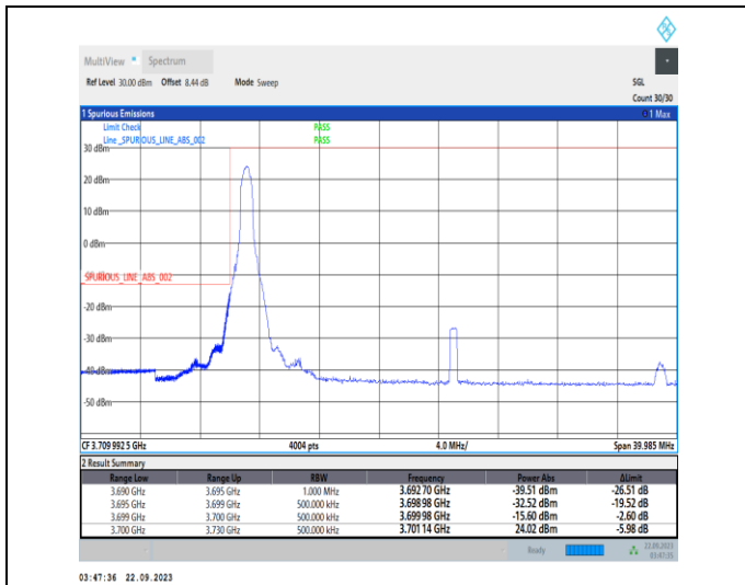
1-N78-3700-3800-PC2-30-30-L-1-DFT-PI2BPSK-Edge_1RB_Left-1@0-Ant12-1--PASS-see graph
