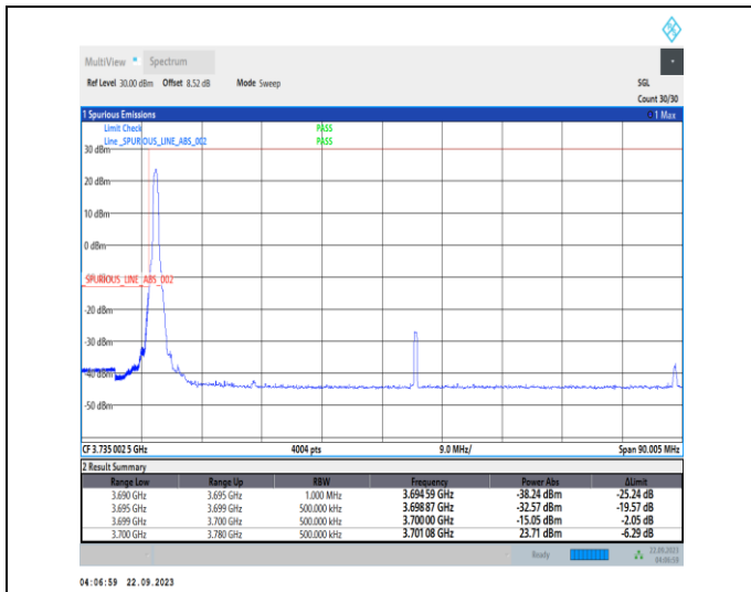
1-N78-3700-3800-PC2-30-80-L-1-DFT-PI2BPSK-Edge_1RB_Left-1@0-Ant12-1--PASS-see graph
