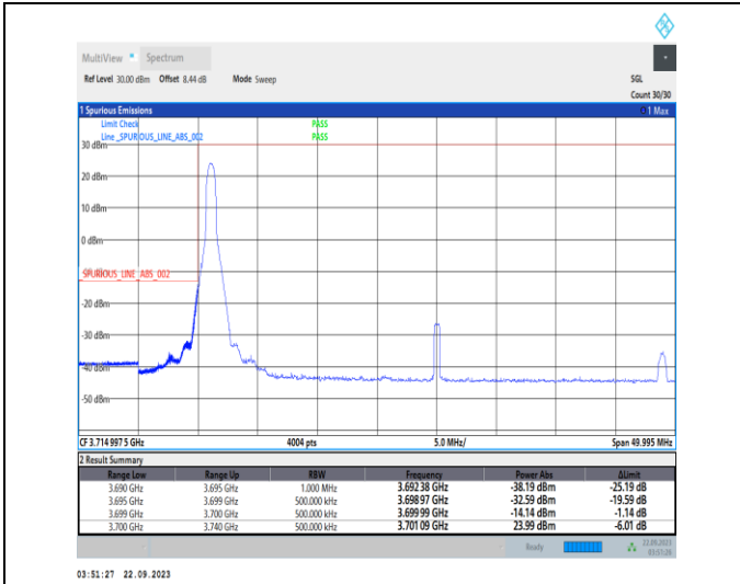
1-N78-3700-3800-PC2-30-40-L-1-DFT-PI2BPSK-Edge_1RB_Left-1@0-Ant12-1--PASS-see graph
