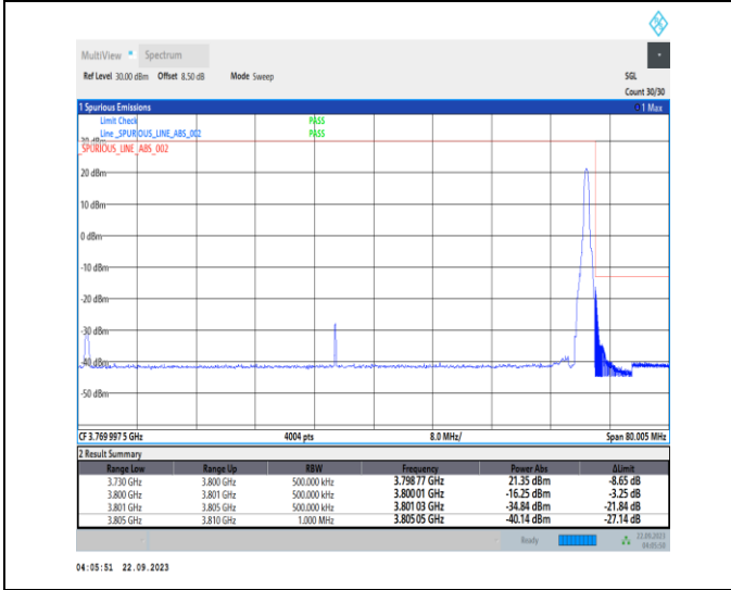
1-N78-3700-3800-PC2-30-70-H-5-CP-QPSK-Edge_1RB_Right-1@188-Ant12-1--PASS-see graph
