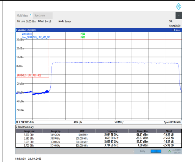
1-N78-3700-3800-PC2-30-40-L-6-CP-QPSK-Outer_Full-106@0-Ant12-1--PASS-see graph
