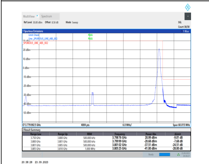
1-N78-3700-3800-PC2-30-50-H-5-CP-QPSK-Edge_1RB_Right-1@132-Ant12-1--PASS-see graph
