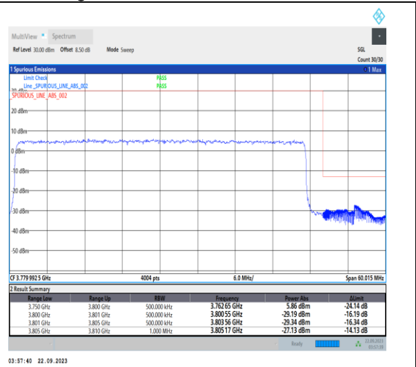
1-N78-3700-3800-PC2-30-50-H-3-DFT-PI2BPSK-Outer_Full-128@0-Ant12-1--PASS-see graph
