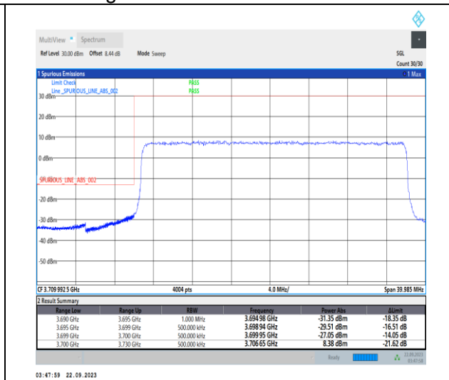
1-N78-3700-3800-PC2-30-30-L-3-DFT-PI2BPSK-Outer_Full-75@0-Ant12-1--PASS-see graph
