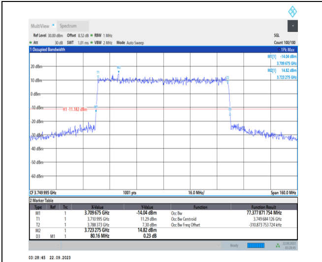
1-N78-3700-3800-PC2-30-80-M-3-DFT-16QAM-Out er_Full-216@0-Ant12-77.378-80.160-≤80-PASS
