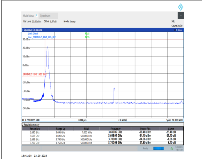
1-N78-3700-3800-PC2-30-60-L-4-CP-QPSK-Edge_1RB_Left-1@0-Ant12-1--PASS-see graph
