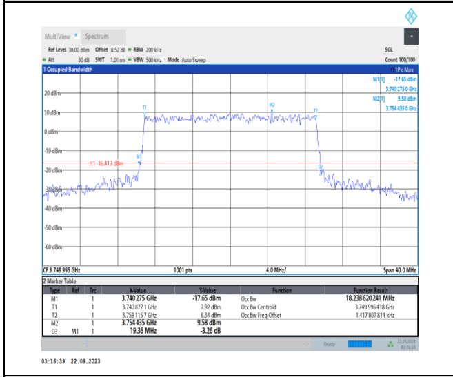
1-N78-3700-3800-PC2-30-20-M-7-CP-16QAM-Outer_Full-51@0-Ant12-18.239-19.360-≤20-PASS
