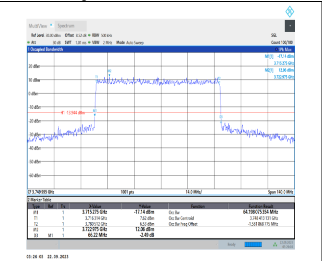
1-N78-3700-3800-PC2-30-70-M-1-DFT-QPSK-Outer_Full-180@0-Ant12-64.198-66.220-≤70-PASS
