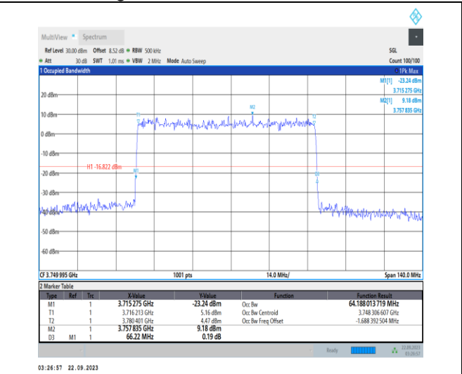
1-N78-3700-3800-PC2-30-70-M-5-DFT-256QAM-Out er_Full-180@0-Ant12-64.188-66.220-≤70-PASS
