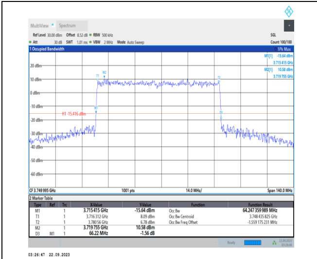
1-N78-3700-3800-PC2-30-70-M-4-DFT-64QAM-Out er_Full-180@0-Ant12-64.247-66.220-≤70-PASS
