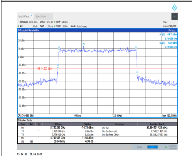
1-N78-3700-3800-PC2-30-60-M-3-DFT-16QAM-Outer_Full-162@0-Ant12-57.864-59.640-≤60-PASS
