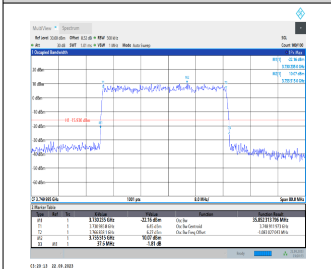
1-N78-3700-3800-PC2-30-40-M-5-DFT-256QAM-Outer_Full-100@0-Ant12-35.852-37.600-≤40-PASS
