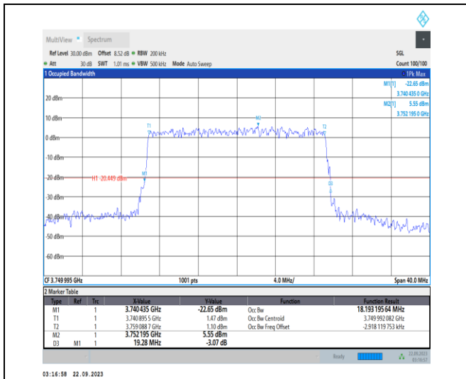
1-N78-3700-3800-PC2-30-20-M-9-CP-256QAM-Out er_Full-51@0-Ant12-18.193-19.280-≤20-PASS
