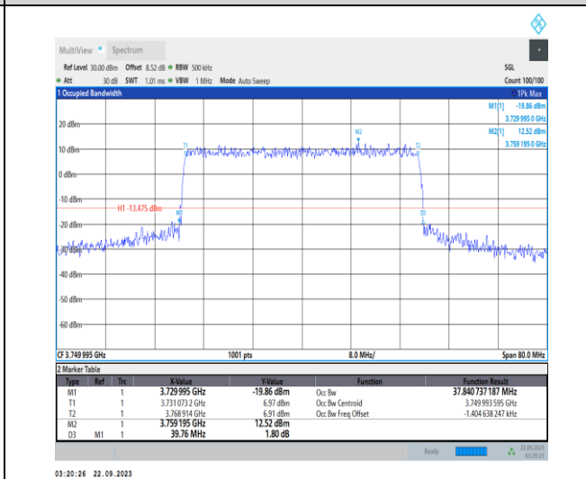
1-N78-3700-3800-PC2-30-40-M-6-CP-QPSK-Outer_Full-106@0-Ant12-37.841-39.760-≤40-PASS
