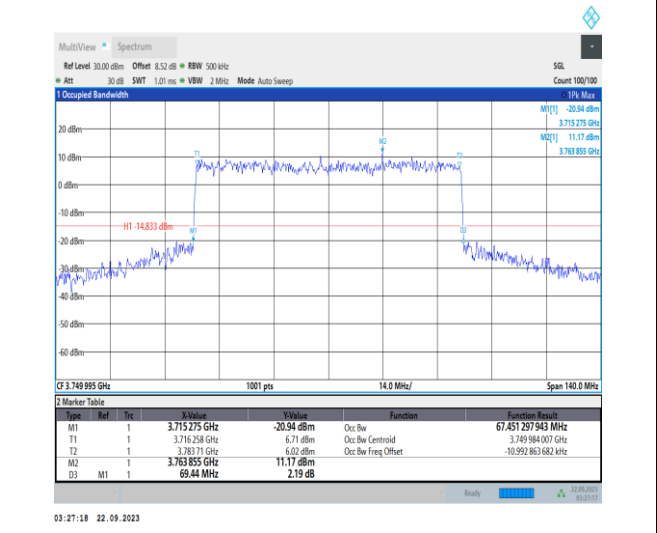
1-N78-3700-3800-PC2-30-70-M-7-CP-16QAM-Outer Full-189@0-Ant12-67.451-69.440-≤70-PASS
