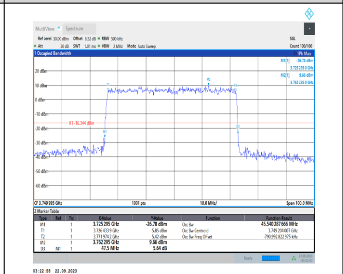
1-N78-3700-3800-PC2-30-50-M-5-DFT-256QAM-Outer_Full-128@0-Ant12-45.54-47.500-≤50-PASS
