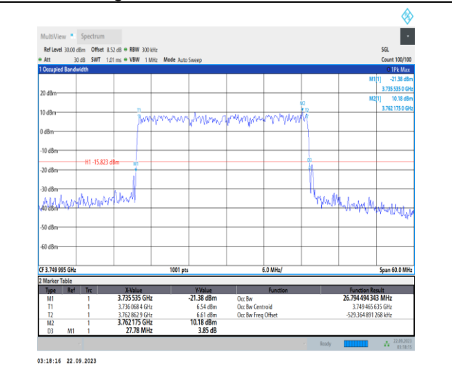
1-N78-3700-3800-PC2-30-30-M-5-DFT-256QAM-Out er_Full-75@0-Ant12-26.794-27.780-≤30-PASS
