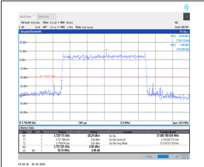
1-N78-3700-3800-PC2-30-60-M-9-CP-256QAM-Out er_Full-162@0-Ant12-57.686-59.760-≤60-PASS
