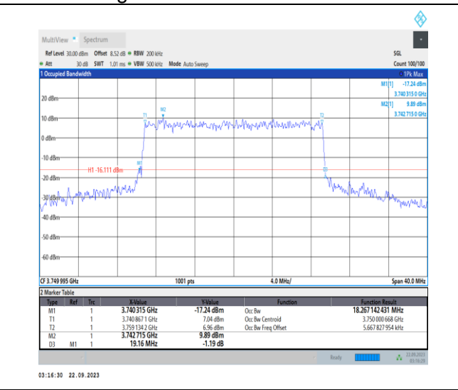
1-N78-3700-3800-PC2-30-20-M-6-CP-QPSK-Outer_Full-51@0-Ant12-18.267-19.160-≤20-PASS
