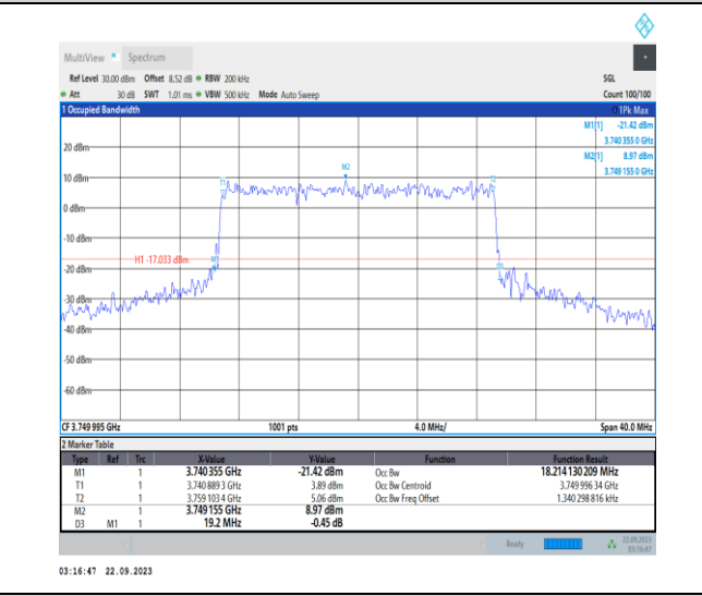
1-N78-3700-3800-PC2-30-20-M-8-CP-64QAM-Outer_Full-51@0-Ant12-18.214-19.200-≤20-PASS
