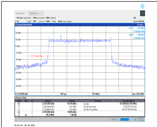
1-N78-3700-3800-PC2-30-50-M-6-CP-QPSK-Outer_Full-133@0-Ant12-47.46-49.200-≤50-PASS
