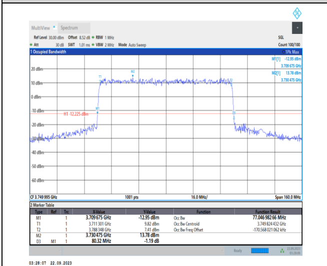
1-N78-3700-3800-PC2-30-80-M-1-DFT-QPSK-Outer_Full-216@0-Ant12-77.047-80.320-≤80-PASS
