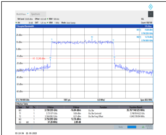
1-N78-3700-3800-PC2-30-40-M-3-DFT-16QAM-Out er_Full-100@0-Ant12-35.767-37.280-≤40-PASS
