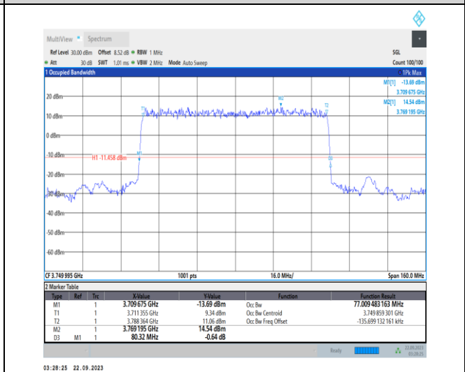
1-N78-3700-3800-PC2-30-80-M-2-DFT-PI2BPSK-Outer_Full-216@0-Ant12-77.009-80.320-≤80-PASS
