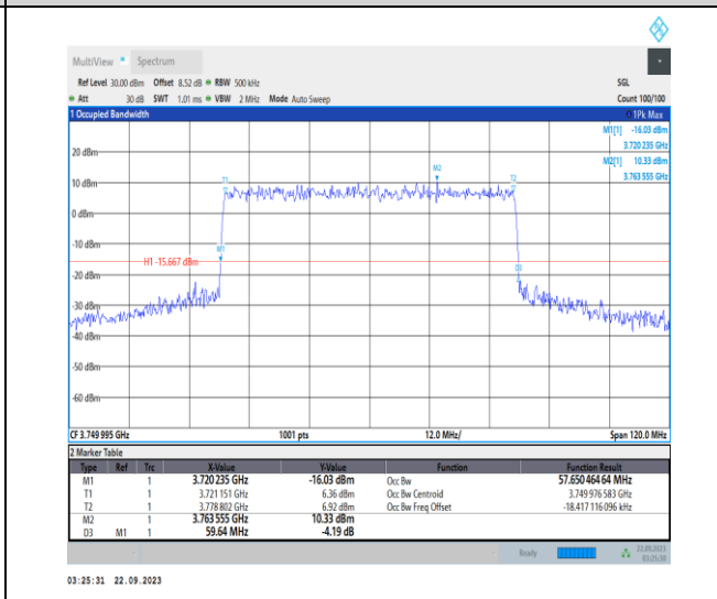
1-N78-3700-3800-PC2-30-60-M-8-CP-64QAM-Outer_Full-162@0-Ant12-57.65-59.640-≤60-PASS
