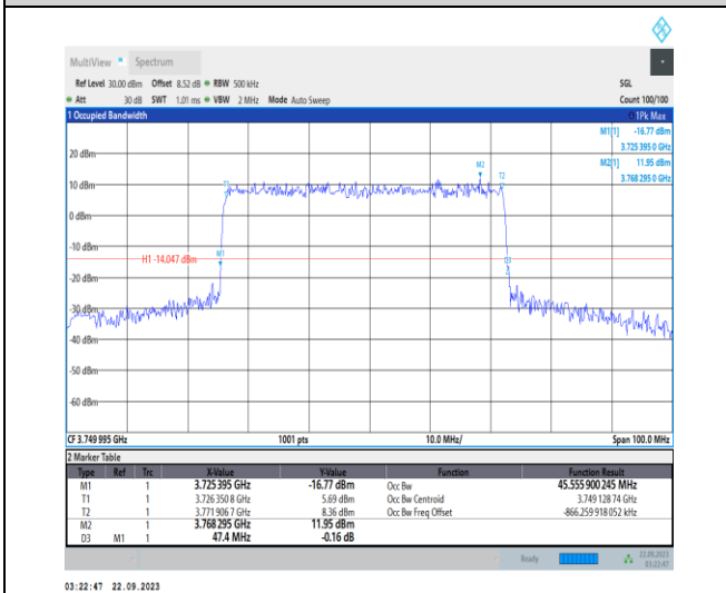
1-N78-3700-3800-PC2-30-50-M-4-DFT-64QAM-Outer_Full-128@0-Ant12-45.556-47.400-≤50-PASS
