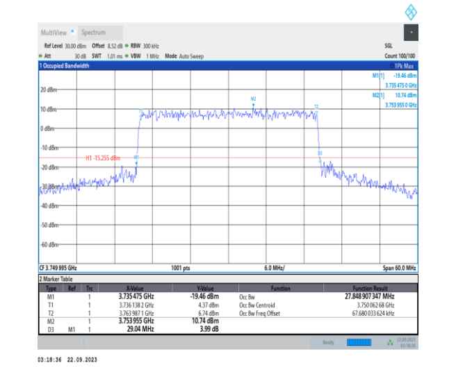
1-N78-3700-3800-PC2-30-30-M-7-CP-16QAM-Outer_Full-78@0-Ant12-27.849-29.040-≤30-PASS
