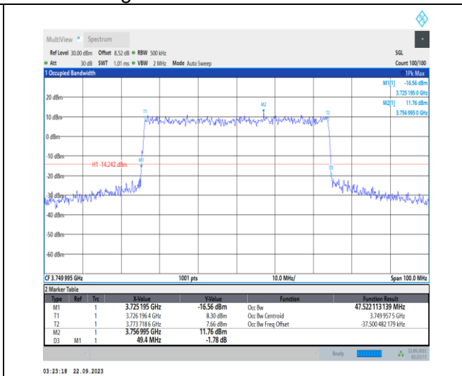
1-N78-3700-3800-PC2-30-50-M-7-CP-16QAM-Outer_Full-133@0-Ant12-47.522-49.400-≤50-PASS
