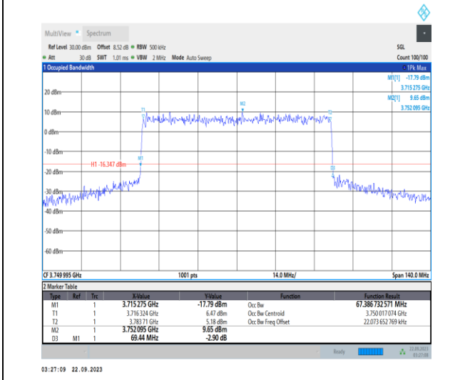
1-N78-3700-3800-PC2-30-70-M-6-CP-QPSK-Outer Full-189@0-Ant12-67.387-69.440-≤70-PASS
