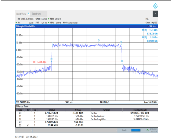
1-N78-3700-3800-PC2-30-70-M-8-CP-64QAM-Outer_Full-189@0-Ant12-67.505-69.440-≤70-PASS
