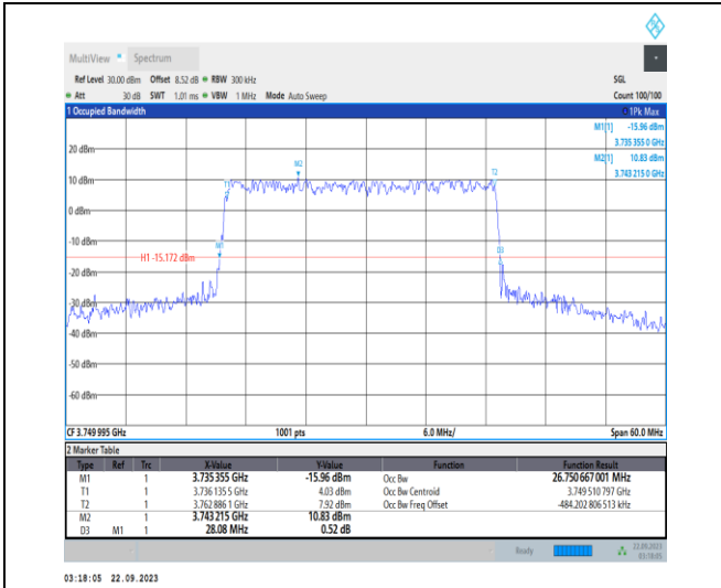
1-N78-3700-3800-PC2-30-30-M-4-DFT-64QAM-Out er_Full-75@0-Ant12-26.751-28.080-≤30-PASS
