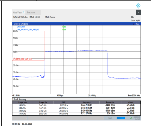
1-N78-3450-3550-PC2-30-100-L-3-DFT-PI2BPSK-Outer_Full-270@0-Ant12-1--PASS-see graph
