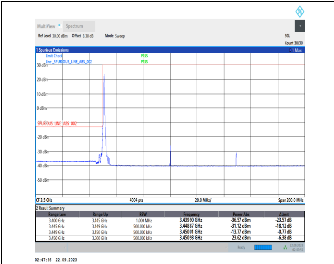
1-N78-3450-3550-PC2-30-100-L-1-DFT-PI2BPSK-Edge_1RB_Left-1@0-Ant12-1--PASS-see graph
