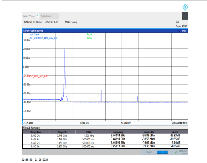
1-N78-3450-3550-PC2-30-90-L-4-CP-QPSK-Edge_1RB_Left-1@0-Ant12-1--PASS-see graph
