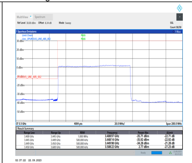
1-N78-3450-3550-PC2-30-90-L-3-DFT-PI2BPSK-Outer_Full-240@0-Ant12-1--PASS-see graph
