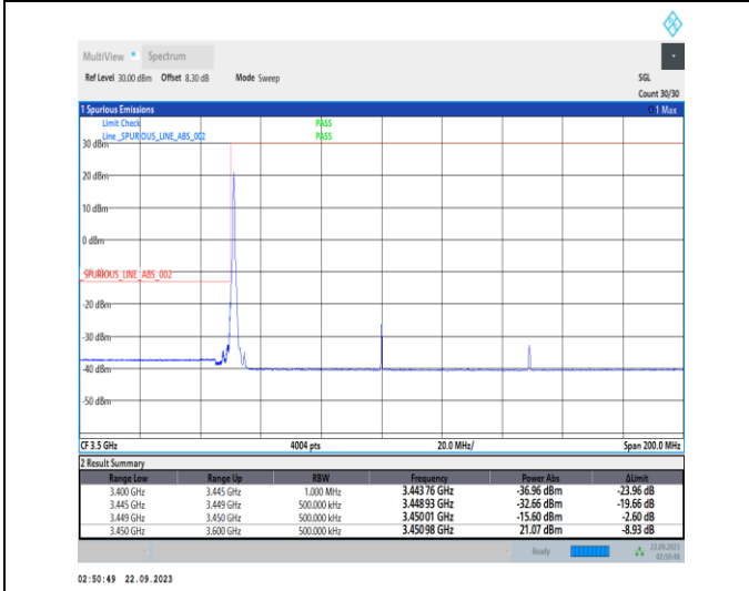
1-N78-3450-3550-PC2-30-100-L-4-CP-QPSK-Edge_1RB_Left-1@0-Ant12-1--PASS-see graph
