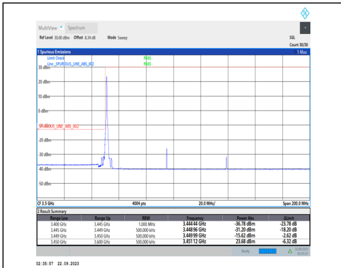
1-N78-3450-3550-PC2-30-90-L-1-DFT-PI2BPSK-Edge_1RB_Left-1@0-Ant12-1--PASS-see graph
