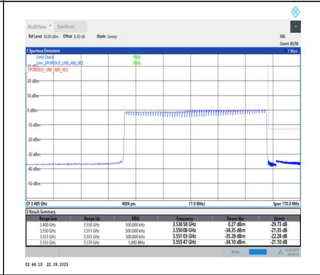
1-N78-3450-3550-PC2-30-90-H-6-CP-QPSK-Outer_Full-245@0-Ant12-1--PASS-see graph
