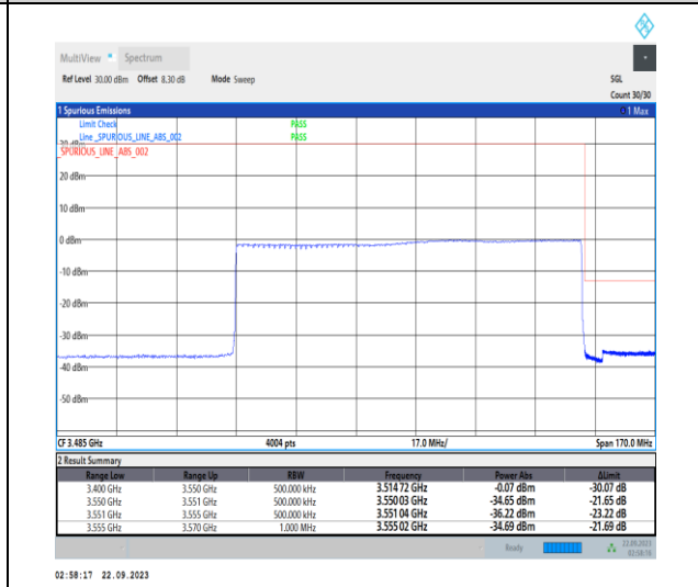
1-N78-3450-3550-PC2-30-100-H-6-CP-QPSK-Outer_Full-273@0-Ant12-1--PASS-see graph
