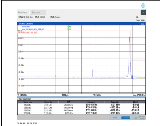
1-N78-3450-3550-PC2-30-100-H-5-CP-QPSK-Edge_1RB_Right-1@272-Ant12-1--PASS-see graph
