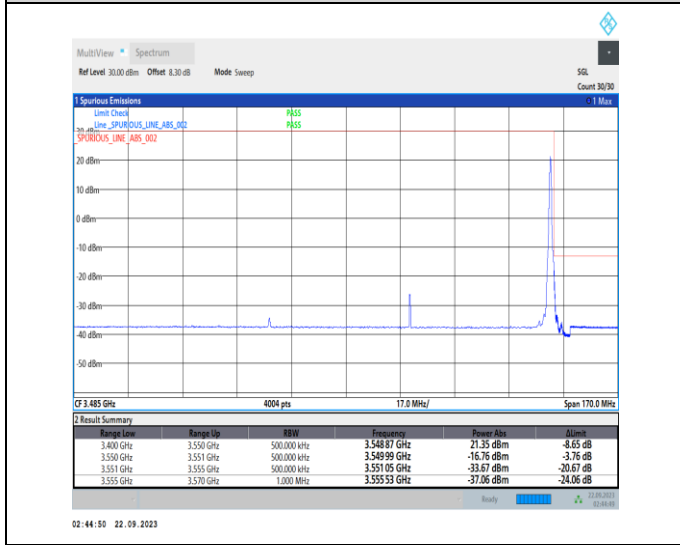
1-N78-3450-3550-PC2-30-90-H-5-CP-QPSK-Edge_1RB_Right-1@244-Ant12-1--PASS-see graph
