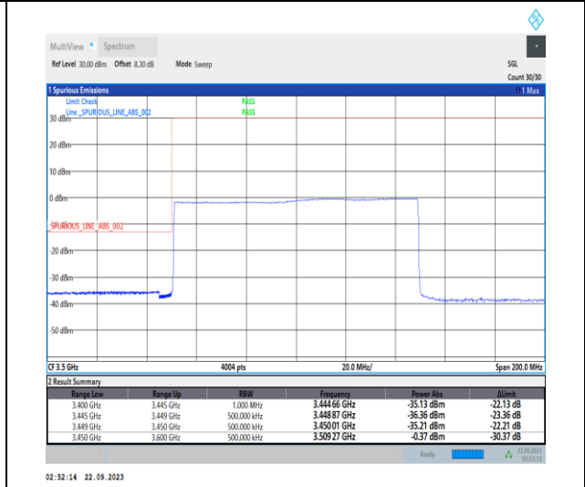
1-N78-3450-3550-PC2-30-100-L-6-CP-QPSK-Outer_Full-273@0-Ant12-1--PASS-see graph
