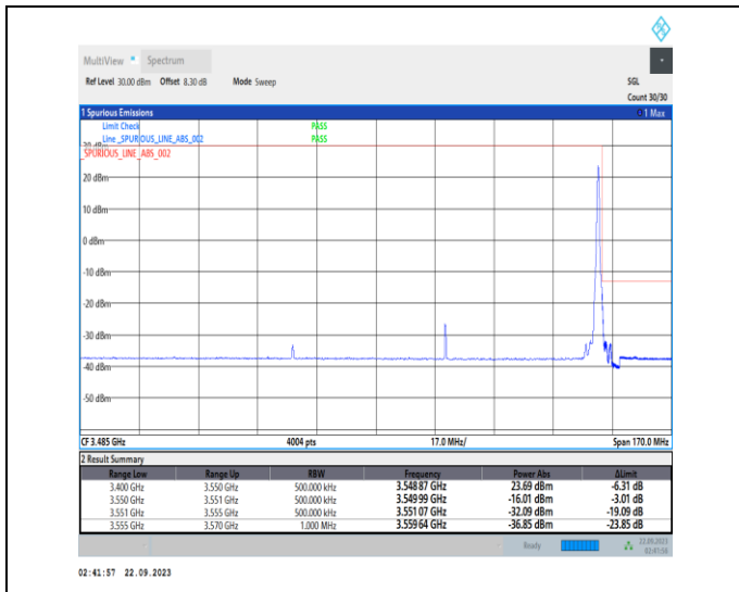
1-N78-3450-3550-PC2-30-90-H-2-DFT-PI2BPSK-Edge_1RB_Right-1@244-Ant12-1--PASS-see graph
