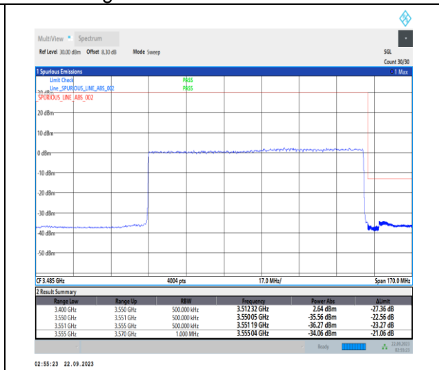
1-N78-3450-3550-PC2-30-100-H-3-DFT-PI2BPSK-Outer_Full-270@0-Ant12-1--PASS-see graph
