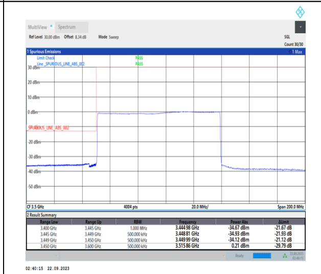
1-N78-3450-3550-PC2-30-90-L-6-CP-QPSK-Outer_Full-245@0-Ant12-1--PASS-see graph
