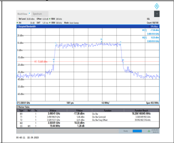
1-N78-3450-3550-PC2-30-20-M-6-CP-QPSK-Outer_Full-51@0-Ant12-18.206-19.440-≤20-PASS
