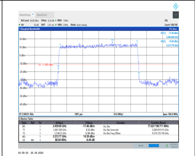
1-N78-3450-3550-PC2-30-80-M-2-DFT-PI2BPSK-Outer_Full-216@0-Ant12-77.021-80.640-≤80-PASS
