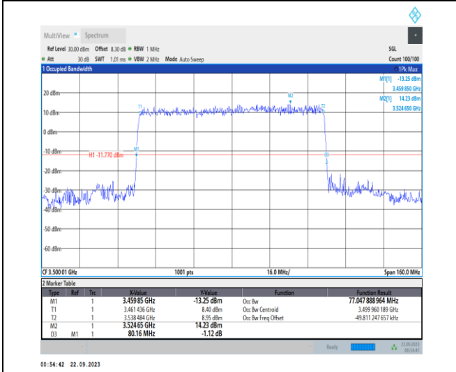
1-N78-3450-3550-PC2-30-80-M-1-DFT-QPSK-Outer_Full-216@0-Ant12-77.048-80.160-≤80-PASS
