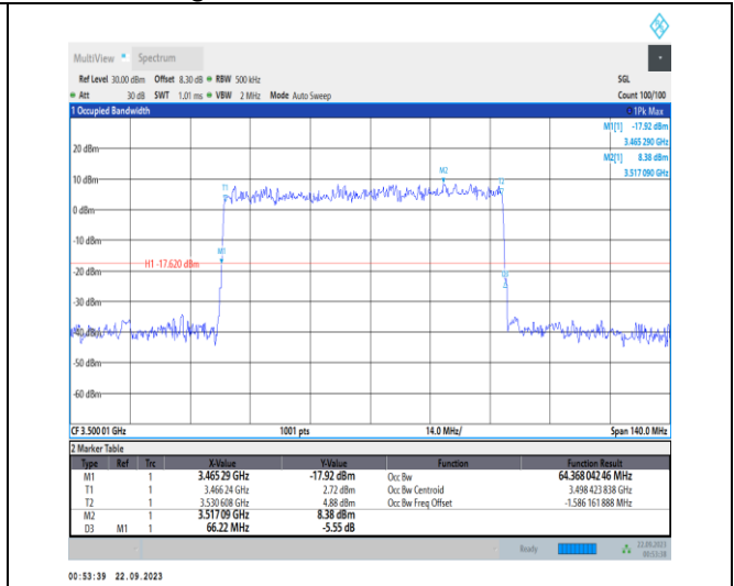
1-N78-3450-3550-PC2-30-70-M-5-DFT-256QAM-Outer_Full-180@0-Ant12-64.368-66.220-≤70-PASS
