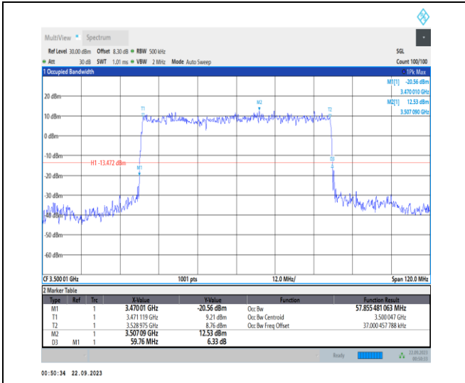
1-N78-3450-3550-PC2-30-60-M-1-DFT-QPSK-Outer_Full-162@0-Ant12-57.855-59.760-≤60-PASS
