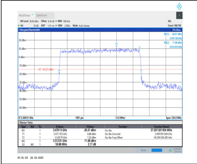
1-N78-3450-3550-PC2-30-60-M-7-CP-16QAM-Outer _Full-162@0-Ant12-57.597-59.880-≤60-PASS
