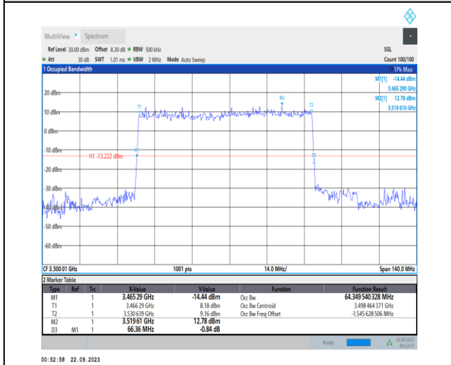
1-N78-3450-3550-PC2-30-70-M-2-DFT-PI2BPSK-Outer_Full-180@0-Ant12-64.35-66.360-≤70-PASS
