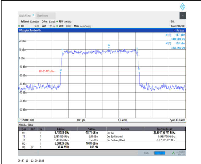
1-N78-3450-3550-PC2-30-40-M-5-DFT-256QAM-Outer_Full-100@0-Ant12-35.834-37.440-≤40-PASS
