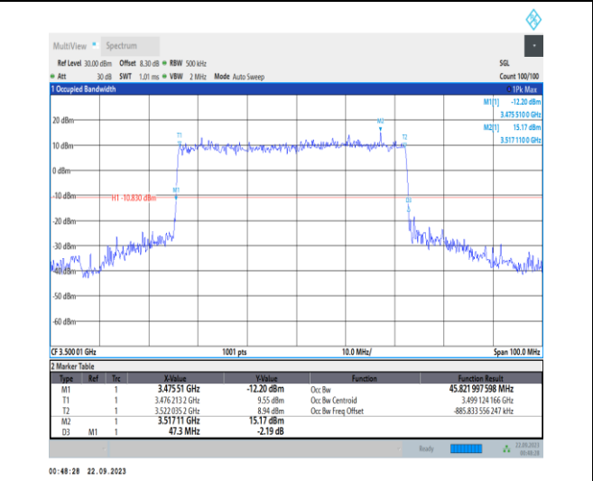
1-N78-3450-3550-PC2-30-50-M-1-DFT-QPSK-Outer_Full-128@0-Ant12-45.822-47.300-≤50-PASS
