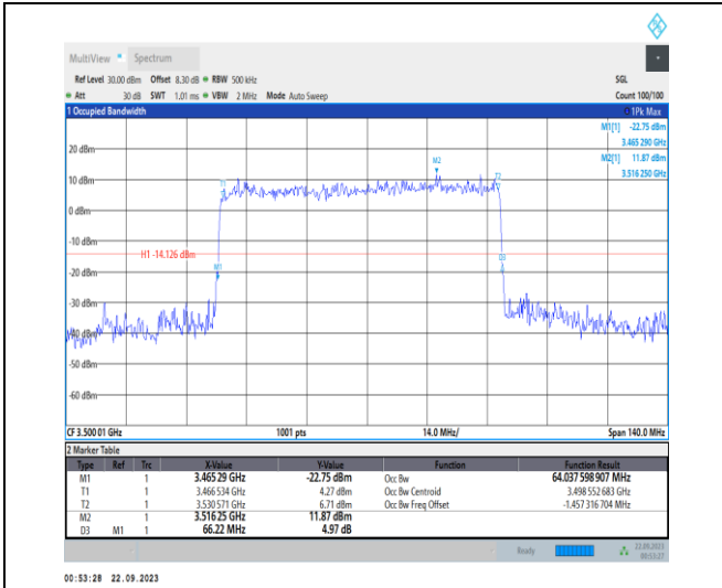
1-N78-3450-3550-PC2-30-70-M-4-DFT-64QAM-Outer_Full-180@0-Ant12-64.038-66.220-≤70-PASS
