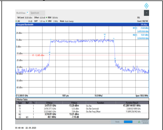
1-N78-3450-3550-PC2-30-50-M-7-CP-16QAM-Outer_Full-133@0-Ant12-47.289-49.100-≤50-PASS
