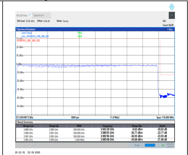
1-N77-3700-3980-PC2-30-100-H-3-DFT-PI2BPSK-Outer_Full-270@0-Ant12-1--PASS-see graph
