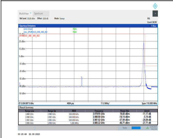
1-N77-3700-3980-PC2-30-100-H-5-CP-QPSK-Edge_1RB_Right-1@272-Ant12-1--PASS-see graph
