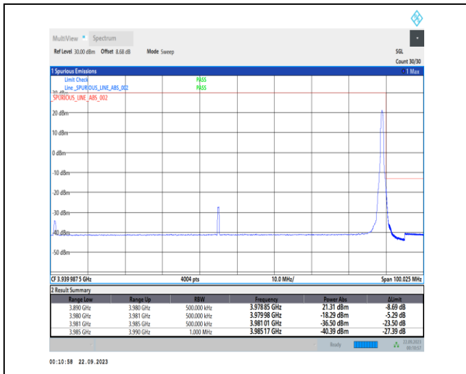
1-N77-3700-3980-PC2-30-90-H-2-DFT-PI2BPSK-Edge_1RB_Right-1@244-Ant12-1--PASS-see graph
