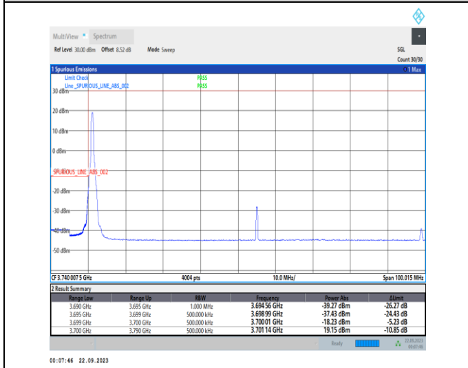
1-N77-3700-3980-PC2-30-90-L-4-CP-QPSK-Edge_1RB_Left-1@0-Ant12-1--PASS-see graph
