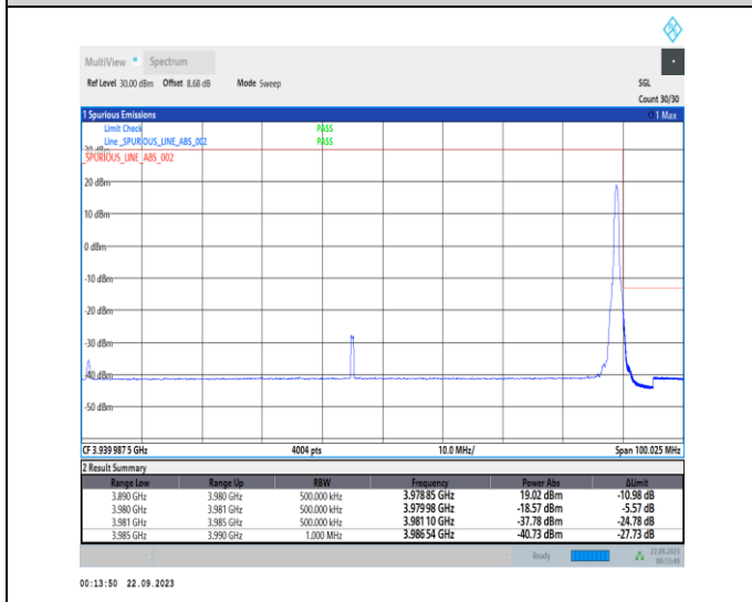
1-N77-3700-3980-PC2-30-90-H-5-CP-QPSK-Edge_1RB_Right-1@244-Ant12-1--PASS-see graph
