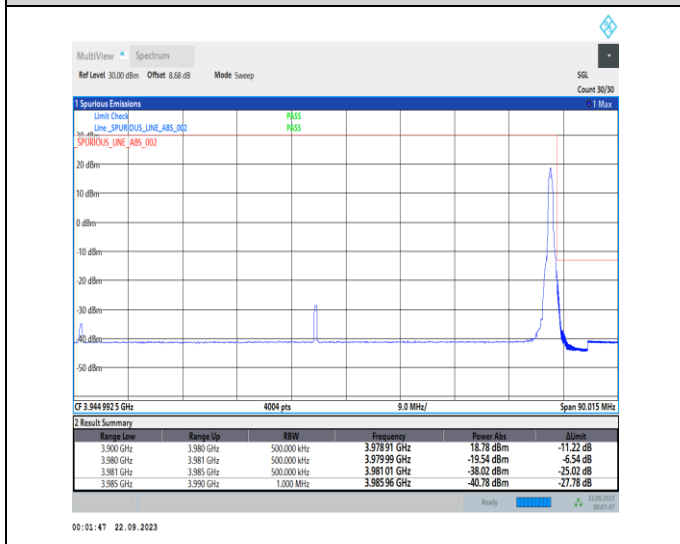
1-N77-3700-3980-PC2-30-80-H-5-CP-QPSK-Edge_1RB_Right-1@216-Ant12-1--PASS-see graph
