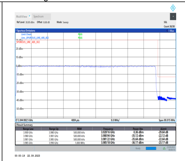
1-N77-3700-3980-PC2-30-80-H-3-DFT-PI2BPSK-Outer_Full-216@0-Ant12-1--PASS-see graph
