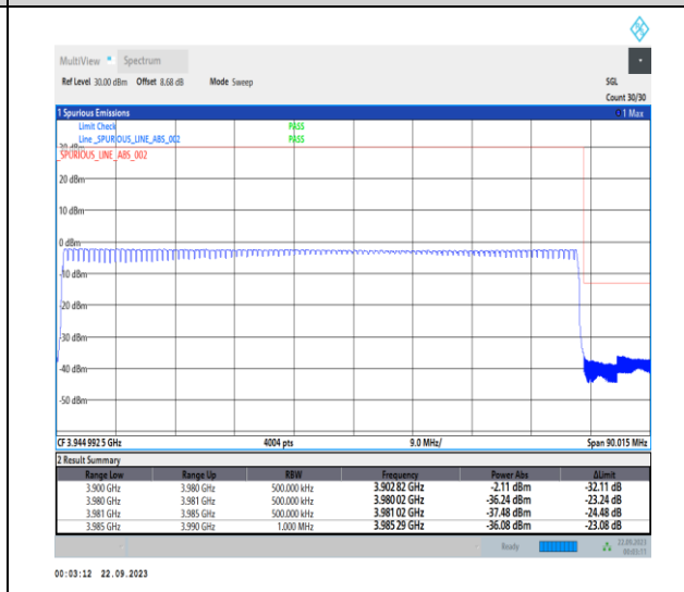
1-N77-3700-3980-PC2-30-80-H-6-CP-QPSK-Outer_Full-217@0-Ant12-1--PASS-see graph
