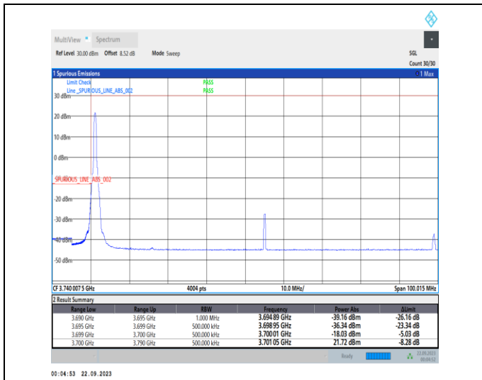
1-N77-3700-3980-PC2-30-90-L-1-DFT-PI2BPSK-Edge_1RB_Left-1@0-Ant12-1--PASS-see graph
