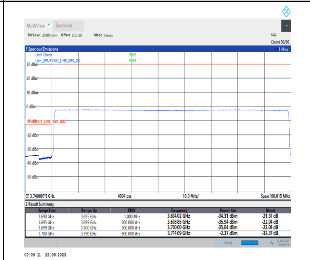
1-N77-3700-3980-PC2-30-90-L-6-CP-QPSK-Outer_Full-245@0-Ant12-1--PASS-see graph
