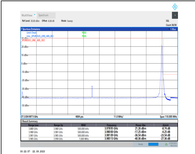
1-N77-3700-3980-PC2-30-100-H-2-DFT-PI2BPSK-Edge_1RB_Right-1@272-Ant12-1--PASS-see graph
