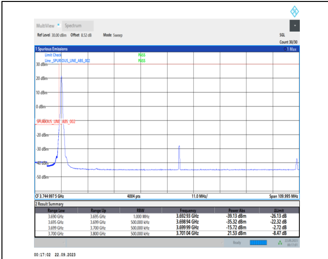
1-N77-3700-3980-PC2-30-100-L-1-DFT-PI2BPSK-Edge_1RB_Left-1@0-Ant12-1--PASS-see graph
