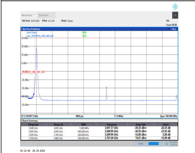
1-N77-3700-3980-PC2-30-100-L-4-CP-QPSK-Edge_1RB_Left-1@0-Ant12-1--PASS-see graph
