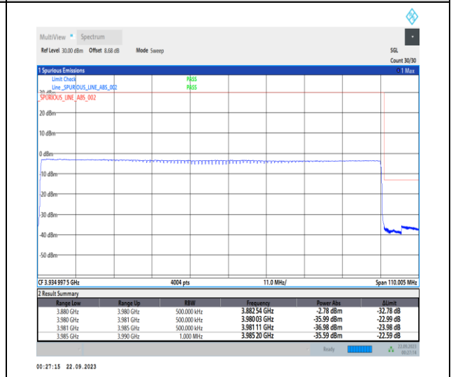
1-N77-3700-3980-PC2-30-100-H-6-CP-QPSK-Outer_Full-273@0-Ant12-1--PASS-see graph
