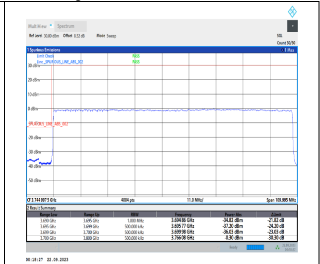
1-N77-3700-3980-PC2-30-100-L-3-DFT-PI2BPSK-Outer_Full-270@0-Ant12-1--PASS-see graph
