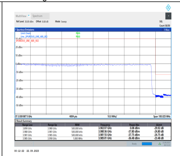
1-N77-3700-3980-PC2-30-90-H-3-DFT-PI2BPSK-Outer_Full-240@0-Ant12-1--PASS-see graph
