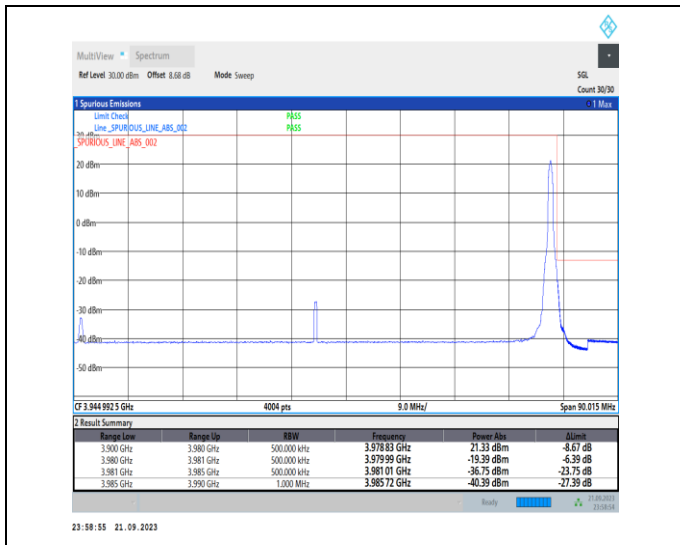
1-N77-3700-3980-PC2-30-80-H-2-DFT-PI2BPSK-Edge_1RB_Right-1@216-Ant12-1--PASS-see graph
