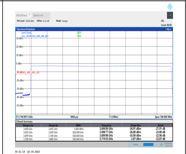
1-N77-3700-3980-PC2-30-100-L-6-CP-QPSK-Outer_Full-273@0-Ant12-1--PASS-see graph
