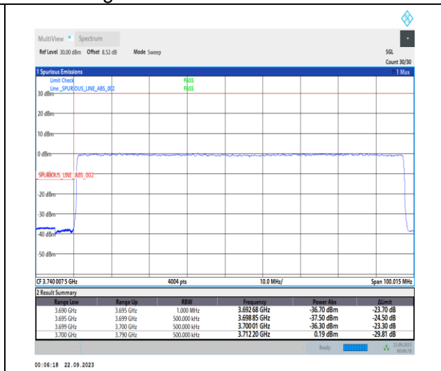
1-N77-3700-3980-PC2-30-90-L-3-DFT-PI2BPSK-Outer_Full-240@0-Ant12-1--PASS-see graph
