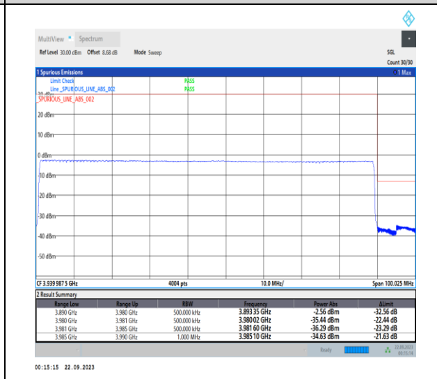
1-N77-3700-3980-PC2-30-90-H-6-CP-QPSK-Outer_Full-245@0-Ant12-1--PASS-see graph
