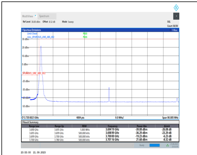
1-N77-3700-3980-PC2-30-80-L-1-DFT-PI2BPSK-Edge_1RB_Left-1@0-Ant12-1--PASS-see graph
