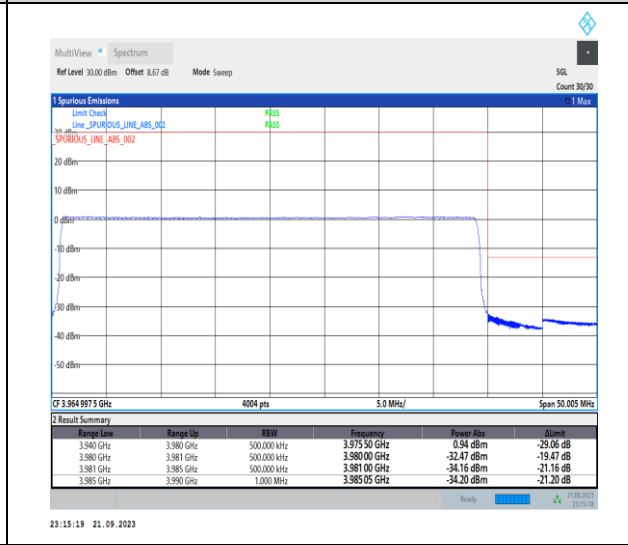
1-N77-3700-3980-PC2-30-40-H-6-CP-QPSK-Outer_Full-106@0-Ant12-1--PASS-see graph
