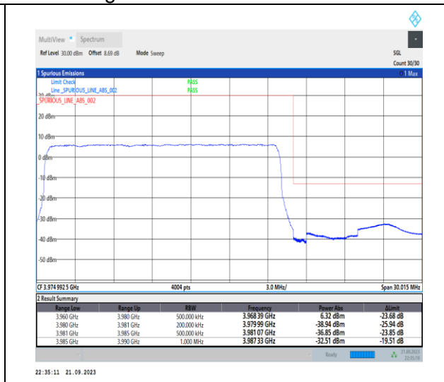
1-N77-3700-3980-PC2-30-20-H-3-DFT-PI2BPSK-Outer_Full-50@0-Ant12-1--PASS-see graph
