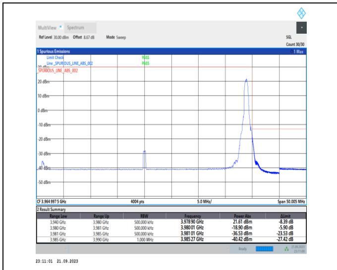
1-N77-3700-3980-PC2-30-40-H-2-DFT-PI2BPSK-Edge_1RB_Right-1@105-Ant12-1--PASS-see graph
