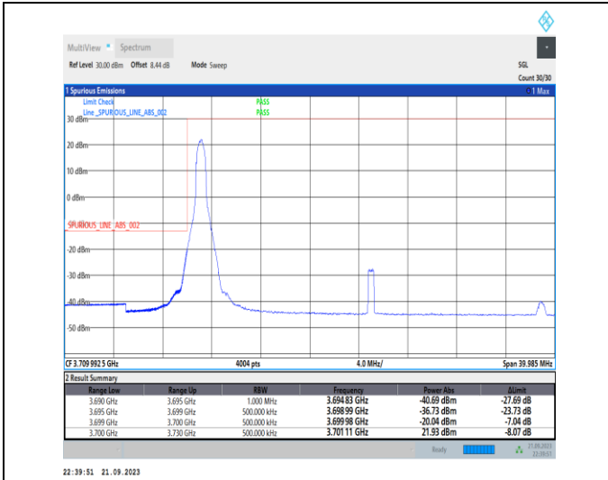
1-N77-3700-3980-PC2-30-30-L-1-DFT-PI2BPSK-Edge_1RB_Left-1@0-Ant12-1--PASS-see graph
