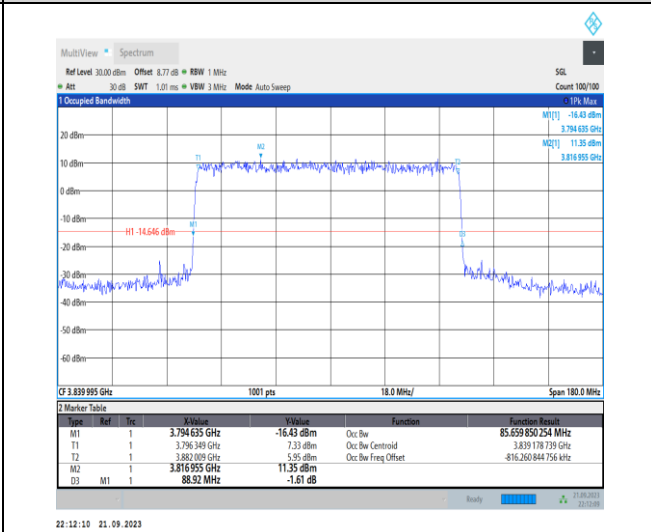
1-N77-3700-3980-PC2-30-90-M-1-DFT-QPSK-Outer _Full-240@0-Ant12-85.66-88.920-≤90-PASS
