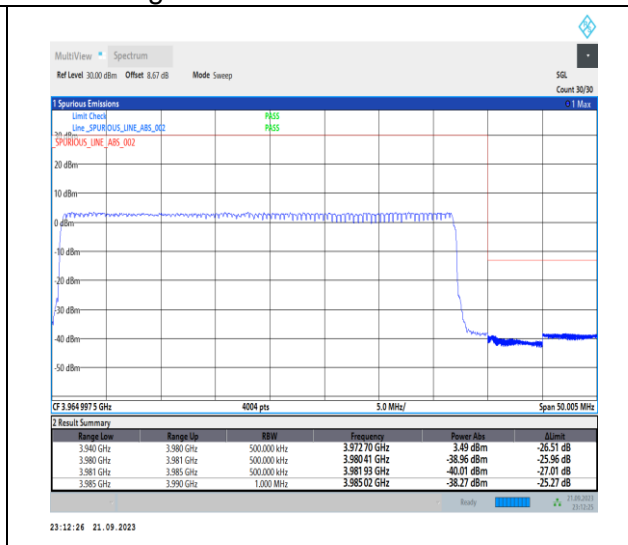
1-N77-3700-3980-PC2-30-40-H-3-DFT-PI2BPSK-Outer_Full-100@0-Ant12-1--PASS-see graph
