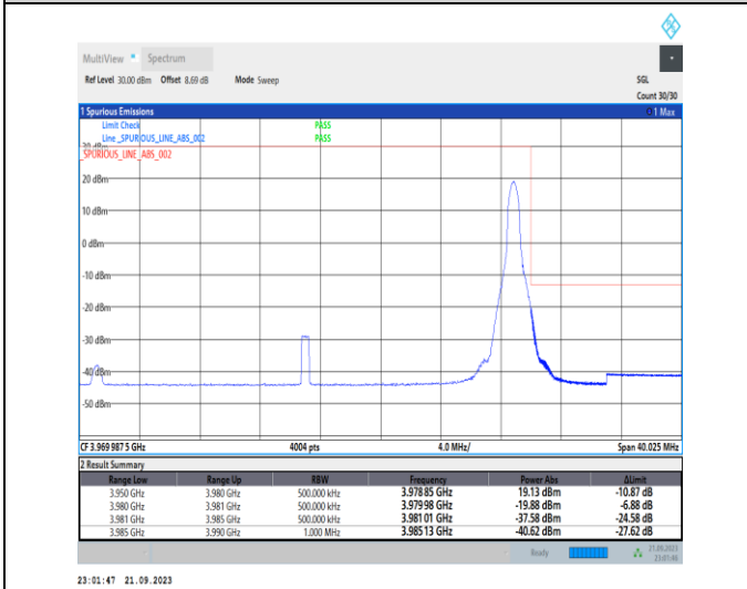
1-N77-3700-3980-PC2-30-30-H-5-CP-QPSK-Edge_1RB_Right-1@77-Ant12-1--PASS-see graph
