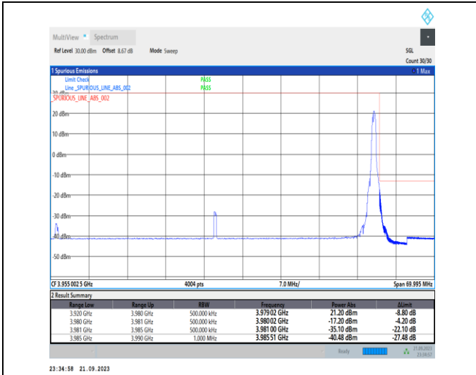
1-N77-3700-3980-PC2-30-60-H-2-DFT-PI2BPSK-Edge_1RB_Right-1@161-Ant12-1--PASS-see graph
