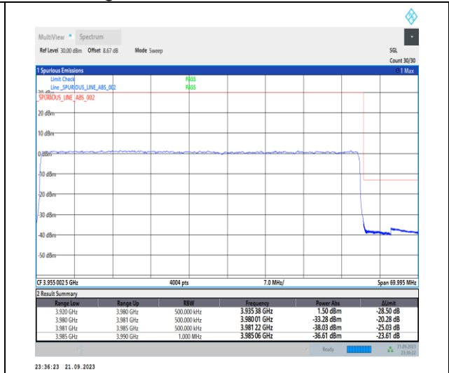
1-N77-3700-3980-PC2-30-60-H-3-DFT-PI2BPSK-Outer_Full-162@0-Ant12-1--PASS-see graph
