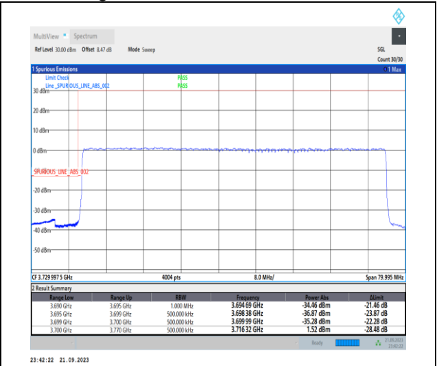
1-N77-3700-3980-PC2-30-70-L-3-DFT-PI2BPSK-Outer_Full-180@0-Ant12-1--PASS-see graph
