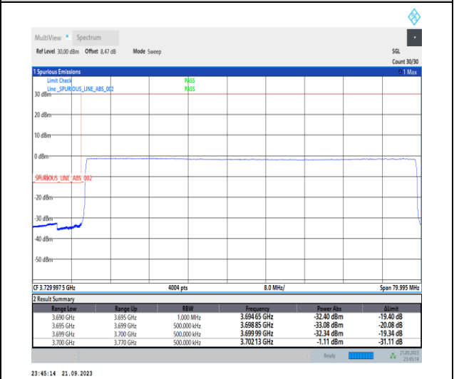
1-N77-3700-3980-PC2-30-70-L-6-CP-QPSK-Outer_Full-189@0-Ant12-1--PASS-see graph
