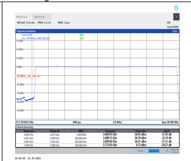
1-N77-3700-3980-PC2-30-80-L-3-DFT-PI2BPSK-Outer_Full-216@0-Ant12-1--PASS-see graph
