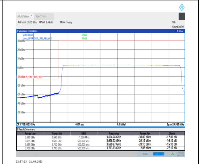
1-N77-3700-3980-PC2-30-30-L-6-CP-QPSK-Outer_Full-78@0-Ant12-1--PASS-see graph
