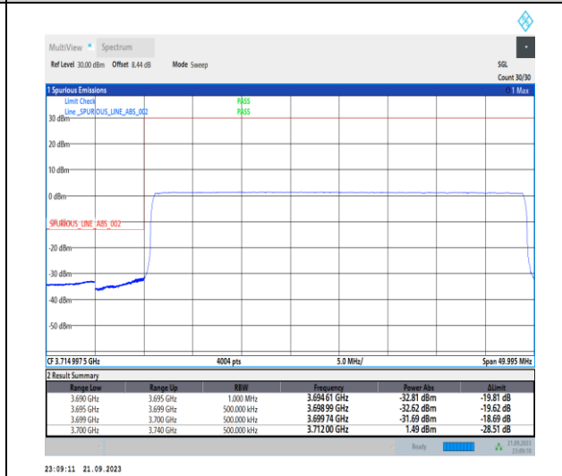
1-N77-3700-3980-PC2-30-40-L-6-CP-QPSK-Outer_Full-106@0-Ant12-1--PASS-see graph
