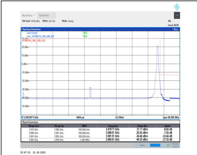
1-N77-3700-3980-PC2-30-70-H-2-DFT-PI2BPSK-Edge_1RB_Right-1@188-Ant12-1--PASS-see graph
