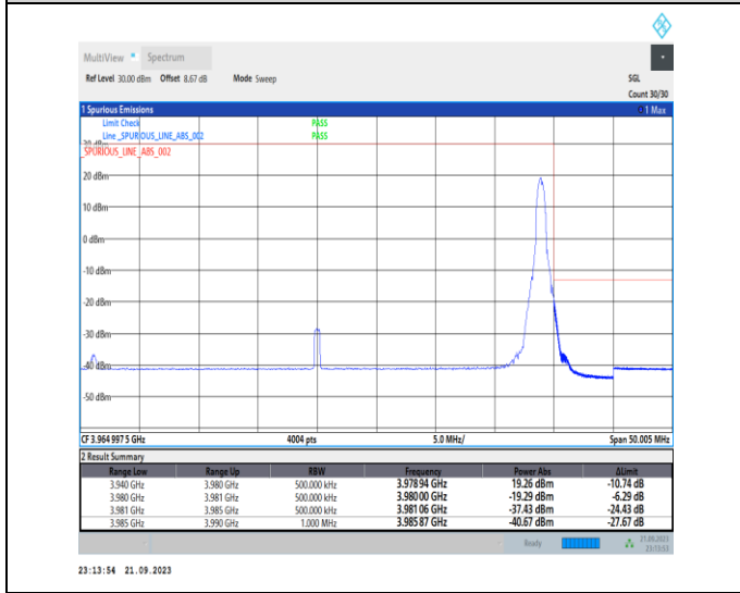
1-N77-3700-3980-PC2-30-40-H-5-CP-QPSK-Edge_1RB_Right-1@105-Ant12-1--PASS-see graph
