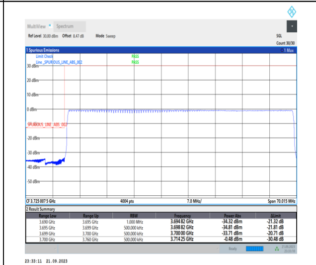
1-N77-3700-3980-PC2-30-60-L-6-CP-QPSK-Outer_Full-162@0-Ant12-1--PASS-see graph
