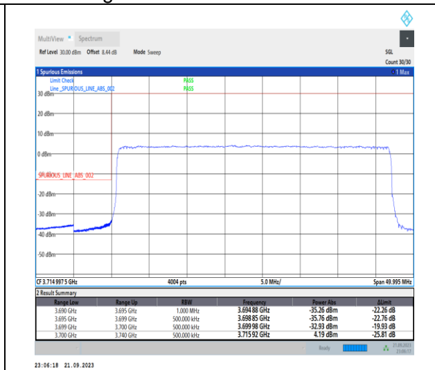
1-N77-3700-3980-PC2-30-40-L-3-DFT-PI2BPSK-Outer_Full-100@0-Ant12-1--PASS-see graph
