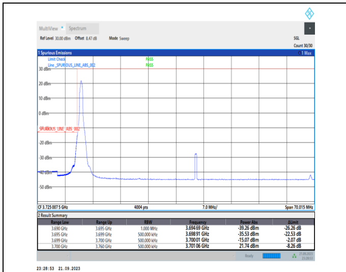
1-N77-3700-3980-PC2-30-60-L-1-DFT-PI2BPSK-Edge_1RB_Left-1@0-Ant12-1--PASS-see graph
