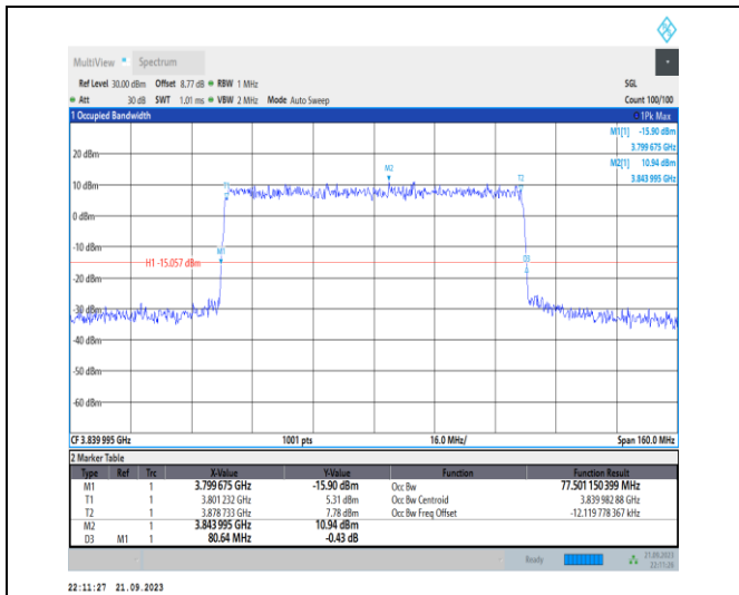
1-N77-3700-3980-PC2-30-80-M-7-CP-16QAM-Outer _Full-217@0-Ant12-77.501-80.640-≤80-PASS
