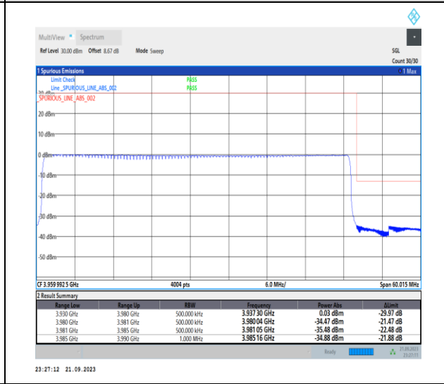
1-N77-3700-3980-PC2-30-50-H-6-CP-QPSK-Outer_Full-133@0-Ant12-1--PASS-see graph
