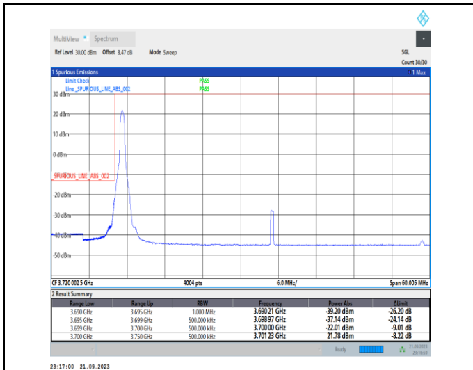
1-N77-3700-3980-PC2-30-50-L-1-DFT-PI2BPSK-Edge_1RB_Left-1@0-Ant12-1--PASS-see graph
