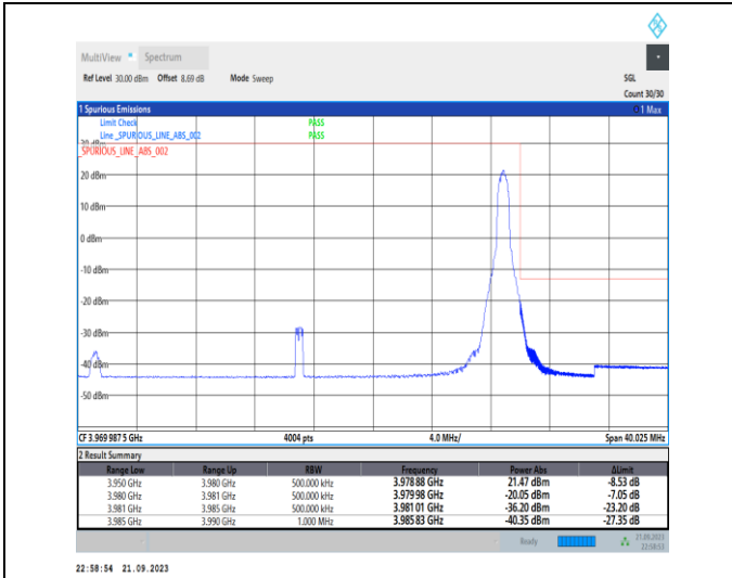
1-N77-3700-3980-PC2-30-30-H-2-DFT-PI2BPSK-Edge_1RB_Right-1@77-Ant12-1--PASS-see graph
