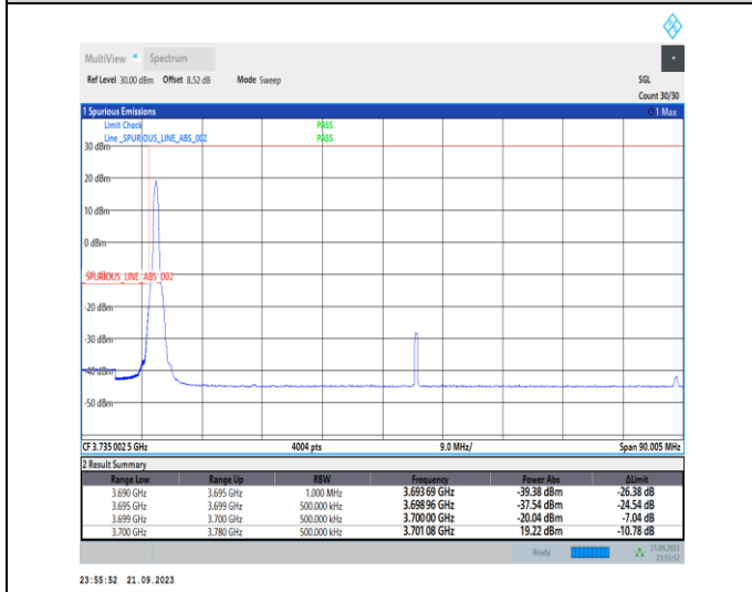
1-N77-3700-3980-PC2-30-80-L-4-CP-QPSK-Edge_1RB_Left-1@0-Ant12-1--PASS-see graph
