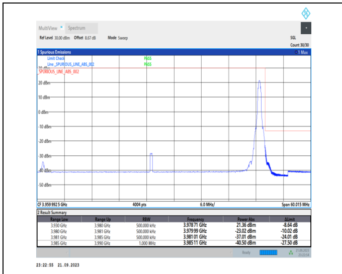
1-N77-3700-3980-PC2-30-50-H-2-DFT-PI2BPSK-Edge_1RB_Right-1@132-Ant12-1--PASS-see graph
