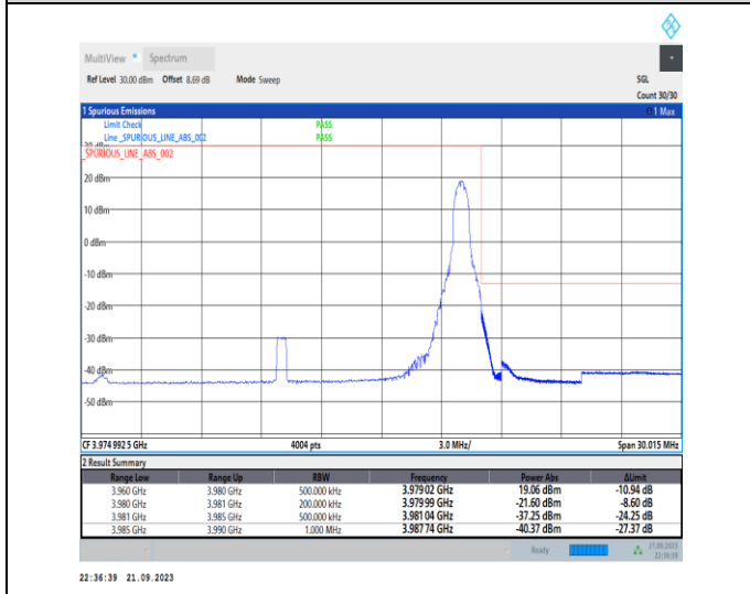
1-N77-3700-3980-PC2-30-20-H-5-CP-QPSK-Edge_1RB_Right-1@50-Ant12-1--PASS-see graph
