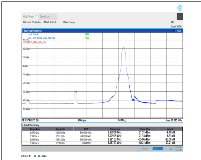
1-N77-3700-3980-PC2-30-20-H-2-DFT-PI2BPSK-Edge_1RB_Right-1@50-Ant12-1--PASS-see graph
