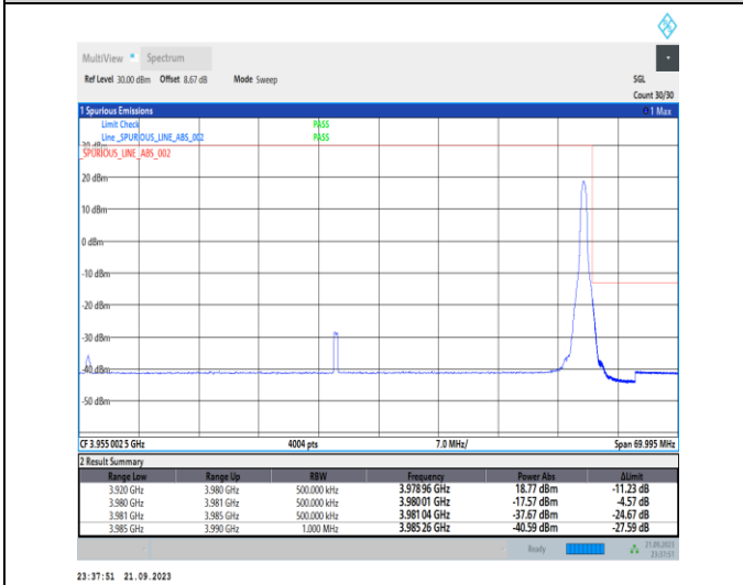
1-N77-3700-3980-PC2-30-60-H-5-CP-QPSK-Edge_1RB_Right-1@161-Ant12-1--PASS-see graph
