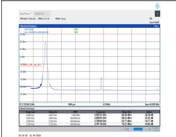
1-N77-3700-3980-PC2-30-50-L-4-CP-QPSK-Edge_1RB_Left-1@0-Ant12-1--PASS-see graph
