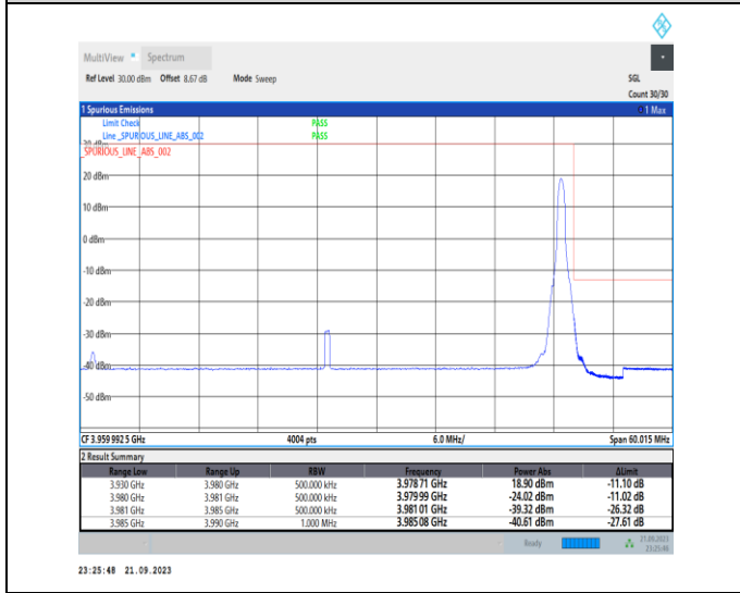
1-N77-3700-3980-PC2-30-50-H-5-CP-QPSK-Edge_1RB_Right-1@132-Ant12-1--PASS-see graph
