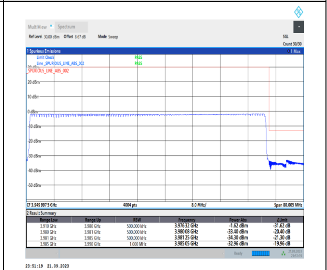
1-N77-3700-3980-PC2-30-70-H-6-CP-QPSK-Outer_Full-189@0-Ant12-1--PASS-see graph
