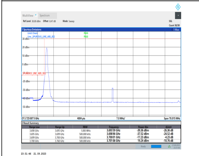
1-N77-3700-3980-PC2-30-60-L-4-CP-QPSK-Edge_1RB_Left-1@0-Ant12-1--PASS-see graph
