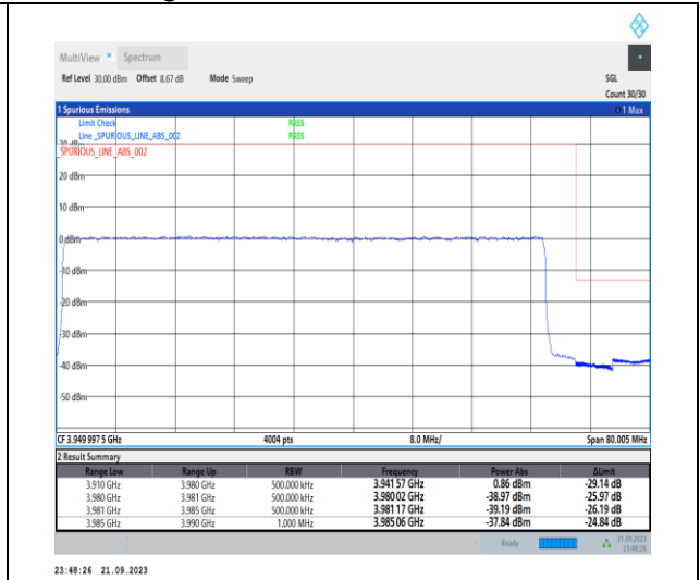
1-N77-3700-3980-PC2-30-70-H-3-DFT-PI2BPSK-Outer_Full-180@0-Ant12-1--PASS-see graph
