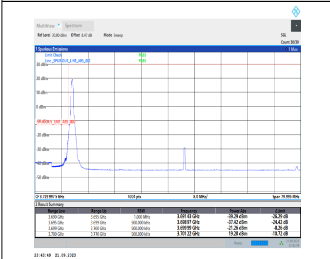
1-N77-3700-3980-PC2-30-70-L-4-CP-QPSK-Edge_1RB_Left-1@0-Ant12-1--PASS-see graph
