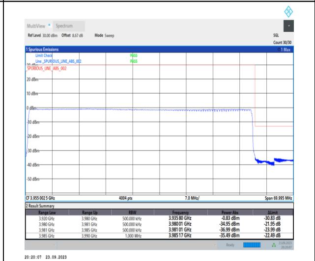
1-N77-3700-3980-PC2-30-60-H-6-CP-QPSK-Outer_Full-162@0-Ant12-1--PASS-see graph
