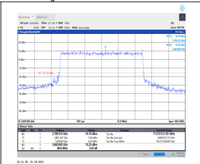
1-N77-3700-3980-PC2-30-80-M-8-CP-64QAM-Outer _Full-217@0-Ant12-77.574-80.800-≤80-PASS
