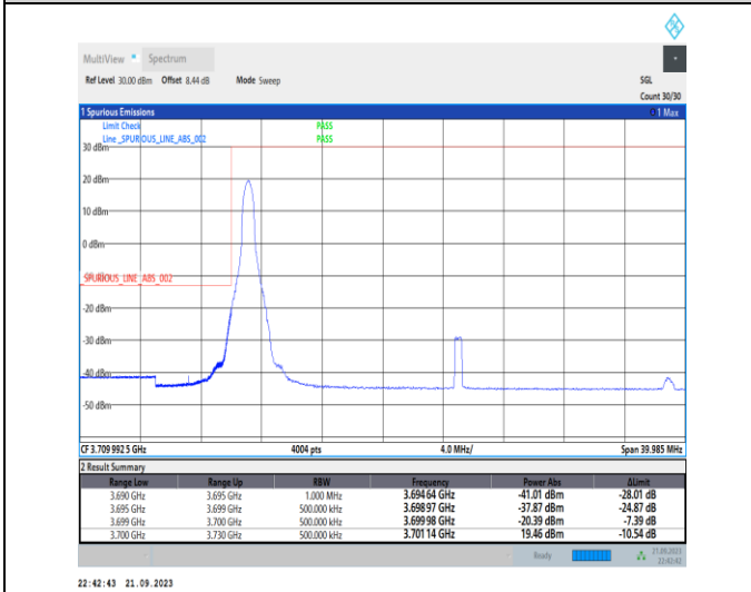
1-N77-3700-3980-PC2-30-30-L-4-CP-QPSK-Edge_1RB_Left-1@0-Ant12-1--PASS-see graph
