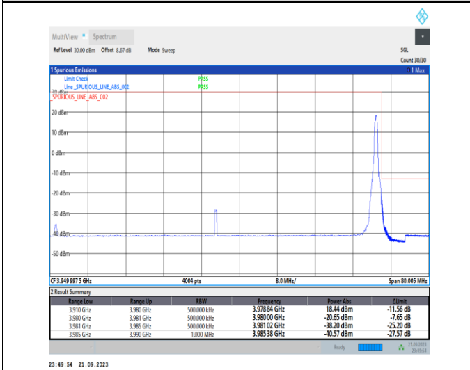
1-N77-3700-3980-PC2-30-70-H-5-CP-QPSK-Edge_1RB_Right-1@188-Ant12-1--PASS-see graph
