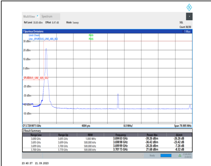
1-N77-3700-3980-PC2-30-70-L-1-DFT-PI2BPSK-Edge_1RB_Left-1@0-Ant12-1--PASS-see graph
