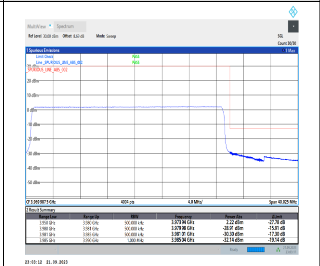
1-N77-3700-3980-PC2-30-30-H-6-CP-QPSK-Outer_Full-78@0-Ant12-1--PASS-see graph
