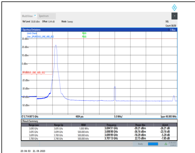
1-N77-3700-3980-PC2-30-40-L-1-DFT-PI2BPSK-Edge_1RB_Left-1@0-Ant12-1--PASS-see graph
