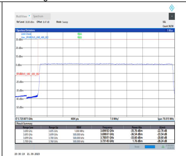
1-N77-3700-3980-PC2-30-60-L-3-DFT-PI2BPSK-Outer_Full-162@0-Ant12-1--PASS-see graph
