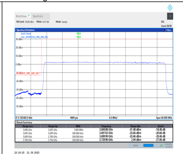
1-N77-3700-3980-PC2-30-50-L-3-DFT-PI2BPSK-Outer_Full-128@0-Ant12-1--PASS-see graph
