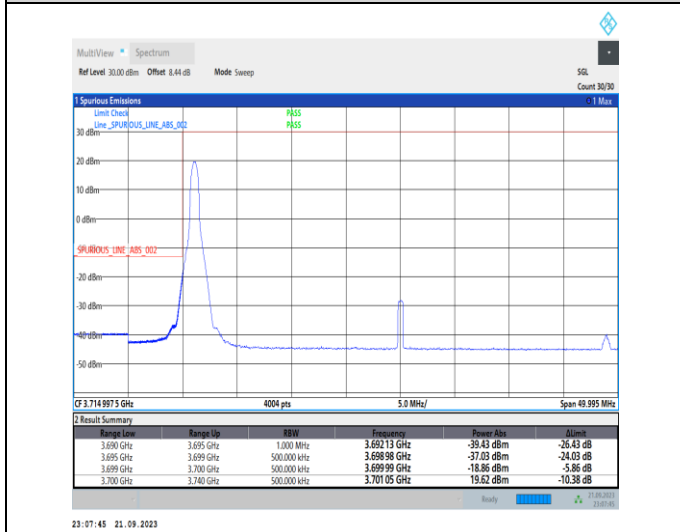
1-N77-3700-3980-PC2-30-40-L-4-CP-QPSK-Edge_1RB_Left-1@0-Ant12-1--PASS-see graph
