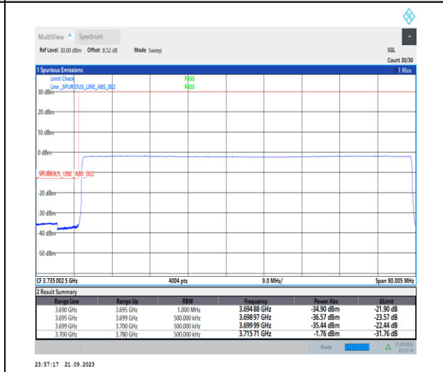
1-N77-3700-3980-PC2-30-80-L-6-CP-QPSK-Outer_Full-217@0-Ant12-1--PASS-see graph
