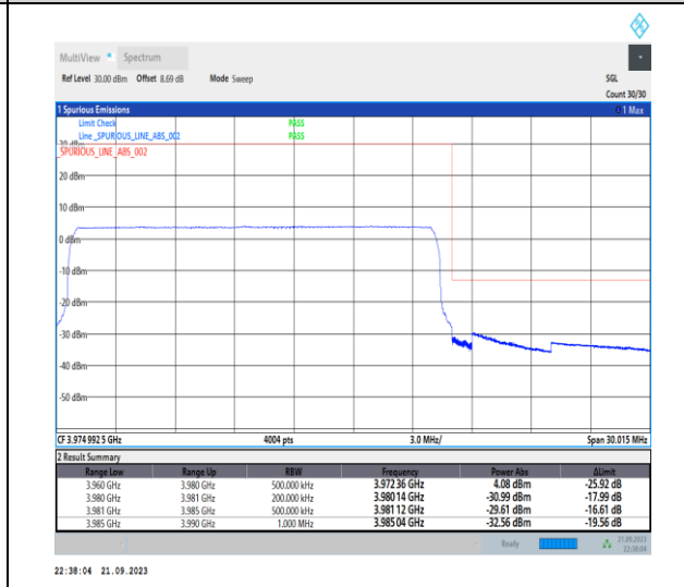
1-N77-3700-3980-PC2-30-20-H-6-CP-QPSK-Outer_Full-51@0-Ant12-1--PASS-see graph
