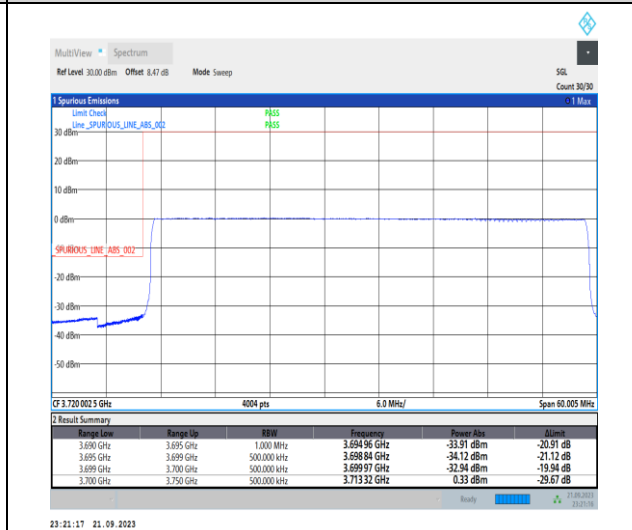
1-N77-3700-3980-PC2-30-50-L-6-CP-QPSK-Outer_Full-133@0-Ant12-1--PASS-see graph
