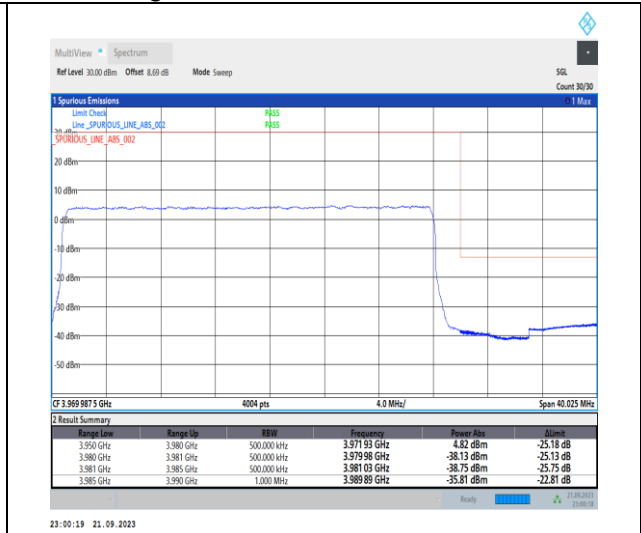
1-N77-3700-3980-PC2-30-30-H-3-DFT-PI2BPSK-Outer_Full-75@0-Ant12-1--PASS-see graph
