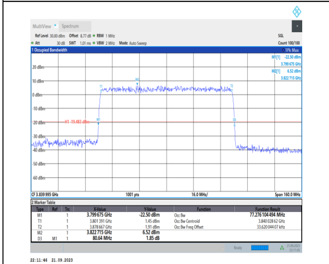
1-N77-3700-3980-PC2-30-80-M-9-CP-256QAM-Outer _Full-217@0-Ant12-77.276-80.640-≤80-PASS
