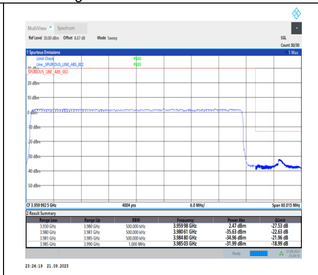
1-N77-3700-3980-PC2-30-50-H-3-DFT-PI2BPSK-Outer_Full-128@0-Ant12-1--PASS-see graph
