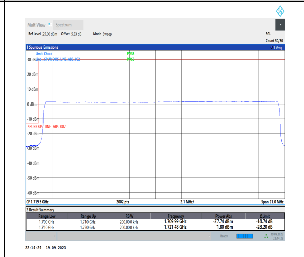
1-N66-PC3-15-20-L-6-CP-QPSK-Outer_Full-106@0-Ant31-1-seegraph-PASS-see graph
