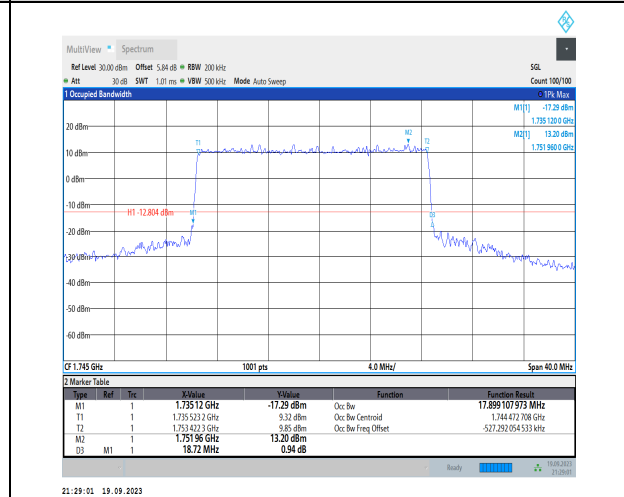
1-N66-PC3-15-20-M-1-DFT-QPSK-Outer_Full-100@0-Ant31-17.899-18.720-≤20-PASS
