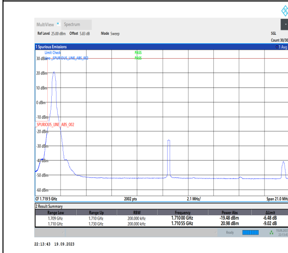
1-N66-PC3-15-20-L-4-CP-QPSK-Edge_1RB_Left-1@0-Ant31-1-seegraph-PASS-see graph
