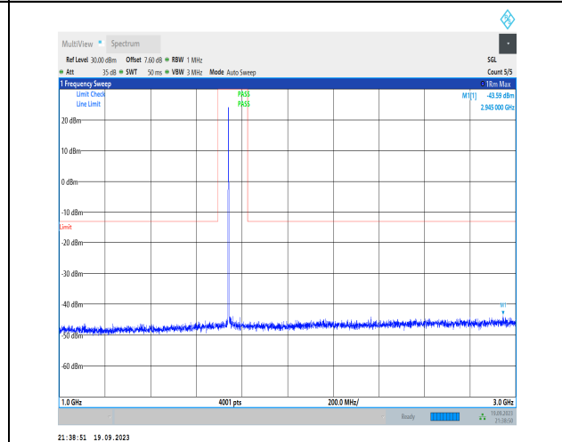
1-N66-PC3-15-40-H-1-DFT-PI2BPSK-Inner_1RB_Lef t-1@1-1000-3000-Ant31-2945.00--43.59--13-PASS
