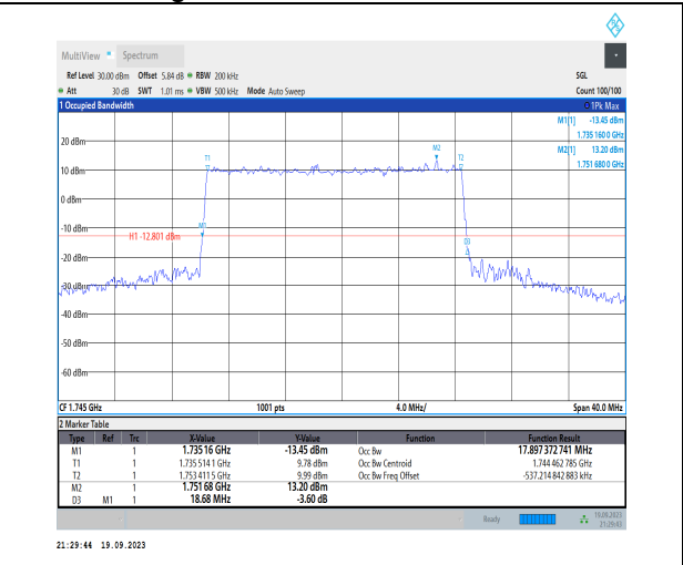
1-N66-PC3-15-20-M-3-DFT-16QAM-Outer_Full-100 @0-Ant31-17.897-18.680-≤20-PASS
