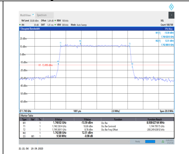
1-N66-PC3-15-10-M-1-DFT-QPSK-Outer_Full-50@0 -Ant31-8.939-9.580-≤10-PASS
