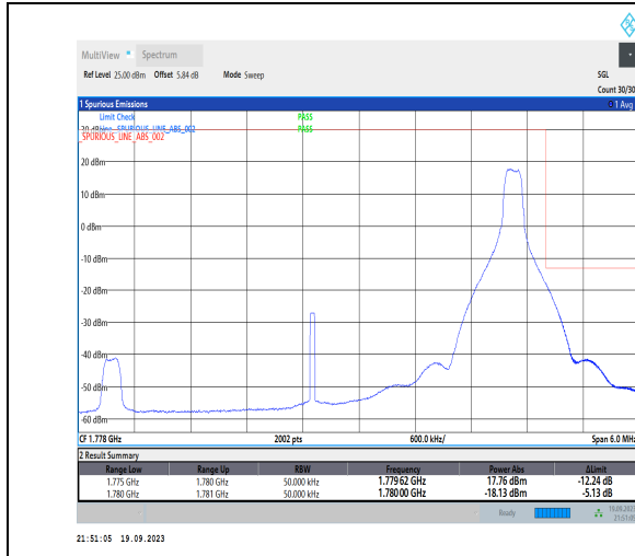
1-N66-PC3-15-5-H-2-DFT-PI2BPSK-Edge_1RB_Right-1@24-Ant31-1-seegraph-PASS-see graph
