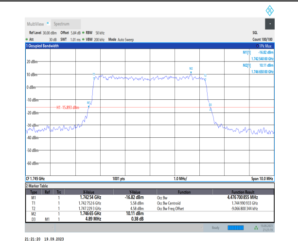
1-N66-PC3-15-5-M-8-CP-64QAM-Outer_Full-25@0- Ant31-4.477-4.890- \leq 5-PASS
