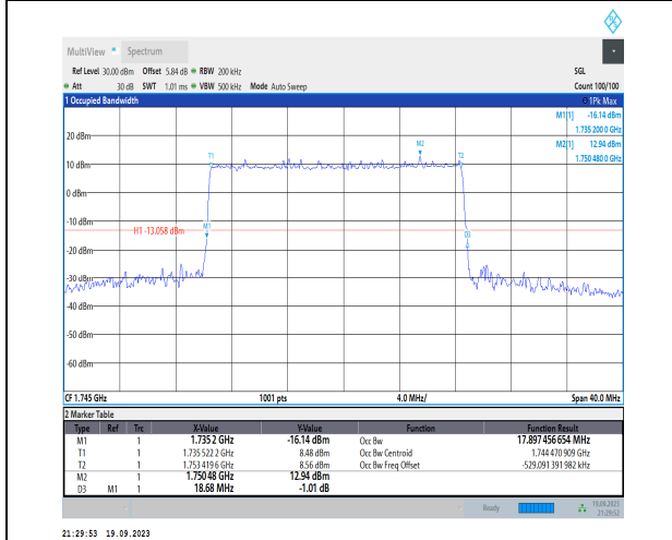
1-N66-PC3-15-20-M-4-DFT-64QAM-Outer_Full-100 @0-Ant31-17.897-18.680-≤20-PASS
