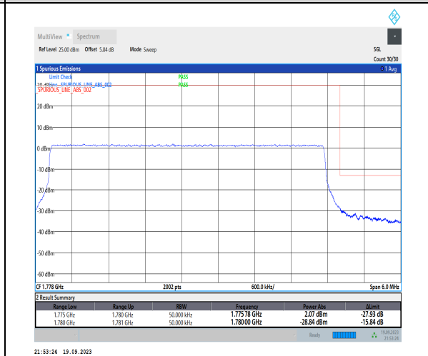
1-N66-PC3-15-5-H-6-CP-QPSK-Outer_Full-25@0-Ant31-1-seegraph-PASS-see graph
