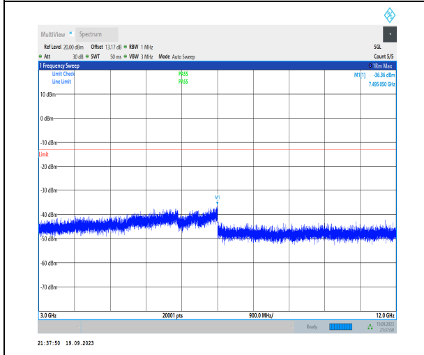
1-N66-PC3-15-40-M-1-DFT-PI2BPSK-Inner_1RB_L eft-1@1-3000-12000-Ant31-7495.05--36.36--13-PA SS
