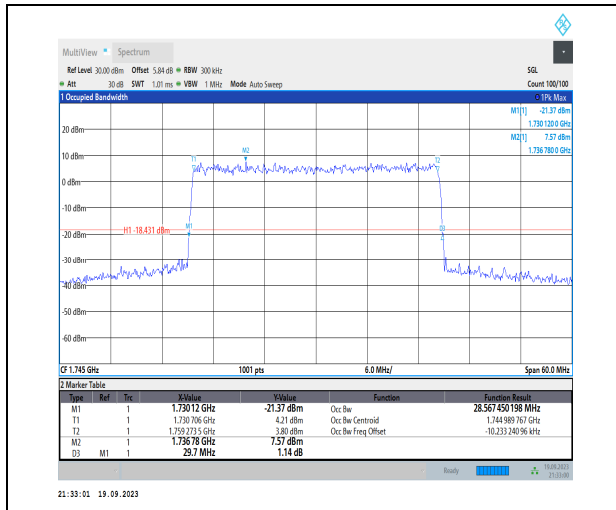
1-N66-PC3-15-30-M-9-CP-256QAM-Outer_Full-160 @0-Ant31-28.567-29.700-≤30-PASS
