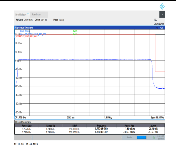
1-N66-PC3-15-15-H-6-CP-QPSK-Outer_Full-79@ 0-Ant31-1-seegraph-PASS-see graph
