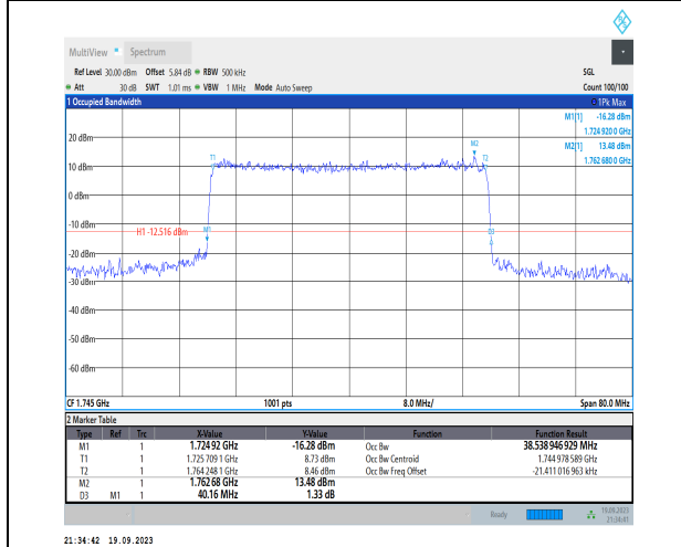
1-N66-PC3-15-40-M-6-CP-QPSK-Outer_Full-216@0 -Ant31-38.539-40.160-<math>\leq 40</math>-PASS
