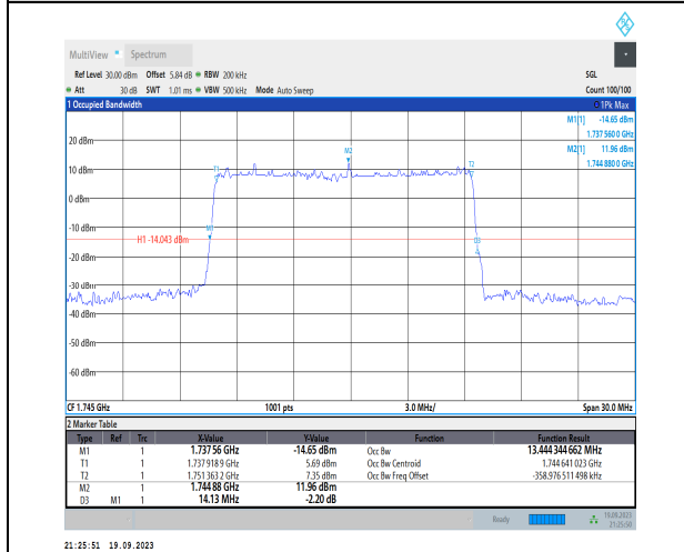
1-N66-PC3-15-15-M-5-DFT-256QAM-Outer_Full-75 @0-Ant31-13.444-14.130-≤15-PASS
