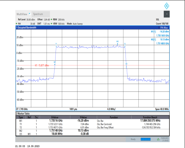
1-N66-PC3-15-20-M-5-DFT-256QAM-Outer_Full-100 @0-Ant31-17.884-18.640-≤20-PASS
