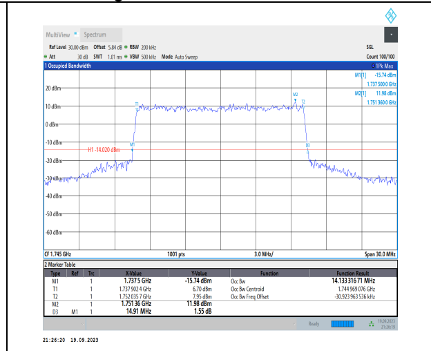
1-N66-PC3-15-15-M-8-CP-64QAM-Outer_Full-79@0 -Ant31-14.133-14.910-≤15-PASS
