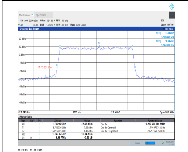
1-N66-PC3-15-10-M-6-CP-QPSK-Outer_Full-52@0- Ant31-9.288-9.980-≤10-PASS
