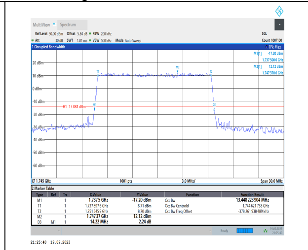
1-N66-PC3-15-15-M-4-DFT-64QAM-Outer_Full-75@ 0-Ant31-13.448-14.220-≤15-PASS
