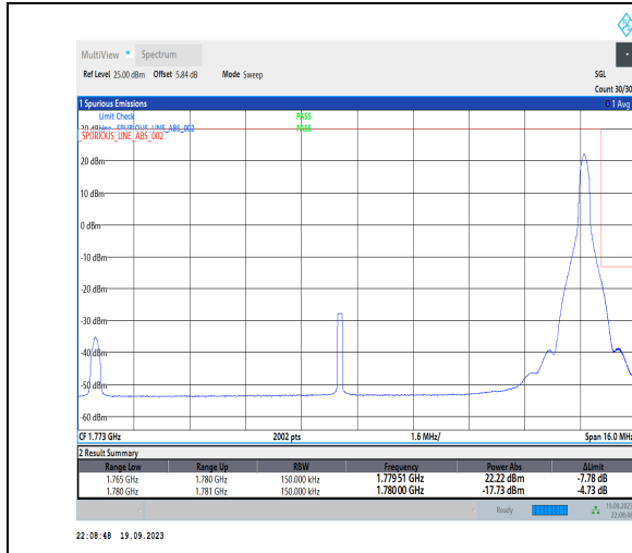
1-N66-PC3-15-15-H-2-DFT-PI2BPSK-Edge_1RB_Right t-1@78-Ant31-1-seegraph-PASS-see graph
