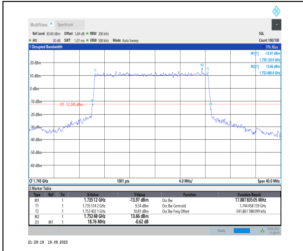
1-N66-PC3-15-20-M-2-DFT-PI2BPSK-Outer_Full-100 @0-Ant31-17.888-18.760-≤20-PASS
