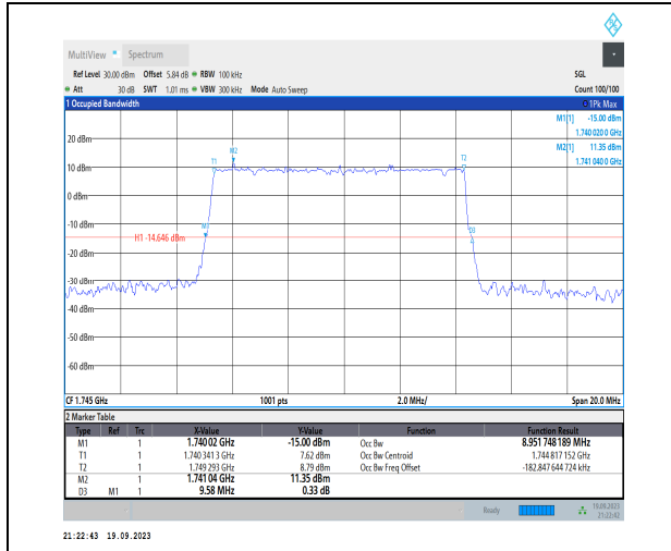
1-N66-PC3-15-10-M-4-DFT-64QAM-Outer_Full-50@ 0-Ant31-8.952-9.580-≤10-PASS
