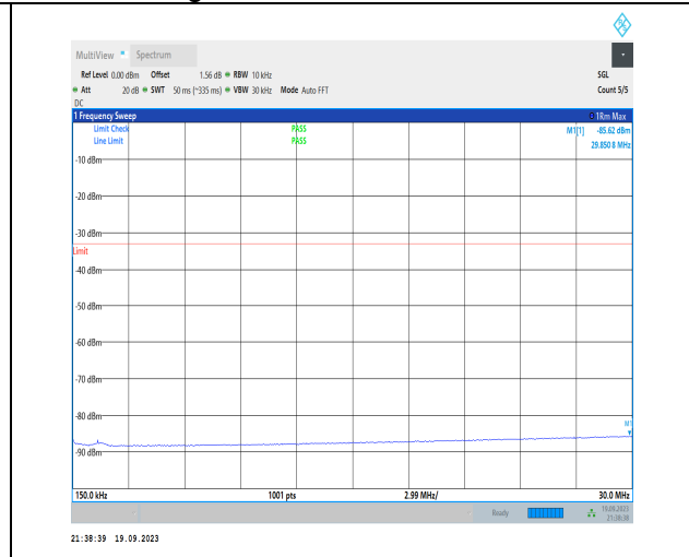
1-N66-PC3-15-40-H-1-DFT-PI2BPSK-Inner_1RB_Lef t-1@1-0.15-30-Ant31-29.85--85.62--33-PASS
