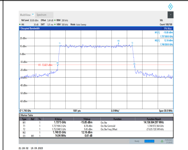
1-N66-PC3-15-15-M-6-CP-QPSK-Outer_Full-79@0- Ant31-14.136-14.940-≤15-PASS
