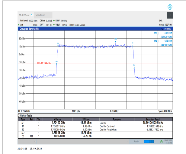
1-N66-PC3-15-40-M-4-DFT-64QAM-Outer_Full-216 @0-Ant31-38.592-40.160-<math>\leq 40</math>-PASS
