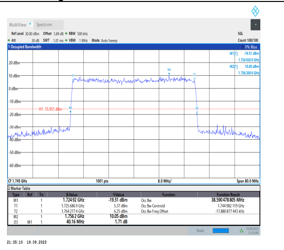
1-N66-PC3-15-40-M-9-CP-256QAM-Outer_Full-216 @0-Ant31-38.59-40.160-<40-PASS
