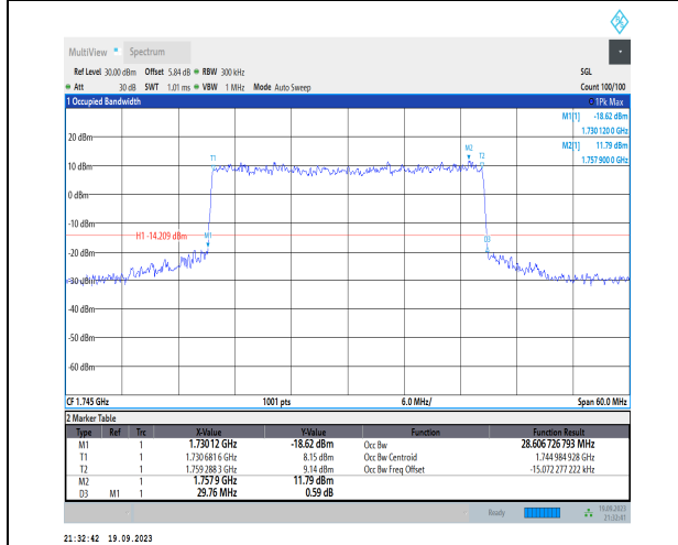
1-N66-PC3-15-30-M-7-CP-16QAM-Outer_Full-160@0-Ant31-28.607-29.760-≤30-PASS
