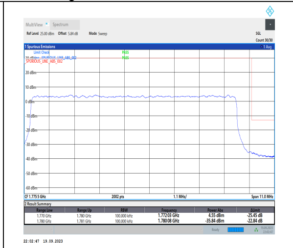
1-N66-PC3-15-10-H-3-DFT-PI2BPSK-Outer_Full-5 0@0-Ant31-1-seegraph-PASS-see graph
