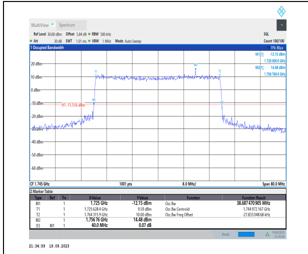
1-N66-PC3-15-40-M-8-CP-64QAM-Outer_Full-216@ 0-Ant31-38.687-40.000-<40-PASS
