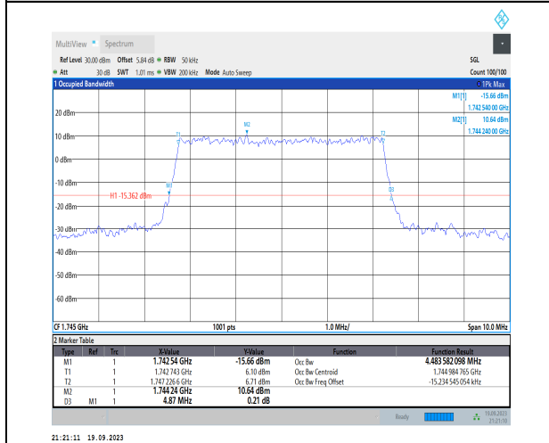
1-N66-PC3-15-5-M-7-CP-16QAM-Outer_Full-25@0- Ant31-4.484-4.870- \leq 5-PASS
