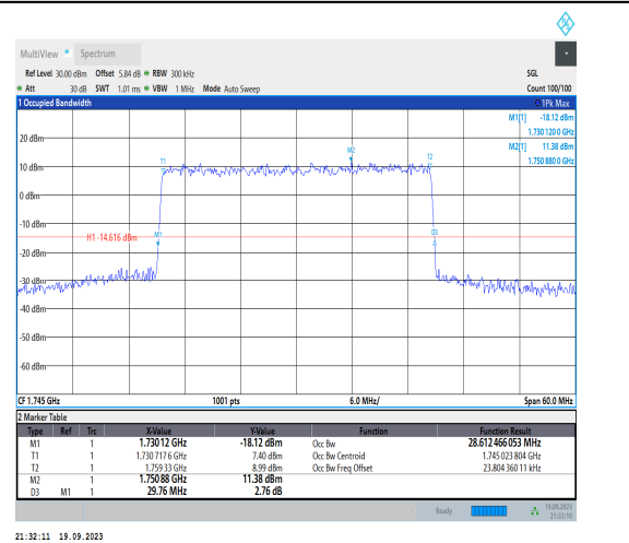
1-N66-PC3-15-30-M-4-DFT-64QAM-Outer_Full-160@0-Ant31-28.612-29.760-≤30-PASS
