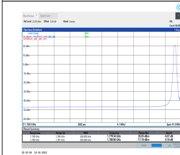
1-N66-PC3-15-40-H-5-CP-QPSK-Edge_1RB_Right-1 @215-Ant31-1-seegraph-PASS-see graph
