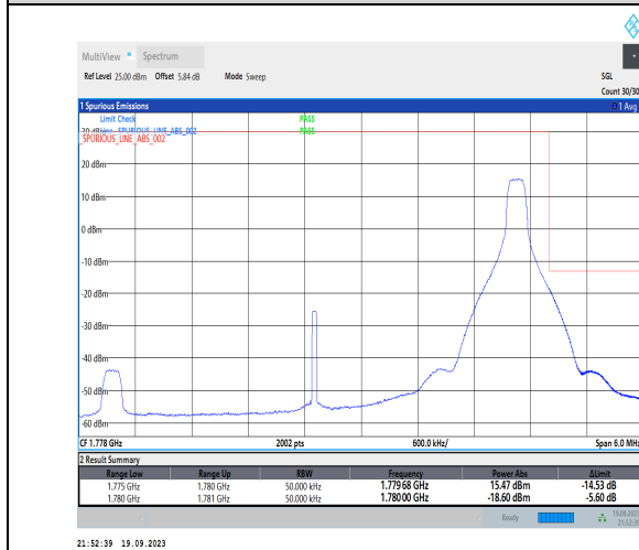
1-N66-PC3-15-5-H-5-CP-QPSK-Edge_1RB_Right-1@24-Ant31-1-seegraph-PASS-see graph
