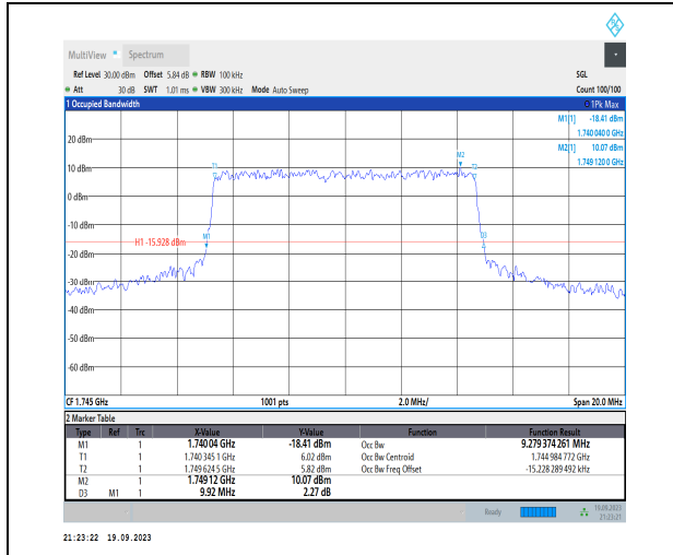
1-N66-PC3-15-10-M-8-CP-64QAM-Outer_Full-52@0 -Ant31-9.279-9.920-≤10-PASS
