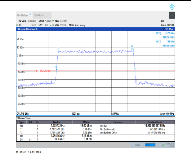
1-N66-PC3-15-20-M-9-CP-256QAM-Outer_Full-106@0 @0-Ant31-18.927-19.800-≤20-PASS
