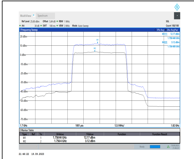
1-N66-PC3-15-40-H-1-DFT-256QAM-Outer_Full-216 @0-Ant31-9.05-100%-0.00-9.05-PASS<math>\leq 13</math>
