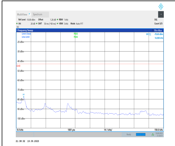
1-N66-PC3-15-40-H-1-DFT-PI2BPSK-Inner_1RB_L eft-1@1-0.009-0.15-Ant31-0.16--78.60--43-PASS
