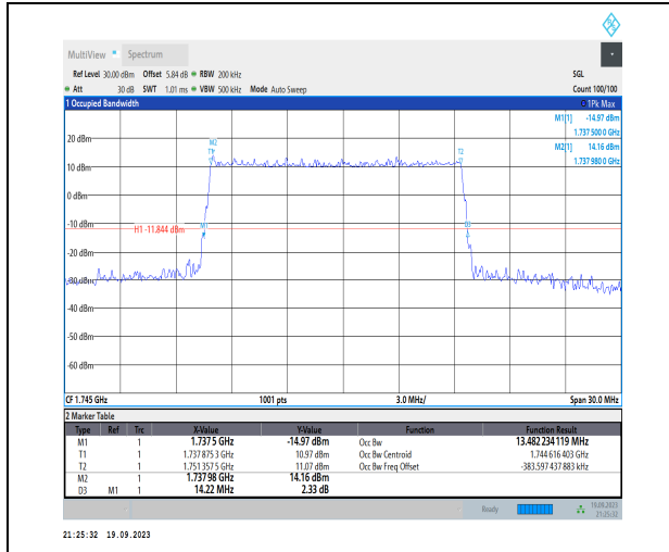
1-N66-PC3-15-15-M-3-DFT-16QAM-Outer_Full-75@ 0-Ant31-13.482-14.220-≤15-PASS
