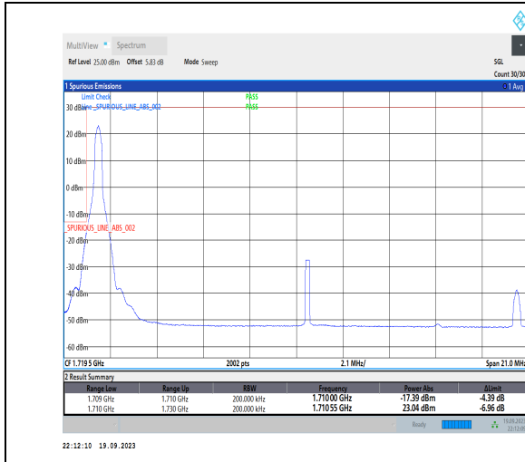
1-N66-PC3-15-20-L-1-DFT-PI2BPSK-Edge_1RB_Left-1@0-Ant31-1-seegraph-PASS-see graph
