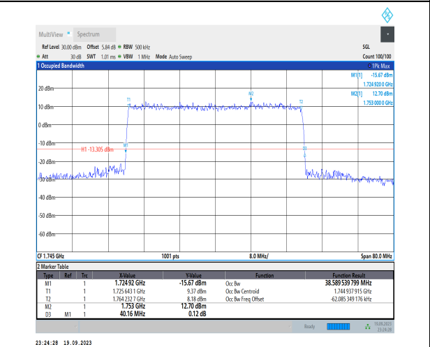
1-N66-PC3-15-40-M-3-DFT-16QAM-Outer_Full-216 @0-Ant31-38.59-40.160-≤40-PASS
