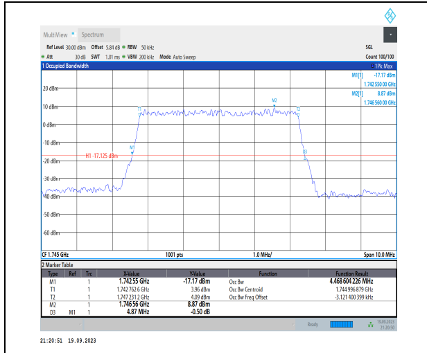
1-N66-PC3-15-5-M-5-DFT-256QAM-Outer_Full-25@ 0-Ant31-4.469-4.870- \leq 5-PASS
