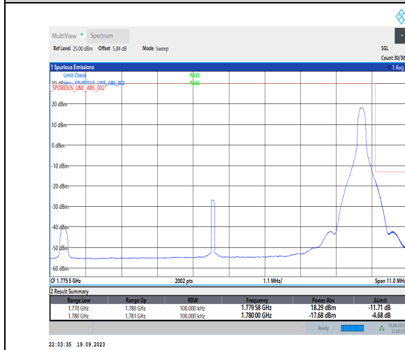
1-N66-PC3-15-10-H-5-CP-QPSK-Edge_1RB_Right-1 @51-Ant31-1-seegraph-PASS-see graph
