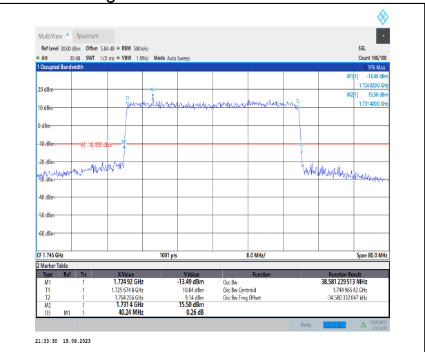
1-N66-PC3-15-40-M-1-DFT-QPSK-Outer_Full-216@ 0-Ant31-38.581-40.240-≤40-PASS
