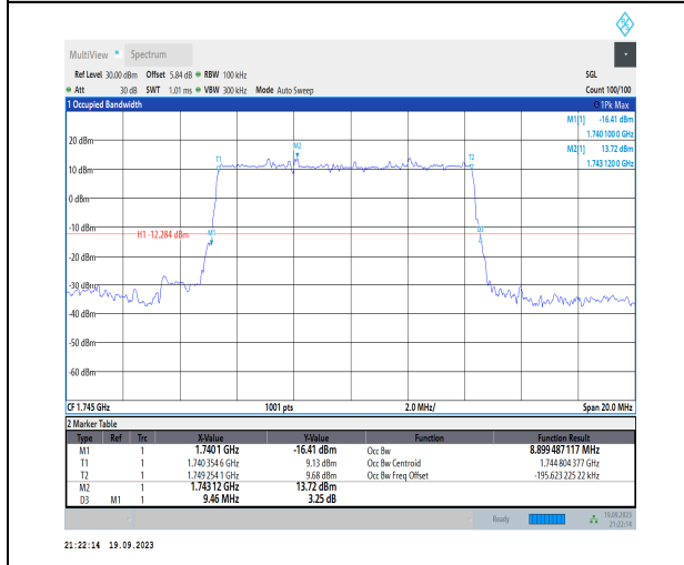
1-N66-PC3-15-10-M-2-DFT-PI2BPSK-Outer_Full-50 @0-Ant31-8.899-9.460-≤10-PASS
