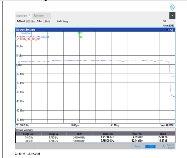
1-N66-PC3-15-40-H-3-DFT-PI2BPSK-Outer_Full-2 16@0-Ant31-1-seegraph-PASS-see graph
