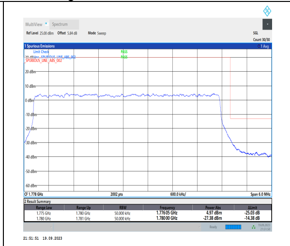
1-N66-PC3-15-5-H-3-DFT-PI2BPSK-Outer_Full-25@0-Ant31-1-seegraph-PASS-see graph
