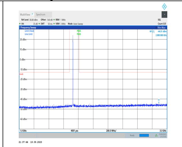
1-N66-PC3-15-40-M-1-DFT-PI2BPSK-Inner_1RB_Lef t-1@1-1000-3000-Ant31-2890.00--44.31--13-PASS
