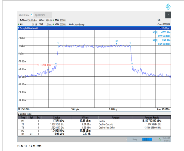
1-N66-PC3-15-15-M-7-CP-16QAM-Outer_Full-79@0 -Ant31-14.12-14.910-≤15-PASS
