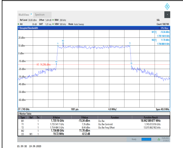
1-N66-PC3-15-20-M-8-CP-64QAM-Outer_Full-106@0 0-Ant31-18.943-19.720-≤20-PASS
