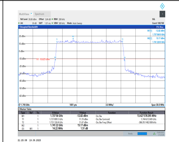
1-N66-PC3-15-15-M-2-DFT-PI2BPSK-Outer_Full-75@0 @0-Ant31-13.428-14.220-≤15-PASS
