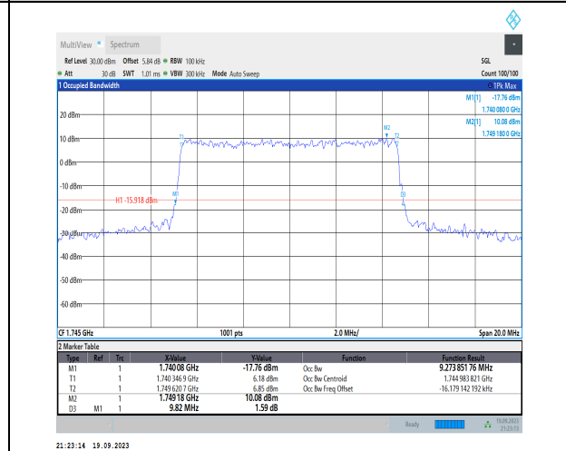
1-N66-PC3-15-10-M-7-CP-16QAM-Outer_Full-52@0 -Ant31-9.274-9.820-≤10-PASS
