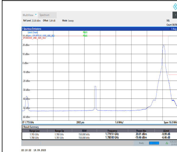
1-N66-PC3-15-15-H-5-CP-QPSK-Edge_1RB_Right-1 @78-Ant31-1-seegraph-PASS-see graph
