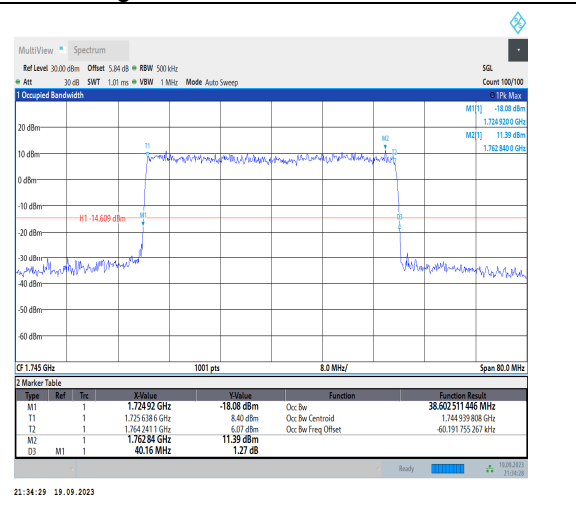
1-N66-PC3-15-40-M-5-DFT-256QAM-Outer_Full-216 @0-Ant31-38.603-40.160-<math>\leq 40</math>-PASS
