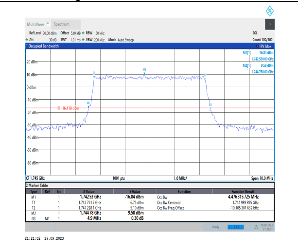
1-N66-PC3-15-5-M-6-CP-QPSK-Outer_Full-25@0-A nt31-4.476-4.900- \leq 5-PASS
