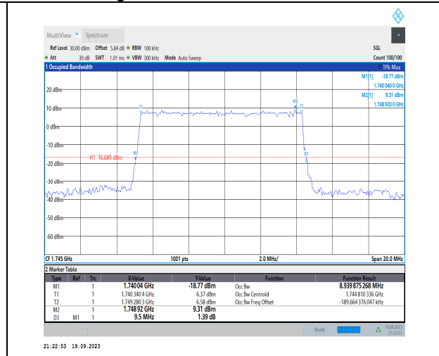
1-N66-PC3-15-10-M-5-DFT-256QAM-Outer_Full-50 @0-Ant31-8.94-9.500-≤10-PASS
