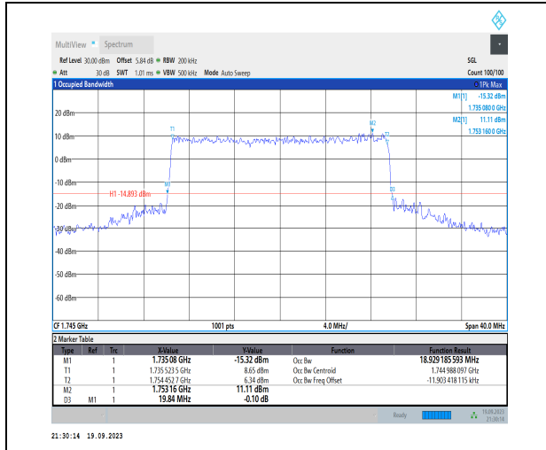
1-N66-PC3-15-20-M-6-CP-QPSK-Outer_Full-106@0 -Ant31-18.929-19.840-≤20-PASS
