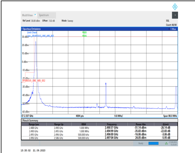
1-N41-PC2-30-90-L-1-DFT-PI2BPSK-Edge_1RB_Left-1@0-Ant11-1--PASS-see graph
