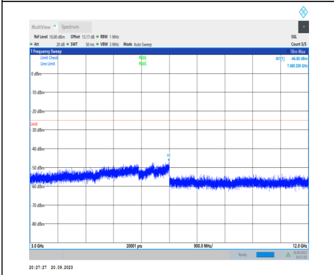
1-N41-30-100-M-1-DFT-PI2BPSK-Inner_1RB_Left-1 @ 1-3000-12000-Ant11-7480.20--46.80--25-PASS
