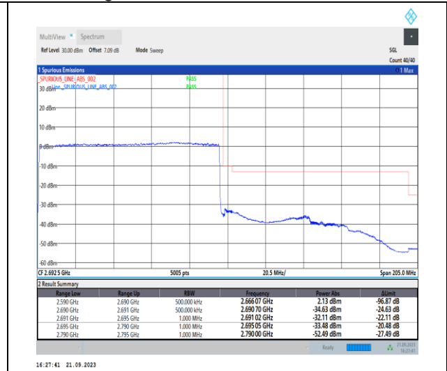
1-N41-PC2-30-100-H-3-DFT-PI2BPSK-Outer_Full-270@0-Ant11-1--PASS-see graph
