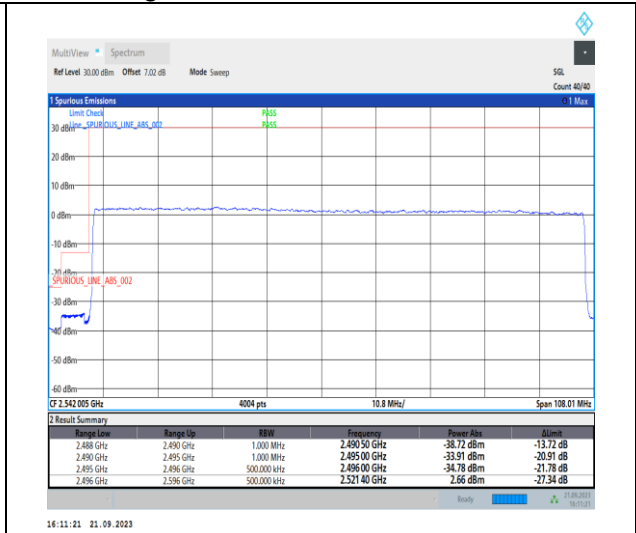
1-N41-PC2-30-100-L-3-DFT-PI2BPSK-Outer_Full-270@0-Ant11-1--PASS-see graph
