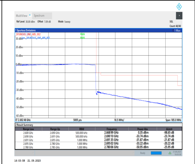
1-N41-PC2-30-90-H-6-CP-QPSK-Outer_Full-245@0-Ant11-1--PASS-see graph
