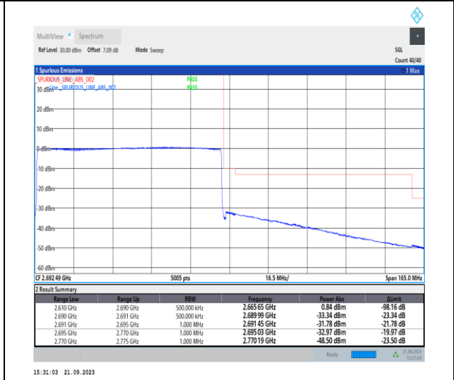
1-N41-PC2-30-80-H-6-CP-QPSK-Outer_Full-216@0-Ant11-1--PASS-see graph
