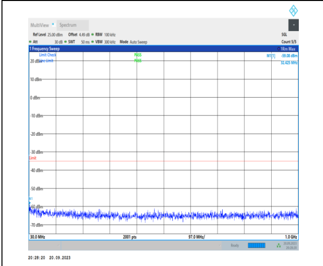
1-N41-30-100-H-1-DFT-PI2BPSK-Inner_1RB_Left-1 @1-30-1000-Ant11-32.43--59.08--35-PASS
