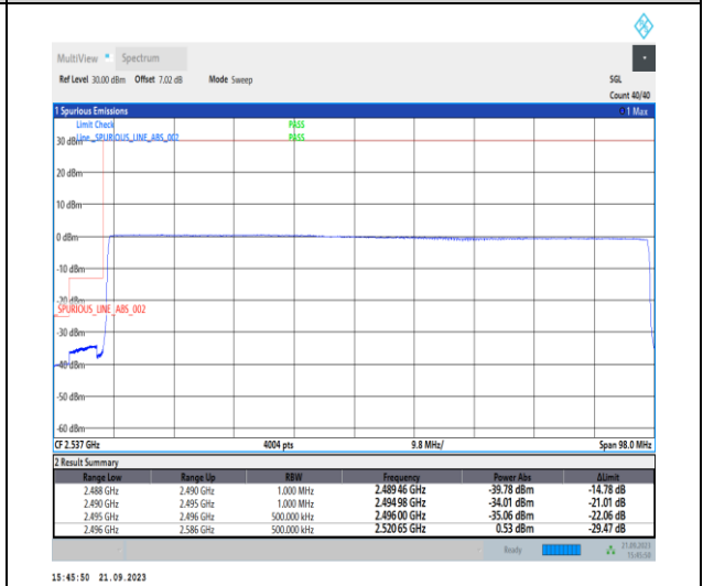
1-N41-PC2-30-90-L-6-CP-QPSK-Outer_Full-245@0-Ant11-1--PASS-see graph
