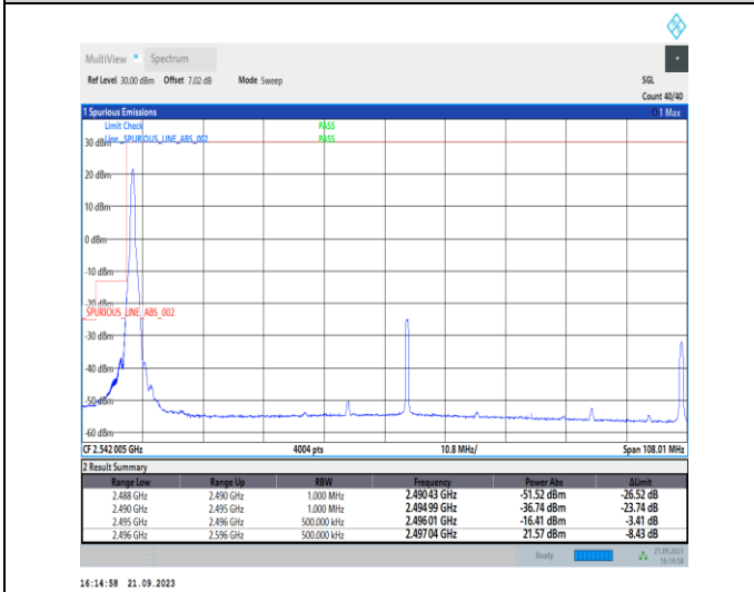
1-N41-PC2-30-100-L-4-CP-QPSK-Edge_1RB_Left-1@0-Ant11-1--PASS-see graph
