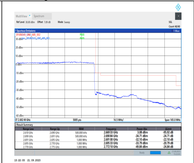
1-N41-PC2-30-80-H-3-DFT-PI2BPSK-Outer_Full-216@0-Ant11-1--PASS-see graph
