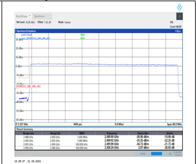
1-N41-PC2-30-90-L-3-DFT-PI2BPSK-Outer_Full-240@0-Ant11-1--PASS-see graph
