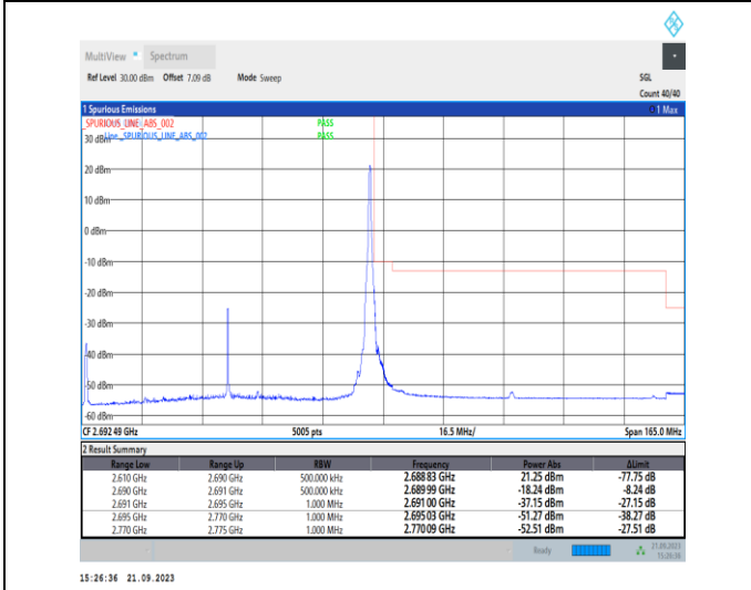
1-N41-PC2-30-80-H-5-CP-QPSK-Edge_1RB_Right-1@216-Ant11-1--PASS-see graph
