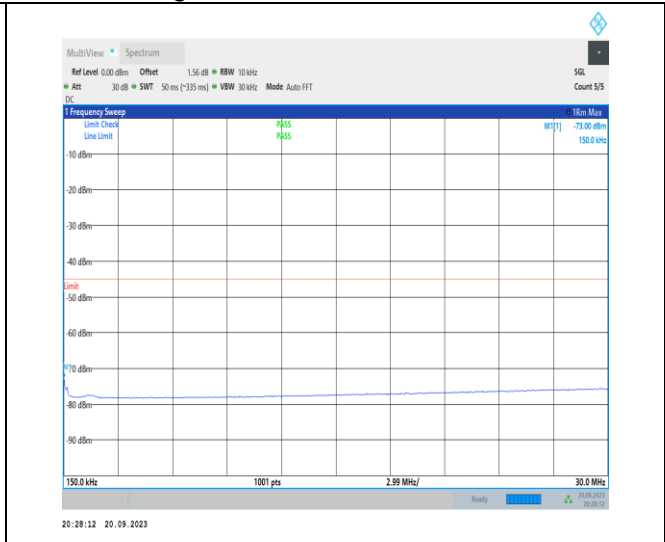
1-N41-30-100-H-1-DFT-PI2BPSK-Inner_1RB_Left-1 @1-0.15-30-Ant11-0.15--73.00--45-PASS
