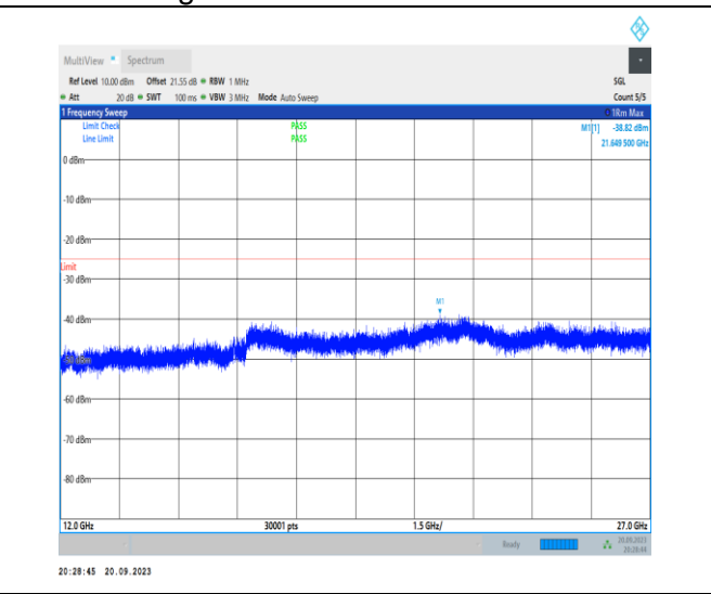
1-N41-30-100-H-1-DFT-PI2BPSK-Inner_1RB_Left-1 @1-12000-27000-Ant11-21649.50--38.82--25-PASS
