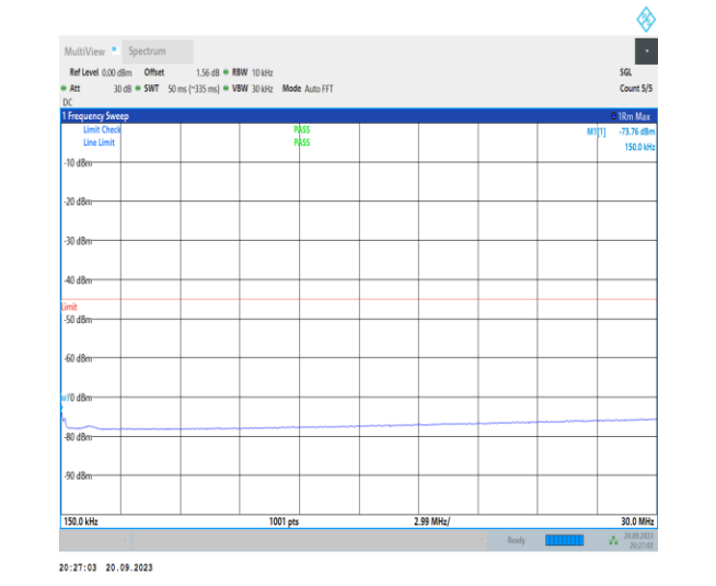
1-N41-30-100-M-1-DFT-PI2BPSK-Inner_1RB_Left-1 @ 1-0.15-30-Ant11-0.15--73.76--45-PASS
