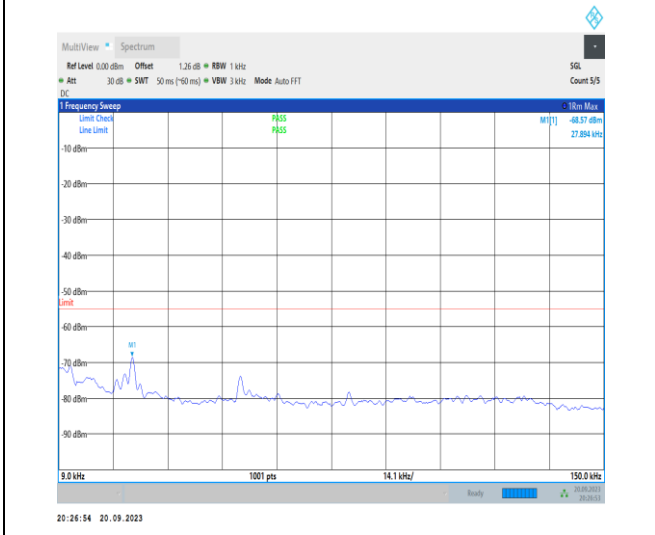
1-N41-30-100-M-1-DFT-PI2BPSK-Inner_1RB_Left-1 @ 1-0.009-0.15-Ant11-0.028--68.57--55-PASS
