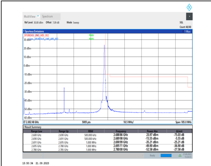
1-N41-PC2-30-90-H-2-DFT-PI2BPSK-Edge_1RB_Right-t-1@244-Ant11-1--PASS-see graph
