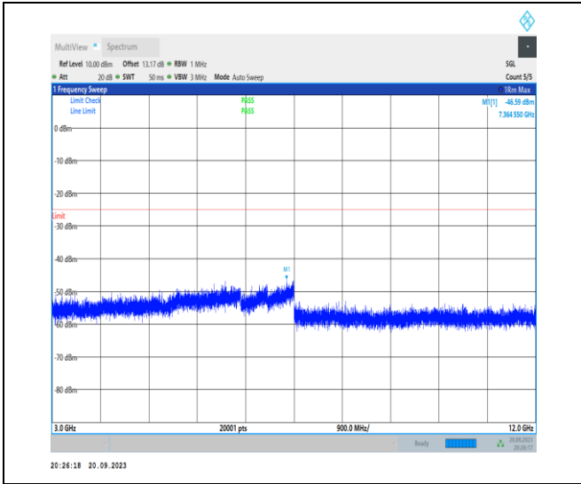
1-N41-30-100-L-1-DFT-PI2BPSK-Inner_1RB_Left-1 @ 1-3000-12000-Ant11-7364.55--46.59--25-PASS
