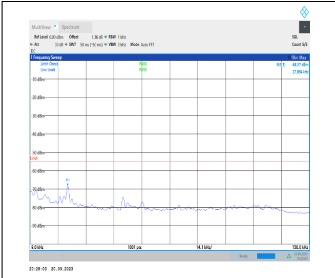
1-N41-30-100-H-1-DFT-PI2BPSK-Inner_1RB_Left-1 @1-0.009-0.15-Ant11-0.028--68.57--55-PASS
