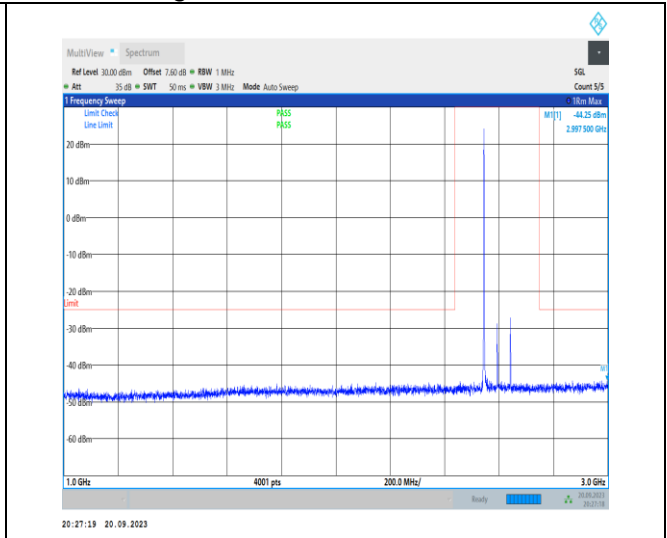
1-N41-30-100-M-1-DFT-PI2BPSK-Inner_1RB_Left-1 @ 1-1000-3000-Ant11-2997.50--44.25--25-PASS
