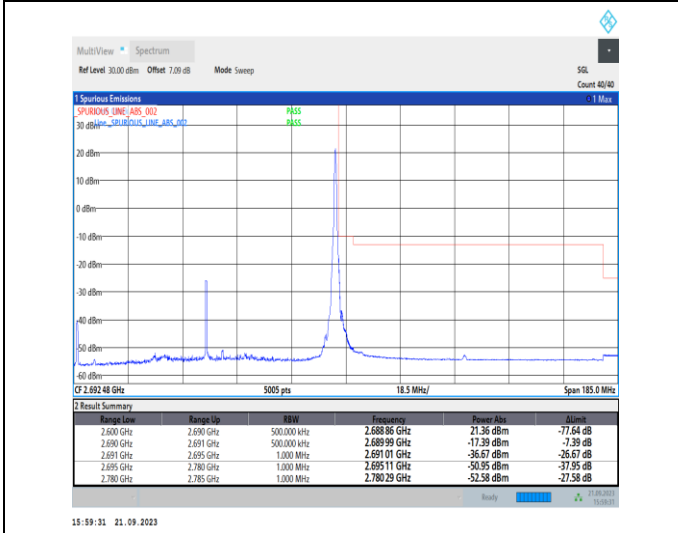
1-N41-PC2-30-90-H-5-CP-QPSK-Edge_1RB_Right-1@244-Ant11-1--PASS-see graph
