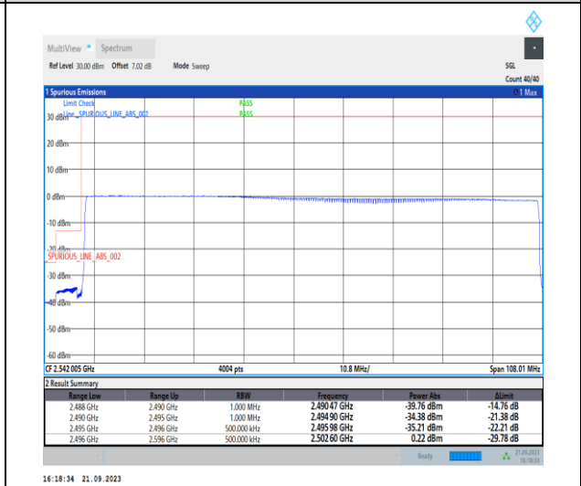
1-N41-PC2-30-100-L-6-CP-QPSK-Outer_Full-273@0-Ant11-1--PASS-see graph
