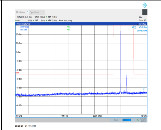
1-N41-30-100-H-1-DFT-PI2BPSK-Inner_1RB_Left-1 @1-1000-3000-Ant11-2947.5.00--43.62--25-PASS
