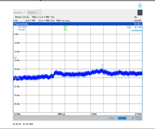
1-N41-30-100-L-1-DFT-PI2BPSK-Inner_1RB_Left-1 @ 1-12000-27000-Ant11-22379.00--39.11--25-PASS
