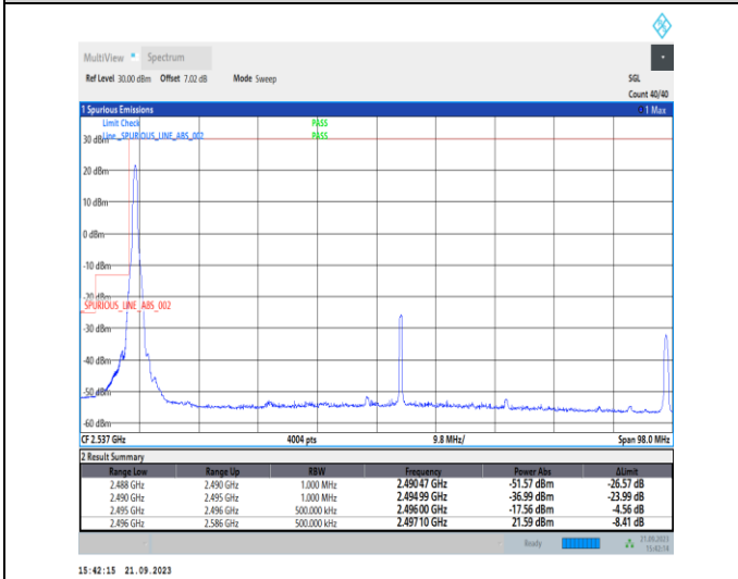
1-N41-PC2-30-90-L-4-CP-QPSK-Edge_1RB_Left-1@0-Ant11-1--PASS-see graph
