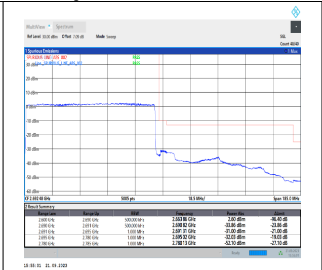
1-N41-PC2-30-90-H-3-DFT-PI2BPSK-Outer_Full-240@0-Ant11-1--PASS-see graph
