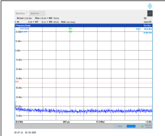
1-N41-30-100-M-1-DFT-PI2BPSK-Inner_1RB_Left-1 @ 1-30-1000-Ant11-33.88--58.50--35-PASS
