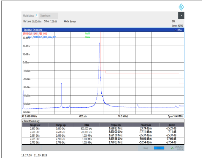
1-N41-PC2-30-80-H-2-DFT-PI2BPSK-Edge_1RB_Right-t-1@216-Ant11-1--PASS-see graph
