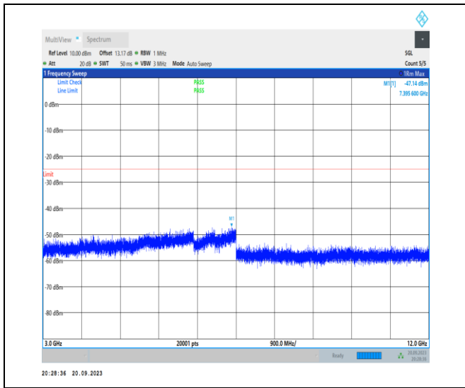
1-N41-30-100-H-1-DFT-PI2BPSK-Inner_1RB_Left-1 @1-3000-12000-Ant11-7395.6.00--47.14--25-PASS
