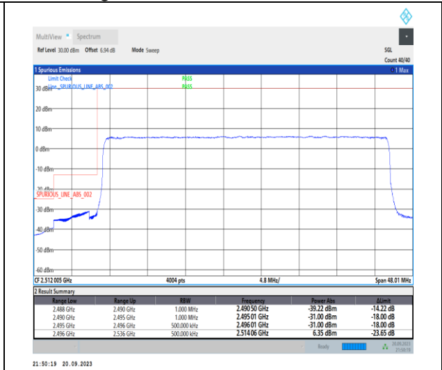
1-N41-PC2-30-40-L-3-DFT-PI2BPSK-Outer_Full-100@0-Ant11-1--PASS-see graph
