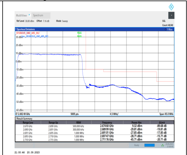
1-N41-PC2-30-20-H-3-DFT-PI2BPSK-Outer_Full-5 0@0-Ant11-1--PASS-see graph
