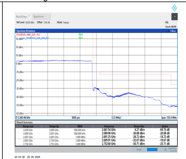
1-N41-PC2-30-60-H-3-DFT-PI2BPSK-Outer_Full-162@0-Ant11-1--PASS-see graph
