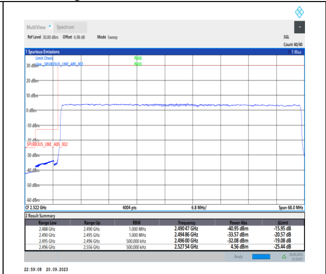
1-N41-PC2-30-60-L-3-DFT-PI2BPSK-Outer_Full-162@0-Ant11-1--PASS-see graph
