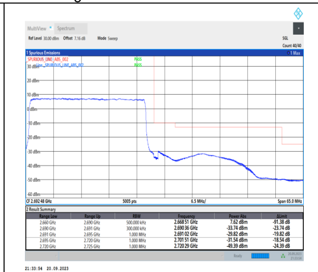
1-N41-PC2-30-30-H-3-DFT-PI2BPSK-Outer_Full-7 5@0-Ant11-1--PASS-see graph
