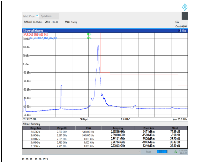
1-N41-PC2-30-40-H-2-DFT-PI2BPSK-Edge_1RB_Righ t-1@105-Ant11-1--PASS-see graph
