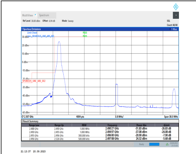
1-N41-PC2-30-30-L-1-DFT-PI2BPSK-Edge_1RB_Left-1@0-Ant11-1--PASS-see graph
