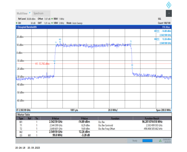
1-N41-PC2-30-100-M-4-DFT-64QAM-Outer_Full-270 @0-Ant11-96.202-99.800-≤100-PASS
