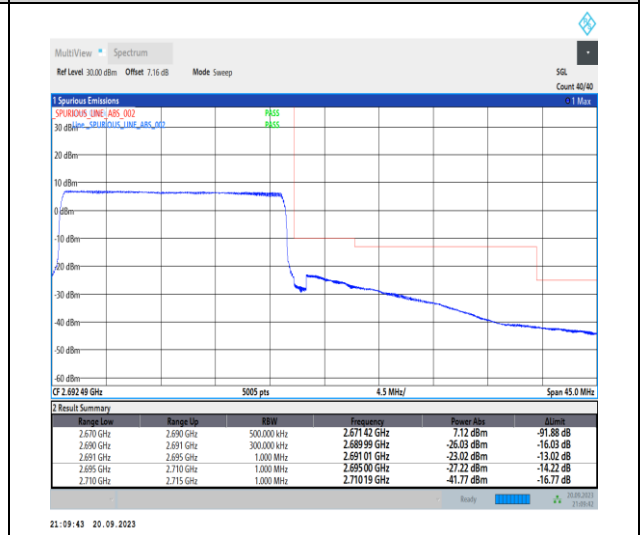
1-N41-PC2-30-20-H-6-CP-QPSK-Outer_Full-51 @0-Ant11-1--PASS-see graph
