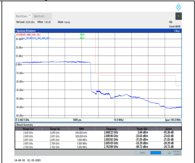
1-N41-PC2-30-70-H-3-DFT-PI2BPSK-Outer_Full-1 80@0-Ant11-1--PASS-see graph
