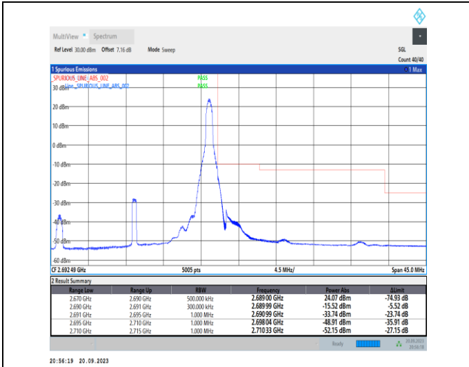
1-N41-PC2-30-20-H-2-DFT-PI2BPSK-Edge_1RB_Righ t-1@50-Ant11-1--PASS-see graph
