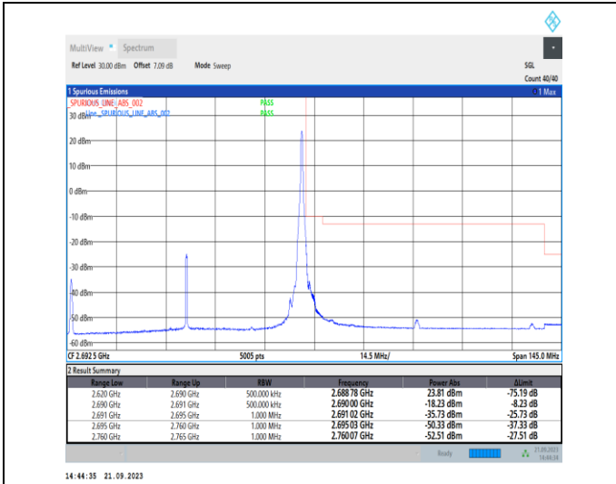
1-N41-PC2-30-70-H-2-DFT-PI2BPSK-Edge_1RB_Righ t-1@188-Ant11-1--PASS-see graph
