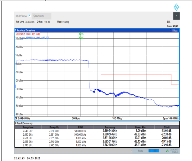
1-N41-PC2-30-50-H-3-DFT-PI2BPSK-Outer_Full-1 28@0-Ant11-1--PASS-see graph
