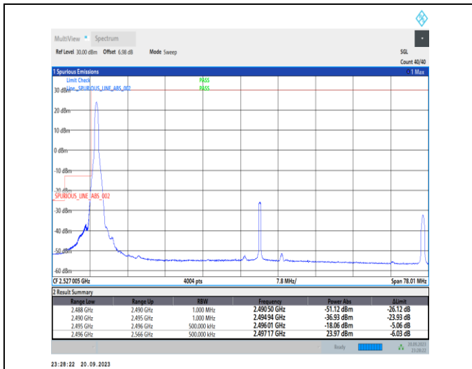
1-N41-PC2-30-70-L-1-DFT-PI2BPSK-Edge_1RB_Left-1@0-Ant11-1--PASS-see graph
