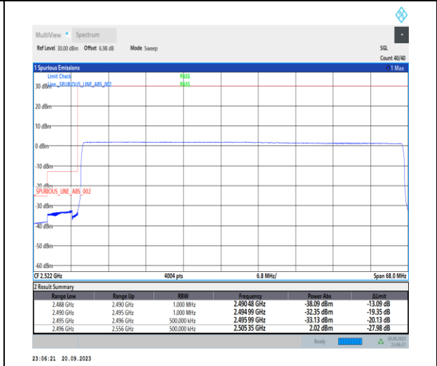
1-N41-PC2-30-60-L-6-CP-QPSK-Outer_Full-162@0-Ant11-1--PASS-see graph
