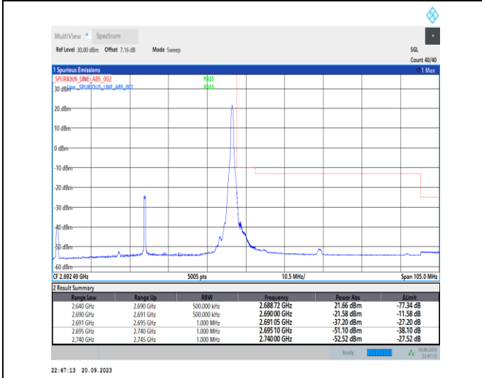
1-N41-PC2-30-50-H-5-CP-QPSK-Edge_1RB_Righ t-1 @132-Ant11-1--PASS-see graph
