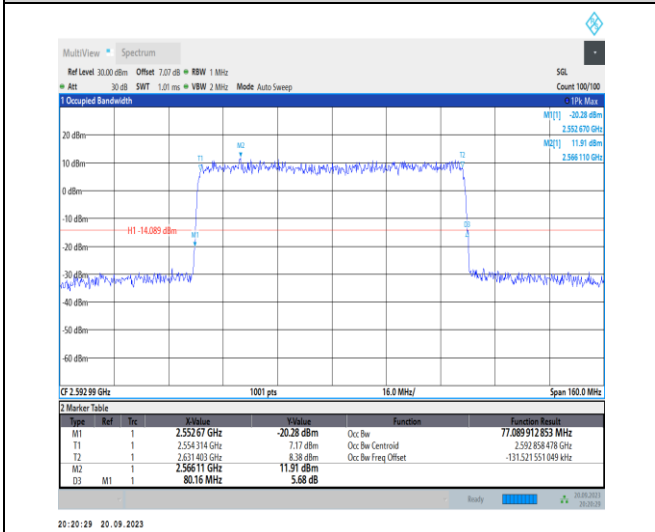
1-N41-PC2-30-80-M-5-DFT-256QAM-Outer_Full-216 @0-Ant11-77.09-80.160-≤80-PASS
