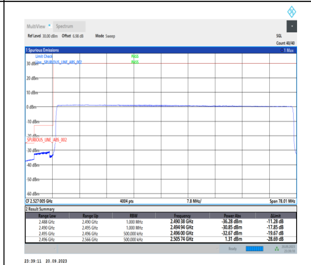
1-N41-PC2-30-70-L-6-CP-QPSK-Outer_Full-189@0-Ant11-1--PASS-see graph
