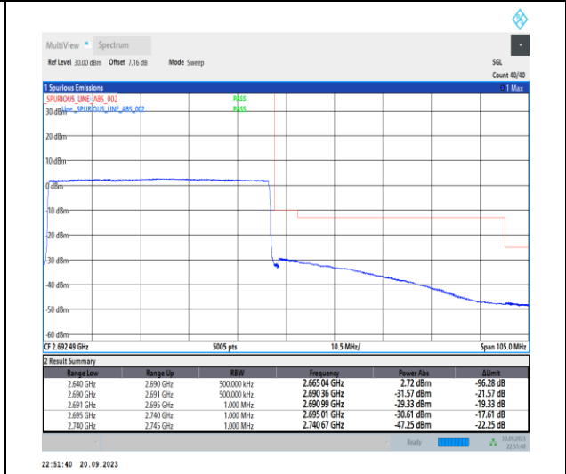
1-N41-PC2-30-50-H-6-CP-QPSK-Outer_Full-133 @0-Ant11-1--PASS-see graph
