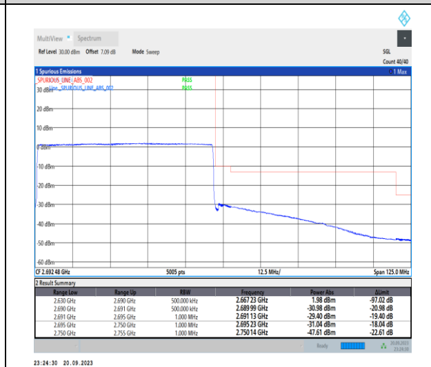
1-N41-PC2-30-60-H-6-CP-QPSK-Outer_Full-162@0-Ant11-1--PASS-see graph
