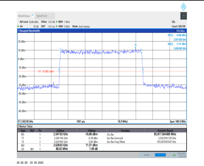
1-N41-PC2-30-90-M-5-DFT-256QAM-Outer_Full-240 @0-Ant11-85.817-88.920-≤90-PASS
