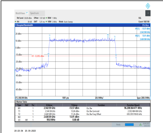
1-N41-PC2-30-100-M-1-DFT-QPSK-Outer_Full-270 @0-Ant11-96.208-99.800-≤100-PASS
