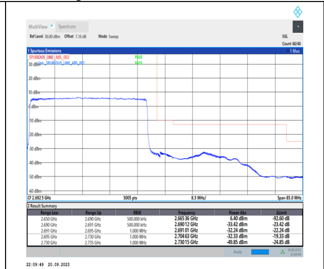
1-N41-PC2-30-40-H-3-DFT-PI2BPSK-Outer_Full-1 00@0-Ant11-1--PASS-see graph
