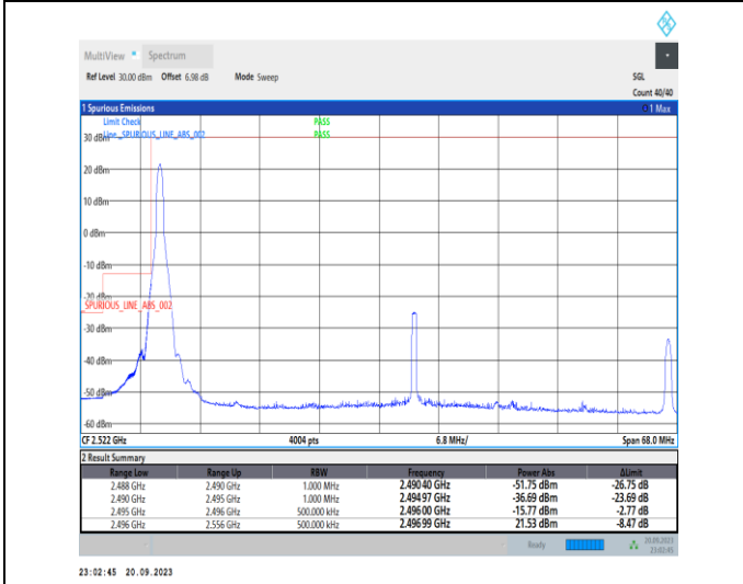
1-N41-PC2-30-60-L-4-CP-QPSK-Edge_1RB_Left-1@0-Ant11-1--PASS-see graph
