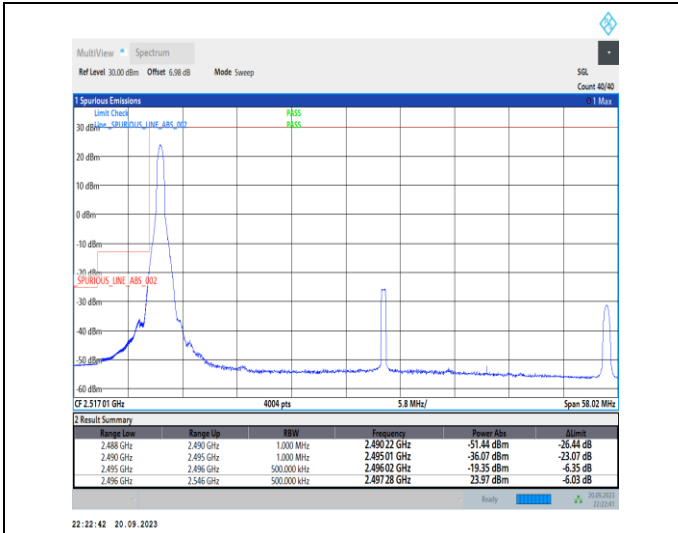
1-N41-PC2-30-50-L-1-DFT-PI2BPSK-Edge_1RB_Left-1@0-Ant11-1--PASS-see graph
