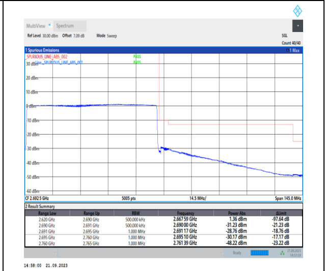
1-N41-PC2-30-70-H-6-CP-QPSK-Outer_Full-189 @0-Ant11-1--PASS-see graph
