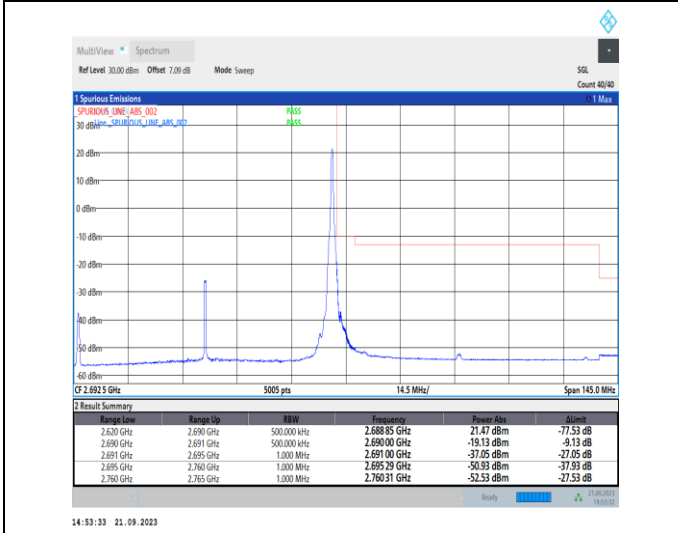
1-N41-PC2-30-70-H-5-CP-QPSK-Edge_1RB_Righ t-1@188-Ant11-1--PASS-see graph
