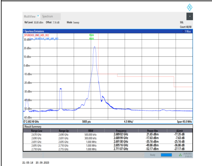
1-N41-PC2-30-20-H-5-CP-QPSK-Edge_1RB_Righ t-1@50-Ant11-1--PASS-see graph
