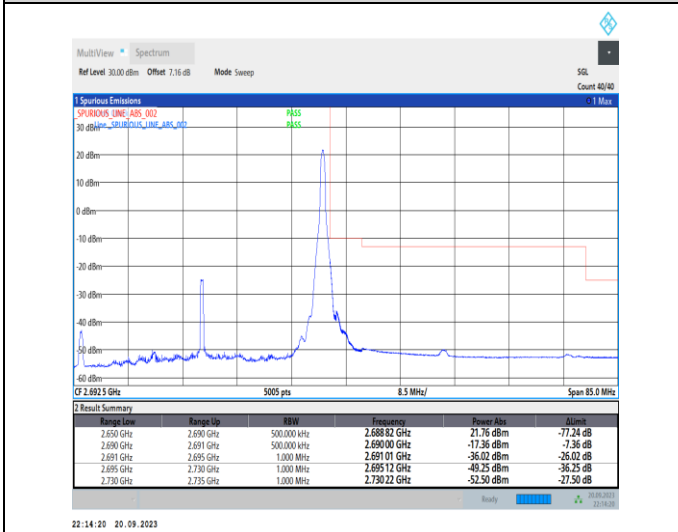
1-N41-PC2-30-40-H-5-CP-QPSK-Edge_1RB_Righ t-1@105-Ant11-1--PASS-see graph
