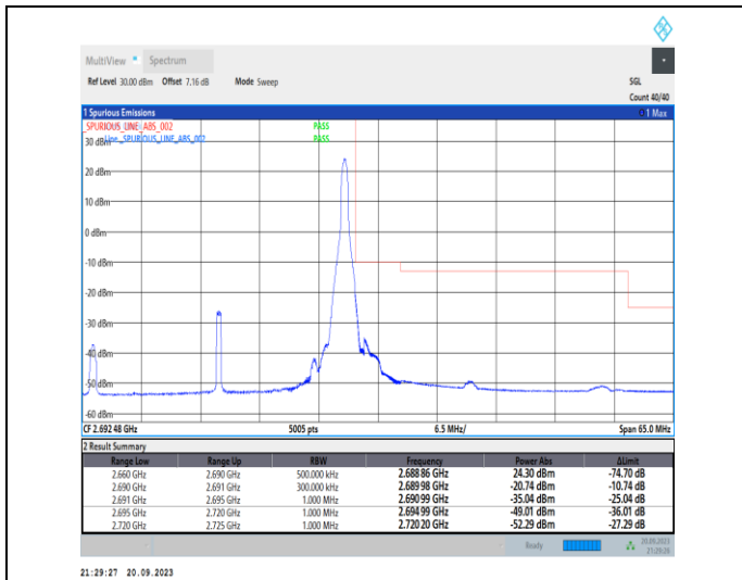
1-N41-PC2-30-30-H-2-DFT-PI2BPSK-Edge_1RB_Righ t-1@77-Ant11-1--PASS-see graph
