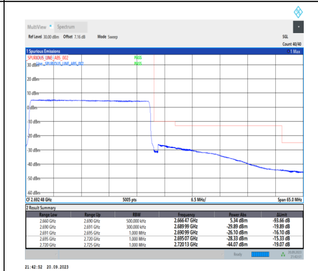
1-N41-PC2-30-30-H-6-CP-QPSK-Outer_Full-78@ 0-Ant11-1--PASS-see graph
