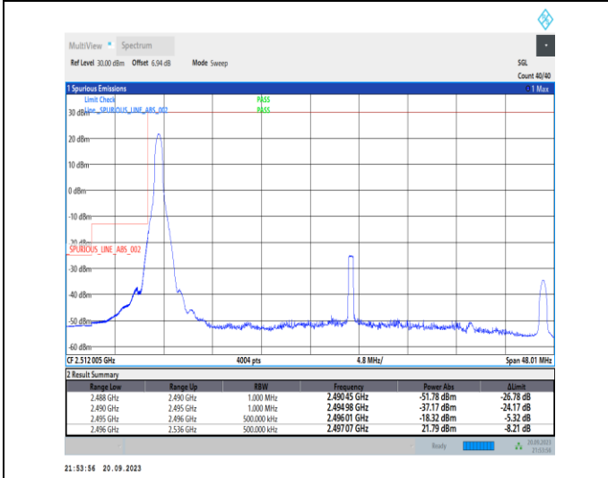
1-N41-PC2-30-40-L-4-CP-QPSK-Edge_1RB_Left-1@0-Ant11-1--PASS-see graph
