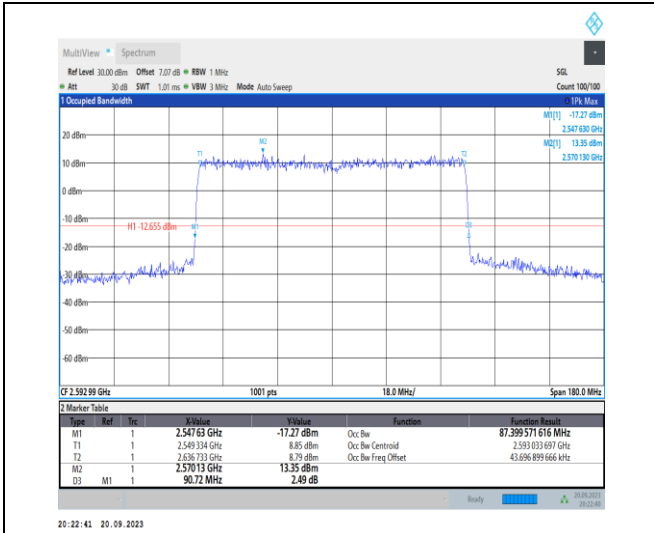
1-N41-PC2-30-90-M-6-CP-QPSK-Outer_Full-245@0 -Ant11-87.4-90.720-≤90-PASS
