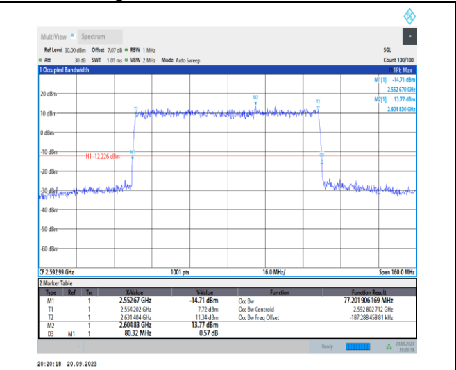
1-N41-PC2-30-80-M-4-DFT-64QAM-Outer_Full-216 @0-Ant11-77.202-80.320-≤80-PASS
