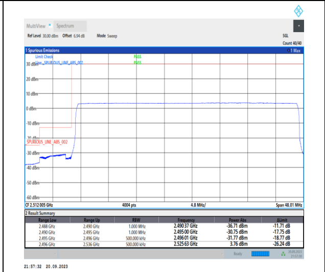
1-N41-PC2-30-40-L-6-CP-QPSK-Outer_Full-106@0-Ant11-1--PASS-see graph
