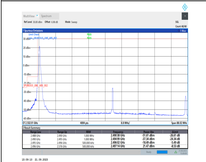
1-N41-PC2-30-80-L-4-CP-QPSK-Edge_1RB_Left-1@0-Ant11-1--PASS-see graph
