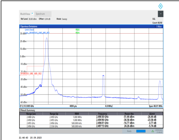
1-N41-PC2-30-40-L-1-DFT-PI2BPSK-Edge_1RB_Left-1@0-Ant11-1--PASS-see graph
