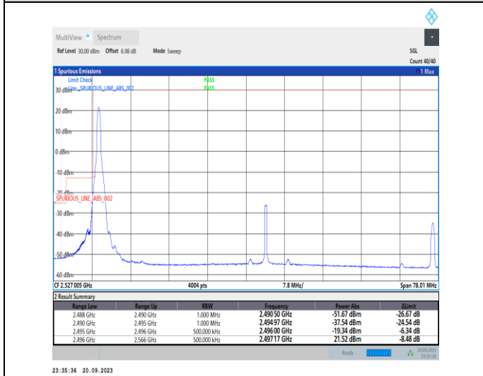
1-N41-PC2-30-70-L-4-CP-QPSK-Edge_1RB_Left-1@0-Ant11-1--PASS-see graph
