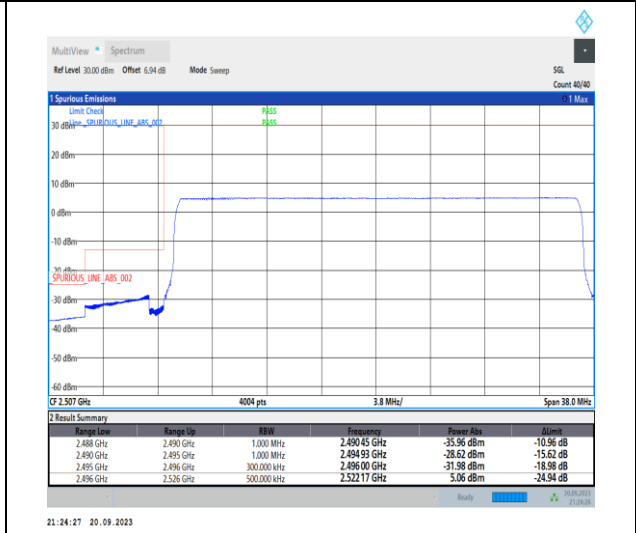
1-N41-PC2-30-30-L-6-CP-QPSK-Outer_Full-78@0-Ant11-1--PASS-see graph
