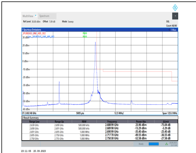
1-N41-PC2-30-60-H-2-DFT-PI2BPSK-Edge_1RB_Right-t-1@161-Ant11-1--PASS-see graph
