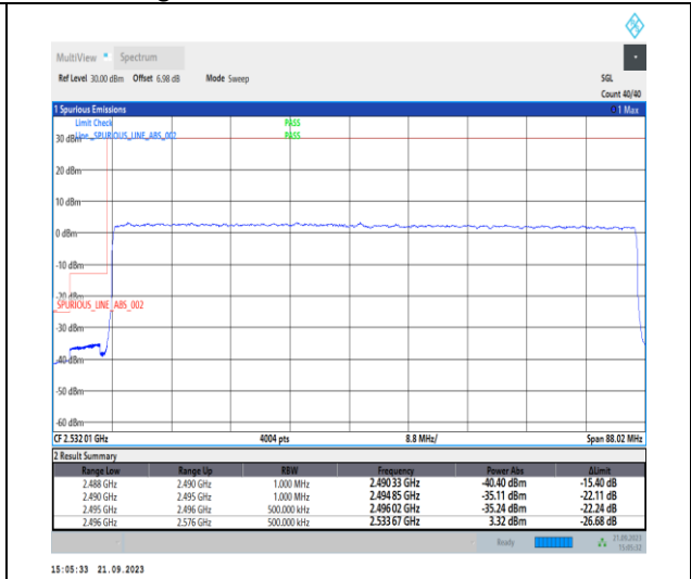
1-N41-PC2-30-80-L-3-DFT-PI2BPSK-Outer_Full-216@0-Ant11-1--PASS-see graph
