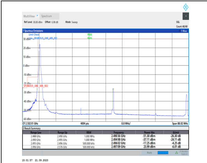
1-N41-PC2-30-80-L-1-DFT-PI2BPSK-Edge_1RB_Left-1@0-Ant11-1--PASS-see graph
