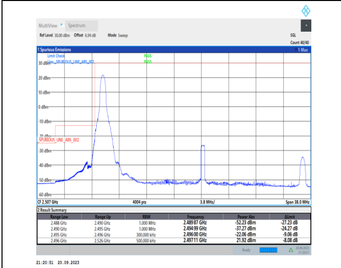
1-N41-PC2-30-30-L-4-CP-QPSK-Edge_1RB_Left-1@0-Ant11-1--PASS-see graph
