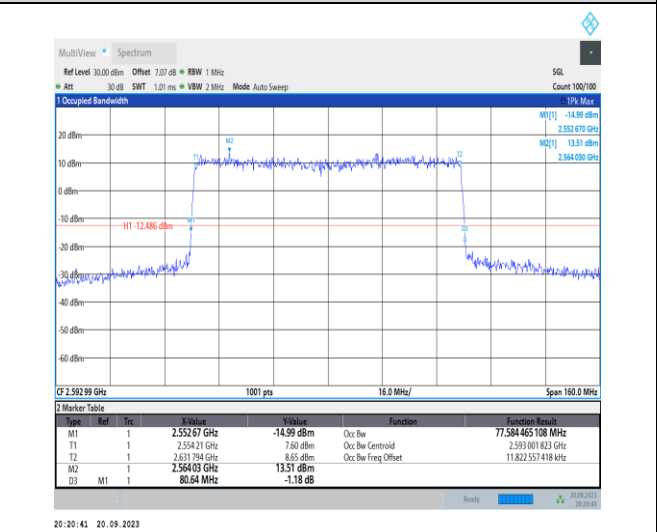
1-N41-PC2-30-80-M-6-CP-QPSK-Outer_Full-217@0 -Ant11-77.584-80.640-≤80-PASS
