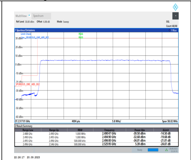
1-N41-PC2-30-50-L-3-DFT-PI2BPSK-Outer_Full-128@0-Ant11-1--PASS-see graph
