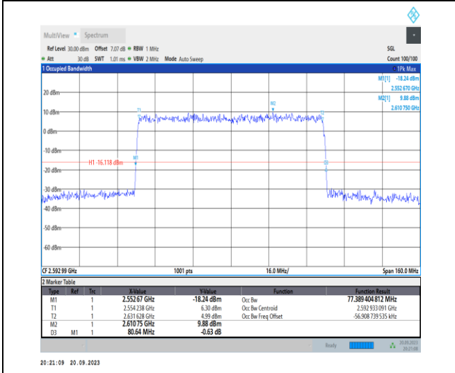
1-N41-PC2-30-80-M-9-CP-256QAM-Outer_Full-217 @0-Ant11-77.389-80.640-≤80-PASS
