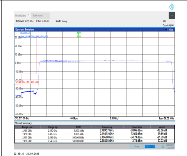
1-N41-PC2-30-50-L-6-CP-QPSK-Outer_Full-133@0-Ant11-1--PASS-see graph
