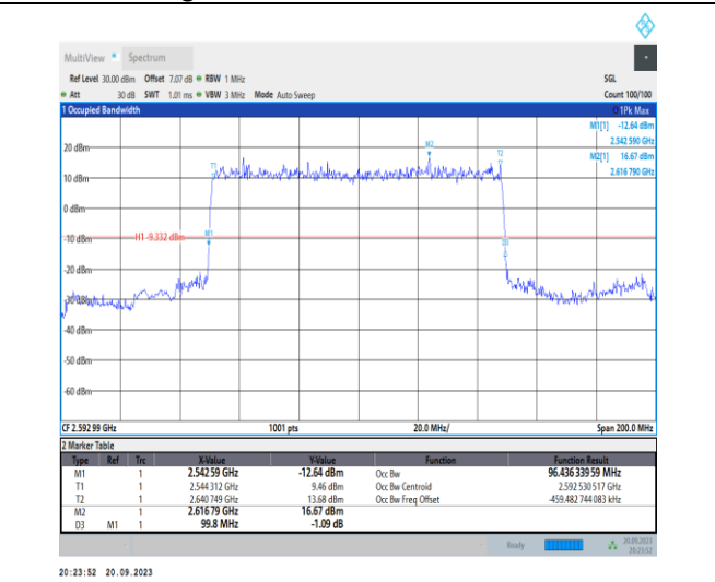
1-N41-PC2-30-100-M-2-DFT-PI2BPSK-Outer_Full-270 @0-Ant11-96.436-99.800-≤100-PASS
