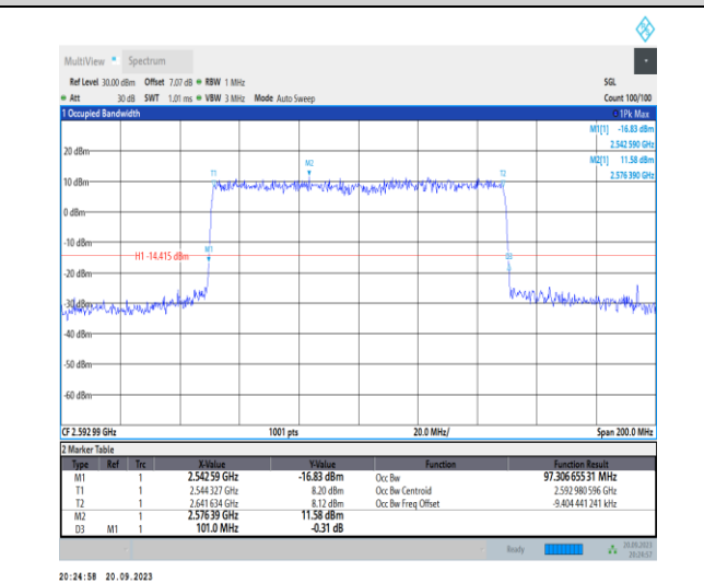
1-N41-PC2-30-100-M-8-CP-64QAM-Outer_Full-273@0-Ant11-97.307-101.000-≤100-PASS
