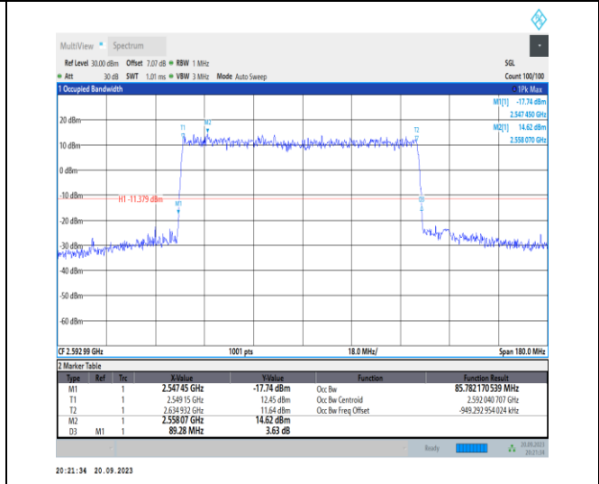
1-N41-PC2-30-90-M-1-DFT-QPSK-Outer_Full-240@ 0-Ant11-85.782-89.280-≤90-PASS
