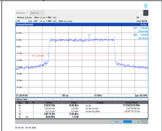
1-N41-PC2-30-80-M-8-CP-64QAM-Outer_Full-217@ 0-Ant11-77.319-80.640-≤80-PASS
