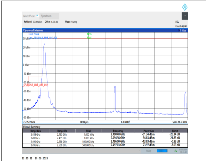
1-N41-PC2-30-60-L-1-DFT-PI2BPSK-Edge_1RB_Left-1@0-Ant11-1--PASS-see graph
