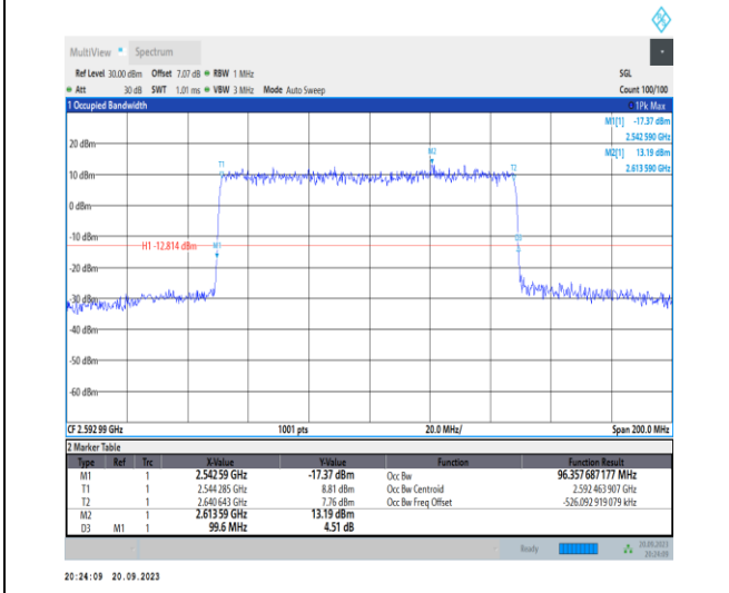
1-N41-PC2-30-100-M-3-DFT-16QAM-Outer_Full-270 @0-Ant11-96.358-99.600-≤100-PASS
