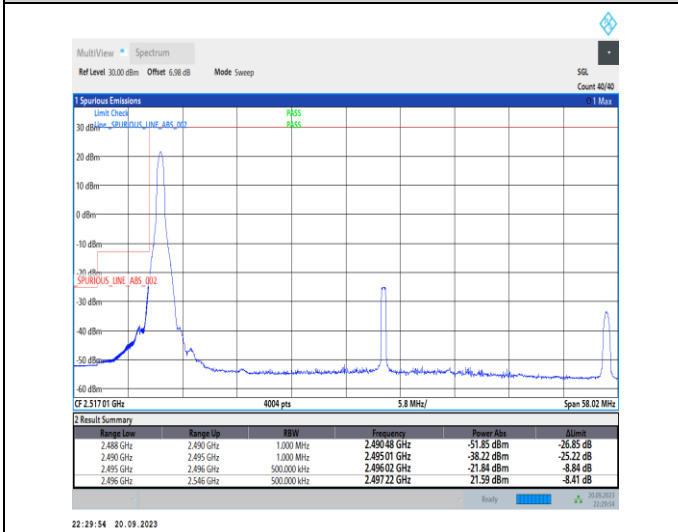
1-N41-PC2-30-50-L-4-CP-QPSK-Edge_1RB_Left-1@0-Ant11-1--PASS-see graph
