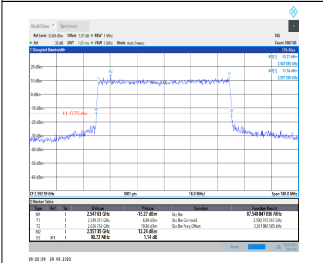
1-N41-PC2-30-90-M-8-CP-64QAM-Outer_Full-245@0-Ant11-87.549-90.720-≤90-PASS
