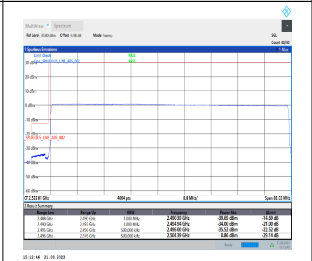
1-N41-PC2-30-80-L-6-CP-QPSK-Outer_Full-217@0-Ant11-1--PASS-see graph
