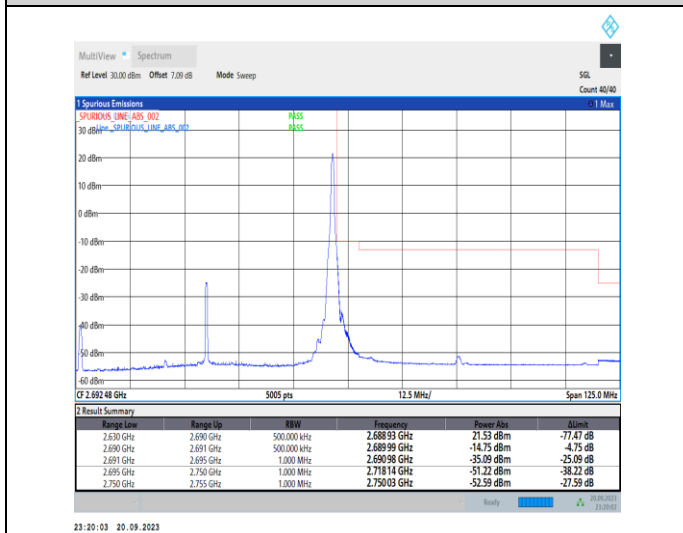
1-N41-PC2-30-60-H-5-CP-QPSK-Edge_1RB_Right-1@161-Ant11-1--PASS-see graph
