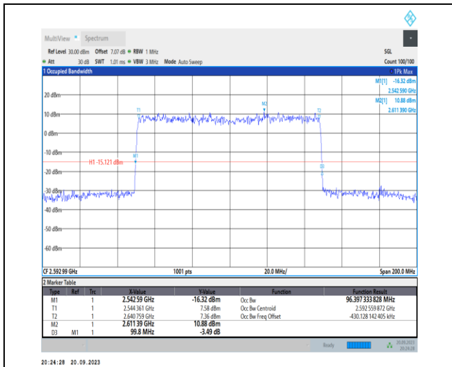
1-N41-PC2-30-100-M-5-DFT-256QAM-Outer_Full-270@0-Ant11-96.397-99.800-≤100-PASS
