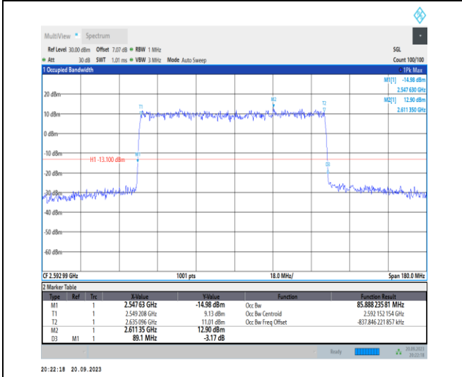
1-N41-PC2-30-90-M-4-DFT-64QAM-Outer_Full-240 @0-Ant11-85.888-89.100-≤90-PASS
