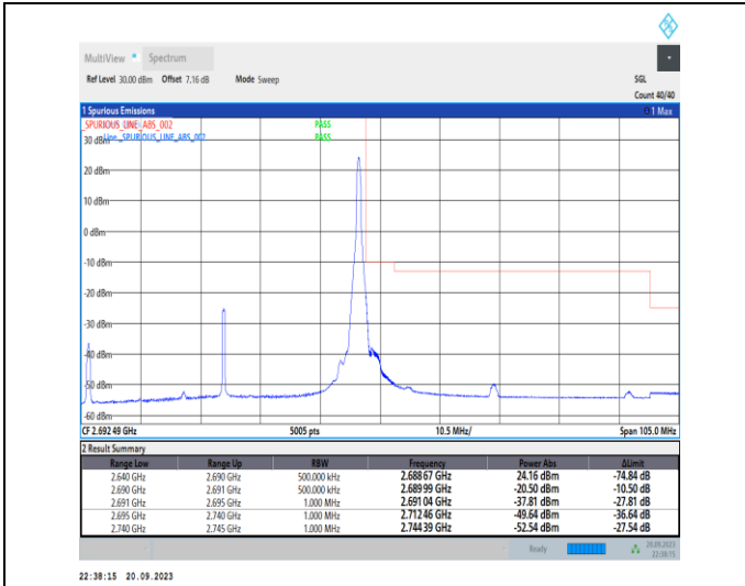
1-N41-PC2-30-50-H-2-DFT-PI2BPSK-Edge_1RB_Righ t-1@132-Ant11-1--PASS-see graph
