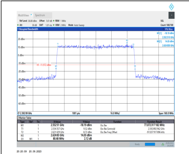
1-N41-PC2-30-80-M-3-DFT-16QAM-Outer_Full-216 @0-Ant11-77.072-80.480-≤80-PASS
