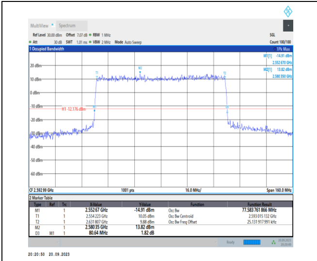
1-N41-PC2-30-80-M-7-CP-16QAM-Outer_Full-217@ 0-Ant11-77.584-80.640-≤80-PASS
