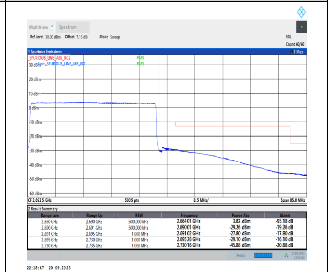
1-N41-PC2-30-40-H-6-CP-QPSK-Outer_Full-106 @0-Ant11-1--PASS-see graph
