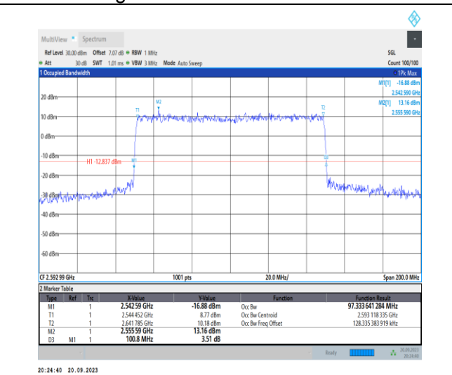
1-N41-PC2-30-100-M-6-CP-QPSK-Outer_Full-273@0-Ant11-97.334-100.800-≤100-PASS
