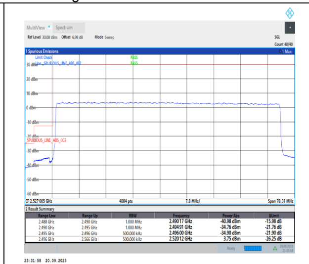
1-N41-PC2-30-70-L-3-DFT-PI2BPSK-Outer_Full-180@0-Ant11-1--PASS-see graph
