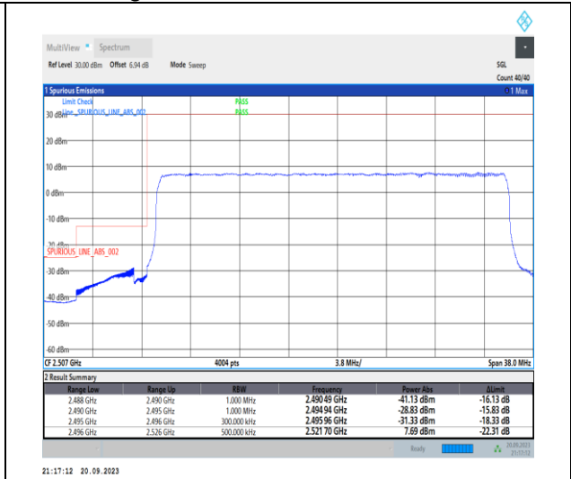
1-N41-PC2-30-30-L-3-DFT-PI2BPSK-Outer_Full-75@0-Ant11-1--PASS-see graph
