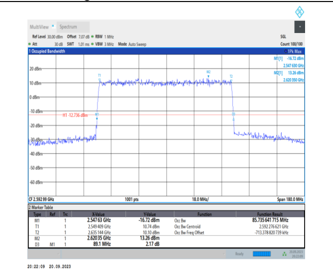
1-N41-PC2-30-90-M-3-DFT-16QAM-Outer_Full-240 @0-Ant11-85.736-89.100-≤90-PASS
