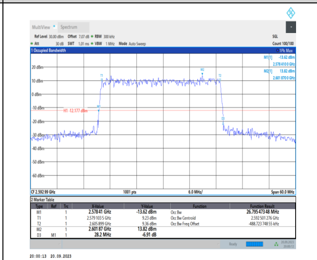
1-N41-PC2-30-30-M-3-DFT-16QAM-Outer_Full-75@ 0-Ant11-26.795-28.200-<math>\leq 30</math>-PASS
