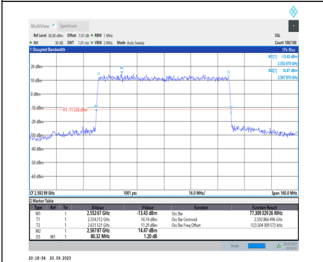
1-N41-PC2-30-80-M-1-DFT-QPSK-Outer_Full-216@ 0-Ant11-77.309-80.320-≤80-PASS
