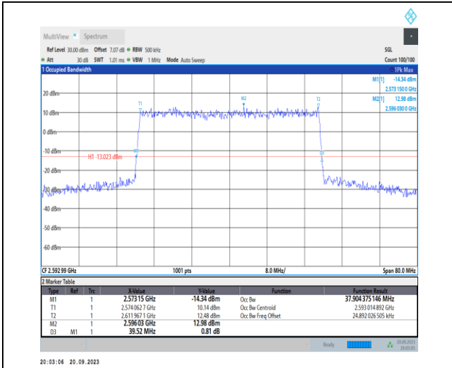
1-N41-PC2-30-40-M-7-CP-16QAM-Outer_Full-106@ 0-Ant11-37.904-39.520-≤40-PASS
