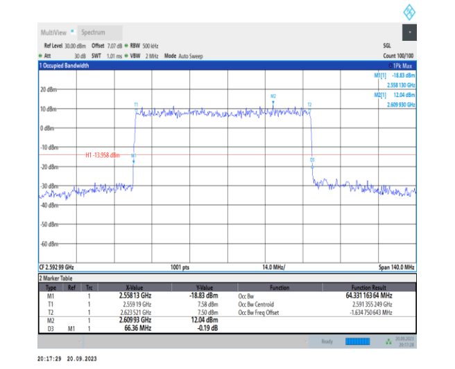
1-N41-PC2-30-70-M-3-DFT-16QAM-Outer_Full-180 @0-Ant11-64.331-66.360-≤70-PASS
