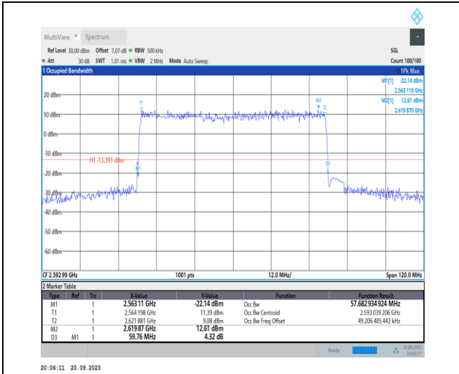
1-N41-PC2-30-60-M-1-DFT-QPSK-Outer_Full-162@ 0-Ant11-57.683-59.760-≤60-PASS
