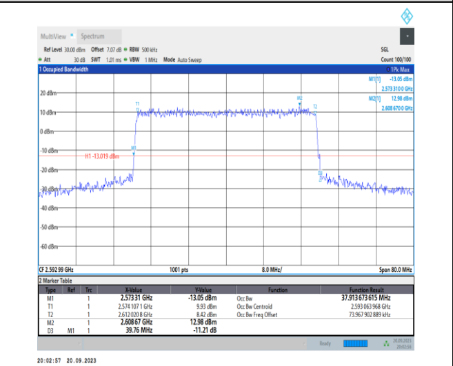
1-N41-PC2-30-40-M-6-CP-QPSK-Outer_Full-106@0 -Ant11-37.914-39.760-≤40-PASS
