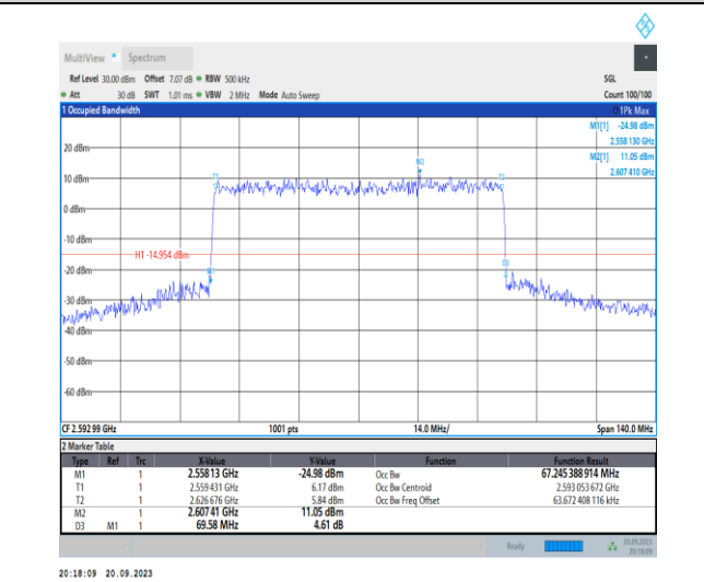
1-N41-PC2-30-70-M-7-CP-16QAM-Outer_Full-189@0 -Ant11-67.245-69.580-≤70-PASS
