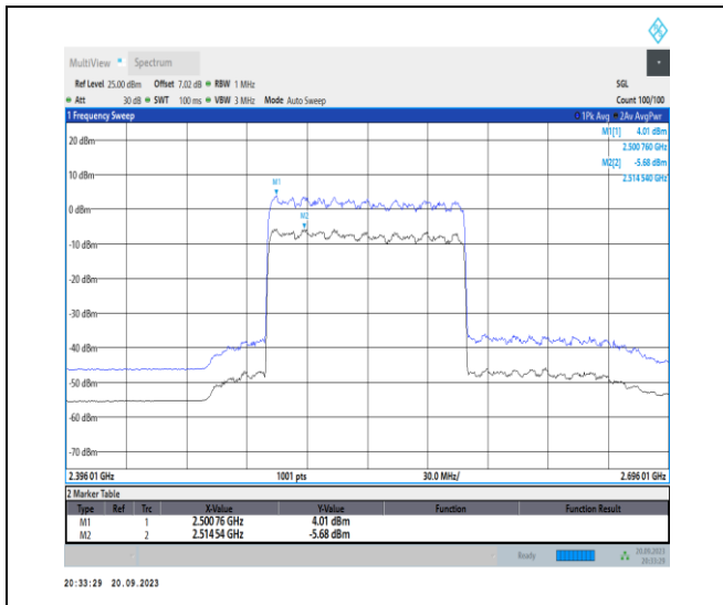
1-N41-PC2-30-100-L-1-DFT-256QAM-Outer_Full-27 0@0-Ant11-9.69-100%-0.00-9.69-PASS-≤13
