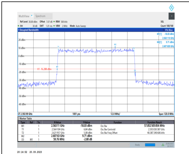
1-N41-PC2-30-60-M-5-DFT-256QAM-Outer_Full-162 @0-Ant11-57.853-59.760-≤60-PASS
