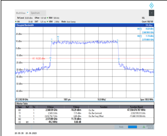
1-N41-PC2-30-50-M-8-CP-64QAM-Outer_Full-133@0-Ant11-47.557-49.200-≤50-PASS
