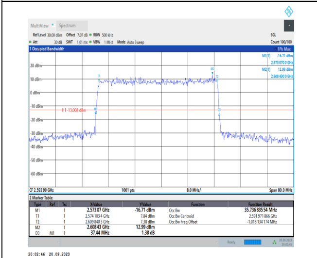
1-N41-PC2-30-40-M-5-DFT-256QAM-Outer_Full-100 @0-Ant11-35.737-37.440-≤40-PASS
