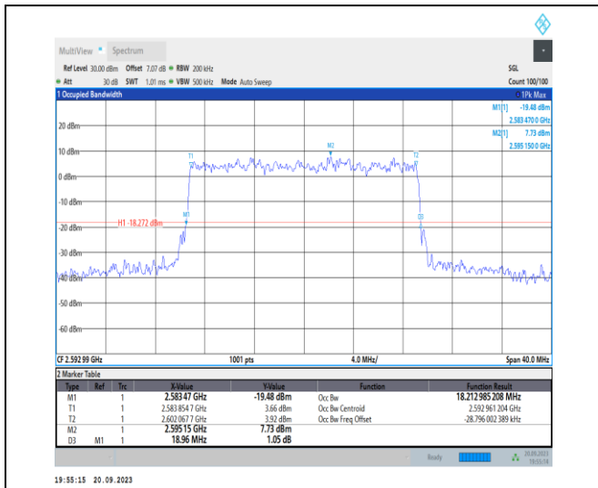
1-N41-PC2-30-20-M-9-CP-256QAM-Outer_Full-51@ 0-Ant11-18.213-18.960-<math>\leq 20</math>-PASS
