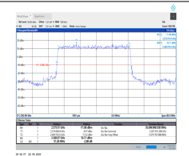
1-N41-PC2-30-40-M-2-DFT-PI2BPSK-Outer_Full-100@0-Ant11-35.697-37.280-≤40-PASS
