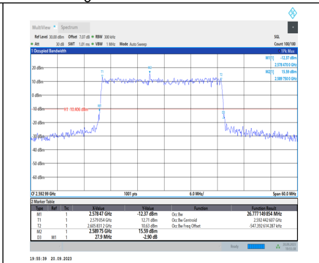
1-N41-PC2-30-30-M-1-DFT-QPSK-Outer_Full-75@0 -Ant11-26.777-27.900-<math>\leq 30</math>-PASS
