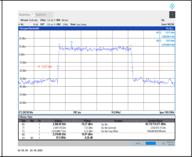
1-N41-PC2-30-50-M-5-DFT-256QAM-Outer_Full-128 @0-Ant11-45.711-47.400-≤50-PASS
