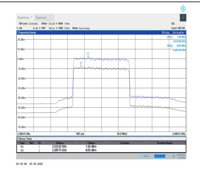
1-N41-PC2-30-100-L-2-CP-256QAM-Outer_Full-273 @0-Ant11-9.68-100%-0.00-9.68-PASS-≤13
