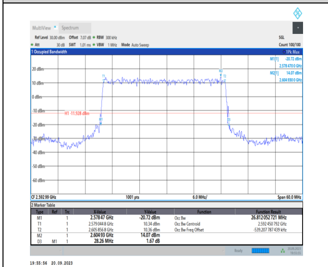
1-N41-PC2-30-30-M-2-DFT-PI2BPSK-Outer_Full-75@ 0-Ant11-26.812-28.260-<math>\leq 30</math>-PASS
