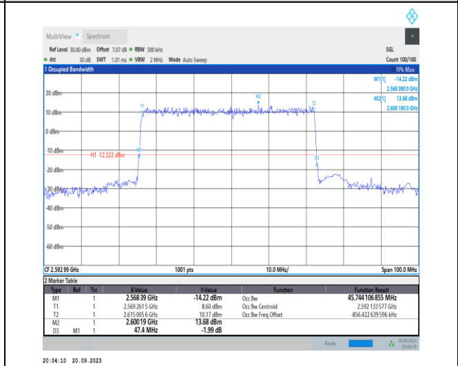
1-N41-PC2-30-50-M-1-DFT-QPSK-Outer_Full-128@ 0-Ant11-45.744-47.400-≤50-PASS
