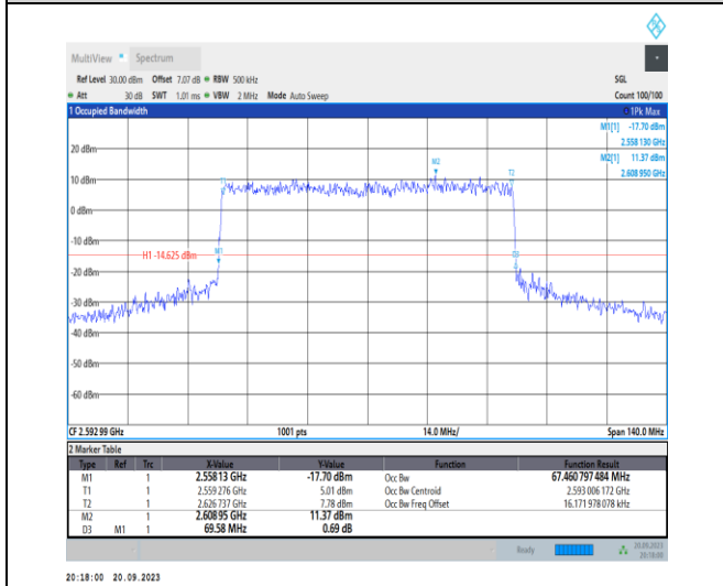
1-N41-PC2-30-70-M-6-CP-QPSK-Outer_Full-189@0 -Ant11-67.461-69.580-≤70-PASS
