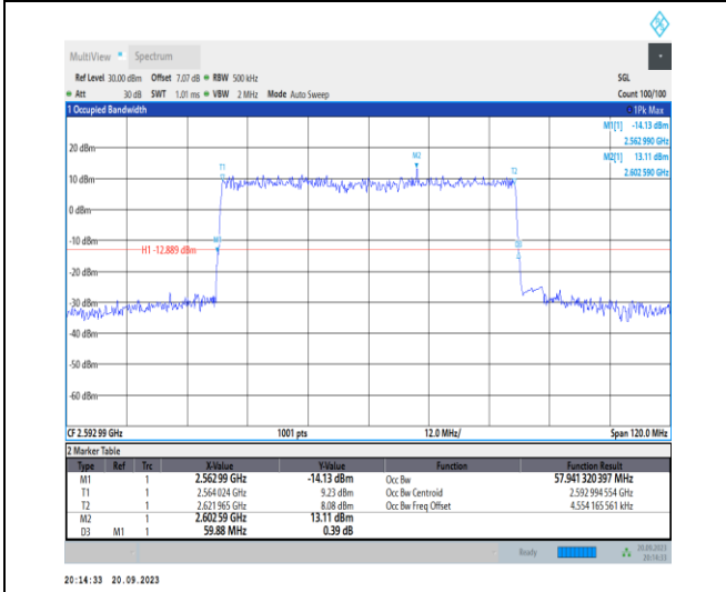
1-N41-PC2-30-60-M-3-DFT-16QAM-Outer_Full-162@ 0-Ant11-57.941-59.880-≤60-PASS
