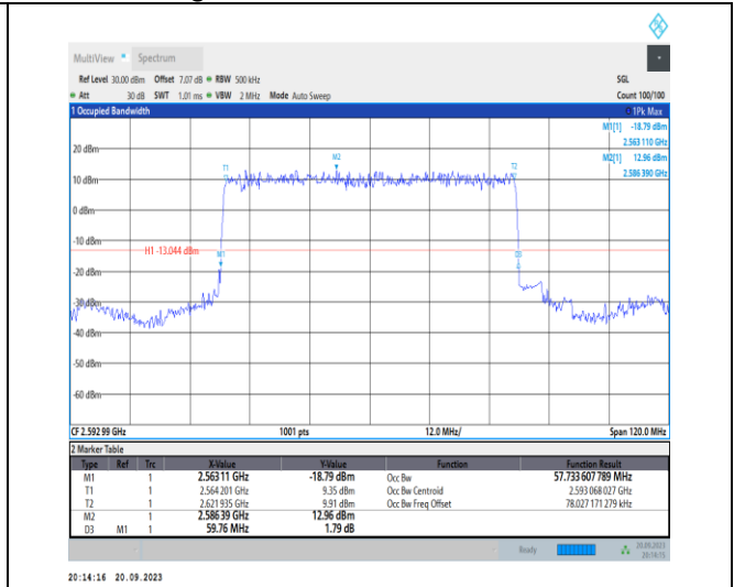
1-N41-PC2-30-60-M-2-DFT-PI2BPSK-Outer_Full-162@ 0-Ant11-57.734-59.760-≤60-PASS
