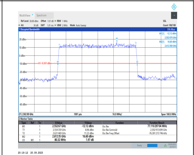
1-N41-PC2-30-80-M-2-DFT-PI2BPSK-Outer_Full-21 6@0-Ant11-77.11-80.320-≤80-PASS
