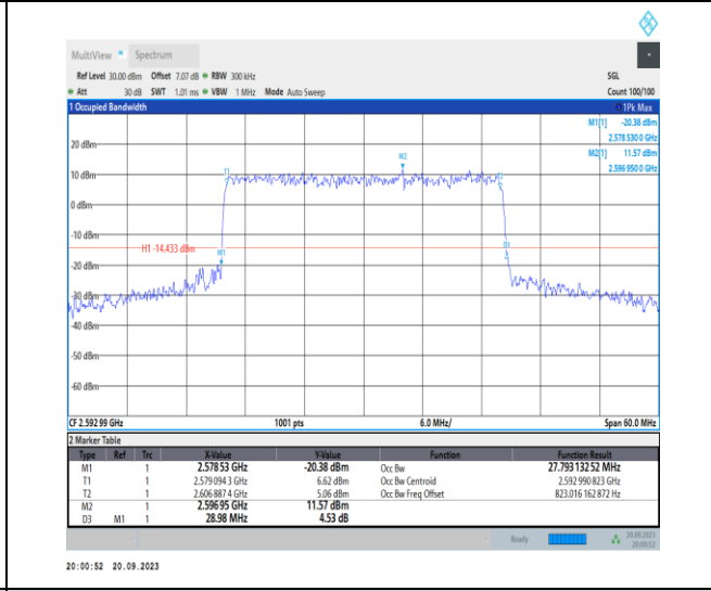
1-N41-PC2-30-30-M-7-CP-16QAM-Outer_Full-78@0-Ant11-27.793-28.980-≤30-PASS
