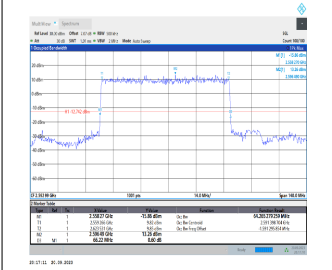
1-N41-PC2-30-70-M-2-DFT-PI2BPSK-Outer_Full-18 @0-Ant11-64.265-66.220-≤70-PASS
