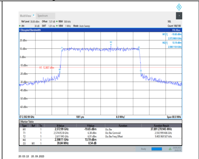
1-N41-PC2-30-40-M-8-CP-64QAM-Outer_Full-106@ 0-Ant11-37.891-39.840-≤40-PASS
