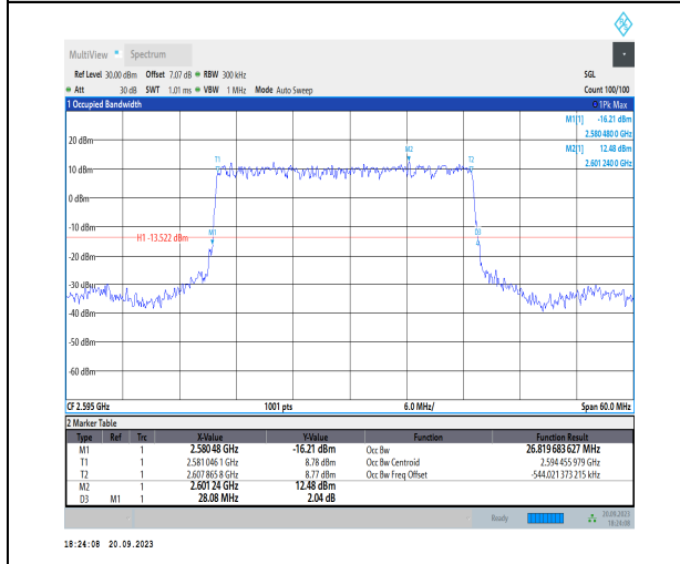
1-N38-PC3-30-30-M-2-DFT-PI2BPSK-Outer_Full-75 @0-Ant11-26.82-28.080-<=30-PASS
