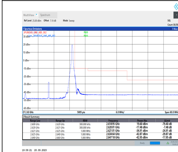
1-N38-PC3-30-20-H-5-CP-QPSK-Edge_1RB_Right-1@50-Ant11-1--PASS-see graph
