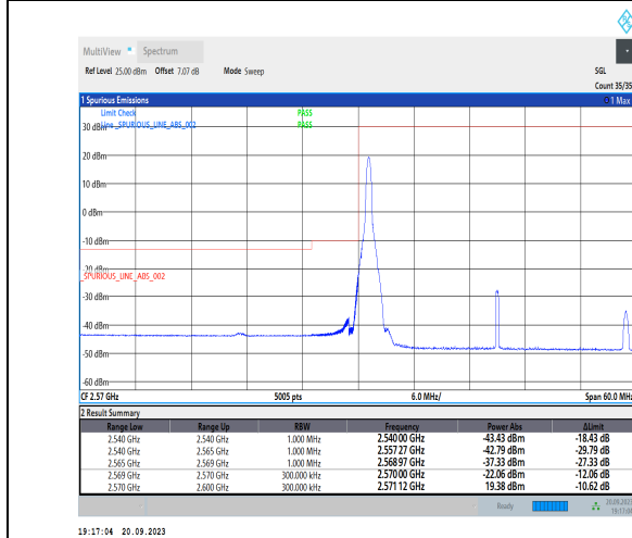
1-N38-PC3-30-30-L-4-CP-QPSK-Edge_1RB_Left-1@0-Ant11-1--PASS-see graph
