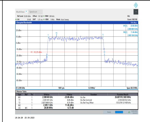
1-N38-PC3-30-30-M-3-DFT-16QAM-Outer_Full-75@ 0-Ant11-26.808-28.080-<=30-PASS
