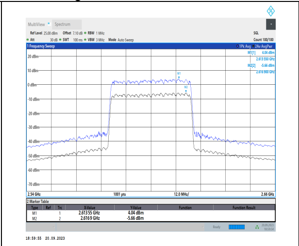
1-N38-PC3-30-40-H-2-CP-256QAM-Outer_Full-106 @0-Ant11-9.70-100%-0.00-9.70-PASS<math>\leq 13</math>
