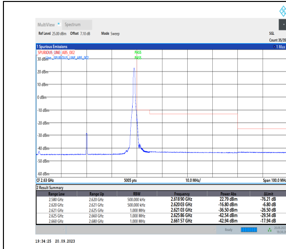
1-N38-PC3-30-40-H-2-DFT-PI2BPSK-Edge_1RB_Righ t-1@105-Ant11-1--PASS-see graph
