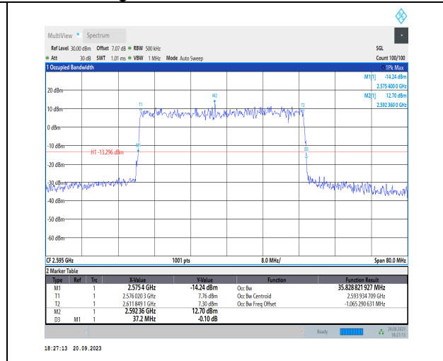
1-N38-PC3-30-40-M-4-DFT-64QAM-Outer_Full-100 @0-Ant11-35.829-37.200-<40-PASS
