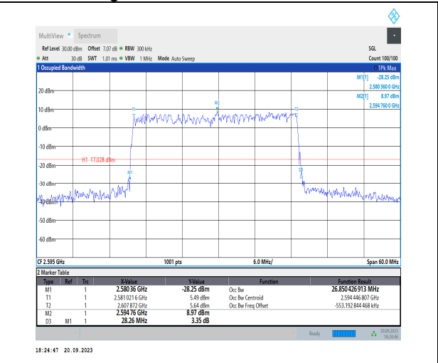
1-N38-PC3-30-30-M-5-DFT-256QAM-Outer_Full-75 @0-Ant11-26.85-28.260-<math>\leq</math>30-PASS
