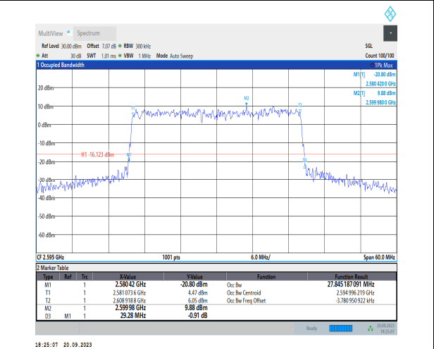
1-N38-PC3-30-30-M-7-CP-16QAM-Outer_Full-78@0 -Ant11-27.845-29.280-<math>\leq</math>30-PASS
