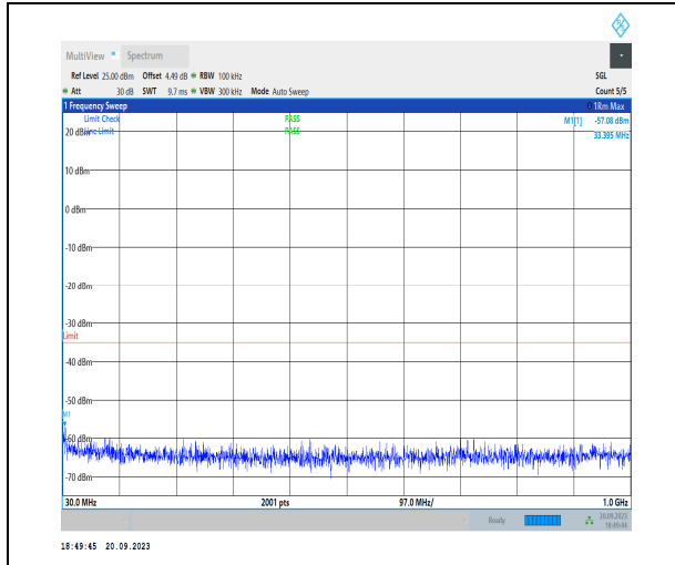
1-N38-30-40-M-1-DFT-PI2BPSK-Inner_1RB_Left-1 @1-30-1000-Ant11-33.395-57.08-35-PASS
