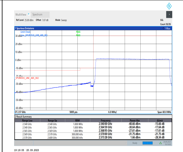
1-N38-PC3-30-30-L-6-CP-QPSK-Outer_Full-78@0-Ant11-1--PASS-see graph
