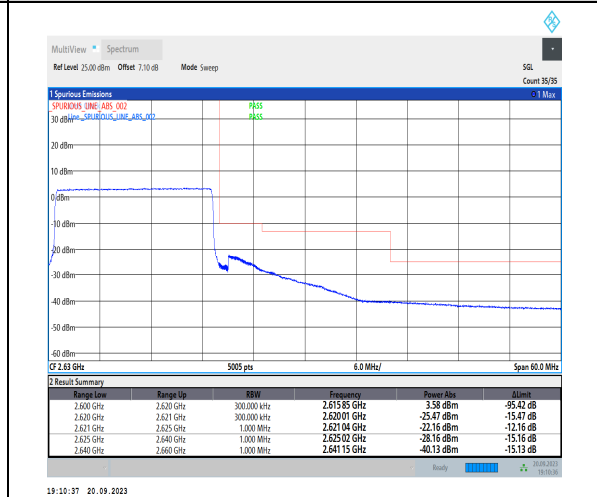
1-N38-PC3-30-20-H-6-CP-QPSK-Outer_Full-51@0-Ant11-1--PASS-see graph
