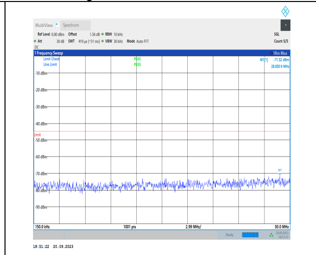
1-N38-30-40-H-1-DFT-PI2BPSK-Inner_1RB_Left-1 @ 1-0.15-30-Ant11-29.94--71.66--45-PASS
