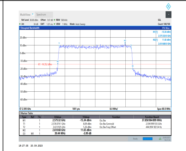
1-N38-PC3-30-40-M-6-CP-QPSK-Outer_Full-106@0 -Ant11-37.851-39.440-<40-PASS
