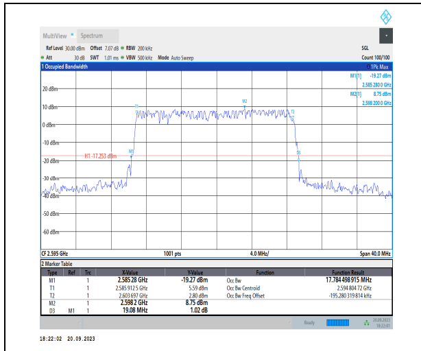
1-N38-PC3-30-20-M-5-DFT-256QAM-Outer_Full-50@0-Ant11-17.784-19.080-≤20-PASS
