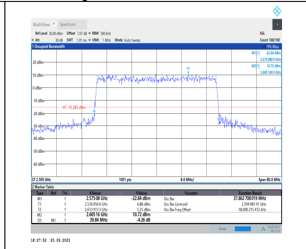
1-N38-PC3-30-40-M-8-CP-64QAM-Outer_Full-106@ 0-Ant11-37.863-39.840-<40-PASS
