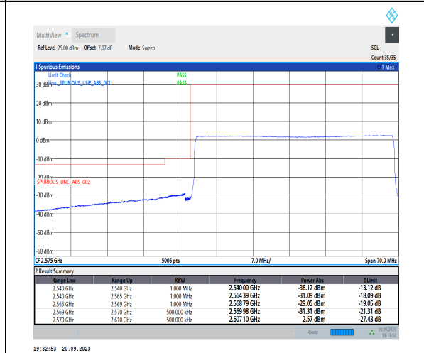
1-N38-PC3-30-40-L-6-CP-QPSK-Outer_Full-106@0-Ant11-1--PASS-see graph
