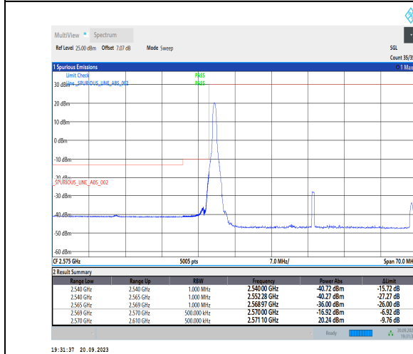
1-N38-PC3-30-40-L-4-CP-QPSK-Edge_1RB_Left-1@0-Ant11-1--PASS-see graph
