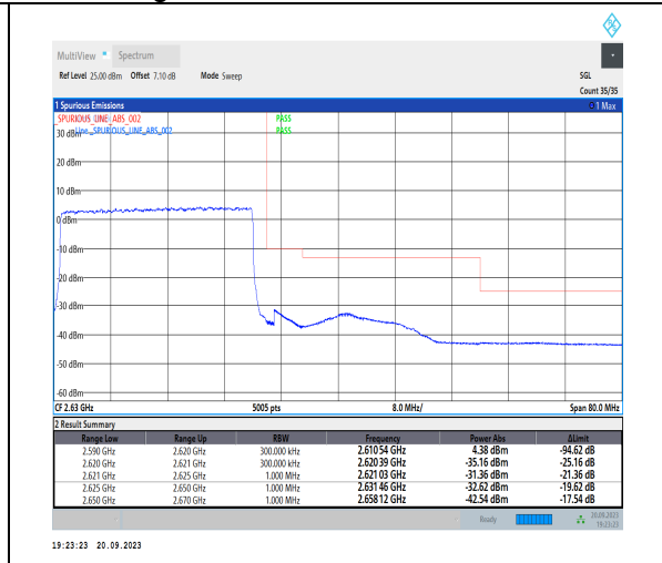
1-N38-PC3-30-30-H-3-DFT-PI2BPSK-Outer_Full-7 5@0-Ant11-1--PASS-see graph
