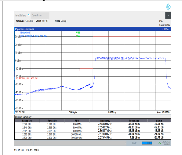
1-N38-PC3-30-30-L-3-DFT-PI2BPSK-Outer_Full-75@0-Ant11-1--PASS-see graph
