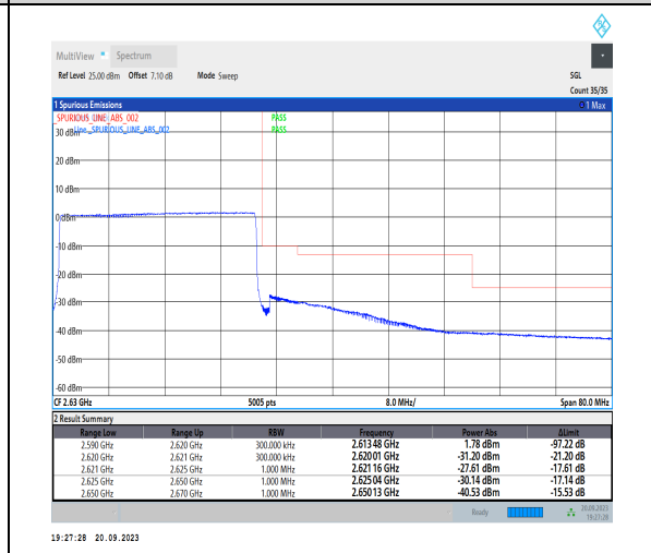
1-N38-PC3-30-30-H-6-CP-QPSK-Outer_Full-78@ 0-Ant11-1--PASS-see graph
