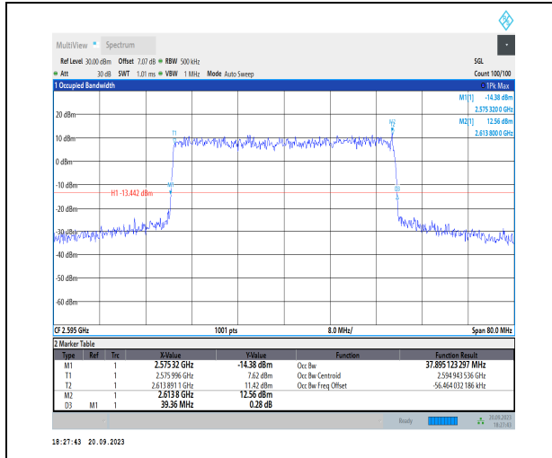
1-N38-PC3-30-40-M-7-CP-16QAM-Outer_Full-106@ 0-Ant11-37.895-39.360-<40-PASS
