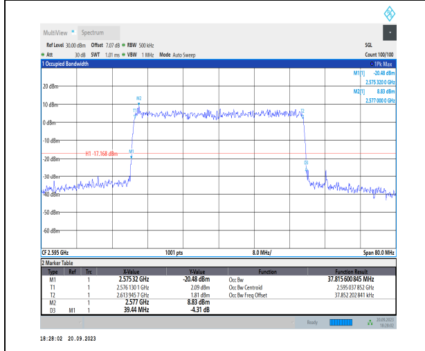
1-N38-PC3-30-40-M-9-CP-256QAM-Outer_Full-106 @0-Ant11-37.816-39.440-<40-PASS
