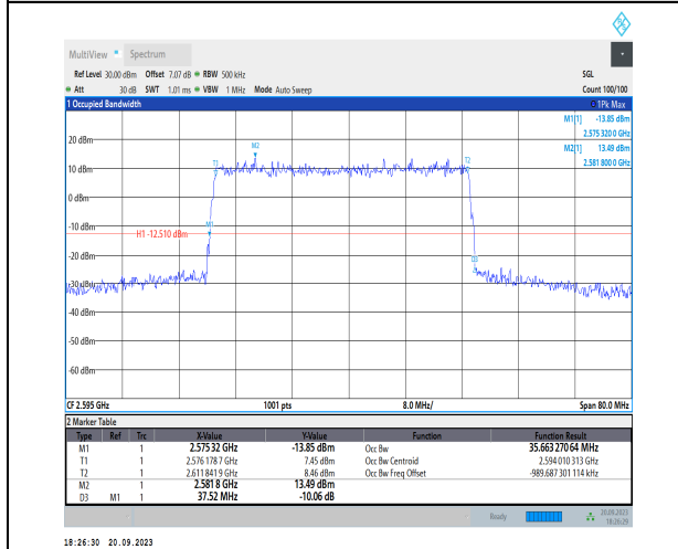
1-N38-PC3-30-40-M-1-DFT-QPSK-Outer_Full-100@0 0-Ant11-35.663-37.520-≤40-PASS
