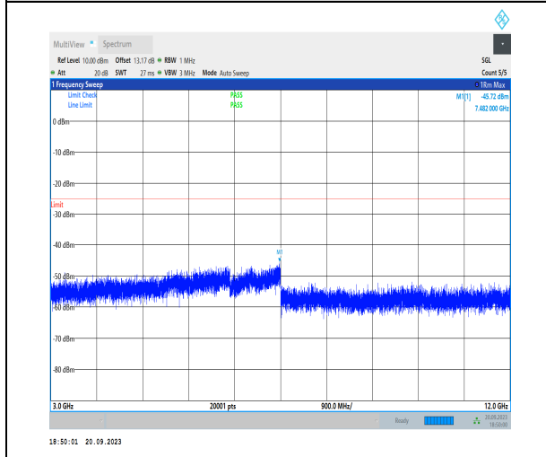
1-N38-30-40-M-1-DFT-PI2BPSK-Inner_1RB_Left-1 @1-3000-12000-Ant11-7482.00-45.72-25-PASS
