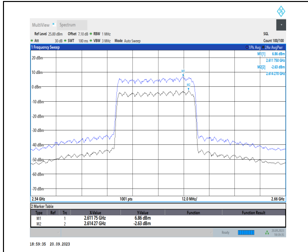
1-N38-PC3-30-40-H-1-DFT-256QAM-Outer_Full-100 @0-Ant11-9.49-100%-0.00-9.49-PASS<math>\leq 13</math>
