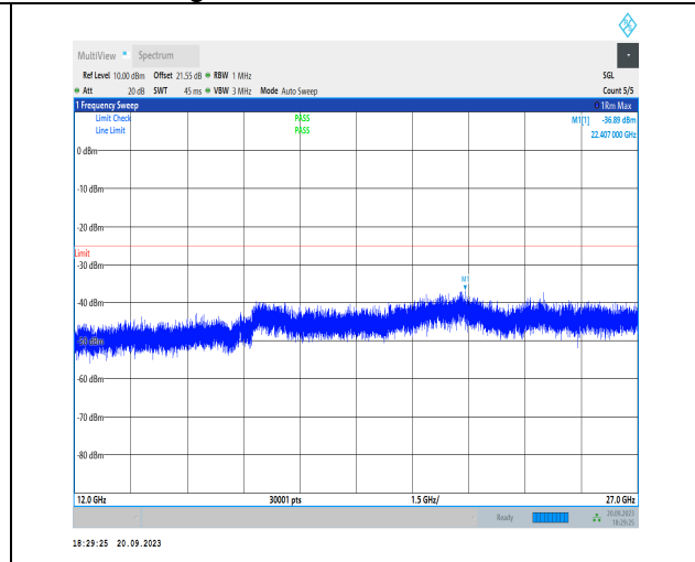
1-N38-30-40-L-1-DFT-PI2BPSK-Inner_1RB_Left-1@ 1-12000-27000-Ant11-22407.00--36.89--25-PASS
