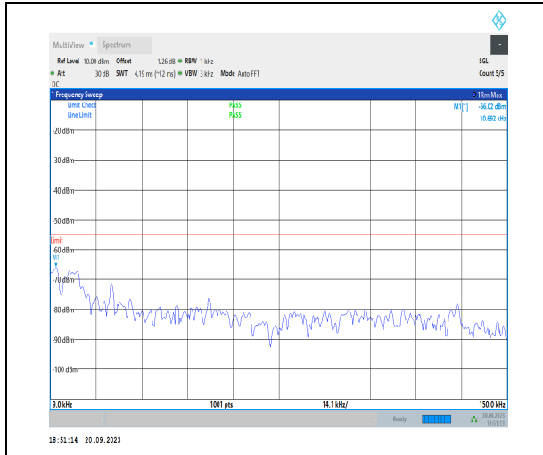
1-N38-30-40-H-1-DFT-PI2BPSK-Inner_1RB_Left-1 @ 1-0.009-0.15-Ant11-0.13--80.65--55-PASS
