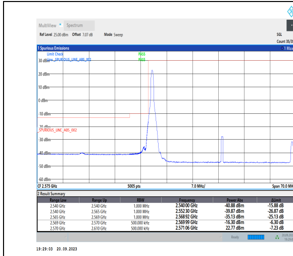
1-N38-PC3-30-40-L-1-DFT-PI2BPSK-Edge_1RB_Left-1@0-Ant11-1--PASS-see graph
