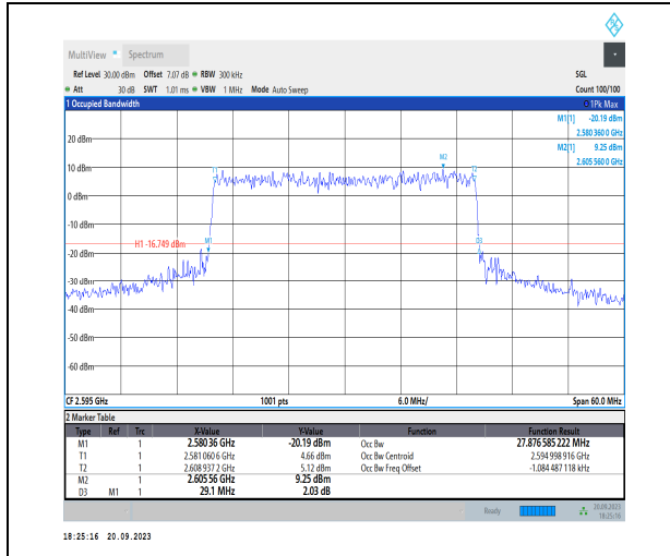
1-N38-PC3-30-30-M-8-CP-64QAM-Outer_Full-78@0 -Ant11-27.877-29.100-≤30-PASS
