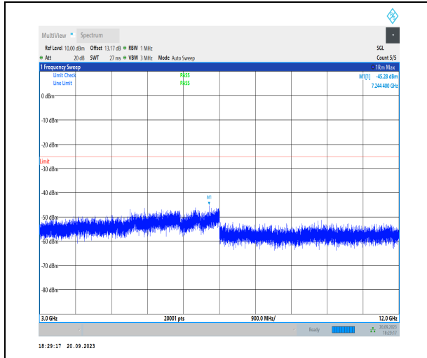
1-N38-30-40-L-1-DFT-PI2BPSK-Inner_1RB_Left-1 @ 1-3000-12000-Ant11-7244.40--45.28--25-PASS
