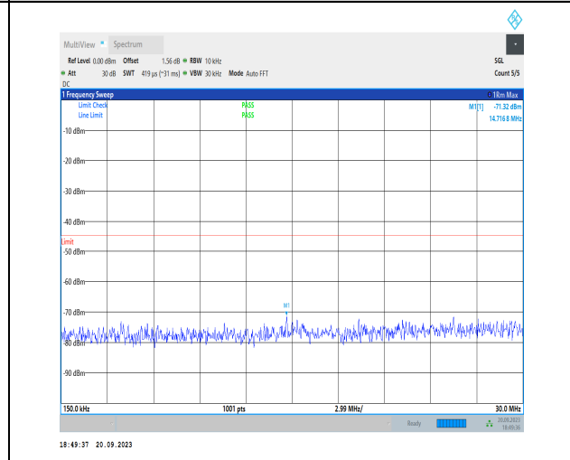
1-N38-30-40-M-1-DFT-PI2BPSK-Inner_1RB_Left-1@ 1-0.15-30-Ant11-14.72--71.32--45-PASS
