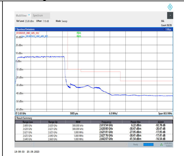
1-N38-PC3-30-20-H-3-DFT-PI2BPSK-Outer_Full-50@0-Ant11-1--PASS-see graph
