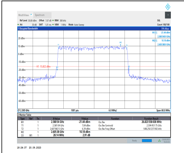
1-N38-PC3-30-30-M-4-DFT-64QAM-Outer_Full-75@ 0-Ant11-26.824-28.140-<math>\leq</math>30-PASS
