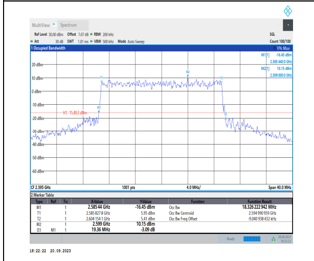
1-N38-PC3-30-20-M-7-CP-16QAM-Outer_Full-51@0-Ant11-18.326-19.360-≤20-PASS
