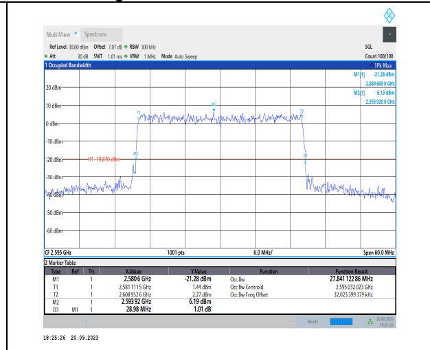
1-N38-PC3-30-30-M-9-CP-256QAM-Outer_Full-78@0 0-Ant11-27.841-28.980-≤30-PASS
