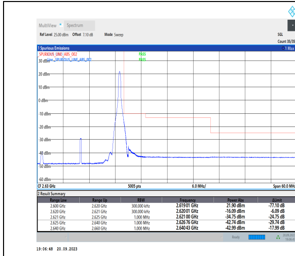
1-N38-PC3-30-20-H-2-DFT-PI2BPSK-Edge_1RB_Right-t1@50-Ant11-1--PASS-see graph
