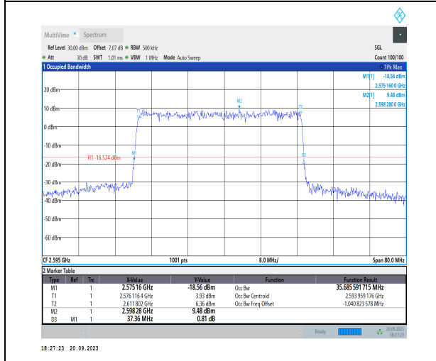
1-N38-PC3-30-40-M-5-DFT-256QAM-Outer_Full-100 @0-Ant11-35.686-37.360-<40-PASS
