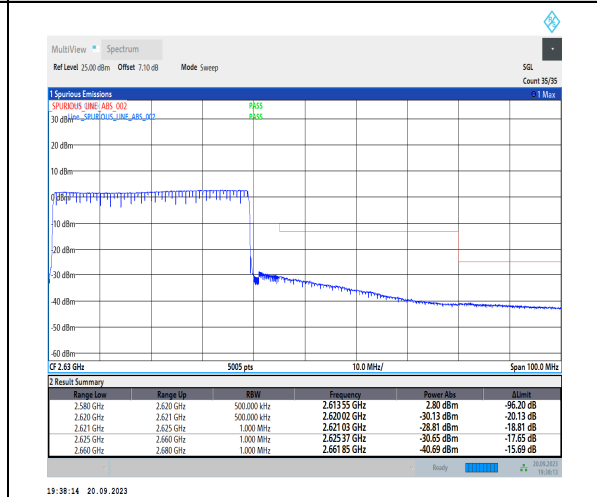
1-N38-PC3-30-40-H-6-CP-QPSK-Outer_Full-106 @0-Ant11-1--PASS-see graph
