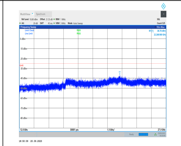
1-N38-30-40-M-1-DFT-PI2BPSK-Inner_1RB_Left-1@ 1-12000-27000-Ant11-22268.00-36.78-25-PASS
