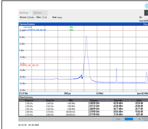
1-N38-PC3-30-30-L-1-DFT-PI2BPSK-Edge_1RB_Left-1@0-Ant11-1--PASS-see graph
