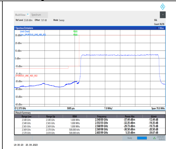
1-N38-PC3-30-40-L-3-DFT-PI2BPSK-Outer_Full-100@0-Ant11-1--PASS-see graph
