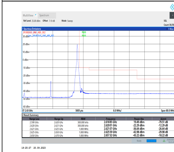
1-N38-PC3-30-30-H-5-CP-QPSK-Edge_1RB_Right-1 @77-Ant11-1--PASS-see graph
