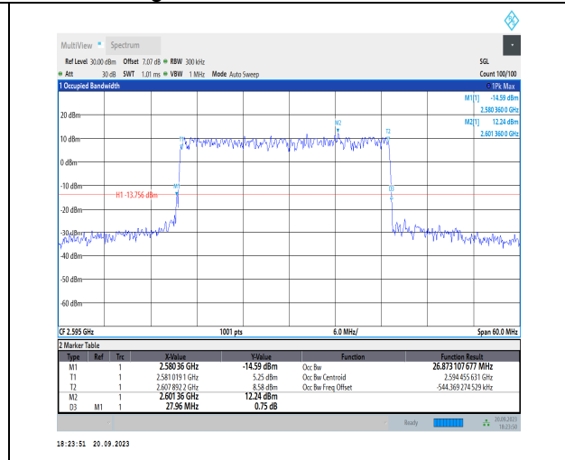
1-N38-PC3-30-30-M-1-DFT-QPSK-Outer_Full-75@ 0-Ant11-26.873-27.960-<=30-PASS
