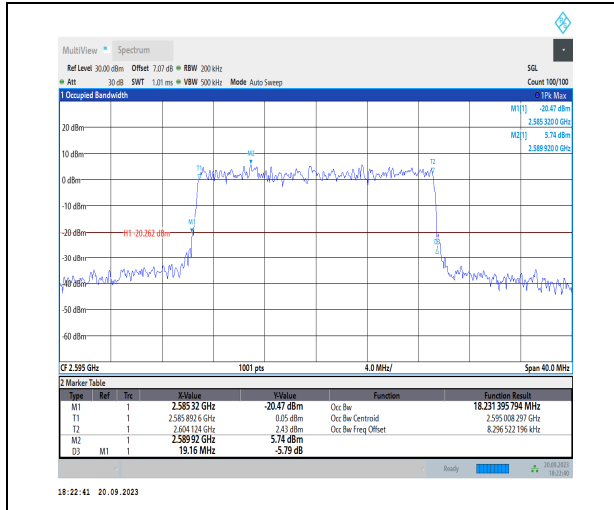
1-N38-PC3-30-20-M-9-CP-256QAM-Outer_Full-51@ 0-Ant11-18.231-19.160-<=20-PASS
