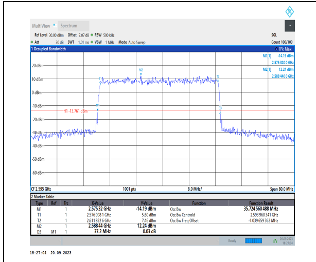
1-N38-PC3-30-40-M-3-DFT-16QAM-Outer_Full-100 @0-Ant11-35.725-37.200-<40-PASS
