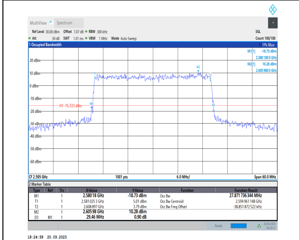
1-N38-PC3-30-30-M-6-CP-QPSK-Outer_Full-78@0- Ant11-27.872-29.460-<math>\leq</math>30-PASS
