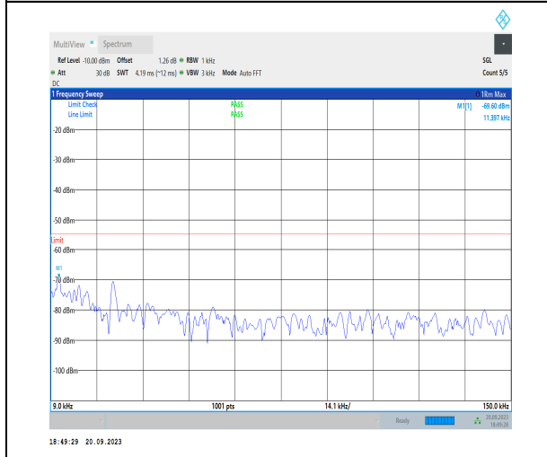
1-N38-30-40-M-1-DFT-PI2BPSK-Inner_1RB_Left-1 @ 1-0.009-0.15-Ant11-0.011--69.60--55-PASS
