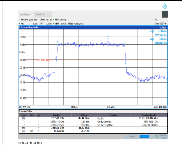
1-N38-PC3-30-40-M-2-DFT-PI2BPSK-Outer_Full-100@0 0-Ant11-35.838-37.360-≤40-PASS
