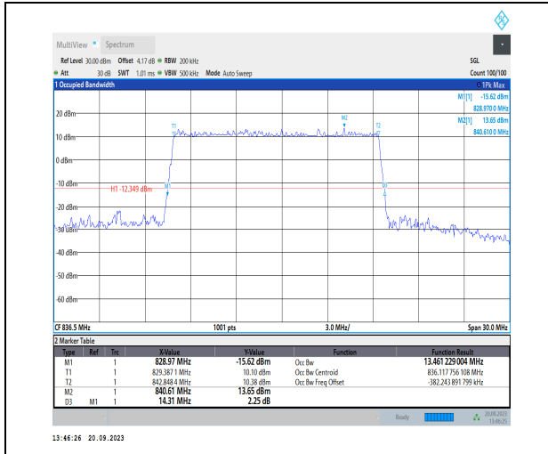
1-N26-824-849-PC3-15-15-M-3-DFT-16QAM-Outer_Full-75@0-Ant41-13.461-14.310-≤15-PASS
