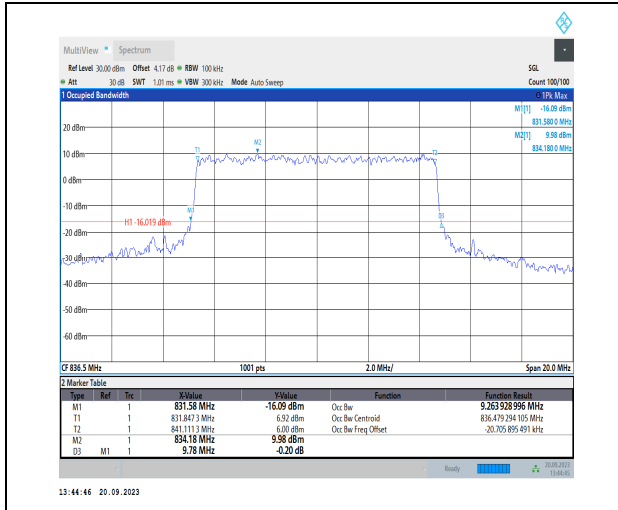
1-N26-824-849-PC3-15-10-M-8-CP-64QAM-Outer_F ull-52@0-Ant41-9.264-9.780-<=10-PASS
