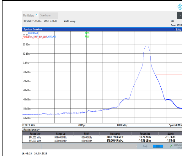
1-N26-824-849-PC3-15-5-H-5-CP-QPSK-Edge_1RB_Right-1@24-Ant41-1-seegraph-PASS-see graph
