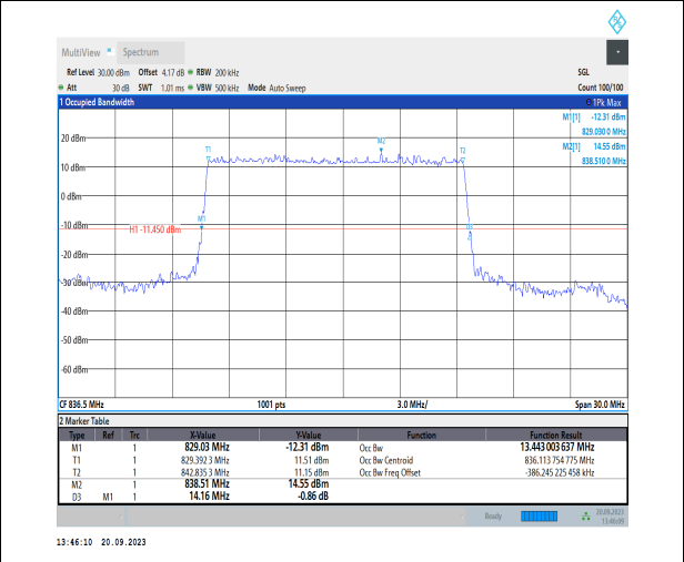
1-N26-824-849-PC3-15-15-M-2-DFT-PI2BPSK-Outer_F ull-75@0-Ant41-13.443-14.160-<=15-PASS
