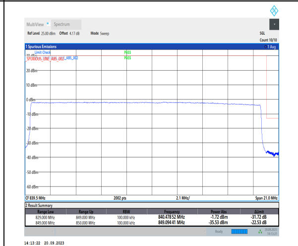
1-N26-824-849-PC3-15-20-H-6-CP-QPSK-Outer_F ull-106@0-Ant41-1-seegraph-PASS-see graph
