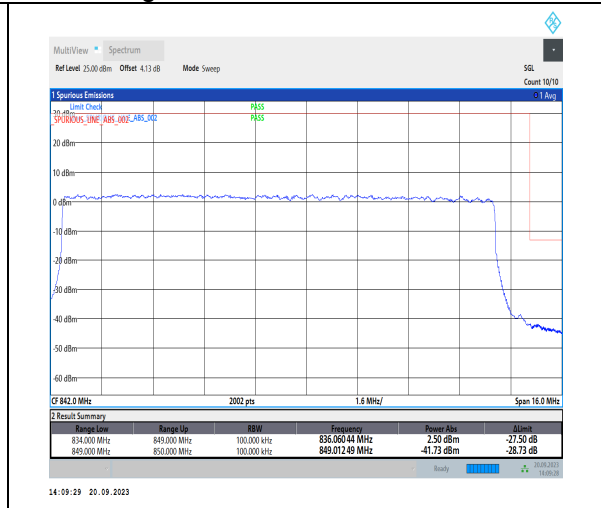
1-N26-824-849-PC3-15-15-H-3-DFT-PI2BPSK-Outer_Full-75@0-Ant41-1-seegraph-PASS-see graph
