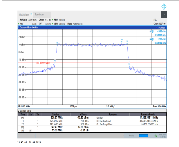
1-N26-824-849-PC3-15-15-M-7-CP-16QAM-Outer_F ull-79@0-Ant41-14.129-15.030-≤15-PASS
