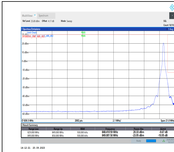
1-N26-824-849-PC3-15-20-H-2-DFT-PI2BPSK-Edge_1 RB_Right-1@105-Ant41-1-seegraph-PASS-see graph
