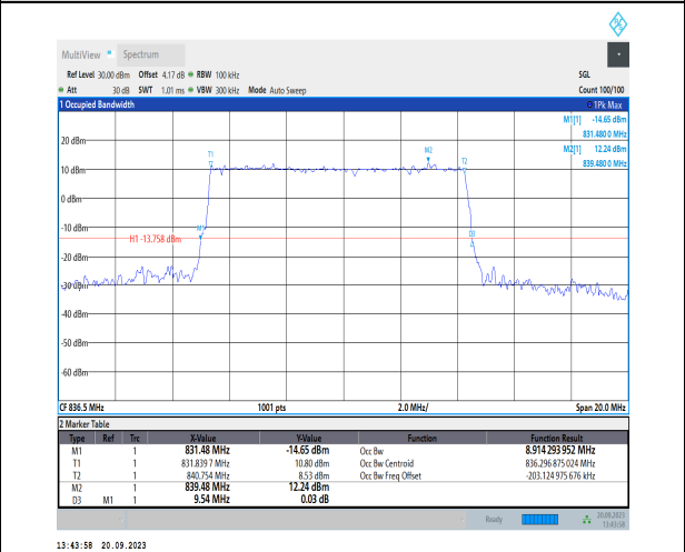
1-N26-824-849-PC3-15-10-M-3-DFT-16QAM-Outer_F ull-50@0-Ant41-8.914-9.540-≤10-PASS
