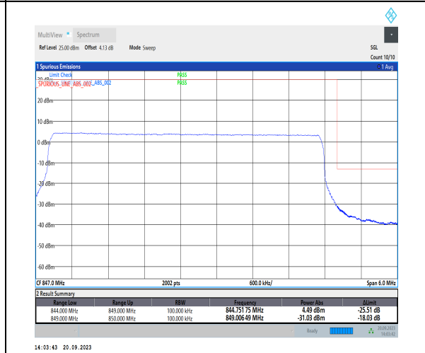
1-N26-824-849-PC3-15-5-H-6-CP-QPSK-Outer_Full-25@0-Ant41-1-seegraph-PASS-see graph
