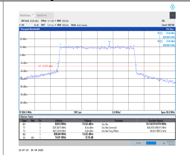
1-N26-824-849-PC3-15-15-M-8-CP-64QAM-Outer_F ull-79@0-Ant41-14.143-14.910-≤15-PASS
