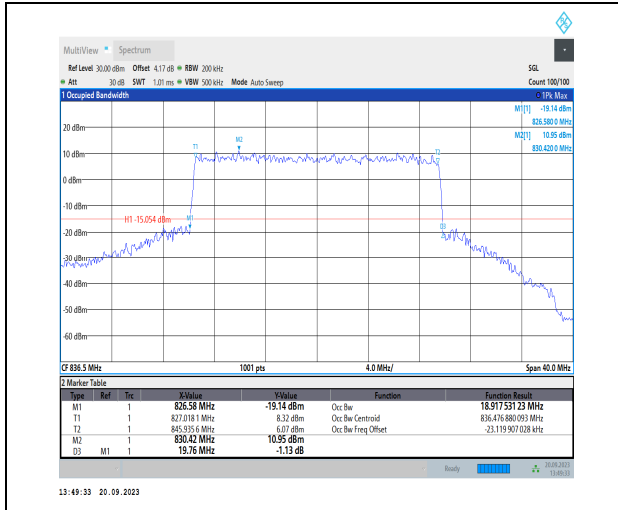
1-N26-824-849-PC3-15-20-M-6-CP-QPSK-Outer_Full-106@0-Ant41-18.918-19.760-≤20-PASS
