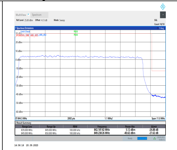
1-N26-824-849-PC3-15-10-H-3-DFT-PI2BPSK-Out er_Full-50@0-Ant41-1-seegraph-PASS-see graph
