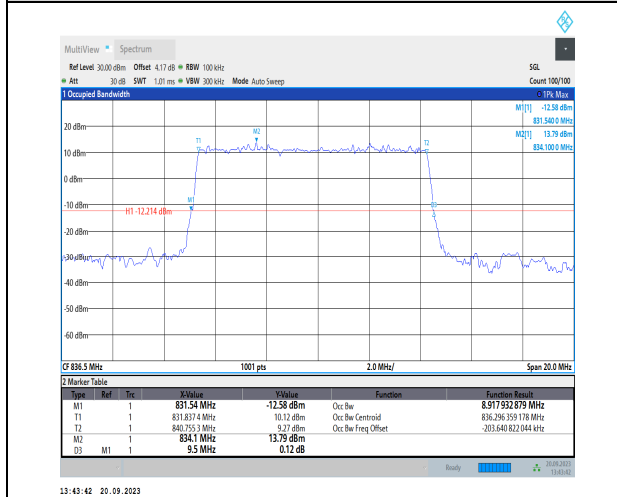
1-N26-824-849-PC3-15-10-M-2-DFT-PI2BPSK-Outer_F ull-50@0-Ant41-8.918-9.500-≤10-PASS
