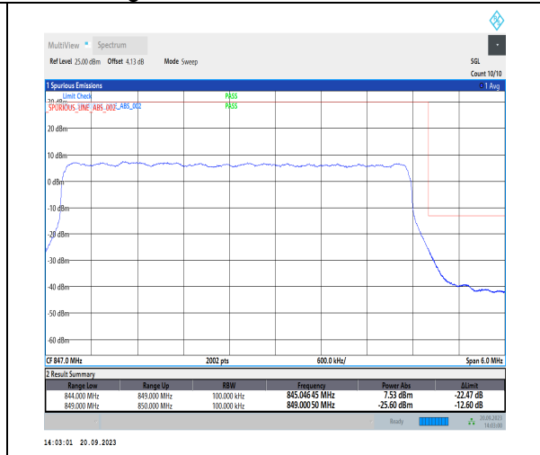
1-N26-824-849-PC3-15-5-H-3-DFT-PI2BPSK-Outer_Full-25@0-Ant41-1-seegraph-PASS-see graph
