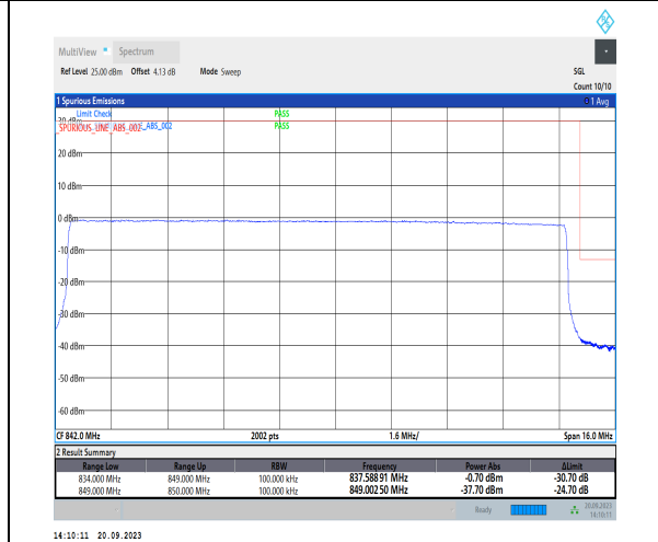
1-N26-824-849-PC3-15-15-H-6-CP-QPSK-Outer_Full-79@0-Ant41-1-seegraph-PASS-see graph
