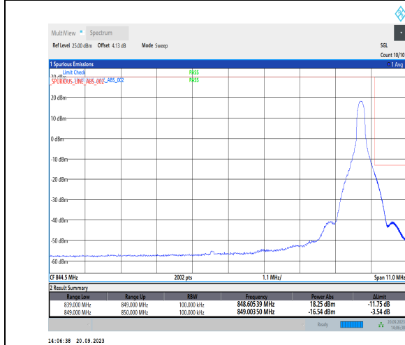
1-N26-824-849-PC3-15-10-H-5-CP-QPSK-Edge_1RB _Right-1@51-Ant41-1-seegraph-PASS-see graph
