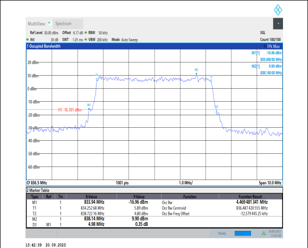
1-N26-824-849-PC3-15-5-M-8-CP-64QAM-Outer_Fu. II-25@0-Ant41-4.469-4.980-≤5-PASS
