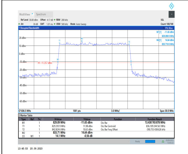
1-N26-824-849-PC3-15-15-M-1-DFT-QPSK-Outer_F ull-75@0-Ant41-13.431-14.100-<=15-PASS
