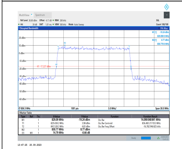
1-N26-824-849-PC3-15-15-M-9-CP-256QAM-Outer_F ull-79@0-Ant41-14.09-14.790-≤15-PASS
