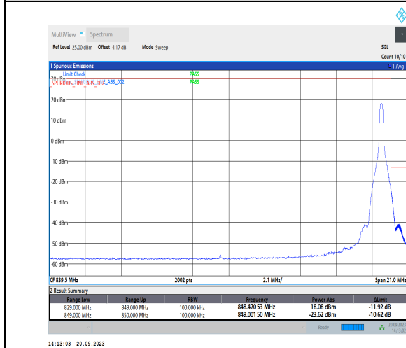
1-N26-824-849-PC3-15-20-H-5-CP-QPSK-Edge_1RB _Right-1@105-Ant41-1-seegraph-PASS-see graph
