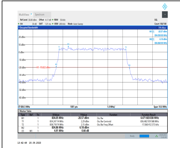
1-N26-824-849-PC3-15-5-M-9-CP-256QAM-Outer_F ull-25@0-Ant41-4.472-4.910-≤5-PASS
