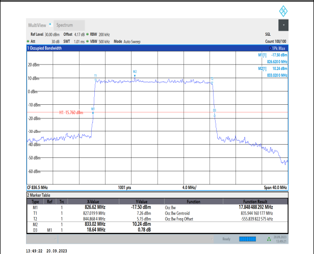
1-N26-824-849-PC3-15-20-M-5-DFT-256QAM-Outer_Full-100@0-Ant41-17.848-18.640-≤20-PASS
