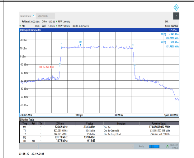
1-N26-824-849-PC3-15-20-M-1-DFT-QPSK-Outer_F ull-100@0-Ant41-17.848-18.720-≤20-PASS
