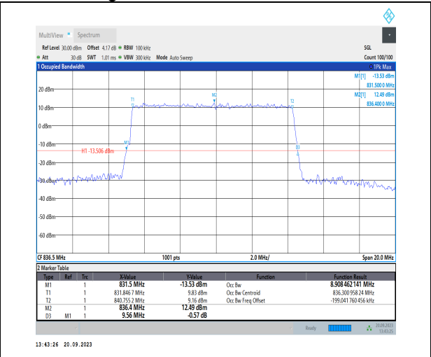
1-N26-824-849-PC3-15-10-M-1-DFT-QPSK-Outer_F ull-50@0-Ant41-8.908-9.560-≤10-PASS
