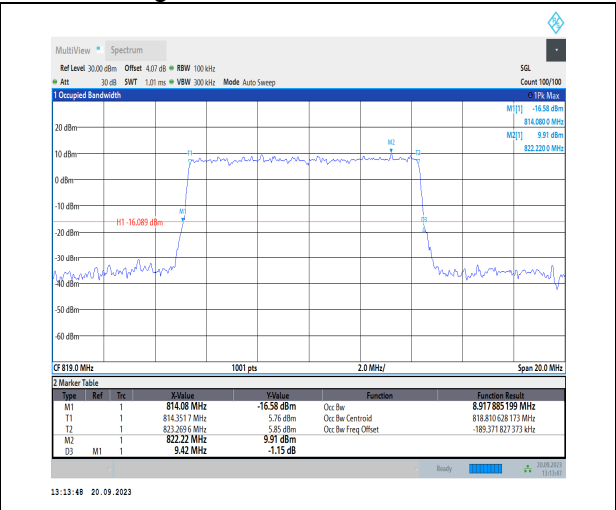
1-N26-814-824-PC3-15-10-M-5-DFT-256QAM-Outer_Full-50@0-Ant41-8.918-9.420-≤10-PASS
