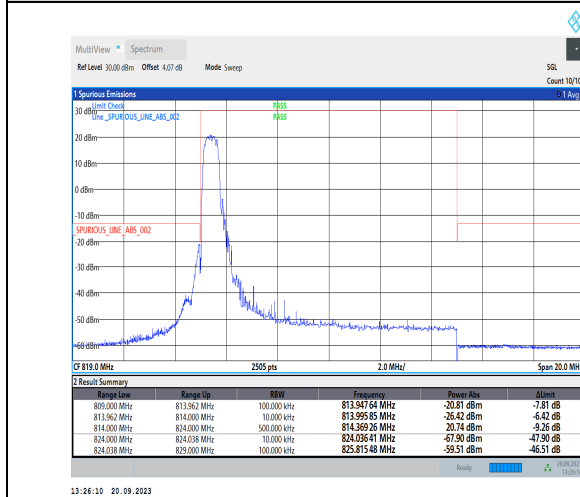
1-N26-814-824-PC3-15-10-L-4-CP-QPSK-Edge_1RB_Left-1@0-Ant41-1--PASS-see graph
