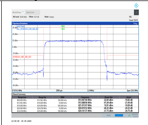
1-N26-814-824-PC3-15-10-L-3-DFT-PI2BPSK-Out er_Full-50@0-Ant41-1--PASS-see graph
