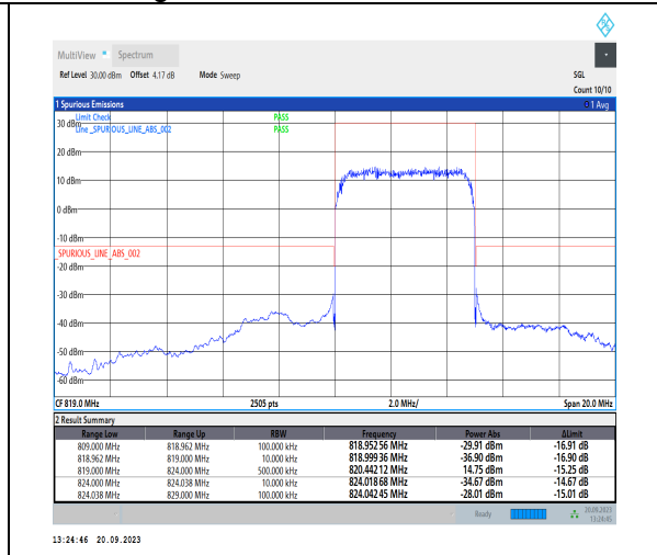
1-N26-814-824-PC3-15-5-H-3-DFT-PI2BPSK-Outer_Full-25@0-Ant41-1--PASS-see graph
