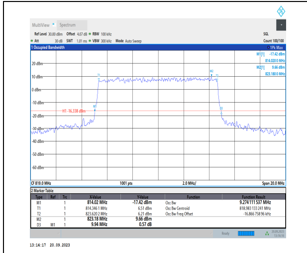
1-N26-814-824-PC3-15-10-M-8-CP-64QAM-Outer_F ull-52@0-Ant41-9.274-9.940-≤10-PASS
