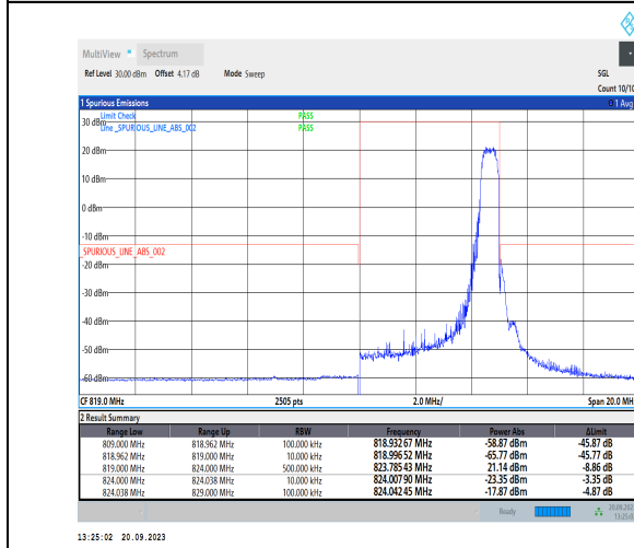
1-N26-814-824-PC3-15-5-H-5-CP-QPSK-Edge_1RB_Right-1@24-Ant41-1--PASS-see graph
