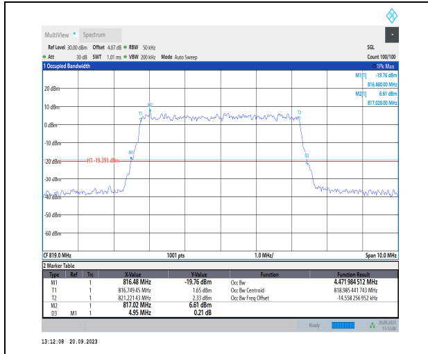
1-N26-814-824-PC3-15-5-M-9-CP-256QAM-Outer_F ull-25@0-Ant41-4.472-4.950-≤5-PASS
