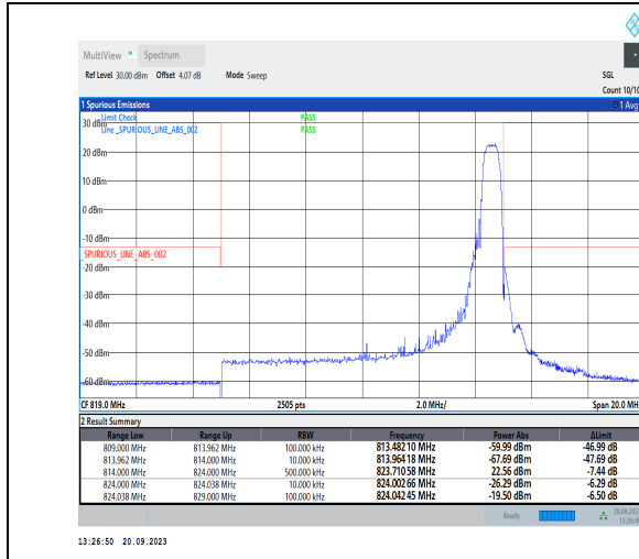
1-N26-814-824-PC3-15-10-H-2-DFT-PI2BPSK-Edge_1 RB_Right-1@51-Ant41-1--PASS-see graph
