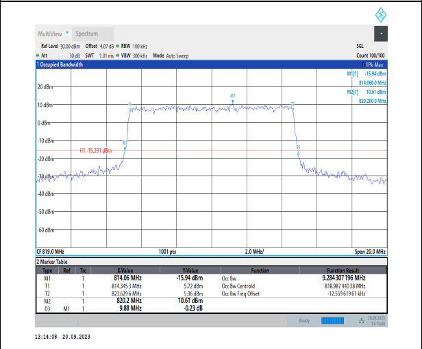
1-N26-814-824-PC3-15-10-M-7-CP-16QAM-Outer_Full-52@0-Ant41-9.284-9.880-≤10-PASS
