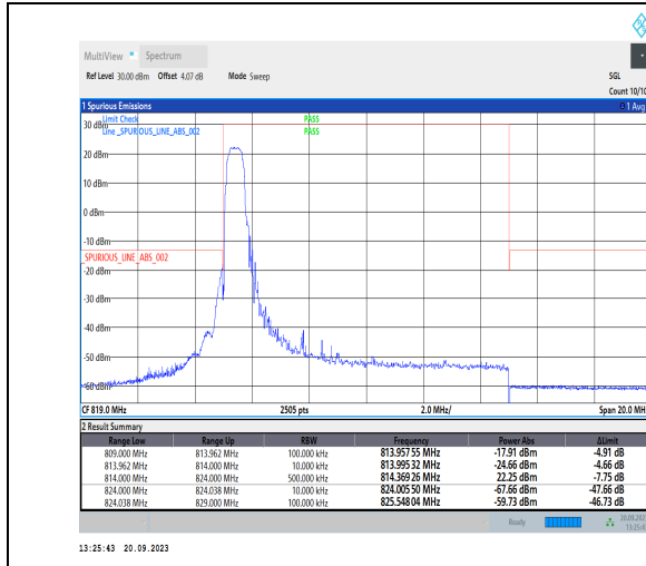
1-N26-814-824-PC3-15-10-L-1-DFT-PI2BPSK-Edge_1 RB_Left-1@0-Ant41-1--PASS-see graph
