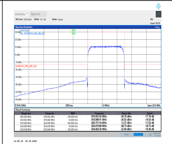
1-N26-814-824-PC3-15-5-H-6-CP-QPSK-Outer_Full-25@0-Ant41-1--PASS-see graph
