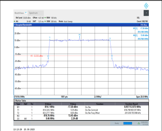
1-N26-814-824-PC3-15-10-M-3-DFT-16QAM-Outer_F ull-50@0-Ant41-8.958-9.460-≤10-PASS
