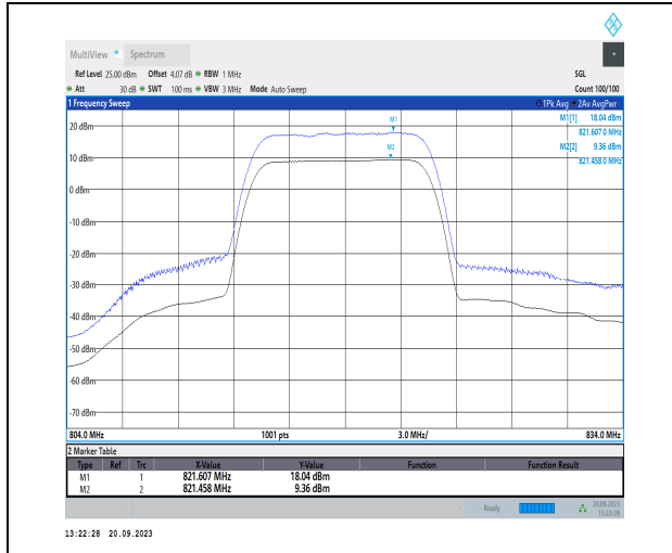
1-N26-814-824-PC3-15-10-H-1-DFT-256QAM-Outer_Full-50@0-Ant41-8.68-100%-0.00-8.68-PASS-<=13
