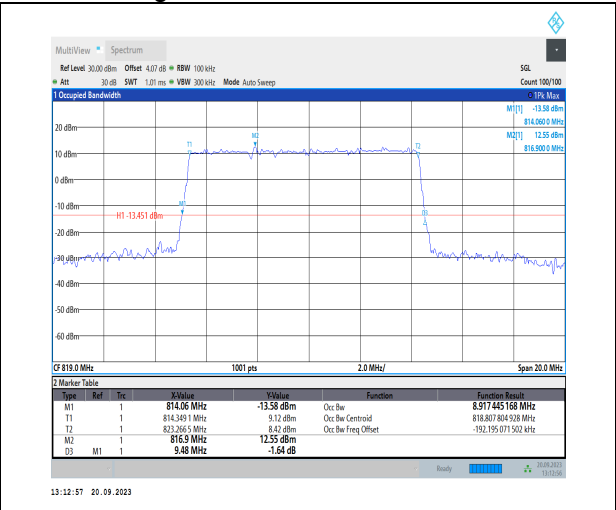
1-N26-814-824-PC3-15-10-M-1-DFT-QPSK-Outer_F ull-50@0-Ant41-8.917-9.480-≤10-PASS
