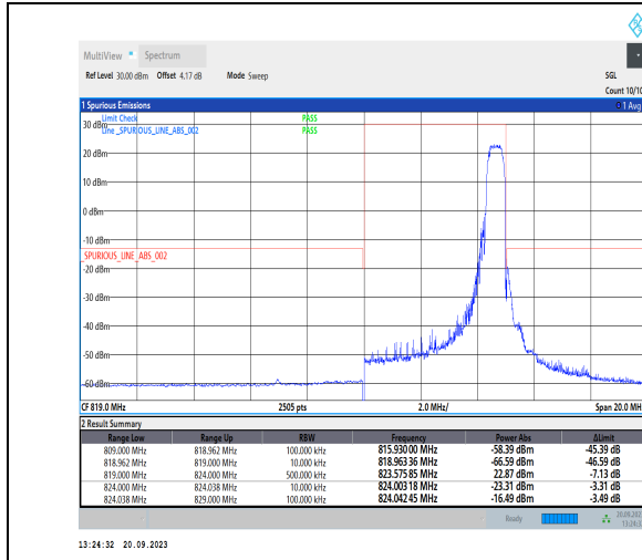
1-N26-814-824-PC3-15-5-H-2-DFT-PI2BPSK-Edge_1 RB_Right-1@24-Ant41-1--PASS-see graph
