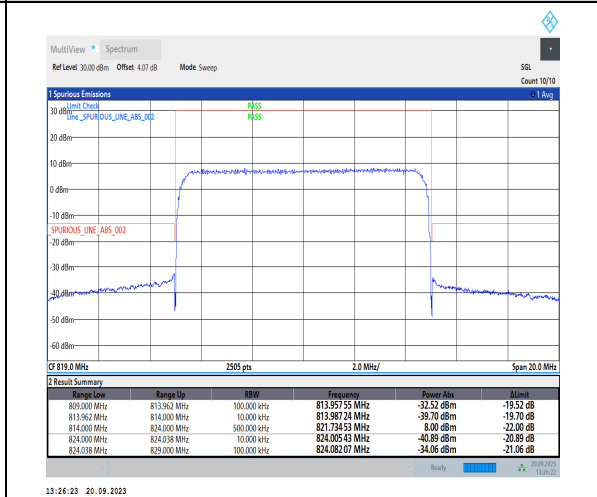
1-N26-814-824-PC3-15-10-L-6-CP-QPSK-Outer_Full-52@0-Ant41-1--PASS-see graph
