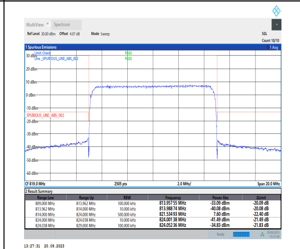
1-N26-814-824-PC3-15-10-H-6-CP-QPSK-Outer Full-52@0-Ant41-1--PASS-see graph
