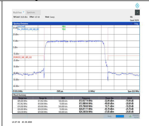
1-N26-814-824-PC3-15-10-H-3-DFT-PI2BPSK-Out er_Full-50@0-Ant41-1--PASS-see graph
