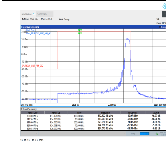
1-N26-814-824-PC3-15-10-H-5-CP-QPSK-Edge_1RB_Right-1@51-Ant41-1--PASS-see graph
