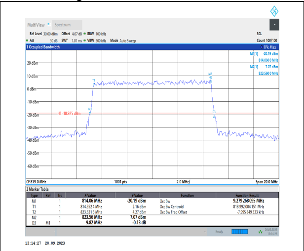
1-N26-814-824-PC3-15-10-M-9-CP-256QAM-Outer_F ull-52@0-Ant41-9.279-9.820-≤10-PASS
