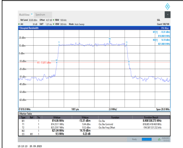
1-N26-814-824-PC3-15-10-M-2-DFT-PI2BPSK-Outer_F ull-50@0-Ant41-8.909-9.500-≤10-PASS
