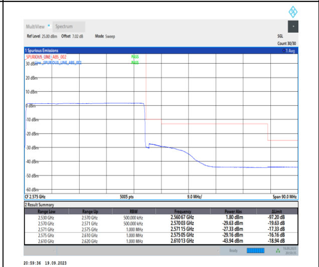
1-N7-PC3-15-40-H-6-CP-QPSK-Outer_Full-216@0-Ant31-1--PASS-see graph
