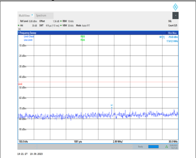
1-N7-PC3-15-40-H-1-DFT-PI2BPSK-Inner_1RB_Left- 1 @ 1-0.15-30-Ant31-17.61--70.63--45-PASS
