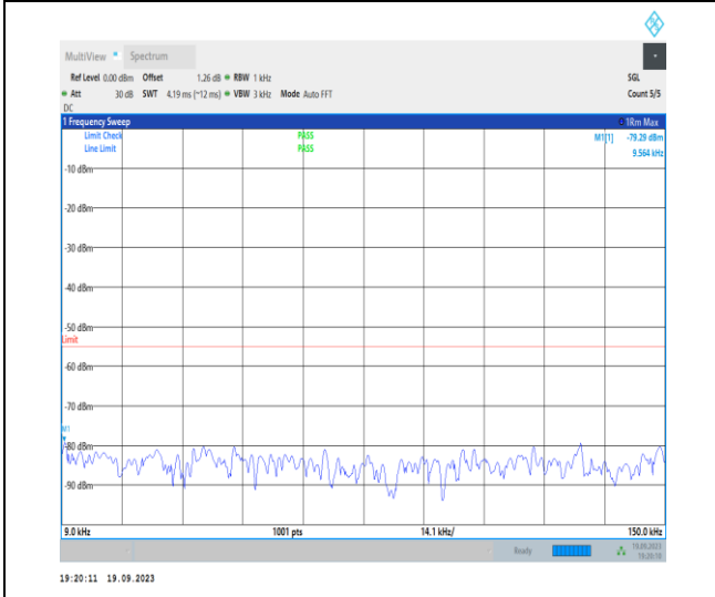
1-N7-PC3-15-40-M-1-DFT-PI2BPSK-Inner_1RB_Left -1 @ 1-0.009-0.15-Ant31-0.09--79.29--55-PASS
