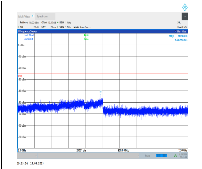
1-N7-PC3-15-40-L-1-DFT-PI2BPSK-Inner_1RB_Left -1 @ 1-3000-12000-Ant31-7405.05--43.92--25-PASS
