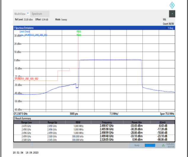
1-N7-PC3-15-30-L-6-CP-QPSK-Outer_Full-160 @0-Ant31-1--PASS-see graph
