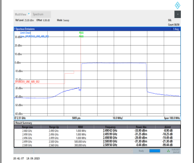
1-N7-PC3-15-40-L-6-CP-QPSK-Outer_Full-216 @0-Ant31-1--PASS-see graph
