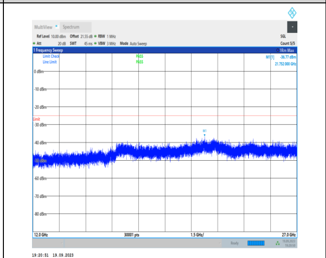
1-N7-PC3-15-40-M-1-DFT-PI2BPSK-Inner_1RB_Left-1 @ 1-12000-27000-Ant31-21752.00--36.77--25-PASS
