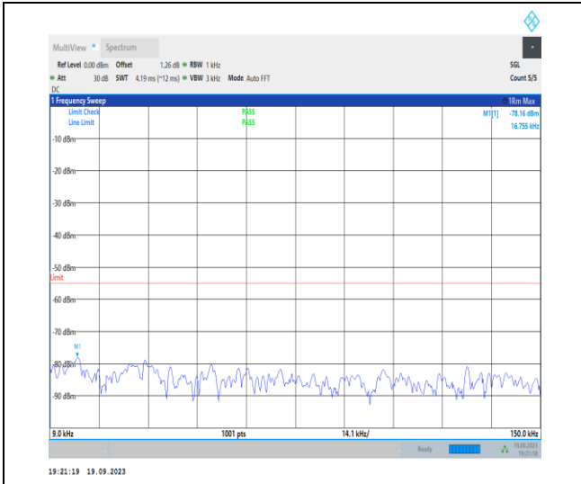
1-N7-PC3-15-40-H-1-DFT-PI2BPSK-Inner_1RB_Lef t-1 @ 1-0.009-0.15-Ant31-0.17--78.16--55-PASS
