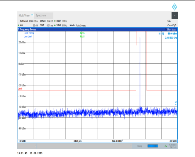
1-N7-PC3-15-40-H-1-DFT-PI2BPSK-Inner_1RB_Left- 1 @ 1-1000-3000-Ant31-2981.50--39.00--25-PASS
