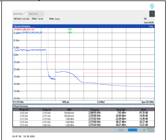
1-N7-PC3-15-5-H-3-DFT-PI2BPSK-Outer_Full-25 @0-Ant31-1--PASS-see graph
