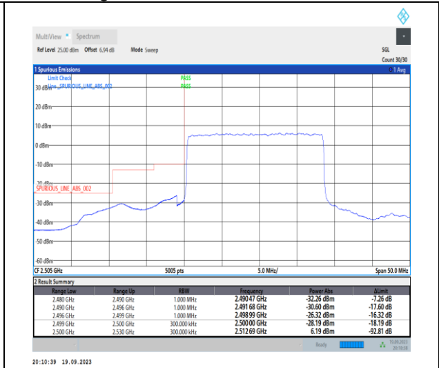
1-N7-PC3-15-20-L-3-DFT-PI2BPSK-Outer_Full-10 0@0-Ant31-1--PASS-see graph
