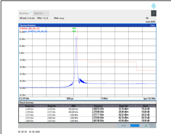
1-N7-PC3-15-30-H-2-DFT-PI2BPSK-Edge_1RB_Right-1@159-Ant31-1--PASS-see graph
