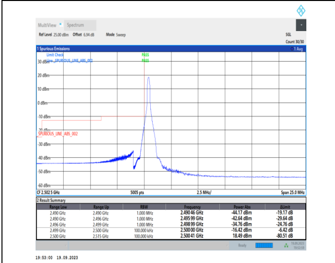
1-N7-PC3-15-10-L-4-CP-QPSK-Edge_1RB_Left-1 @0-Ant31-1--PASS-see graph
