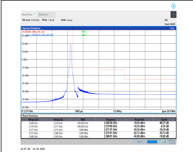
1-N7-PC3-15-10-H-5-CP-QPSK-Edge_1RB_Right-1@51-Ant31-1--PASS-see graph
