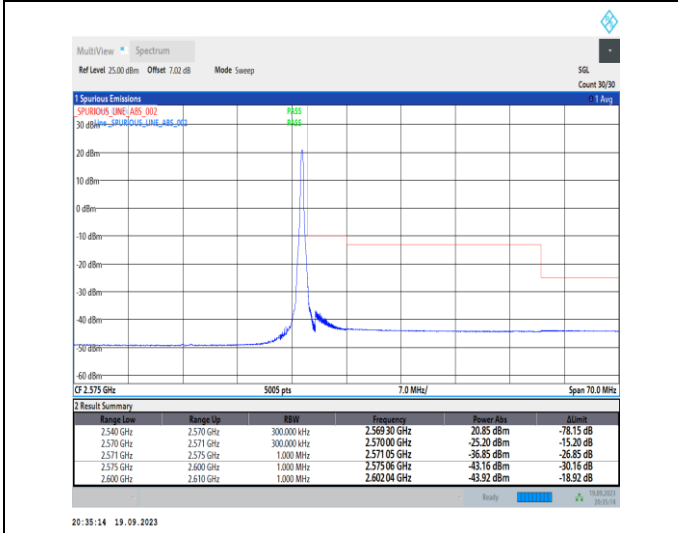
1-N7-PC3-15-30-H-5-CP-QPSK-Edge_1RB_Right-1@159-Ant31-1--PASS-see graph
