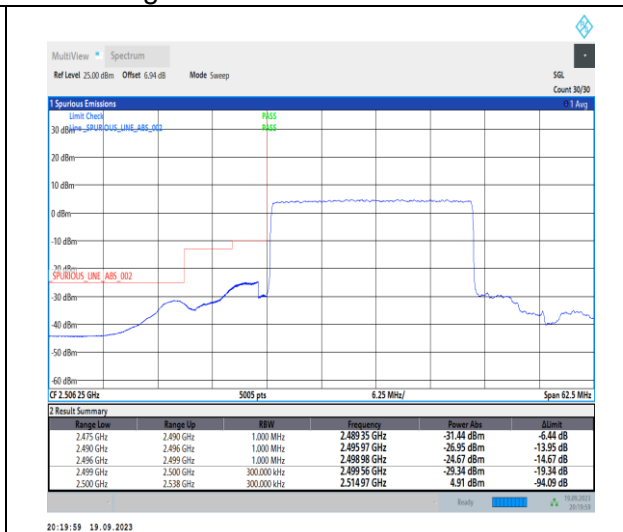
1-N7-PC3-15-25-L-3-DFT-PI2BPSK-Outer_Full-12 8@0-Ant31-1--PASS-see graph
