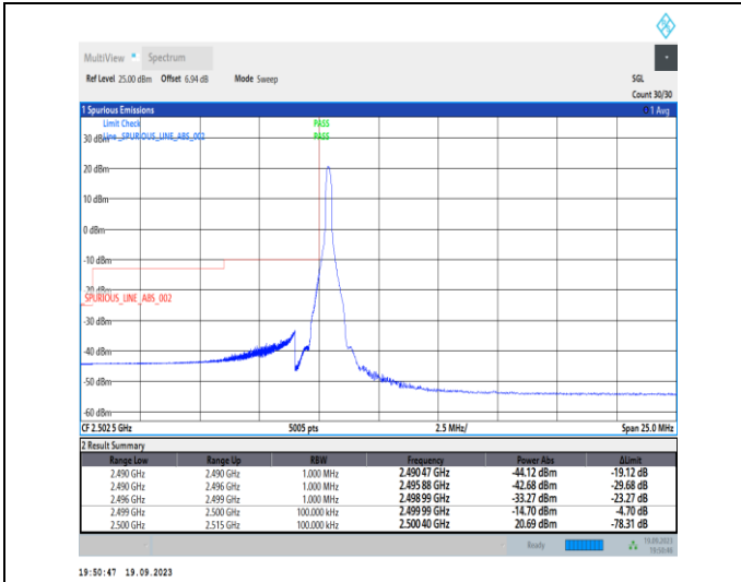
1-N7-PC3-15-10-L-1-DFT-PI2BPSK-Edge_1RB_Left-1 @0-Ant31-1--PASS-see graph
