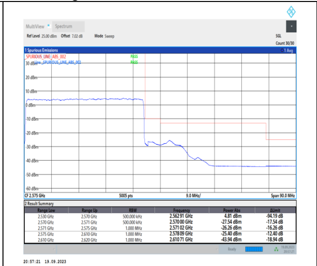
1-N7-PC3-15-40-H-3-DFT-PI2BPSK-Outer_Full-216@0-Ant31-1--PASS-see graph
