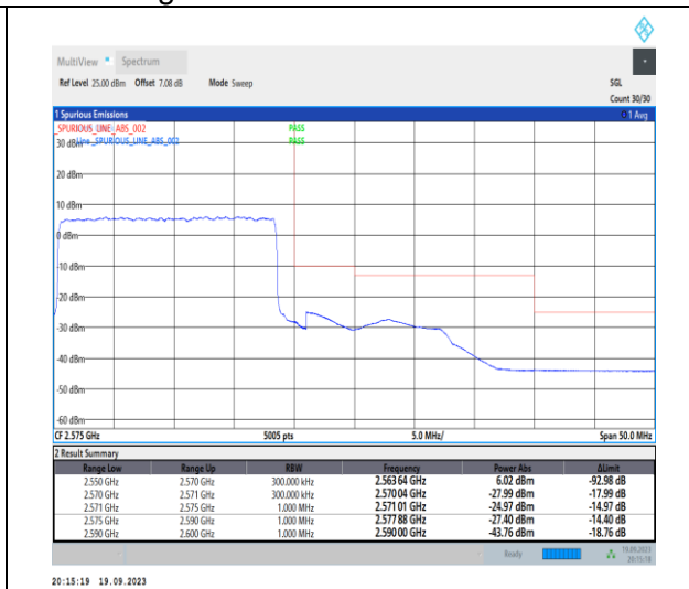
1-N7-PC3-15-20-H-3-DFT-PI2BPSK-Outer_Full-100@0-Ant31-1--PASS-see graph
