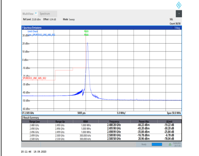
1-N7-PC3-15-20-L-4-CP-QPSK-Edge_1RB_Left-1 @0-Ant31-1--PASS-see graph
