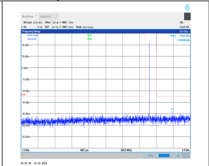
1-N7-PC3-15-40-M-1-DFT-PI2BPSK-Inner_1RB_Left-1 @ 1-1000-3000-Ant31-2785.00--39.42--25-PASS
