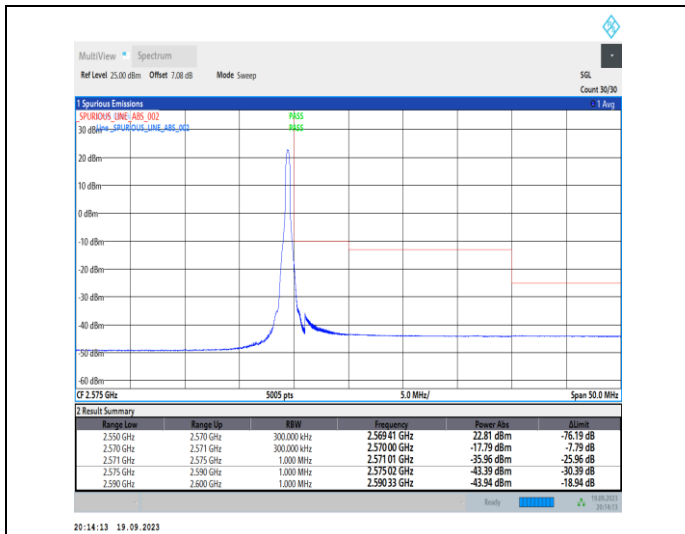
1-N7-PC3-15-20-H-2-DFT-PI2BPSK-Edge_1RB_Right-1@105-Ant31-1--PASS-see graph
