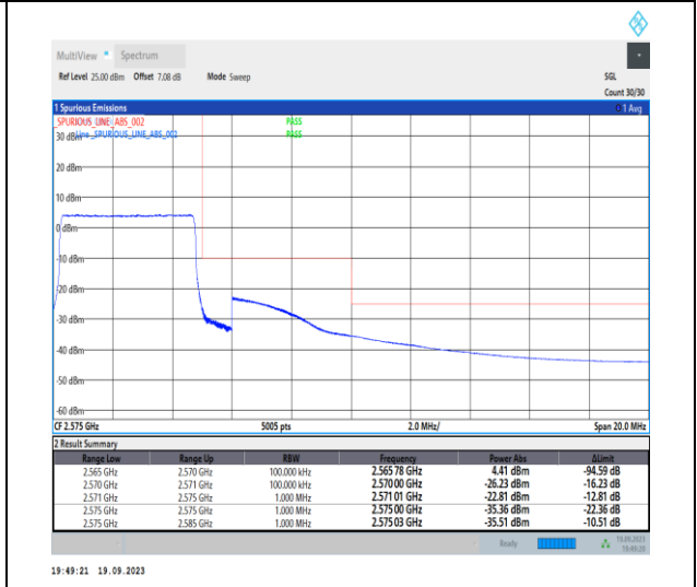
1-N7-PC3-15-5-H-6-CP-QPSK-Outer_Full-25 @0-Ant31-1--PASS-see graph
