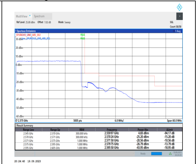
1-N7-PC3-15-25-H-3-DFT-PI2BPSK-Outer_Full-128@0-Ant31-1--PASS-see graph
