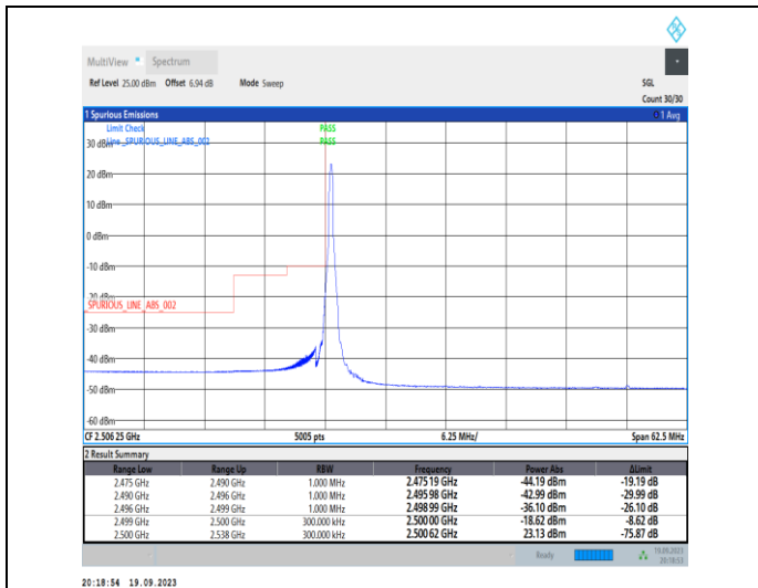
1-N7-PC3-15-25-L-1-DFT-PI2BPSK-Edge_1RB_Left-1 @0-Ant31-1--PASS-see graph
