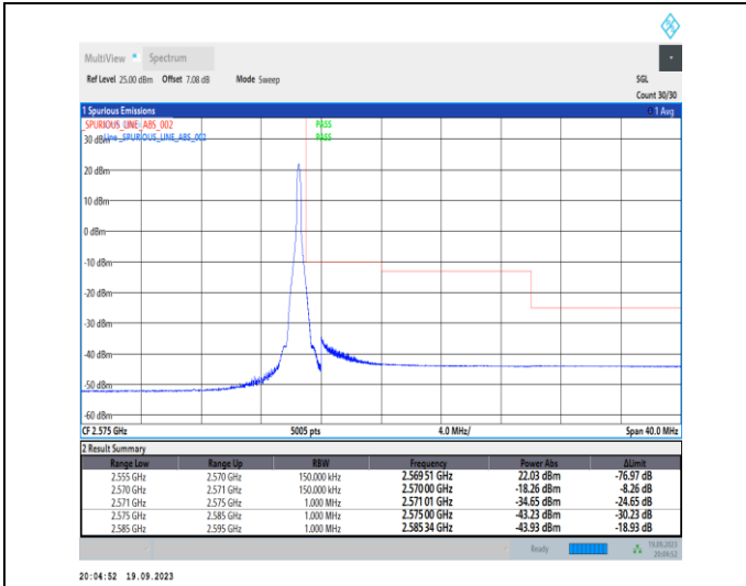
1-N7-PC3-15-15-H-2-DFT-PI2BPSK-Edge_1RB_Right-1@78-Ant31-1--PASS-see graph
