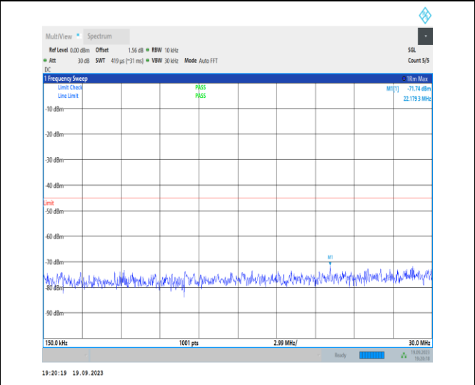
1-N7-PC3-15-40-M-1-DFT-PI2BPSK-Inner_1RB_Left -1 @ 1-0.15-30-Ant31-22.18--71.74--45-PASS
