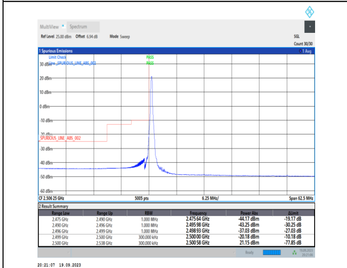
1-N7-PC3-15-25-L-4-CP-QPSK-Edge_1RB_Left-1 @0-Ant31-1--PASS-see graph
