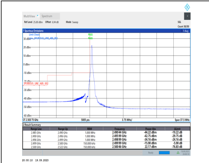
1-N7-PC3-15-15-L-1-DFT-PI2BPSK-Edge_1RB_Left-1 @0-Ant31-1--PASS-see graph
