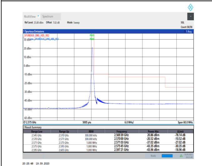
1-N7-PC3-15-25-H-5-CP-QPSK-Edge_1RB_Right-1@132-Ant31-1--PASS-see graph
