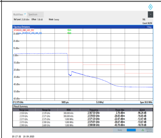
1-N7-PC3-15-20-H-6-CP-QPSK-Outer_Full-106@0-Ant31-1--PASS-see graph
