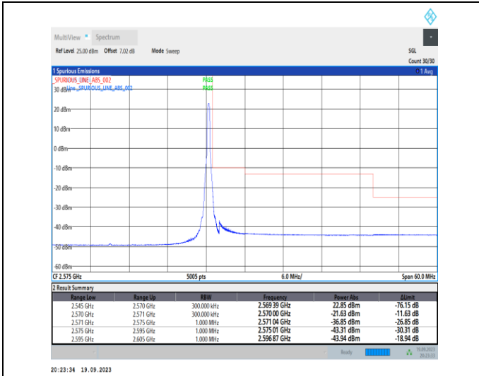
1-N7-PC3-15-25-H-2-DFT-PI2BPSK-Edge_1RB_Right-1@132-Ant31-1--PASS-see graph
