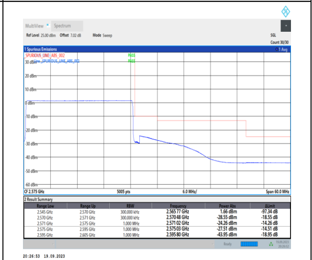
1-N7-PC3-15-25-H-6-CP-QPSK-Outer_Full-133@0-Ant31-1--PASS-see graph
