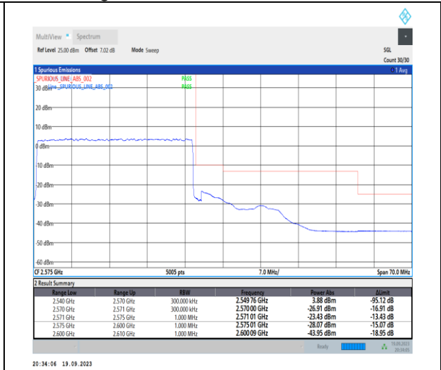
1-N7-PC3-15-30-H-3-DFT-PI2BPSK-Outer_Full-160@0-Ant31-1--PASS-see graph
