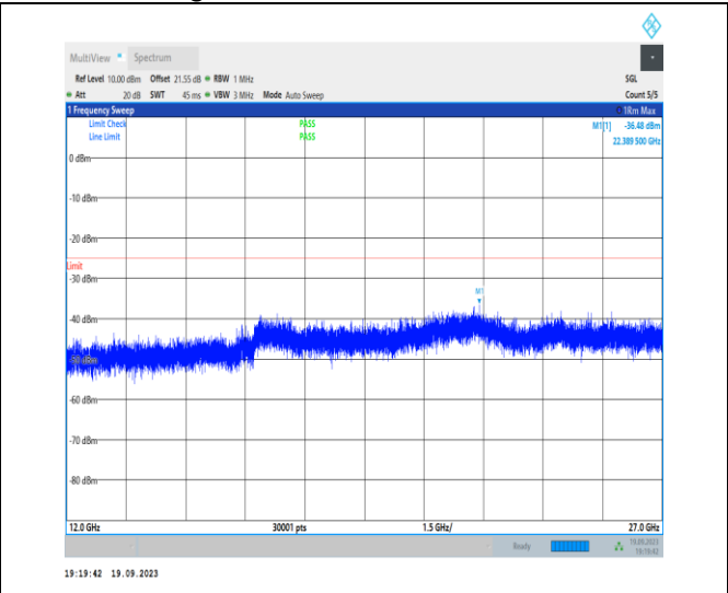
1-N7-PC3-15-40-L-1-DFT-PI2BPSK-Inner_1RB_Left -1 @ 1-12000-27000-Ant31-22389.50--36.48--25-PASS
