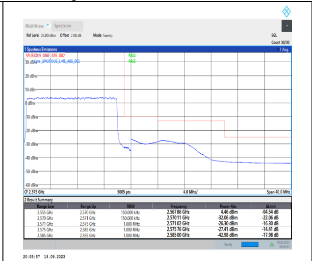
1-N7-PC3-15-15-H-3-DFT-PI2BPSK-Outer_Full-75@0-Ant31-1--PASS-see graph
