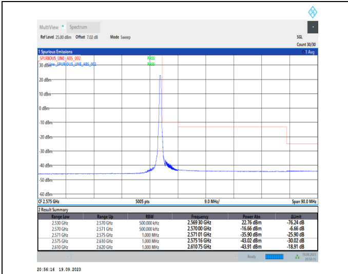
1-N7-PC3-15-40-H-2-DFT-PI2BPSK-Edge_1RB_Right-1@215-Ant31-1--PASS-see graph
