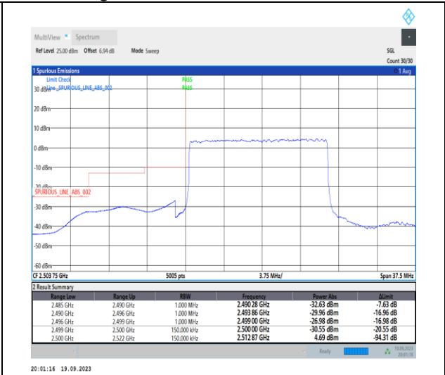
1-N7-PC3-15-15-L-3-DFT-PI2BPSK-Outer_Full-75 @0-Ant31-1--PASS-see graph
