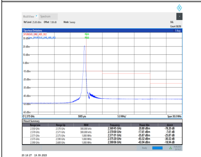
1-N7-PC3-15-20-H-5-CP-QPSK-Edge_1RB_Right-1@105-Ant31-1--PASS-see graph
