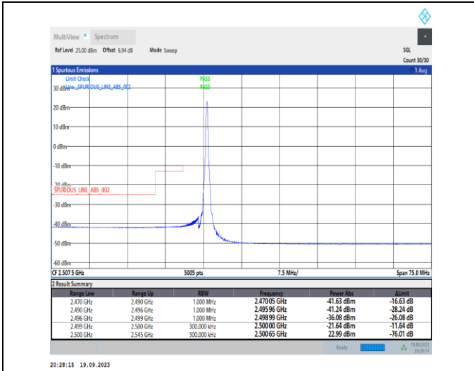
1-N7-PC3-15-30-L-1-DFT-PI2BPSK-Edge_1RB_Left-1 @0-Ant31-1--PASS-see graph
