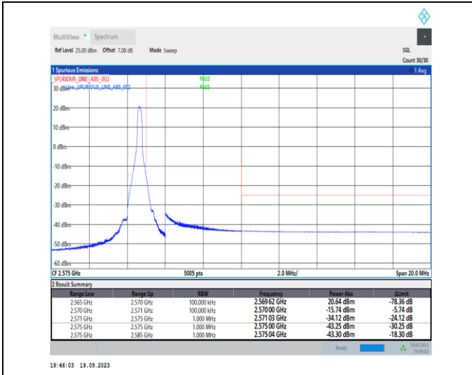
1-N7-PC3-15-5-H-2-DFT-PI2BPSK-Edge_1RB_Right-1 @24-Ant31-1--PASS-see graph
