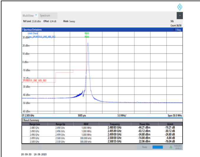
1-N7-PC3-15-20-L-1-DFT-PI2BPSK-Edge_1RB_Left-1 @0-Ant31-1--PASS-see graph
