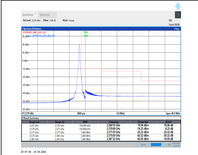
1-N7-PC3-15-15-H-5-CP-QPSK-Edge_1RB_Right-1@78-Ant31-1--PASS-see graph
