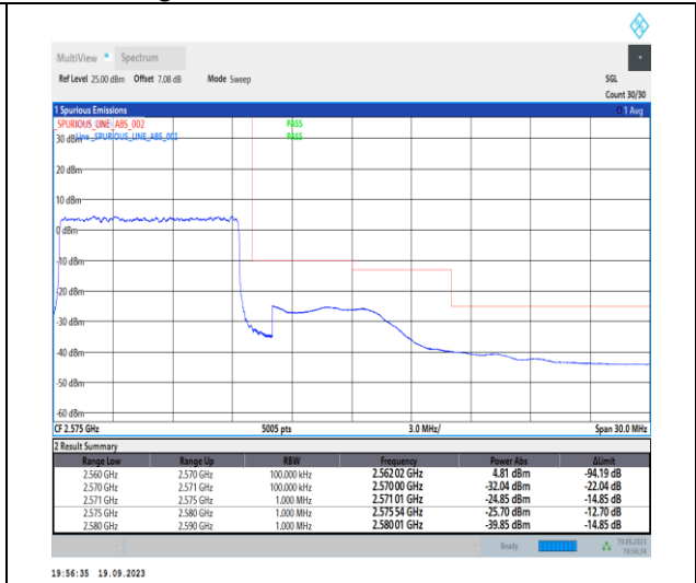
1-N7-PC3-15-10-H-3-DFT-PI2BPSK-Outer_Full-50@0-Ant31-1--PASS-see graph
