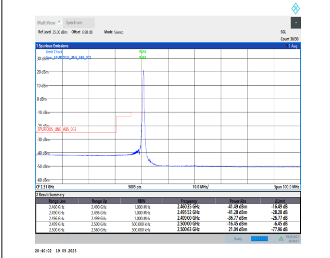
1-N7-PC3-15-40-L-4-CP-QPSK-Edge_1RB_Left-1 @0-Ant31-1--PASS-see graph
