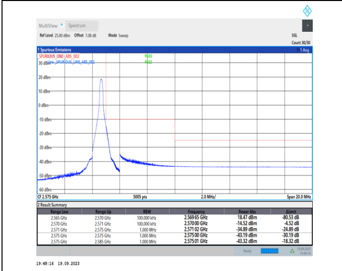
1-N7-PC3-15-5-H-5-CP-QPSK-Edge_1RB_Right-1 @2 4-Ant31-1--PASS-see graph
