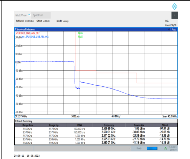
1-N7-PC3-15-15-H-6-CP-QPSK-Outer_Full-79@0-Ant31-1--PASS-see graph
