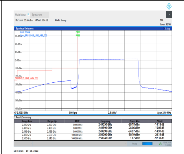
1-N7-PC3-15-10-L-6-CP-QPSK-Outer_Full-52 @0-Ant31-1--PASS-see graph
