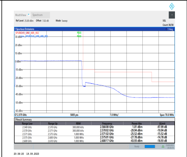
1-N7-PC3-15-30-H-6-CP-QPSK-Outer_Full-160@0-Ant31-1--PASS-see graph
