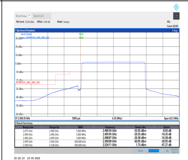
1-N7-PC3-15-25-L-6-CP-QPSK-Outer_Full-133 @0-Ant31-1--PASS-see graph
