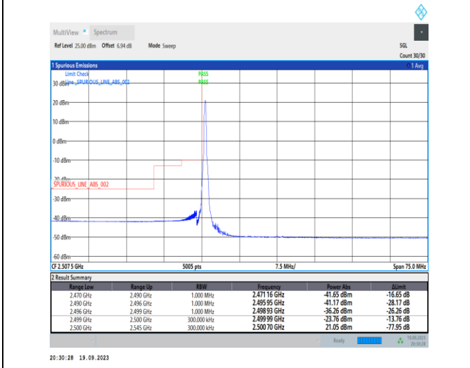
1-N7-PC3-15-30-L-4-CP-QPSK-Edge_1RB_Left-1 @0-Ant31-1--PASS-see graph
