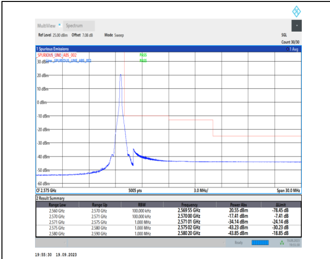
1-N7-PC3-15-10-H-2-DFT-PI2BPSK-Edge_1RB_Right-1@51-Ant31-1--PASS-see graph
