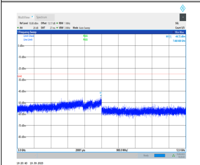
1-N7-PC3-15-40-M-1-DFT-PI2BPSK-Inner_1RB_Lef t-1 @ 1-3000-12000-Ant317460.40--44.72--25-PASS
