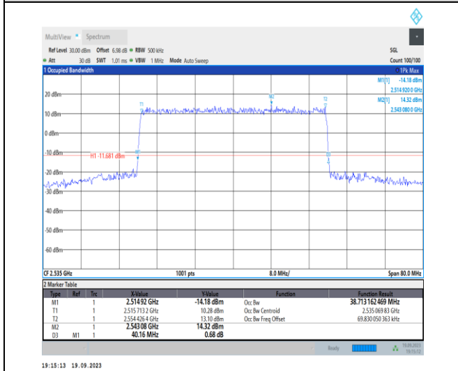
1-N7-PC3-15-40-M-1-DFT-QPSK-Outer_Full-216@0 -Ant31-38.713-40.160-≤40-PASS
