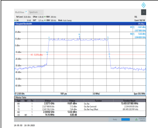
1-N7-PC3-15-15-M-5-DFT-256QAM-Outer_Full-75@0 -Ant31-13.435-14.160-≤15-PASS
