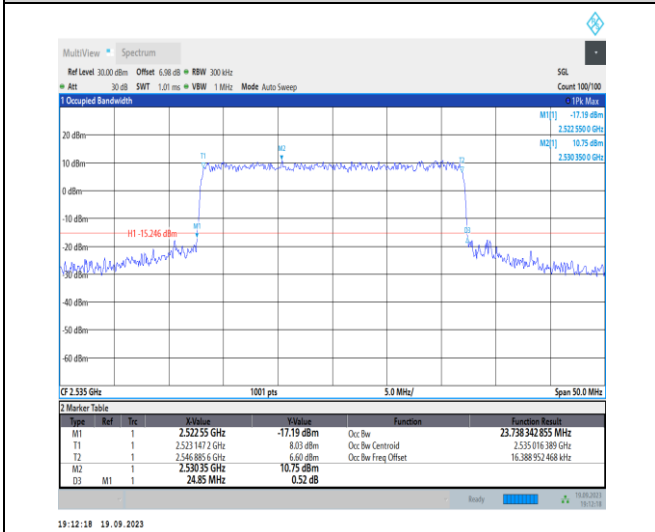
1-N7-PC3-15-25-M-7-CP-16QAM-Outer_Full-133@0 -Ant31-23.738-24.850-≤25-PASS
