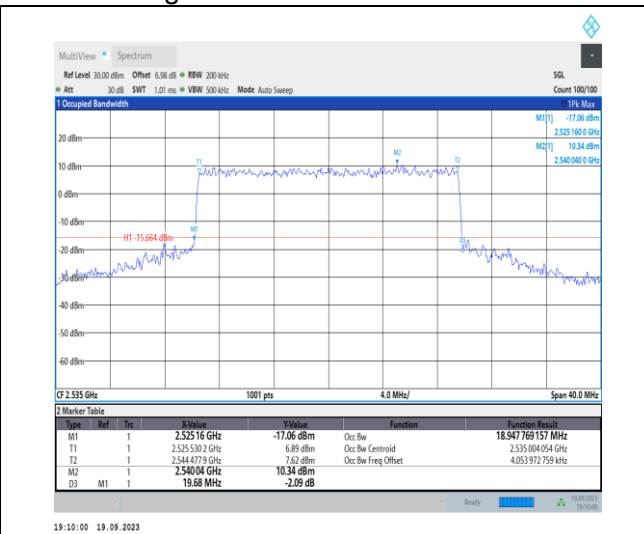
1-N7-PC3-15-20-M-7-CP-16QAM-Outer_Full-106@0-Ant31-18.948-19.680-≤20-PASS
