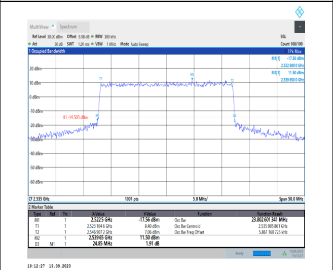
1-N7-PC3-15-25-M-8-CP-64QAM-Outer_Full-133@0 -Ant31-23.803-24.850-≤25-PASS
