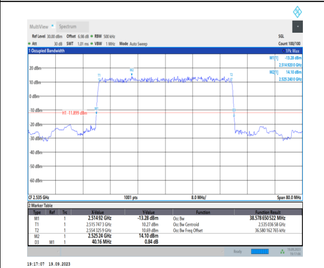
1-N7-PC3-15-40-M-2-DFT-PI2BPSK-Outer_Full-216@0 -Ant31-38.579-40.160-≤40-PASS
