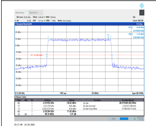
1-N7-PC3-15-40-M-5-DFT-256QAM-Outer_Full-216 @0-Ant31-38.52-40.160-≤40-PASS
