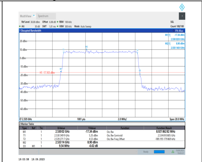
1-N7-PC3-15-10-M-5-DFT-256QAM-Outer_Full-50@0-Ant31-8.922-9.540-≤10-PASS
