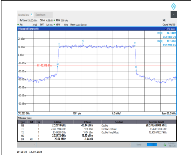
1-N7-PC3-15-30-M-2-DFT-PI2BPSK-Outer_Full-160 @0-Ant31-28.57-29.640-≤30-PASS
