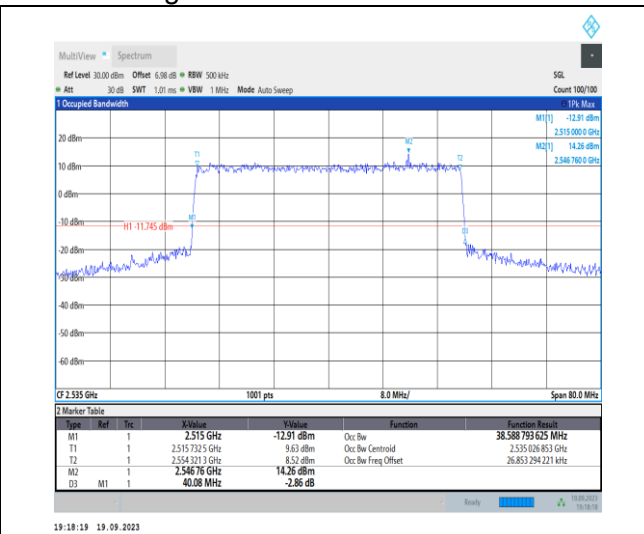
1-N7-PC3-15-40-M-8-CP-64QAM-Outer_Full-216@0 -Ant31-38.589-40.080-≤40-PASS
