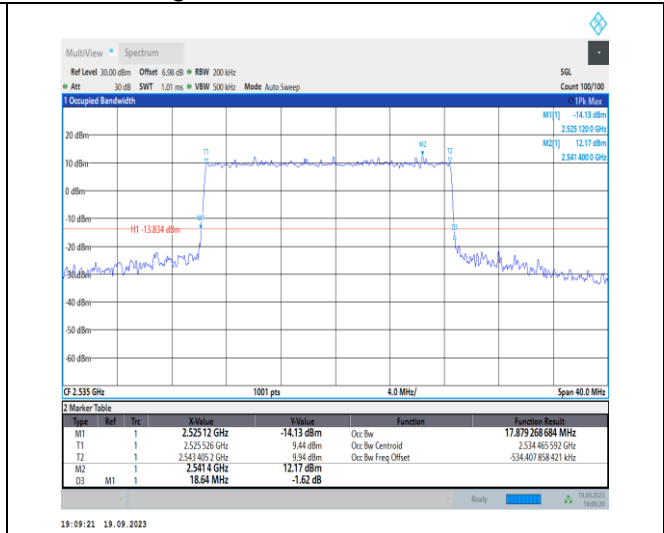
1-N7-PC3-15-20-M-3-DFT-16QAM-Outer_Full-100 @0-Ant31-17.879-18.640-≤20-PASS
