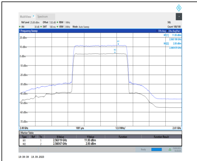
1-N7-PC3-15-40-H-1-DFT-256QAM-Outer_Full-216 @0-Ant31-9.00-100%-0.00-9.00-PASS-≤13
