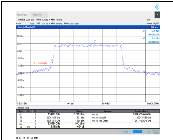
1-N7-PC3-15-10-M-8-CP-64QAM-Outer_Full-52@0-Ant31-9.299-9.880-≤10-PASS
