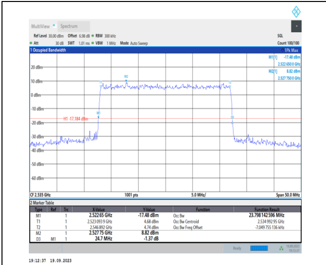
1-N7-PC3-15-25-M-9-CP-256QAM-Outer_Full-133@ 0-Ant31-23.798-24.700-≤25-PASS
