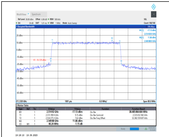
1-N7-PC3-15-40-M-7-CP-16QAM-Outer_Full-216@0 -Ant31-38.486-40.240-≤40-PASS
