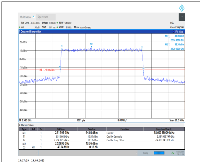
1-N7-PC3-15-40-M-3-DFT-16QAM-Outer_Full-216@ 0-Ant31-38.608-40.240-≤40-PASS
