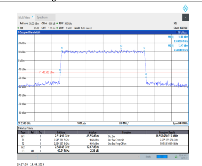
1-N7-PC3-15-40-M-4-DFT-64QAM-Outer_Full-216@ 0-Ant31-38.556-40.240-≤40-PASS
