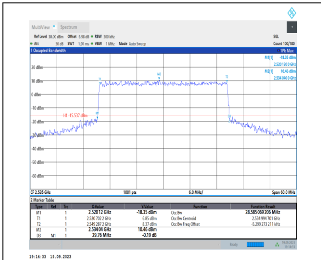
1-N7-PC3-15-30-M-8-CP-64QAM-Outer_Full-160@0 -Ant31-28.585-29.760-≤30-PASS
