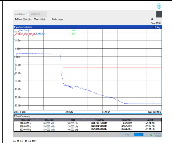
1-N5-PC3-15-5-H-6-CP-QPSK-Outer_Full-25@0-Ant41-1--PASS-see graph
