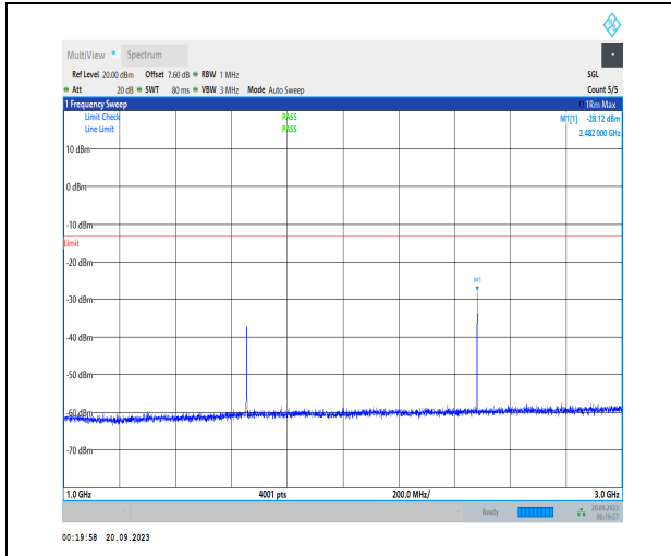
1-N5-PC3-15-20-M-1-DFT-PI2BPSK-Inner_1RB_Left -1@1-1000-3000-Ant41-2482.00--28.12--13-PASS
