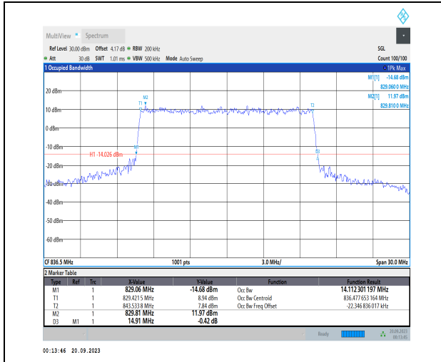
1-N5-PC3-15-15-M-7-CP-16QAM-Outer_Full-79@0- -Ant41-14.112-14.910-≤15-PASS
