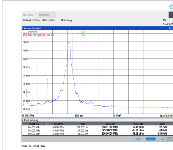
1-N5-PC3-15-5-H-2-DFT-PI2BPSK-Edge_1RB_Right-1 @24-Ant41-1--PASS-see graph
