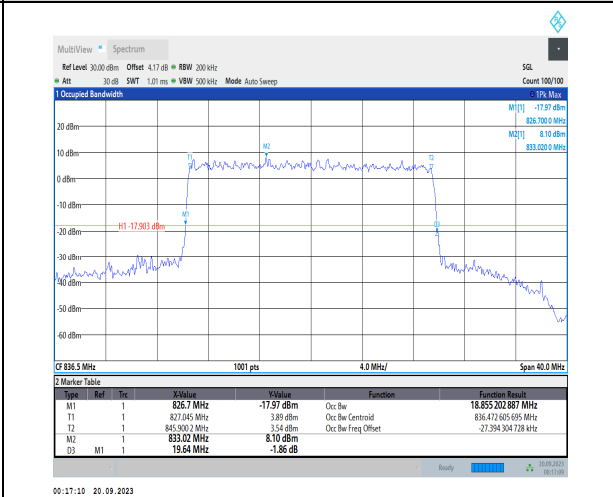
1-N5-PC3-15-20-M-9-CP-256QAM-Outer_Full-106@0-Ant41-18.855-19.640-≤20-PASS
