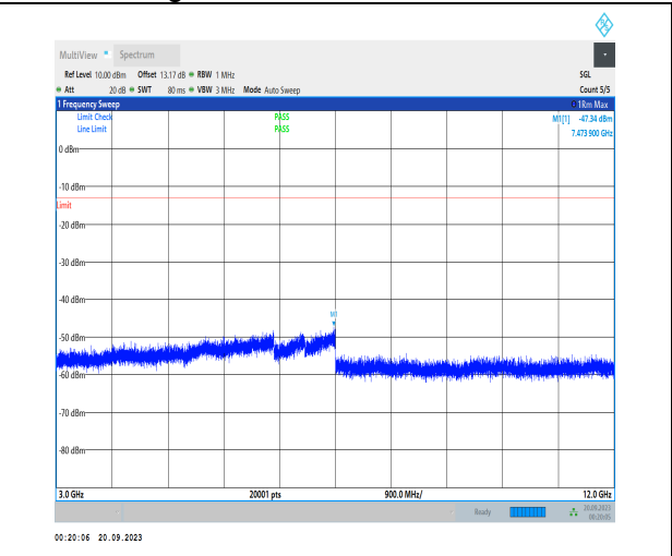
1-N5-PC3-15-20-M-1-DFT-PI2BPSK-Inner_1RB_Left -1@1-3000-12000-Ant41-7473.90--47.34--13-PASS
