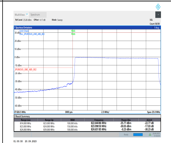
1-N5-PC3-15-15-L-6-CP-QPSK-Outer_Full-79@0-Ant41-1--PASS-see graph
