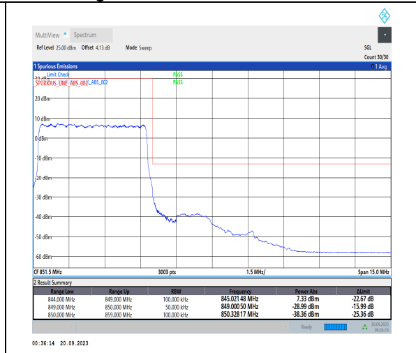
1-N5-PC3-15-5-H-3-DFT-PI2BPSK-Outer_Full-25 @0-Ant41-1--PASS-see graph
