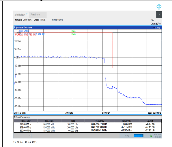
1-N5-PC3-15-20-H-3-DFT-PI2BPSK-Outer_Full-100@0-Ant41-1--PASS-see graph
