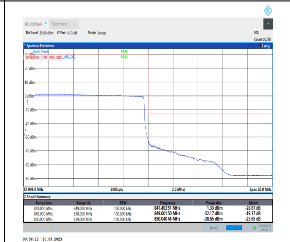
1-N5-PC3-15-10-H-6-CP-QPSK-Outer_Full-52@0-Ant41-1--PASS-see graph
