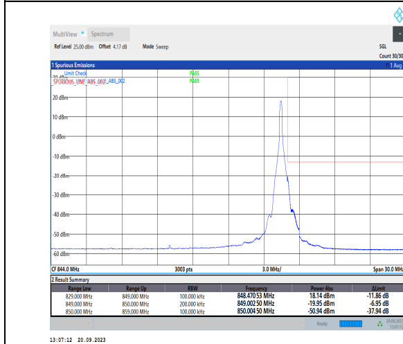
1-N5-PC3-15-20-H-5-CP-QPSK-Edge_1RB_Right-1@105-Ant41-1--PASS-see graph
