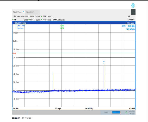
1-N5-PC3-15-20-H-1-DFT-PI2BPSK-Inner_1RB_Left -1@1-1000-3000-Ant41-2489.00--28.31--13-PASS
