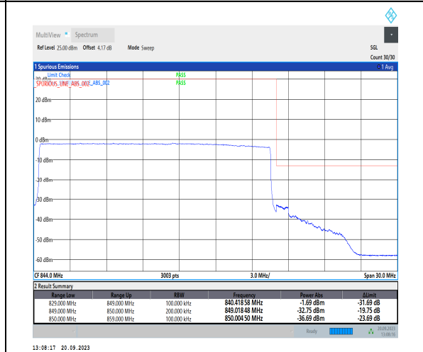
1-N5-PC3-15-20-H-6-CP-QPSK-Outer_Full-106@0-Ant41-1--PASS-see graph
