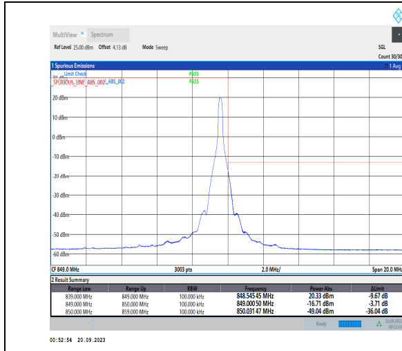
1-N5-PC3-15-10-H-2-DFT-PI2BPSK-Edge_1RB_Right-1@51-Ant41-1--PASS-see graph
