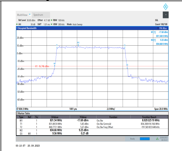
1-N5-PC3-15-10-M-5-DFT-256QAM-Outer_Full-50@0-Ant41-8.929-9.560-≤10-PASS
