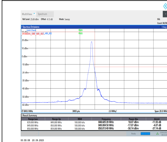
1-N5-PC3-15-10-H-5-CP-QPSK-Edge_1RB_Right-1@51-Ant41-1--PASS-see graph
