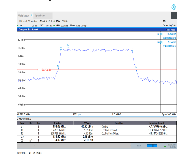
1-N5-PC3-15-5-M-6-CP-QPSK-Outer_Full-25@0-An t41-4.475-4.890-≤5-PASS
