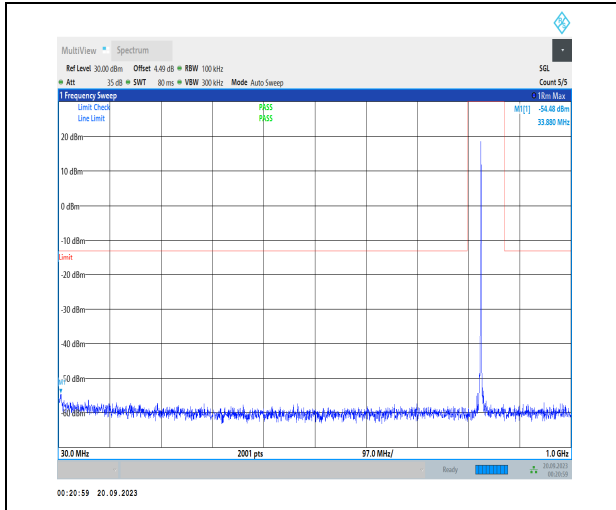
1-N5-PC3-15-20-H-1-DFT-PI2BPSK-Inner_1RB_Left -1@1-30-1000-Ant41-33.88--54.48--13-PASS
