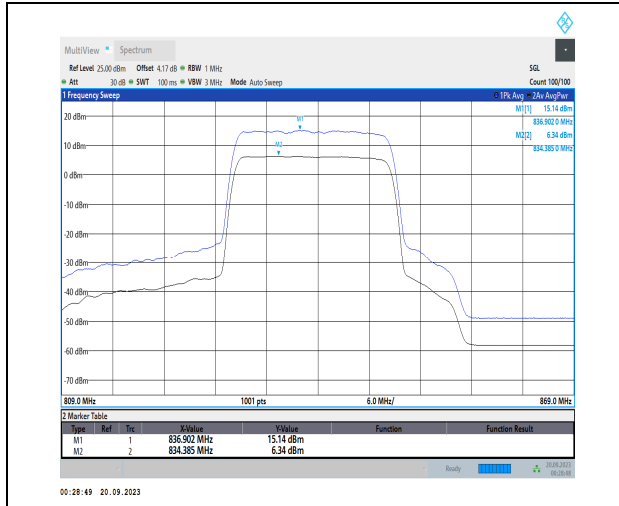
1-N5-PC3-15-20-H-1-DFT-256QAM-Outer_Full-100 @0-Ant41-8.80-100%-0.00-8.80-PASS<=13
