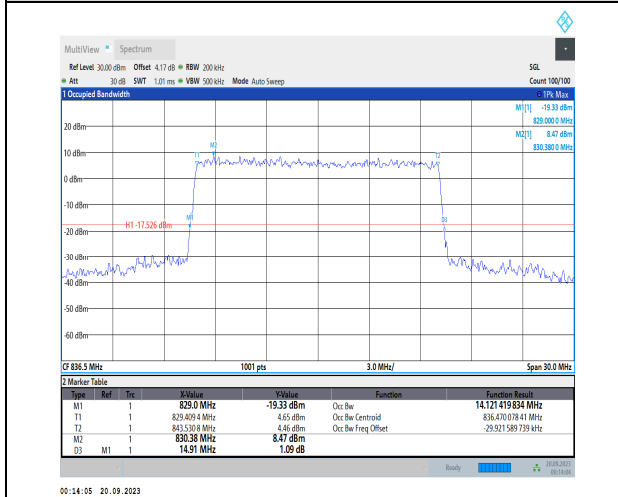
1-N5-PC3-15-15-M-9-CP-256QAM-Outer_Full-79@0- -Ant41-14.121-14.910-≤15-PASS
