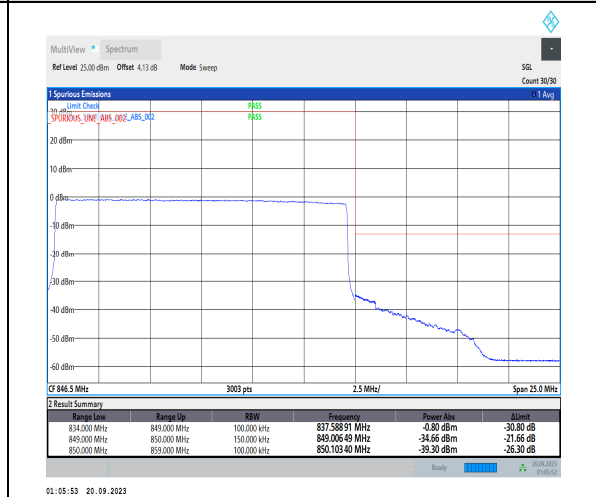
1-N5-PC3-15-15-H-6-CP-QPSK-Outer_Full-79@0-Ant41-1--PASS-see graph
