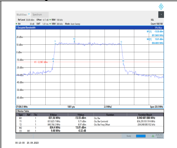
1-N5-PC3-15-10-M-1-DFT-QPSK-Outer_Full-50@0-Ant41-8.94-9.480-≤10-PASS
