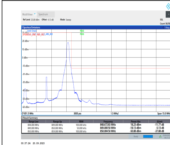
1-N5-PC3-15-5-H-5-CP-QPSK-Edge_1RB_Right-1@2 4-Ant41-1--PASS-see graph
