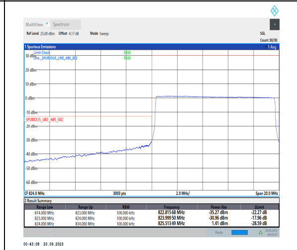
1-N5-PC3-15-10-L-6-CP-QPSK-Outer_Full-52@0-Ant41-1--PASS-see graph
