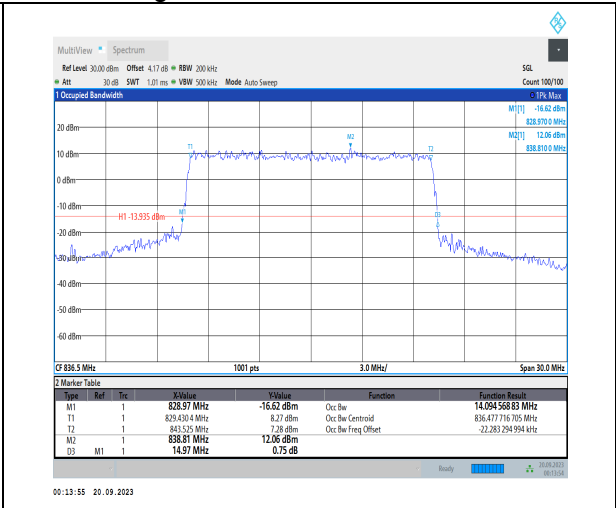
1-N5-PC3-15-15-M-8-CP-64QAM-Outer_Full-79@0- -Ant41-14.095-14.970-≤15-PASS
