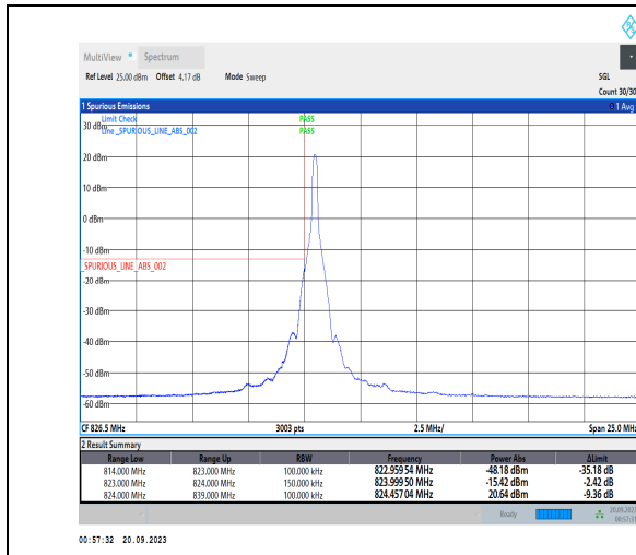
1-N5-PC3-15-15-L-1-DFT-PI2BPSK-Edge_1RB_Left-1 @0-Ant41-1--PASS-see graph
