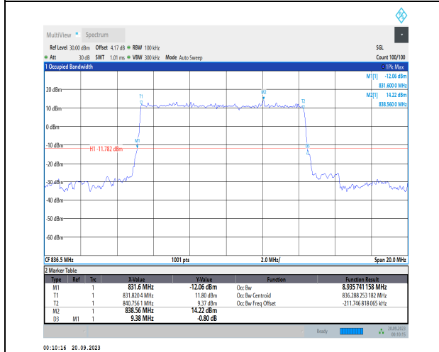
1-N5-PC3-15-10-M-2-DFT-PI2BPSK-Outer_Full-50@0-Ant41-8.936-9.380-≤10-PASS
