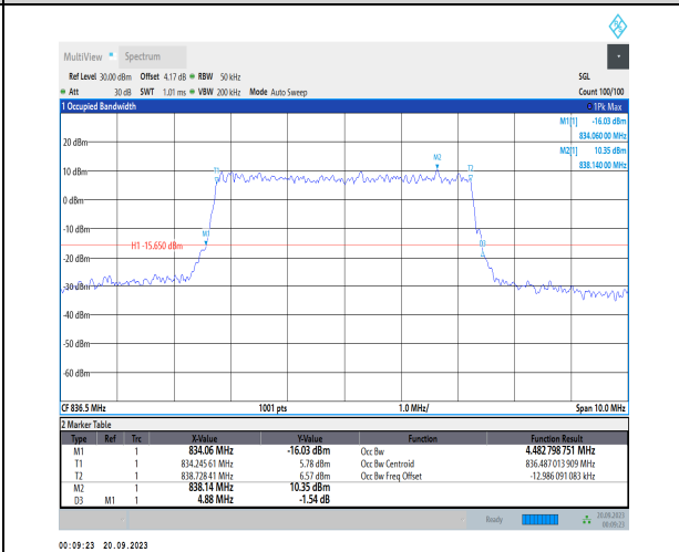
1-N5-PC3-15-5-M-8-CP-64QAM-Outer_Full-25@0-A nt41-4.483-4.880-≤5-PASS
