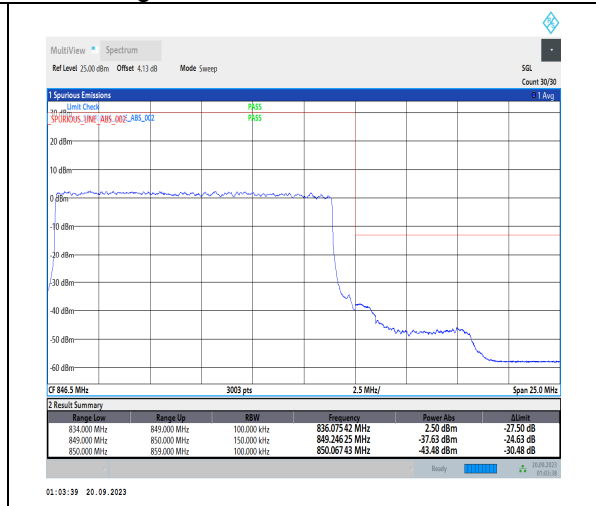
1-N5-PC3-15-15-H-3-DFT-PI2BPSK-Outer_Full-75@0-Ant41-1--PASS-see graph
