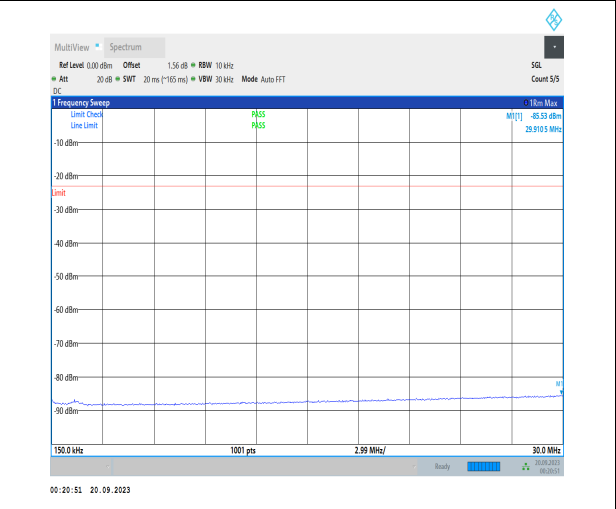
1-N5-PC3-15-20-H-1-DFT-PI2BPSK-Inner_1RB_Left -1@1-0.15-30-Ant41-29.91--85.53--23-PASS
