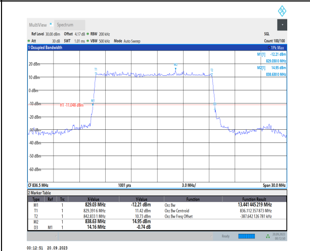
1-N5-PC3-15-15-M-2-DFT-PI2BPSK-Outer_Full-75@0-Ant41-13.441-14.160-≤15-PASS
