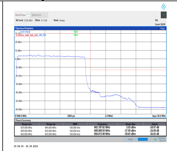
1-N5-PC3-15-10-H-3-DFT-PI2BPSK-Outer_Full-50@0-Ant41-1--PASS-see graph
