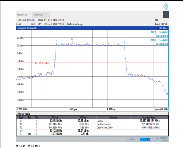
1-N5-PC3-15-20-M-1-DFT-QPSK-Outer_Full-100@0- -Ant41-17.857-18.720-≤20-PASS
