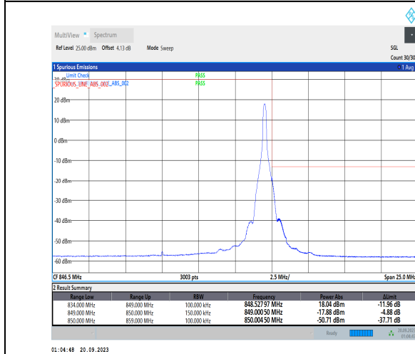
1-N5-PC3-15-15-H-5-CP-QPSK-Edge_1RB_Right-1@78-Ant41-1--PASS-see graph
