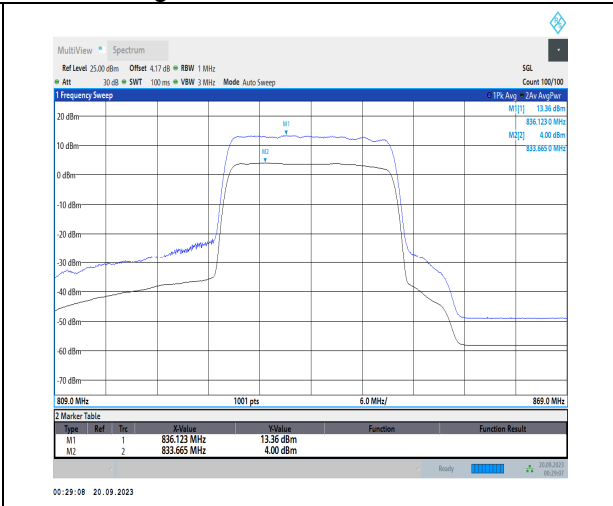
1-N5-PC3-15-20-H-2-CP-256QAM-Outer_Full-106@ 0-Ant41-9.36-100%-0.00-9.36-PASS<=13
