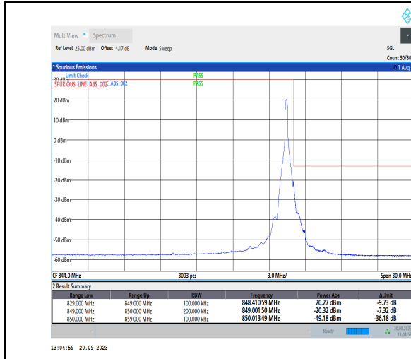
1-N5-PC3-15-20-H-2-DFT-PI2BPSK-Edge_1RB_Right-1@105-Ant41-1--PASS-see graph
