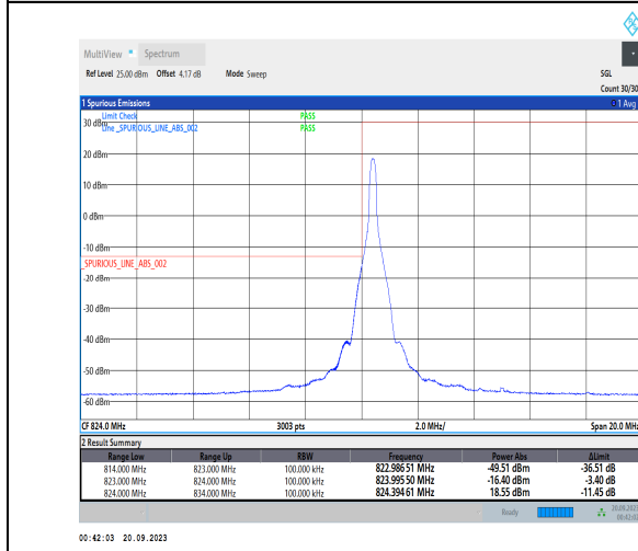
1-N5-PC3-15-10-L-4-CP-QPSK-Edge_1RB_Left-1@0-Ant41-1--PASS-see graph
