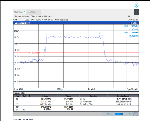
1-N5-PC3-15-10-M-3-DFT-16QAM-Outer_Full-50@0-Ant41-8.957-9.500-≤10-PASS
