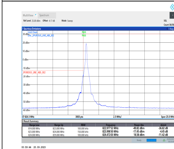
1-N5-PC3-15-15-L-4-CP-QPSK-Edge_1RB_Left-1@0-Ant41-1--PASS-see graph
