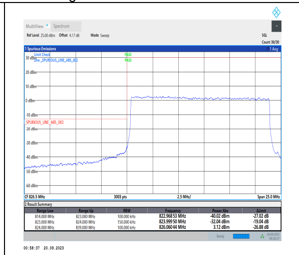
1-N5-PC3-15-15-L-3-DFT-PI2BPSK-Outer_Full-75 @0-Ant41-1--PASS-see graph
