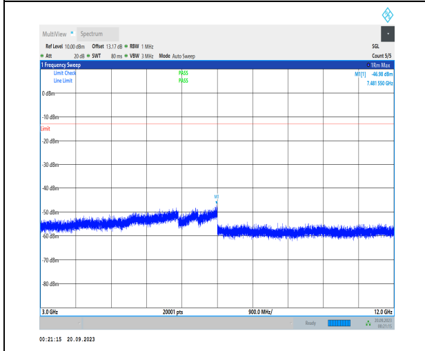
1-N5-PC3-15-20-H-1-DFT-PI2BPSK-Inner_1RB_Left -1@1-3000-12000-Ant41-7481.55--46.98--13-PASS
