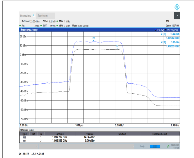
1-N2-PC3-15-20-H-1-DFT-256QAM-Outer_Full-100 @0-Ant31-8.66-100%-0.00-8.66-PASS<13
