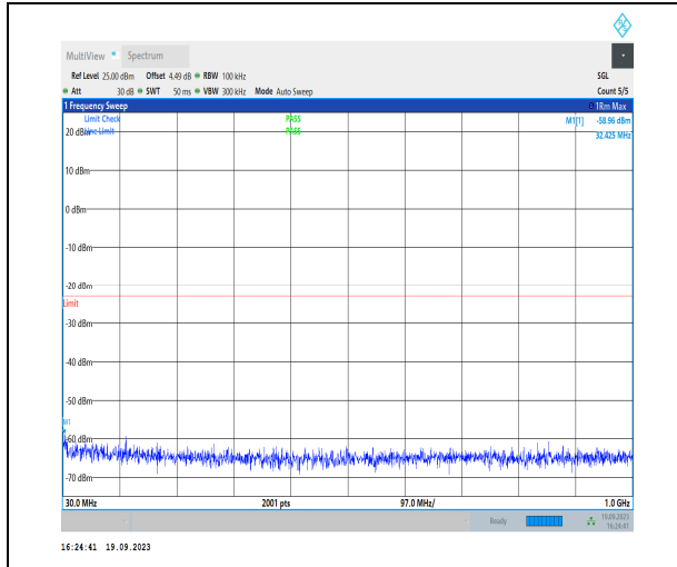
1-N2-PC3-15-20-M-1-N/A-DFT-PI2BPSK-Inner_1RB_Left-1@1-30-1000-Ant31-32.43--58.96--23-PASS
