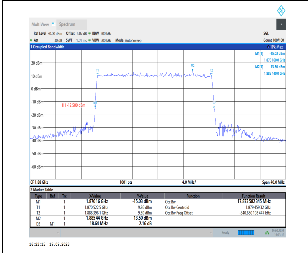
1-N2-PC3-15-20-M-4-DFT-64QAM-Outer_Full-100@ 0-Ant31-17.874-18.640-≤20-PASS
