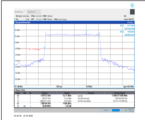
1-N2-PC3-15-20-M-2-DFT-PI2BPSK-Outer_Full-100 @0-Ant31-17.865-18.680-≤20-PASS
