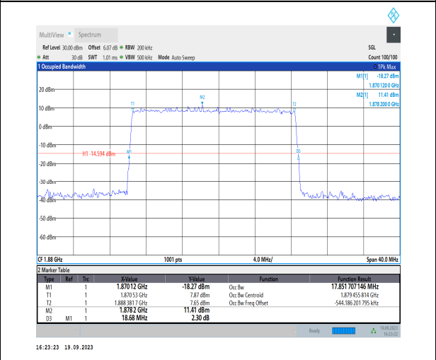
1-N2-PC3-15-20-M-5-DFT-256QAM-Outer_Full-100 @0-Ant31-17.852-18.680-≤20-PASS
