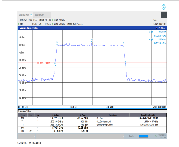
1-N2-PC3-15-15-M-5-DFT-256QAM-Outer_Full-75@0-Ant31-13.436-14.190-≤15-PASS
