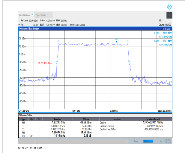
1-N2-PC3-15-15-M-3-DFT-16QAM-Outer_Full-75@0 -Ant31-13.456-14.160-≤15-PASS
