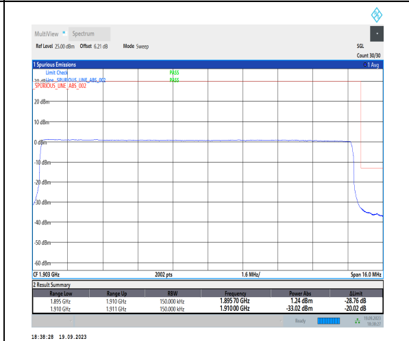
1-N2-PC3-15-15-H-6-CP-QPSK-Outer_Full-79@0-Ant31-1-seegraph-PASS-see graph
