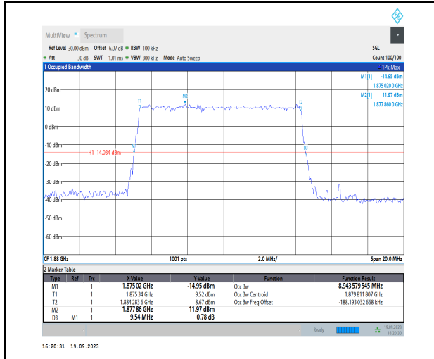
1-N2-PC3-15-10-M-4-DFT-64QAM-Outer_Full-50@0-Ant31-8.944-9.540-≤10-PASS
