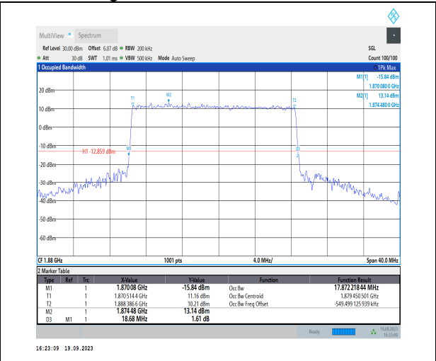
1-N2-PC3-15-20-M-3-DFT-16QAM-Outer_Full-100@ 0-Ant31-17.872-18.680-≤20-PASS
