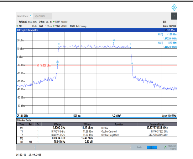
1-N2-PC3-15-20-M-1-DFT-QPSK-Outer_Full-100@0-Ant31-17.877-18.640-≤20-PASS
