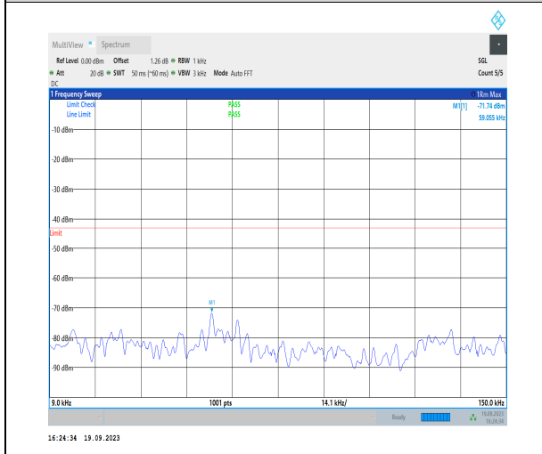
1-N2-PC3-15-20-M-1-N/A-DFT-PI2BPSK-Inner_1RB _Left-1@1-0.009-0.15-Ant31-0.06--71.74--43-PASS
