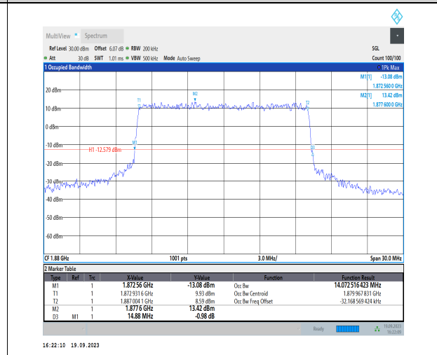
1-N2-PC3-15-15-M-6-CP-QPSK-Outer_Full-79@0-Ant31-14.073-14.880-≤15-PASS
