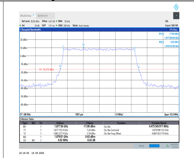
1-N2-PC3-15-5-M-6-CP-QPSK-Outer_Full-25@0-An t31-4.476-4.920-<math>\leq 5</math>-PASS
