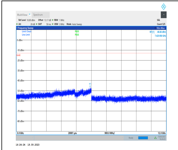
1-N2-PC3-15-20-L-1-N/A-DFT-PI2BPSK-Inner_1RB _Left-1@1-3000-12000-Ant31-7423.05--46.66--13-P ASS
