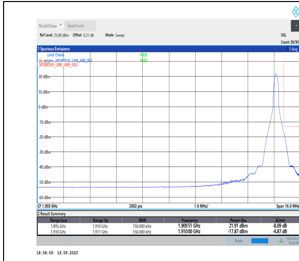
1-N2-PC3-15-15-H-2-DFT-PI2BPSK-Edge_1RB_Right-1@78-Ant31-1-seegraph-PASS-see graph
