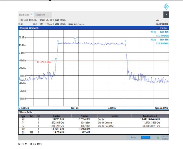
1-N2-PC3-15-15-M-4-DFT-64QAM-Outer_Full-75@0 -Ant31-13.431-14.220-≤15-PASS
