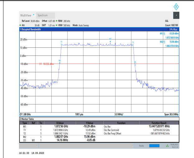
1-N2-PC3-15-15-M-2-DFT-PI2BPSK-Outer_Full-75@0-Ant31-13.448-14.160-≤15-PASS
