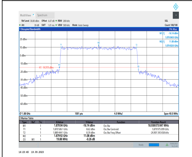
1-N2-PC3-15-20-M-8-CP-64QAM-Outer_Full-106@0-Ant31-18.938-19.880-≤20-PASS
