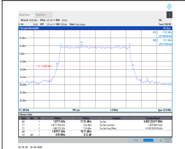
1-N2-PC3-15-5-M-7-CP-16QAM-Outer_Full-25@0-A nt31-4.492-4.950-<math>\leq 5</math>-PASS
