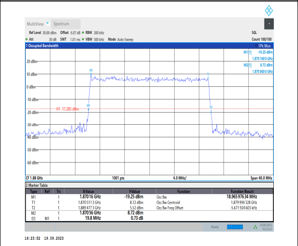
1-N2-PC3-15-20-M-9-CP-256QAM-Outer_Full-106@0-Ant31-18.966-19.800-≤20-PASS
