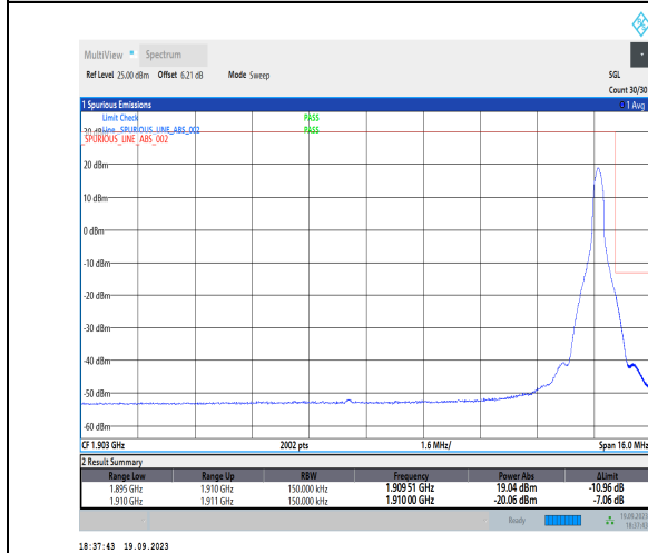
1-N2-PC3-15-15-H-5-CP-QPSK-Edge_1RB_Right-1@78-Ant31-1-seegraph-PASS-see graph
